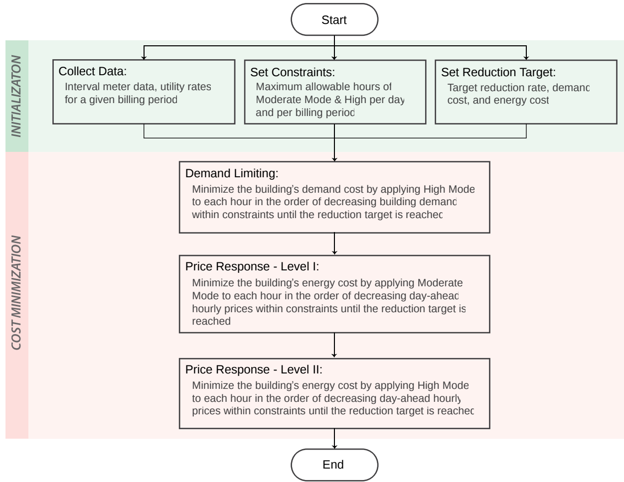
Figure 3. Cost Minimization Flow Chart
