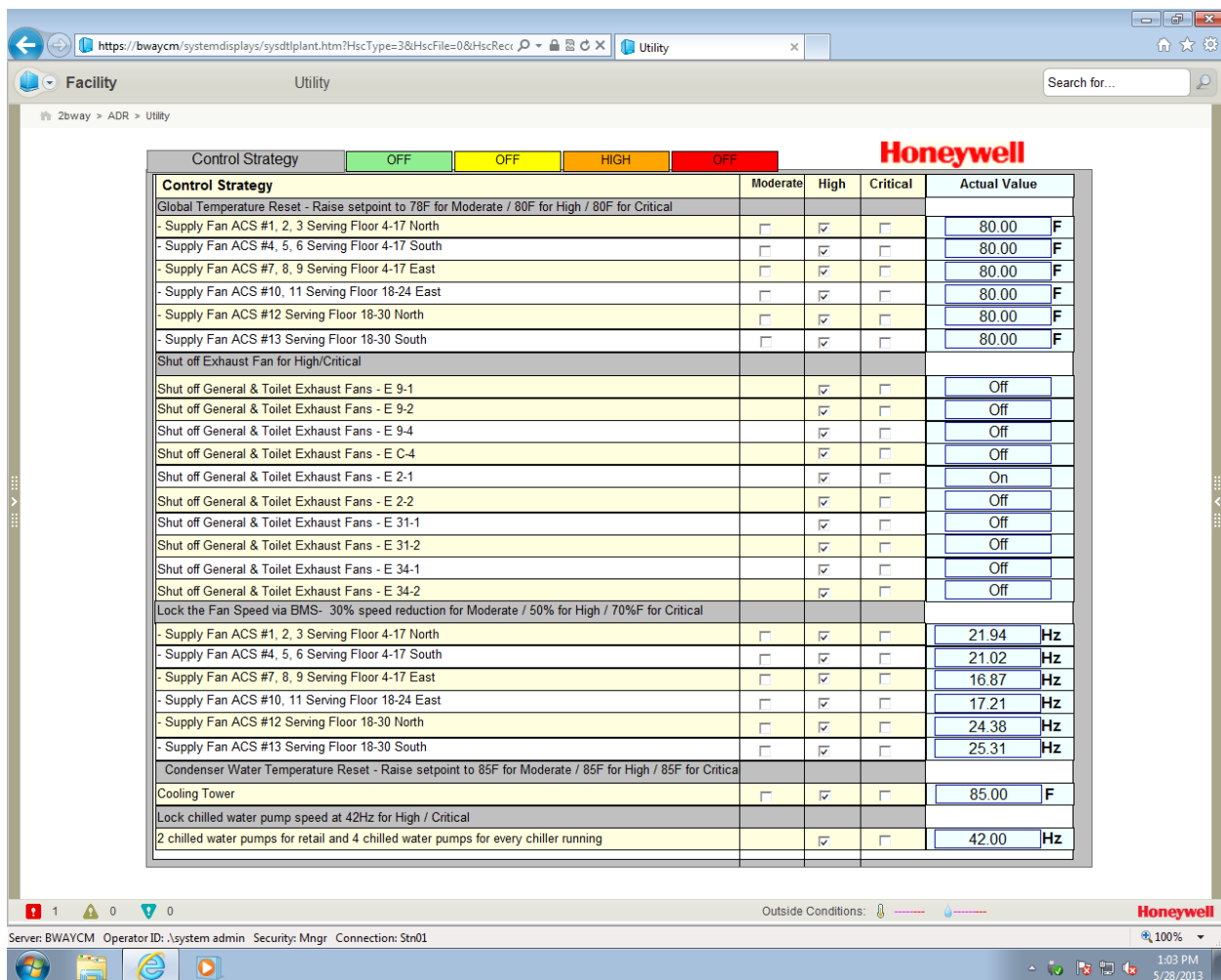
Figure 1. Honeywell's ComfortPoint™ Open Plant Controller User Interface
