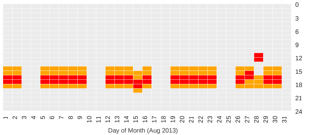
Figure 6. Office Building A - Automated Price Response Schedule for August 2013
