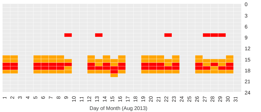
Figure 16. Campus Building - Automated Price Response Schedule for August 2013
