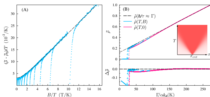
Figure 1: (A) Resistance as function of temperature and magnetic field (blue) falls on a single universal function (black dashed line). (B) Raw data of resistance as a function of field and temperature plotted with respect to a new energy scale that combines magnetic and thermal contributions.
