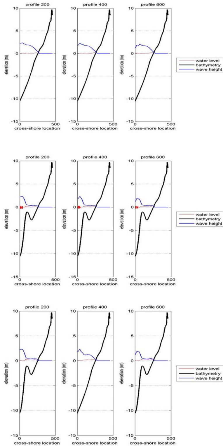
Figure 44. Wave height and water level for H_{m0} = 3.0\text{m} for no bar bathymetry (top), continuous bar bathymetry (middle), and bar-rip bathymetry (bottom)
