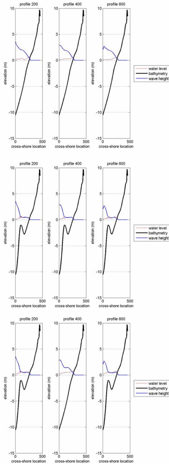
Figure 48. Wave height and water level for H_{m0} = 5.0\text{m} for no bar bathymetry (top), continuous bar bathymetry (middle), and bar-rip bathymetry (bottom)
