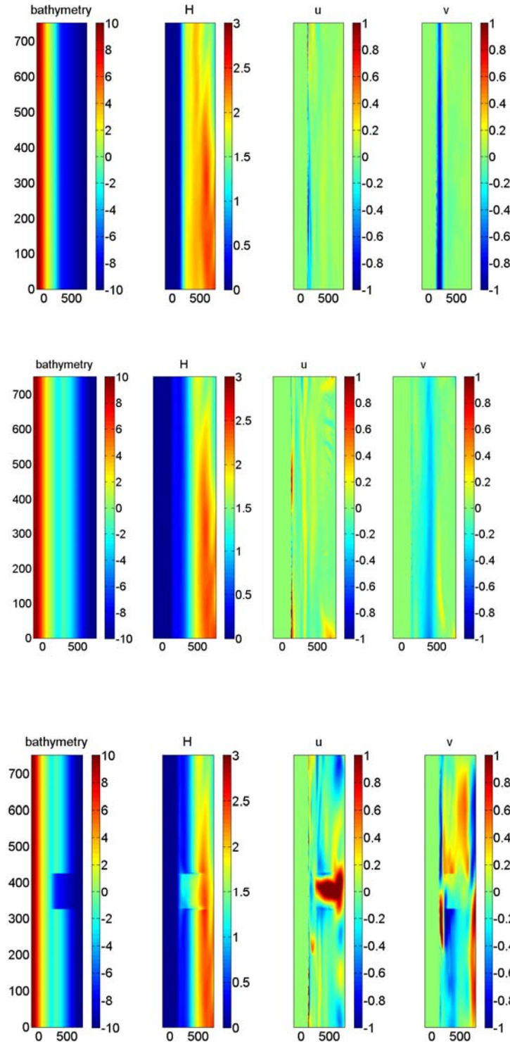
Figure 42. Wave height and velocities for H_{mo} = 3.0m for no bar bathymetry (top), continuous bar bathymetry (middle), and bar-rip bathymetry (bottom)
