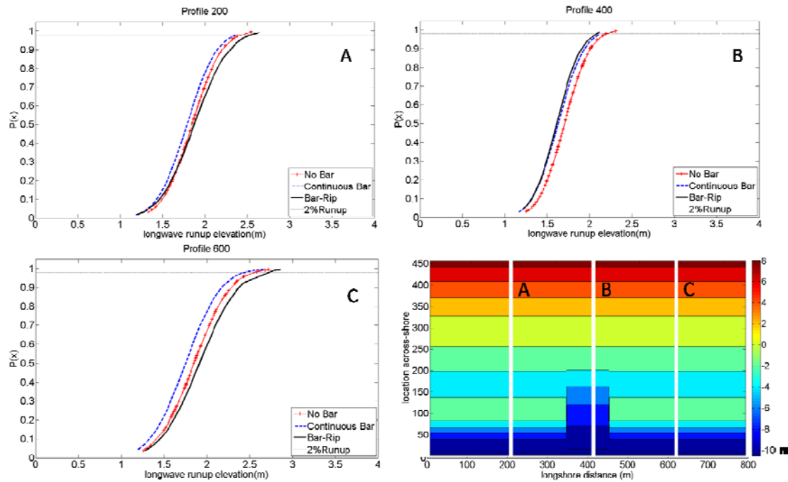
Figure 36. CDF long-wave runup H_{mo} 7.0m
