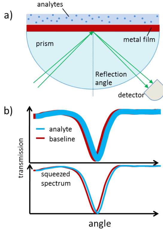
Figure 1: a) A SPR sensor consisting of a prism, metal coating on the backside, a readout light field, and detector which reads angular shift. b) Schematic showing intensity and noise of a reflective SPR sensor as a function of angle.
