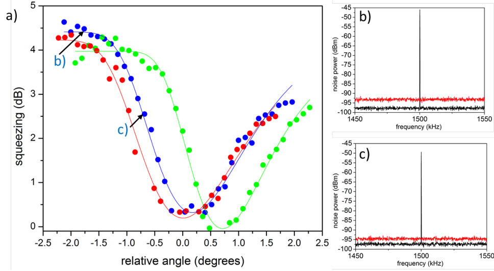
Figure 4: a: Quantum noise reduction as a function of angle of incidence and index of refraction (green: n=1.305 ; blue: n=1.301 ; red: n=1.300 ). b & c: the raw data for two points along the curve. The red line indicates the shot noise level, while the peak is associated with the transmitted probe power. The sidebands that indicate the noise floor associated with each data point fall below the SNL - squeezing is equal to the difference between the black and red sidebands. Squeezing decreases as transmission decreases, but virtually all data points are squeezed. A maximum of 4.6 dB below the SNL is observed in the peak shoulders. A minimum of 0.3 dB is observed in the n=1.300 and n=1.301 datasets, while the n=1.305 dataset minimum is at the SNL.
