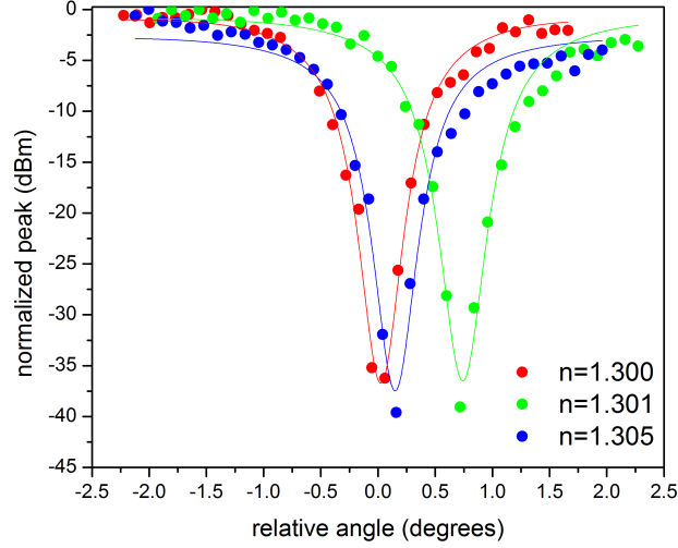
Figure 3: a: Plasmonic resonance as a function of relative angle of incidence ( 0^\circ corresponds to on-resonance for n = 1.3 ) and index of refraction (green: n=1.305 ; blue: n=1.301 ; red: n=1.300 ). The numerical curve fits are intended as a guide to the eye.
