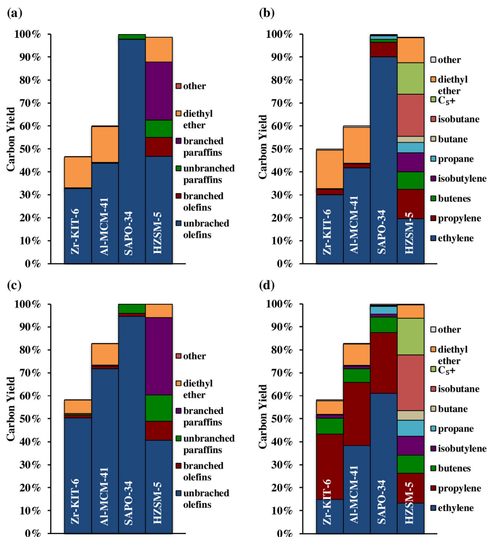
Fig. 4. Carbon yield for mixed alcohol dehydration experiments at 300 °C and WHSV = 0.32 h -1 from the (a, b) ethanol rich mixed alcohol feed and (c, d) C 3 –alcohol rich feed. Data is grouped by (a, c) functional group and branching and by (b, d) major product species. ‘Other’ corresponds to the sum of carbon monoxide, carbon dioxide, propanal and methanol. Data is presented as average of replicate data points at WHSV = 0.32 h -1 except for Zr-KIT-6 in (a, b) which is presented as the first data point at WHSV = 0.32 h -1 .
