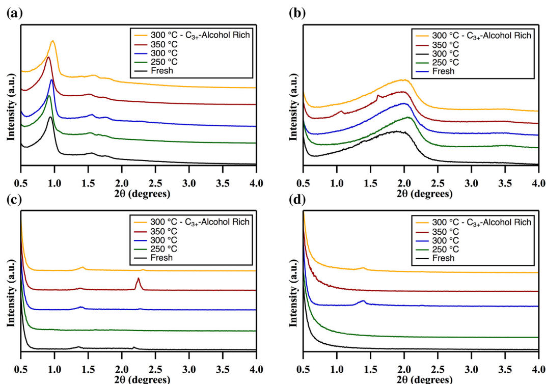
Fig. 6. Small angle scattering patterns for post-reaction catalysts. (a) Zr-KIT-6, (b) Al-MCM-41, (c) SAPO-34 and (d) HZSM-5. Fresh catalyst scattering patterns are shown for reference. Peaks at 1.4° and 2.3° in (c, d), or 1.1° and 1.7° in (b), are due to the glass tray and are not indicative of mesoporous features.
