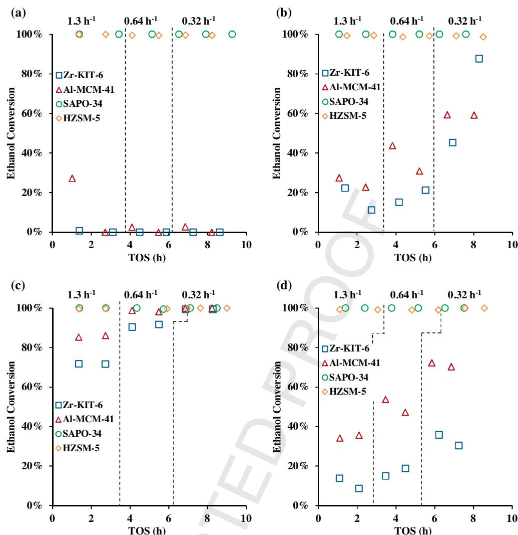
Fig. 3. Ethanol conversion in mixed alcohol dehydration experiments as a function of time-on-stream and WHSV for experiments with the ethanol rich alcohol feed at (a) 250 °C, (b) 300 °C, (c) 350 °C, and (d) with the C 3+ -alcohol rich feed at 300 °C for each catalyst.
