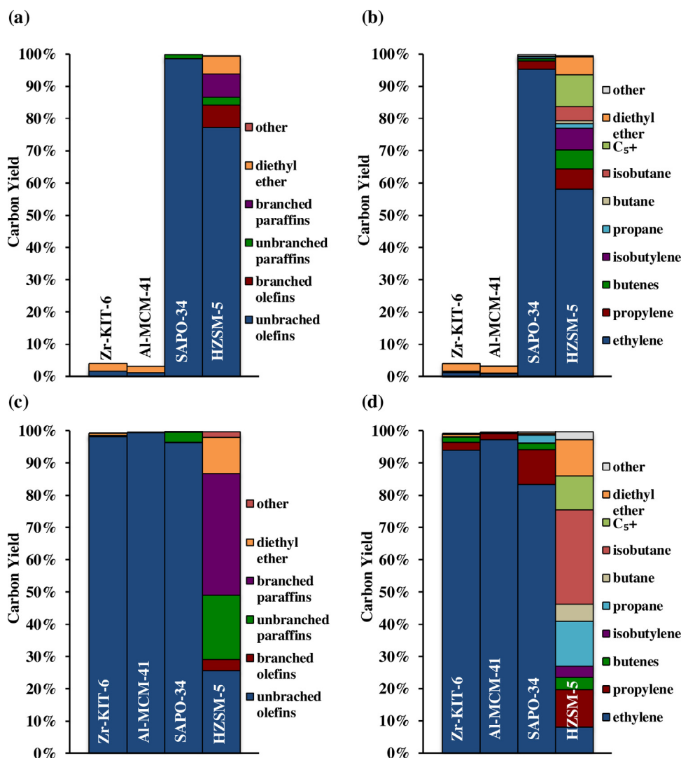
Fig. 5. Carbon yield from mixed alcohol dehydration experiments with the ethanol rich mixed alcohol feed at (a, b) 250 °C and (c, d) 350 °C. Data is grouped by (a, c) functional group and branching and by (b, d) major product species. 'Other' products are carbon monoxide, carbon dioxide, propanal and methanol. Data is presented as average of replicate data points at WHSV = 0.32 h -1 .
