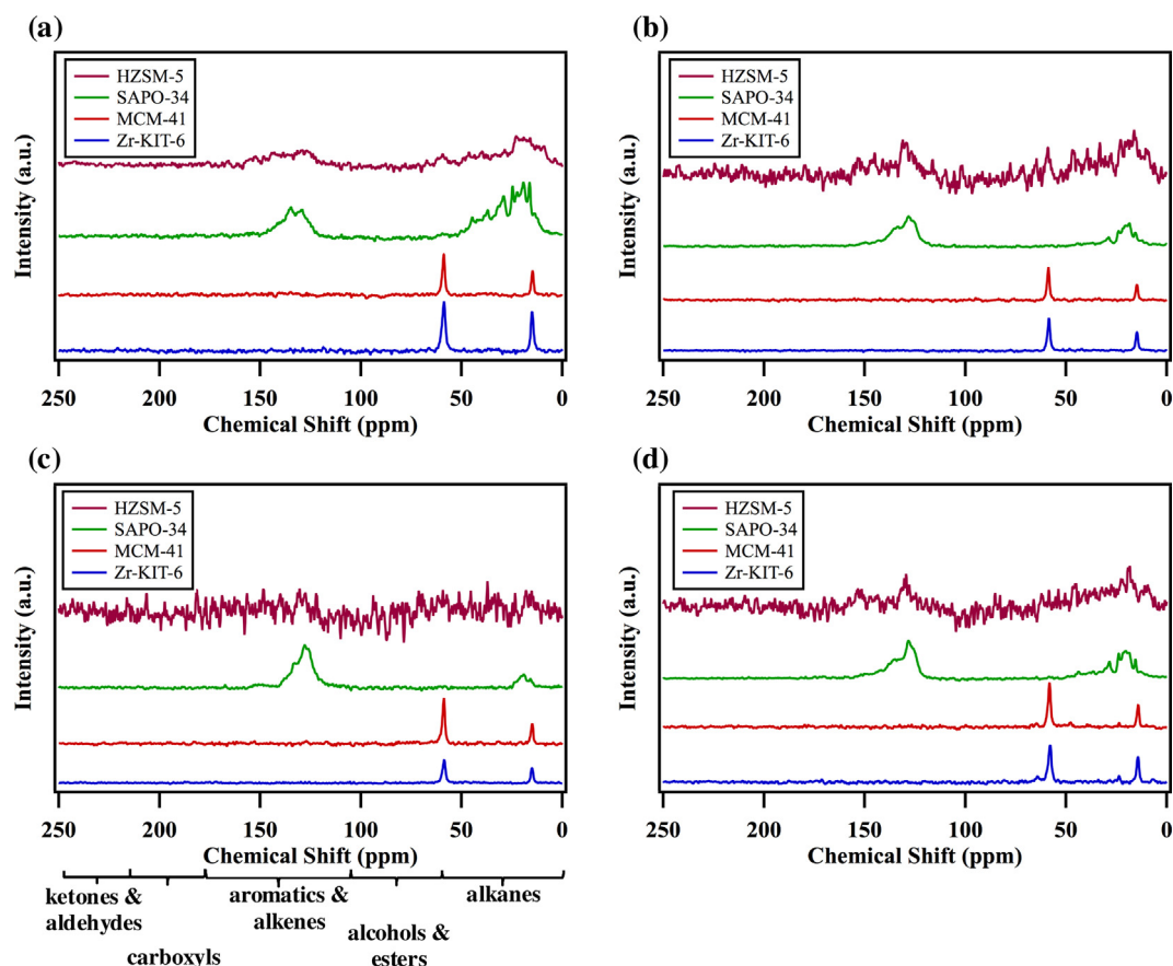
Fig. 8. Solid-state NMR spectra for post-reaction catalysts run at (a) 250 °C, (b) 300 °C and (c) 350 °C with the ethanol rich feed stream and (d) with the C 3+ -alcohol rich feed at 300 °C. Function group regions are shown below (c) for reference.
