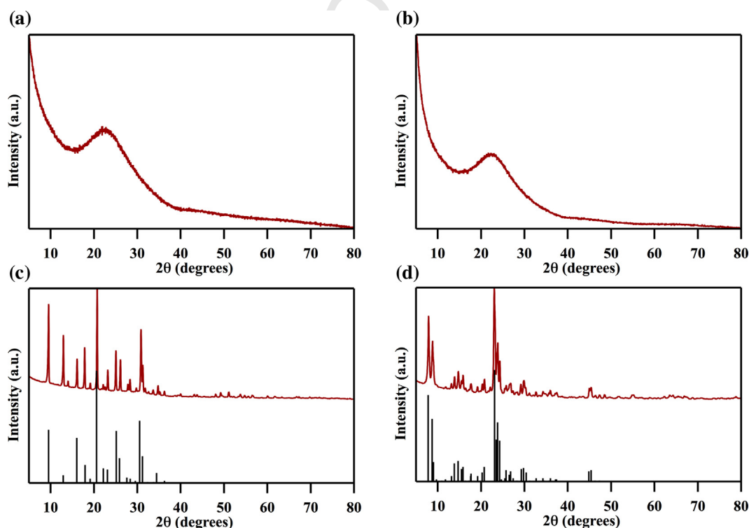
Fig. 2. Powder X-ray diffractograms for fresh (a) Zr-KIT-6, (b) Al-MCM-41, (c) SAPO-34, and (d) HZSM-5 catalysts. Reference diffraction patterns are shown where available (black lines).
