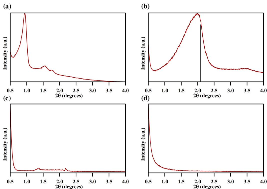
Fig. 1. Small angle scattering patterns for fresh (a) Zr-KIT-6, (b) Al-MCM-41, (c) SAPO-34 and (d) HZSM-5 catalysts. Reference diffraction patterns are shown where available (black lines). Peaks in (c) at 2\theta = 1.4^\circ and 2.25^\circ are due to the glass support slide.
