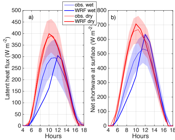
Figure 2. Surface latent and net shortwave heat fluxes as modeled by WRF with the Weak Temperature Gradient compared with observations.
