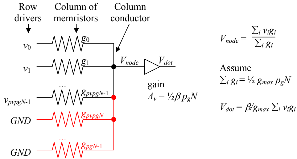
Figure 22: Circuit for analysis of sparse dot product
