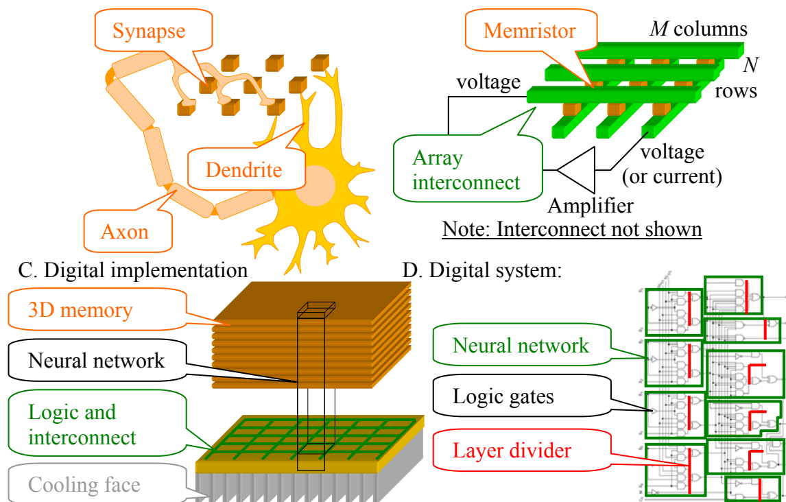
Figure 3: Explanatory implementations of the Turon architecture
