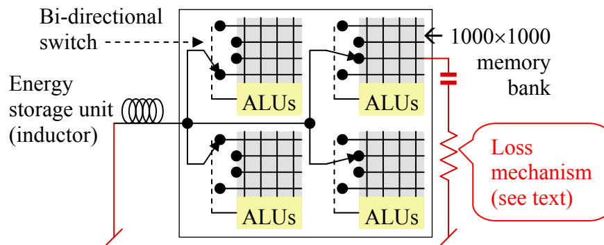
Figure 9: Adiabatic clocking for four PIMS replication units
