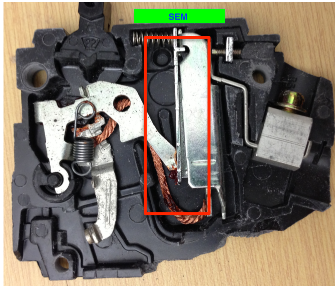
Figure 7: Bimetallic strip circuit breaker innards with SEM annotated and active elements that cause breaker to trip located in the box.
