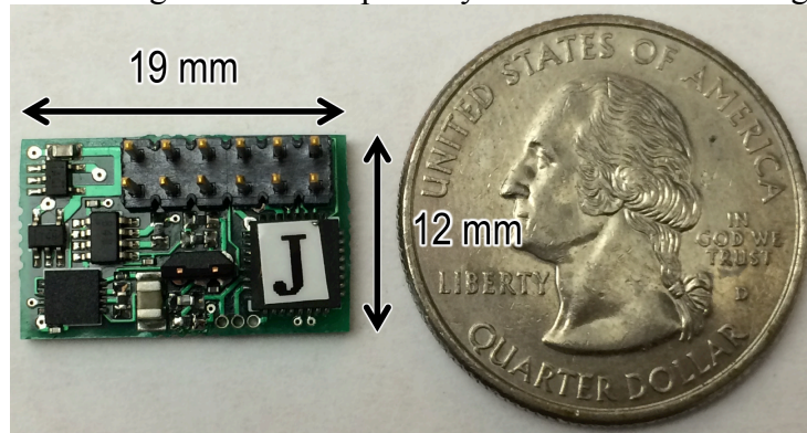
Figure 2: 19 x 12 mm (0.8 x 0.5 in) assembled Stick-on Electricity Meter with size reference
