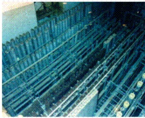
Figure 5. RBOF Storage Racks
