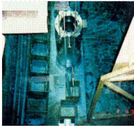
Figure 9. Cask Unloading Basin
