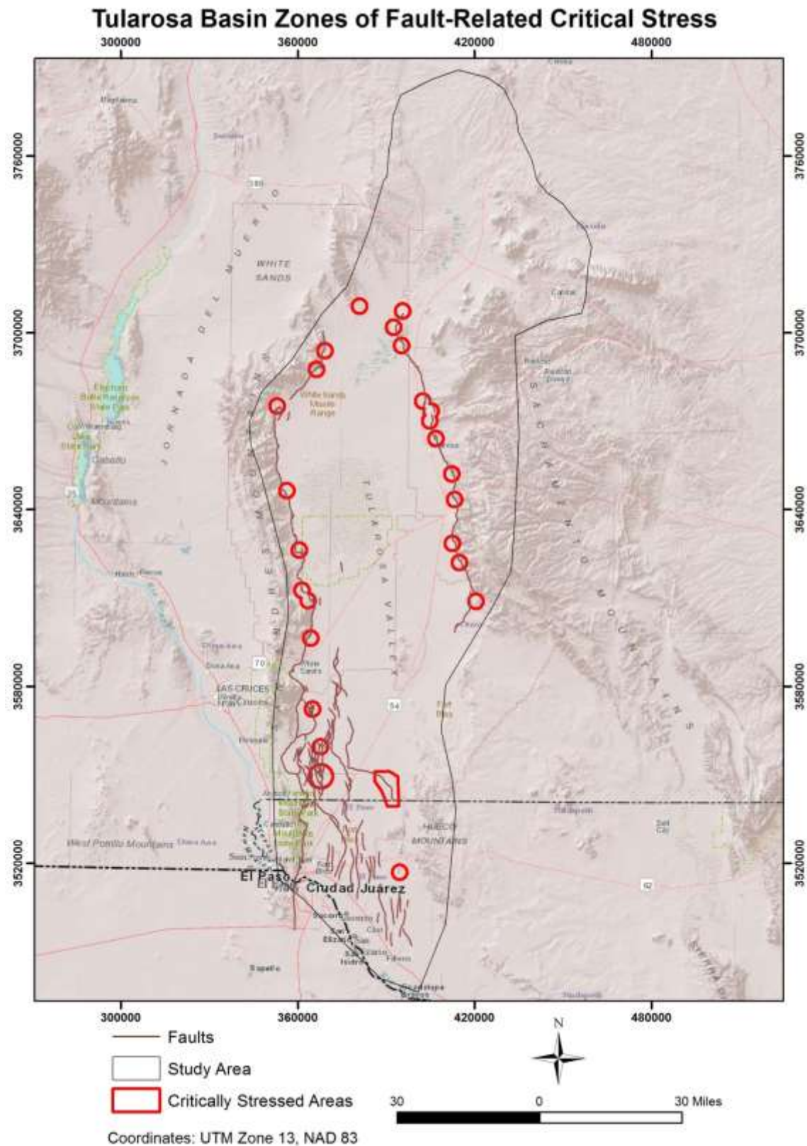
Figure 9. Study area Quaternary faults and zones of critical stress.
