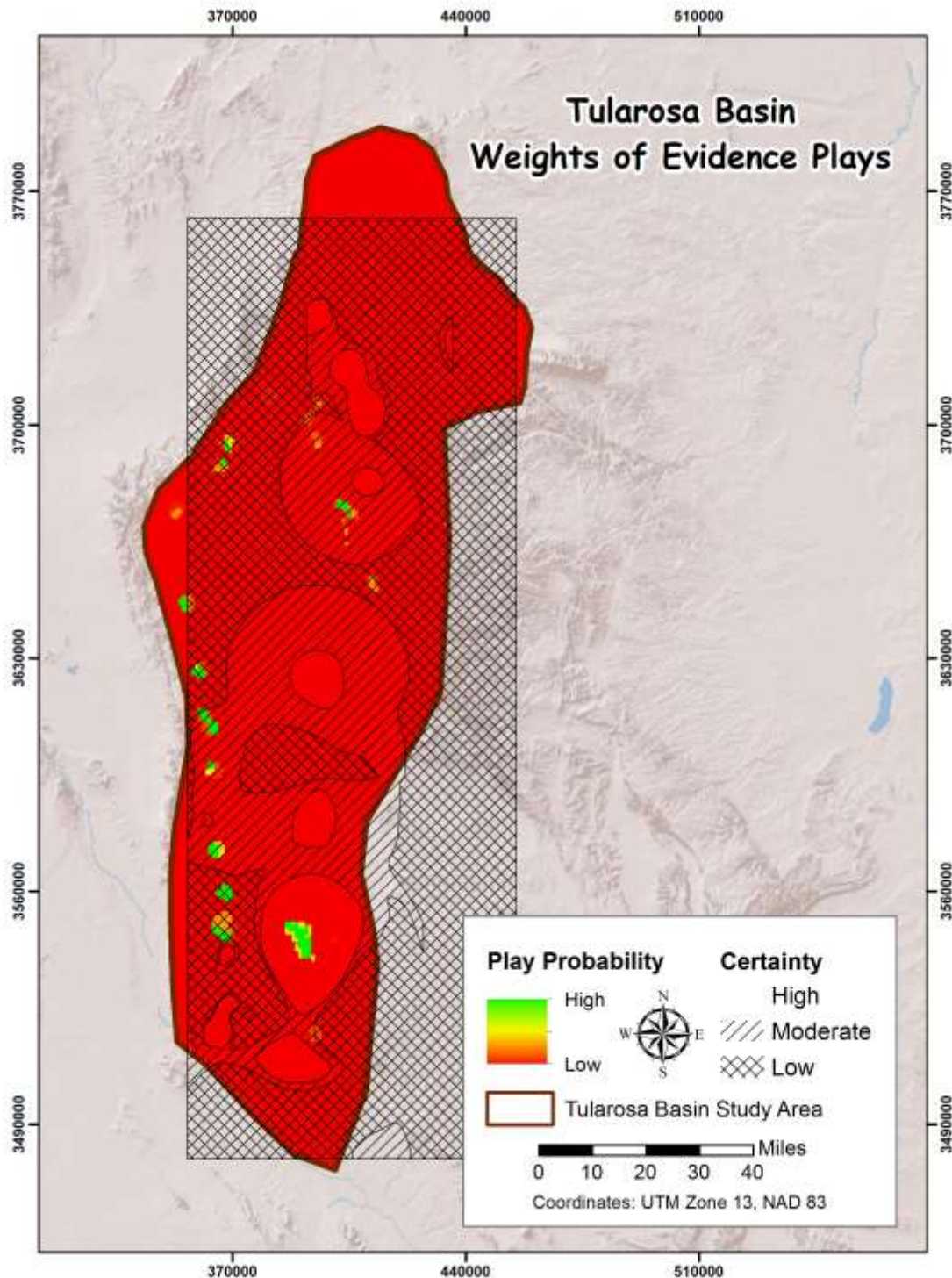
Figure 24. Certainty based upon probability kriging. Heat layers of evidence were used in this analysis, the results of which are more conservative than the WoE confidence surface with only the McGregor Range play having high certainty and three other plays having moderate certainty. Areas outside of the certainty polygon lack control data.
