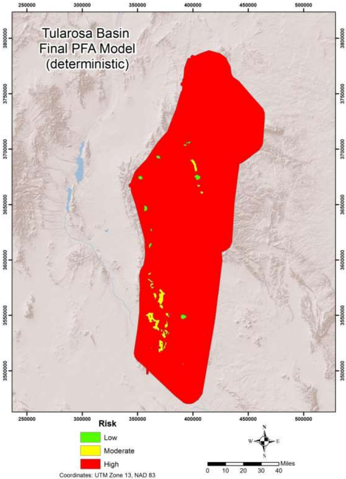
Figure 12. Final petroleum industry logic PFA. This model identified eight plays including the known geothermal system.
