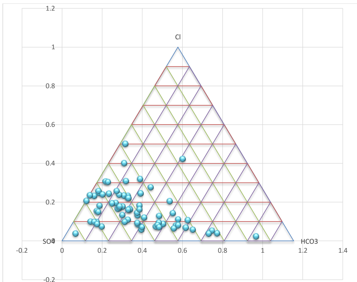
Figure 4. Relative Cl-SO 4 -HCO 3 contents of waters from the northern region of the play fairway.
