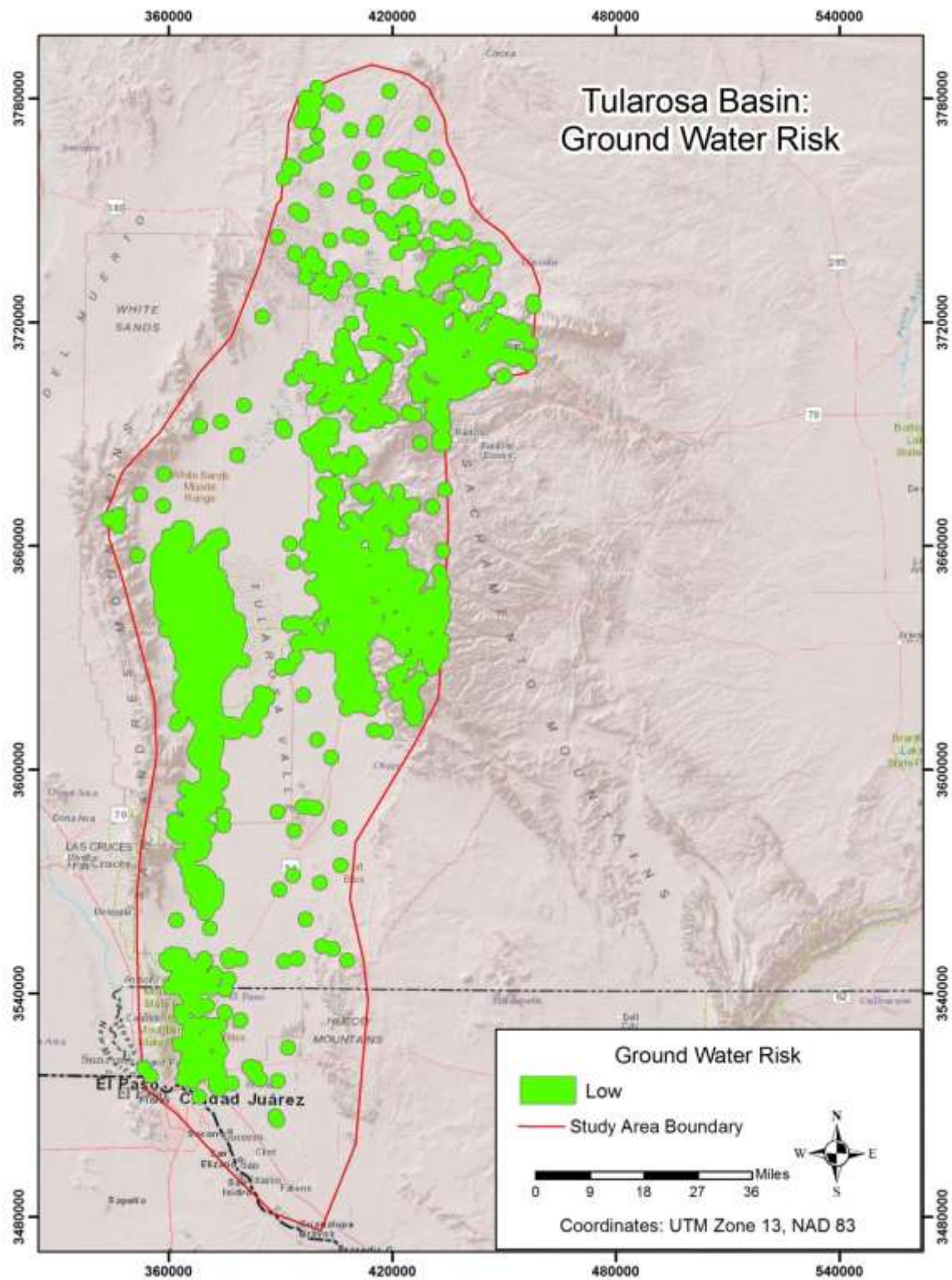
Figure 11. Ground water risk. All areas of the study area not colored in were considered to be high risk.
