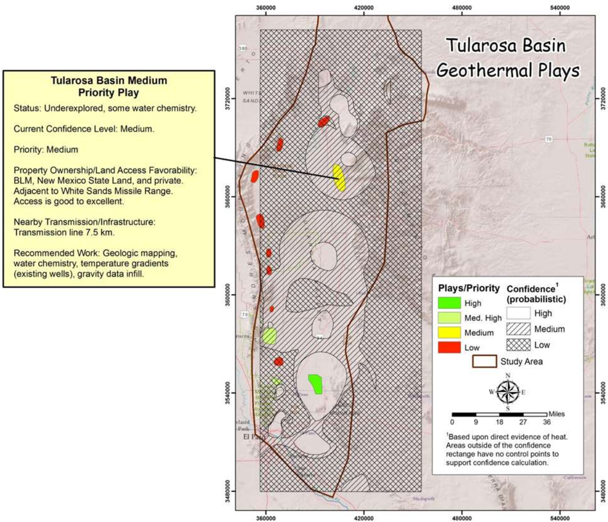
Figure 30. Suggested Phase 2 work for the medium priority play.
