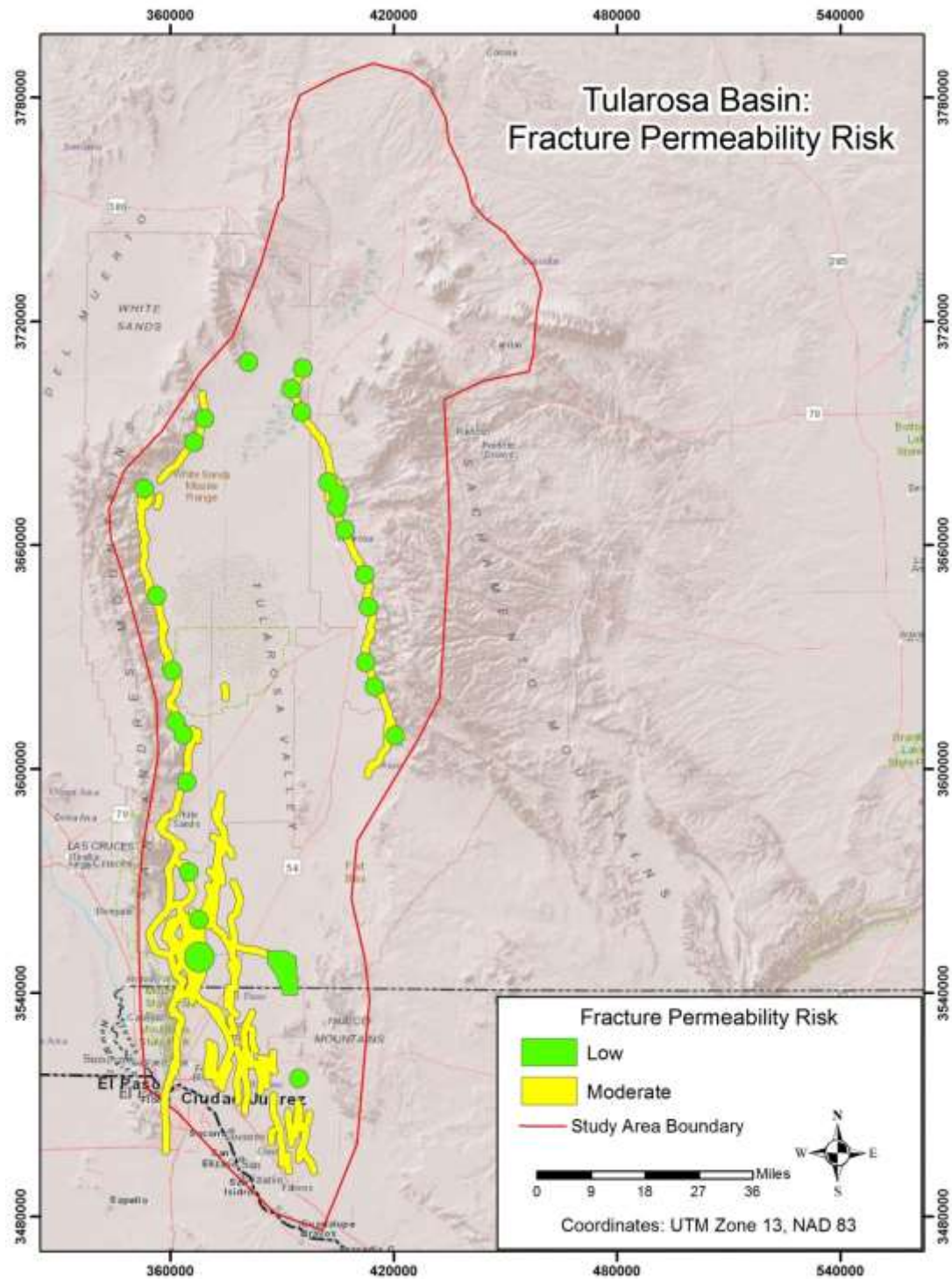
Figure 10. Fracture permeability risk CRS: Integration of Quaternary faults with a 1 km buffer (each side of fault) and 5 km diameter zones of critical stress. All areas within the study area boundary that are not colored are high risk.
