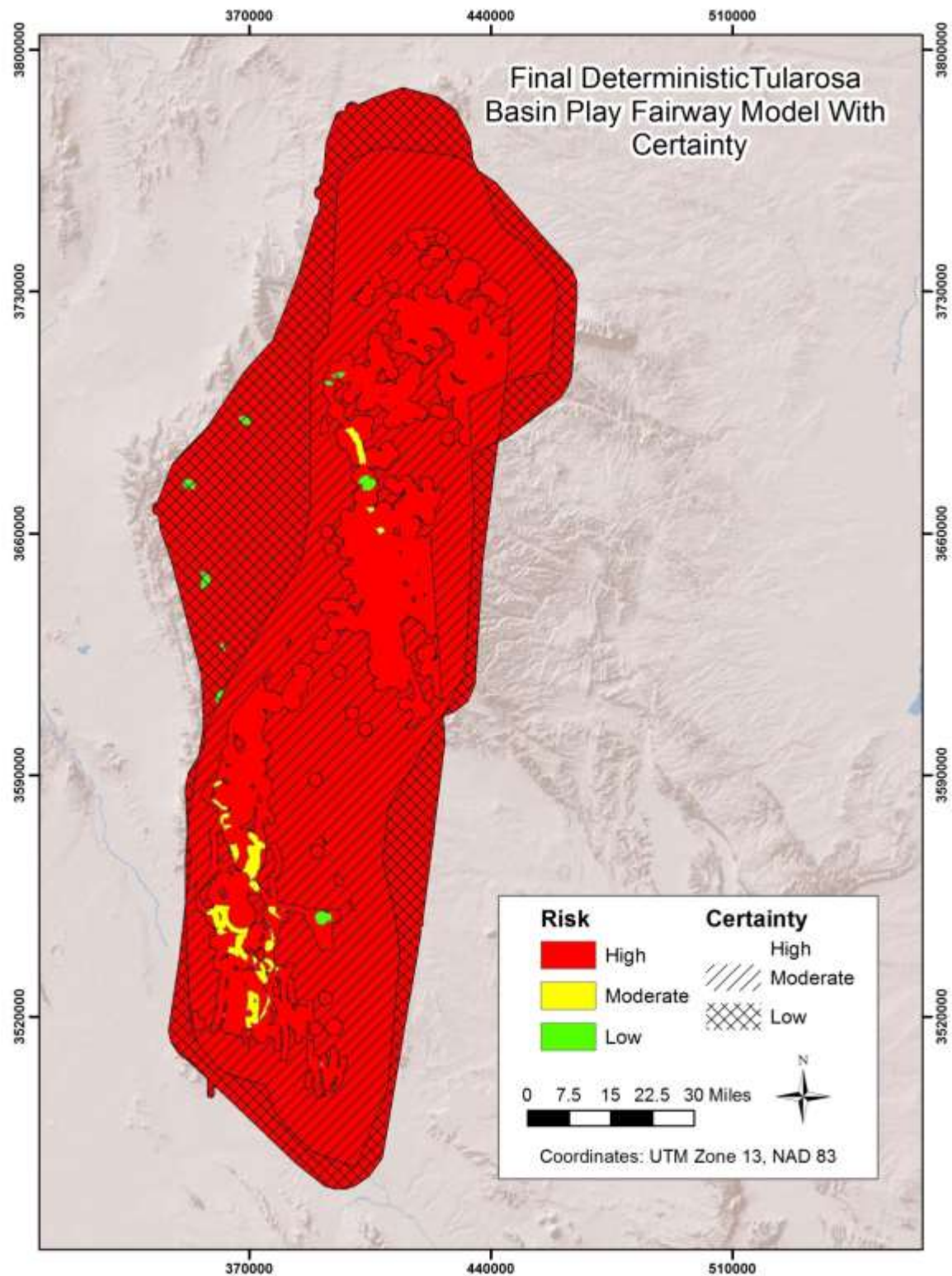
Figure 13. Deterministic certainty draped over the final deterministic PFA model.
