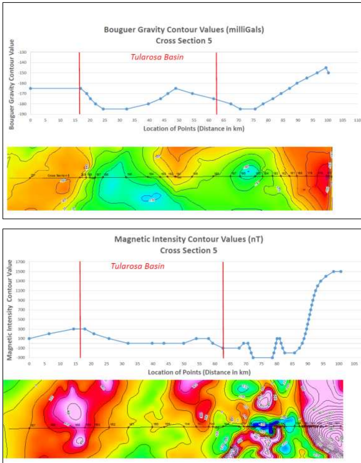
Figure 7. Both the gravity (top) and magnetic data (bottom) suggest the location of basin-bounding faults and what may be the southern margin of the mafic magma chamber related to the Quaternary basalt flow.
