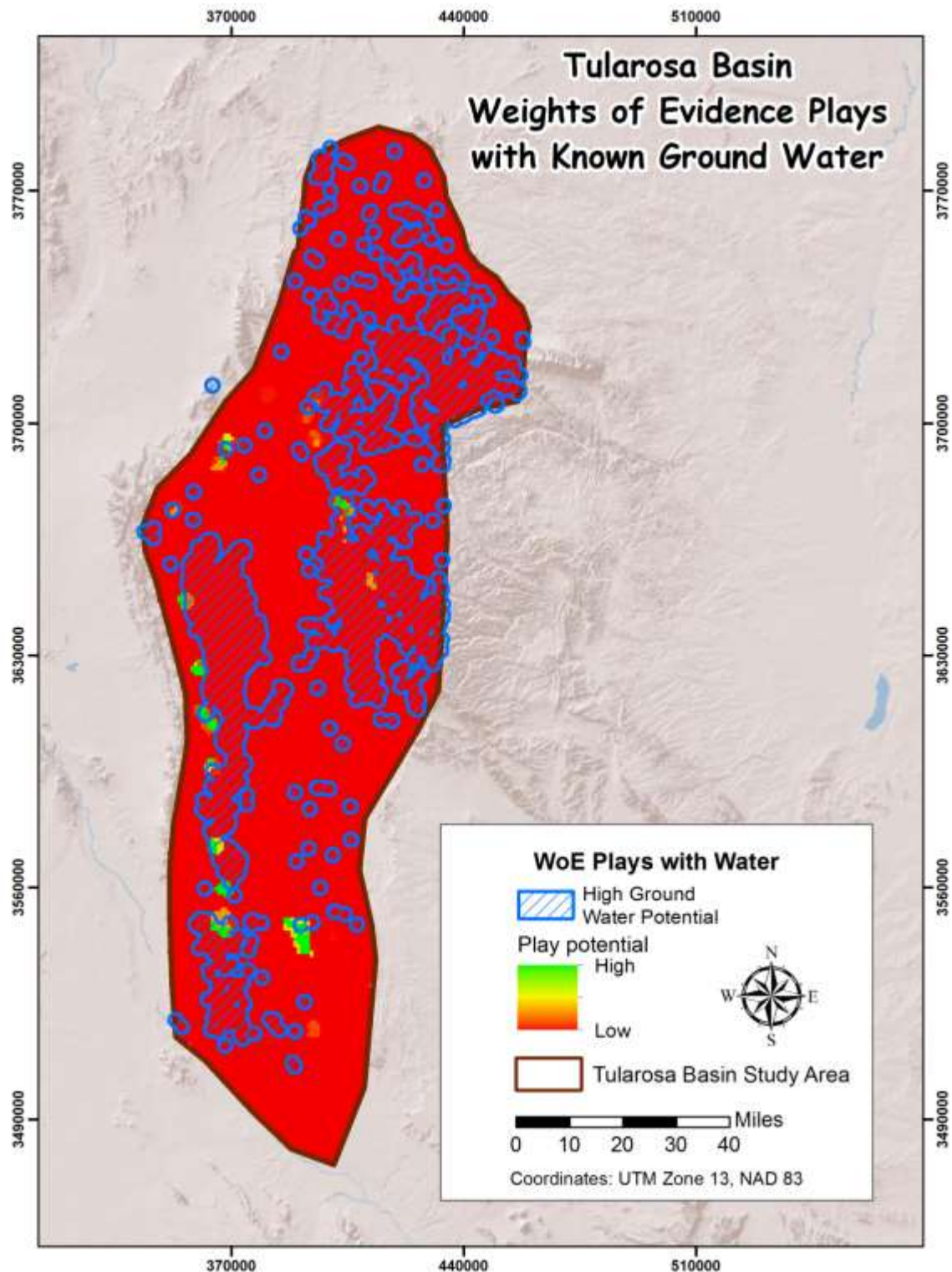
Figure 22. Ground water potential from the deterministic model overlain on WoE plays. Ground water potential is high on or bounding all plays.
