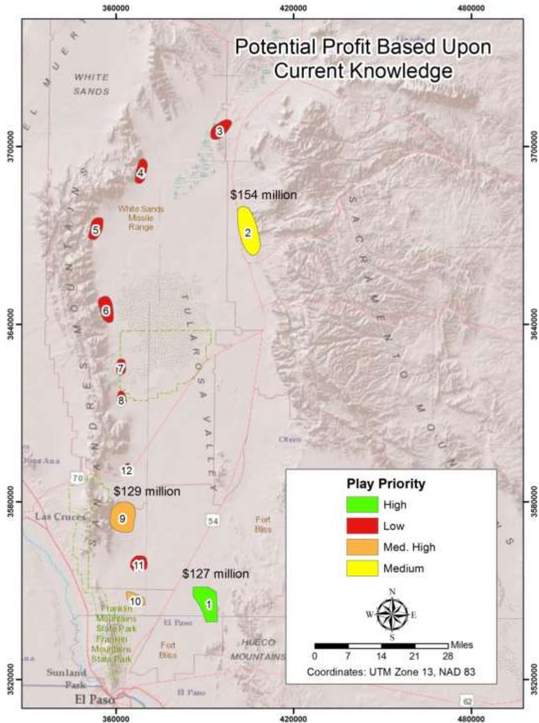
Figure 27. Profit potential of medium to high priority plays. Please note that Play 1 is the most data rich (low uncertainty), yet needs additional work to substantiate economic analysis. Plays 2 and 9 are relatively data poor and need considerably more work to facilitate refinement of this preliminary economic analysis. Please note that Play 10, although considered to be of Medium High priority, has low certainty due to critical data paucity, so no economic analysis was done for this play. Phase 2 addresses additional data needs that will allow better economic modeling.
