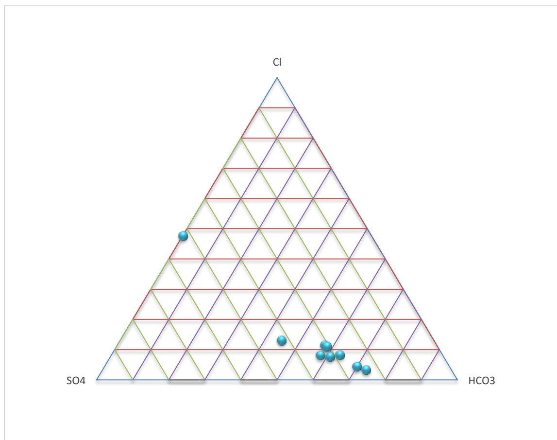
Figure 5. Relative Cl-SO 4 -HCO 3 contents of waters from the central region of the play fairway
