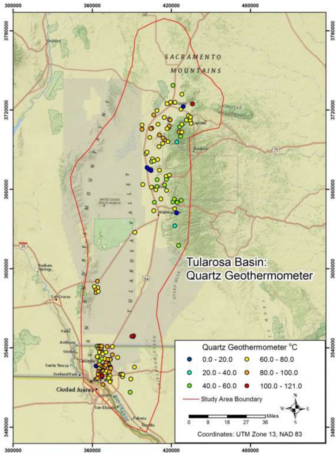
Fig. 8. Quartz (conductive) geothermometer temperatures.
