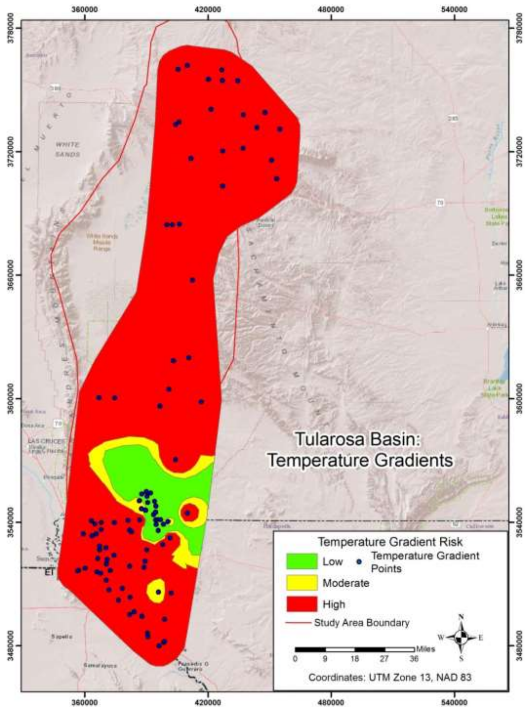
Figure 4. Heat risk -- temperature gradients.
