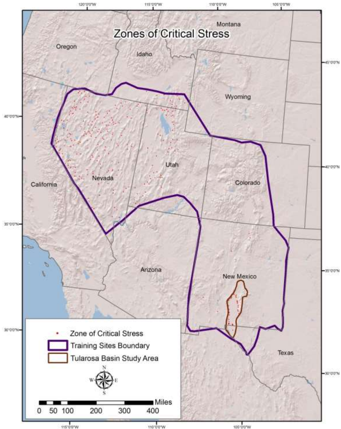
Figure 18. Zones of critical stress.
