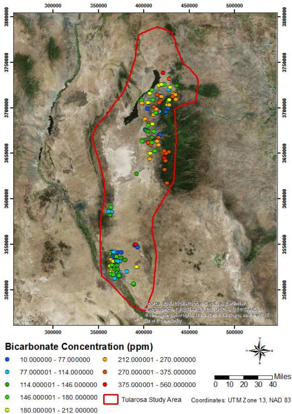
Figure 2. Bicarbonate ( \text{HCO}_3 ) contents of play fairway waters.
