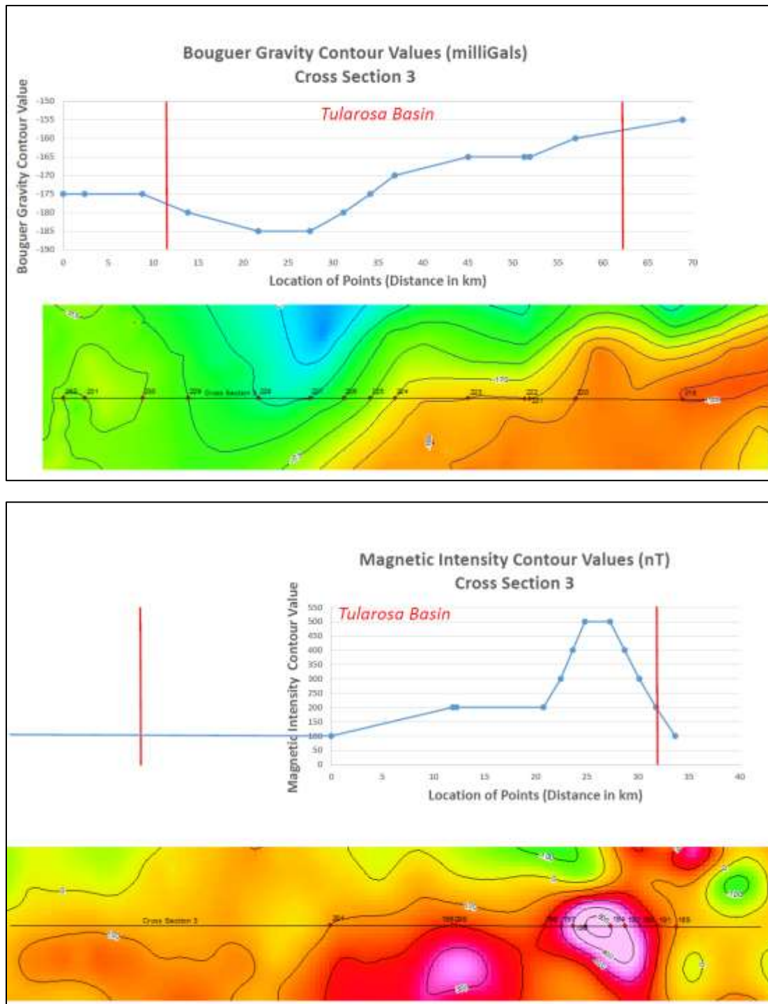
Figure 5. The gravity profile (top) suggest two west-dipping normal faults, one bounding the Sacramento Range and one out-board of the range, as well as an east-dipping normal fault bounding the basin on the west. The magnetic data (bottom) once again peaks on the east side of the cross-section suggestion intrusive rock, which is faulted (fault correlates with gravity fault). As the magnetic data cross-section slopes to the west it crosses a Quaternary basalt flow which may cause the moderate high prior to dropping off to the west.
