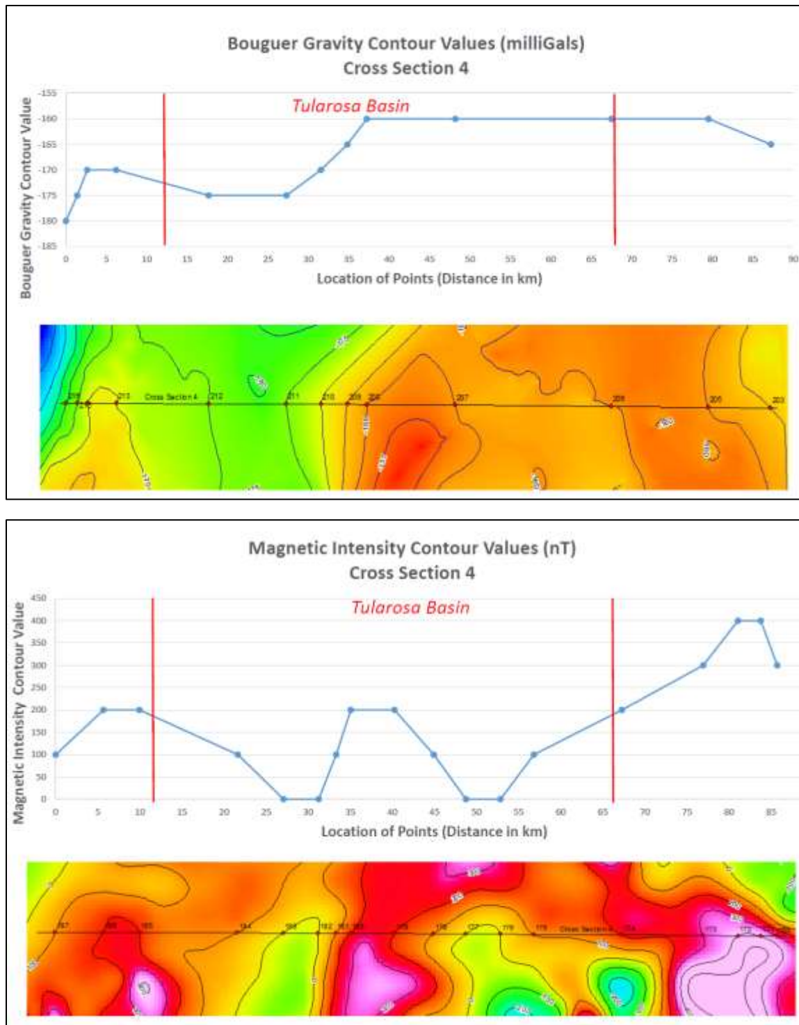
Figure 6. The gravity profile (top) shows a narrowing of the basin with a distinctive west-dipping fault bounding the east side of the valley and possibly another west-dipping fault on the western margin of the profile. The Magnetic data show a prominent high that may represent mafic magma chamber rocks related to the Quaternary basalt flow that this profile crosses.
