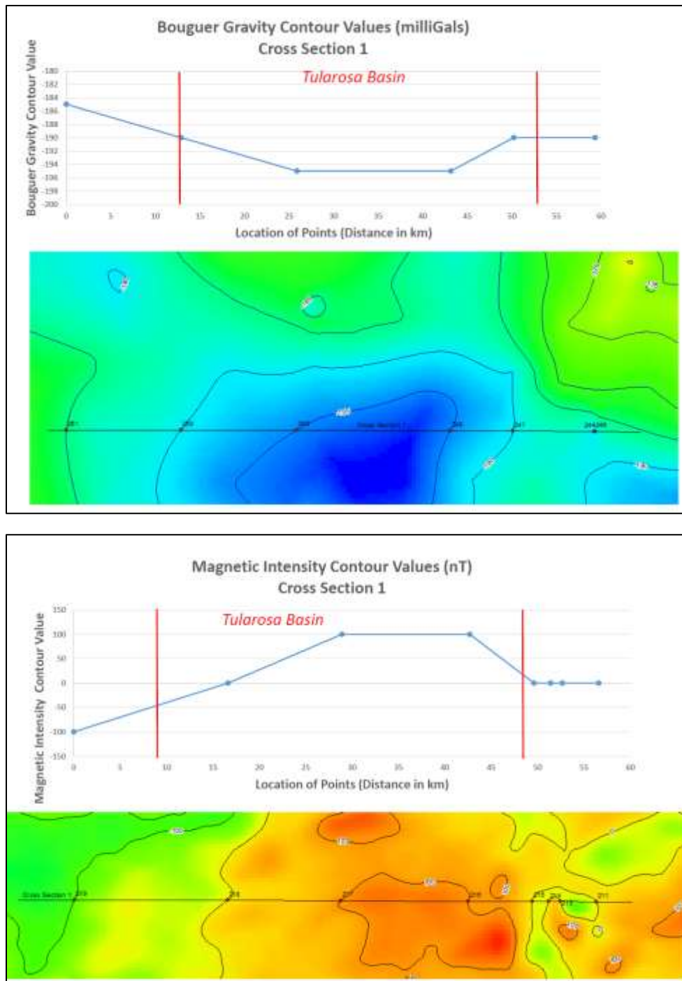
Figure 3. The east-west gravity cross-section (top) shows a relatively simple extensional basin profile. The bottom magnetic cross-section shows a high that is the inverse of the gravity profile, perhaps indicating a down-dropped tertiary intrusive.
