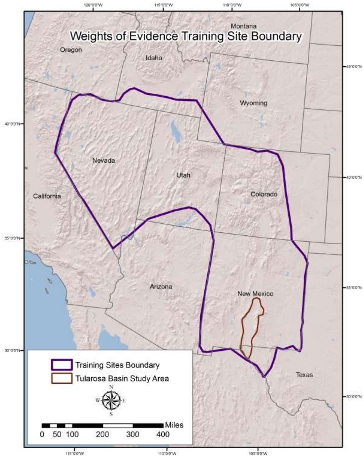
Figure 17. WoE training data boundary.
