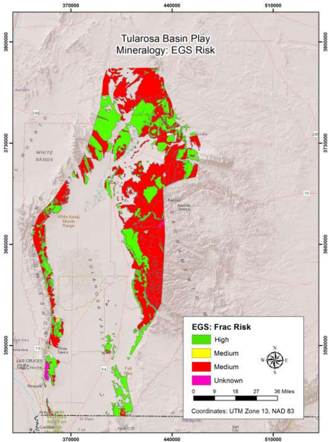
Figure 2. EGS risk based up rock brittleness suggested by ASTER multispectral image analysis.
