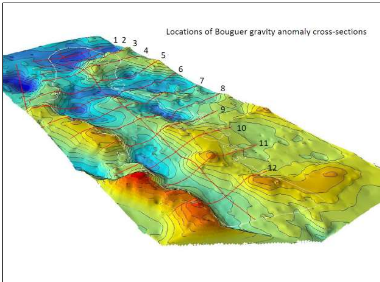
Figure 1. Locations of east-west cross sections for Bouguer gravity anomaly contours. Several sub-basins can be noted in this graphic.
