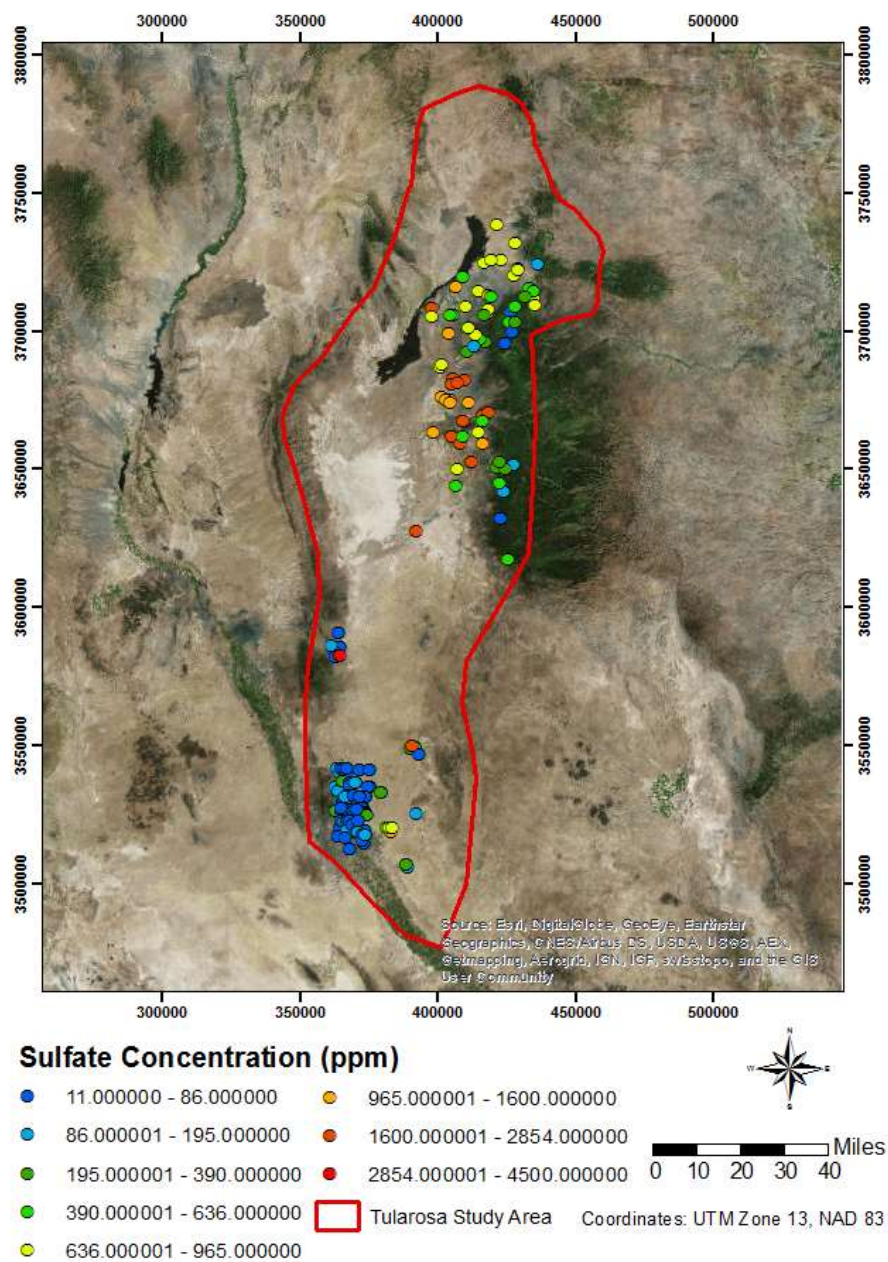
Figure 3. Sulfate ( \text{SO}_4 ) contents of play fairway waters.
