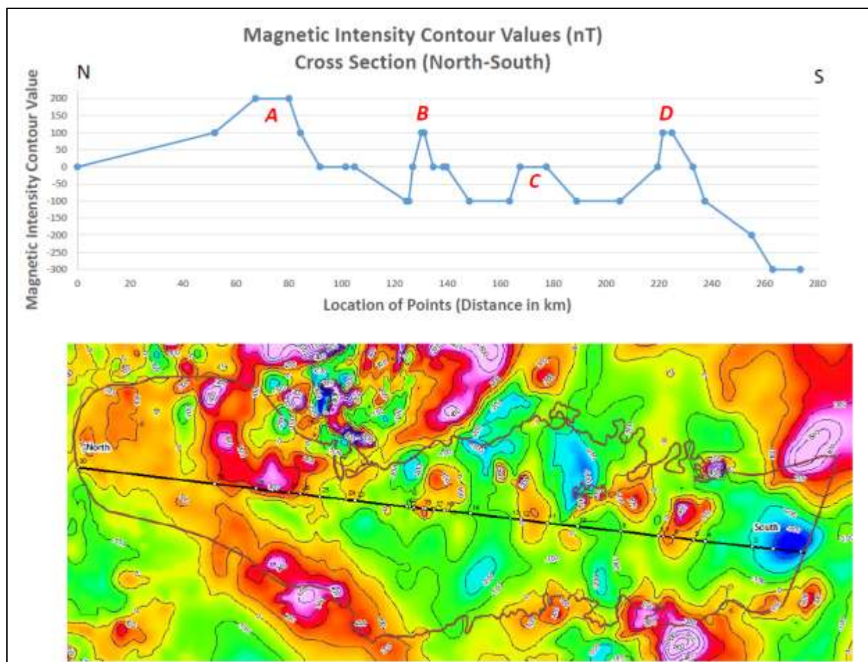
Figure 16. A north-south cross-section of magnetic intensity (in nanno-Tesla) across the Tularosa basin
