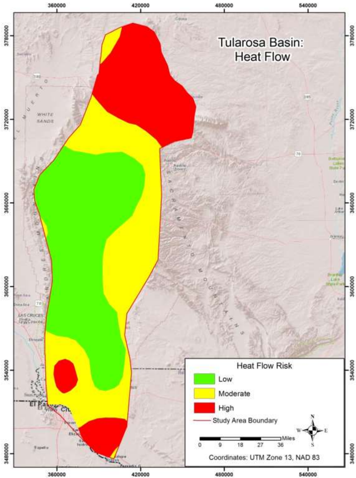
Figure 6. Heat risk – heat flow.
