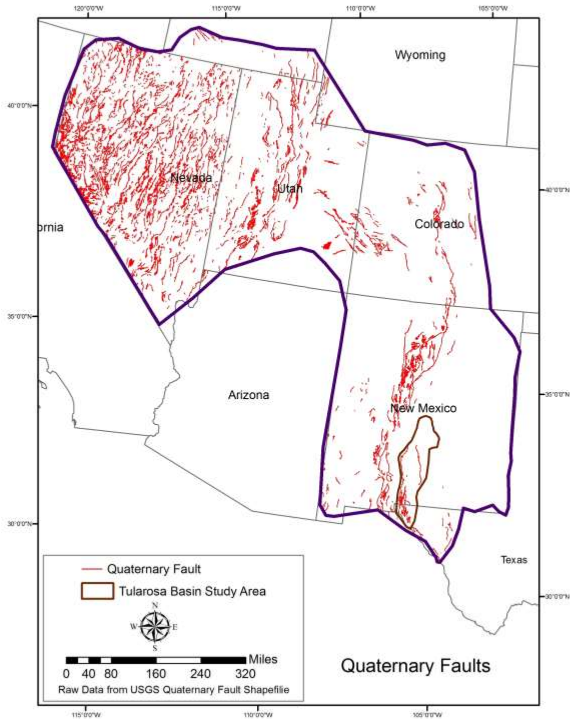
Figure 19. Quaternary faults buffered to 1 km (both sides of fault trace).
