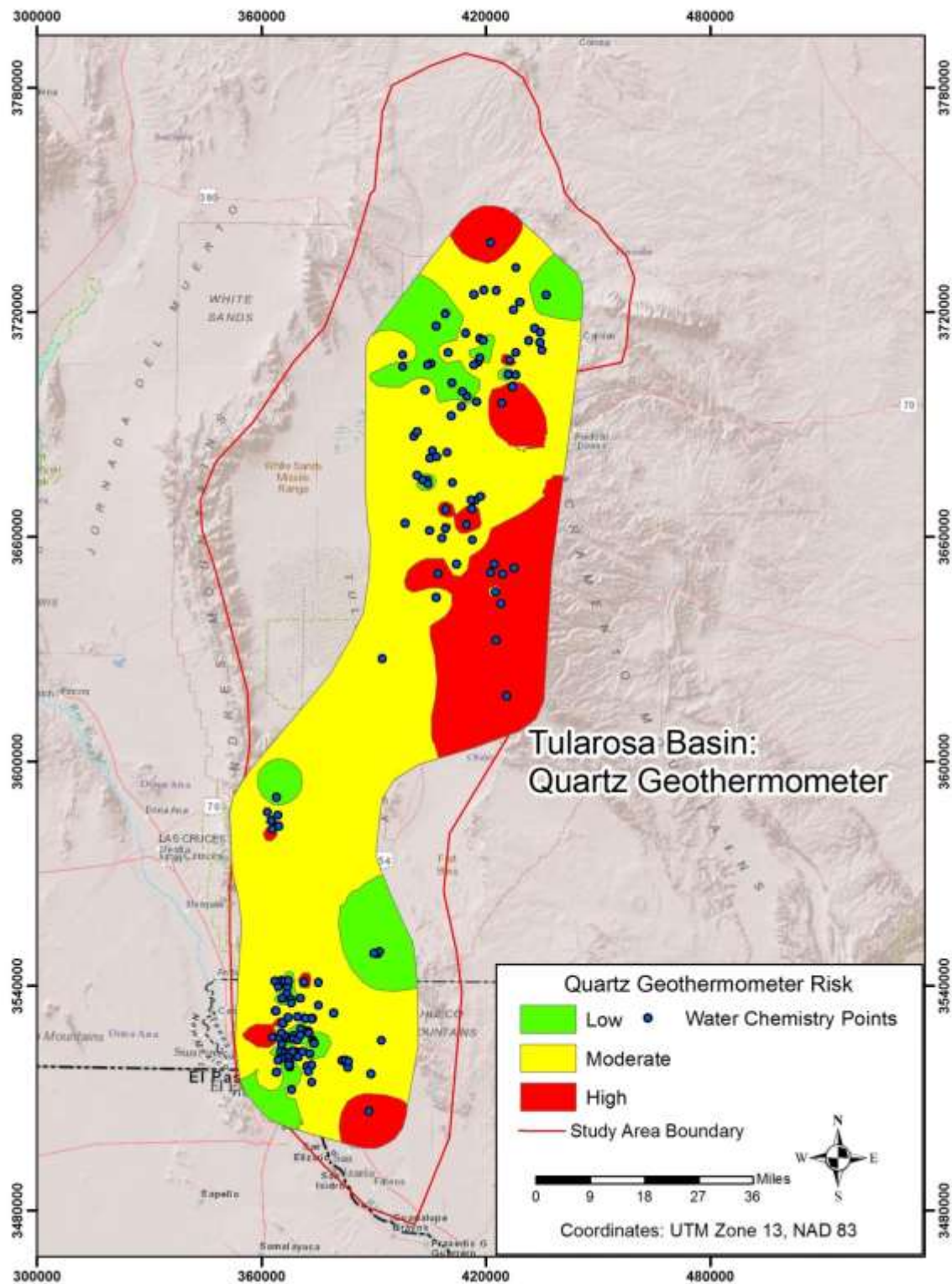
Figure 5. Heat risk – quartz geothermometers.
