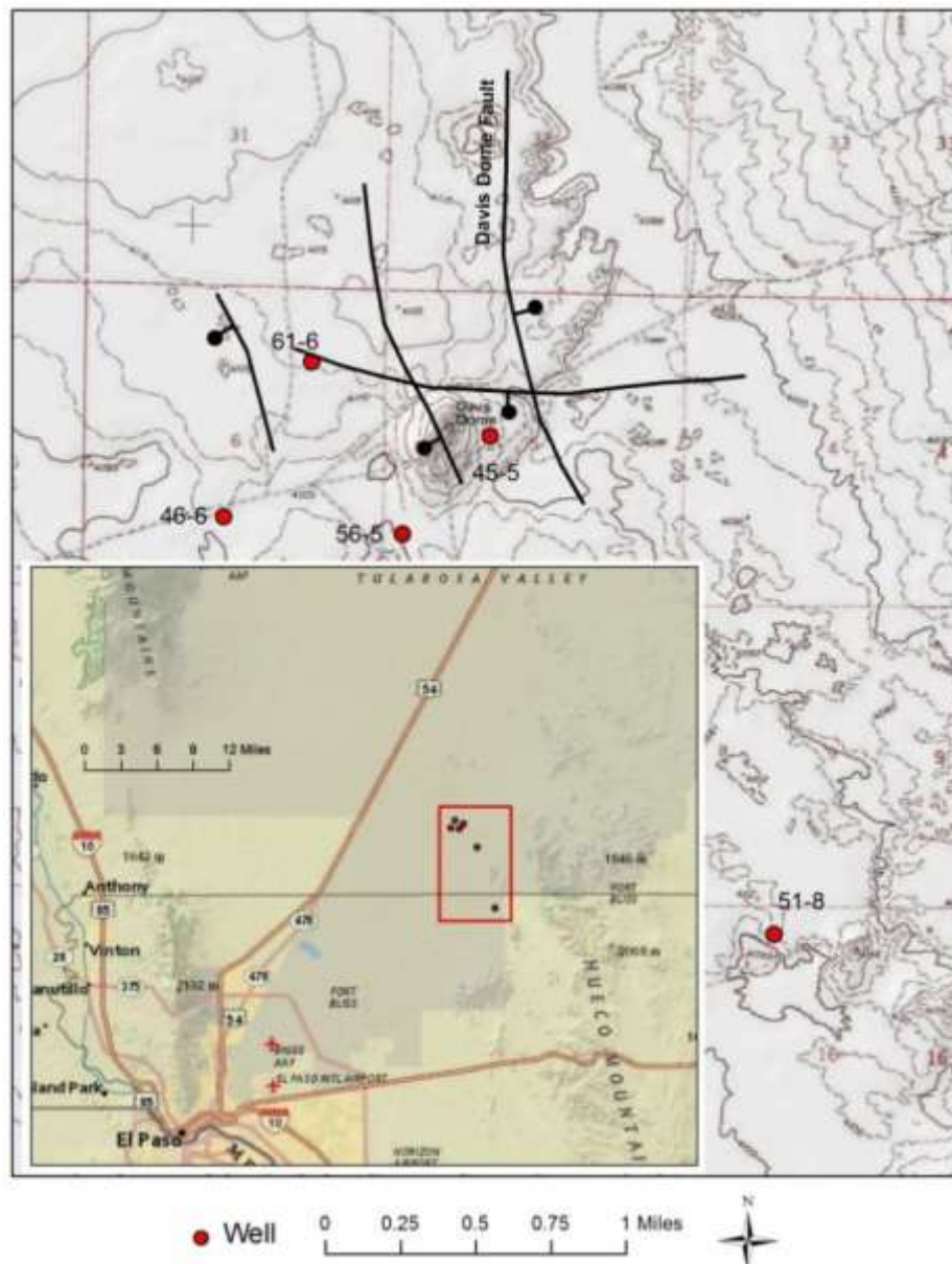
Figure 3. SANDIA slimholes 51-8, 46-6, 61-6, and 45-5 and RMI 56-5.
