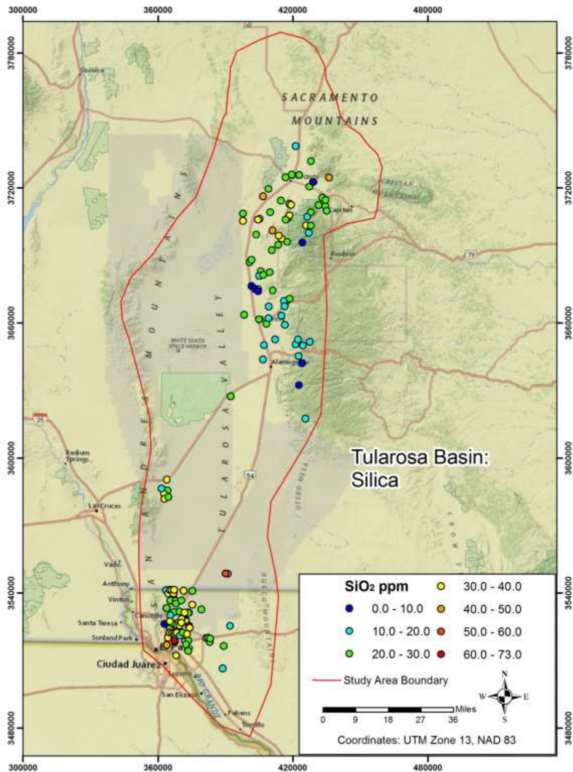
Fig. 7. Silica (SiO 2 ) contents of play fairway waters.
