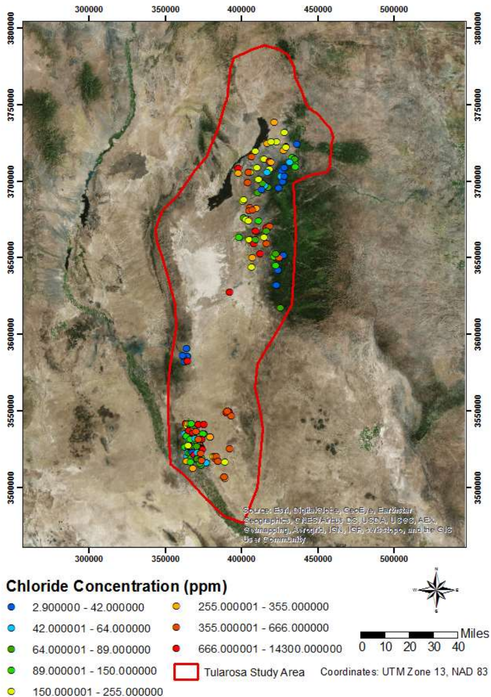
Figure 1. Chloride (Cl) contents of play fairway waters.
