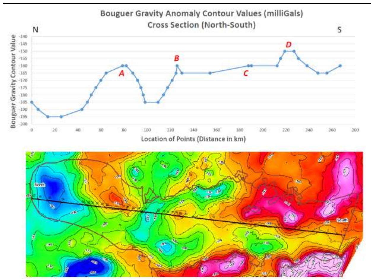
Figure 15. A north-south cross-section of Bouguer gravity anomaly (in milliGals) across the Tularosa basin
