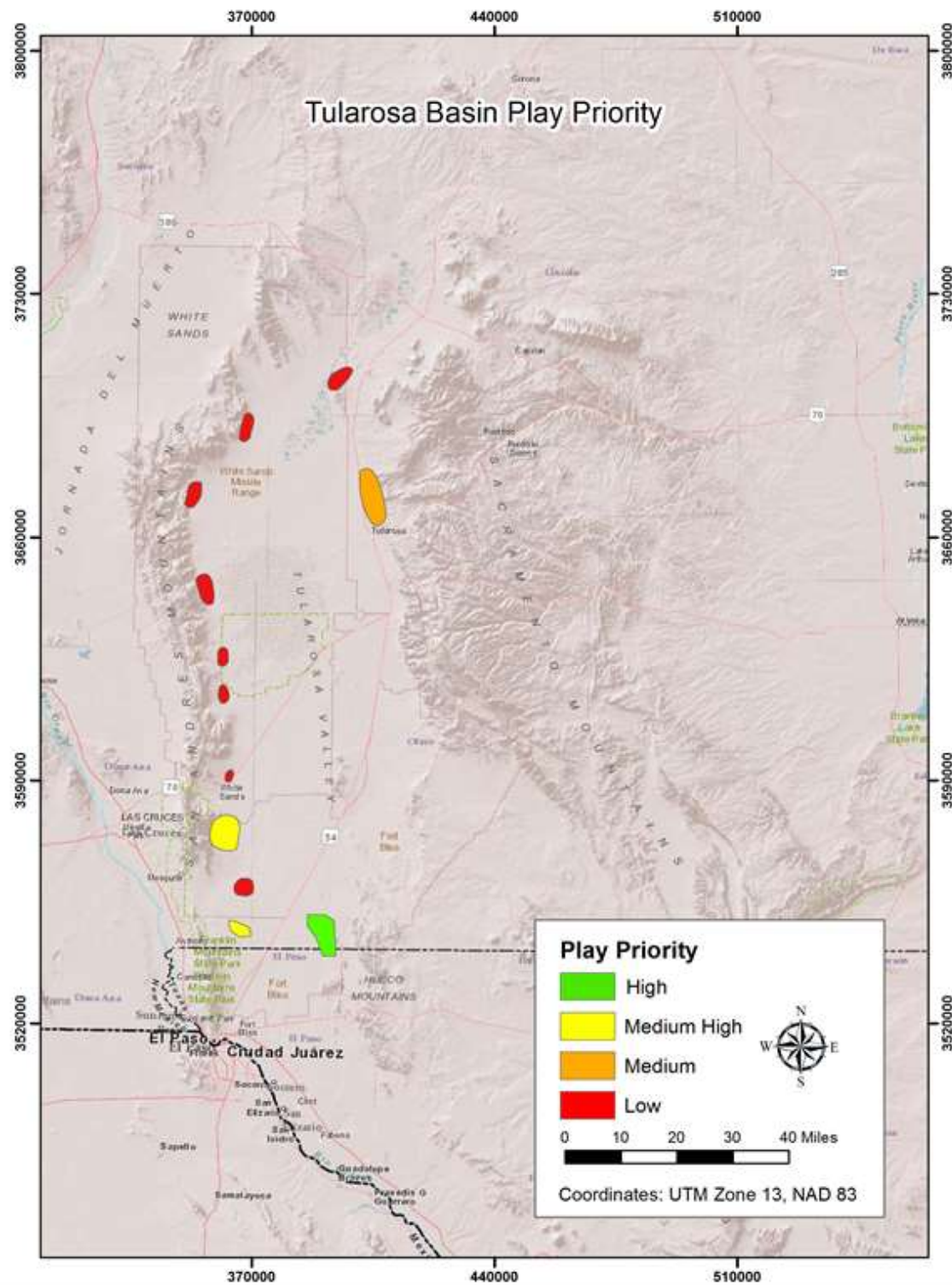
Figure 26. Play priority based upon structure, WoE probability, and proximity to permissible data points.
