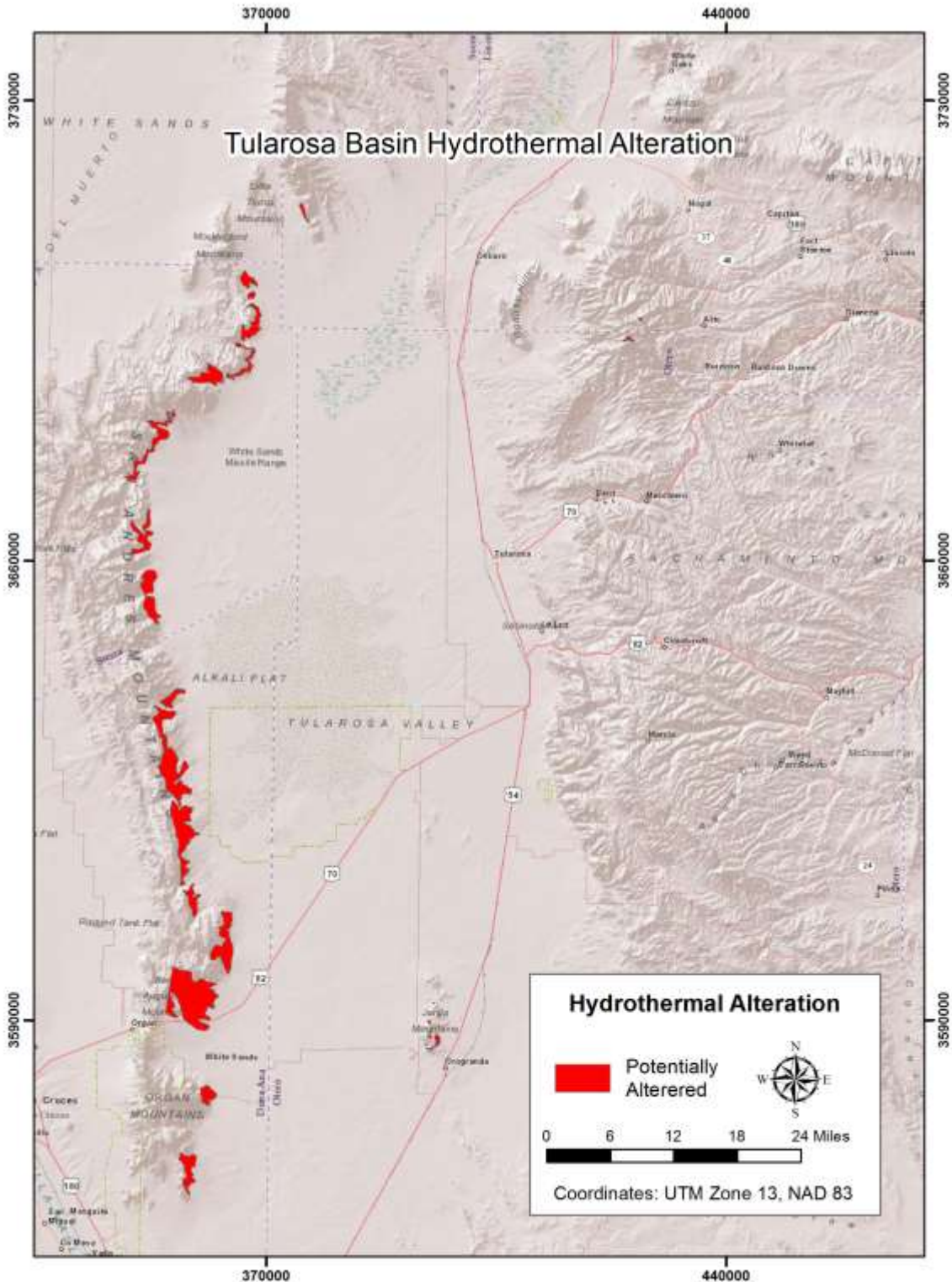
Figure 3. Hydrothermal alteration suggested by ASTER multispectral image analysis. The extensive areas on the west side of the valley are related to Mesoproterozoic granite, and may be from weathering or hydrothermal alteration or both.
