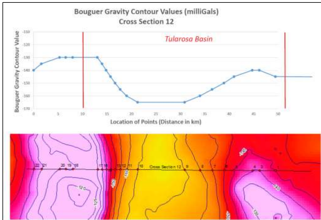
Figure 14. The profiles in this figure cross the basin between near the center of the Franklin Mountains. The gravity profile once again defines basin-bounding normal faults.
