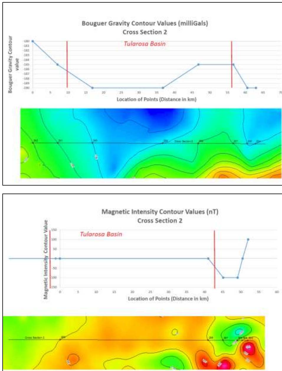
Figure 4. A gravity high (top) on the east side of the basin suggests a horst-like structure just outboard of the northern Sacramento Range that may be buried glide-block of primarily low-magnetic mineral sedimentary rock as suggested by the magnetic low covering part of the same area (bottom). The generally flat nature of the magnetic profile suggests a paucity of magnetic minerals and a sedimentary section in this part of the basin.
