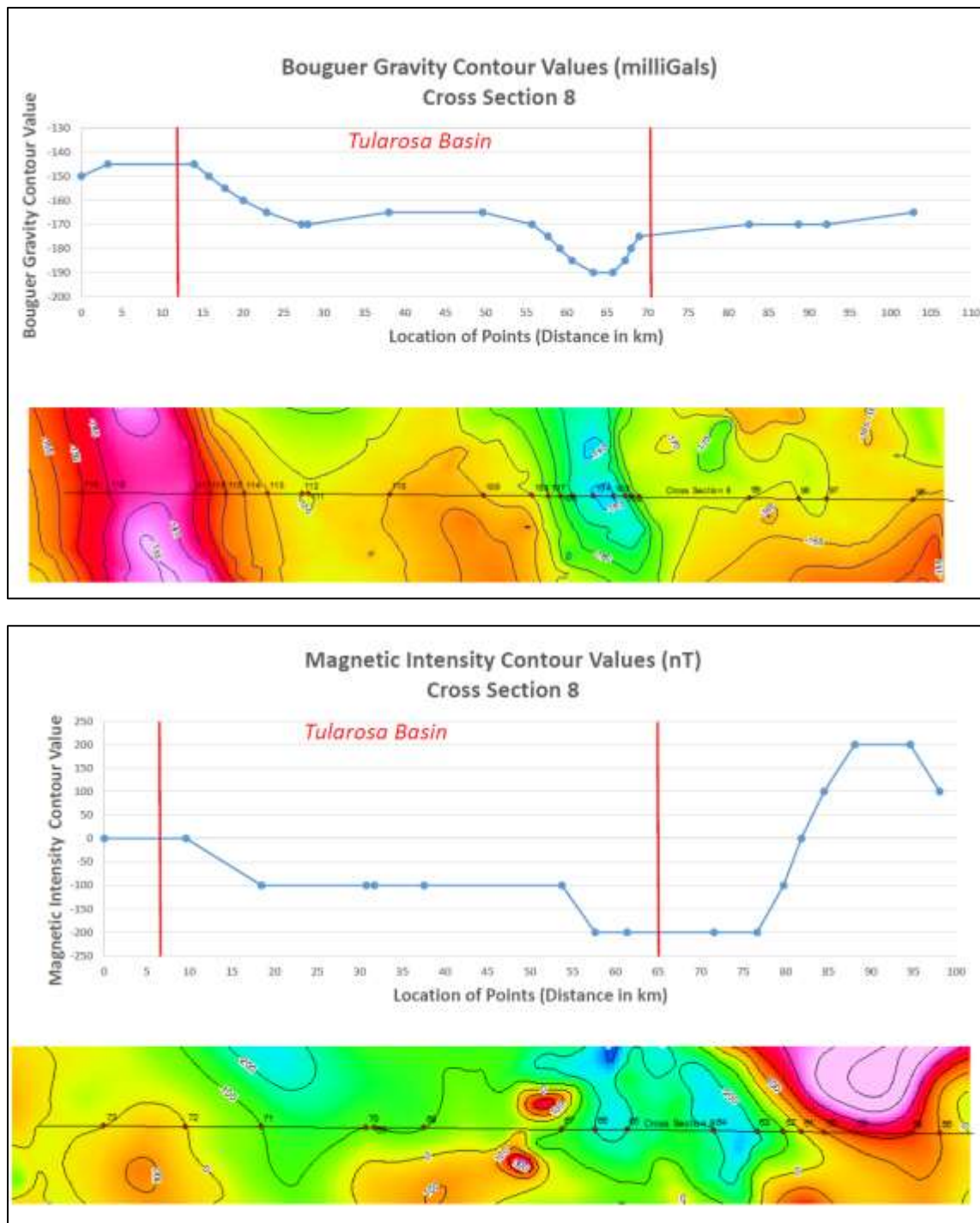
Figure 10. The gravity profile (top) continues to suggest a basement high, which may be an extension of the horst postulated in Figure 9. This is also suggested by the magnetic profile (bottom), although the western edge is truncated.
