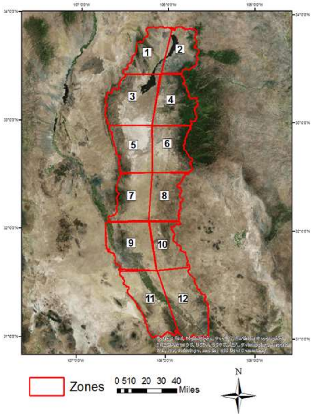
Figure 1. Tularosa Basin, divided into 12 zones for ZR ratio comparisons. Zone 8 and 10 have relatively high strain rates.
