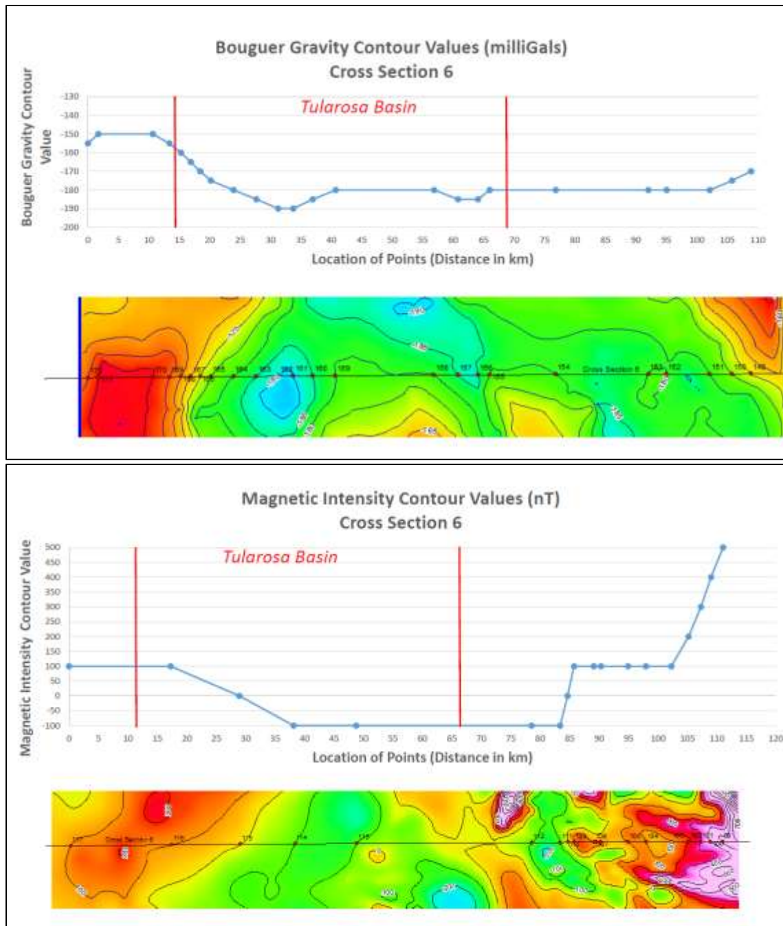
Figure 8. The gravity data profile (top) is relatively flat along the eastern basin margin with only a slight dip. This may be related to relatively young fault propagation of the Sacramento Range bounding faults in this area – a location where fault-tips are coalescing producing critical stress. A basement high is also apparent in the gravity profile. A well-developed east-dipping fault along the western basin margin is suggested by both data profiles.
