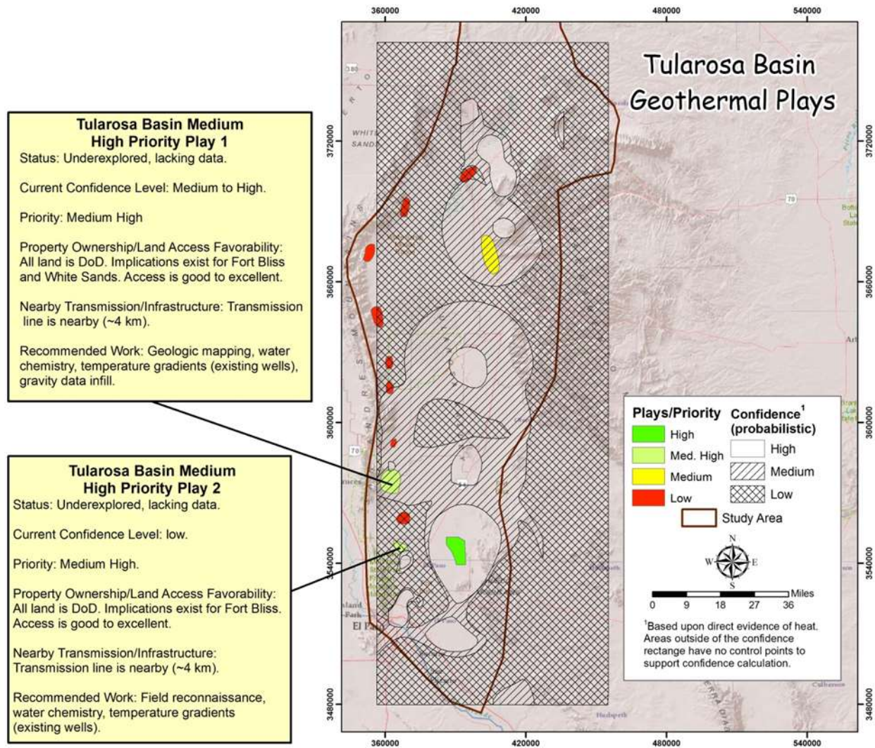
Figure 29. Suggested Phase 2 work for medium-high priority plays. Note that the southernmost play has low certainty which is largely due to a lack of data in the immediate area, so collecting more evidence of heat here would be recommended to raise certainty.
