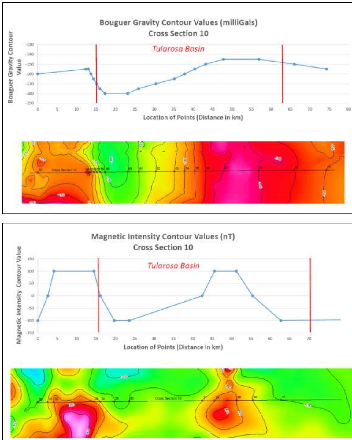
Figure 12. These profiles cross near the southern terminus of the Sacramento Range. The gravity profile has a steep gradient on the western basin margin, but the gradient on the eastern margin is significantly more gentle, suggesting less fault offset. The significant magnetic high on the eastern side of the bottom profile suggests an intrusion in the Sacramento Range and that seen to the west may result from Paleoproterozoic igneous rocks in the San Andreas Range.
