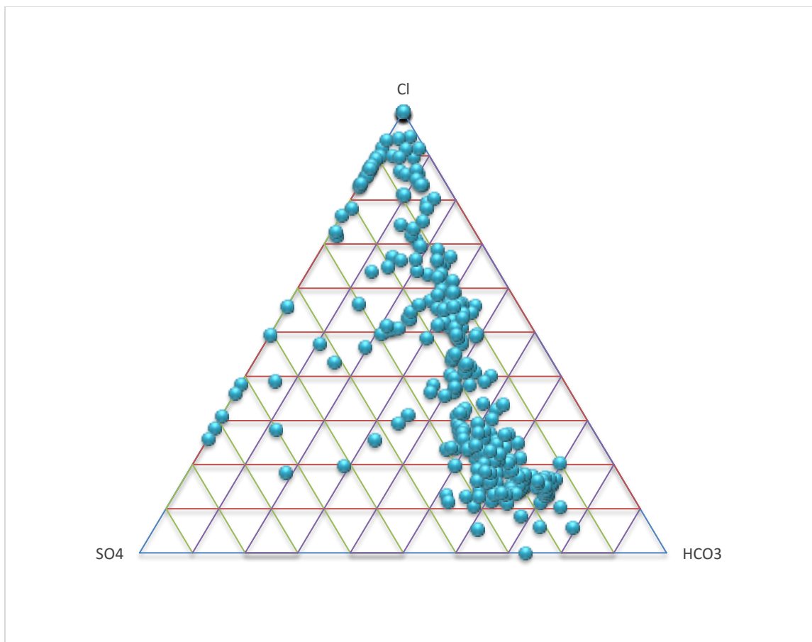
Fig. 6. Relative Cl-SO 4 -HCO 3 contents of waters from the southern region of the play fairway.
