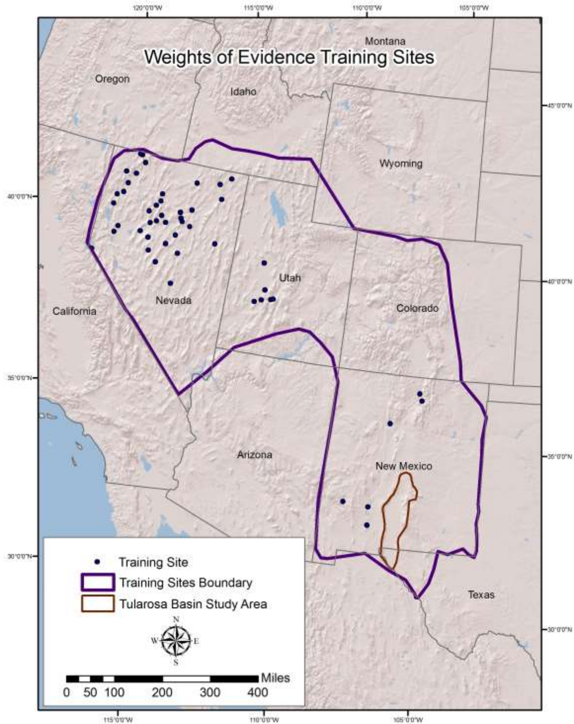
Figure 20. WoE training sites located at hot springs and known geothermal systems.
