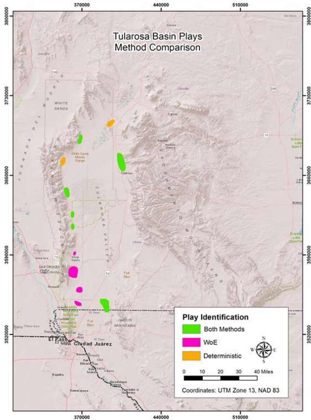
Figure 25. Plays identified by method. Twelve total plays were identified, six by both methods, two additionally by the deterministic method, and four additional by WoE.
