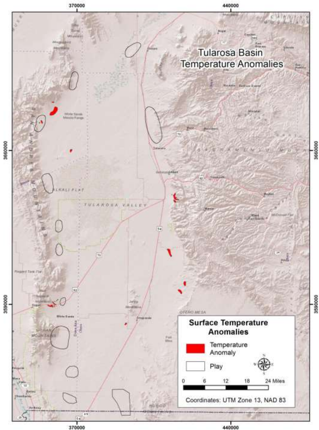
Figure 1. Surface temperature anomalies mapped from ASTER nighttime surface temperature data.
