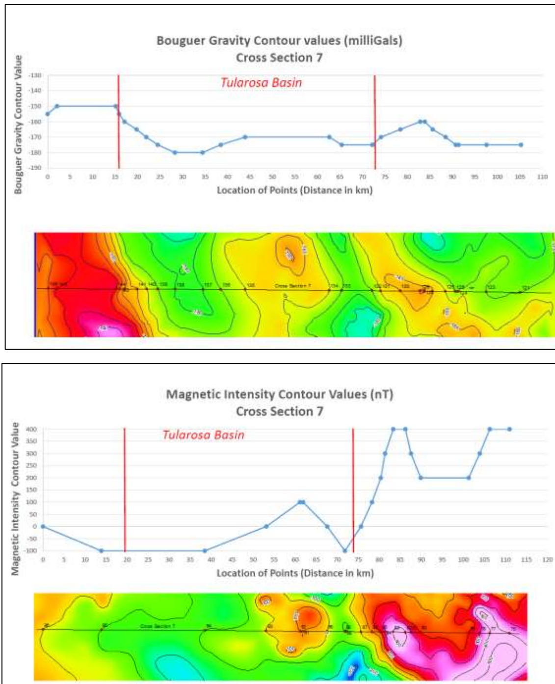
Figure 9. The gravity profile (top) again suggests normal faults bounding both the eastern and western margins of the basin. The basement high is more prominent than in Figure 8 suggesting a buried horst with faulting conjugate to the basin bounding faults. A magnetic high across part of the horst suggests that a portion of its lithology consist of volcanic, volcanoclastic, or intrusive rock. Both datasets suggest a basin flexure in this area, with fault-strikes changing from a predominantly NE direction to a NNW direction.
