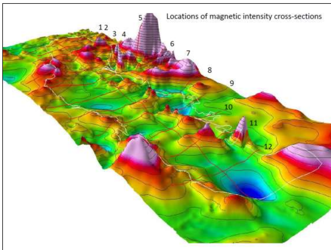
Figure 2. Locations of east-west cross sections for magnetic intensity contours, again indicating the presence of several sub-basins.
