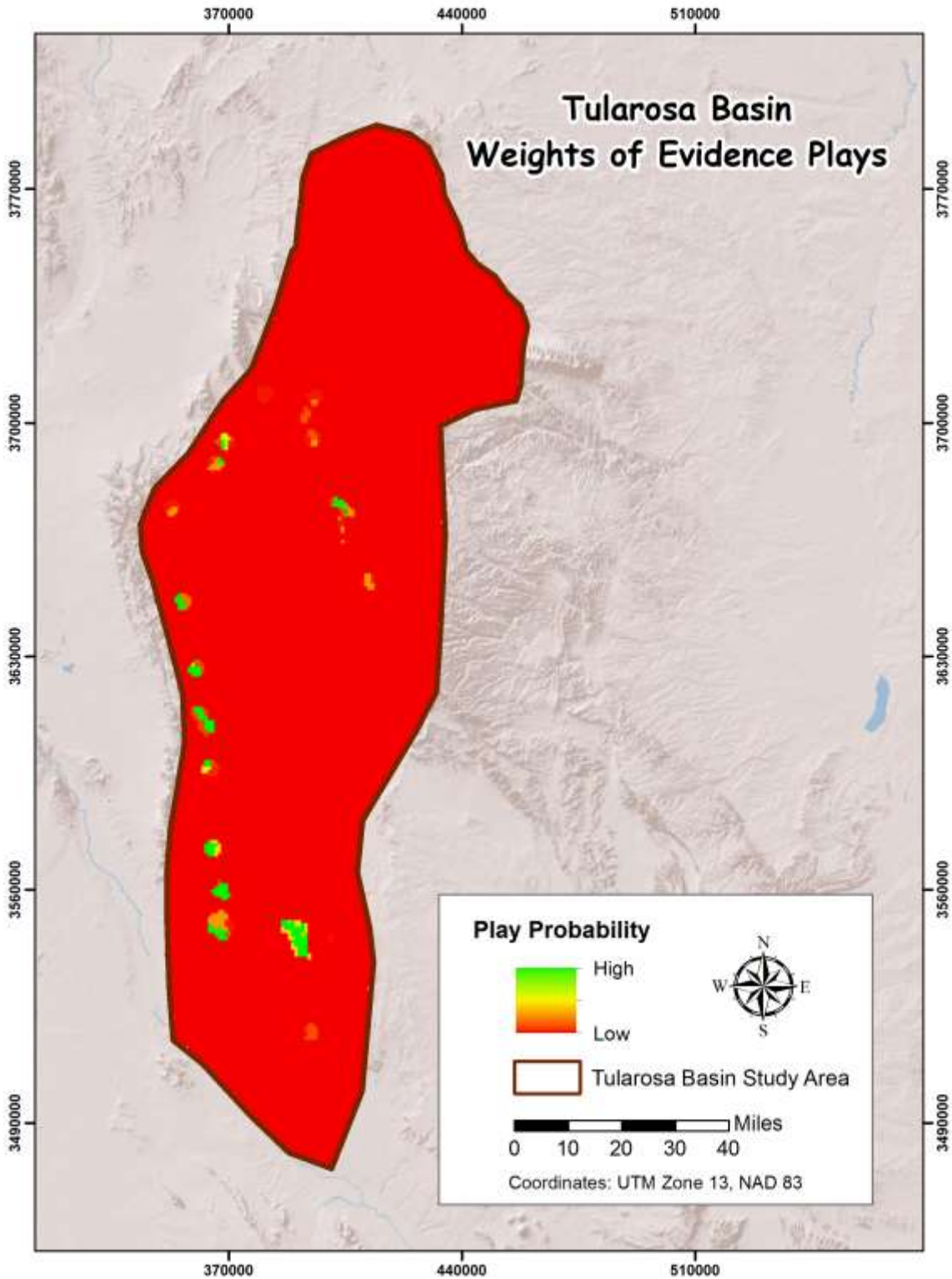
Figure 21. WoE final play probability map.
