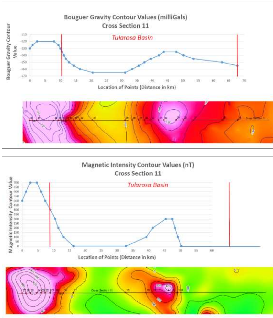
Figure 13. The profiles in this figure cross the basin between the San Andreas and Franklin Mountains. Both the gravity (top) and the Magnetic (bottom) data define basin-bounding normal faults.
