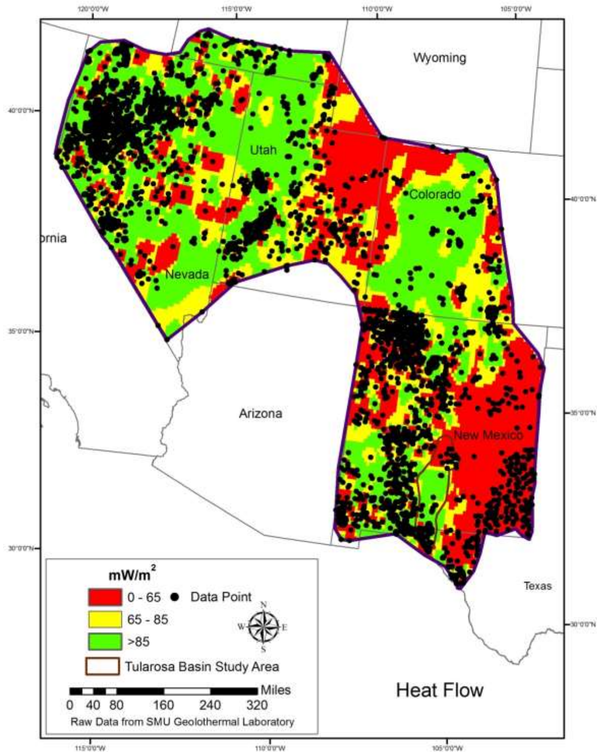
Figure 15. Heat flow evidential layer overlain with data points.
