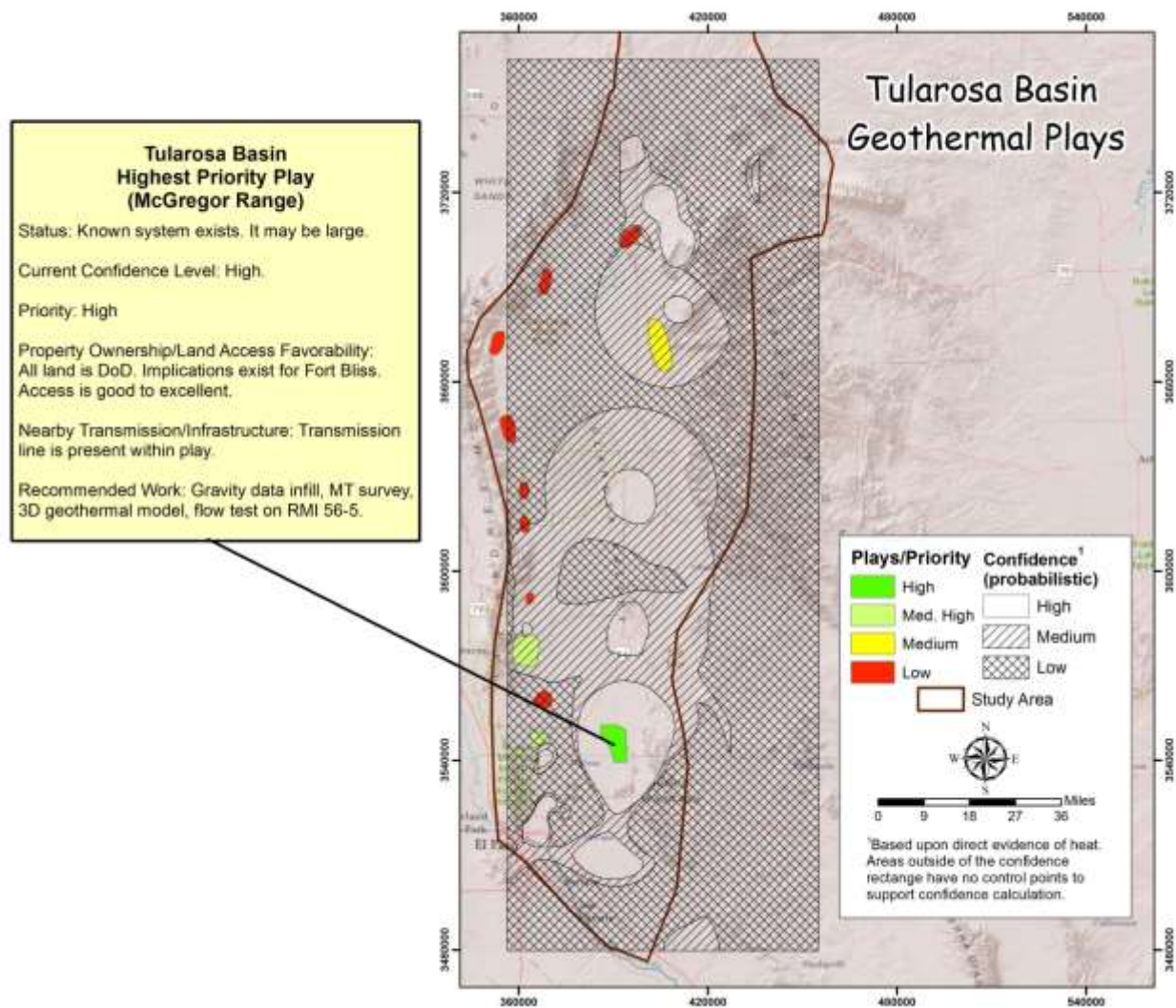
Figure 28. Phase 2 work suggested for the highest priority play.
