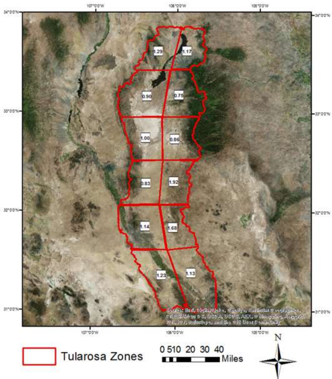
Figure 2. ZR Ratio values per zone. Higher values suggest greater strain and potentially better zones of permeability.
