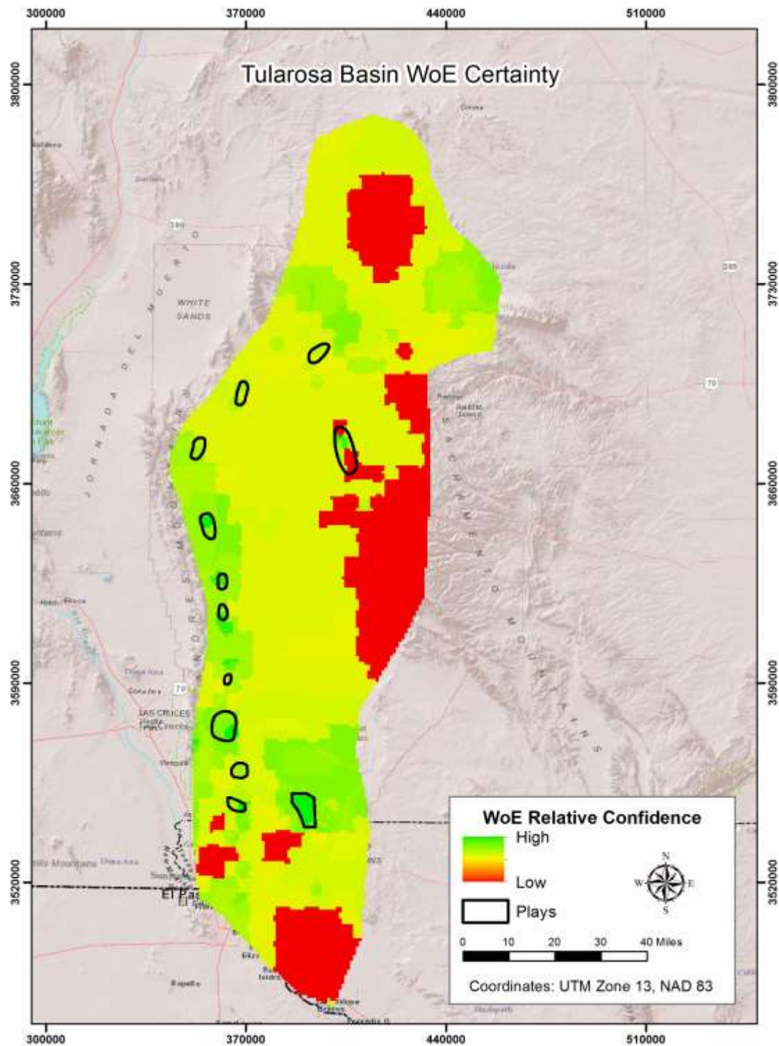
Figure 23. WoE confidence layer generated using the Spatial Data Modeler. All plays are in medium high to high confidence areas; although a single play also has low confidence areas included bounding a high confidence area.
