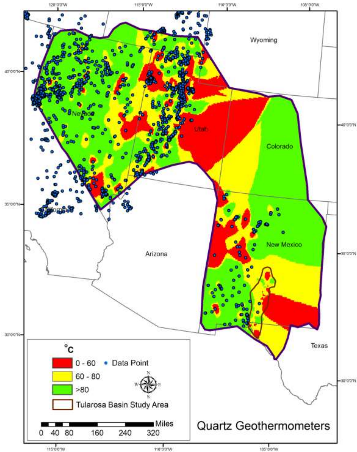
Figure 14. Quartz geothermometer evidential layer overlain with data points. Extrapolation was allowed beyond data points, but training area were all in data rich areas.
