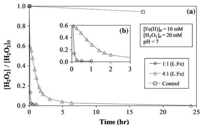
FIG. 4. (a) Role of ferrous iron (Fe(II)) on \text{H}_2\text{O}_2 decomposition with varying [\text{L}]:[\text{Fe}] molar ratio. L = \text{citrate} . (b) \text{H}_2\text{O}_2 decomposition for t = 0 to 3 \text{ h} .
