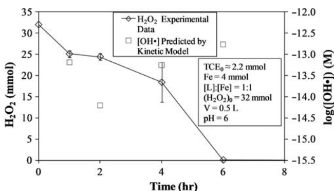
FIG. 8. \text{H}_2\text{O}_2 consumption and [\text{OH}\cdot] for proposed kinetic model using varying [\text{OH}\cdot] [Equation (32)].
