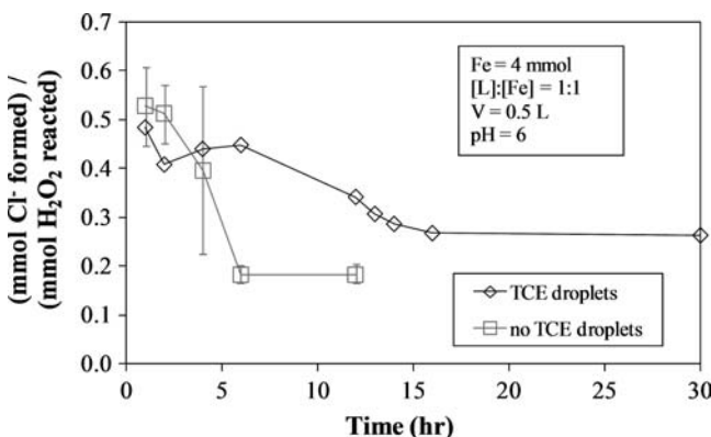
FIG. 13. (\text{mmol Cl}^- \text{ formed})/(\text{mmol H}_2\text{O}_2 \text{ reacted}) for one system containing no TCE droplets ( \text{TCE}_0 \approx 4 \text{ mmol} ) and one with TCE droplets ( \text{TCE}_0 \approx 16 \text{ mmol} ).
