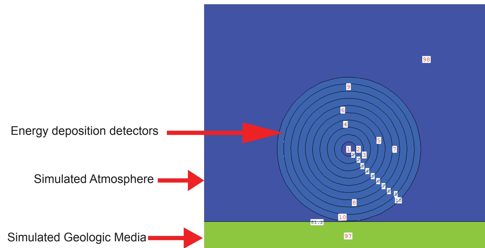
Figure 7: An x/z cross section of our generic model. 97 is our defined "unit" based on chemistry input. 98 is simply atmosphere above the geology. The series of nested spheres are filled with atmosphere and count energy deposition within them.
