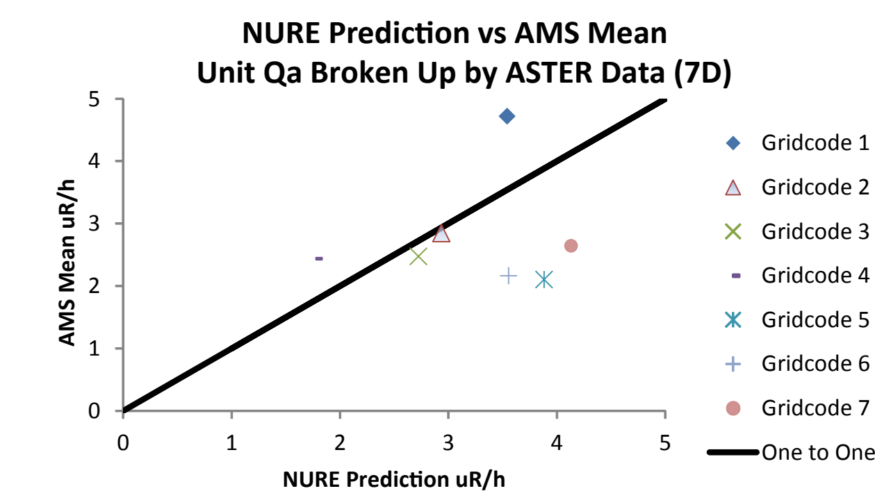
Figure 5B: This model of Government Wash uses the same geologic map as 5A and ASTER band ratio of 1/2 to track the distribution of ferric iron and break up the alluvial fan (Qa). NURE data is assigned to each unit based on location and an exposure rate is calculated using the Grasty Equation. The plot above shows the relationship between our prediction and the aerial survey in the broken up alluvial fan.
