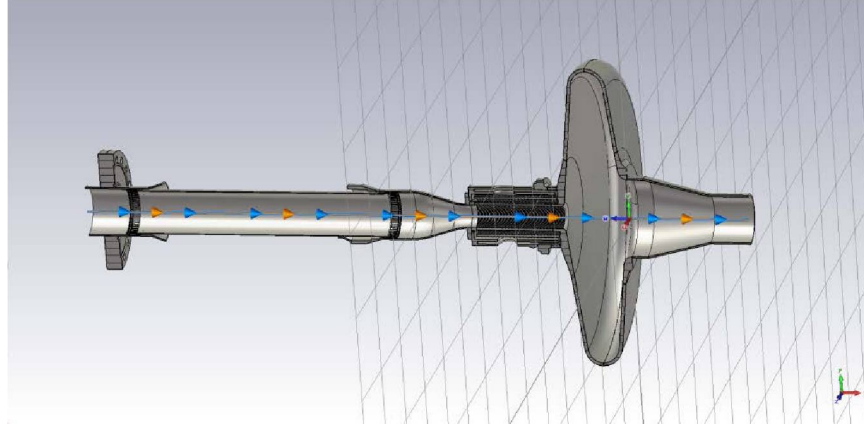
Figure 3: Simplified booster cavity structure in CST simulation.
