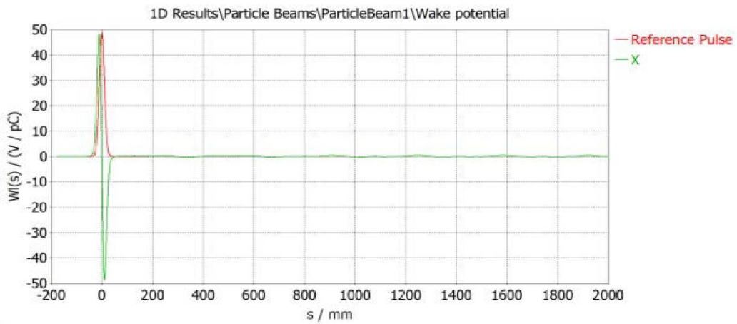
Figure 4: The longitudinal wake potential, denoted by X and shown in green, of the booster cavity with \beta=0.8279 .
