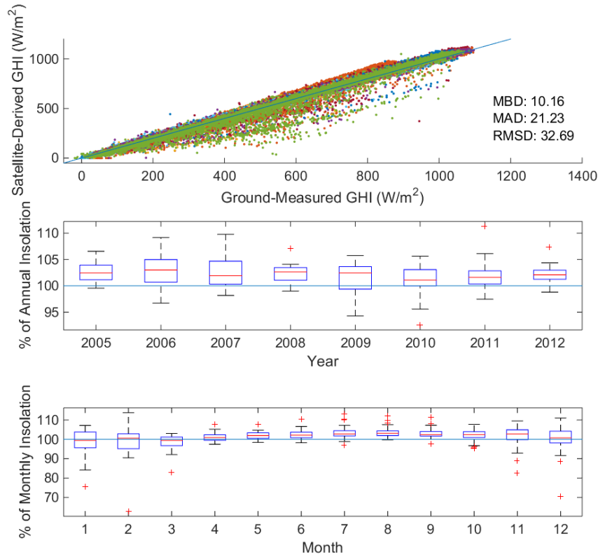
Figure 2. Annual insolation ratios (NSRDB GHI to ground GHI) for clear sky periods.
