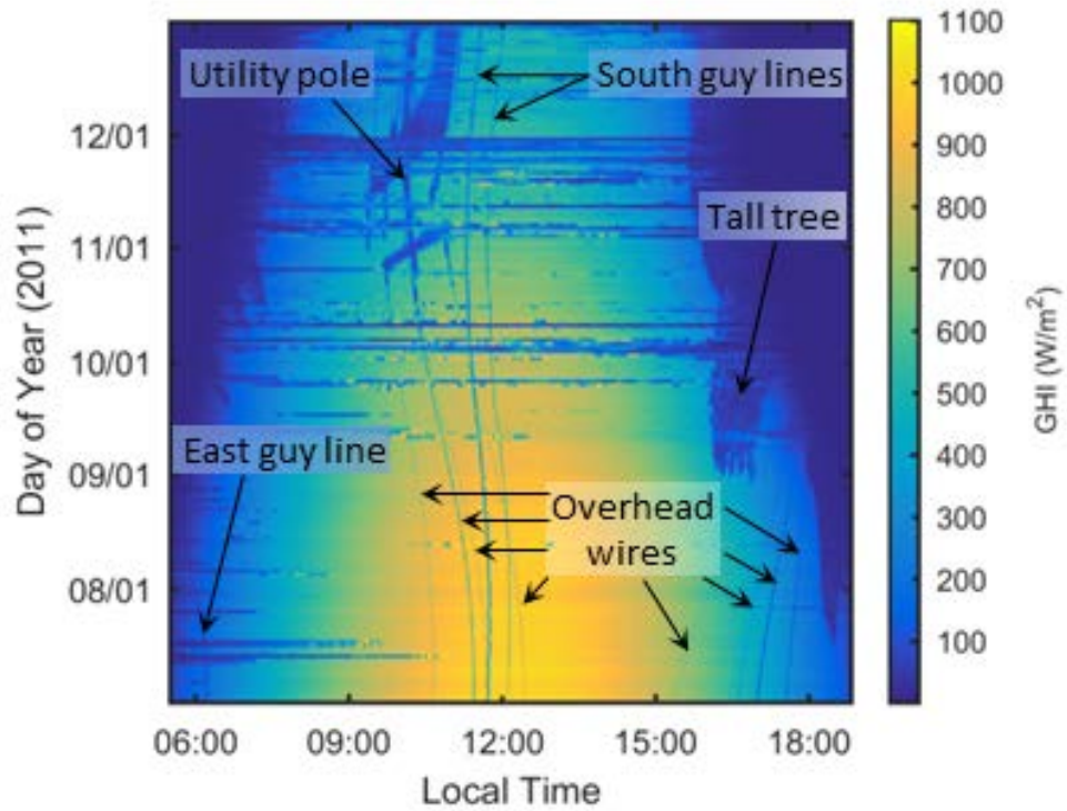
Figure 3. Google Street View image of SMUD station 22 with instrument circled (a); shadows evident in GHI data in image format (b).
