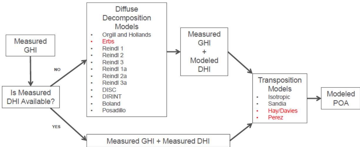
Figure 6. Models considered in our evaluation of GHI to POA irradiance modeling.
