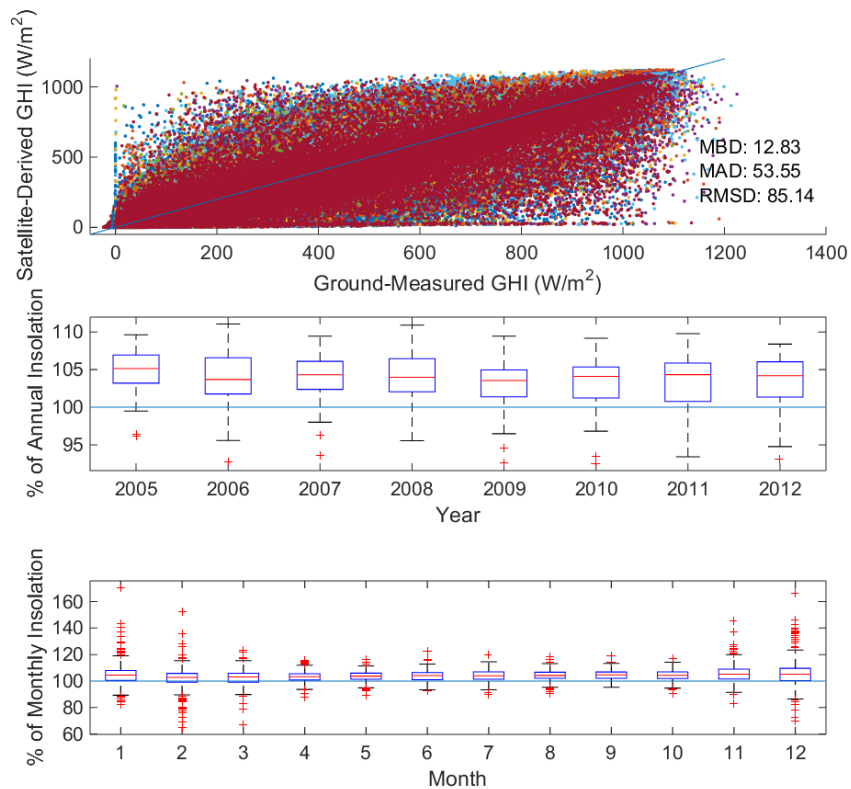
Figure 1. Ratios of NSRDB to ground GHI across 43 locations.
