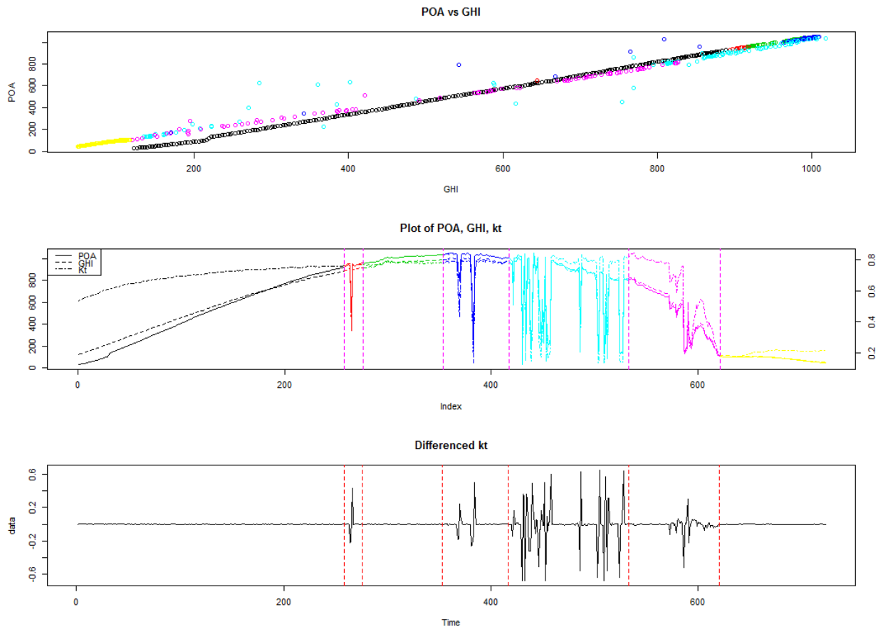
Figure 7. Example data used in exploration of GHI to POA modeling technique, showing GHI to POA comparison (top), partitioning of GHI (middle), and characteristics of differenced kt within each partition element (bottom).
