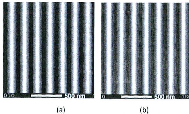
Fig. 13 Actinic images of 26nm L/S. \text{NA}=0.42 , \sigma=0.3 , (a) exposure time = 5 seconds; (b) exposure time = 30 seconds.
