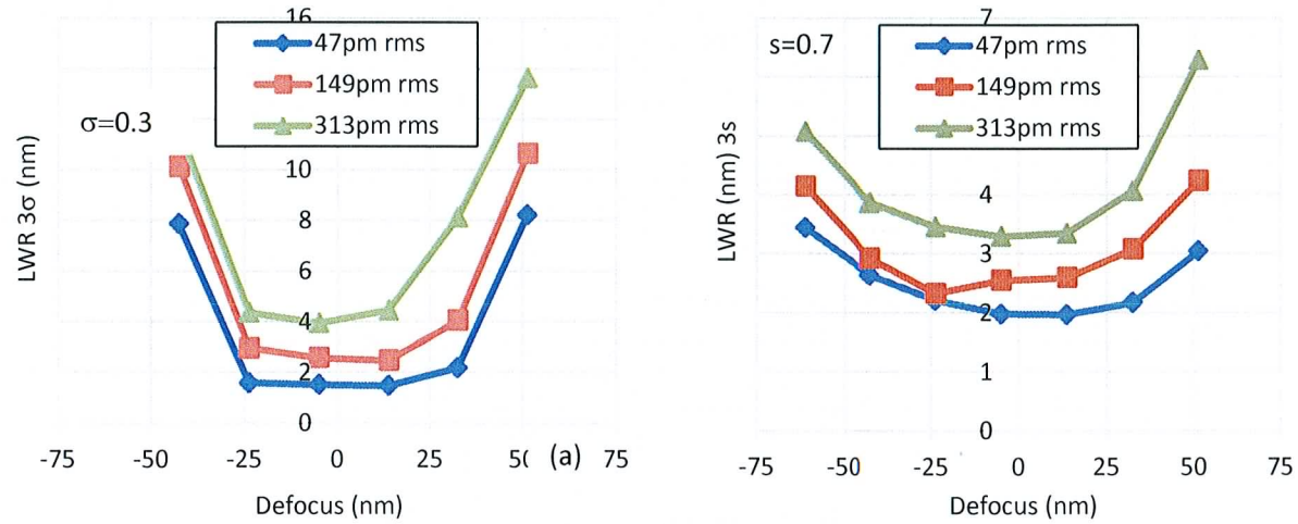
Fig. 10 Plot of LWR as function of defocus for three different ML RSR surface roughness values, (a) for \sigma=0.3 and (b) \sigma=0.7 . The feature size is 20nm and NA used is 0.42. The data collection exposure time is 5 seconds.
