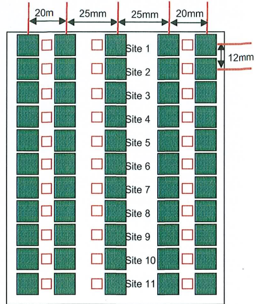
Fig. 5 Schematics of mask pattern layout.
