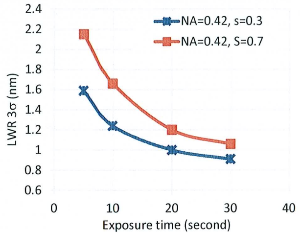
Fig. 14 Plot of 26nm L/S LWR as function exposure time for NA= 0.42, \sigma=0.3 and 0.7, respectively.
