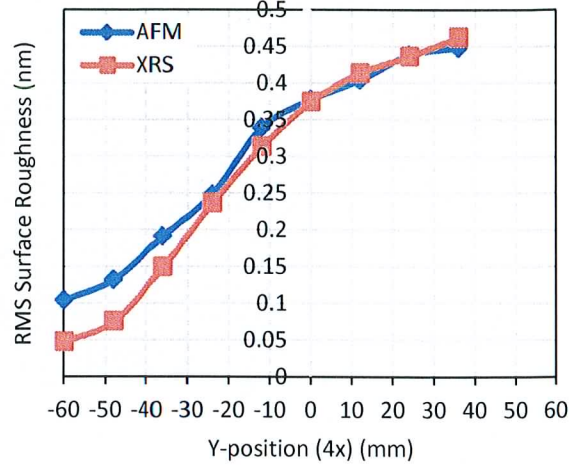
Fig. 4 AFM and EUV scatterometry determined RMS surface roughness as a function of mask y-positions.
