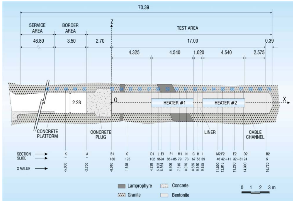
Figure 3-4. The initial configuration of FEBEX in situ test at the Grimsel underground laboratory (Switzerland) (ENRESA, 2000).
