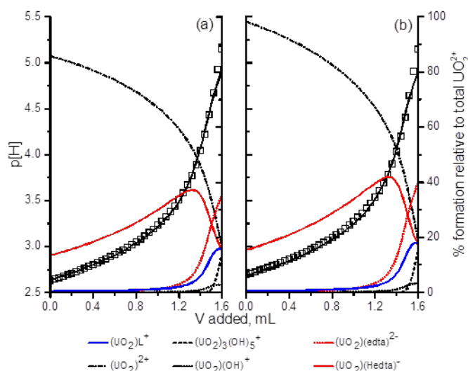
Figure 1. Potentiometric titrations for the complexation of \text{U(VI)} with \text{HL}^{\text{III}} . Left axis: \text{p[H]} , \square experimental, - calculated. The full black curve is calculated by using the protonation constants in Table 1. Right axis: speciation of \text{U(VI)} . Conditions: (a) C_{\text{U}}^0 = 0.46 mM, C_{\text{H}}^0 = 4.82 mM, C_{\text{L}}^0 = 1.95 mM, C_{\text{edta}}^0 = 0.23 mM, C_{\text{OH}}^{\text{titr.}} = 20.0 mM; (b) C_{\text{U}}^0 = 0.41 mM, C_{\text{H}}^0 = 3.75 mM, C_{\text{L}}^0 = 1.21 mM, C_{\text{edta}}^0 = 0.21 mM, C_{\text{OH}}^{\text{titr.}} = 20.0 mM.
