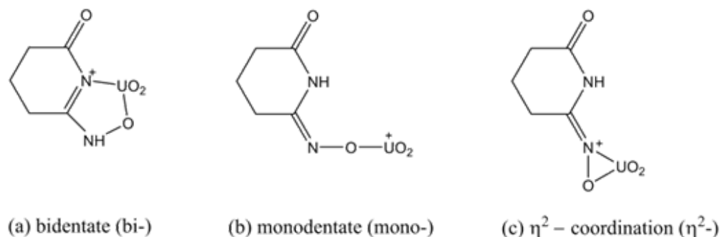
Figure 2. Possible coordination modes between \text{HL}^{\text{III}} and \text{UO}_2^{2+} .
