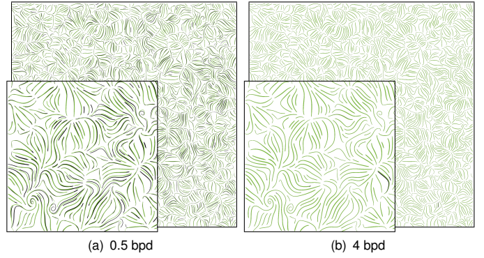
Fig. 9: Streamlines extracted from compressed Rayleigh-Taylor velocity fields. The green lines from each compressed field overlay the black lines from the uncompressed field.
