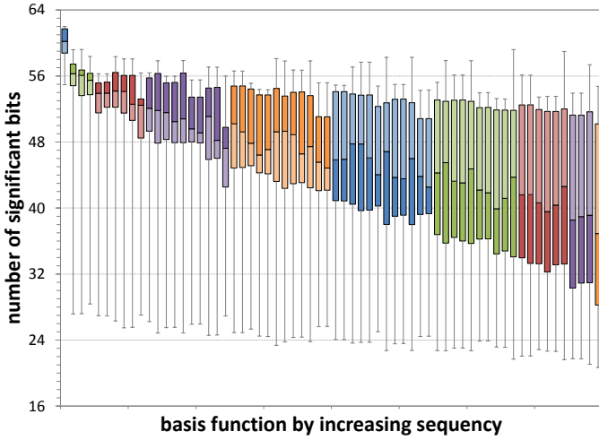
Fig. 3: Box plot showing the distributions of the number of significant bits for the coefficients associated with the 64 basis functions (grouped and color coded by frequency) based on data from 30 different fields. This plot confirms that the energy is concentrated in the low frequencies.
