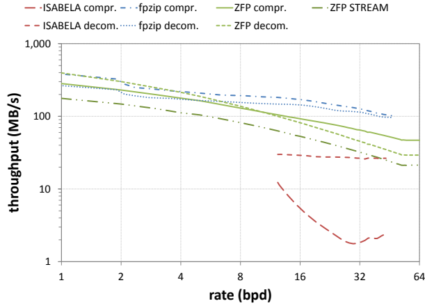
Fig. 6: Raw compression and decompression throughput in number of uncompressed bytes input or output per second. Higher rates require more bit plane passes in ZFP and thus more time.
