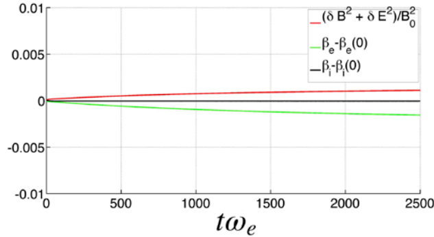
Figure 1: Results of a run with no initial fluctuation energy, quantifying the numerical effects on particle heating. The electromagnetic (red), electron (green) and ion (black) energy densities normalized by the background magnetic field energy density are shown.
