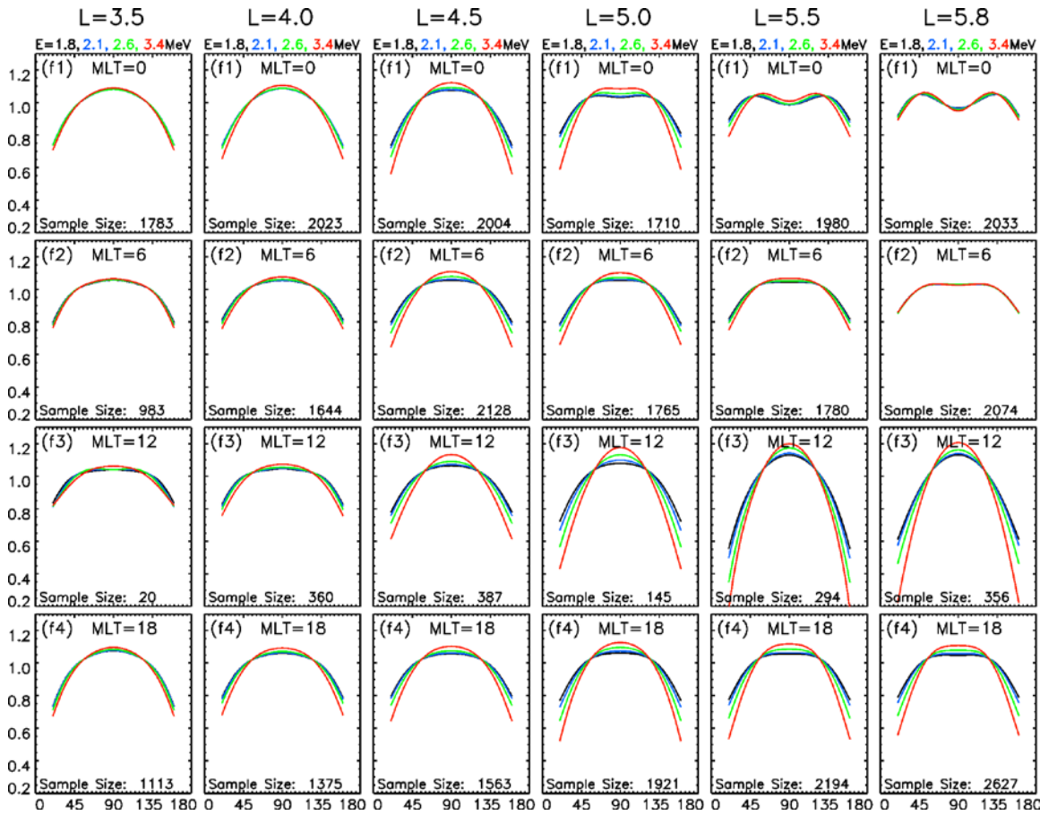
Figure 1. The averaged PADs of 1.8, 2.1, 2.6, and 3.4 MeV electrons as a function of L and MLT, reconstructed from the statistical relativistic electron PAD model.
