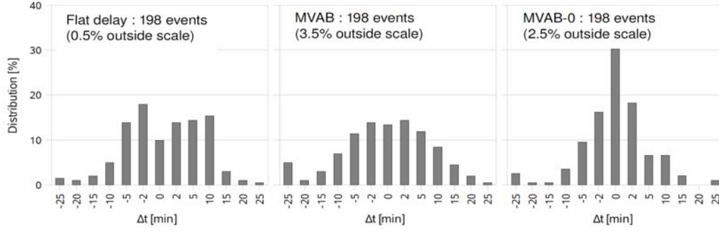
Figure 4: A comparison of the error in the arrival time between different methods (flat delay, MVAB, and MVAB-0) for calculating the solar wind time delay [adapted from Mailyan et al. [17]]
