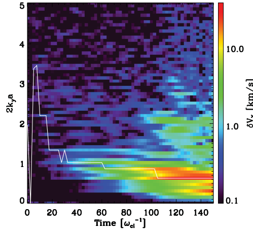
Figure 4: Temporal evolution of the spatial Fourier spectrum of perpendicular velocity disturbance at X = 0 .
