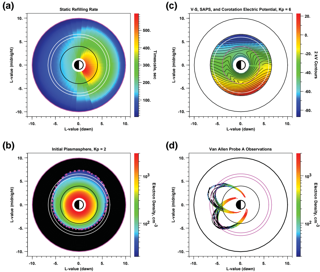
Figure 1: Overview of the equatorial plasmaspheric electron density model, RAM-CPL, used in this study with each plot presented in SM-equatorial coordinates with the sun to the right and earth at center and circles drawn at 4, 6, 6.6, and 10 R_E . The simulations are initialized at a resolution of .25 L by .5 MLT with an extended plasmasphere (b) that is specified by refilling the system to saturation during geomagnetically quiet conditions ( K_p < 2 ). Empirical models of outgoing particle flux from the ionosphere yield the diurnally dependent rate of refilling (a), which is effective on the dayside. The evolution of plasmaspheric densities driven by \mathbf{E} \times \mathbf{B} convective erosion is described by a Volland-Stern and Subauroral Polarization Stream (SAP) electric potential (c) parameterized by the solar wind and K_p . Simulations are restricted from 1.75 < L < 6.5 to compare with the limits of Van Allen Probes EMFISIS density observations shown for RBSP-A in panel (d) where 31 May - 5 June, 2013 observations occur in the pre-midnight magnetic local time sector while 15 - 20 January, 2013 observations fall in the post-midnight sector. A low-density threshold ( 20 \text{ cm}^{-3} ) plasmapause is indicated by the broken magenta line surrounding (b) the initial two-dimensional plasmasphere for illustration.
