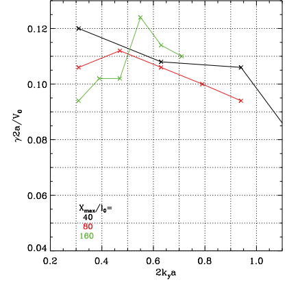
Figure 10: KHI growth rate with wavenumber for different system sizes: X_{max} = 40 l_0 (black), 80 l_0 (red), and 160 l_0 (green).
