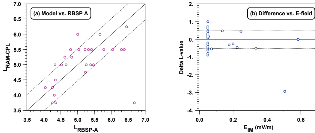
Figure 6: Simulated plasmapause locations versus actual plasmapause locations on 15 - 20 January, 2013 with respect to their correspondence (a) and correlation (b) with the driving inner magnetospheric electric field, E_{IM} . Greater disagreement was found during quieter conditions.
