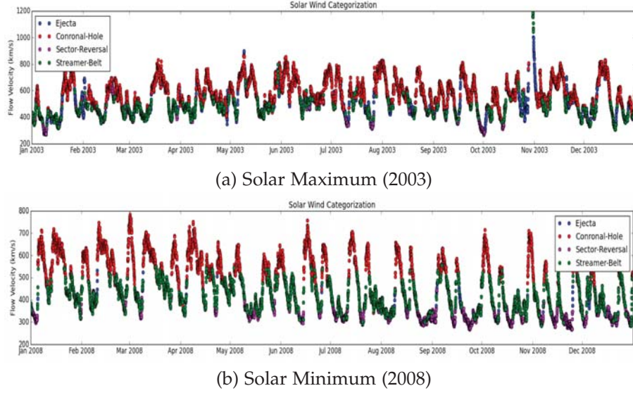
Figure 2: Testing solar wind data in OMNI dataset against 4-categorization scheme during (a) solar maximum and (b) solar minimum conditions. The wind categorizations are indicated in the figure legend.
