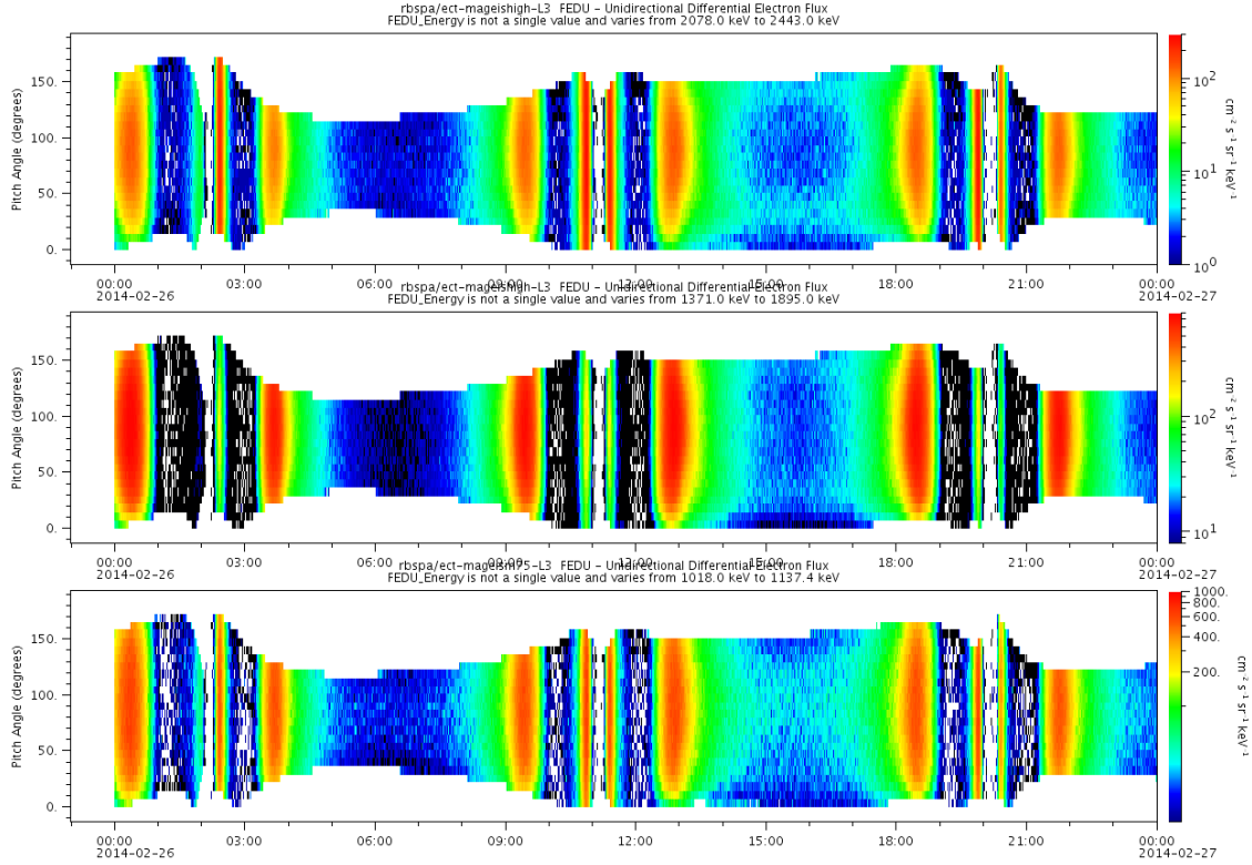
Figure 4. The PADs of ~2.3, 1.6, and 1 MeV electrons on 26 Feb 2014 measured by MagEIS on the Van Allen Probe-A.
