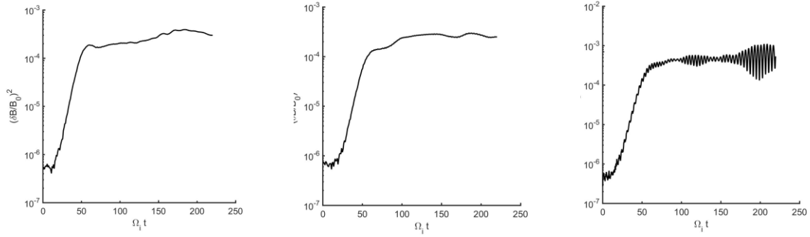
Figure 3: Energy-history of (left) Run I, (centre) Run II, (right) Run III
