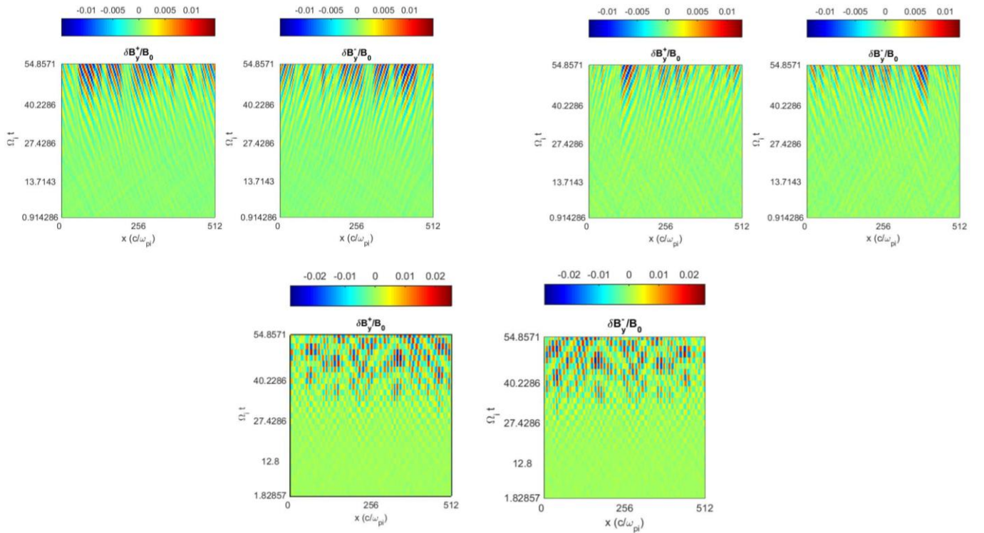
Figure 4: Positive and negative helical components for (top-left) Run I, (top-right) Run II, and (bottom) Run III
