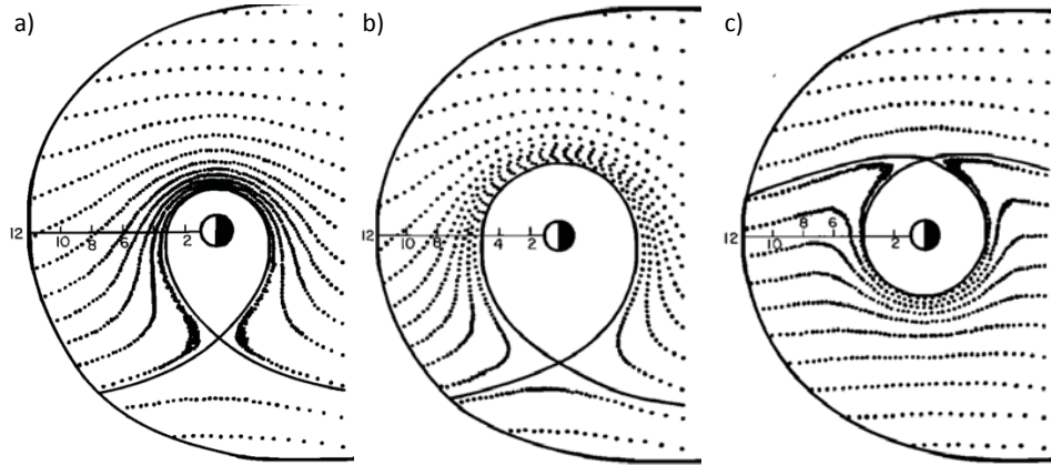
Figure 1: Particle drift paths for a) \gamma\mu = 0 . Low energy particles of both species are dominated by electric field drifts. They have the stagnation point at dusk. b) electrons with \gamma\mu = 0.05\text{keV}/\gamma . c) protons with \gamma\mu = 0.05\text{keV}/\gamma . (where \gamma = 1 \times 10^{-9} T) (Kavanagh et al., 1968).
