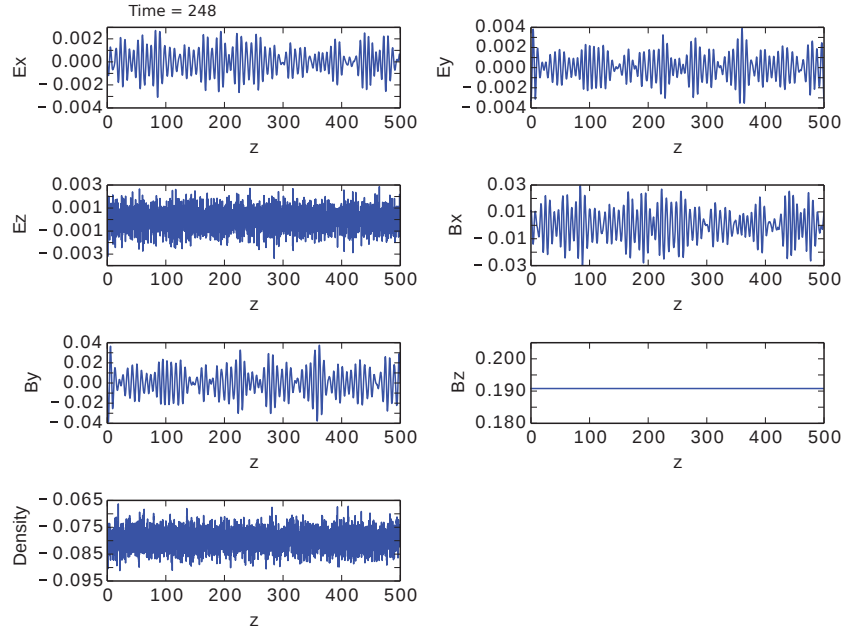
Figure 1: The generation of whistler wave on 1D grid with uniform background magnetic field. Results at t = 248\Omega_{ce}^{-1} are shown. The unit of length is c/\omega_{pe} . Note that all the values are in normalized units.
