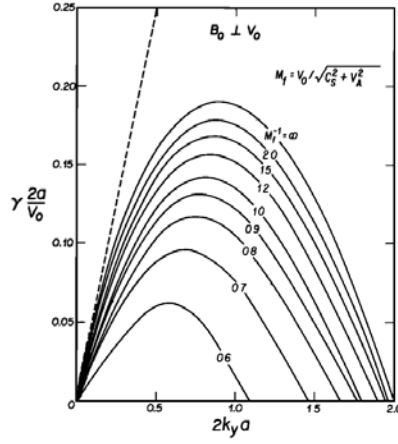
Figure 1: Normalized growth rate dependence on the normalized wavenumber for inverse magnetosonic Mach numbers ranging from 0.6 to \infty from the eigen-mode analysis of Miura and Pritchett (1982).
