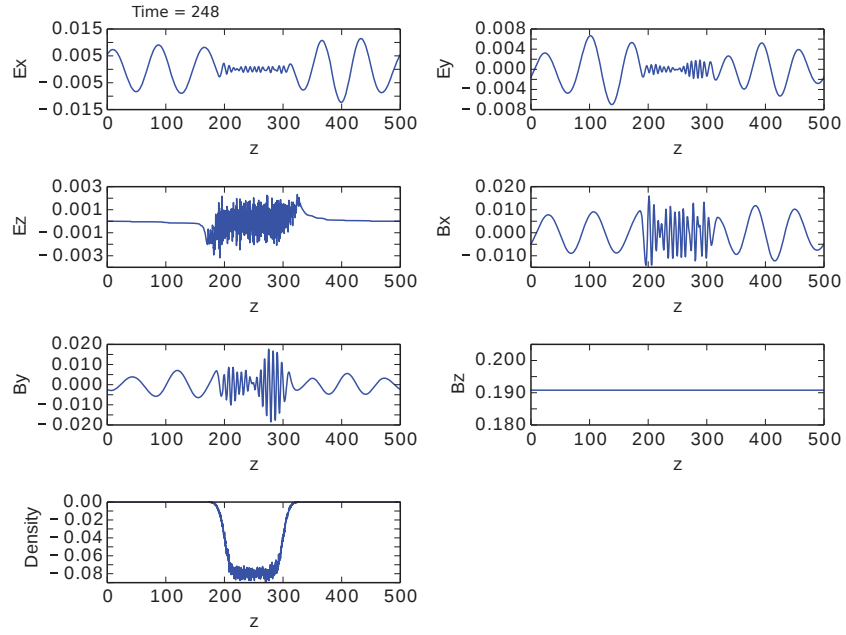
Figure 3: Simulation results at t = 248\Omega_{ce}^{-1} for locally distributed plasma.
