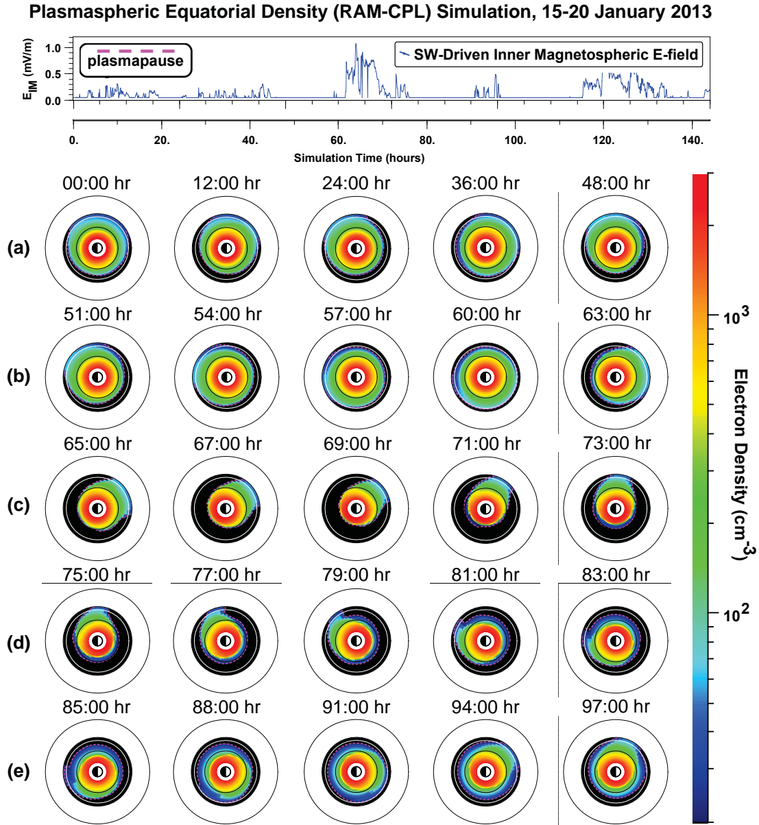
Figure 3: Summary of RAM-CPL simulation for the post-midnight event on 15 - 20 January, 2013. Each dial plot is presented in the SM-coordinate equatorial system with the sun at right and the earth at center. Circles drawn provide an approximate indication of radial distance for 4, 6, 6.6, and 10 L. Each timestamp above the output dial gives the number of hours since the initialization of the equatorial plasmaspheric density model on 00:00 UT 15 January, 2013. The hours during storm onset between 63:00 and 97:00 as indicated by the panel of the solar wind driven inner magnetospheric electric field parameterizing a Volland-Stern convection potential show the formation of a narrow extension of plasma on the dayside that subsequently corotates with the main body of the plasmasphere as the level of geomagnetic activity subsides.
