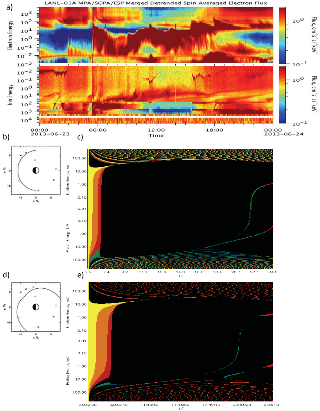
Figure 6: a) Detrended differential electron and proton flux on 23 June 2013 for LANL-01A which is at \sim 18:30 MLT at the time of injection. At this satellite a dispersionless injection is also observed at 05:24 UT. b) The injection boundary used for the modelled dispersion pattern in c) . c) The modelled dispersion pattern where the colours indicate whether a particle from the injection region has access to the satellite at a particular time and if so, the MLT sector from which the particle originates. d) The double spiral rotated by \pi/4 injection boundary used in e) for the modelled dispersion pattern. e) The modelled dispersion pattern using a rotated injection boundary. The axes for the observations and models are in the same layout as Figure 3.
