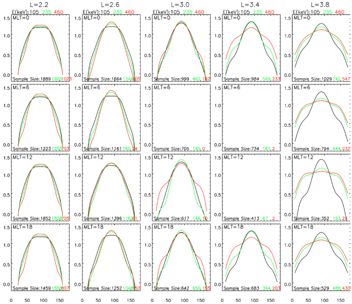
Figure 6. Similar format with Figure 5 but for results in the slot region.
