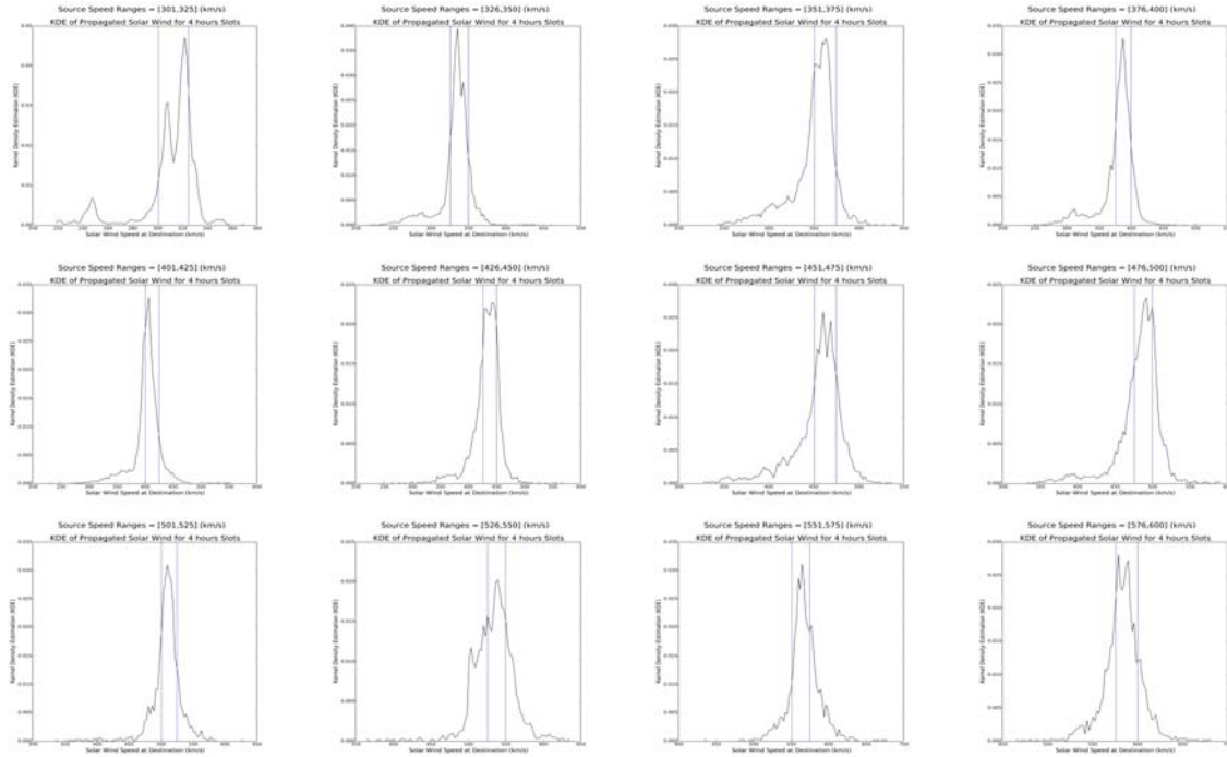
Figure 7: Uncategorized Kernel Density Estimation (KDE) functions of solar wind wind that are measured at IMP8 spacecraft based on three years of advected measurements from ACE spacecraft to the IMP8 location using the flat-delay method. The vertical blue lines represent the interval of solar wind speeds measured at ACE.
