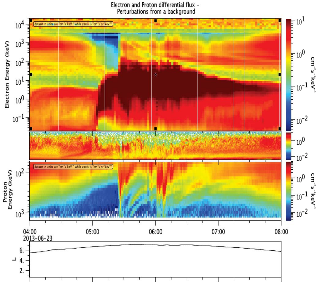
Figure 3: Dispersionless injection observed by Van Allen Probe A on 23 June 2013 at 05:24 UT. Top panel- detrended differential electron flux observed from HOPE, MagEIS and REPT instruments. Middle two panels- detrended differential proton flux observed from HOPE, MagEIS and REPT instruments. Note unconventional plot axes- electron energy increasing upwards and proton energy increasing downwards. Bottom panel- satellite L-shell.
