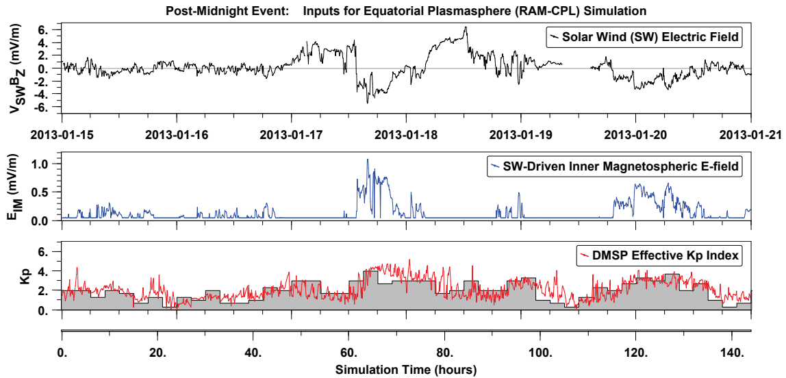
Figure 2: Geomagnetic conditions for the post-midnight event on 15 January, 2013 used to as inputs to drive \mathbf{E} \times \mathbf{B} erosion in the RAM-CPL simulations considered here. The solar wind electric field V_{SW}B_{Z,IMF} (from OMNI data) is scaled as described in the text to produce an inner magnetospheric electric field E_{IM} to parameterize a Volland-Stern model for convection. Asymmetric and enhanced flows are included by the addition of an analytical SAPS electric field component whose strength varies by the effective K_p index derived from DMSP with the 3-hour K_p geomagnetic activity index shown for reference.
