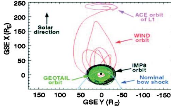
Figure 5: Comparison of the location of ACE and IMP8 in the heliosphere to other spacecraft such as WIND and Geotail. ACE stays in its halo orbit at the first Lagrangian point and IMP8 orbits the Earth and stays outside the nominal bow shock location most of its orbital time. [Adapted after Haggerty et al. [12]]
