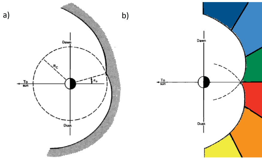
Figure 2: a) Proposed double spiral injection boundary behind which all particles are energised at the time of injection (Mauk and Meng, 1983). b) Injection boundary with colour coded MLT sections. The colours indicated are used to show the location of particle origin. If the initial particle position in local time is: 18:00-20:00 yellow, 20:00-22:00 orange, 22:00-00:00 red, 00:00-02:00 green, 02:00- 04:00 light blue, 04:00-06:00 dark blue (adapted from Mauk and Meng (1983)).
