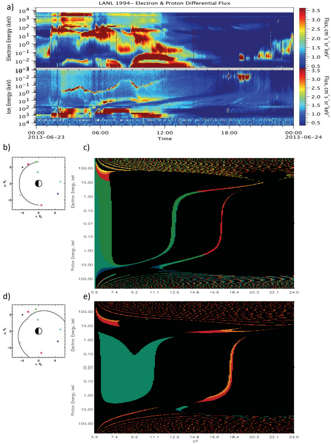
Figure 7: a) Detrended differential electron and proton flux on 23 June 2013 for 1994-084 which is located at \sim 02:00 MLT at the time of injection. At this satellite no obvious flux enhancement is observed at the time of injection even though the spacecraft is located behind the injection boundary dispersion less injection is expected. b) The injection boundary used for the modelled dispersion pattern in c) . c) The modelled dispersion pattern where the colours indicate whether a particle from the injection region has access to the satellite at a particular time and if so, the MLT sector from which the particle originates. d) The double spiral rotated by \pi/4 injection boundary used in e) for the modelled dispersion pattern. e) The modelled dispersion pattern using a rotated injection boundary. The axes for the observations and models are in the same layout as Figure 3.
