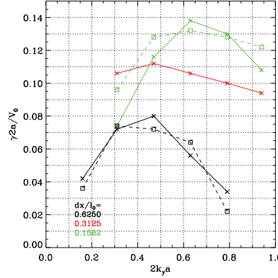
Figure 9: KHI growth rate with wavenumber for different grid spacings: dx = 0.6250 (black), 0.3125 (red), and 0.1562 (green).
