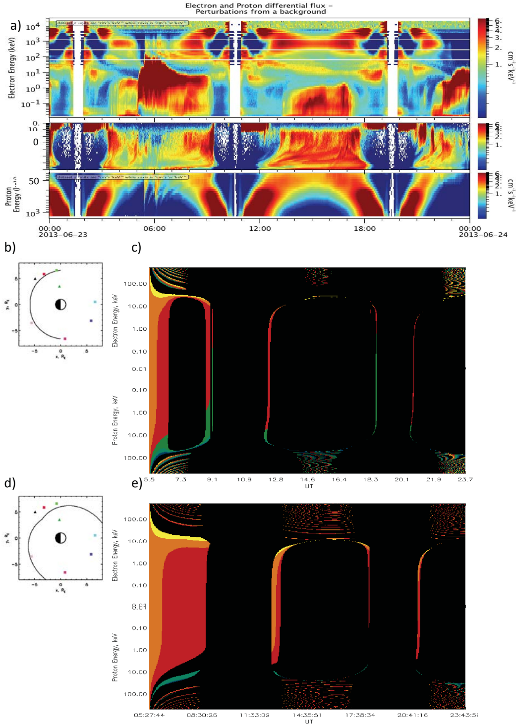
Figure 5: a) Detrended differential electron and proton flux on 23 June 2013 for Van Allen Probe A which is at \sim 21:00 MLT at the time of injection. The dispersionless injection is visible at 05:24UT. b) The injection boundary used for the modelled dispersion pattern in c) . c) The modelled dispersion pattern where the colours indicate whether a particle from the injection region has access to the satellite at a particular time and if so, the MLT sector from which the particle originates. d) The double spiral rotated by \pi/4 injection boundary used in e) for the modelled dispersion pattern. e) The modelled dispersion pattern using a rotated injection boundary. The axes for the observations and models are in the same layout as Figure 3.
