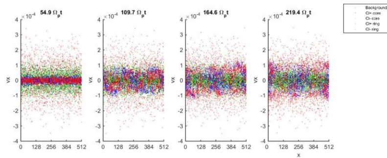
Figure 5: Phasespace of Run III
