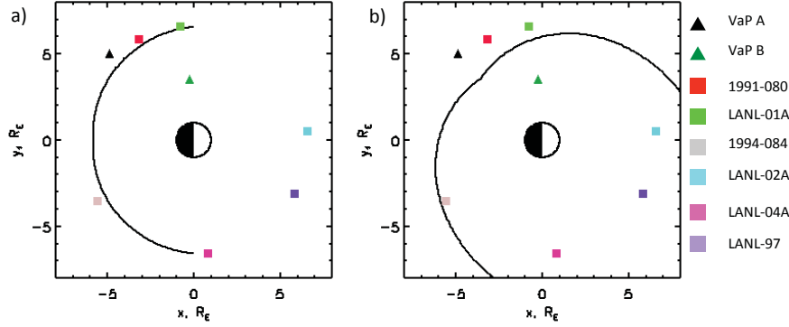
Figure 4: Locations of the LANL and Van Allen Probe satellites at the time of the substorm injection at 05:24 UT with a) an almost circular injection boundary symmetric round 00:00 MLT, b) a more pronounced double spiral boundary rotated by \pi/4
