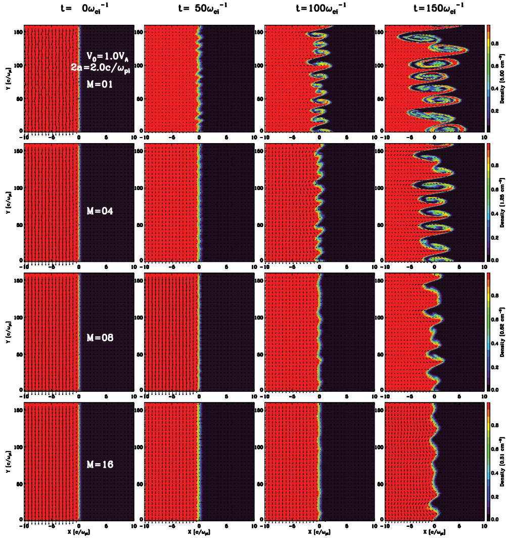
Figure 6: KHI growth for different ion species: mass number M = 1, 4, 8, 16 .
