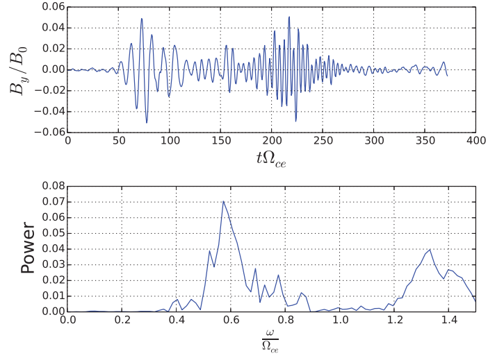
Figure 6: Top: B_y observed at x = 0 and z = 260 . Bottom: the spectral power of B_y .
