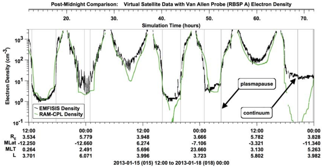
Figure 4: Highlight of EMFISIS RBSP-A in situ density measurements (black) compared to virtual observations (green) through the equatorial plasmaspheric density model RAM-CPL from 12:00 UT on 15th to 00:00 UT on the 18th of January, 2013. Light vertical bars correspond to actual plasmopause crossings of the RBSP-A spacecraft as determined by a low-density ( 20 \text{ cm}^3 ) threshold. As described in the text, a region in which continuum radiation was used to identify the upper limit of the local plasma density is labeled.
