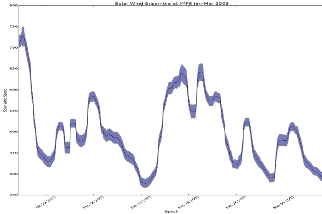
Figure 9: An ensemble of solar wind speed at IMP8 location based on one-point of measurements at ACE spacecraft on Jan-Mar 2003 by using the KDE functions generated for the solar wind data in 1998 - 2000.
