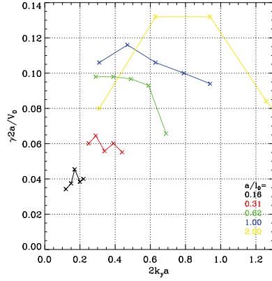
Figure 8: KHI growth rate with wavenumber for different shear widths: a = 0.16 (black), 0.31 (red), 0.62 (green), 1.00 (blue), and 2.00 (yellow).
