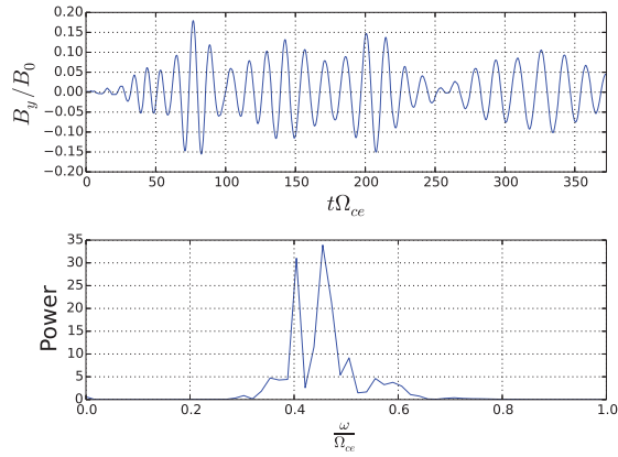
Figure 2: Top: the wave observed at the middle of the simulation domain. Bottom: The frequency spectrum.
