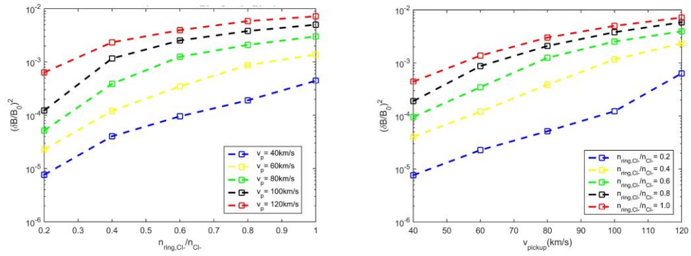
Figure 6: Parametric study of the saturation energy dependence of the instability with respect to variations in the pickup velocity and ring density
