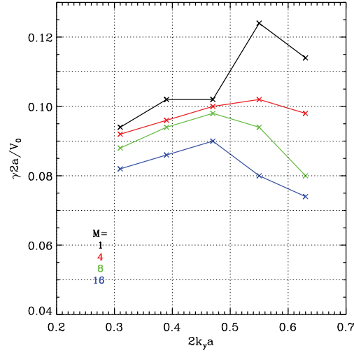
Figure 7: KHI growth rate with wavenumber for different ion species: mass number M = 1, 4, 8, 16 .
