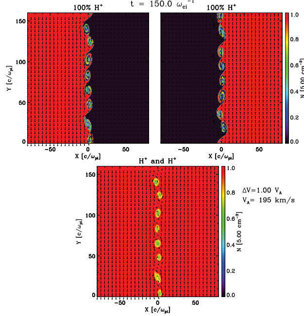
Figure 3: Density contour and flow field at t = 150\omega_{ci}^{-1} .
