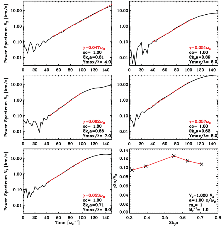
Figure 5: Growth profile of individual wave modes and growth rate with wave number.
