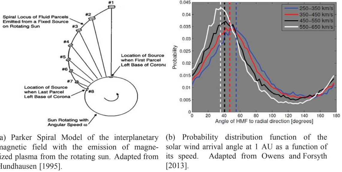
Figure 3: (a) Parker spiral model for the advection of magnetized plasma parcels in the solar wind, and (b) the probability distribution function of the solar wind speed dependence on arrival angle at 1 AU.
