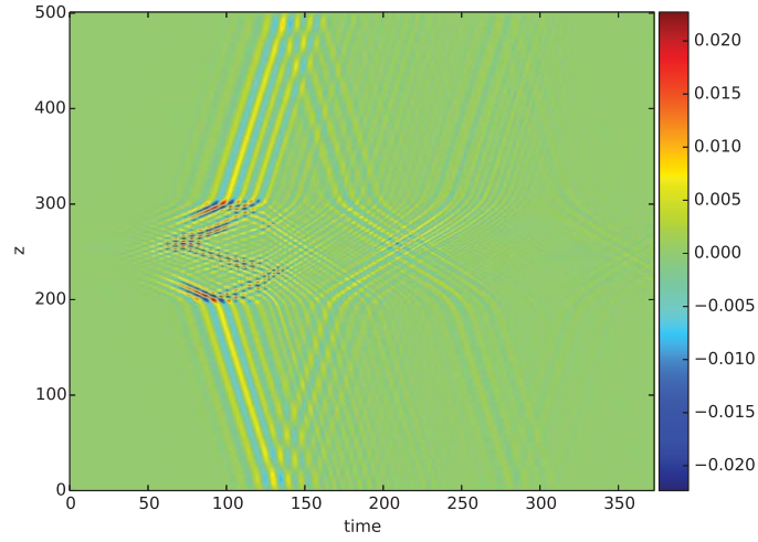
Figure 7: The wave B_y in the 2D simulation along z direction as a function of time.
