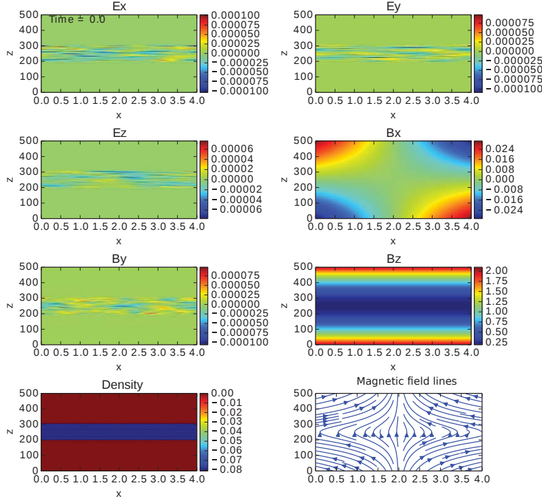
Figure 5: The initial condition for the 2D simulation with curved magnetic field.
