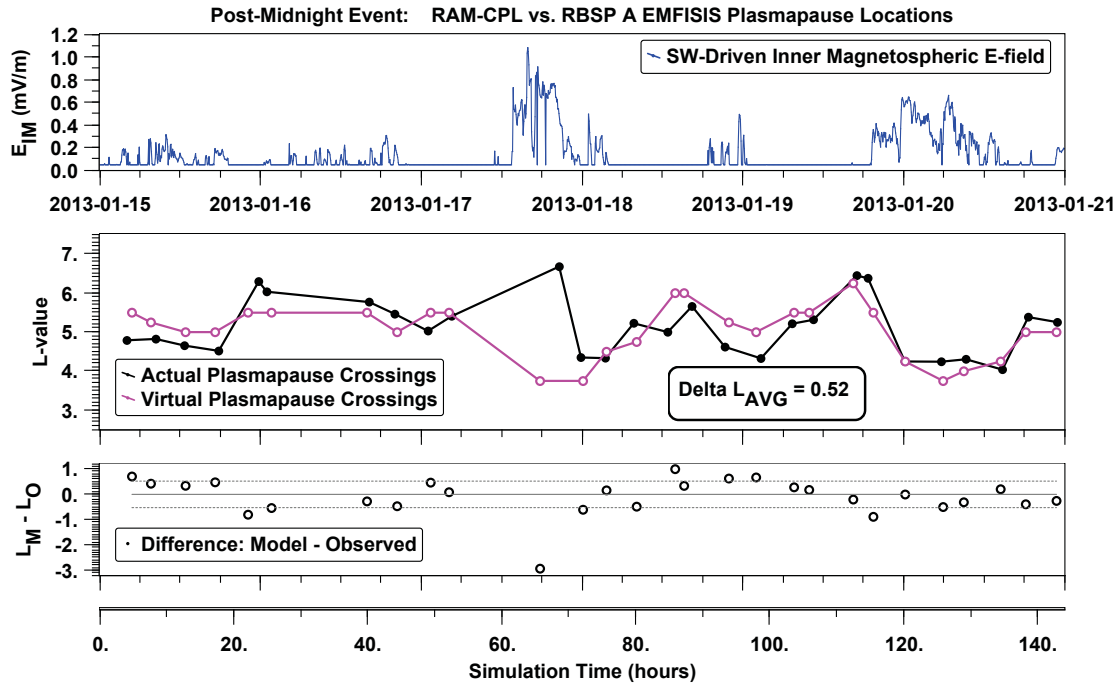
Figure 5: Simulated plasmapause locations from RAM-CPL vs RBSP-A EMFISIS density identifications on 15 - 20 January, 2013. The inner magnetospheric electric field (top panel) controls the extent of the plasmasphere in these simulations and also, to some degree, corresponds to the geomagnetic activity level affecting the actual plasmasphere. Both the actual crossings (black line) and virtual crossings (magenta line) show the relationship between inward plasmapause movement and convection (increased E_{IM} ). The mean difference between both actual and virtual detections is \Delta L_{AVG} = 0.52 \pm 0.15R_E as presented in the bottom panel.
