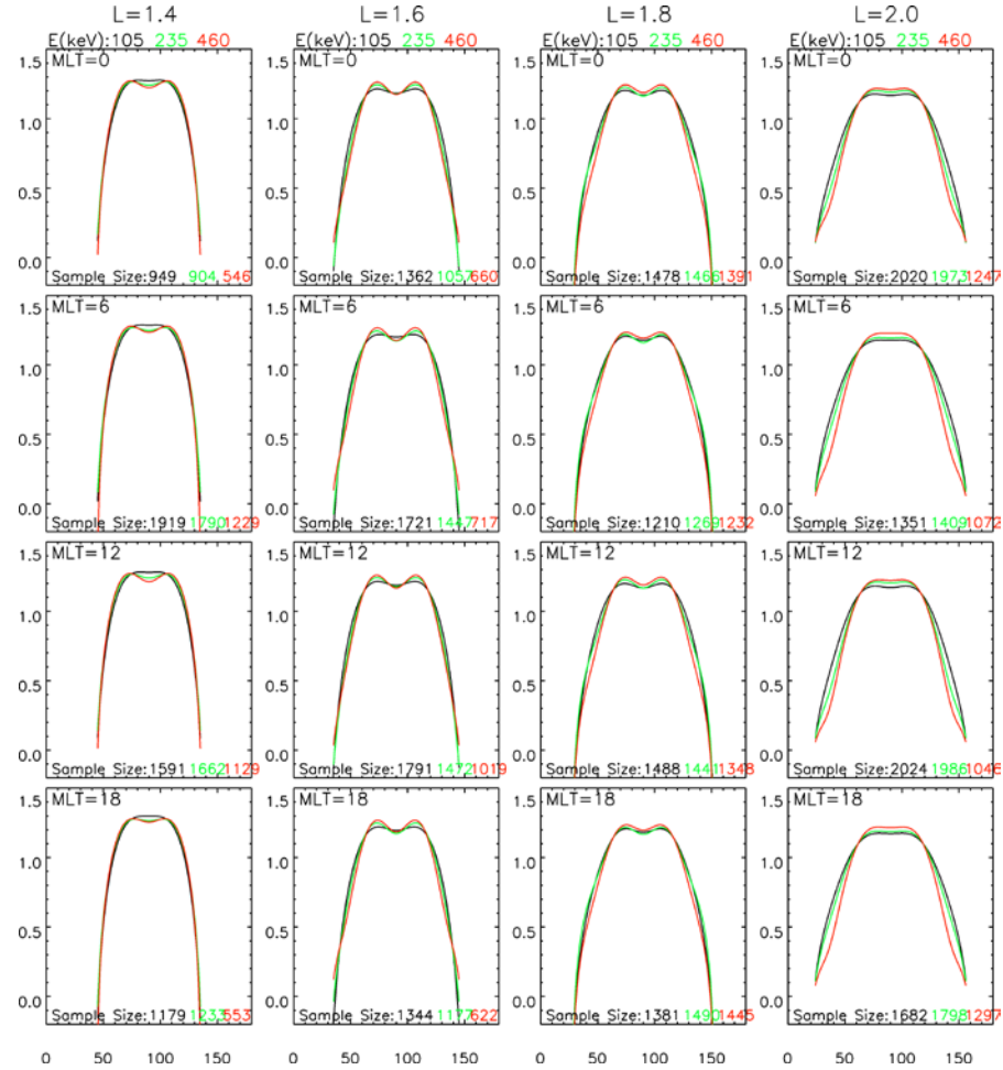
Figure 5. The averaged PADs of \sim 105 , 235, and 460 keV electrons at different MLTs in the inner radiation belt, reconstructed from the statistical relativistic electron PAD model during geomagnetic quiet times ( Dst > -20 nT).
