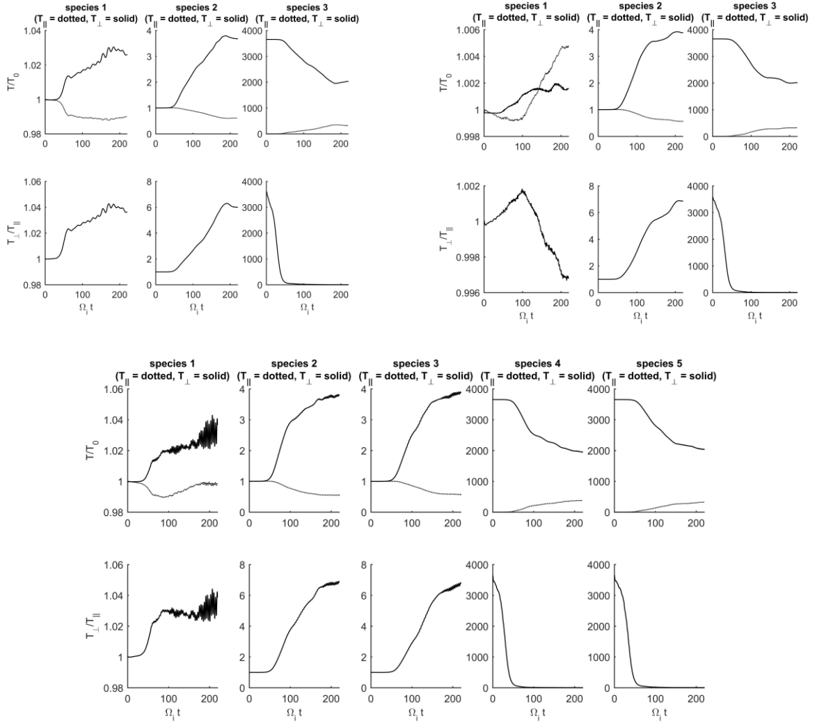
Figure 2: Temperature evolution of (top-left) Run I, (top-right) Run II and (bottom) Run III
