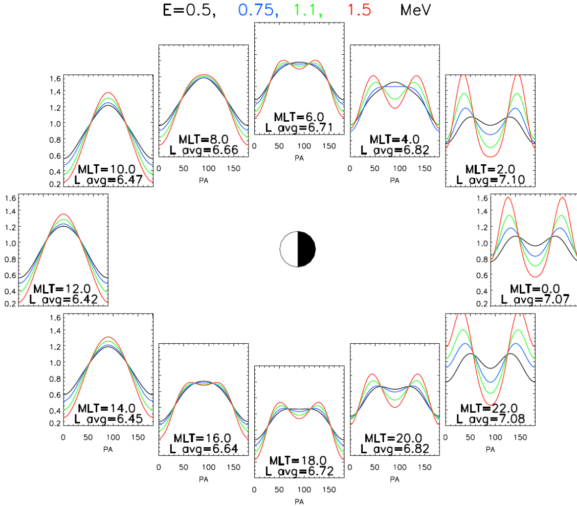
Figure 3. The averaged PADs of 0.5, 0.75, 1.1, and 1.5 MeV electrons as a function of MLT, measured by LANL-GEO satellites.
