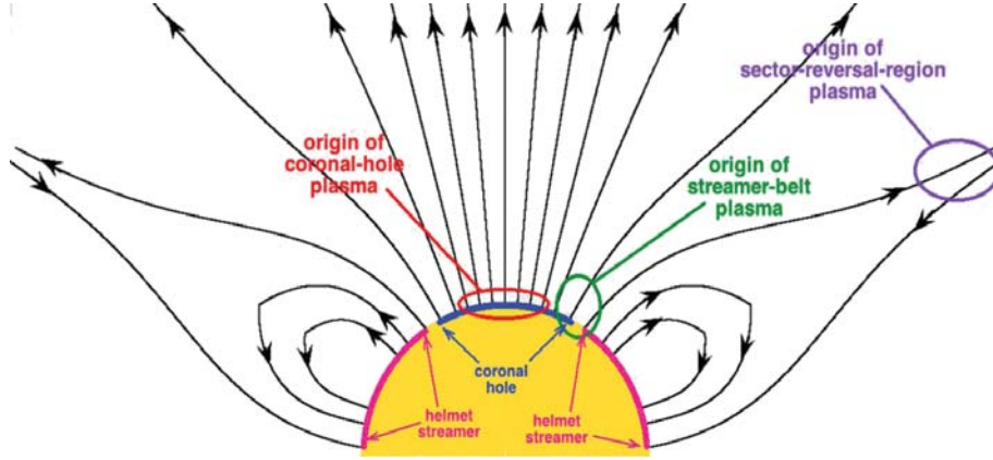
Figure 1: Four Categories of Solar Wind origins in the Solar Corona. Adapted after Xu and Borovsky [2015]
