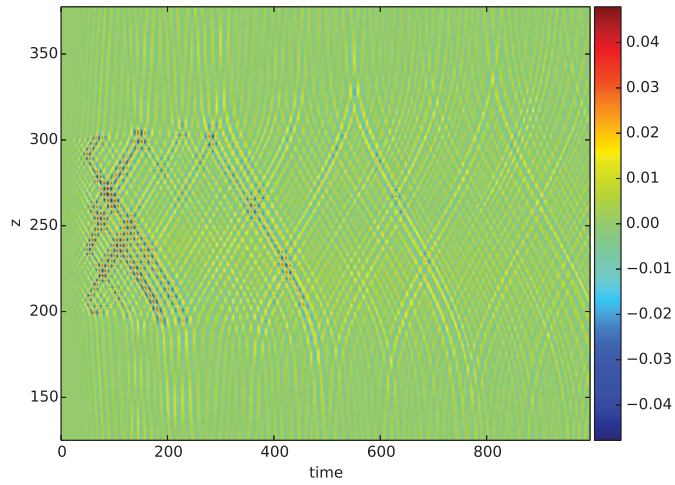
Figure 4: B_y for the whole domain as a function of time.
