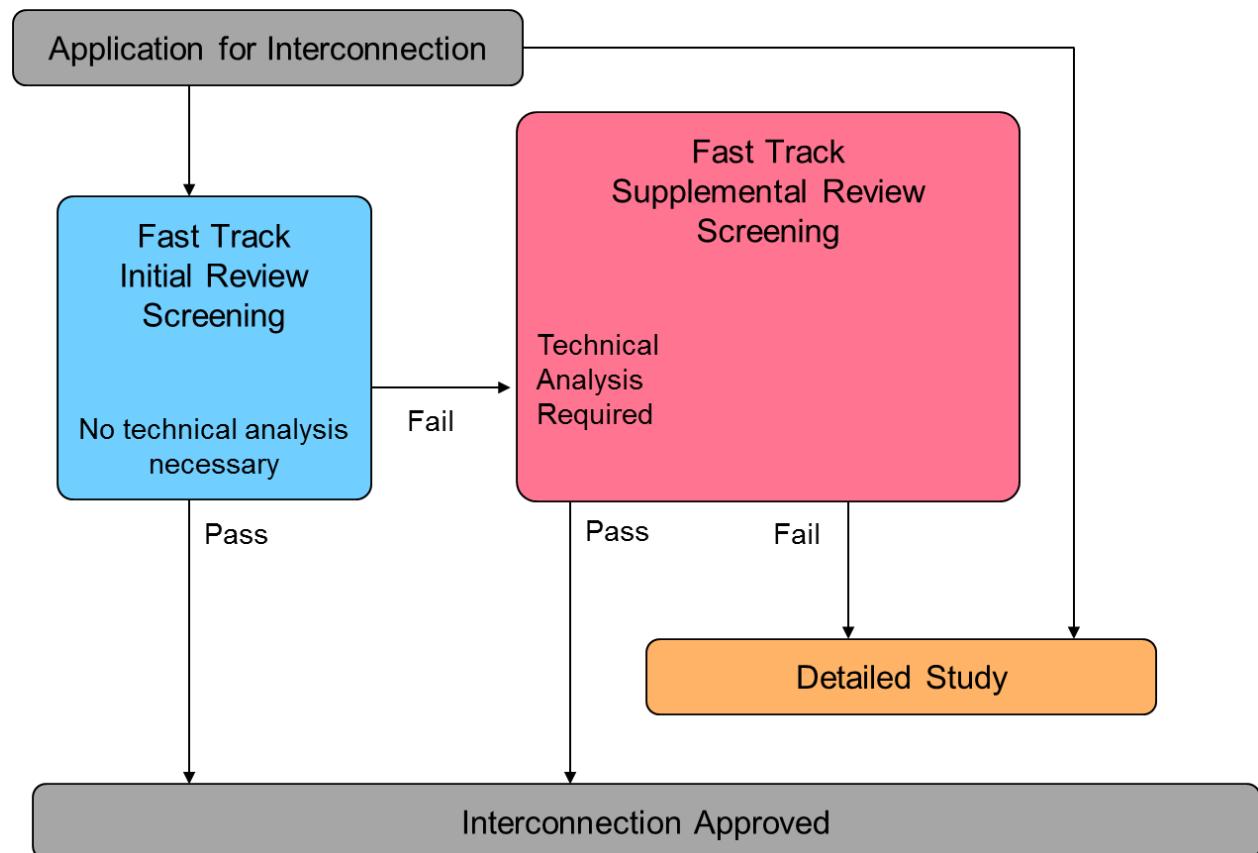
Figure 5. Basic California Rule 21 Screening Process.
