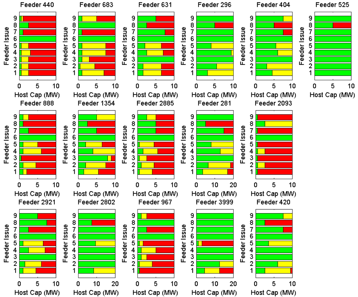
Figure 15. Issue Specific Utility-Scale PV Hosting Capacity.
