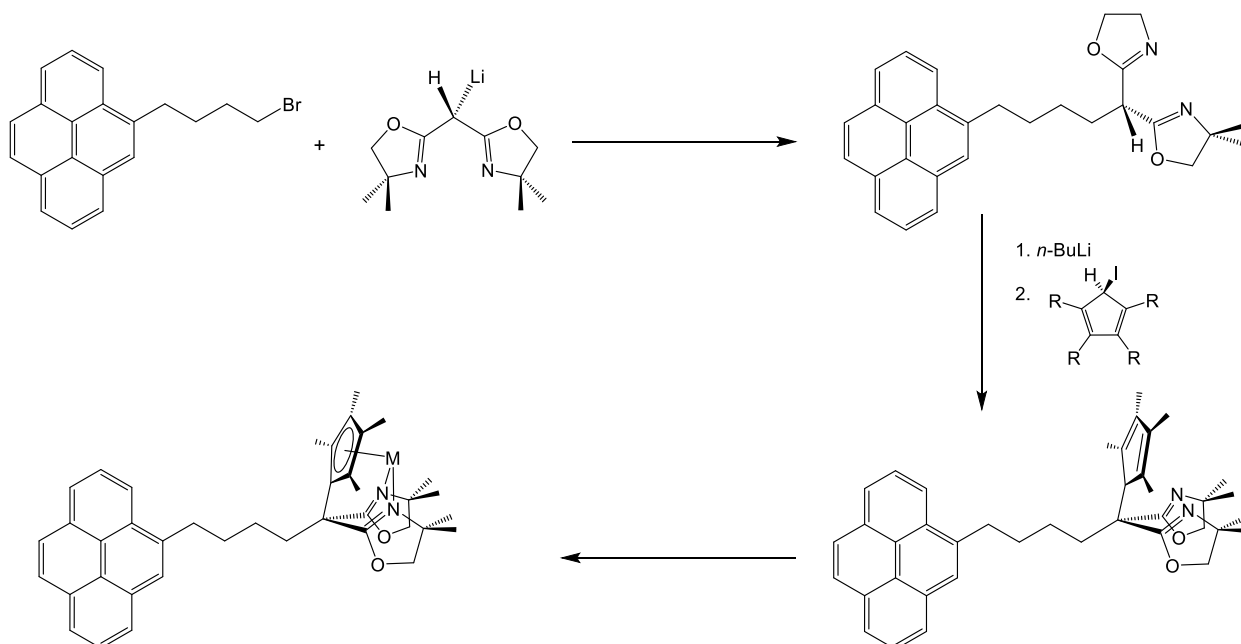
Figure 1: Proposed synthetic route to \{\text{Bo}^{\text{M}}\text{Cp}^{\text{tet}}\} on pyrene
