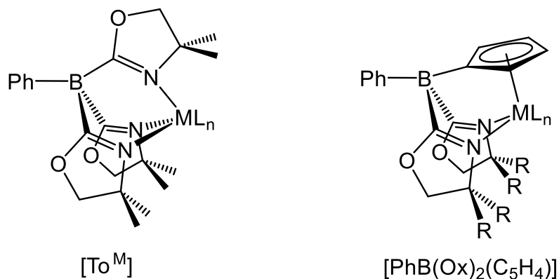
Figure 1: \text{To}^{\text{M}} and \text{PhB}(\text{Ox})_2(\text{C}_5\text{H}_4)
