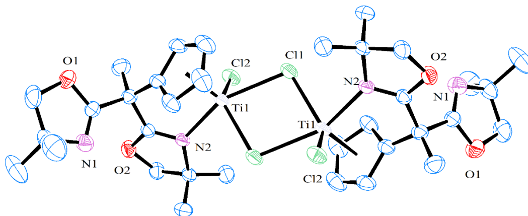
Figure 8: ORTEP diagram of {Bo M Cp}TiCl 2
