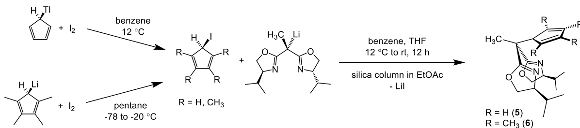
Scheme 3: Synthesis of \text{H}\{\text{Bo}^{\text{P}}\text{Cp}\} and \text{H}\{\text{Bo}^{\text{P}}\text{Cp}^{\text{tet}}\}
