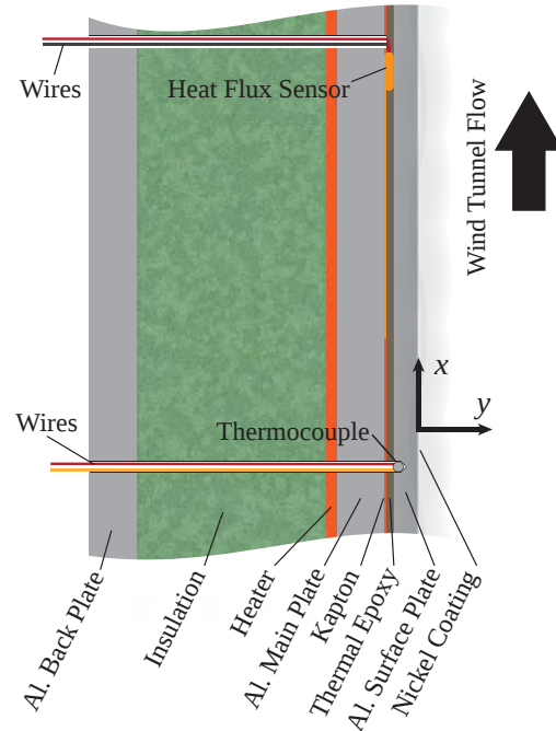
Fig. 2.4: Heated wall cross section with component names as in Table 2.3. The relative thicknesses are to scale.
