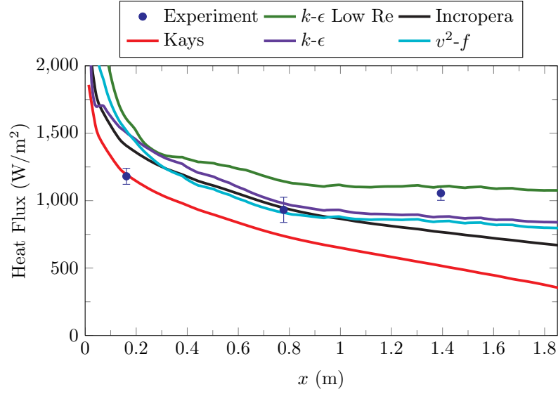
Fig. 5.15: The heat flux for the buoyancy opposed isothermal mixed convection case compared with several CFD models with the k - \epsilon Low Re being the standard model for the mixed cases in this study.
