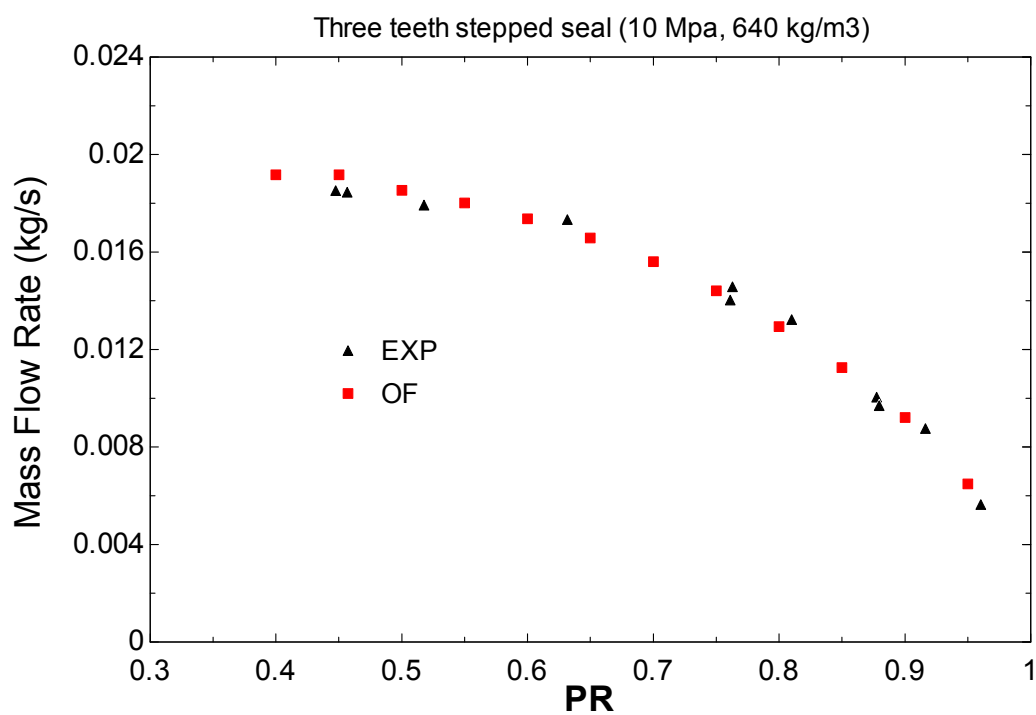
Figure 62 Mass flow rates for three-tooth stepped labyrinth seal for 10 MPa at 640 kg/m 3
