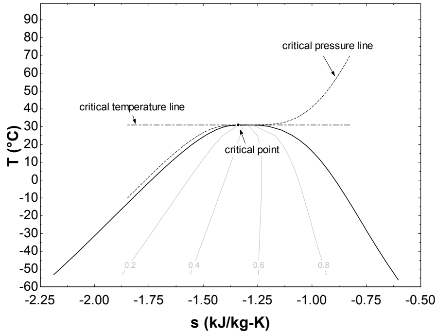
Figure 3 T-S diagram of CO 2
