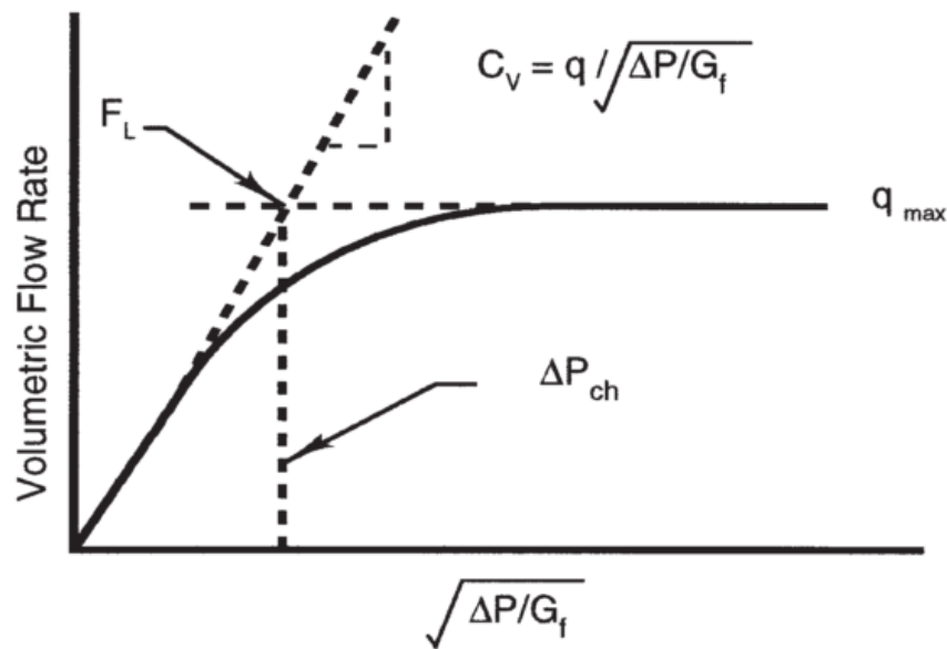
Figure 13 Maximum flow rate occurring due to choked conditions [46]
