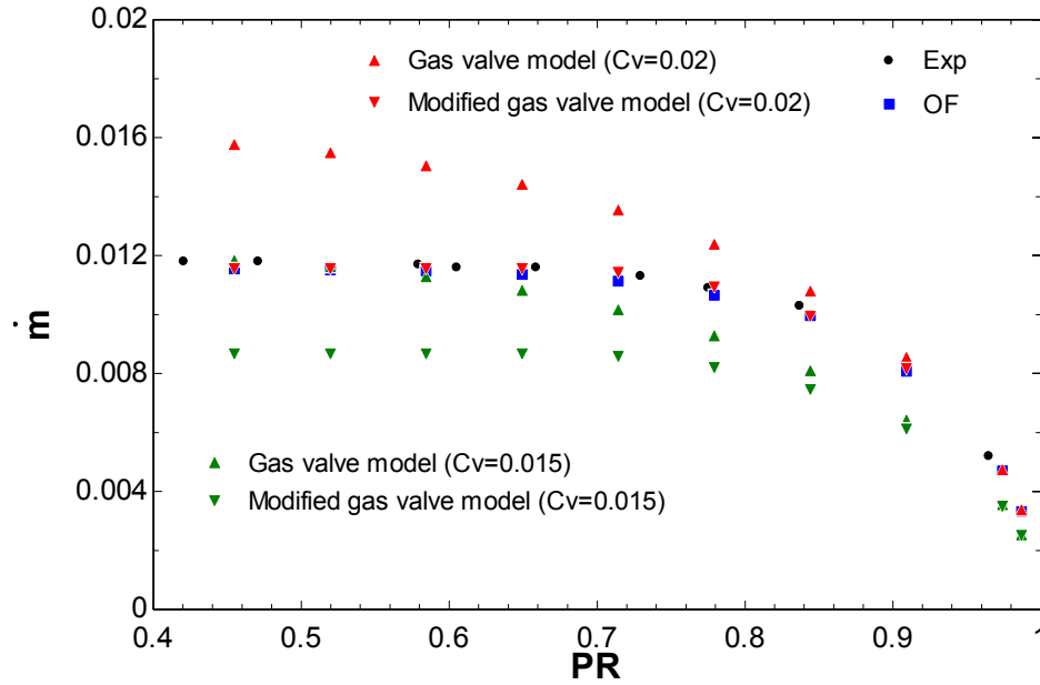
Figure 69 Mass flow rate of valve from different sources at 50% open
