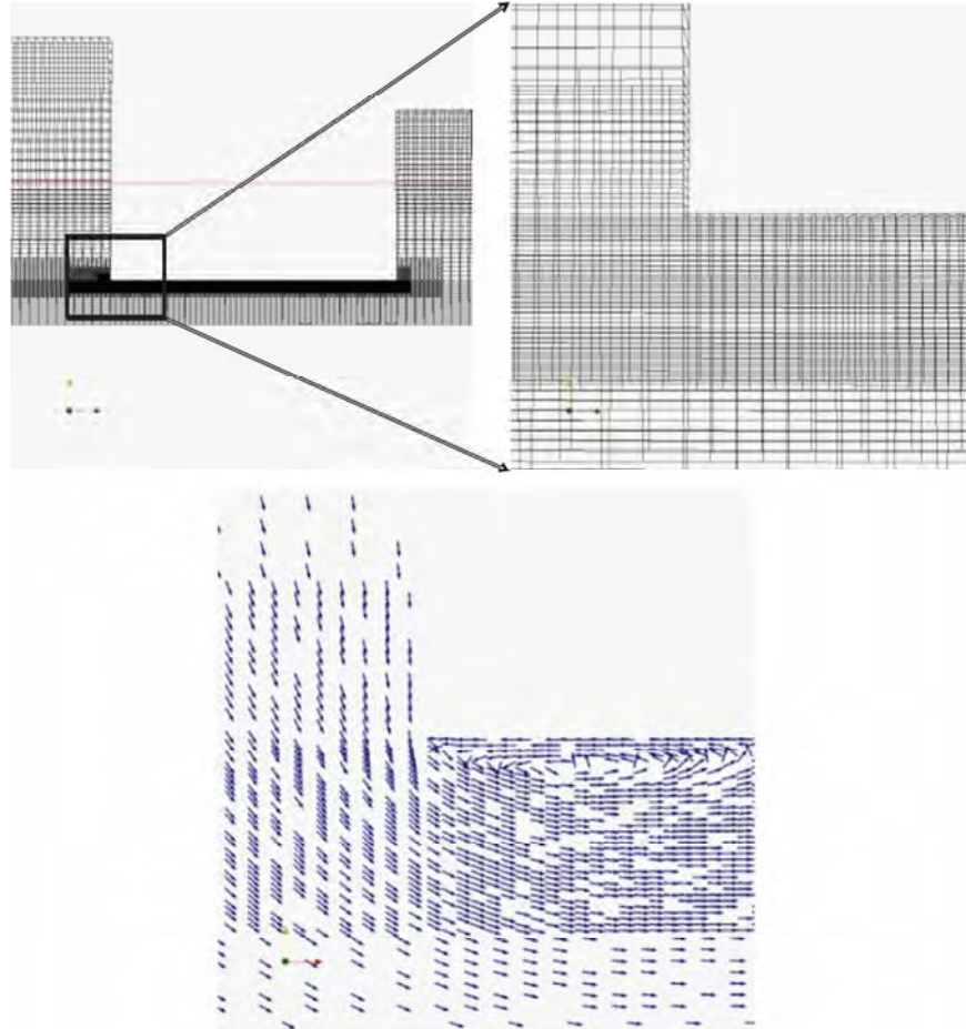
Figure 23 Mesh refinement at entrance
