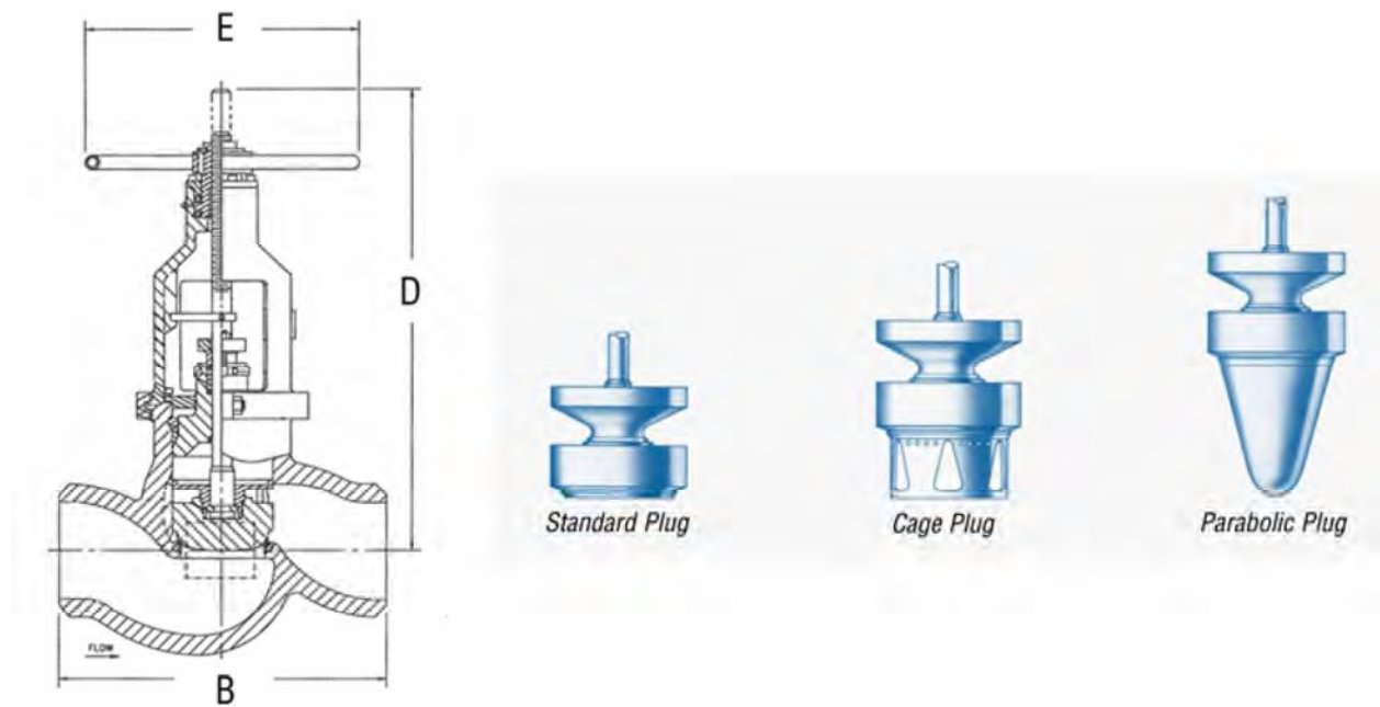
Figure 70 Globe valve by Flowserve[70]
