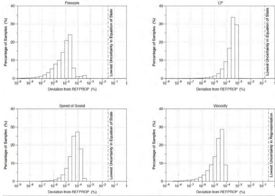
Figure 16 Comparison of FIT and REFPROP for CO 2 [3]
