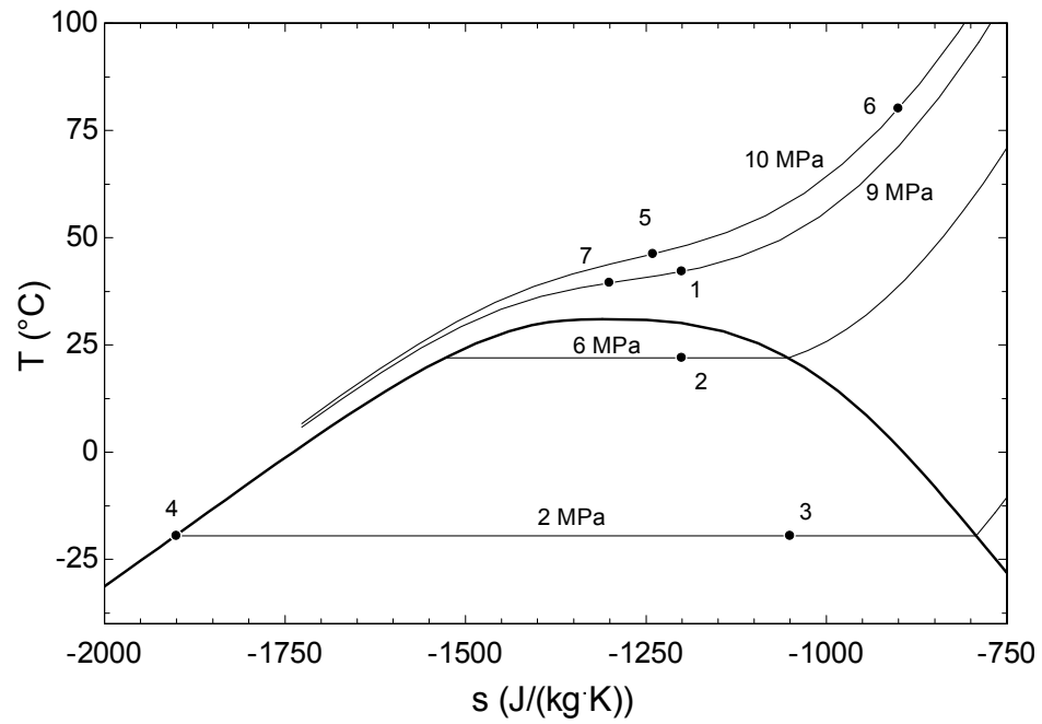
Figure 26 Thermodynamic state of each point in experiment loop
