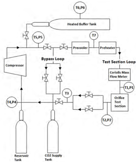
Figure 24 Schematic diagram of experiment facility
