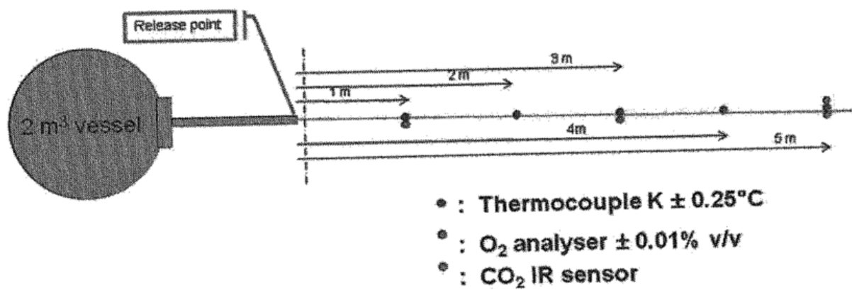
Figure 9 S-CO 2 release test rig by Fairweather [26]
