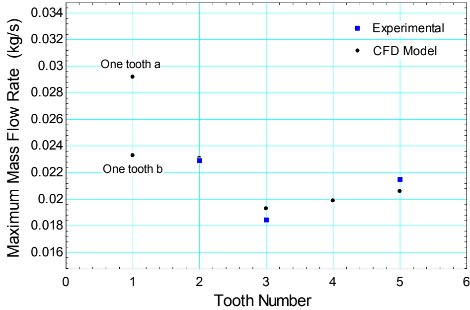
Figure 57 Maximum mass flow rate VS tooth number
