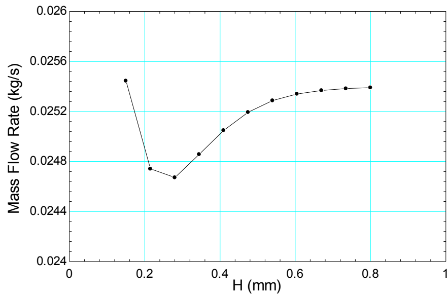
Figure 96 Mass flow rate changes with cavity height at cavity length of 1.27 mm.
