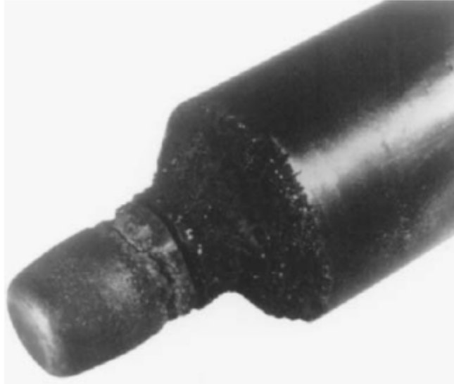
Figure 14 Plug damaged by cavitation [46]
