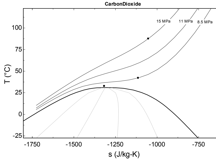
Figure 72 Tested upstream conditions
