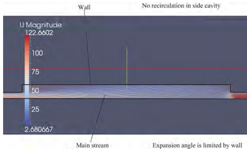
Figure 54 Flow pattern in cavity of labyrinth seal of cavity height of 0.2 mm and cavity length of 3 mm
