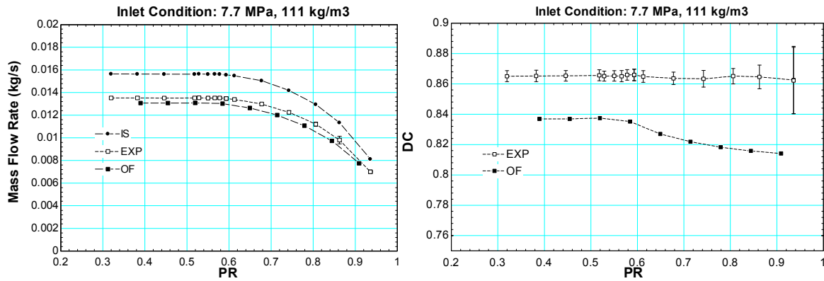
Figure 82 Circular orifice data for inlet condition of 7 MPa, 111 kg/m³
