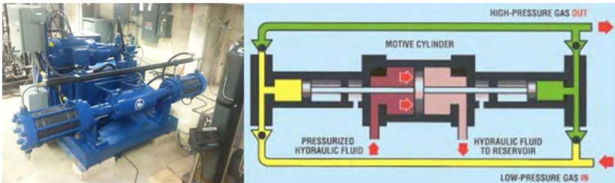
Figure 27 Picture and diagram of Hydro-Pac compressor
