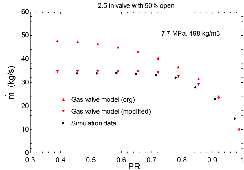
Figure 73 Globe valve with 50% open with upstream condition of 7.7 MPa at 498 \text{kg/m}^3
