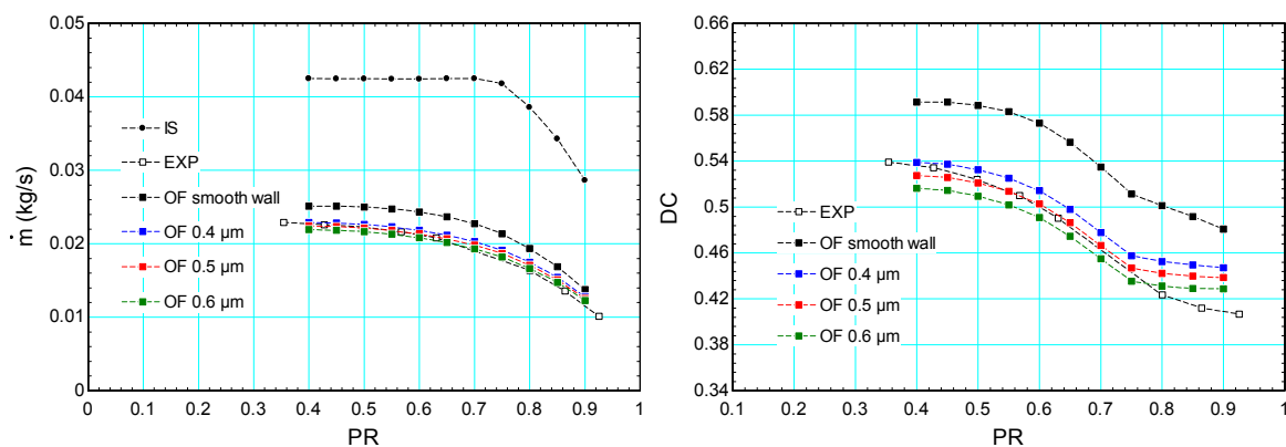
Figure 36 Medium annular orifice data for inlet condition 10 MPa, 475 kg/m³
