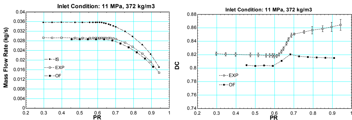
Figure 90 Circular orifice data for inlet condition of 11 MPa, 372 kg/m 3
