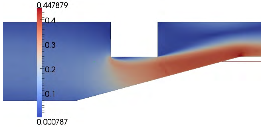
Figure 77 Mach number of upstream of 15 MPa at 383 kg/m 3 , and downstream of 14 MPa
