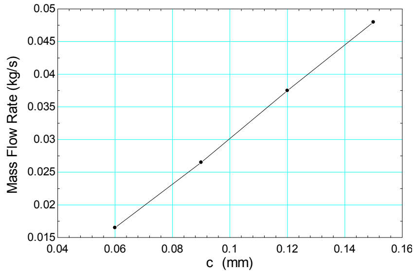
Figure 45 Effect of radial clearance on mass flow rate
