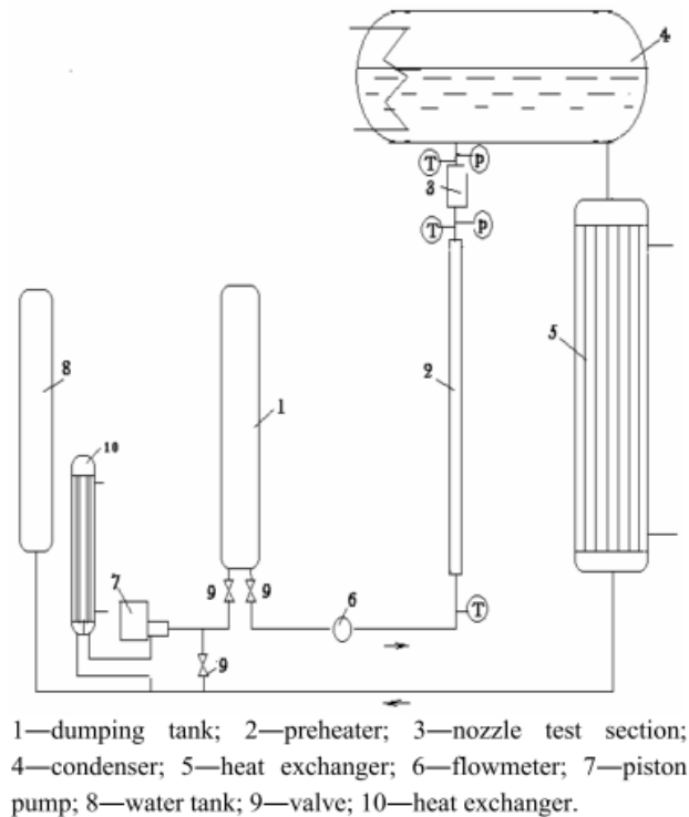
Figure 10 SCW choked flow experiment by Chen [20], [32]
