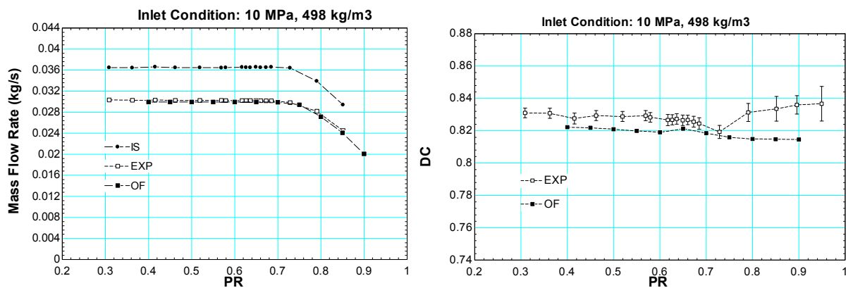
Figure 88 Circular orifice data for inlet condition of 10 MPa, 498 kg/m 3
