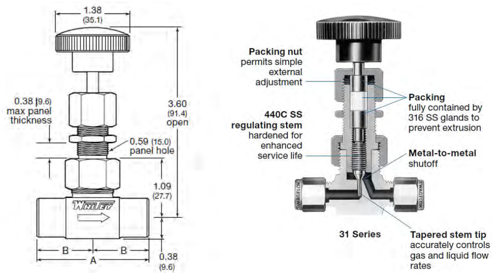
Figure 63 Dimensions and inner geometry of SS-31RS4 [69]
