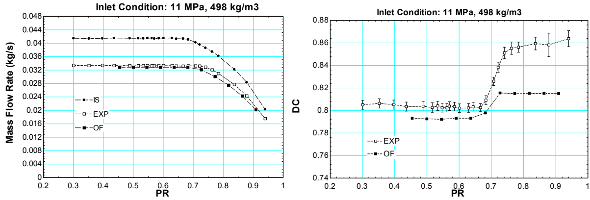
Figure 91 Circular orifice data for inlet condition of 11 MPa, 498 kg/m 3
