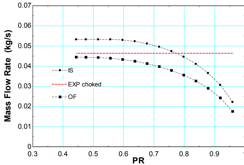
Figure 41 Comparison of simulation and experiment for SCW at 24.8 MPa and 453 °C
