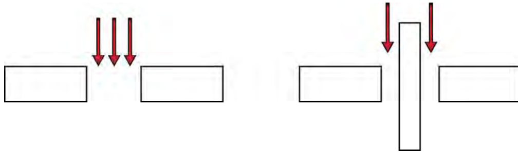
Figure 30 Schematic for the flow through circular and annular orifices
