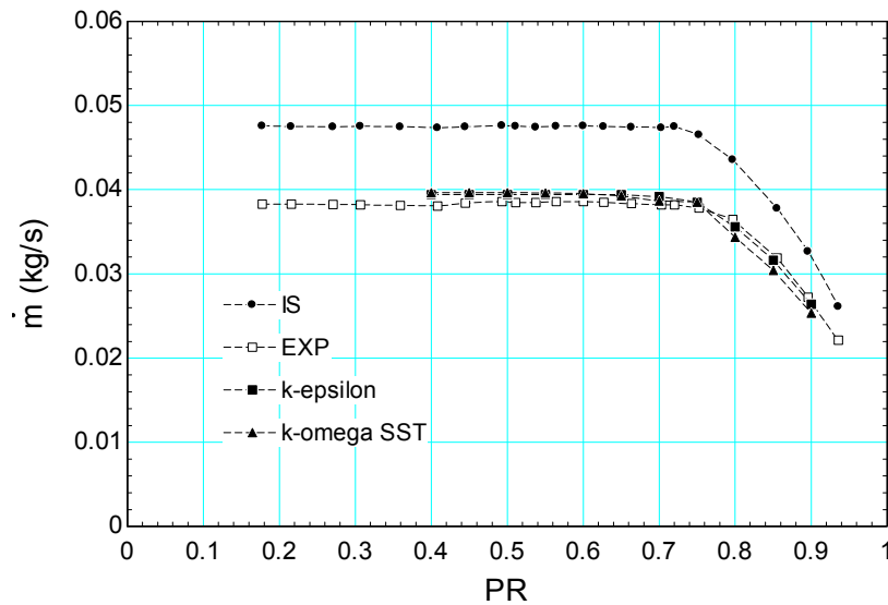
Figure 20 Short annular orifice data for comparison of standard k-epsilon and k-omega SST
