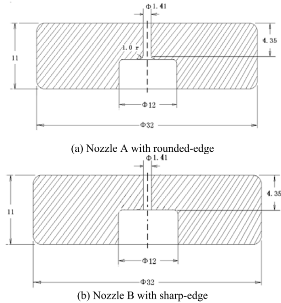
Figure 39 Nozzles tested in SCW choked flow experiment by Chen[20], [32]
