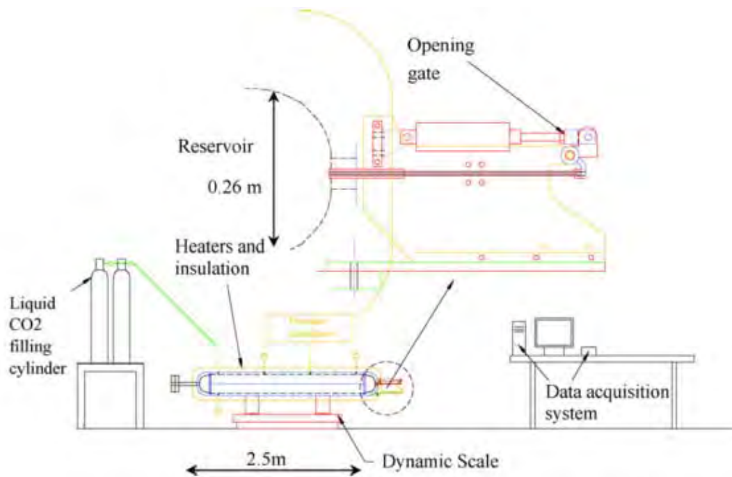
Figure 8 S-CO 2 choked flow experiment by Mignot[27]
