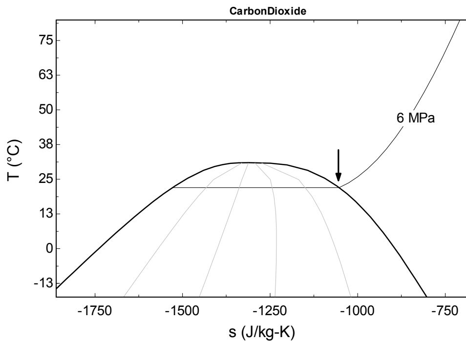
Figure 81 Saturation point at 6 MPa
