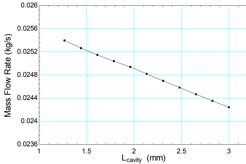
Figure 46 Mass flow rate changes with cavity length at cavity height of 0.88 mm
