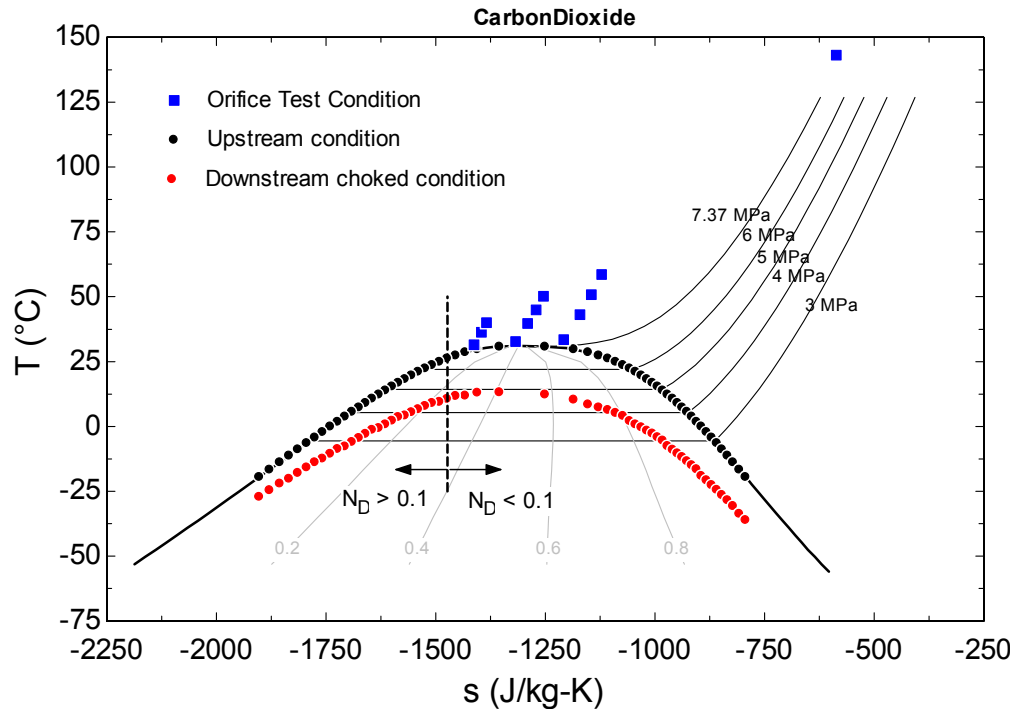
Figure 80 Drift number calculations for saturated upstream conditions
