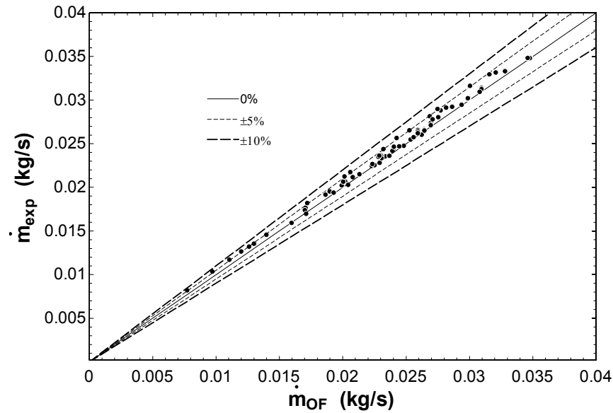
Figure 33 Short circular orifice simulation and experiment data for inlet condition 10 MPa, 372 kg/m³
