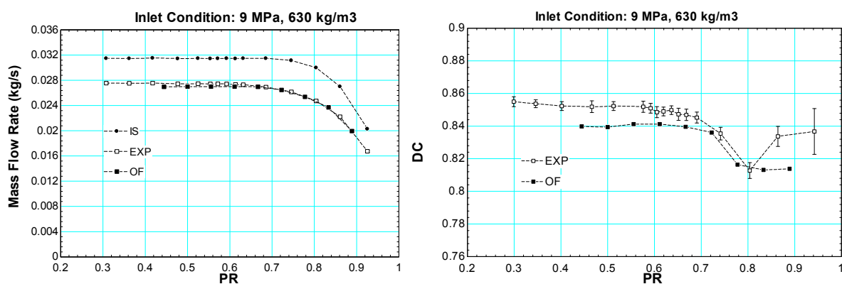
Figure 87 Circular orifice data for inlet condition of 9 MPa, 630 kg/m 3
