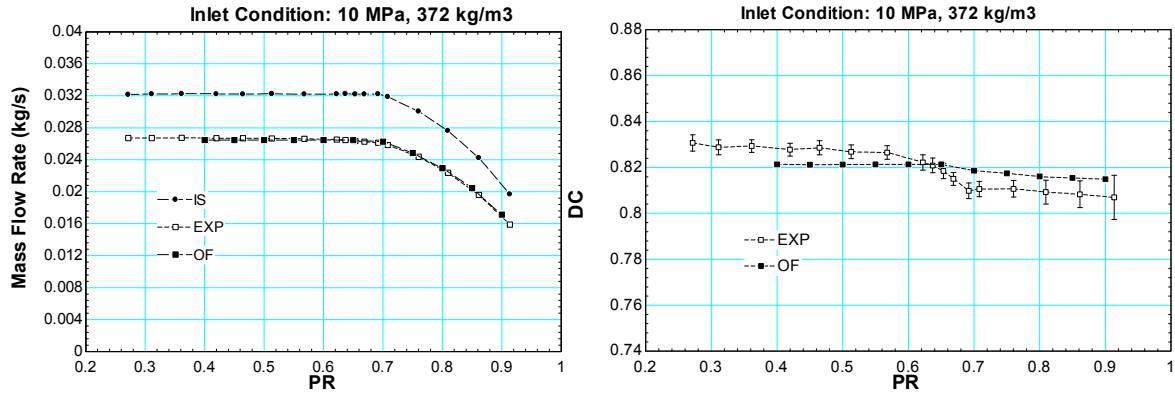
Figure 33 Short circular orifice simulation and experiment data for inlet condition 10 MPa, 372 kg/m³
