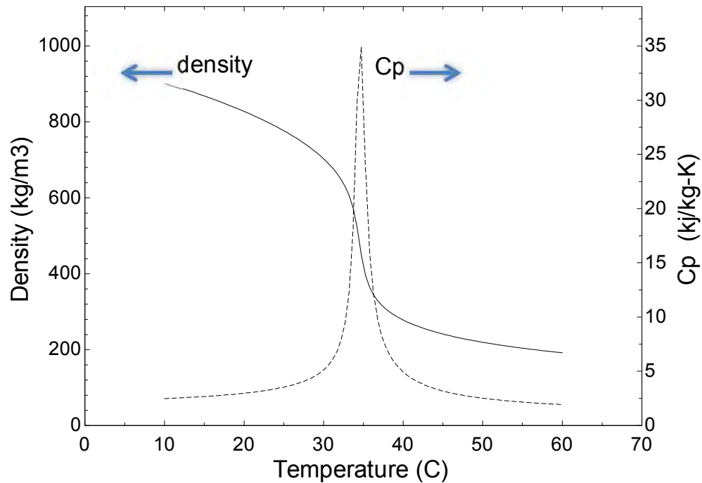
Figure 4 Property change of CO 2 at pseudo-critical point at 8 MPa
