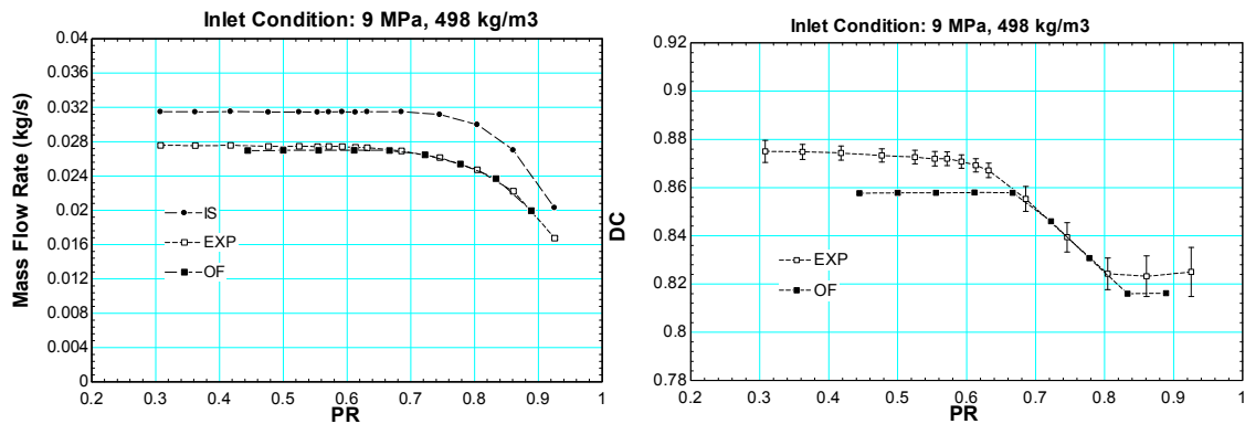
Figure 32 Short circular orifice simulation and experiment data for inlet condition 9 MPa, 498 kg/m 3
