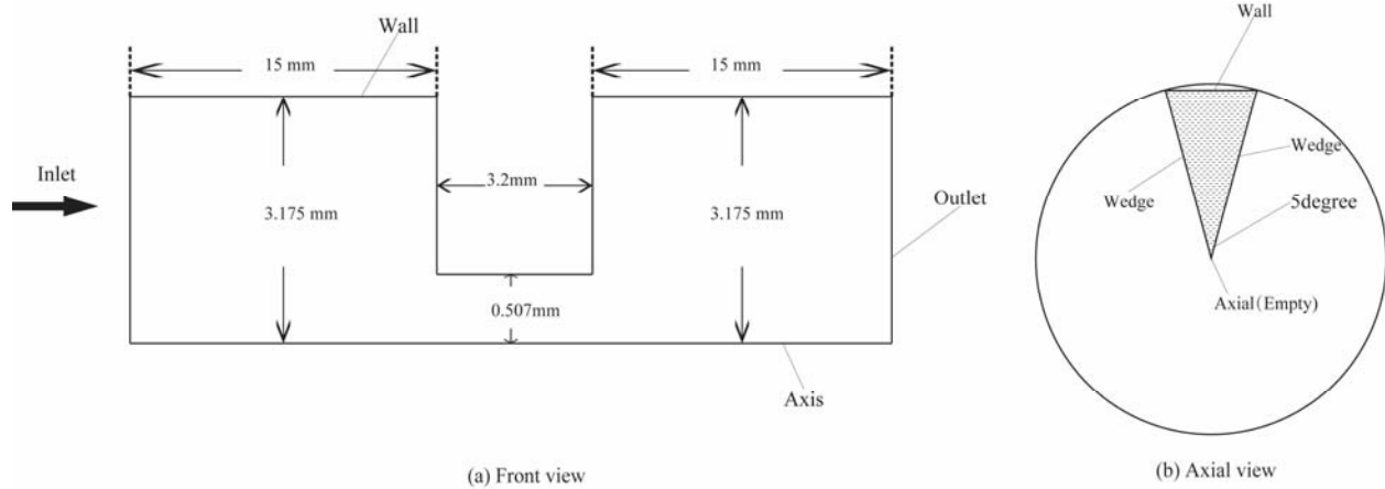
Figure 18 Computational domain and boundary conditions for circular orifice (not to scale) [60]
