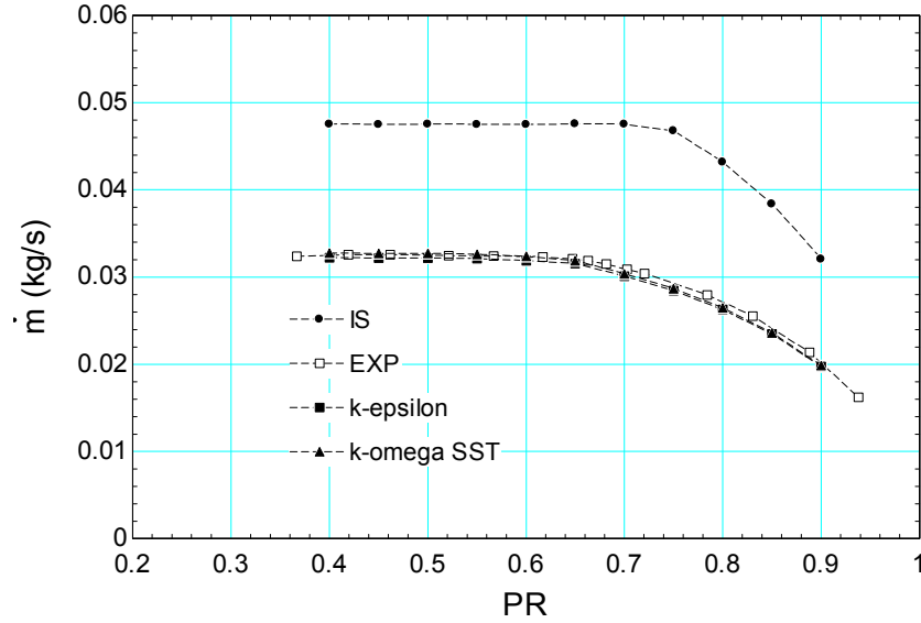
Figure 21 Medium annular orifice data for comparison of standard k-epsilon and k-omega SST
