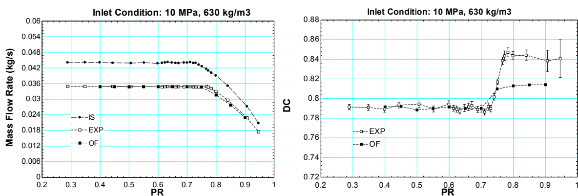
Figure 89 Circular orifice data for inlet condition of 10 MPa, 630 kg/m 3
