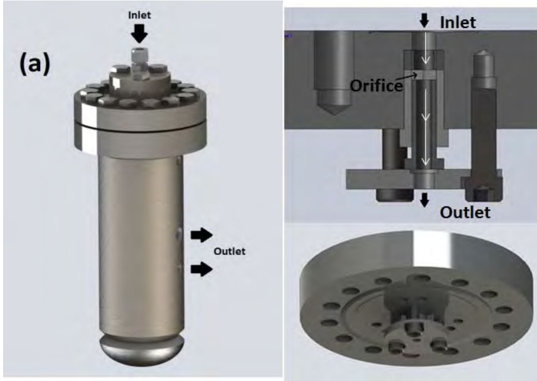
Figure 28 Diagram of test section
