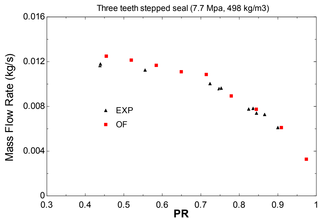
Figure 61 Mass flow rates for three-tooth stepped labyrinth seal for 7.7 MPa at 498 kg/m 3
