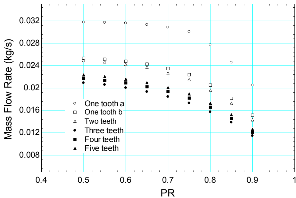
Figure 55 Labyrinth seal designs of same total length
