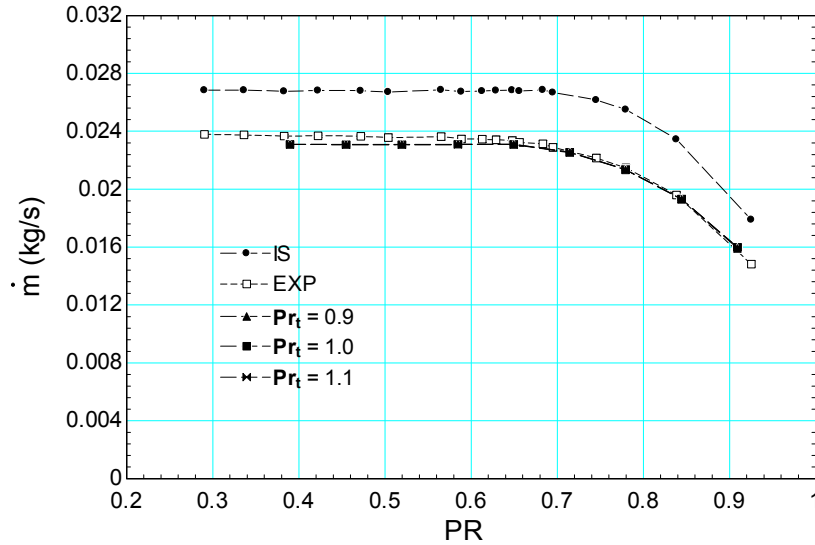
Figure 22 Circular orifice data for different Pr_t using standard k-epsilon model
