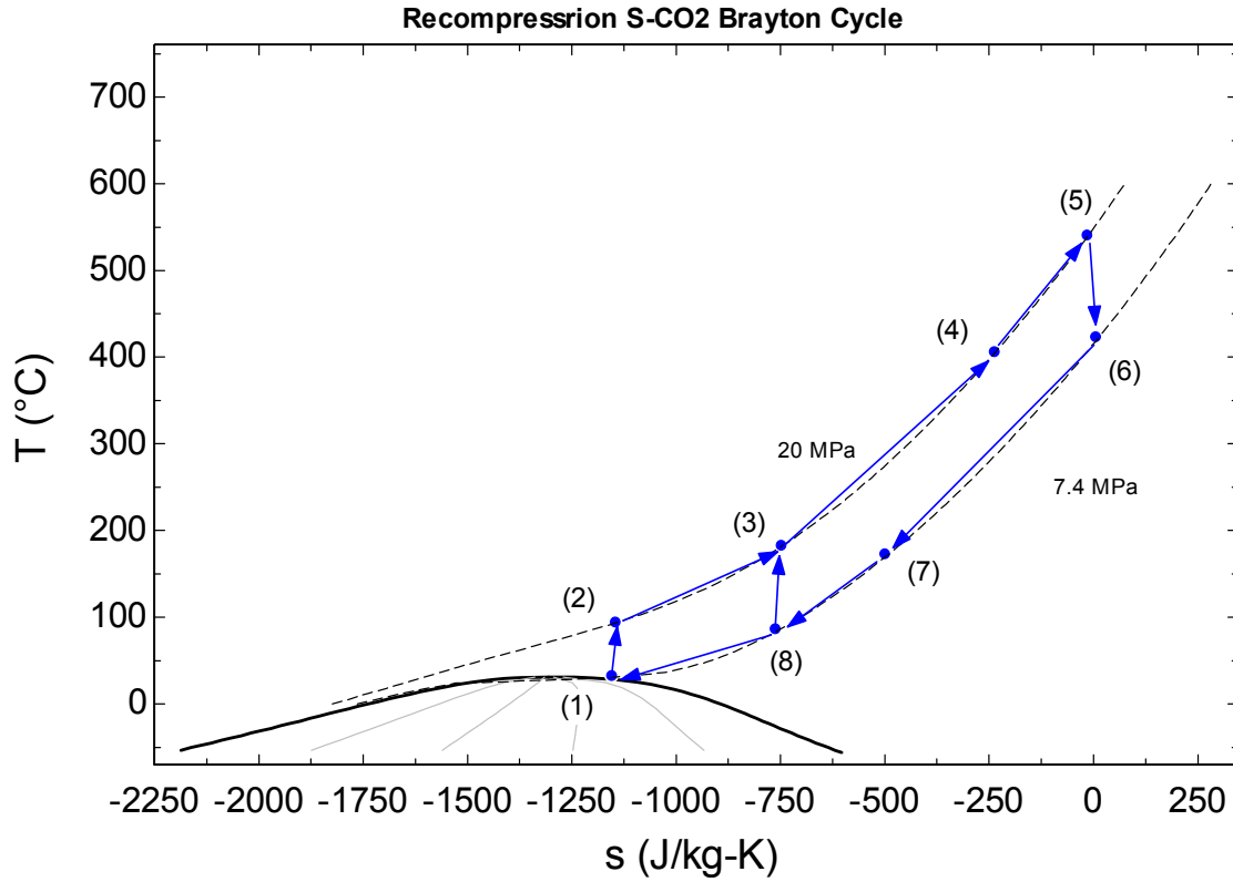
Figure 7 T-S diagram of recompression S-CO 2 Brayton cycle
