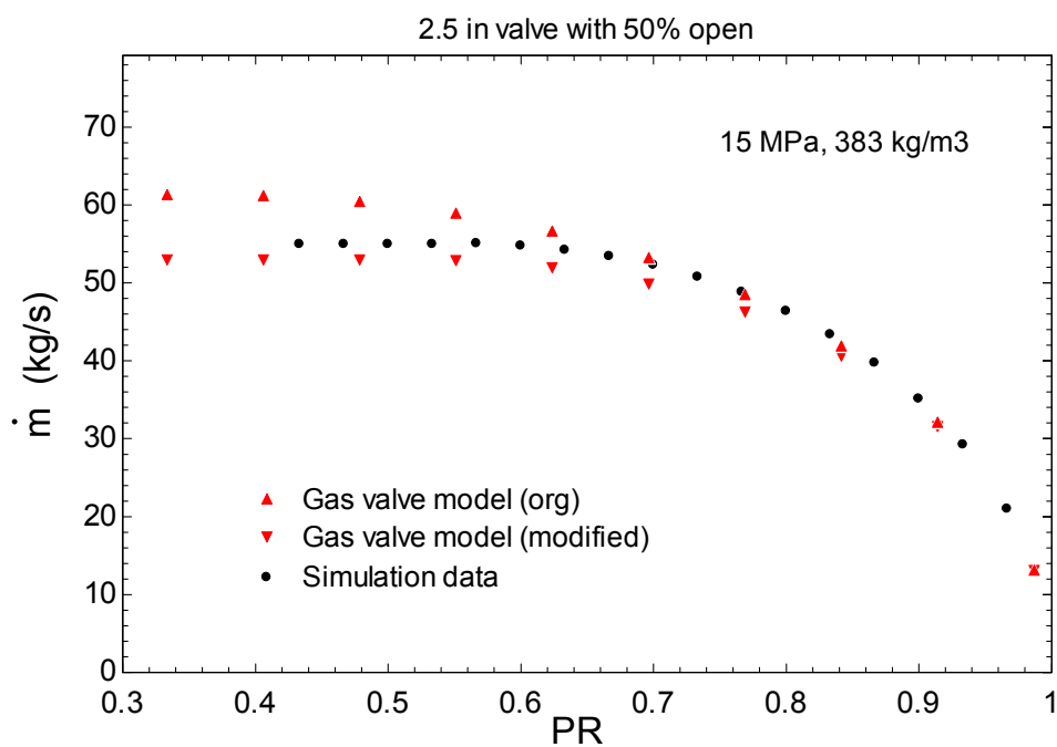
Figure 75 Globe valve with 50% open with upstream condition of 15 MPa at 383 kg/m 3
