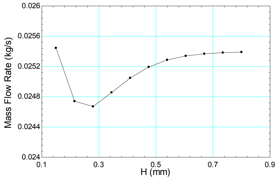
Figure 49 Mass flow rate changes with cavity height at cavity length of 1.27 mm
