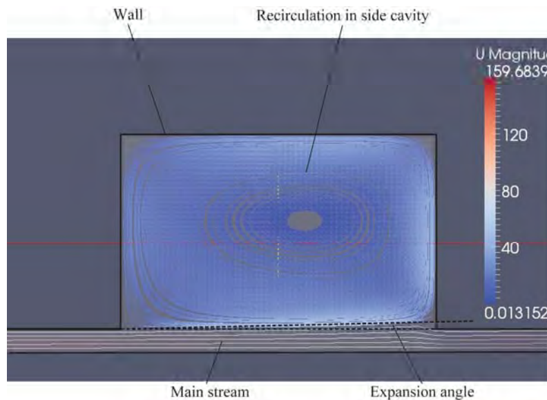
Figure 47 Flow pattern in cavity of labyrinth seal of cavity height of 0.88 mm and cavity length of 1.27 mm
