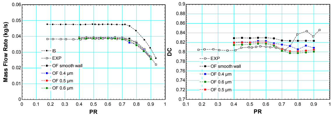
Figure 35 Short annular orifice data for inlet condition 10 MPa, 475 kg/m 3
