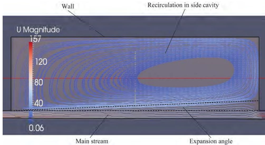
Figure 48 Flow pattern in cavity of labyrinth seal of cavity height of 0.88 mm and cavity length of 3 mm
