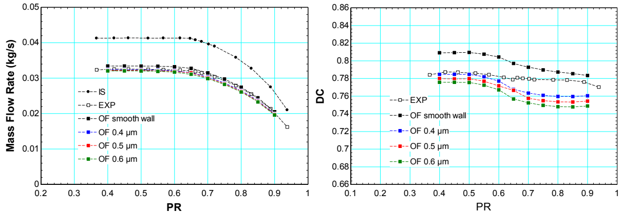
Figure 92 Medium annular orifice data for inlet condition of 10 MPa, 325 kg/m 3
