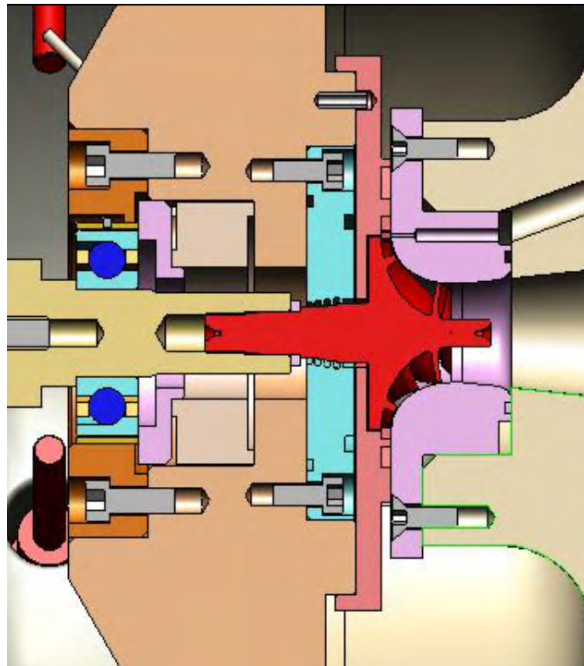
Figure 11 Seal of compressor in SNL S-CO 2 Brayton cycle experiment [15]
