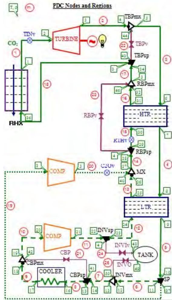
Figure 12 S-CO 2 Brayton cycle design by Moisseytsev [45]
