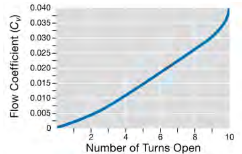
Figure 68 Valve coefficient changes with number of turns for tested valve
