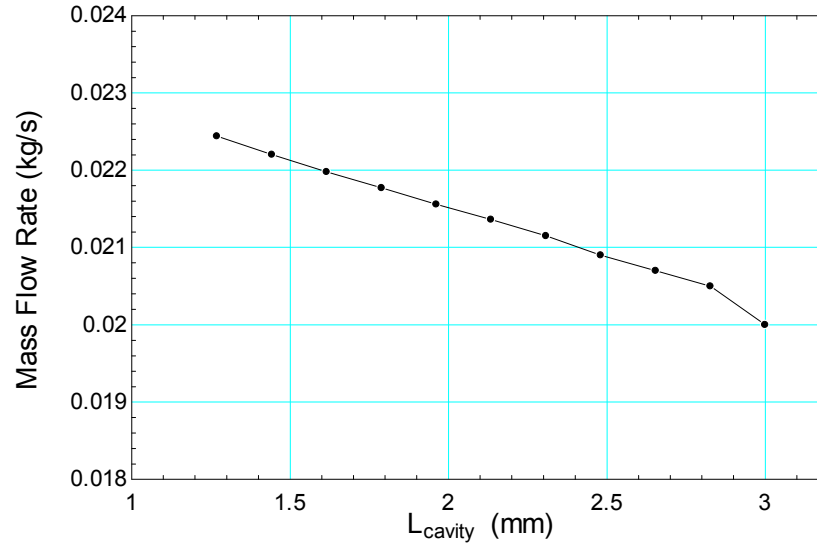
Figure 95 Mass flow rate changes with cavity length at cavity height of 0.88 mm.
