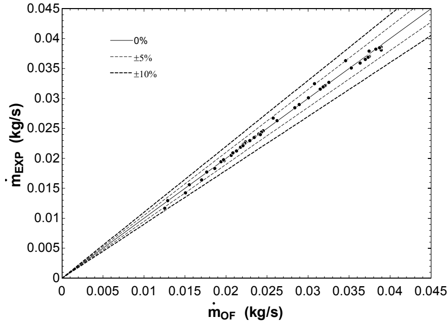
Figure 38 Mass flow rate comparison of annular orifice
