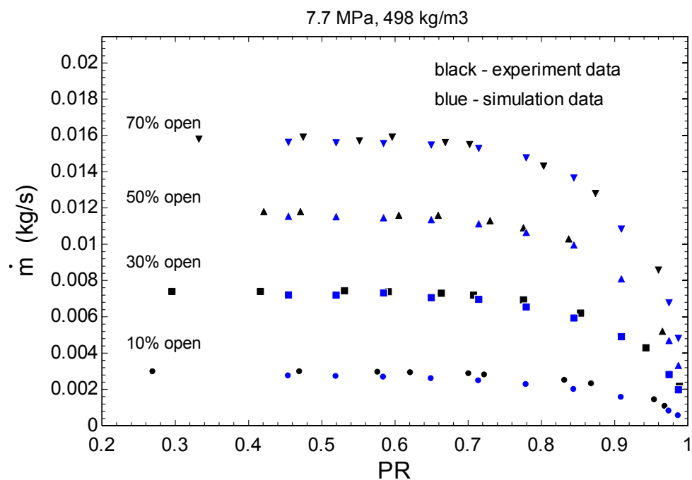
Figure 66 Comparison of experiment and simulation for test valve for 7.7 MPa at 498 kg/m 3
