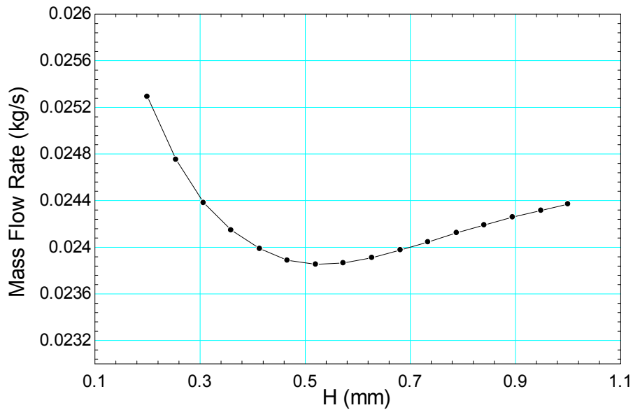
Figure 50 Mass flow rate changes with cavity height at cavity length of 3 mm
