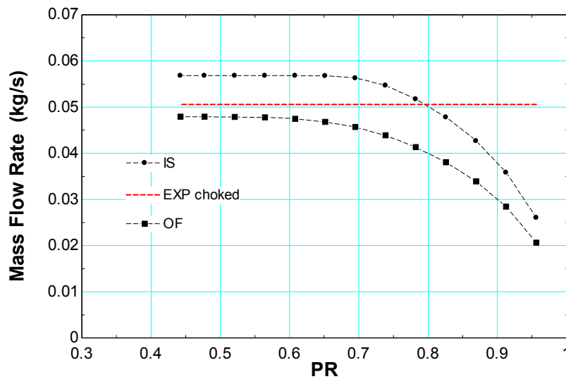
Figure 40 Comparison of simulation and experiment for SCW at 22.95 MPa and 392.5 °C
