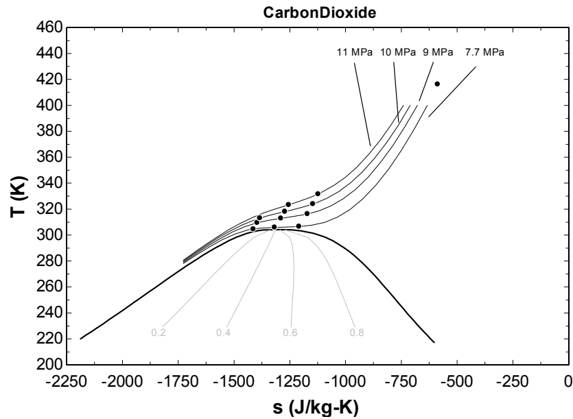
Figure 31 Circular orifice tested inlet conditions on T-S diagram
