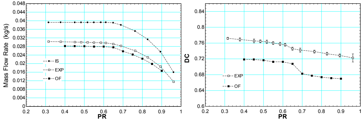
Figure 43 Two-tooth labyrinth seal experiment and simulation comparison (10 MPa, 325 kg/m 3 )
