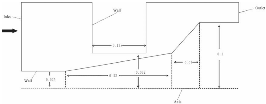
Figure 65 Computational domain for test valve geometry
