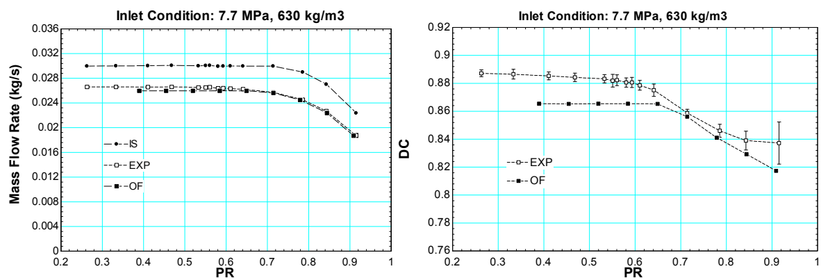
Figure 85 Circular orifice data for inlet condition of 7 MPa, 630 kg/m 3
