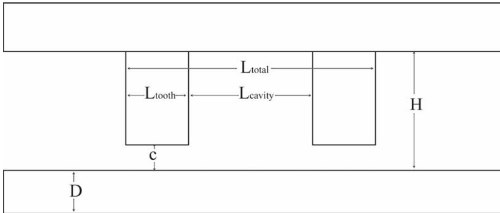
Figure 42 Schematic of two-tooth labyrinth seal (not to scale)
