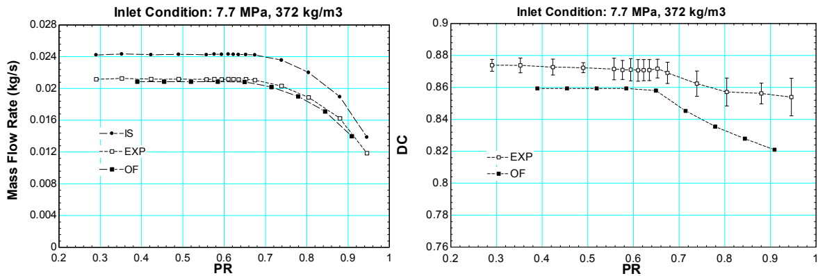
Figure 83 Circular orifice data for inlet condition of 7 MPa, 327 kg/m³
