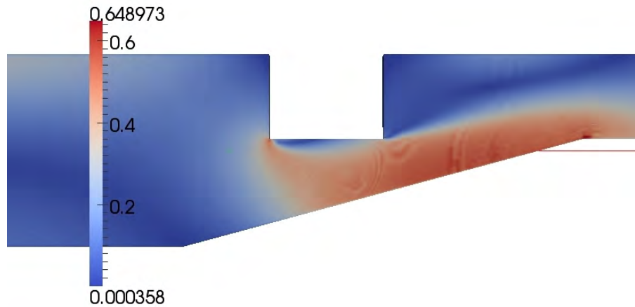
Figure 76 Mach number of upstream of 8.5 MPa at 313 kg/m 3 , and downstream of 7.6 MPa
