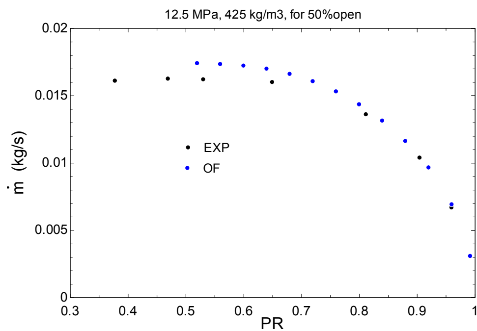
Figure 67 Comparison of experiment and simulation for test valve for 12.5 MPa at 425 kg/m 3 at 50% open
