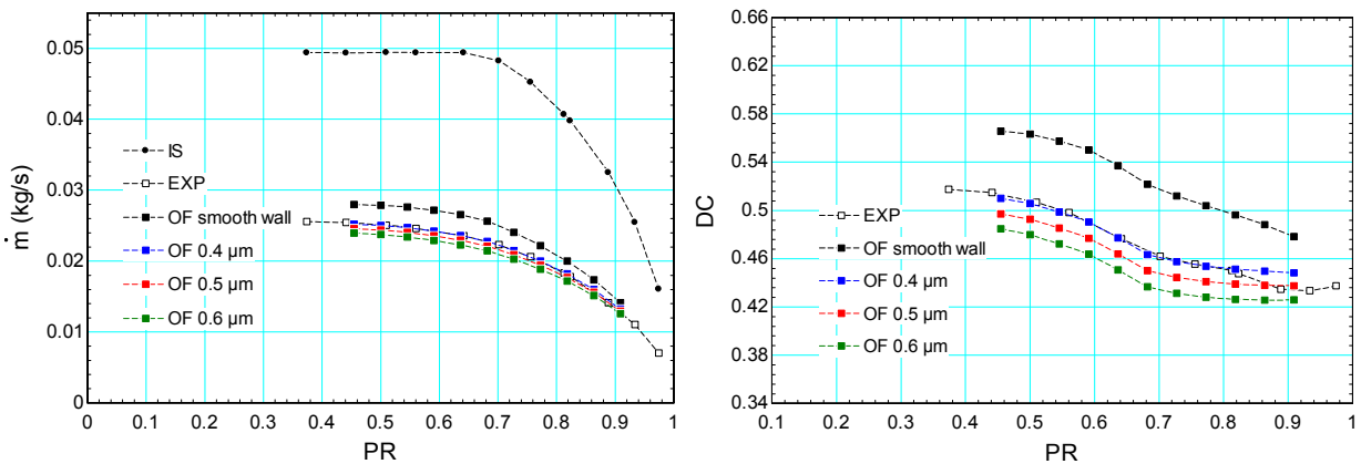
Figure 93 Long annular orifice data for inlet condition of 11 MPa, 498 kg/m 3
