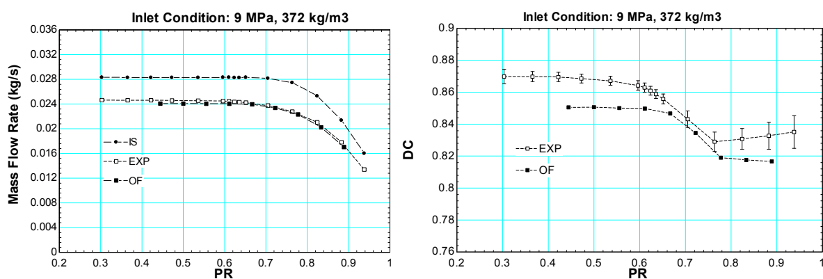
Figure 86 Circular orifice data for inlet condition of 9 MPa, 372 kg/m 3
