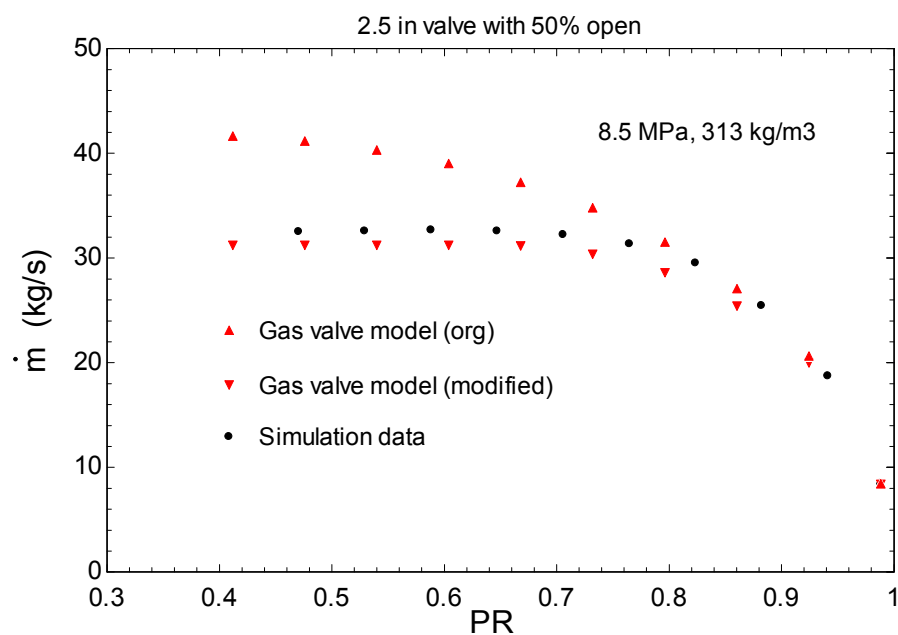
Figure 74 Globe valve with 50% open with upstream condition of 8.5 MPa at 313 kg/m 3
