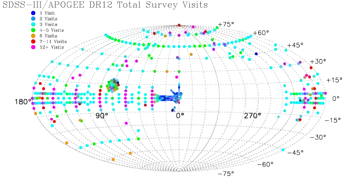
Figure 7. Sky coverage of APOGEE DR12 observations in Galactic coordinates. The number of visits to each field is denoted by the color coding from 1 visit (blue) through 12 or more visits (magenta).
