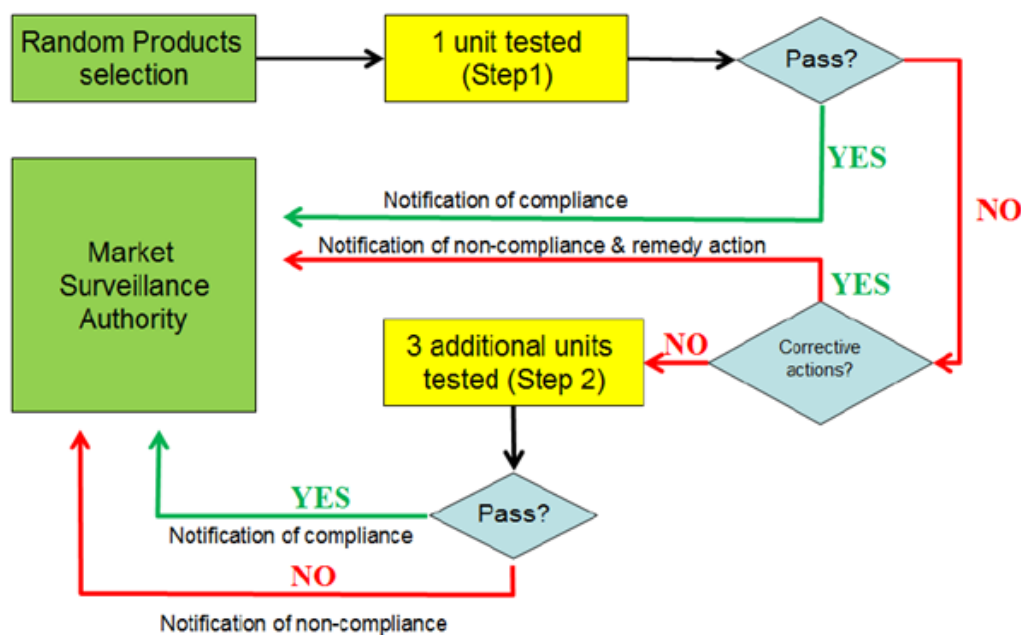
Figure 7: ATLETE recommended procedure for appliance verification (check-testing), Source: ATLETE 2011
