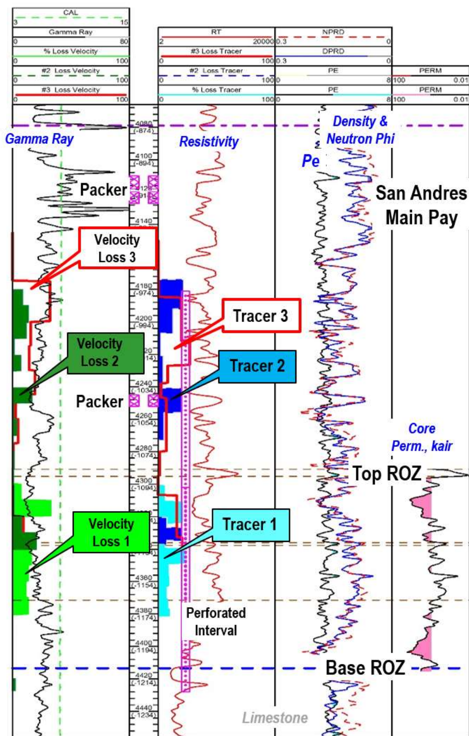
Figure 4.10. Time-Lapse CO 2 Injection Profiles for GLSAU #204R
