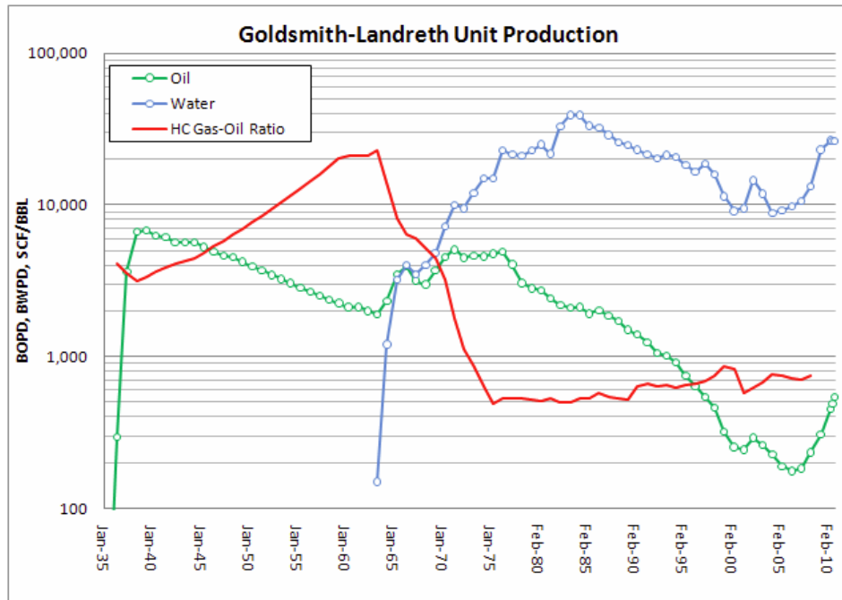
Figure 3.15. Field production performance plot
