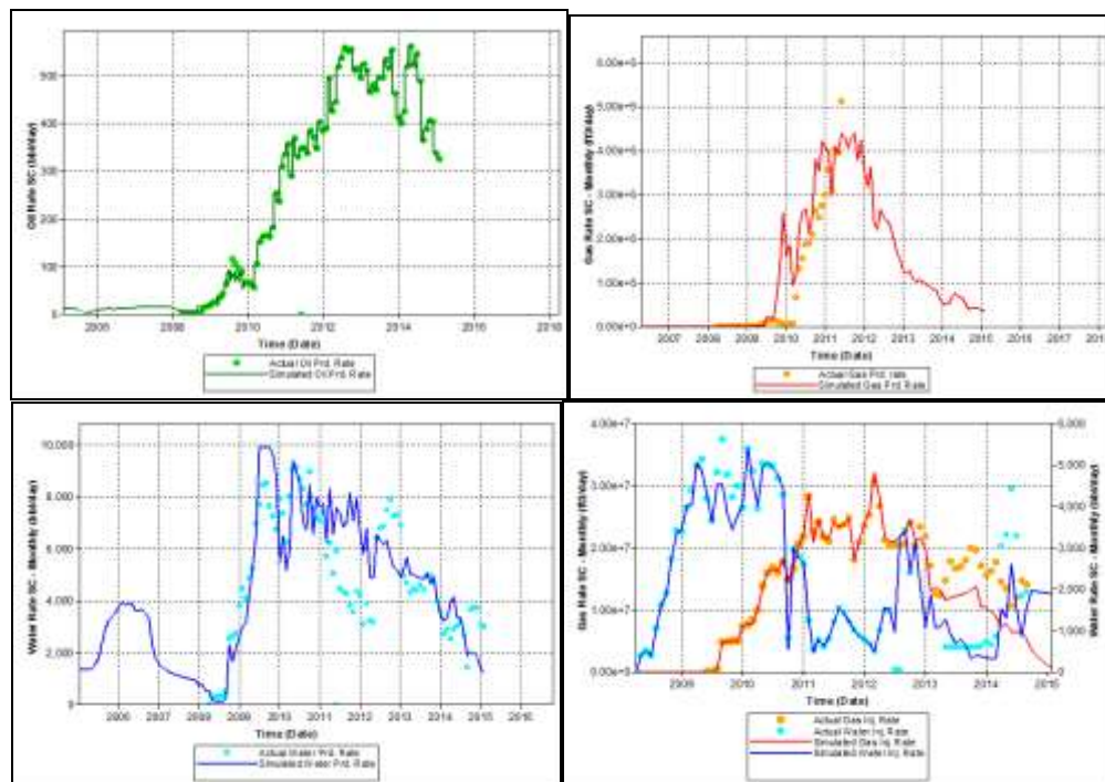
Figure 3.20. Oil, gas, water production rate and gas/water injection rate, post-2008
