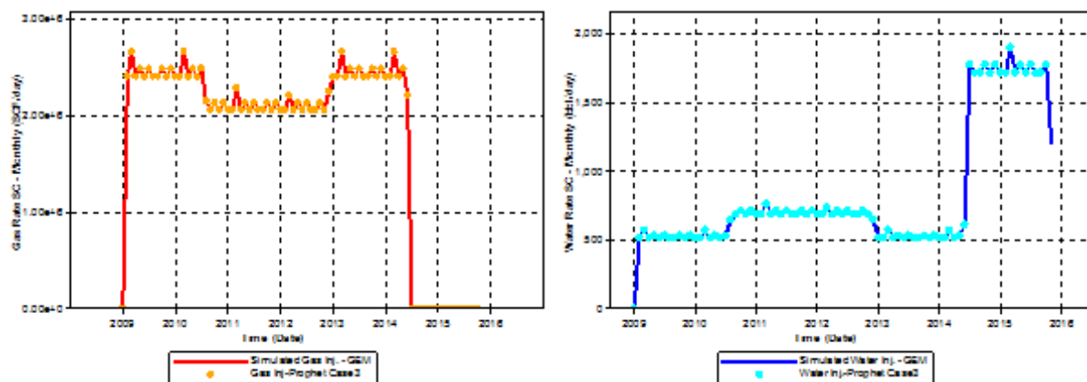
Figure 3.30. Gas (Left) and water injection (Right) in the upper ROZ
