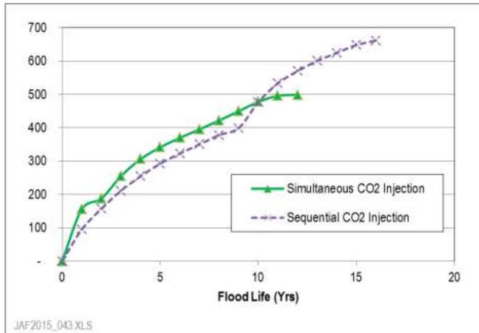
Figure 4.23 Cumulative Oil Production (MBbls)
