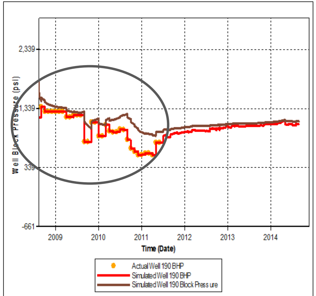
Figure 3.24. BHP and block pressure in well#190 (The circle highlights BHP control)
