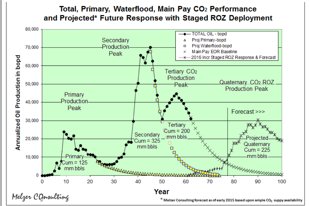
Figure 5.10 – SSAU Production History and Future Forecasted Response
