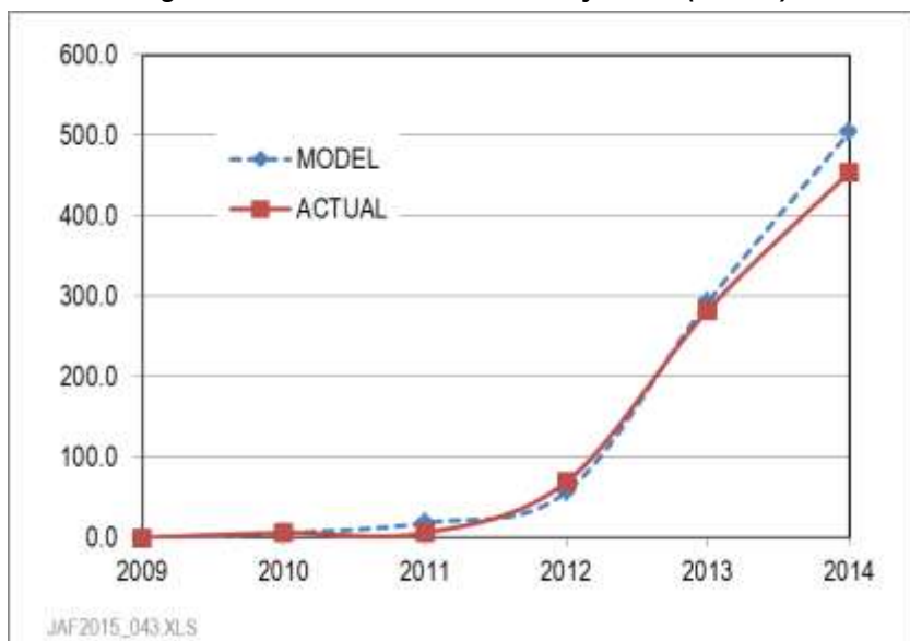
Figure 4.20. Cumulative Water Injection (MBbls)
