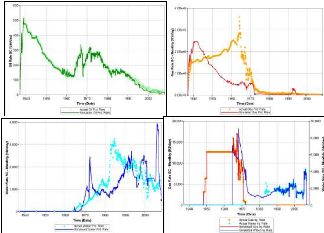
Figure 3.19. Oil, gas, water production rate and gas/water injection rate, pre-2008
