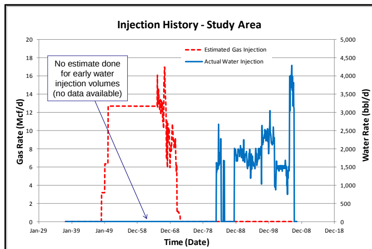
Figure 3.17. Estimated injection rate in the area of study prior to 2008
