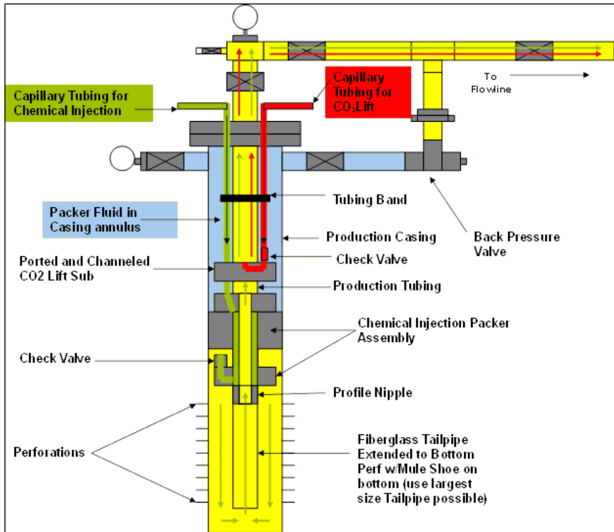
Figure 4.4a - Exterior Banded Capillary Tube System – Selected Method
