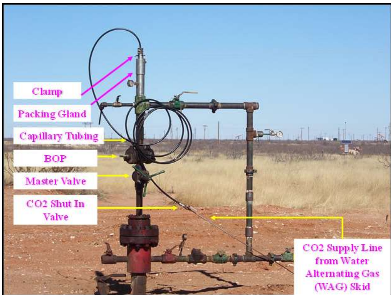
Figure 4.2 - Concentrically Installed Gas Lift – Methods 1-3
