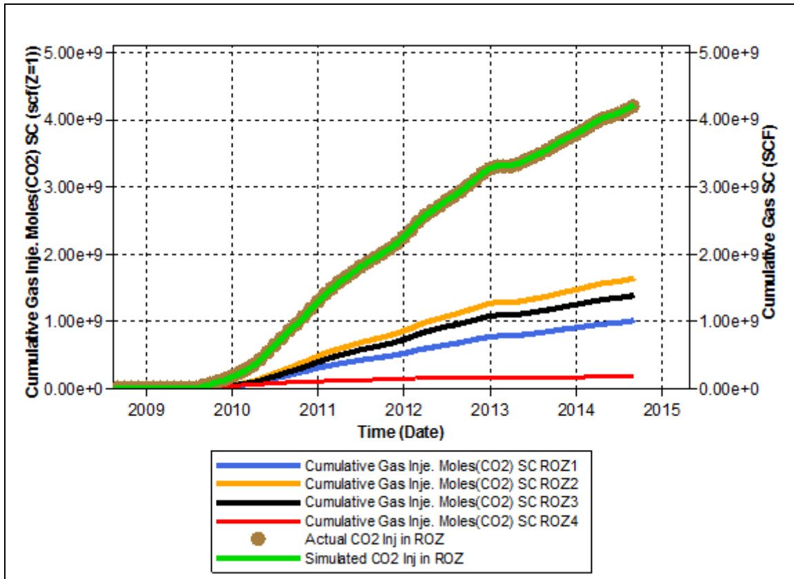
Figure 3.26. CO 2 injection per ROZ layer, #190 pattern
