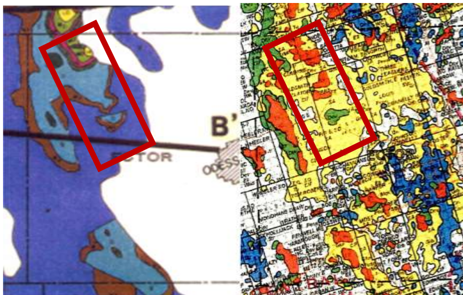
Figure 2.7. Detail from Spine of Platform map (fig 2.4) showing location of Goldsmith Field relative the deep, lower Paleozoic cored structural elements formed during Permo-Penn.
