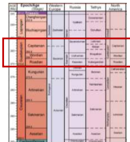
Figure 2.1. Permian Geologic Time Scale. Geologic Time Scale Foundation, 2015.
