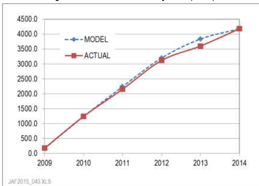
Figure 4.21. Cumulative CO2 Injection (Mmcf)
