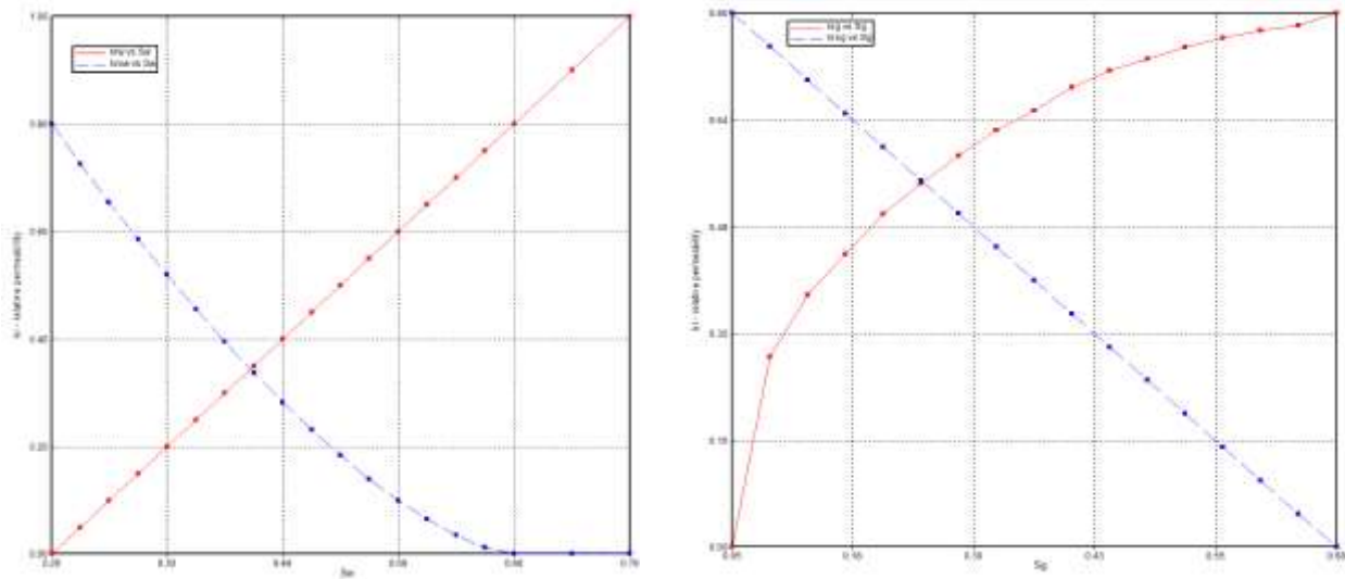
Figure 3.10. Relative permeability curves used in the model
