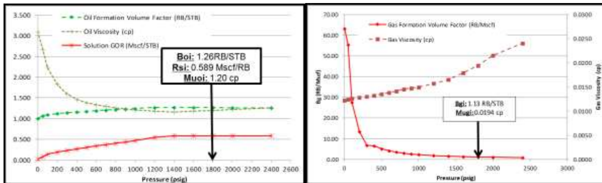
Figure 3.7. Fluid PVT Data - Source: AMOCO Report
