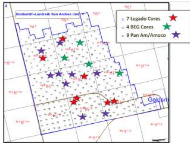
Figure 3.2. Core data coverage across the field.
