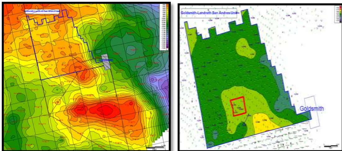
Figure 3.3. Top of San Andres structure (Left) and Base of ROZ (Right)
