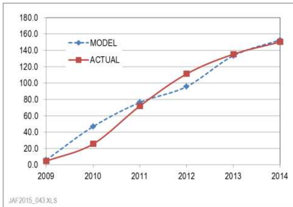
Figure 4.22 Cumulative Oil Production (History Match) (MBbls)
