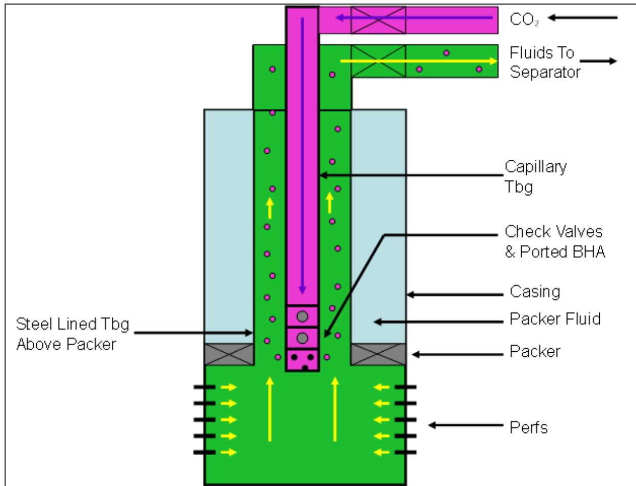
Figure 4.3 - Flowing Well with Concentric Gas Lift Installed
