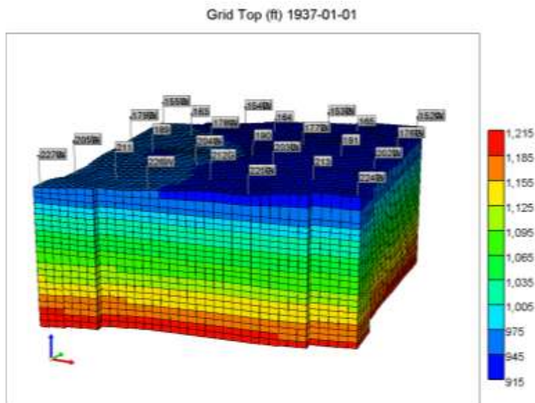
Figure 3.13. 3-D structure of the model and well locations
