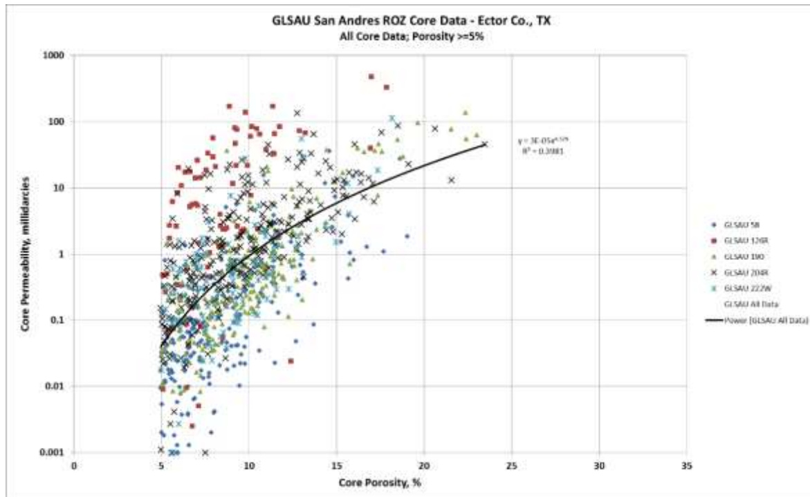
Figure 3.6. Porosity-permeability correlation in ROZ
