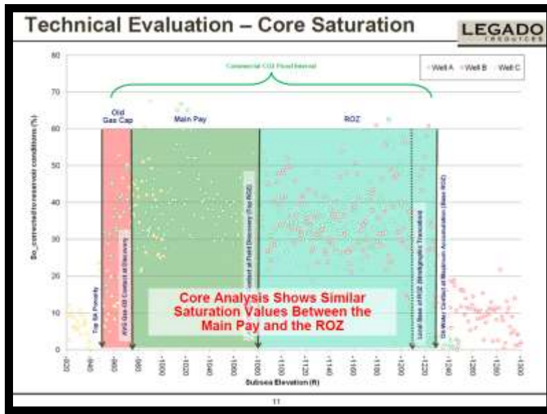
Figure 3.8. Core saturation analysis result in GC, MPZ and ROZ. 2
