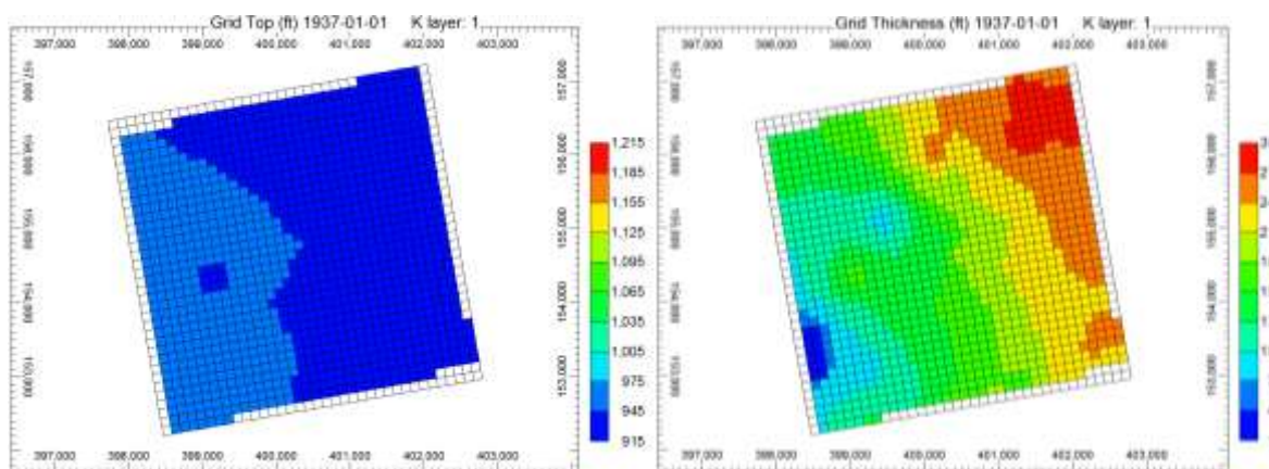
Figure 3.5. The top (Left) and thickness (Right) maps in the first layer
