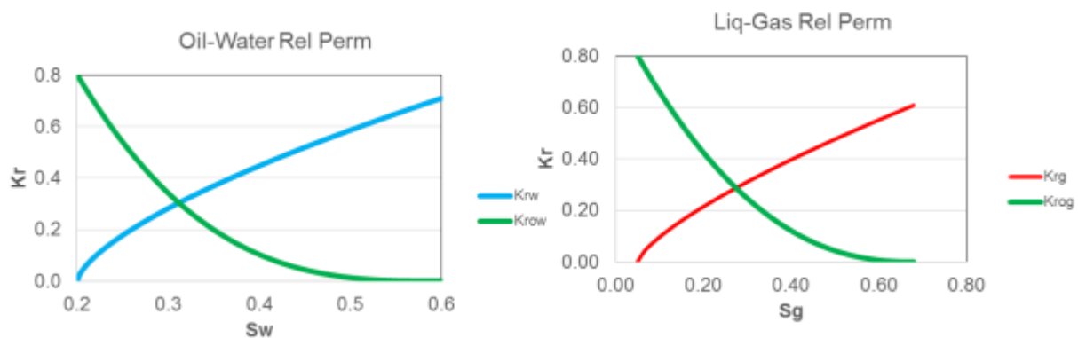
Figure 3.22. Water-oil and liquid-gas relative permeability curves
