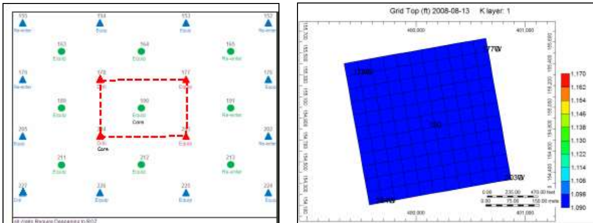
Figure 3.21. Location of the wells and #190 pattern in the study area (Left), the top structure of the pattern model (Right)
