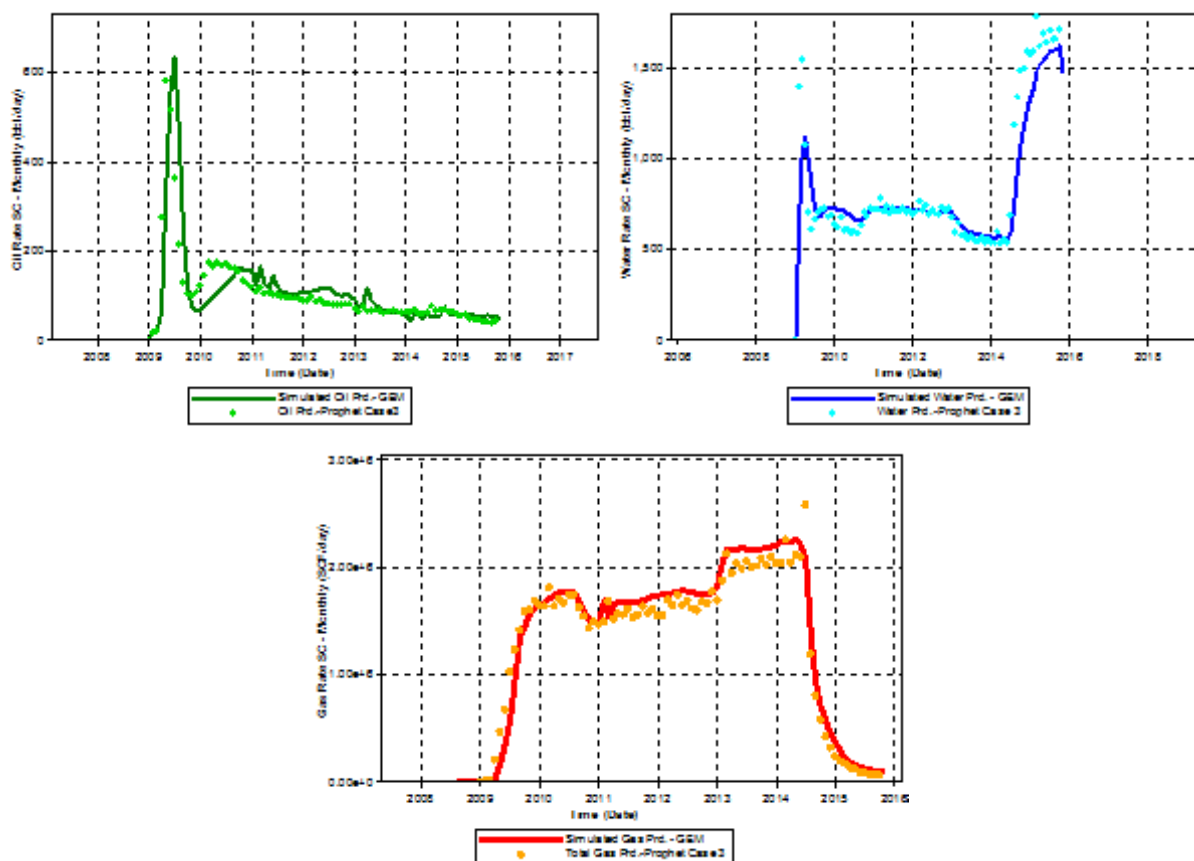
Figure 3.31. Oil (Top Left), water (Top Right), and total gas production (Bottom)
