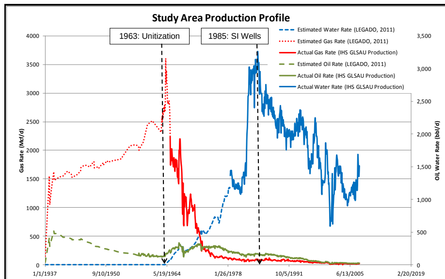
Figure 3.16. Phase I area production history
