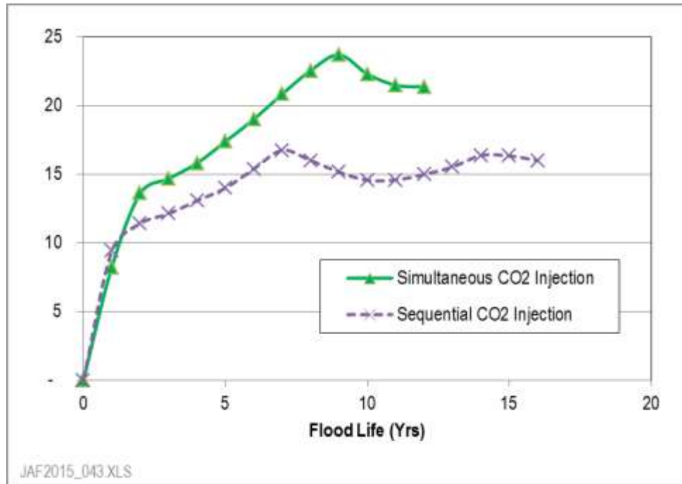
Figure 4.24 CO 2 Ratio (Mcf/B)
