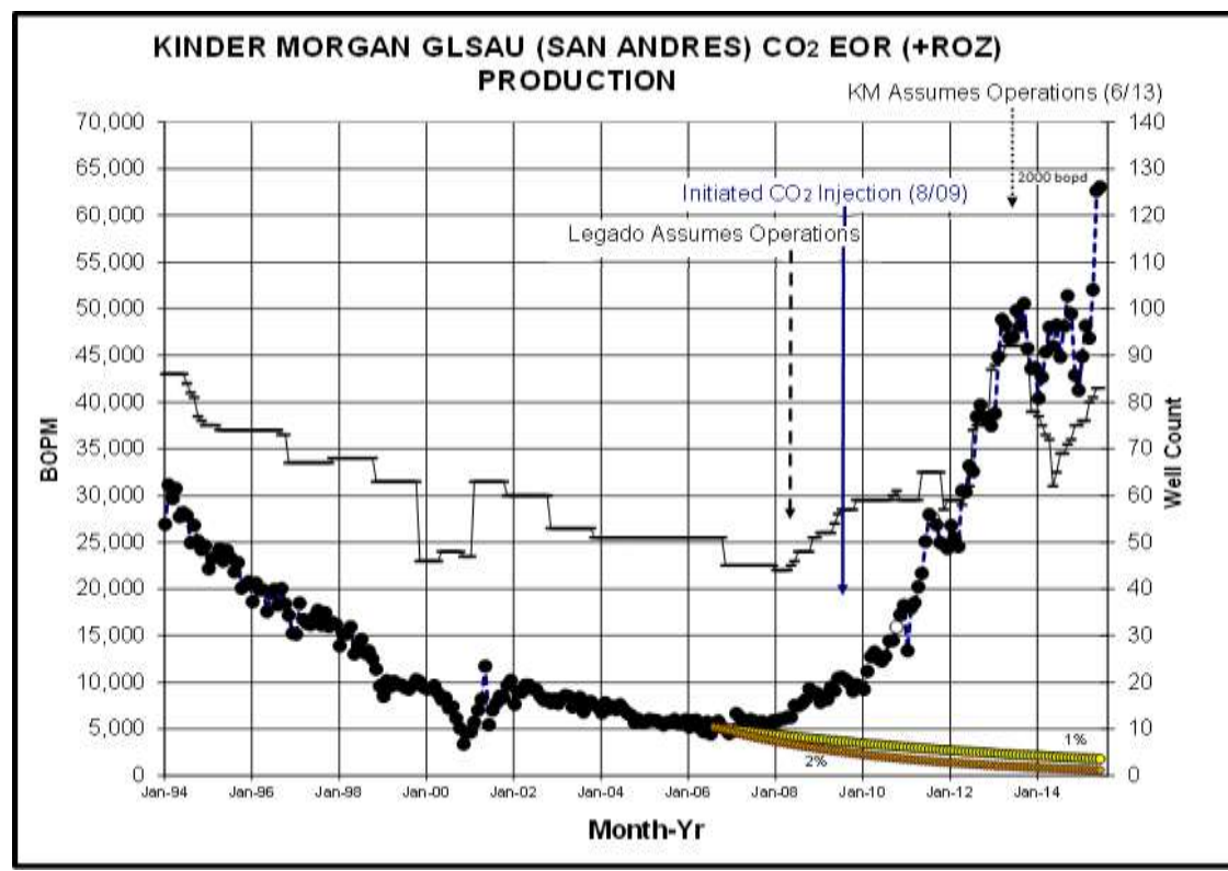
Figure 5.13 – GLSAU Production History: Jan 94 – Jun 15
