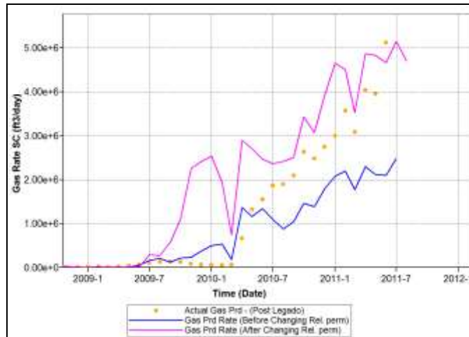
Figure 3.18. Effect of modifying relative permeability on gas production
