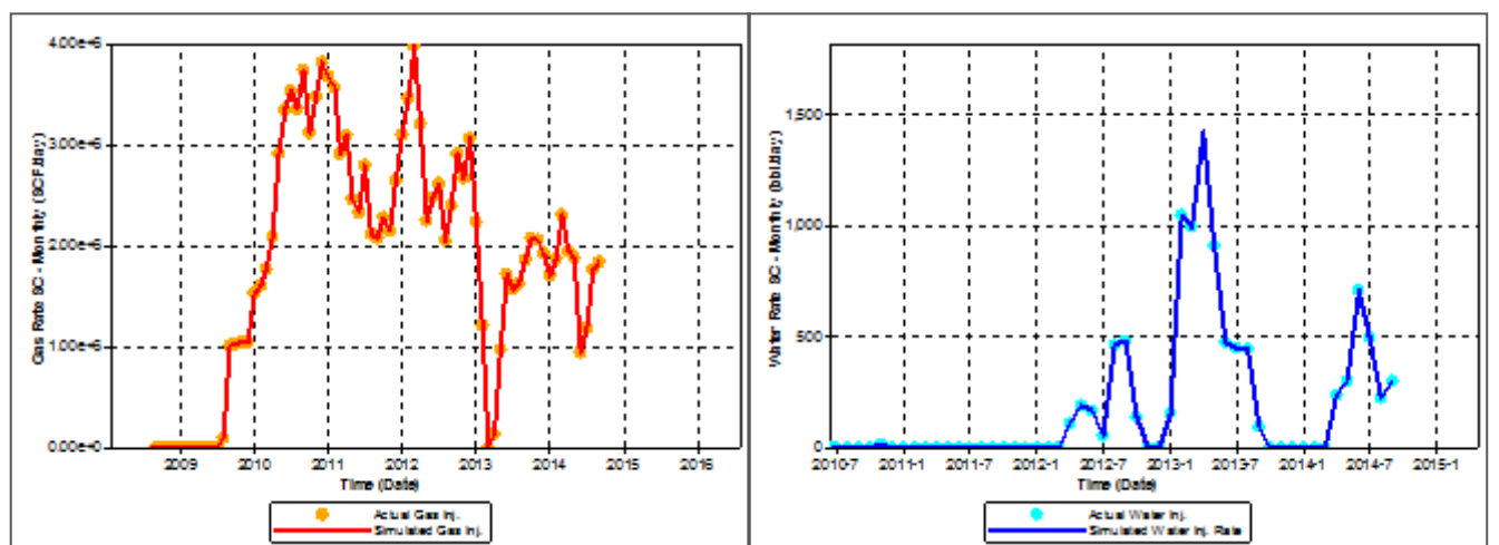
Figure 3.25. CO 2 and water injection in ROZ for the #190 pattern
