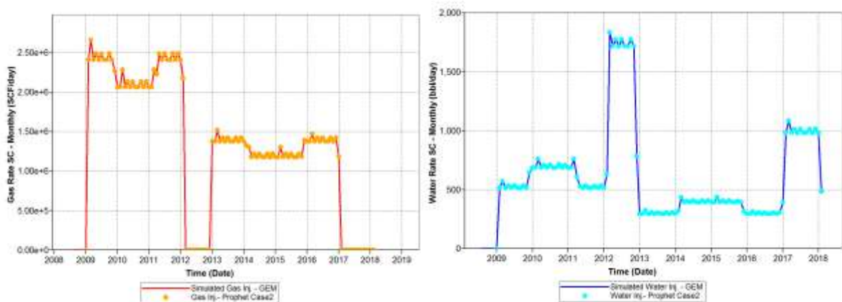
Figure 3.28. Gas (Left) and water injection (Right) profiles
