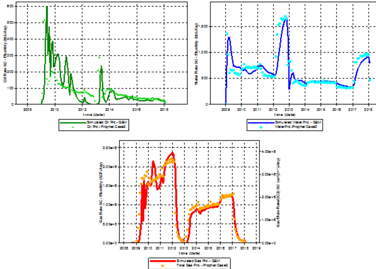
Figure 3.29. Oil (Top Left), water (Top Right), and total gas production (Bottom)
