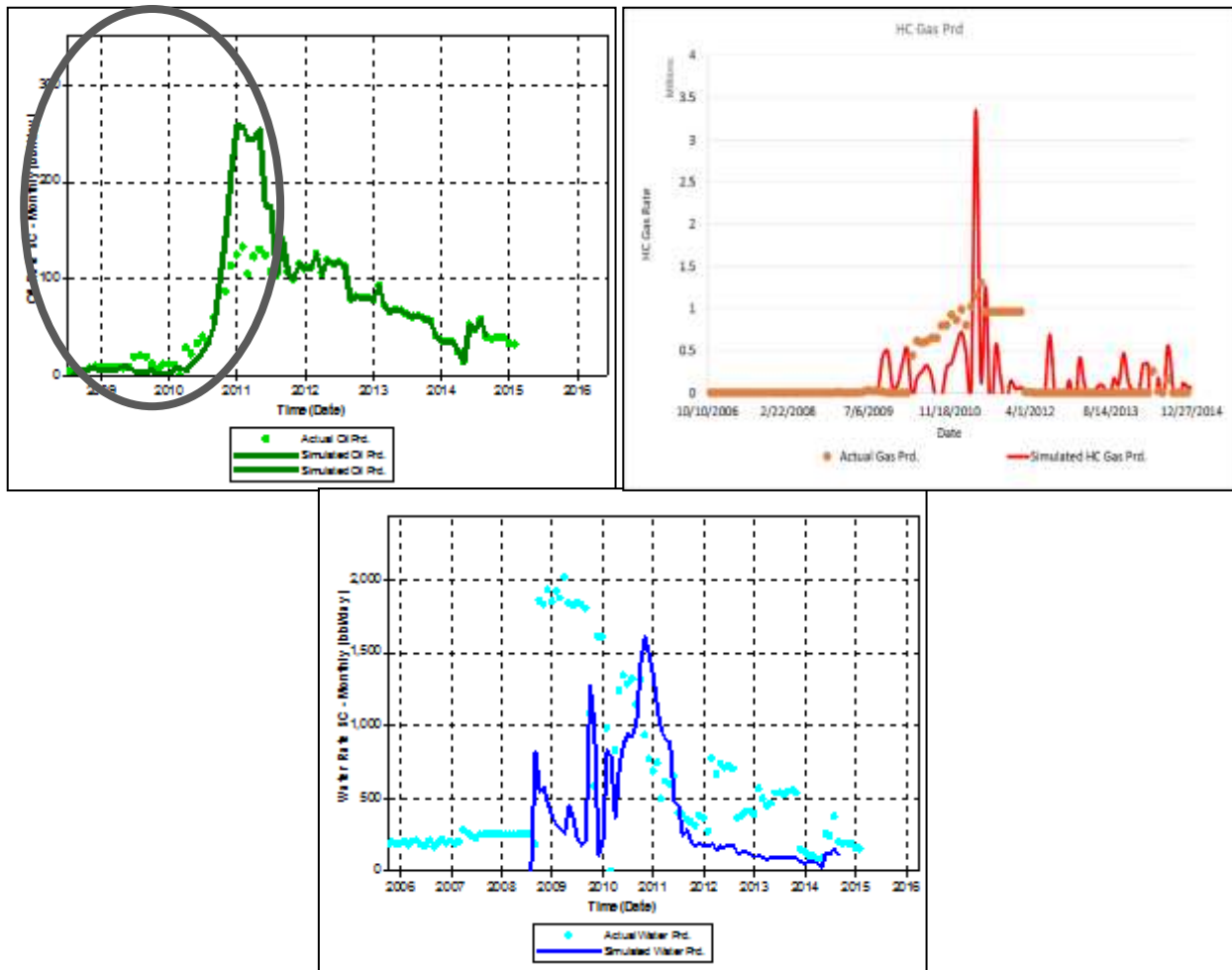
Figure 3.23. Oil, HC gas and water production in the ROZ for the #190 pattern (highlighting ramp up in oil production).
