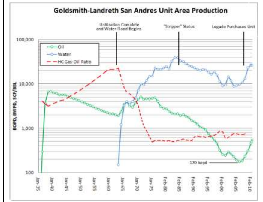
Figure 5.11 – GLSAU Unit Area Production History
