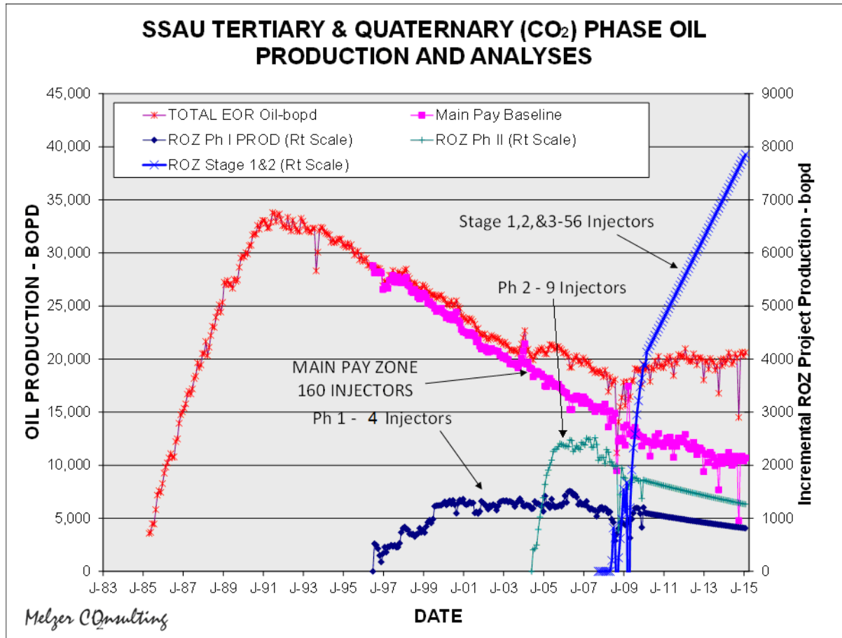
Figure 5.8 – CO 2 Era Production at SSAU by Individual Project
