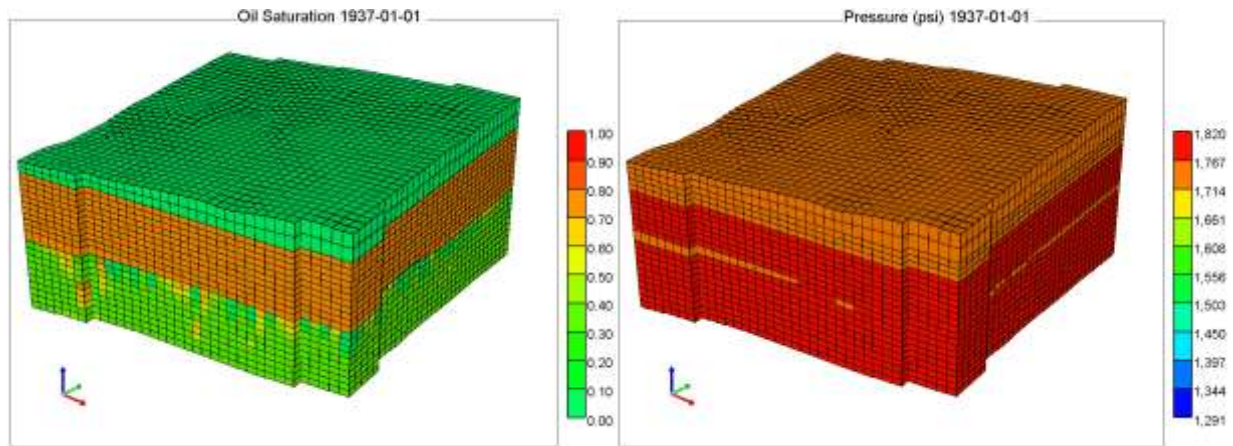
Figure 3.9. 1937 Initial oil saturation (Left) and Pressure (Right) distribution in the reservoir
