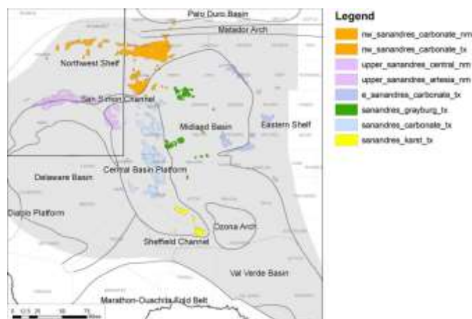
Figure 2.2. Major producing areas and play types or “trends” in the San Andres from Dutton et.al., 2005.
