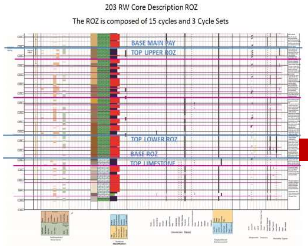
Figure 2.16. Goldsmith Landreth San Andres Unit #203RW core description. The heavy red bar on the right is the interval with increased saturation, believed to be in the CO 2 flood related oil bank. Thin red lines are Cycle boundaries, thicker red lines are Cycle Set boundaries.
