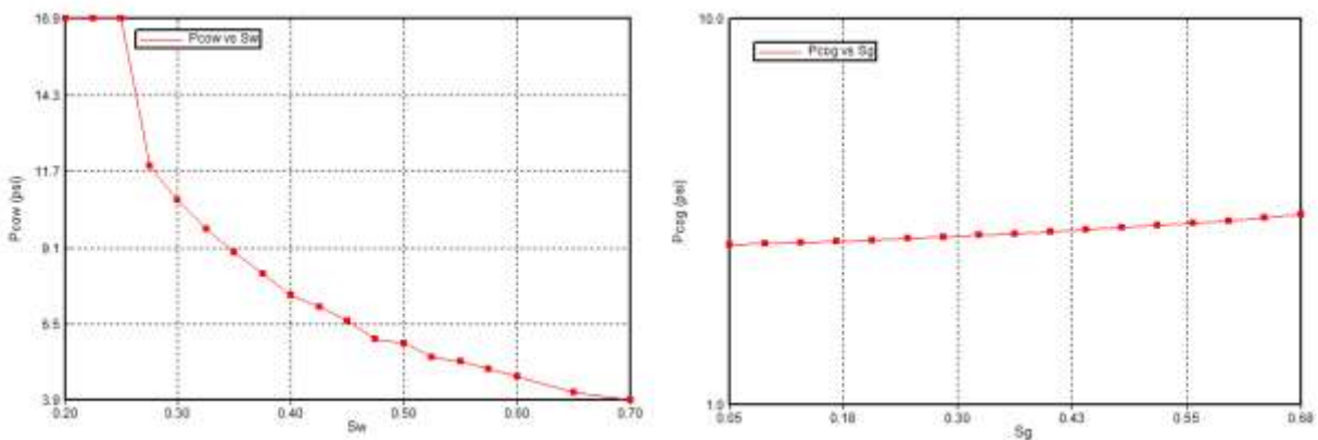
Figure 3.11. Oil-Water (Left) and Gas-Oil (Right) capillary pressure curves
