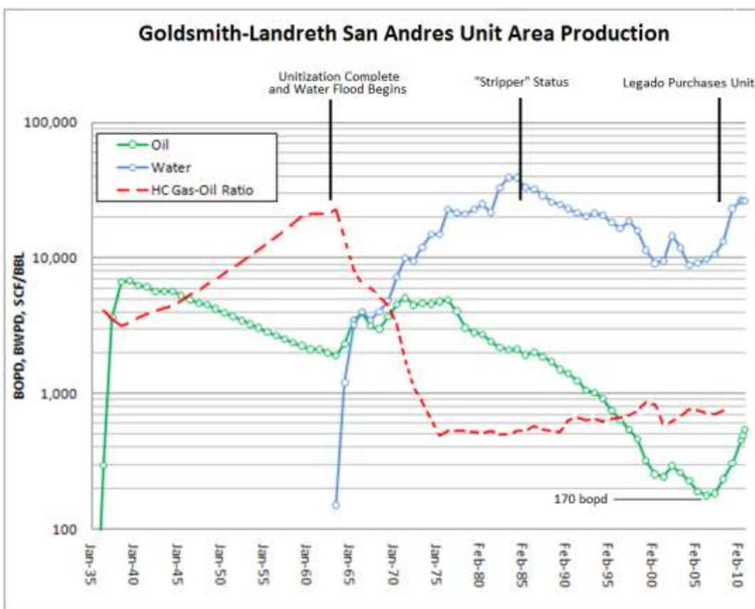
Figure 1.2 – GLSAU Unit Area Production History
