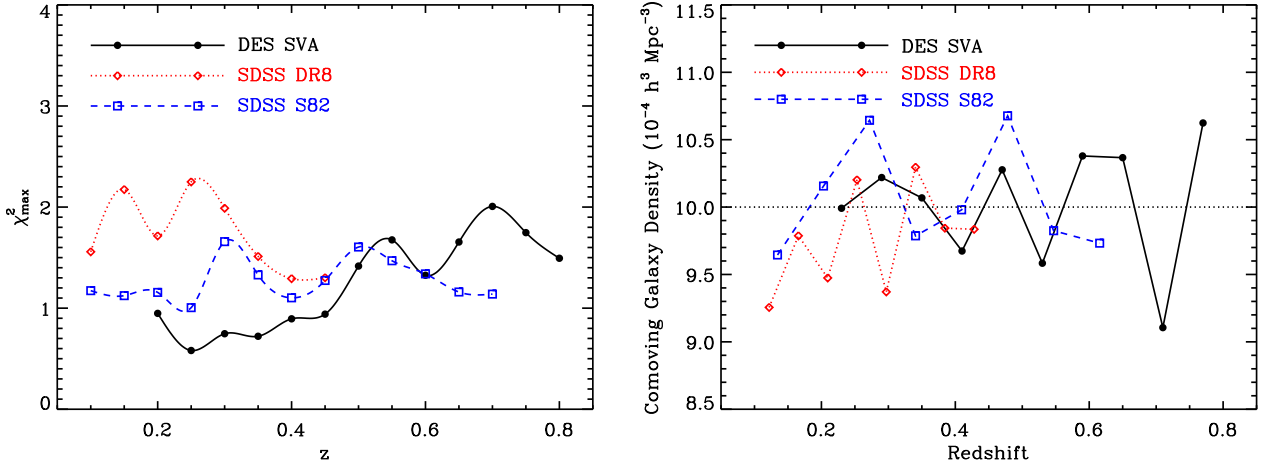
Figure 2. Left: Selection cut \chi^2_{\text{max}} as a function of redshift defining each of the redMaGiC galaxy samples, as labelled. The symbols mark the spline nodes defining the function \chi^2_{\text{max}}(z) , while the lines show the corresponding spline interpolation at every point. Right: redMaGiC comoving galaxy density as a function of redshift for each of the three data sets employed in this work, as labelled. The target comoving space density was 10^{-3} h^3 \text{ Mpc}^{-3} (horizontal dotted line).
