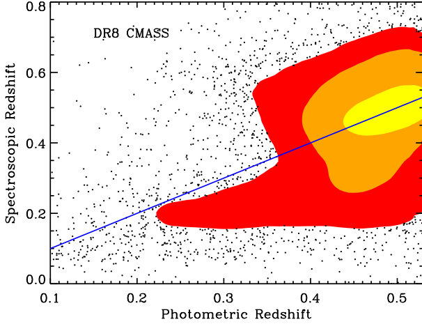
Figure 9. Left: Spectroscopic vs. photometric redshifts for CMASS galaxies using SDSS photo-zs. Colored regions contain 68%, 95%, and 99% of the points. The remaining 1% of galaxies are shown as points. The blue line is the y = x line. Right: As left panel, but for redMaGiC galaxies.
