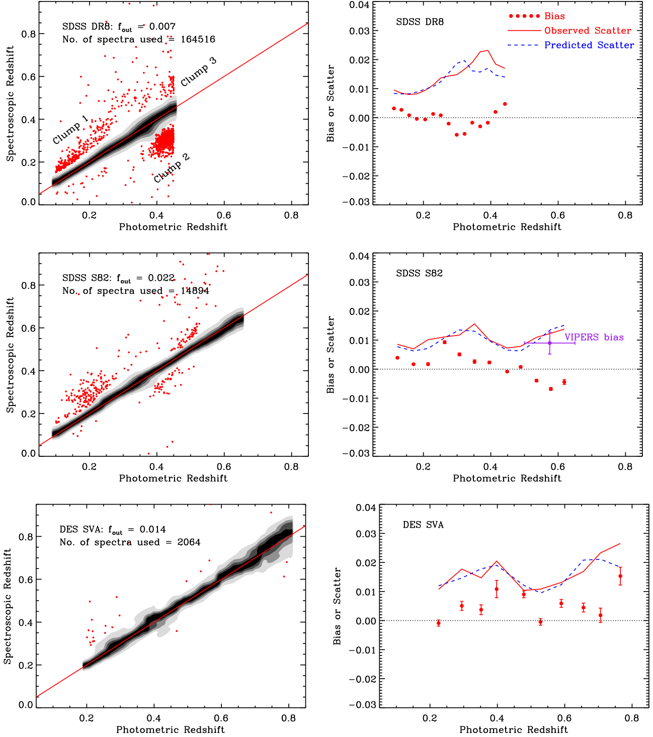
Figure 3. Left: Spectroscopic redshift vs photometric redshift for the fiducial redMaGiC galaxy sample in each of the various data sets considered in this work. Red points are 5\sigma outliers, while the red line corresponds to z_{\text{spec}} = z_{\text{photo}} . Right: Photometric redshift performance statistics. Red points with error bars are the photometric redshift bias, defined as the median value of z_{\text{spec}} - z_{\text{photo}} . All statistics for the SDSS data sets are computed using SDSS spectroscopy, except for the purple VIPERS point for S82. The red curve is the observed scatter of (z_{\text{photo}} - z_{\text{spec}})/(1 + z_{\text{spec}}) , while the dashed blue curve is the predicted scatter based on the available photometry. The horizontal error bar for the S82 plot shows the width of the redshift bin used in the VIPERS measurement.
