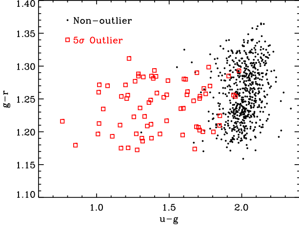
Figure 13. Distribution of our fiducial S82 redMaGiC galaxy sample in u - g and g - r space for galaxies in the photometric redshift bin z_{\text{photo}} \in [0.18, 0.22] . Black points are galaxies where our photometric redshift estimate agrees with the spectroscopic estimate within 2\sigma , while red points correspond to \geq 5\sigma redshift outliers.
