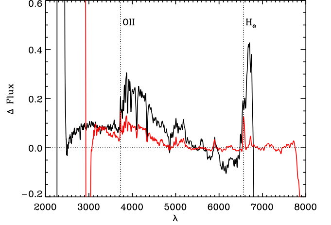
Figure 15. Difference between the outlier and non-outlier stacked rest-frame spectra for Clump 1 (red) and Clump 3 (black) galaxies (see Figure 3). The vertical dotted lines mark the [OII] (left-most line) and H\alpha (right-most line) emission lines. Clump 3 galaxies are qualitatively similar to those in Clump 1, with residual star formation that is not large enough to drive the galaxy from the photometric red sequence at SDSS depths.
