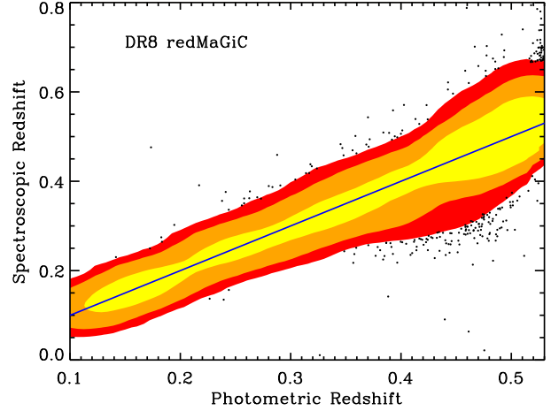
Figure 9. Left: Spectroscopic vs. photometric redshifts for CMASS galaxies using SDSS photo-zs. Colored regions contain 68%, 95%, and 99% of the points. The remaining 1% of galaxies are shown as points. The blue line is the y = x line. Right: As left panel, but for redMaGiC galaxies.
