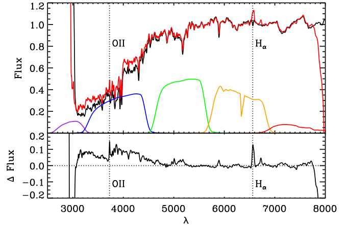
Figure 12. Top panel: Stacked rest-frame spectra for redMaGiC galaxies with z_{\text{photo}} \in [0.18, 0.22] . Outlier galaxies are shown in red (Clump 1 in Figure 3), and non-outliers in black. Also shown are the SDSS ugriz transmission curves for an extended source at z = 0.2 assuming 1.3 air masses (purple, blue, green, orange, red). Bottom panel: Difference between the two spectra in the top panel, showing the excess emission associated with the outlier galaxy population. The vertical dotted lines mark the [OII] (left-most line) and H\alpha (right-most line) emission lines. Clump 1 galaxies have excess blue light, as well as [OII] and H\alpha emission indicative of a small amount of residual star formation.
