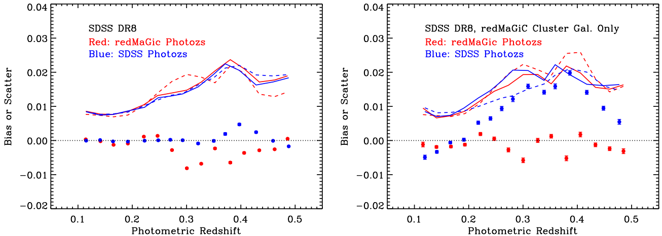
Figure 7. Left: Comparison of the photometric redshift performance of redMaGiC (red) and SDSS photo-zs for redMaGiC galaxies (blue). This plot uses SDSS spectroscopic redshifts to compute the redshift bias and scatter of the redMaGiC photo-zs, and is therefore limited to the brightest redMaGiC galaxies. Points with error bars show the median redshift bias for each of the two samples. Solid lines show the observed photo-z scatter, while dashed lines show the predicted scatter. Right: As for the left panel, only now we test the photo-z performance of the sub-sample of redMaGiC galaxies that are members of redMaPPer clusters. For these galaxies, we assign the photometric redshift of the host redMaPPer clusters as the “spectroscopic” redshift of the redMaGiC galaxy for the purposes of computing photometric redshift biases and scatter. By doing so, we can test the accuracy of the photometric redshifts of faint redMaGiC galaxies with no spectroscopic redshift.
