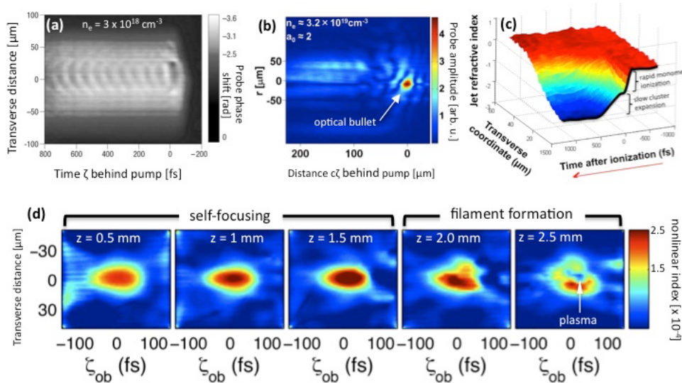
Fig. 2. Examples of single-shot visualization of laser-plasma structures by the PI. (a) Laser wake in plasma of density n_e = 3 \cdot 10^{18} \text{ cm}^{-3} , showing relativistically curved wave fronts [Matlis06]; (b) “optical bullet” of probe light trapped inside a co-propagating plasma bubble [Dong10]; (c) “Texas two-step”: fs evolution of the refractive index of a clustered plasma behind a fs ionization/heating pulse, consisting of instantaneous monomer ionization (step 1) followed by delayed cluster expansion (step 2), used to measure cluster mass fraction in-situ [Gao 12,13]; (d) 5 frames of a single-shot tomographic movie of self-focusing and filament formation by a 100 fs laser pulse in a fused silica Kerr medium [Li13].
