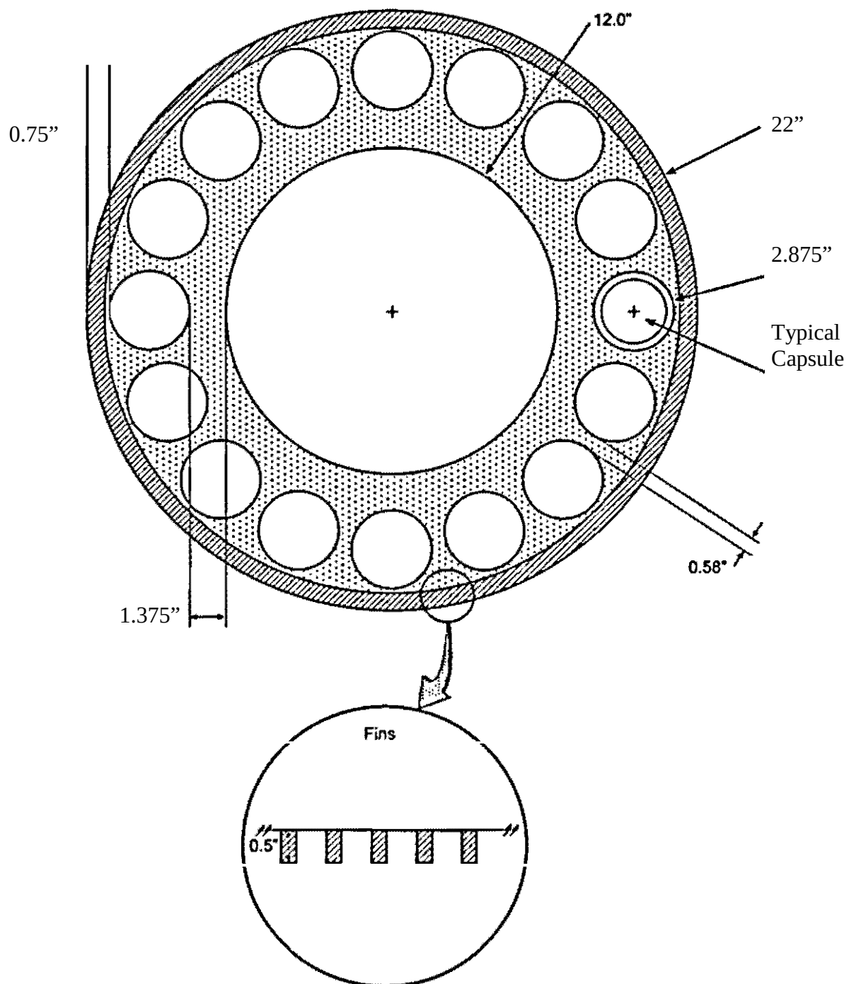
Figure 4-4. Plan View of the CAP Conceptual Design for Dry Storage Overpack with External Fins and a Monolithic Insert Holding 16 Capsules
