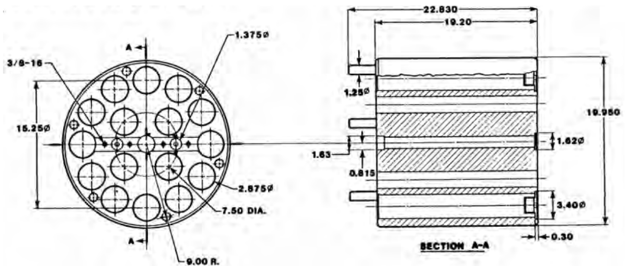
Figure 4-11. Schematic for a Basket Configuration with Capacity for 16 Capsules
