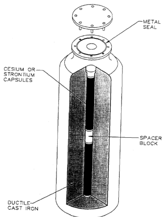
Figure 4-2. Proposed Storage Canister for Cs and Sr Capsules
