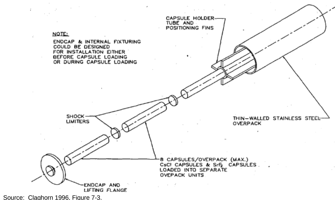
Figure 4-3. A Disposal Overpack Concept for Cs and Sr Capsules
