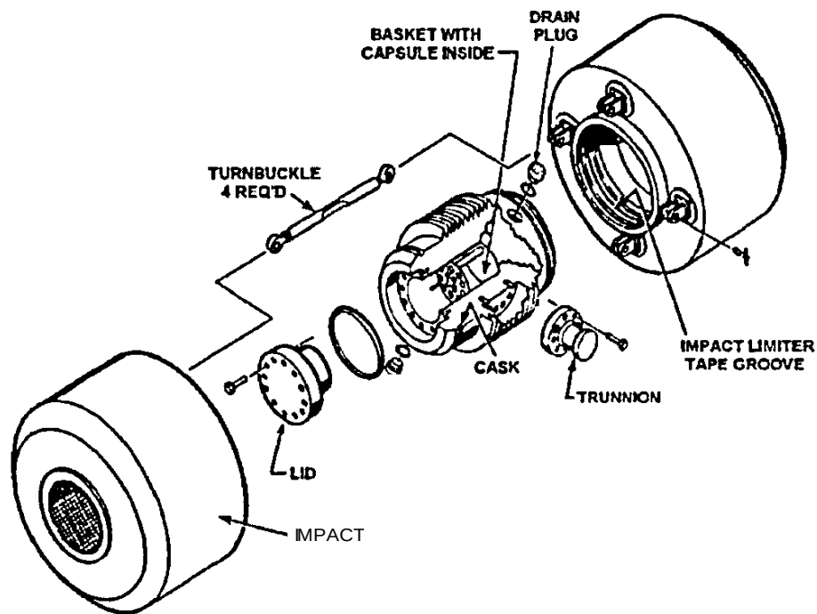
Figure 4-10. Schematic Diagram of the BUSS Cask
