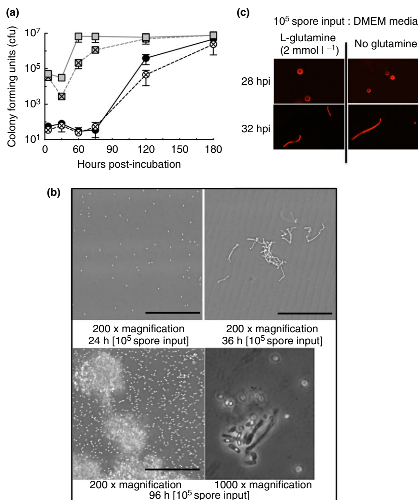
Figure 2 (a) Multiday-time course of heat-resistant spore formation vs total bacterial count at initial 100 and 100 000 spore doses. Total bacteria from 10^5 input-□, heat-resistant spore only from 10^5 input-⊗, total bacteria from 10^2 input-●, heat-resistant spore only from 10^2 input-⊗. were incubated in Dulbecco's modified eagle medium (DMEM) + 2 \text{ mmol l}^{-1} L-glutamine and no serum at 37^\circ\text{C} and 5\% \text{ CO}_2 for a total of 7.5 days (180 h). Standard deviation represents triplicate wells harvested for each time point and no <5 collective plate counts. (b) Microscopy images at 24 h show spore only morphology but by 36 h germination was visible. At 96 h resporulation after germination was evident (left) and at higher 1000× magnification (right) the remaining germinating bacteria appeared to also contain phase-bright spores suggesting they were close to completing sporulation. Scale bar is 50 microns. (c) Further analysis through immunofluorescence of spore sample from DMEM incubation indicates that germination began after 28 h but before 32 h and was not influenced by the addition of glutamine, which is critical to ensure cells survive in vitro .
