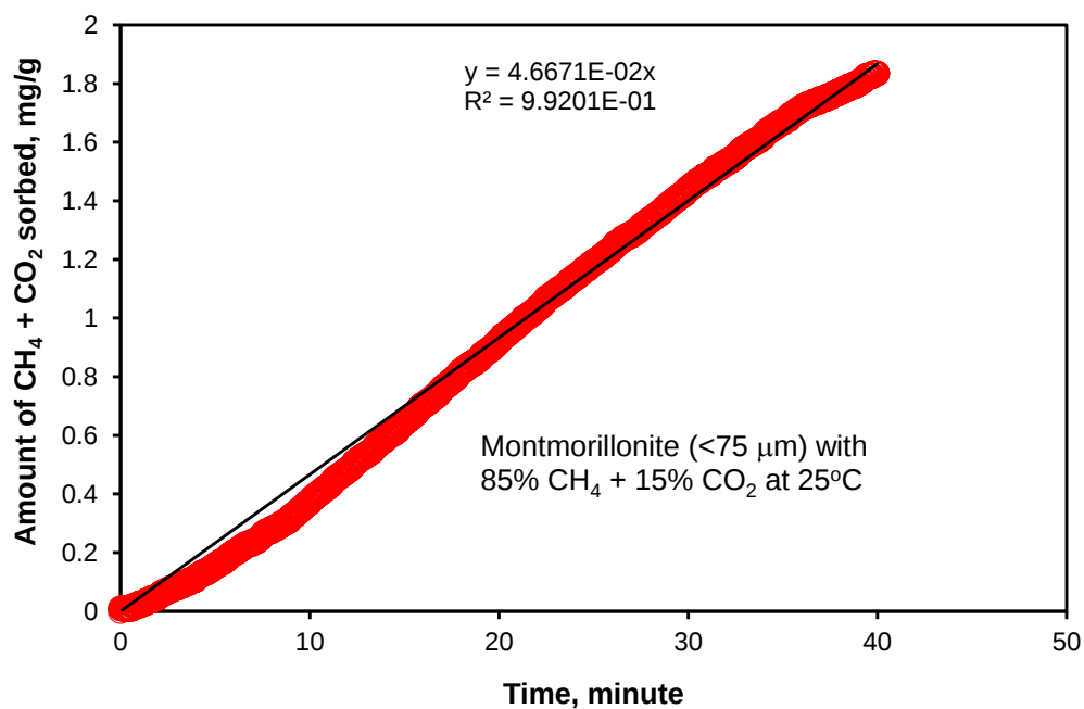
Figure 4. Sorption kinetics with CH 4 + CO 2 for montmorillonite at 25°C temperature and 1 bar
