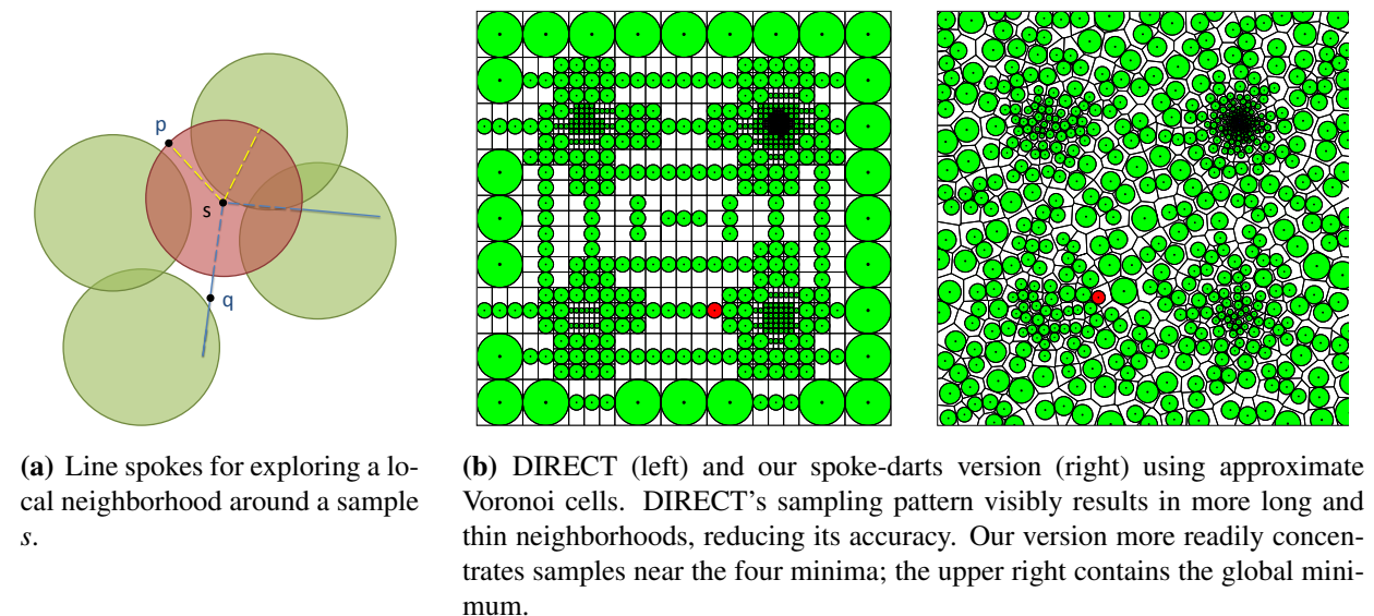
Figure 1.7. Spoke dart sampling and applying it to build a global optimization algorithm.
