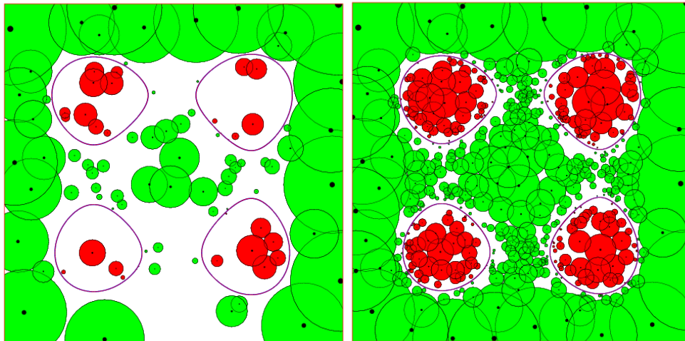
Figure 1.1. Applying POF-Darts to a test problem with four failure regions. After exhausting the sampling budget a GP surrogate is built and utilized to estimate the POF. The failure isocontours from the surrogate are colored in red while the exact one are colored in blue. For this test problem in both cases the isocontours were on top of each other indicating an accurate estimate.
