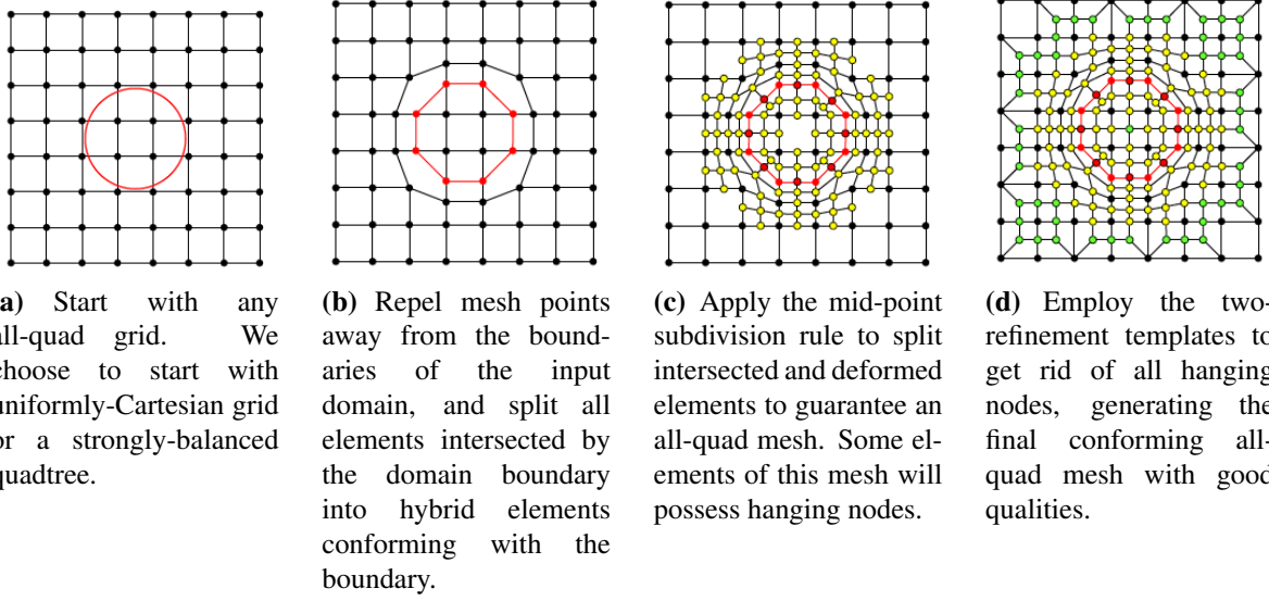
Figure 1.14. “Robust All-Quad Meshing of Domains with Connected Regions” algorithm steps.
