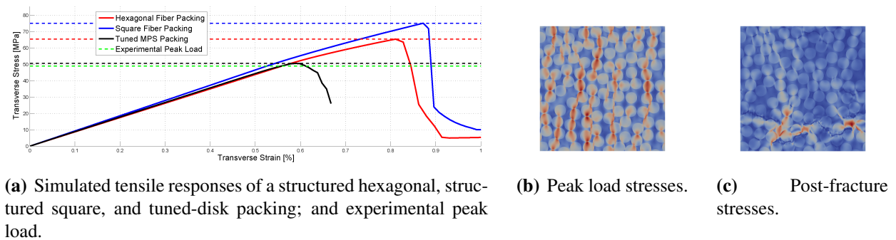
Figure 1.12. Fiber material modeling using “Disk Density Tuning of a Maximal Random Packing.” Tuned disks predict the failure point better than traditional hexagonal or square packings.
