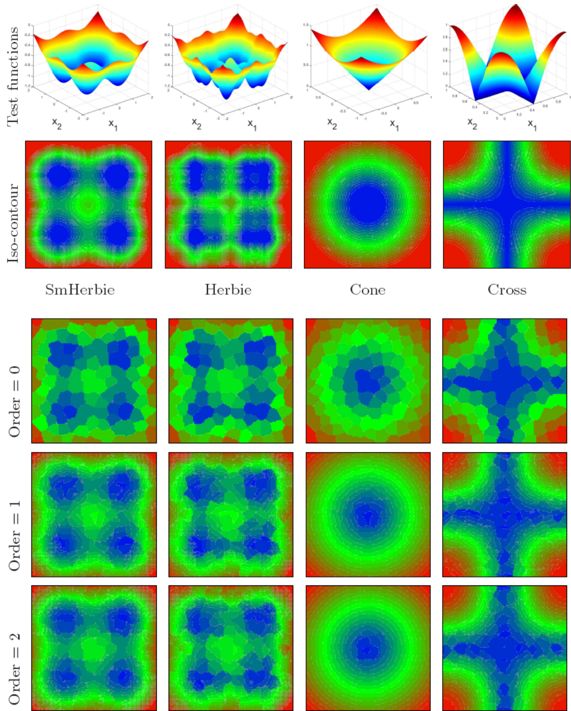
Figure 1.4. VPS surrogates of various orders, compared to the true function and its isocontours.
