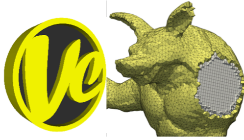
Figure 1.19. An example hex dominant 3D Voronoi mesh reconstructing a surface.
