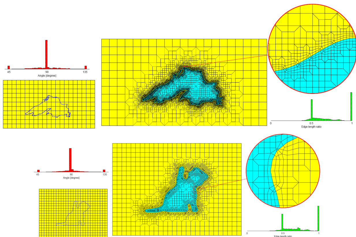
Figure 1.15. “Robust All-Quad Meshing of Domains with Connected Regions” examples.
