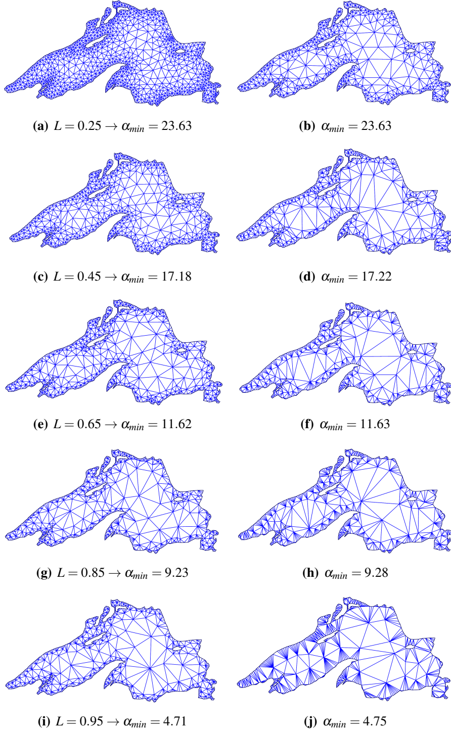
Figure 1.18. Disk-packing sampling meshes discovered the local feature size, without being guided by a prespecified sizing function. Disk radii (inter-point distances) are about the constant L times the local feature size. There is a natural tradeoff between L and the minimum angle \alpha in the mesh.
