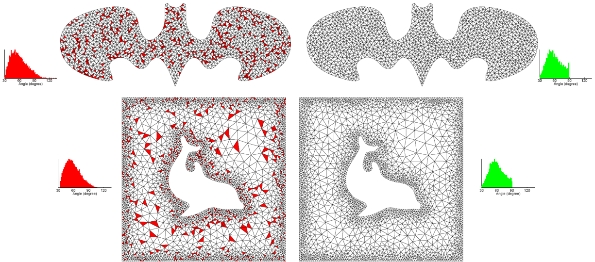
Figure 1.10. Removing obtuse angles in planar meshes using “Disk Density Tuning of a Maximal Random Packing.”
