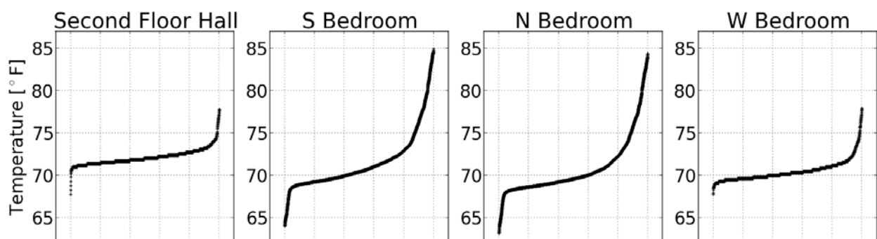
Figure 33. Devens frequency distribution of temperatures
