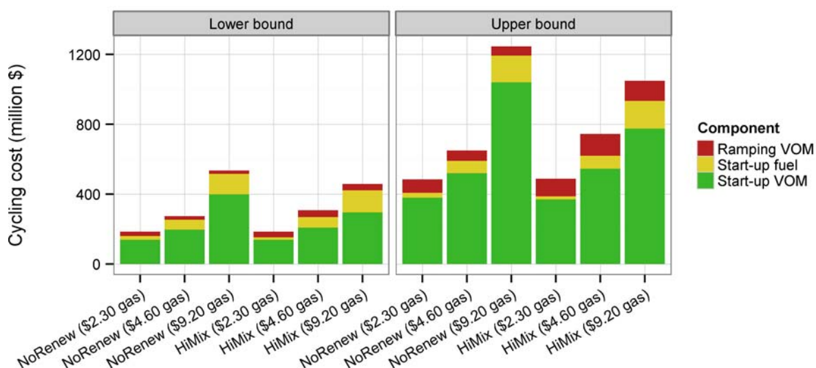
Figure 110. Cycling cost in the gas price sensitivities showing (left) lower and (right) upper bounds
