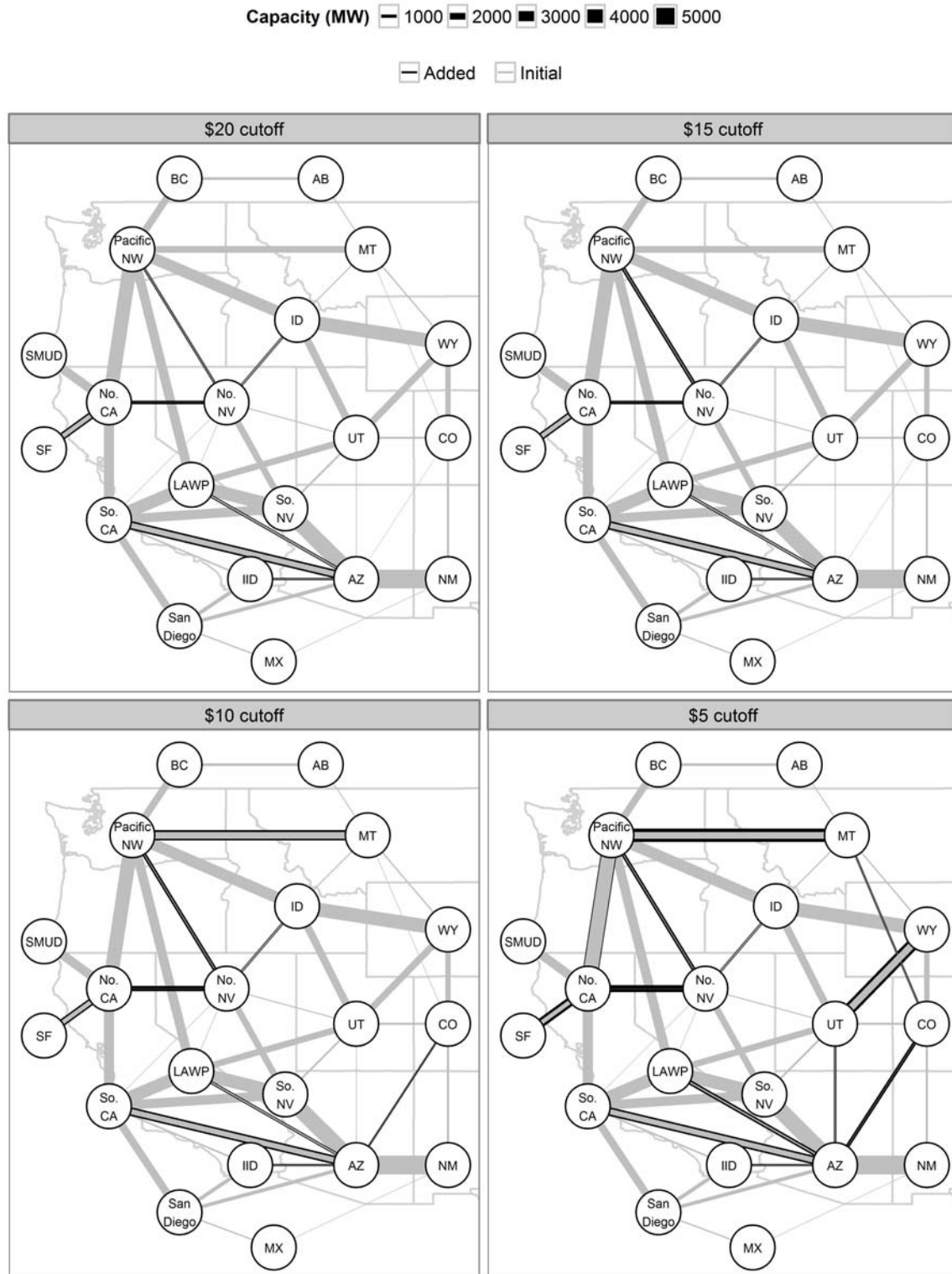
Figure 130. Transmission expansion for the High Mix Scenario showing the (gray) initial and (black) additional transmission for each shadow price cutoff value tested
