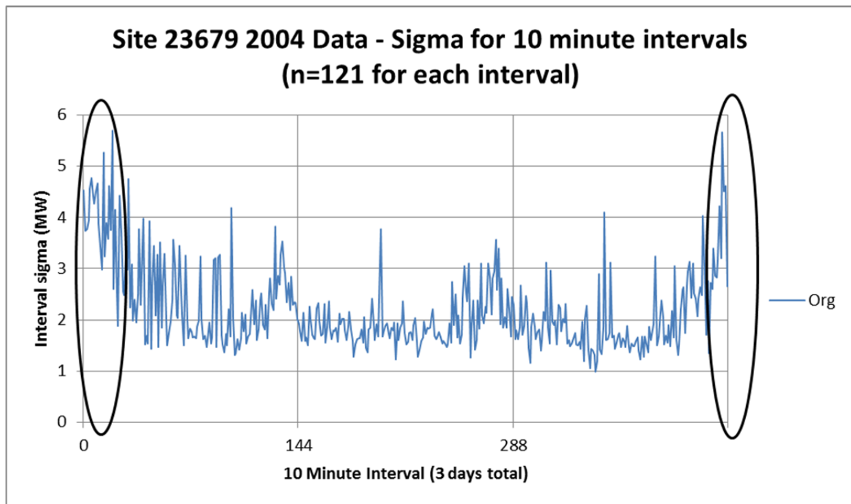
Figure 114. Standard deviation of 10-minute wind deltas by 10-minute interval number
