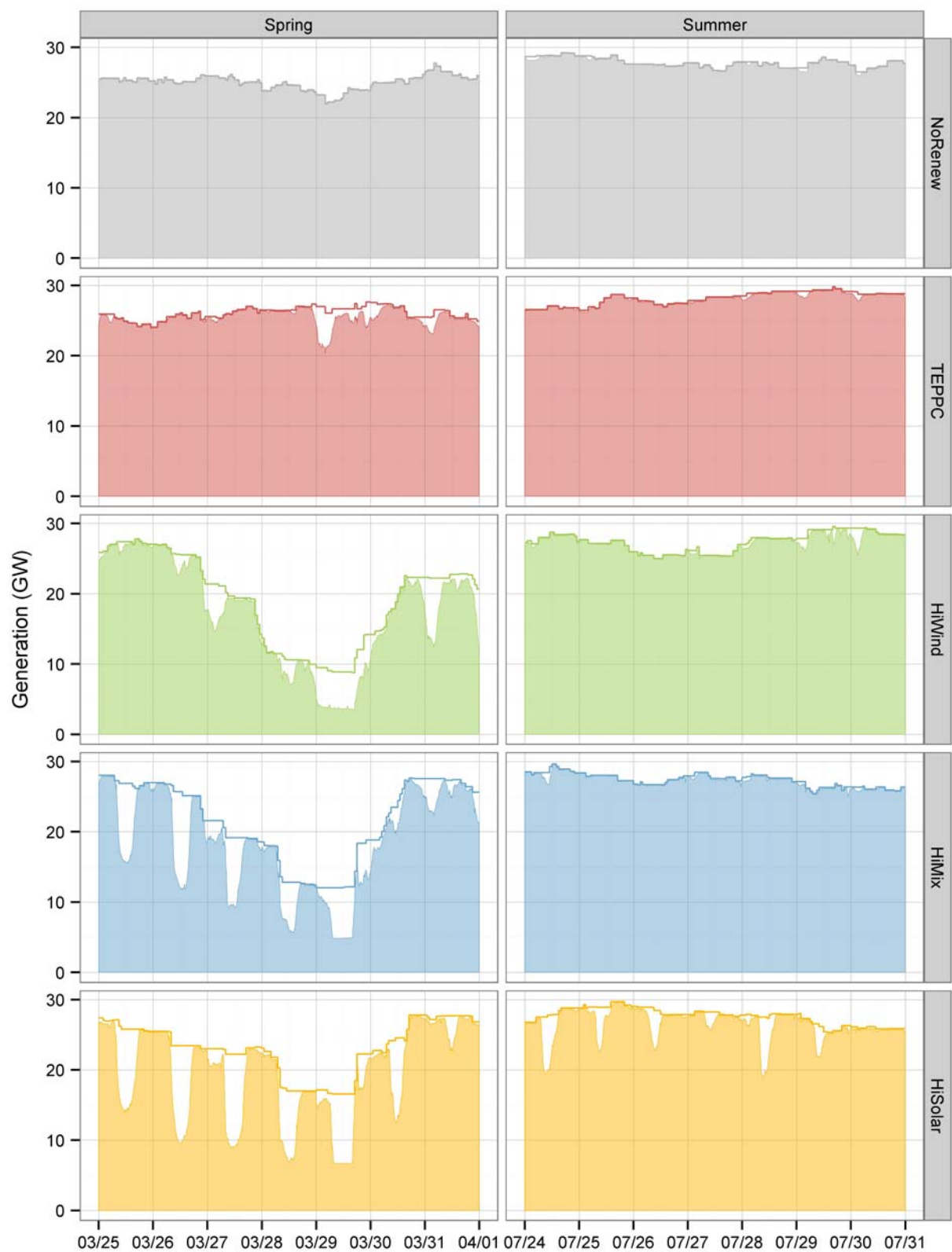
Figure 83. (Solid line) capacity committed and (shaded area) dispatched for coal units during March and July sample weeks for each scenario
