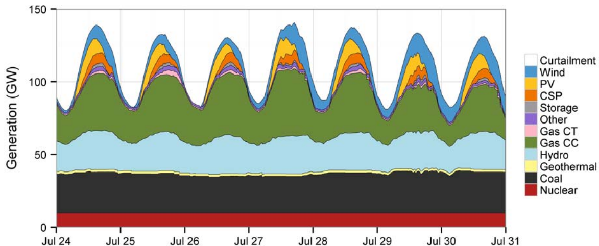
Figure 64. Summer dispatch stacks during the last week of July for the High Wind Scenario
