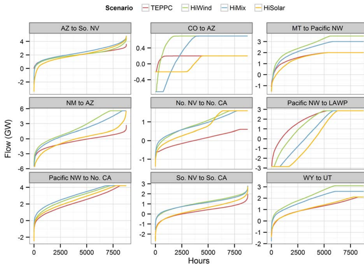
Figure 105. Flow duration curves across selected interfaces for each scenario
