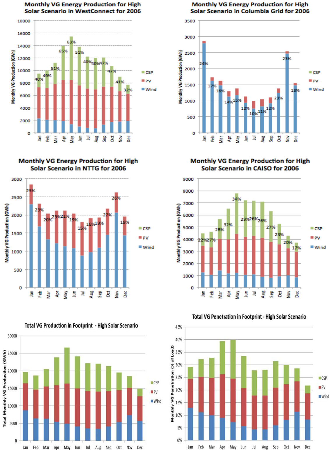
Figure 136. High Solar Scenario—monthly profiles
