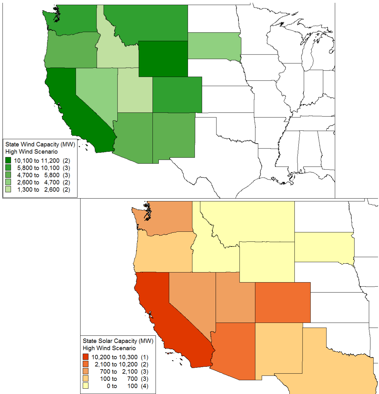
Figure 135. High Wind Scenario—installed capacity by state
