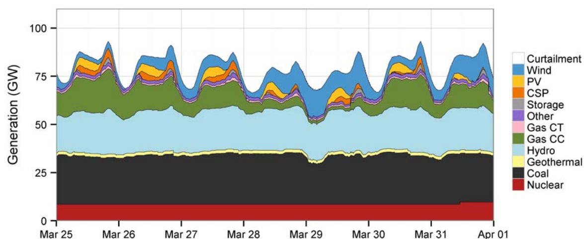
Figure 68. Spring dispatch stacks during the last week of March for the TEPPC Scenario
