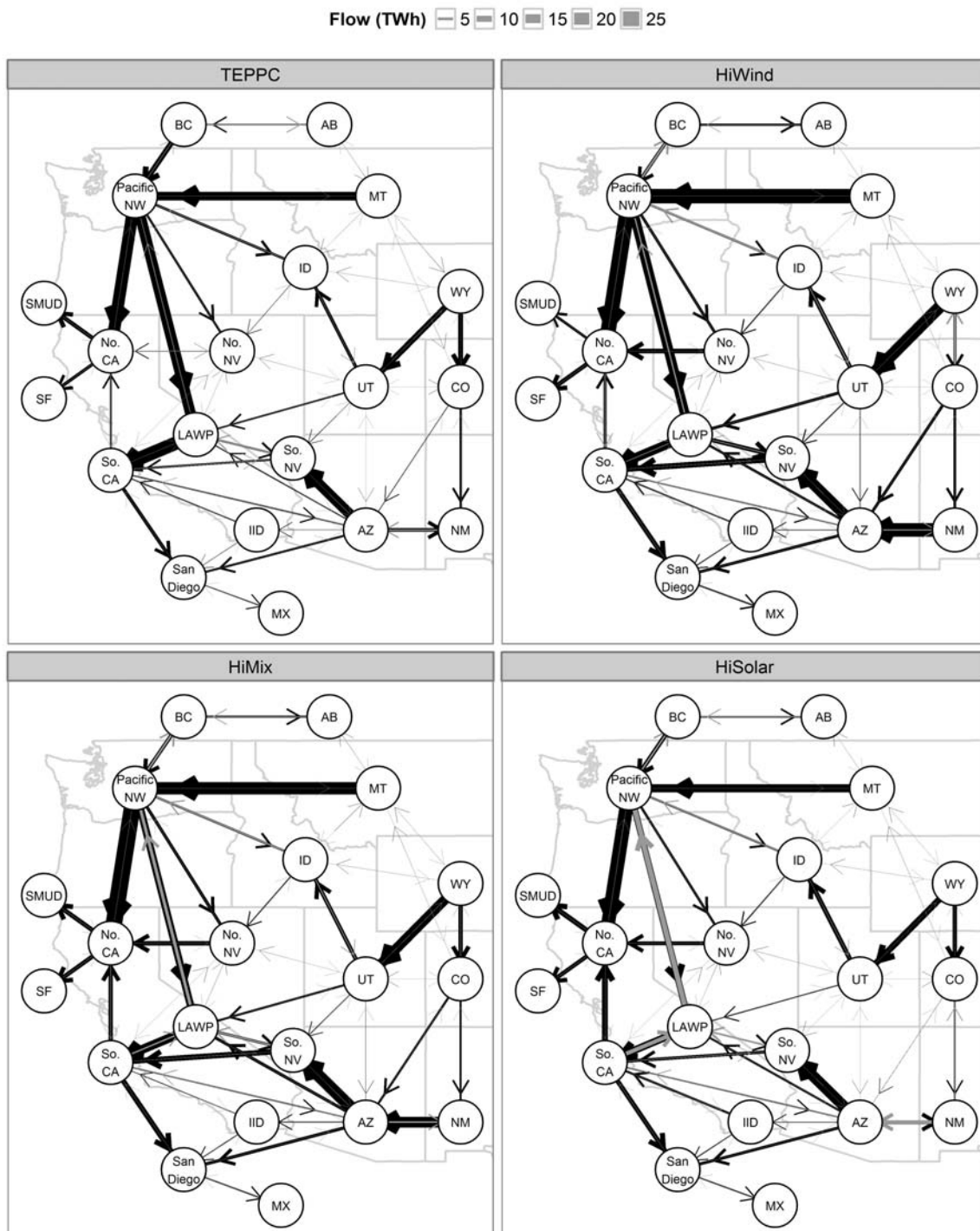
Figure 104. Interface flow map with prices for all scenarios
