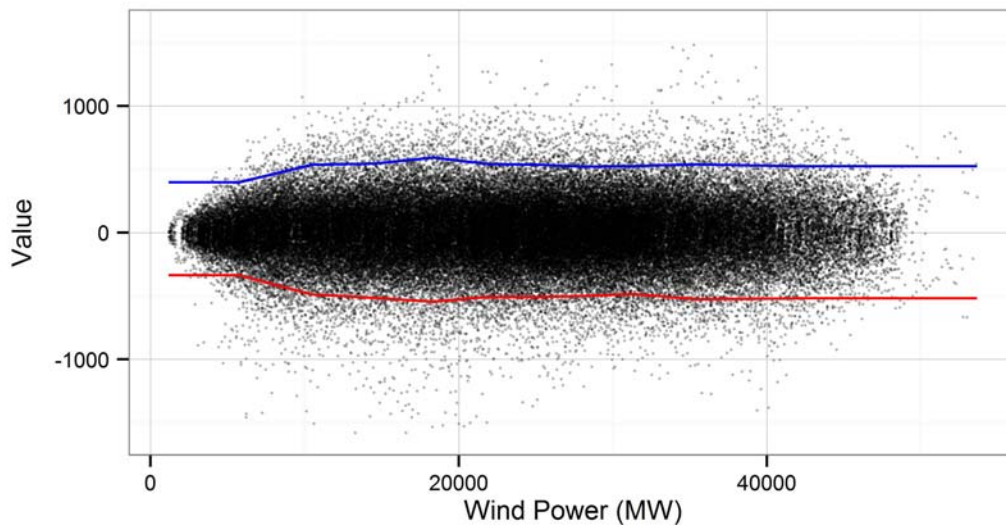
Figure 52. Wind 10-minute forecast errors versus power output, with 95% confidence interval bands for the High Solar Scenario
