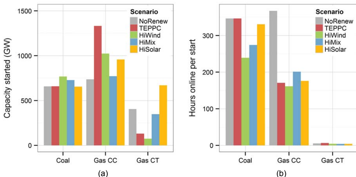
Figure 79. (a) Capacity started and (b) number of hours online per start by plant type for each scenario
