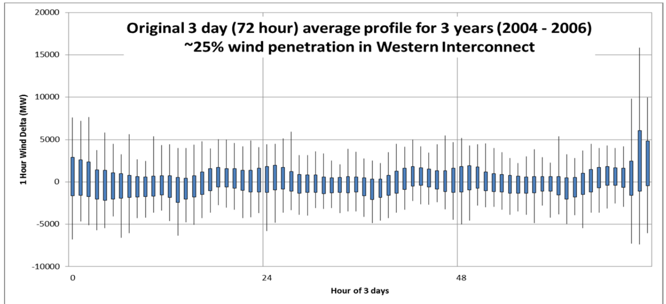
Figure 121. Bar and whisker for hourly changes for original data
