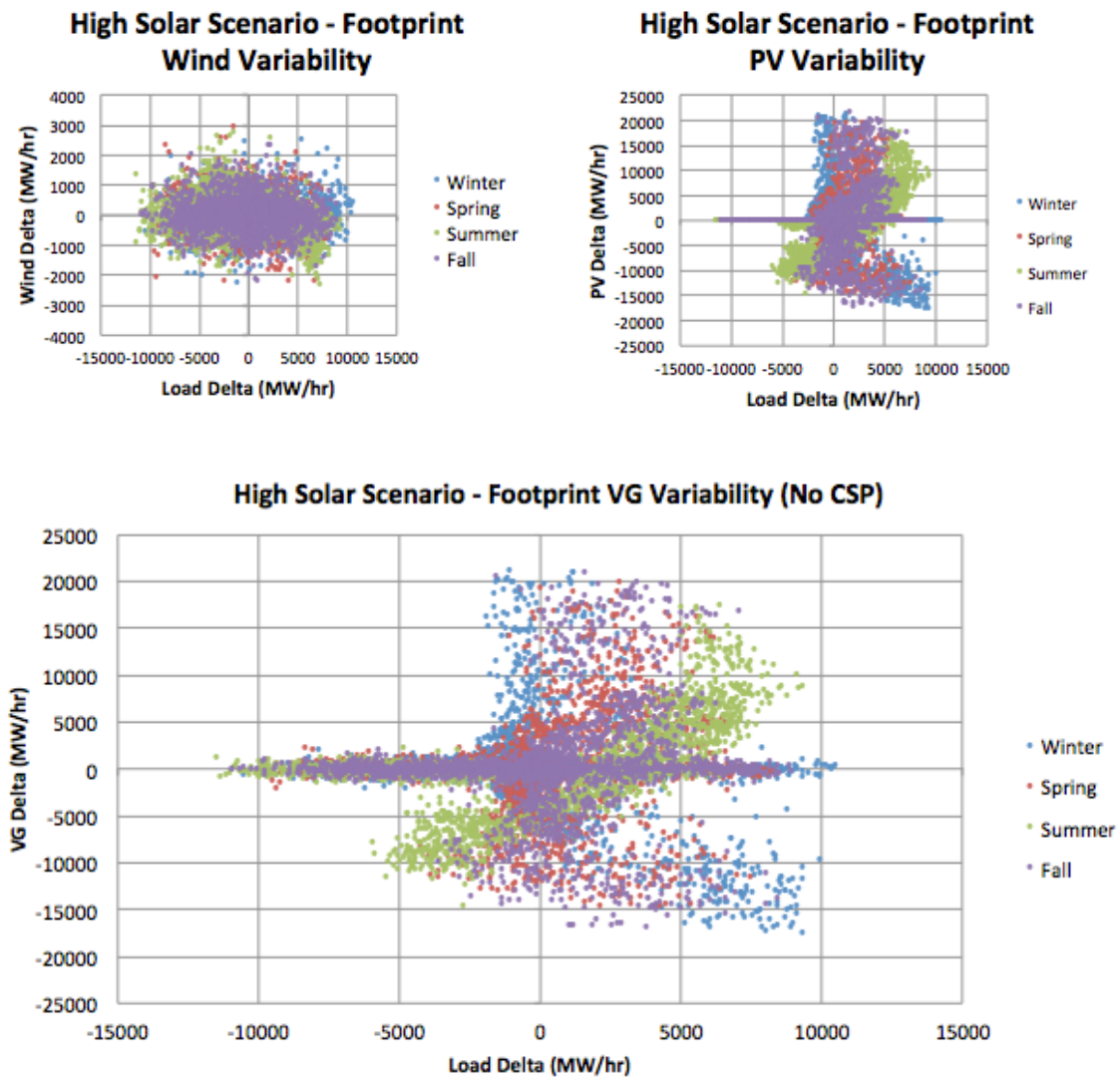
Figure 144. High Solar Scenario—hourly variability by season
