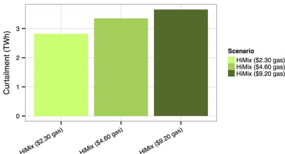
Figure 111. Curtailment in the gas price sensitivities
