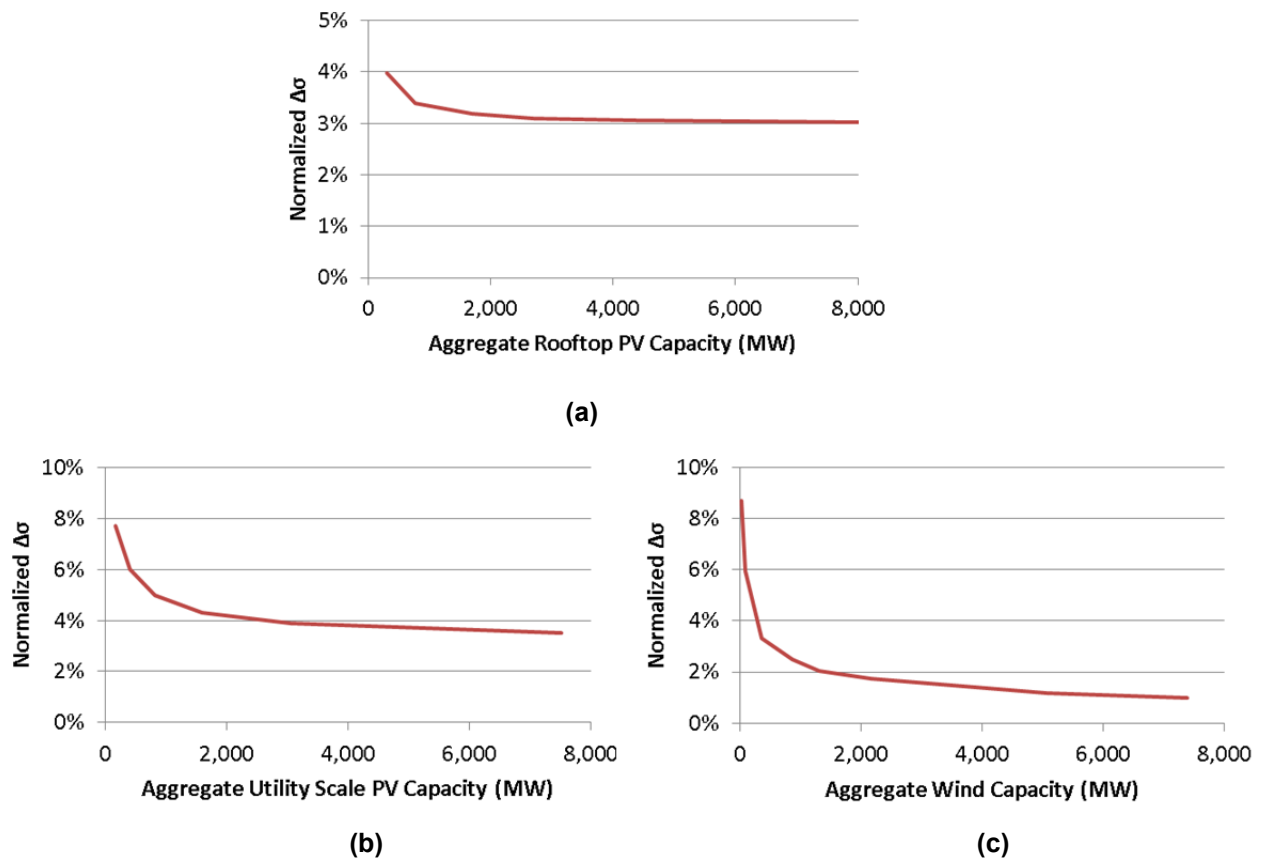
Figure 21. Normalized variability as a function of aggregate capacity for (a) rooftop PV, (b) utility-scale PV, and (c) wind
