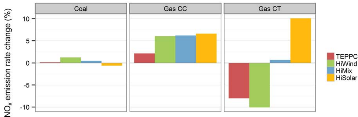
Figure 98. Change in NO x emission rates from the average coal, gas CC, and gas CT unit compared to the No Renewables Scenario
