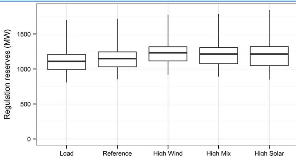
Figure 59. Distribution of regulation reserves by scenario
