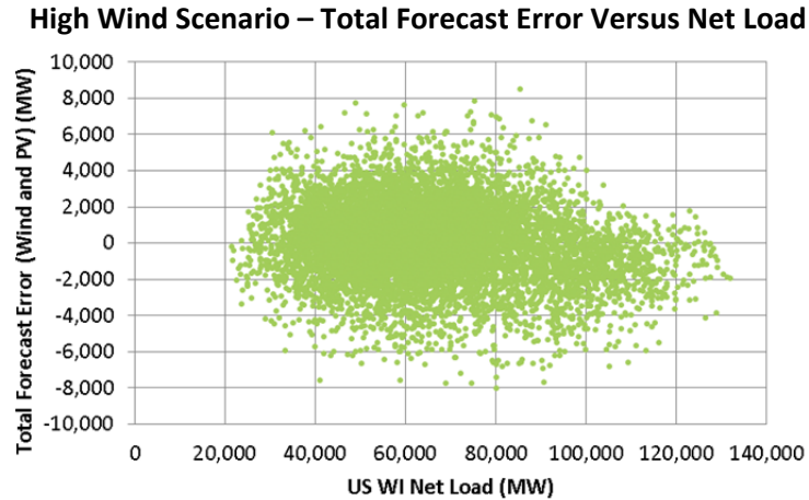
Figure 51. Four-hour-ahead forecast error scatter for the High Wind Scenario
