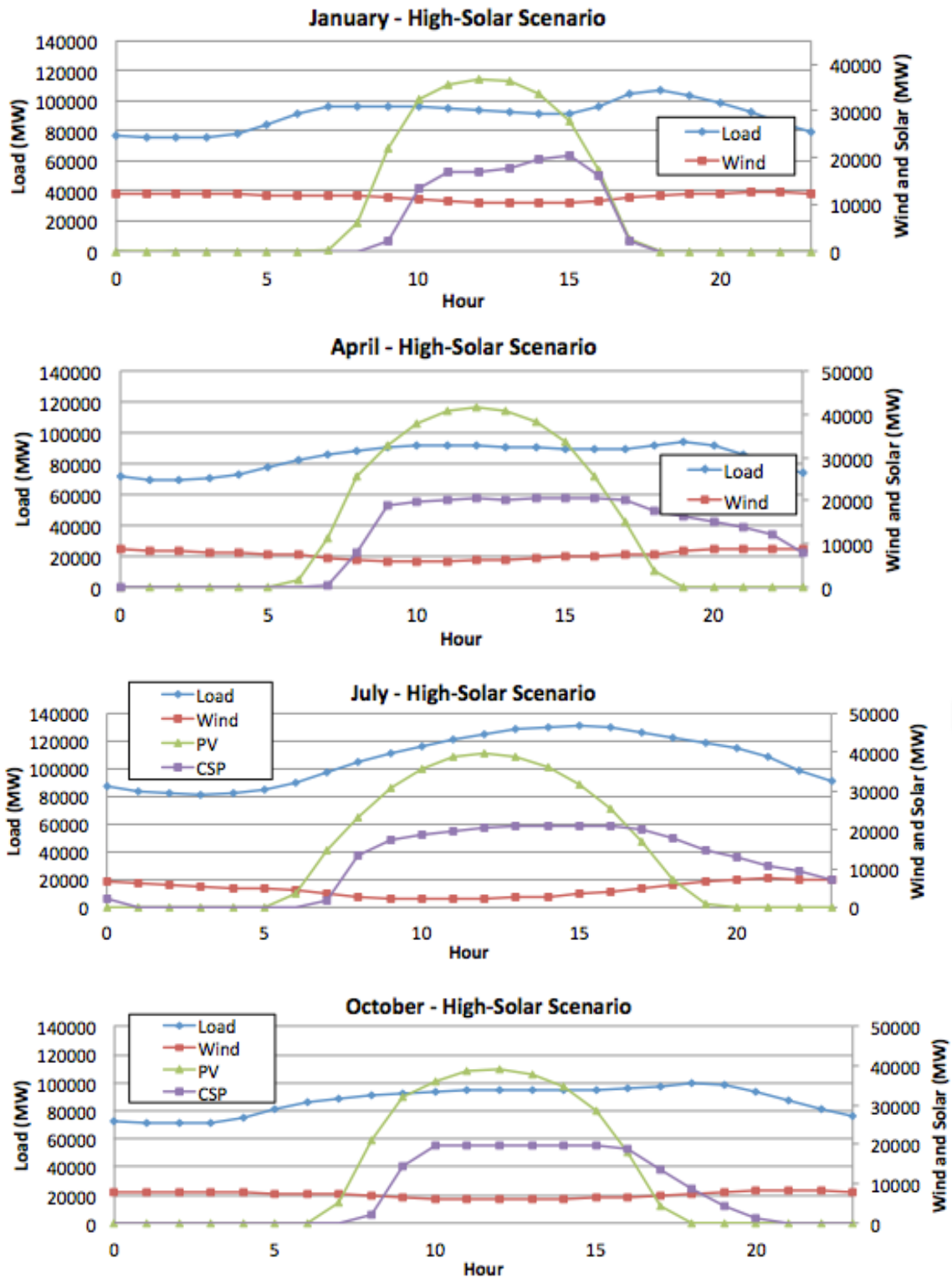
Figure 141. High Solar Scenario—average diurnal profile
