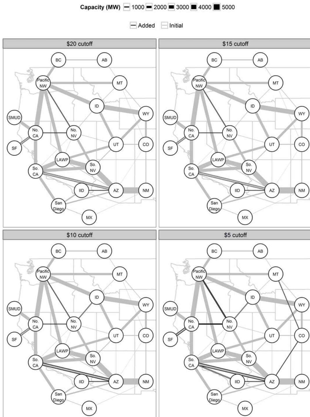
Figure 128. Transmission expansion for the TEPPC Scenario showing the (gray) initial and (black) additional transmission for each shadow price cutoff value tested
