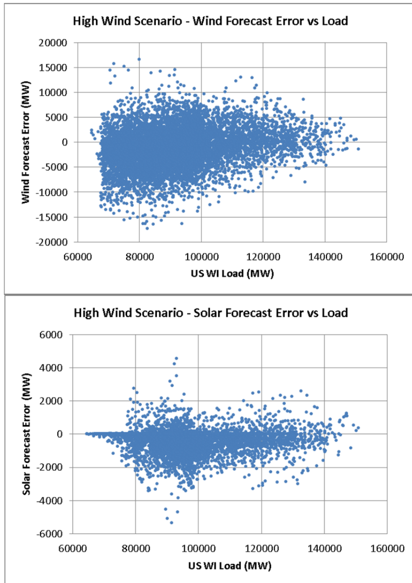
Figure 157. Wind and PV DA forecast error as a function of load level for the High Wind Scenario
