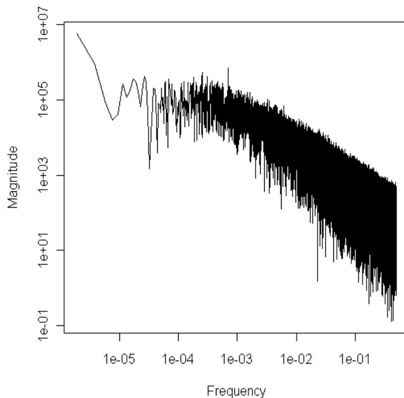
Figure 127. Power spectrum from spliced Cedar Creek turbine data for 1 full year
