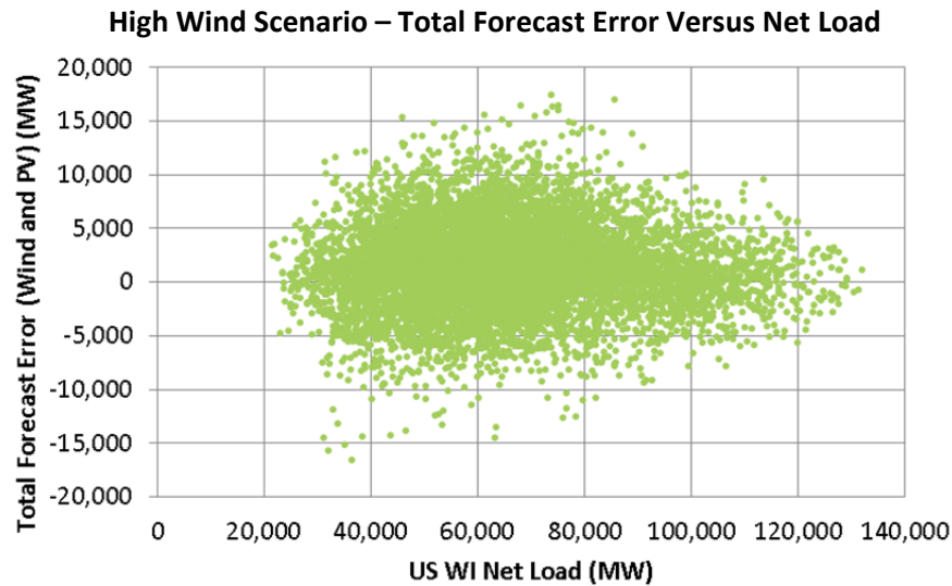
Figure 43. Total forecast error versus net load for the (a) High Solar and (b) High Wind Scenarios
