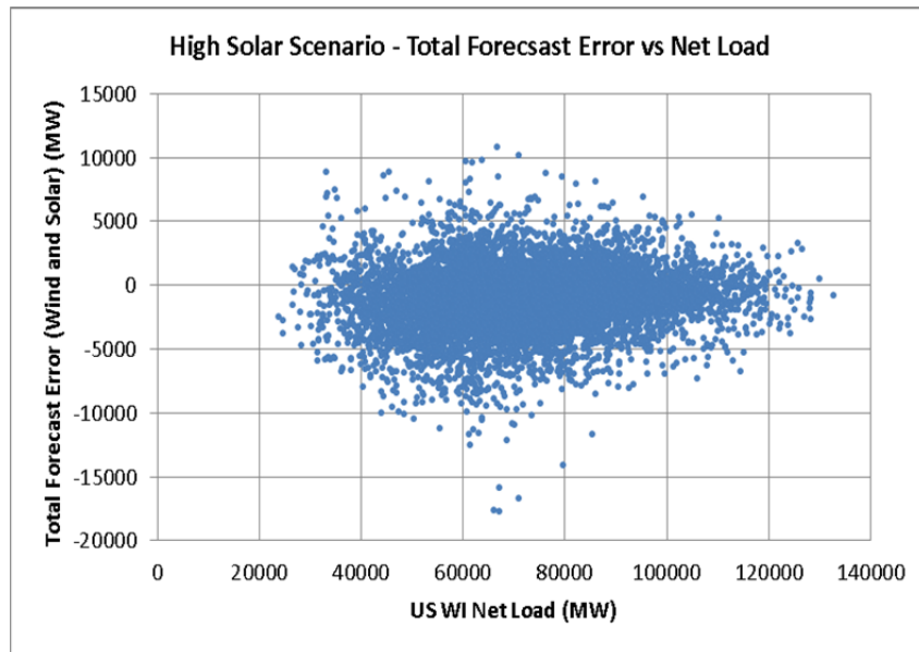
Figure 156. Wind plus PV DA forecast error as a function of net load for the High Solar Scenario
