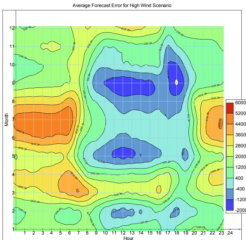
Figure 45. Contour plot of DA VG forecast errors for the High Wind Scenario
