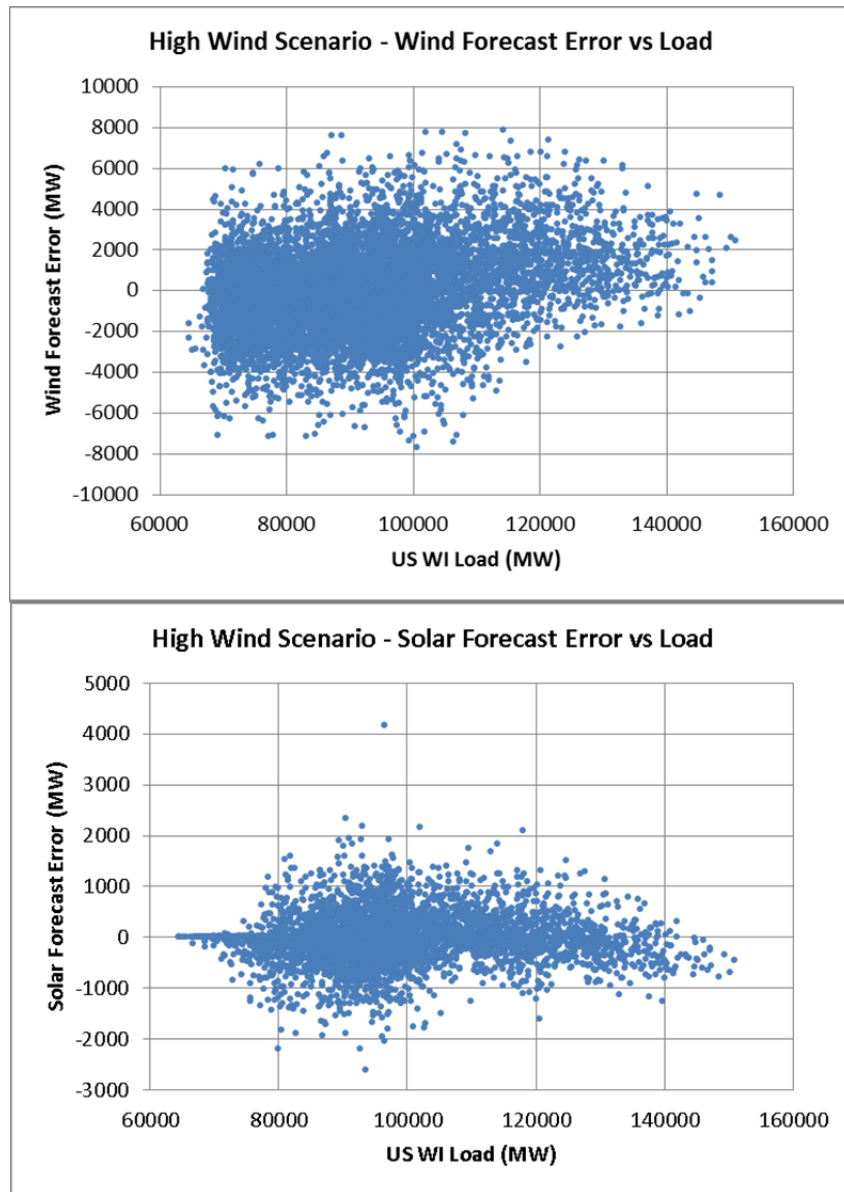
Figure 166. Wind and PV 4HA forecast error as a function of load level for the High Wind Scenario
