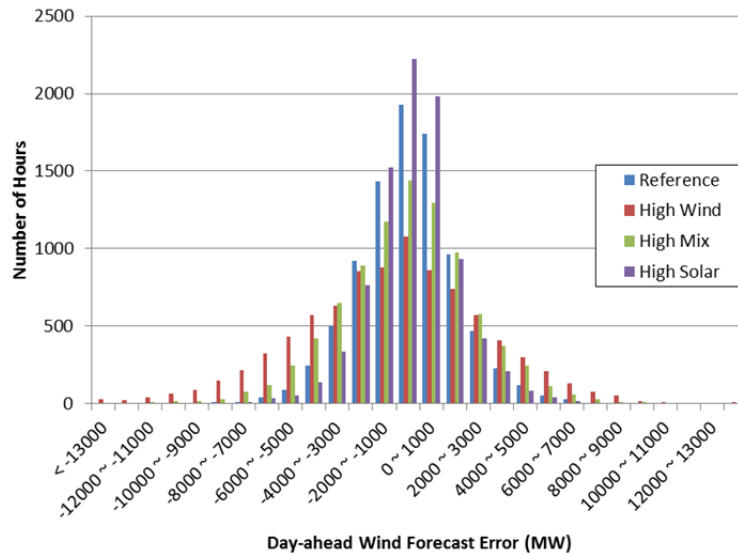
Figure 151. Distribution of DA wind forecast errors
