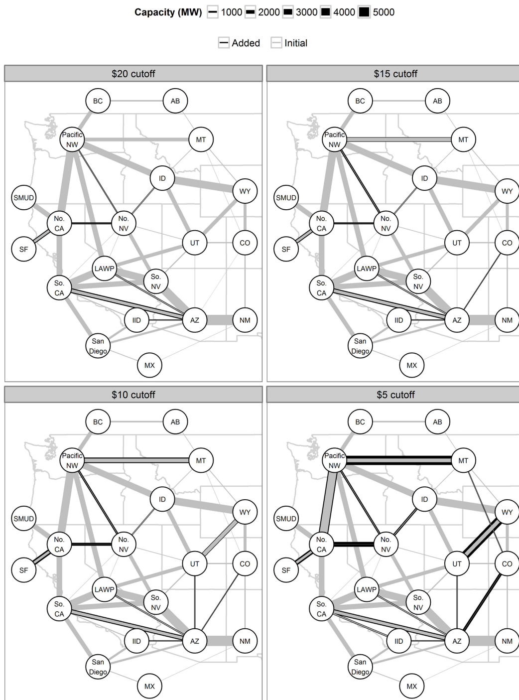
Figure 14. Iterative transmission build-out for the High Wind Scenario showing the different cutoff shadow prices
