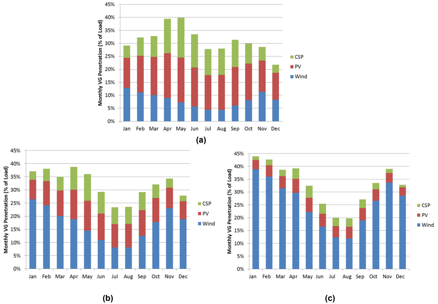
Figure 22. Monthly penetration of wind, PV, and CSP for the (a) High Solar, (b) High Mix, and (c) High Wind Scenarios
