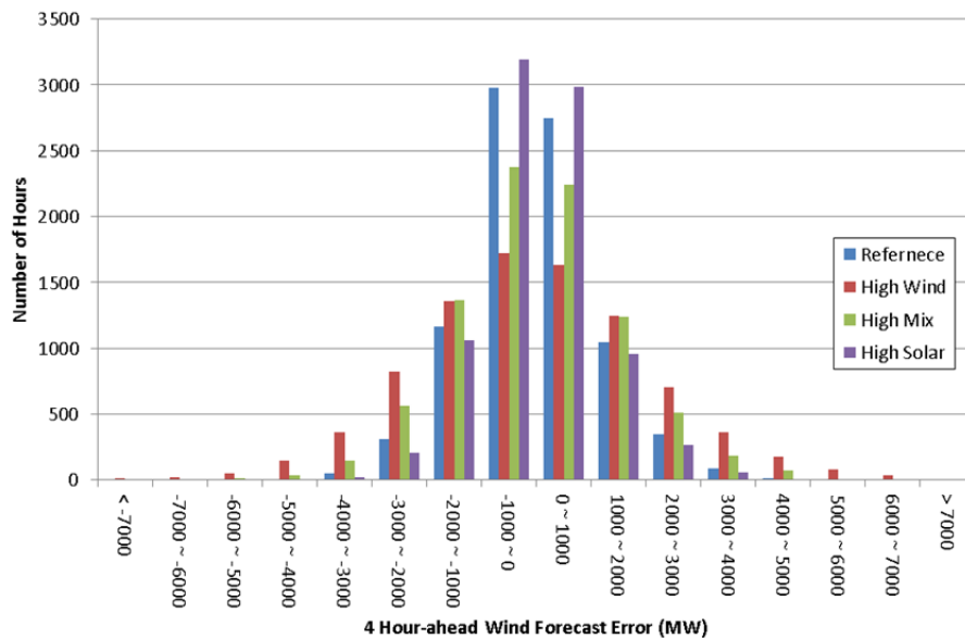
Figure 160. Distribution of 4HA wind forecast errors
