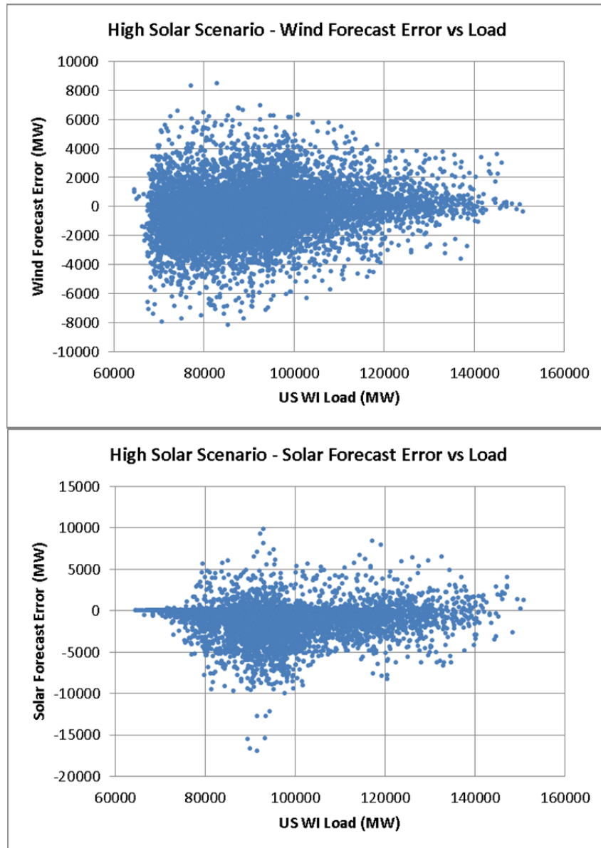
Figure 154. Wind and PV DA forecast error as a function of load level for the High Solar Scenario
