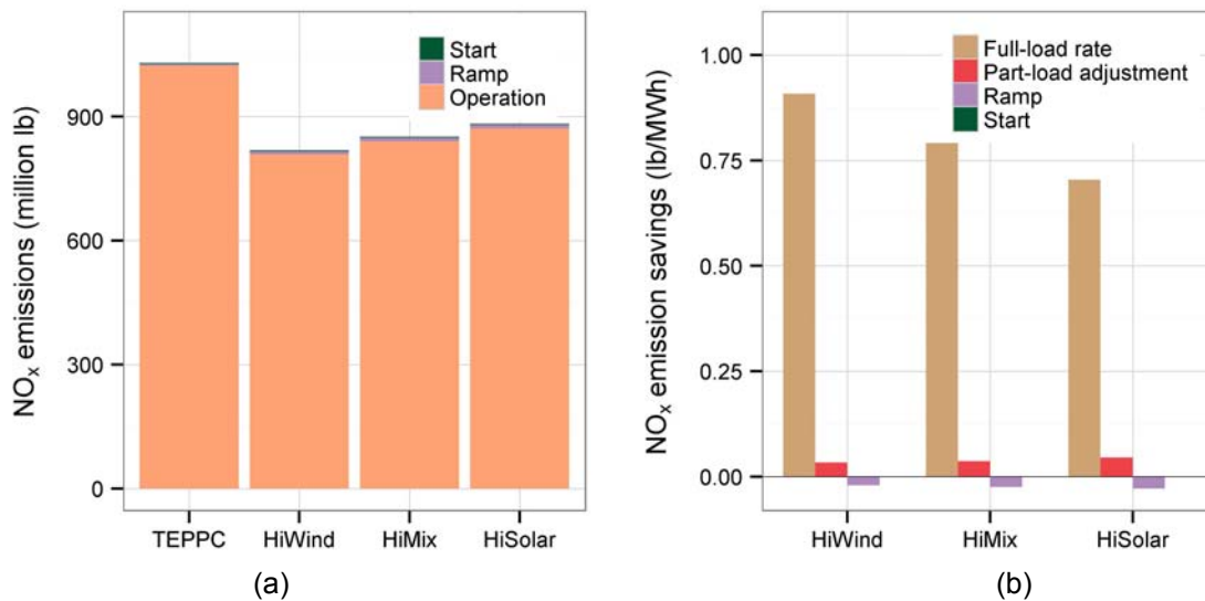
Figure 93. NO x emissions by scenario: (a) absolute NO x emissions for operation, ramping, and starts and (b) NO x emission reductions compared per MWh of wind and solar generation to the No Renewables Scenario, separated into the constant emissions rate assumption and adjustments for part-load impacts, ramping, and starts
