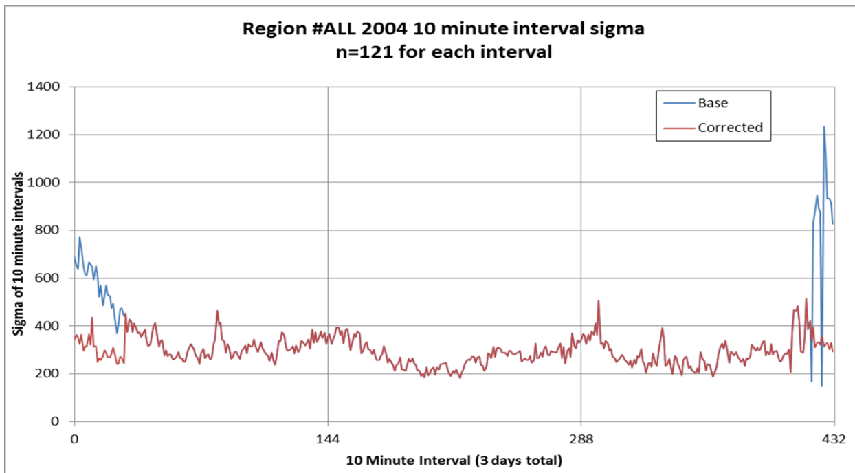
Figure 118. Standard deviation by 10-minute interval for all regions aggregated
