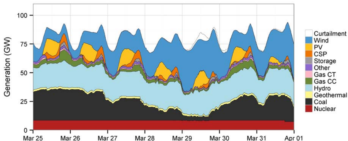
Figure 69. Spring dispatch stacks during the last week of March for the High Wind Scenario
