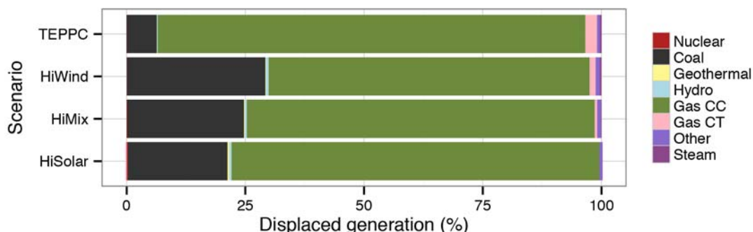
Figure 76. Generation displaced by wind and solar compared to No Renewables Scenario
