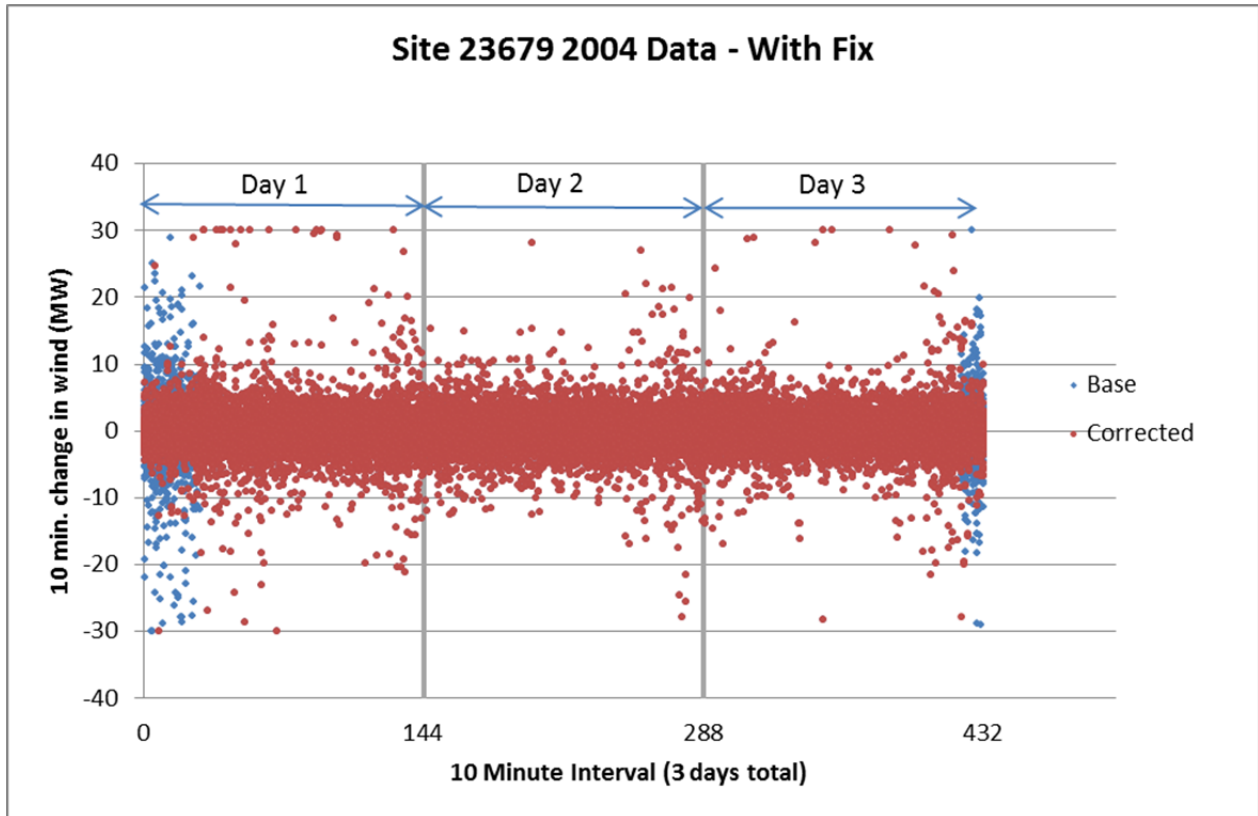
Figure 115. Corrected site data
