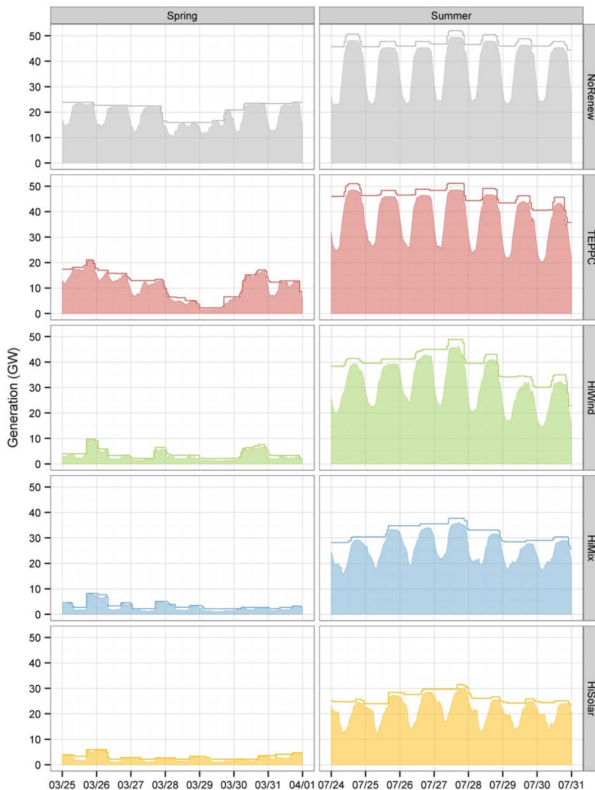
Figure 84. (Solid line) capacity committed and (shaded area) dispatched for gas CC units during March and July sample weeks for each scenario
