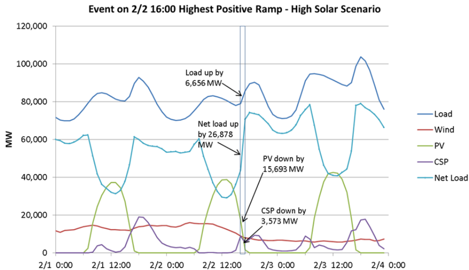
Figure 34. Highest hourly positive ramp (up-ramp) of 26,878 MW in the High Solar Scenario occurs on February 2 at 16:00
