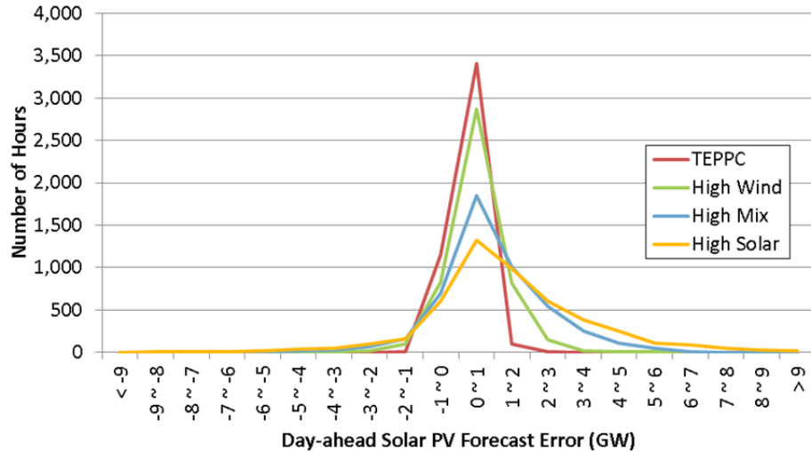
Figure 41. DA PV forecast error distribution for the U.S. Western Interconnection
