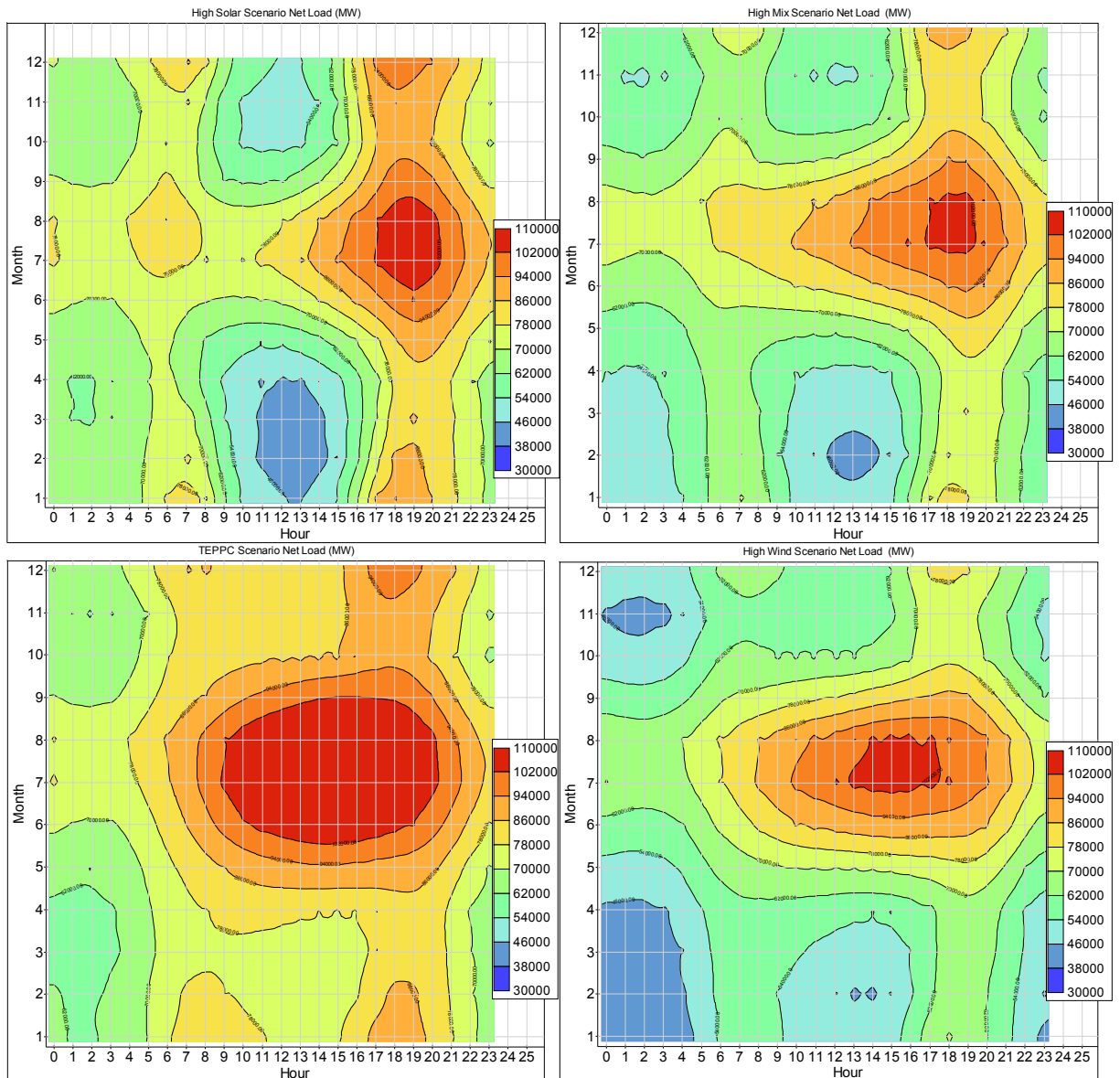
Figure 19. Contour plots of monthly average net load for each hour of the day for each scenario (clockwise from upper left): High Solar, High Mix, High Wind, and TEPPC
