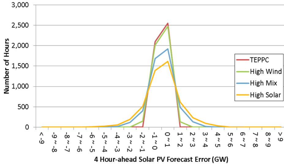
Figure 47. Four-hour-ahead PV forecast error distribution
