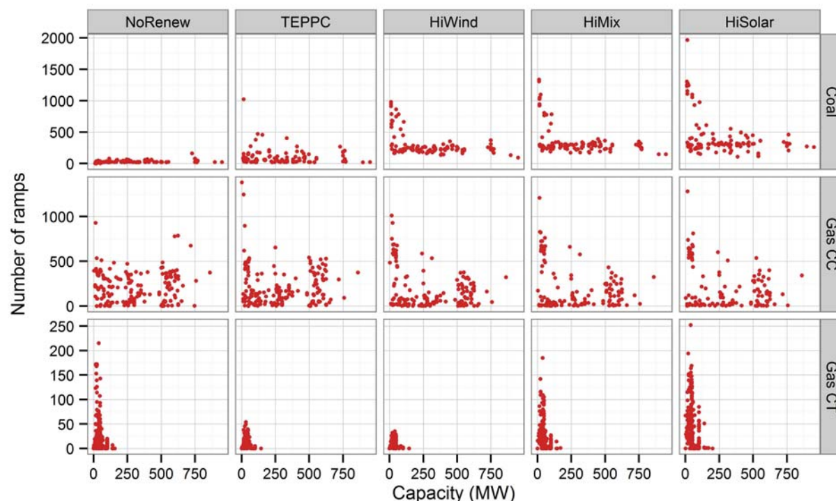
Figure 82. Number of ramps versus capacity for every unit by type and scenario
