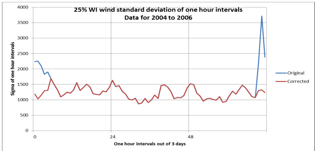
Figure 120. Sigma for 1-hour wind changes for 25% Western Interconnection scenario by hour number
