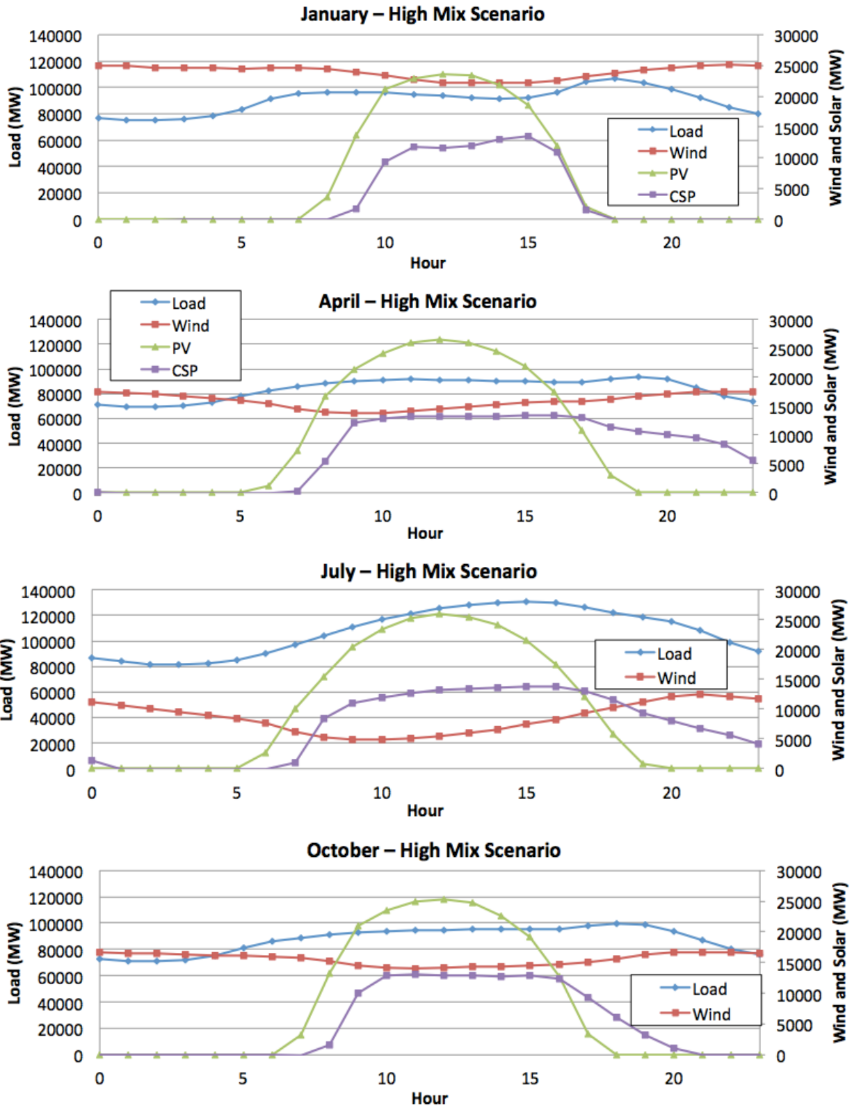
Figure 142. High Mix Scenario—average diurnal profile
