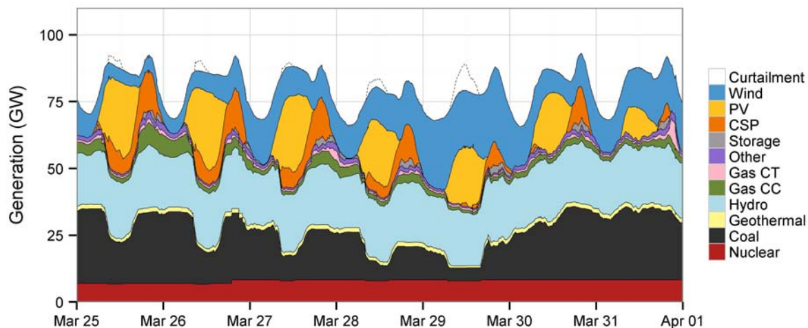
Figure 70. Spring dispatch stacks during the last week of March for the High Mix Scenario
