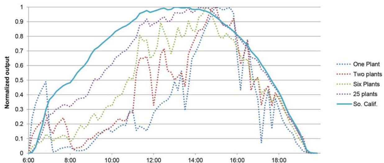
Figure 20. Normalized PV output for increasing aggregation of PV plants in Southern California for a partly cloudy day
