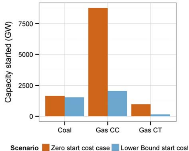
Figure 86. Starts by type for the High Wind Scenario with zero wear-and-tear start costs compared to lower-bound wear-and-tear start costs
