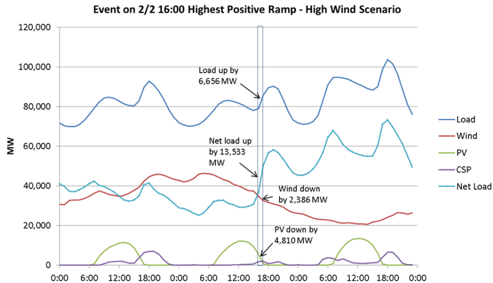
Figure 36. The highest hourly up-ramp of 13,533 MW in the High Wind Scenario occurred on February 2 at 16:00
