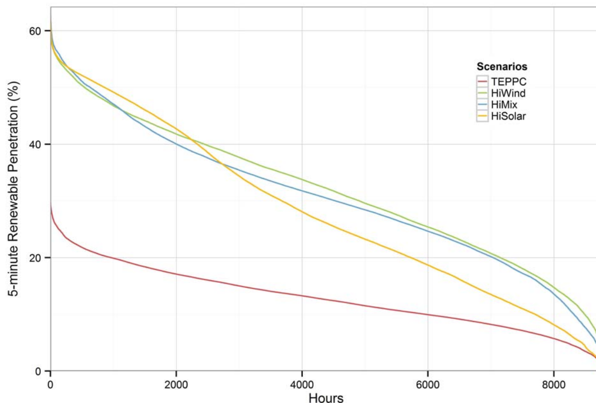
Figure 78. Duration curve of 5-minute wind/solar penetration for each scenario
