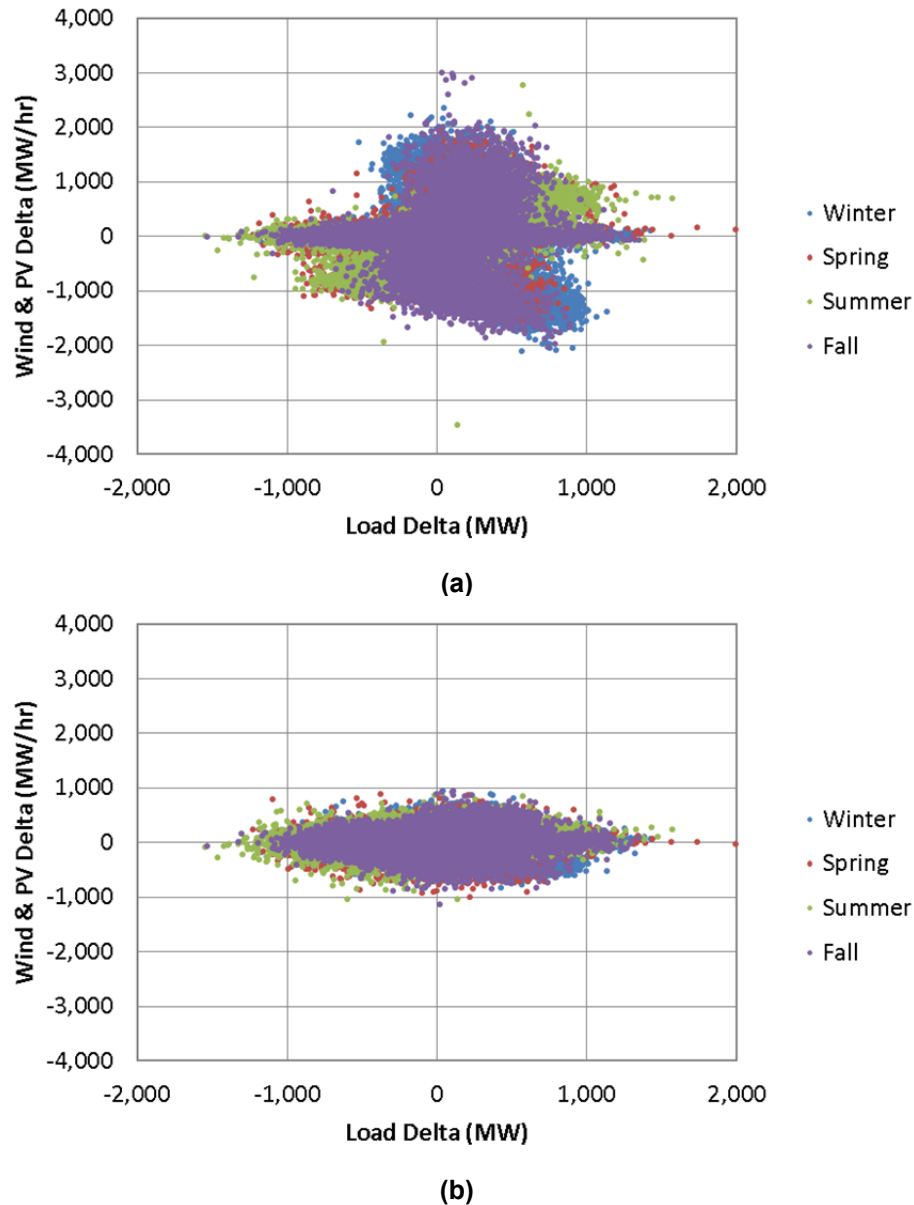
Figure 28. Five-minute changes in load versus 5-minute changes in wind and PV output for the (a) High Solar and (b) High Wind Scenarios
