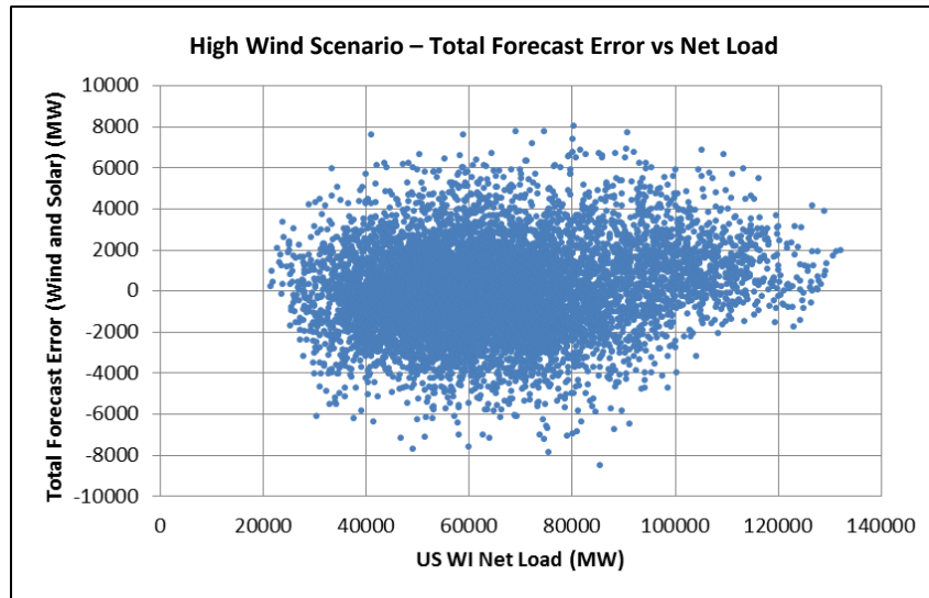
Figure 168. Wind plus PV 4HA forecast error as a function of net load level for the High Wind Scenario
