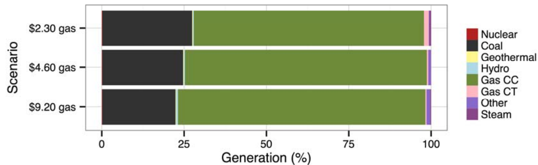
Figure 107. Generation displaced by renewables in the High Mix compared to No Renewables Scenarios for each gas price
