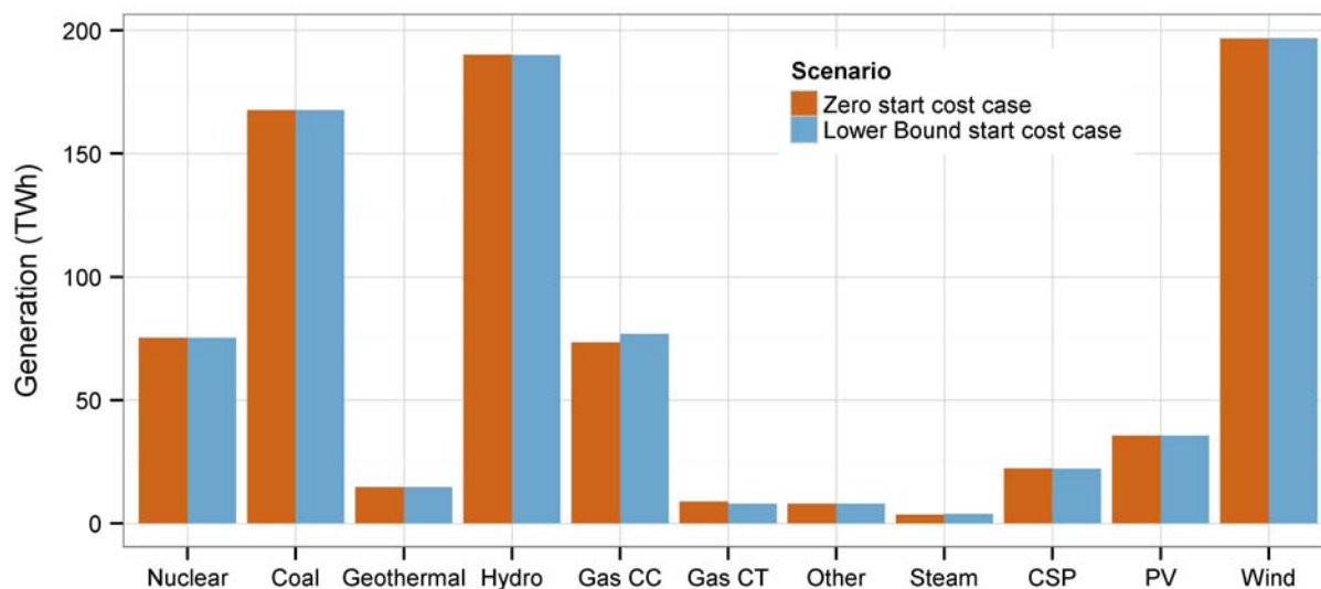
Figure 85. Generation by type for the High Wind Scenario with zero wear-and-tear start costs compared to lower-bound wear-and-tear start costs
