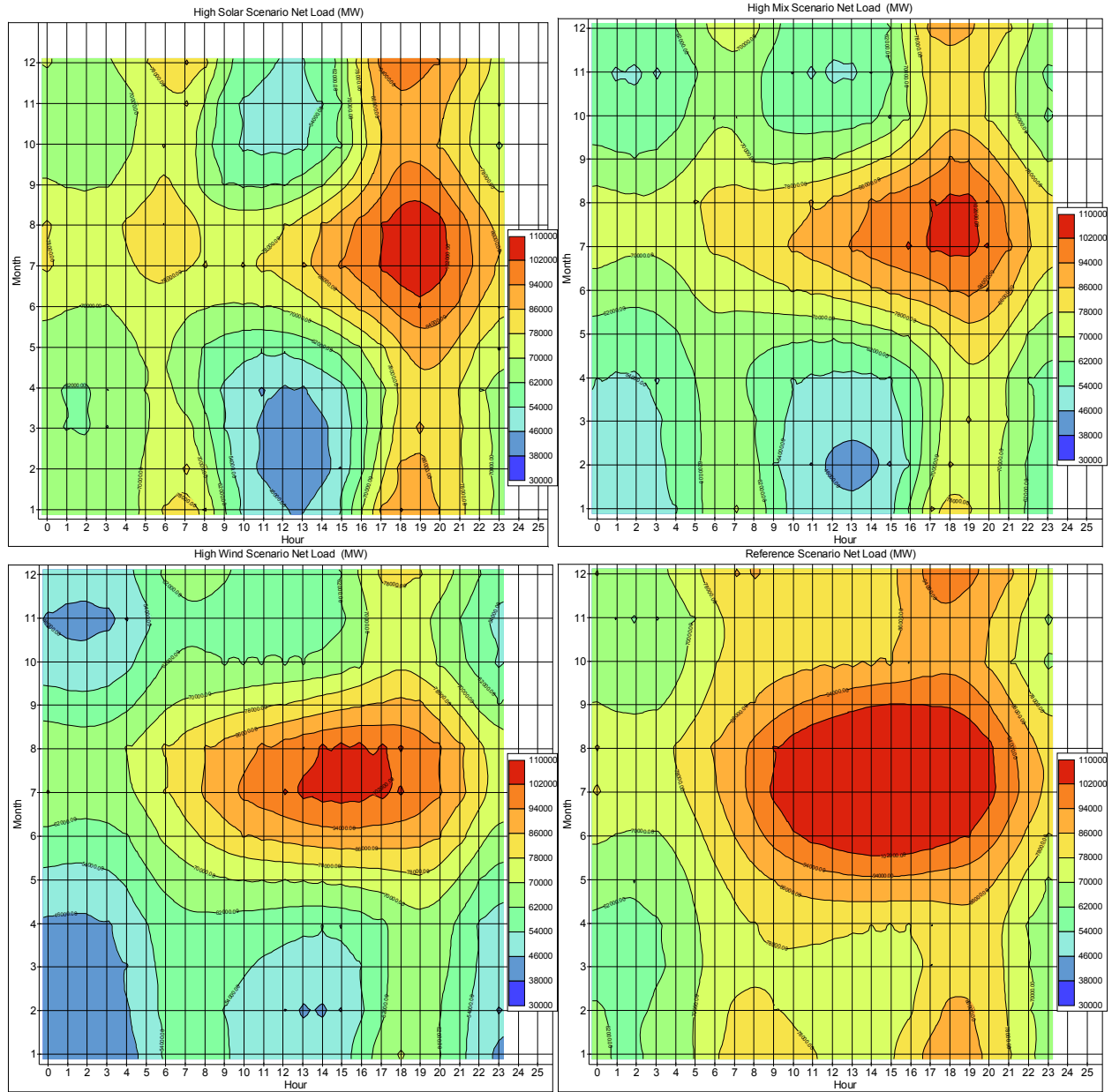
Figure 148. Net load with monthly average values in MW for each scenario
