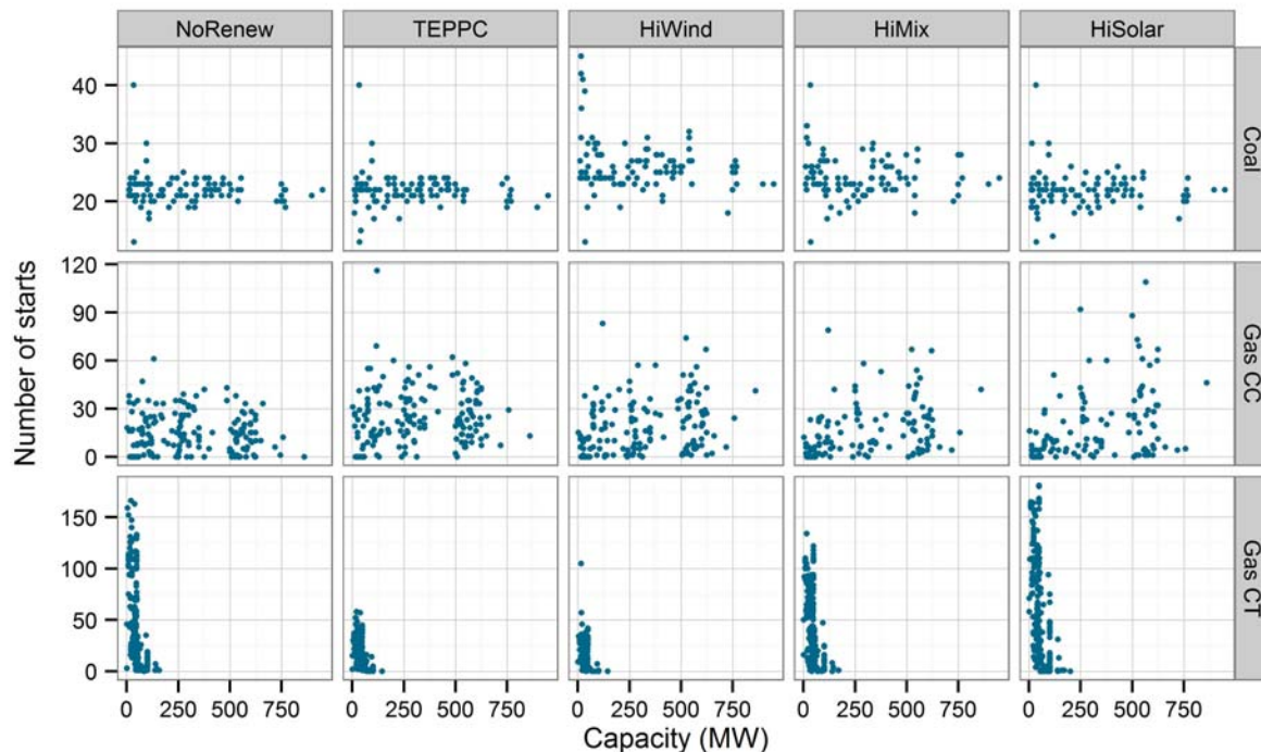
Figure 81. Number of starts versus capacity for every unit by unit type and scenario
