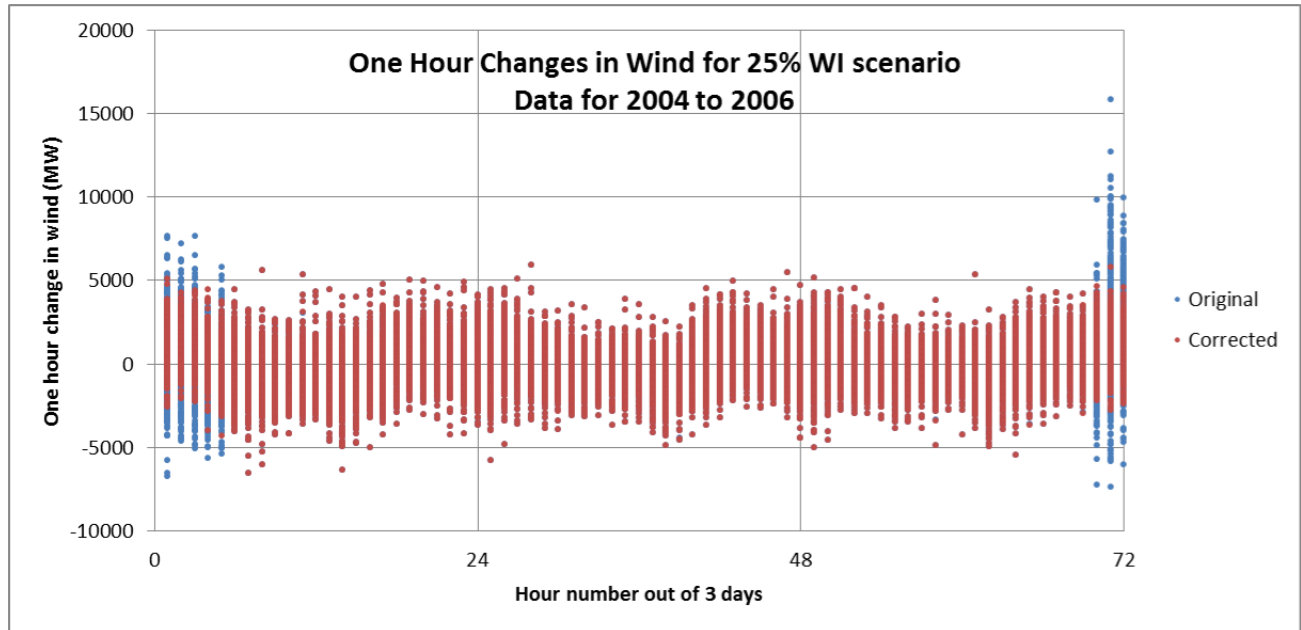
Figure 119. One-hour changes in wind for 25% Western Interconnection scenario by hour number
