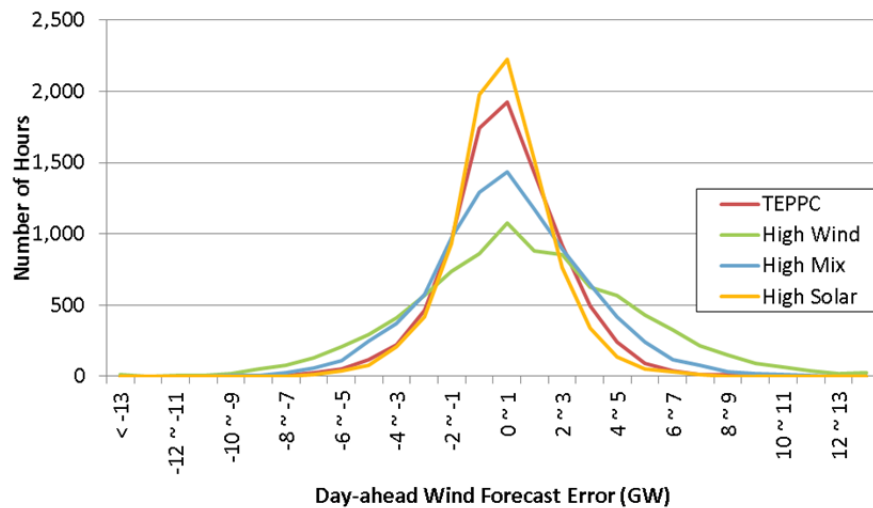
Figure 40. DA wind forecast error distribution for the U.S. Western Interconnection
