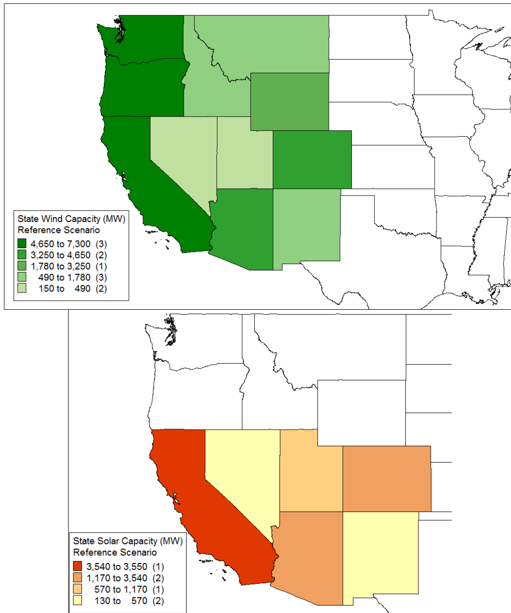
Figure 132. TEPPC Scenario—installed capacity by state
