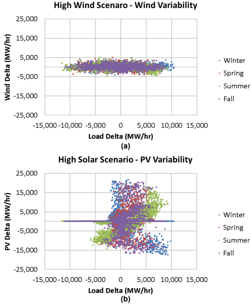
Figure 24. (a) Hourly wind production change versus hourly load change for the High Wind Scenario and (b) hourly PV production change versus hourly load change for the High Solar Scenario
