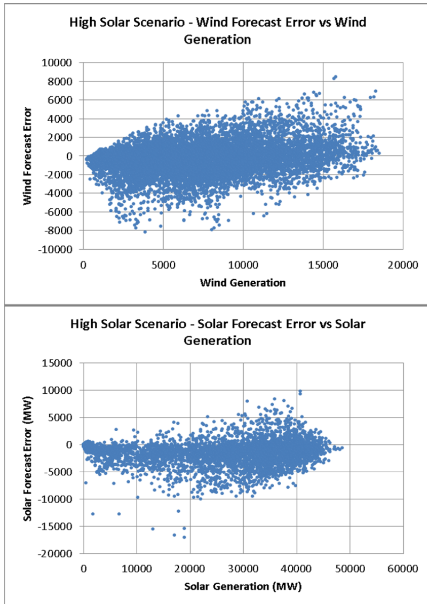
Figure 155. Wind and PV DA forecast error as a function of wind and PV output level for the High Solar Scenario
