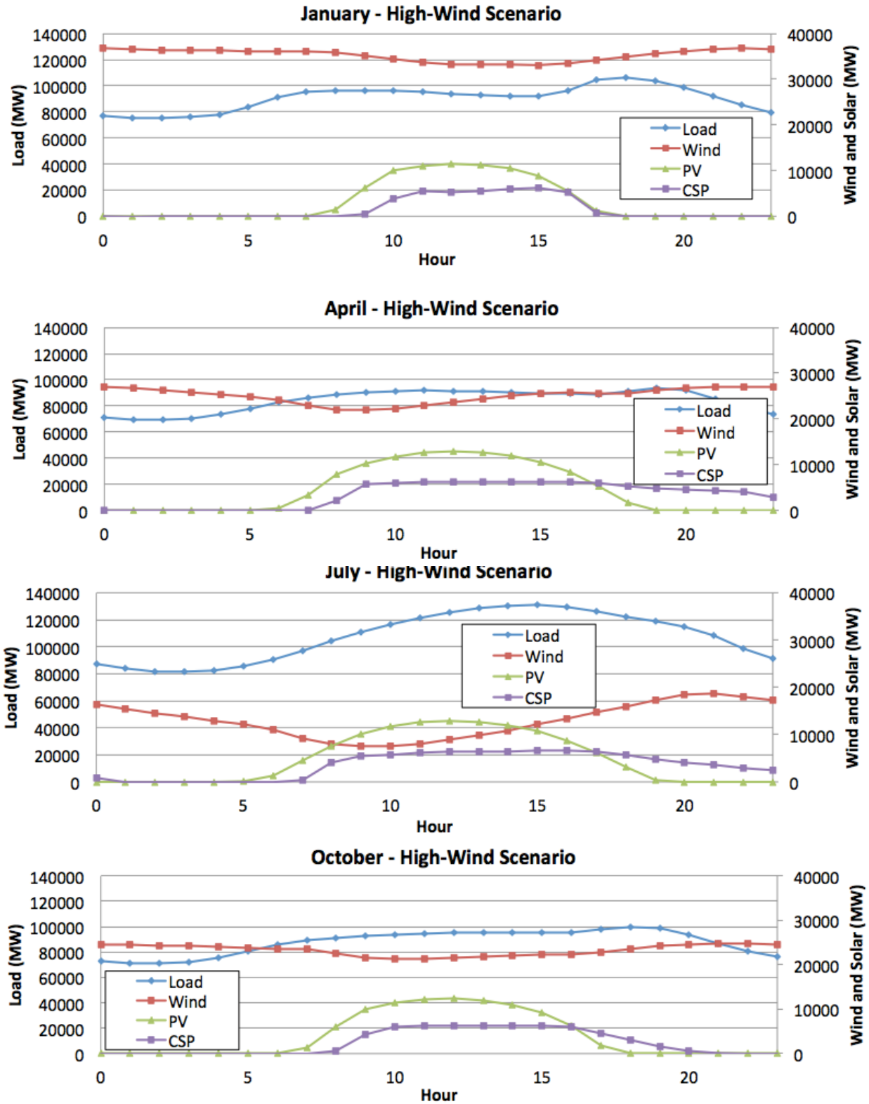
Figure 143. High Wind Scenario—average diurnal profile
