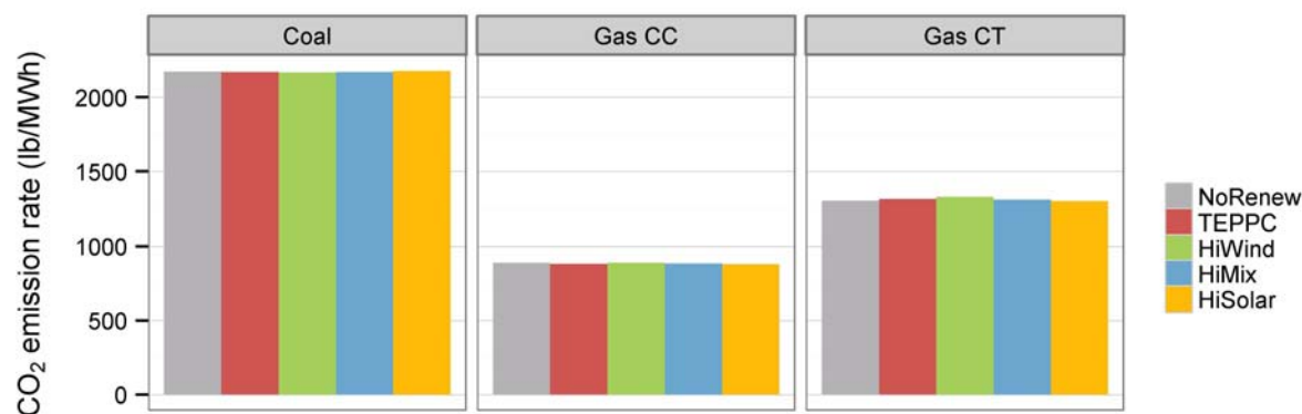
Figure 95. CO 2 emission rates from the average coal, gas CC, and gas CT unit
