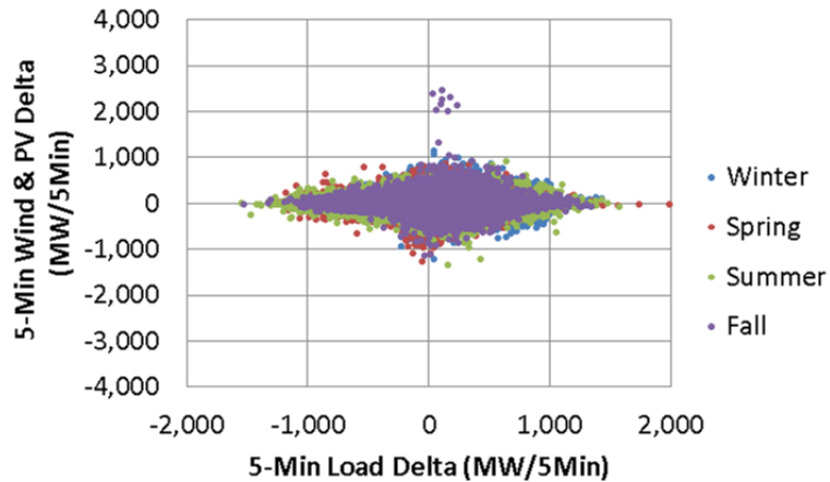
Figure 30. Five-minute total wind and PV variability excluding diurnal solar variability for the High Solar Scenario
