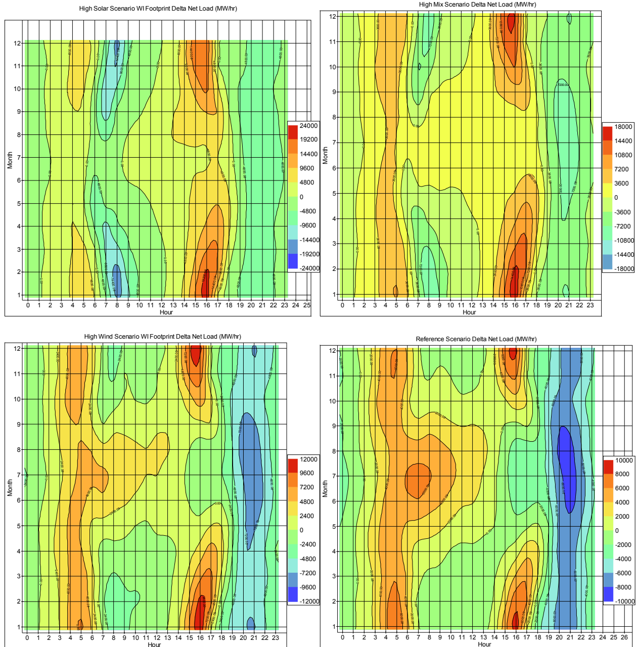
Figure 150. Delta net load with monthly average changes in MW/h for each scenario
