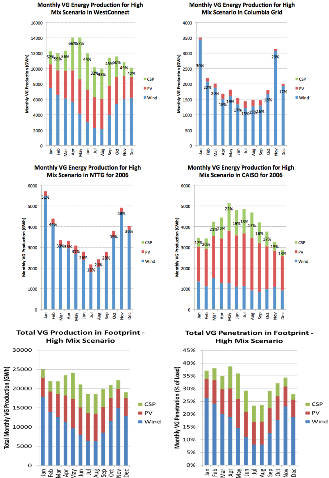
Figure 137. High Mix Scenario—monthly profiles
