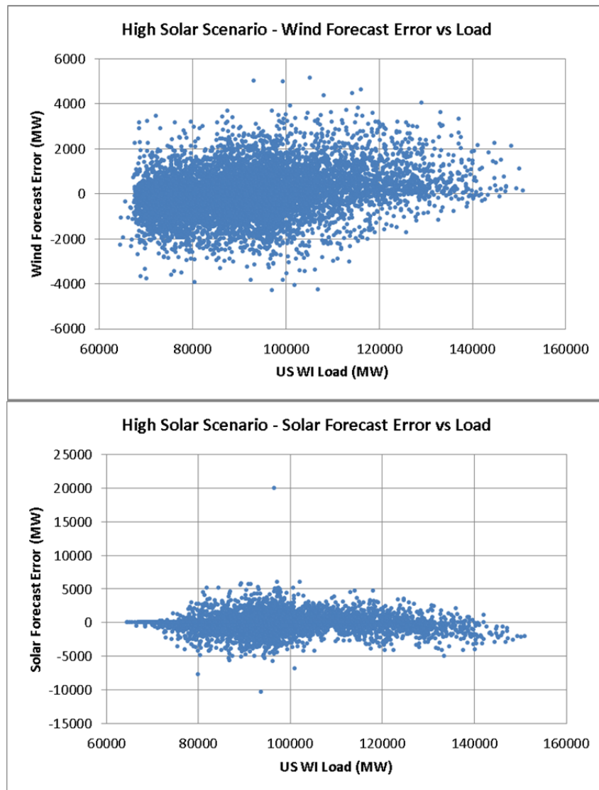
Figure 163. Wind and PV 4HA forecast errors as a function of load level for the High Solar Scenario
