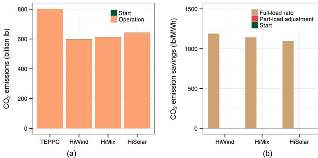
Figure 92. CO 2 emissions by scenario: (a) absolute CO 2 emissions for operation and starts and (b) CO 2 emission reductions per MWh of wind and solar generation compared to the No Renewables Scenario, separated into the constant emissions rate assumption and adjustments for part-load impacts and starts
