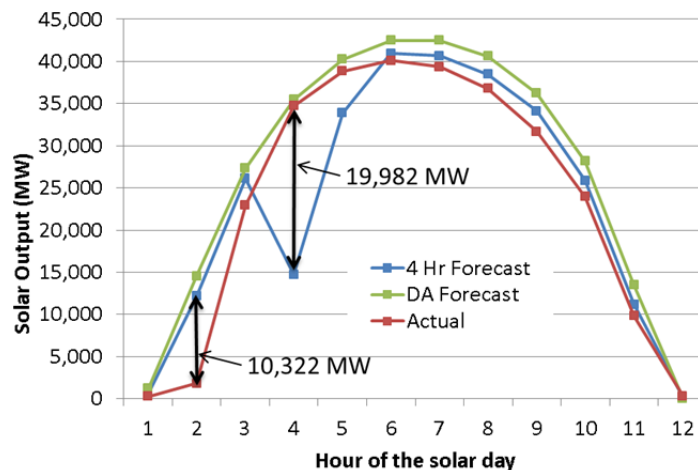
Figure 50. Detail of extreme 4HA solar forecast error caused by methodology used to generate 4HA forecasts
