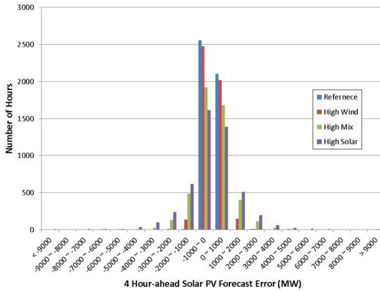
Figure 161. Distribution of 4HA solar forecast errors
