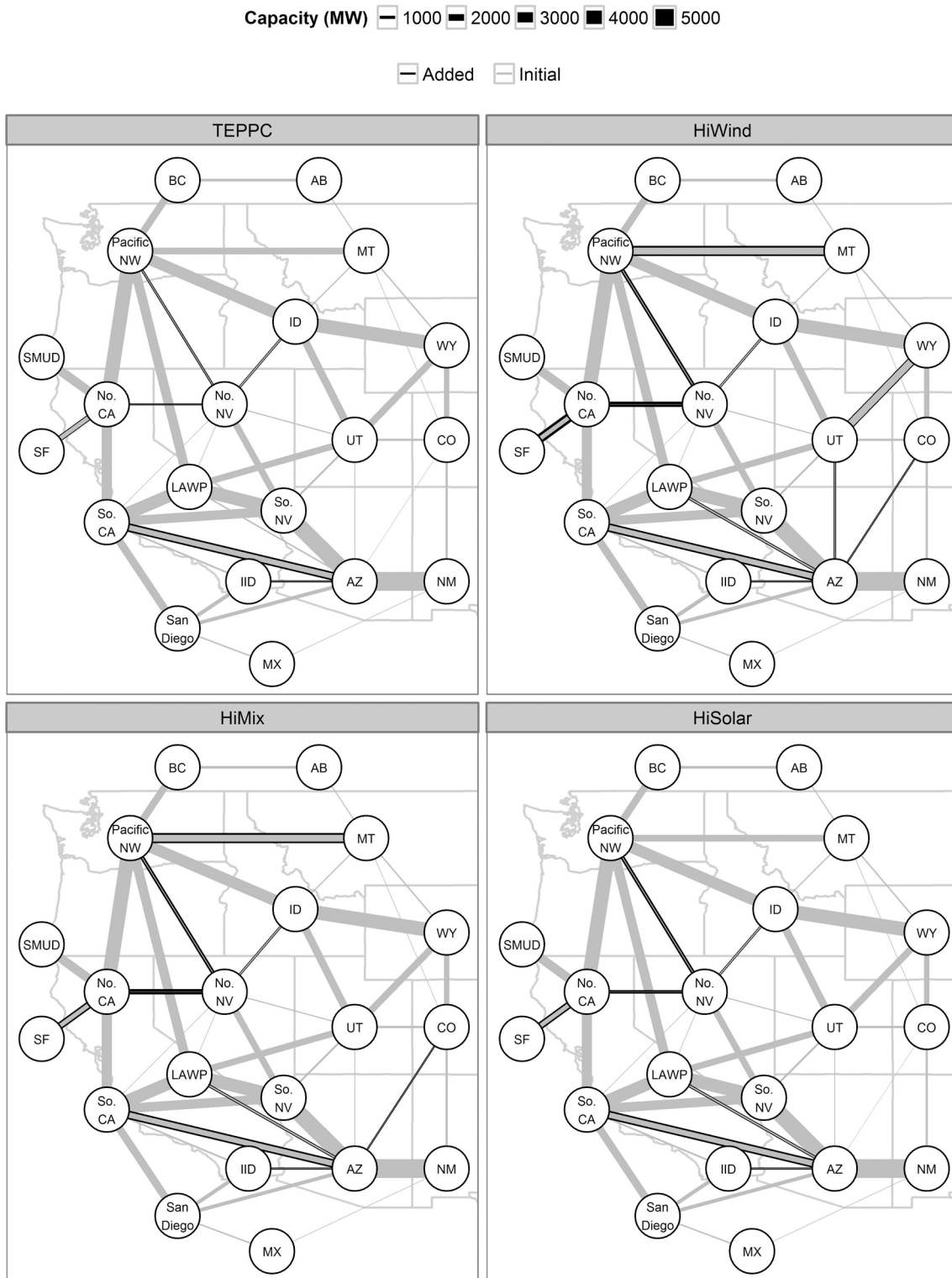
Figure 16. Final transmission build-out by scenario (using the $10 cutoff shadow price)
