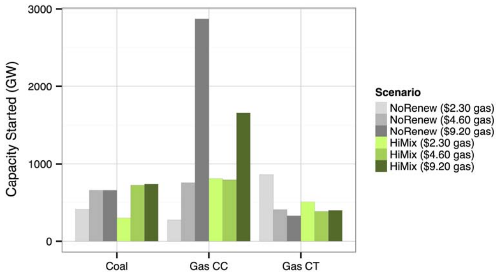
Figure 108. Capacity started in the gas price sensitivities
