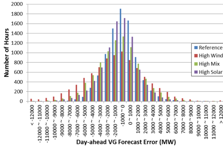
Figure 153. Distribution of DA wind plus PV forecast errors
