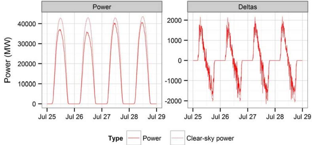
Figure 54. Power and clear-sky power output and ramps
