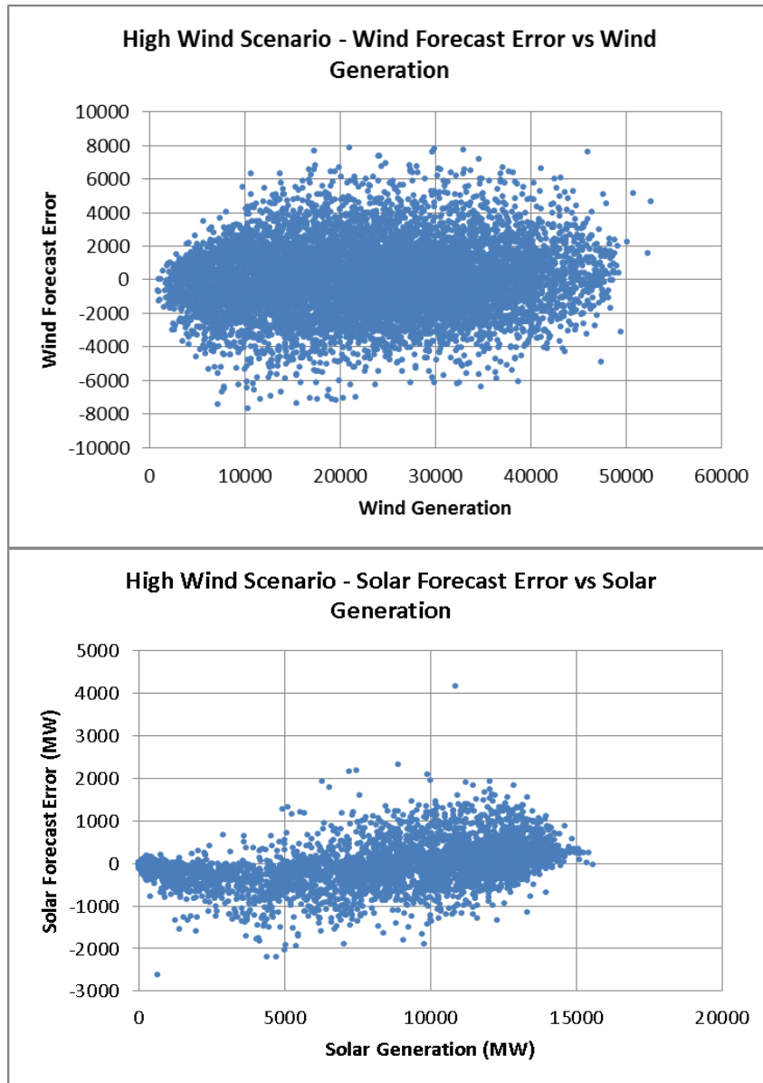
Figure 167. Wind and PV 4HA forecast error as a function of wind and solar output level for the High Wind Scenario
