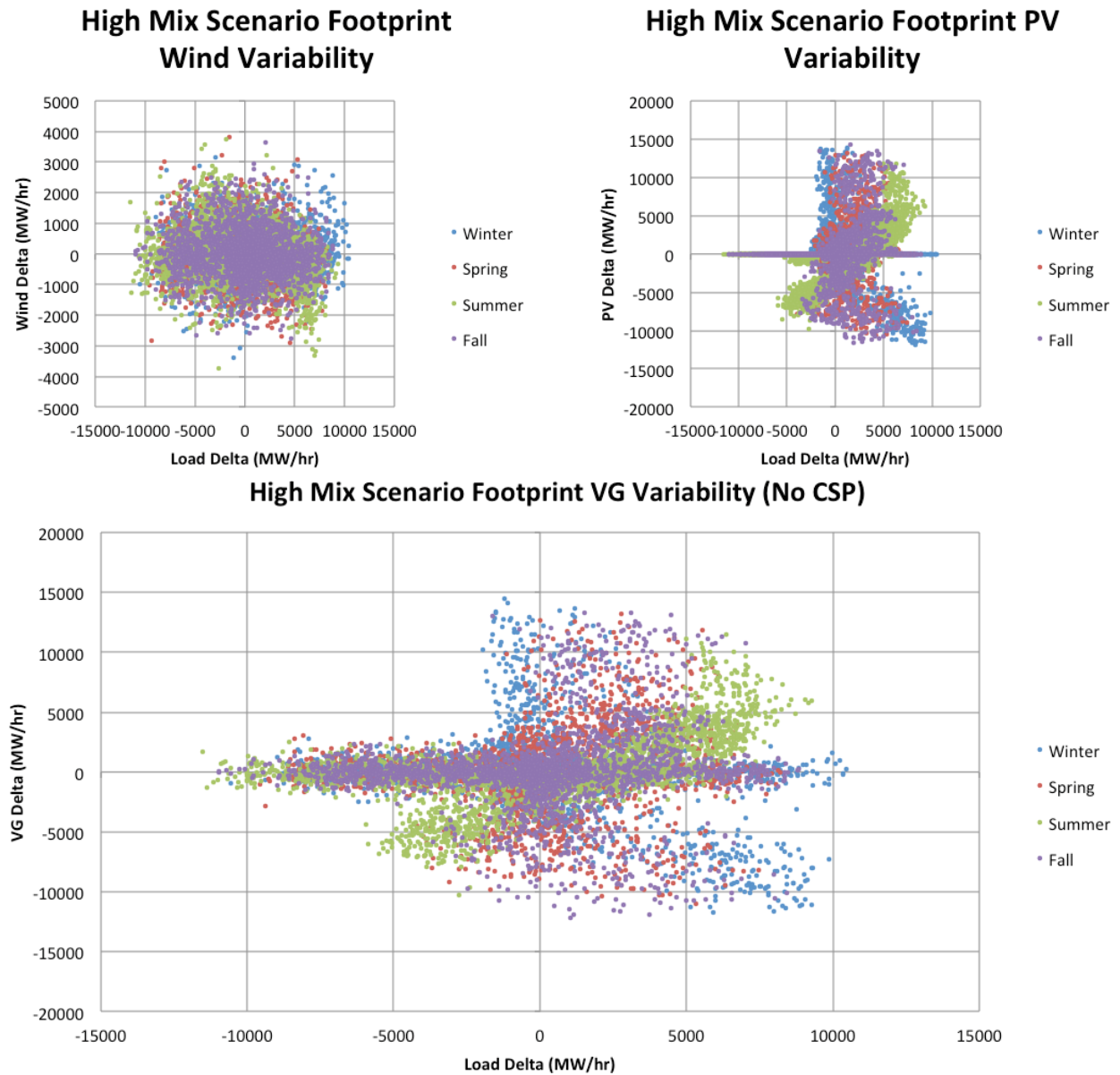
Figure 145. High Mix Scenario—hourly variability by season
