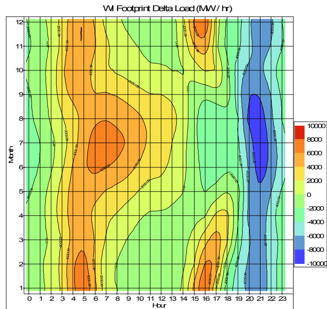
Figure 149. Delta load only with monthly average changes in MW/h
