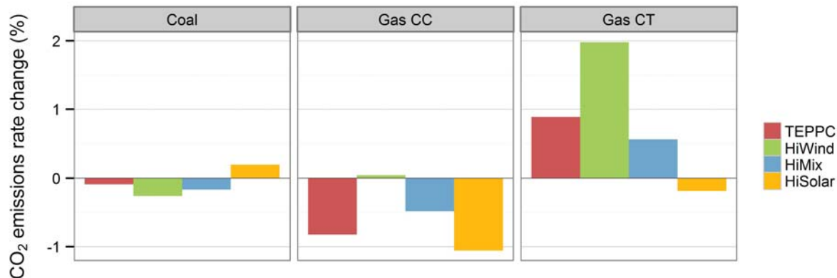
Figure 96. Change in CO 2 emission rates from the average coal, gas CC, and gas CT unit compared to the No Renewables Scenario
