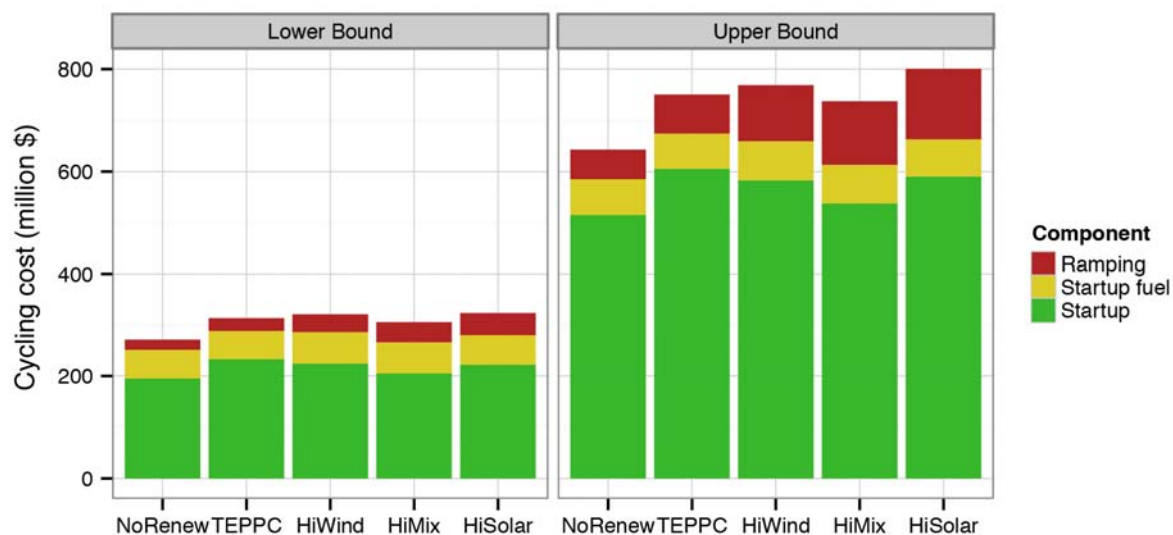
Figure 88. Cycling cost components, showing lower- and upper-bound costs from starts, start fuel, and ramping
