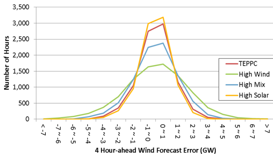
Figure 46. Four-hour-ahead wind forecast error distribution for the U.S. Western Interconnection
