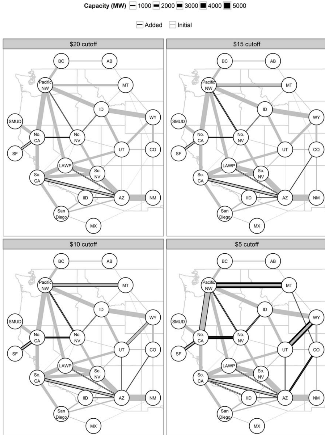
Figure 129. Transmission expansion for the High Wind Scenario showing the (gray) initial and (black) additional transmission for each shadow price cutoff value tested
