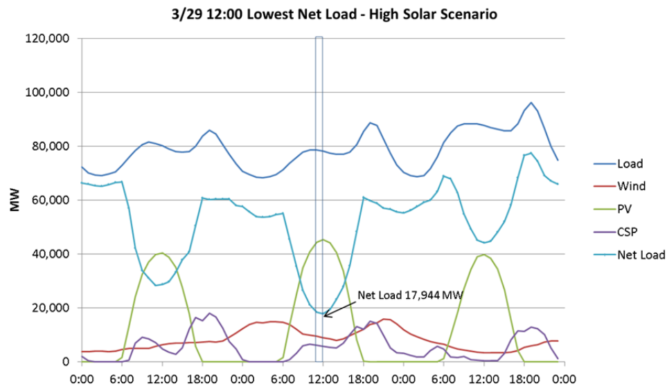
Figure 38. Minimum net load is 17,944 MW at noon on March 29 in the High Solar Scenario
