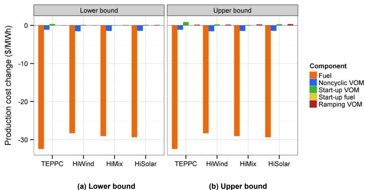
Figure 89. Change in production cost (compared to No Renewables Scenario) per MWh of wind and solar generation
