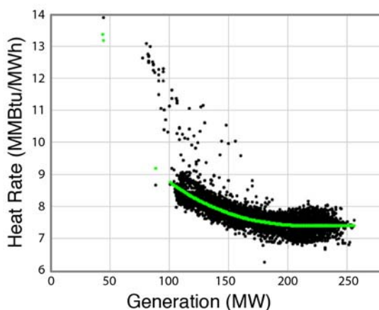
Figure 6. Typical heat-rate curve for a gas CC unit from a measured EPA CEM data set
