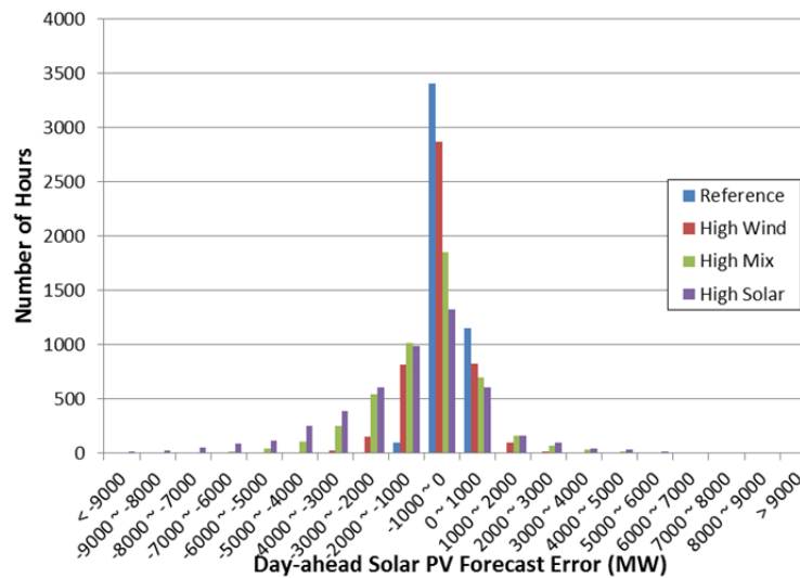
Figure 152. Distribution of DA PV forecast errors
