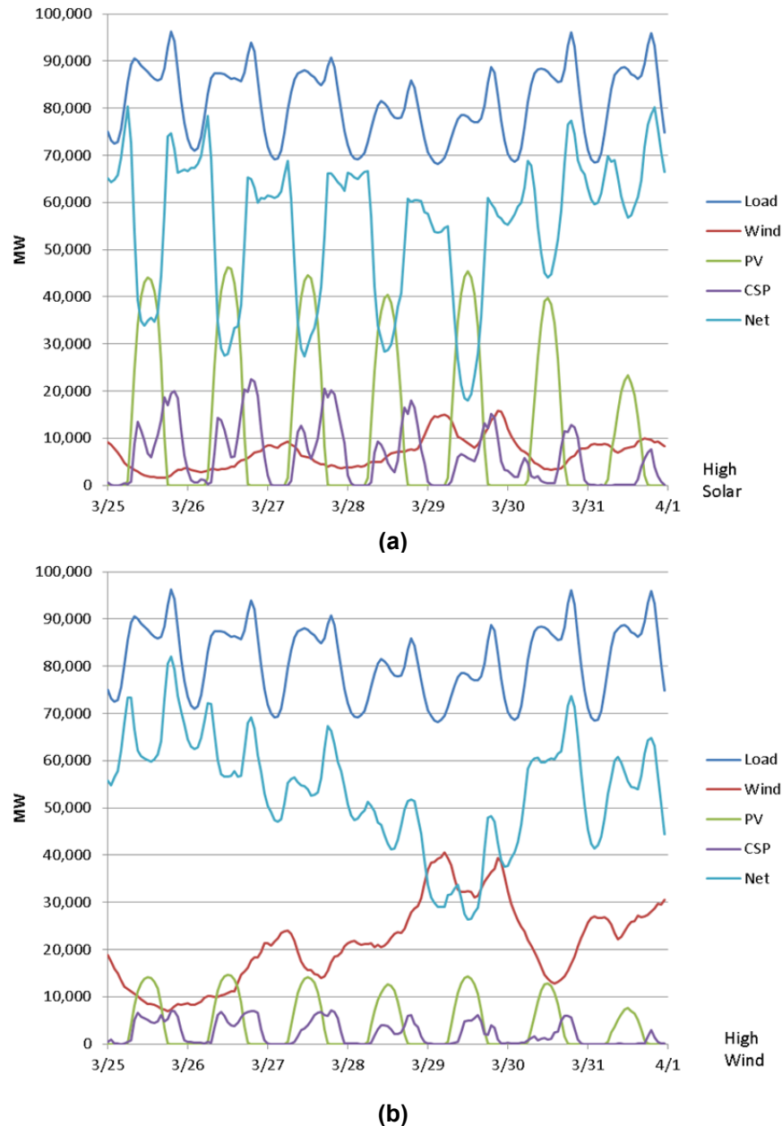
Figure 33. Profiles for the (a) High Solar and (b) High Wind Scenario for a week in March
