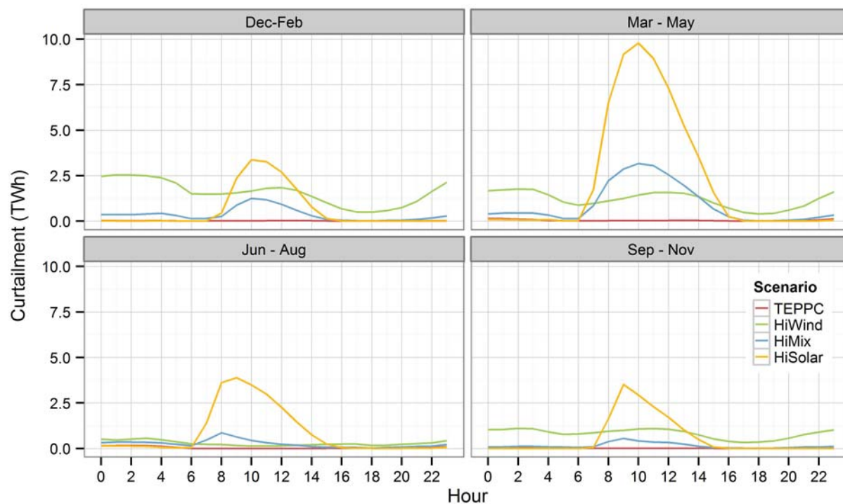
Figure 103. Average diurnal profile of curtailment by season for each scenario
