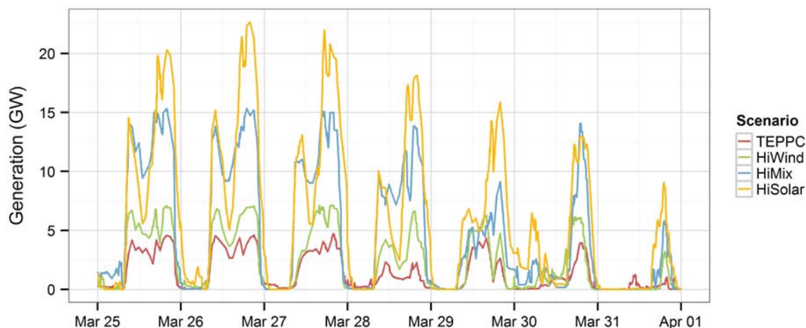
Figure 73. CSP dispatch in the spring for all scenarios
