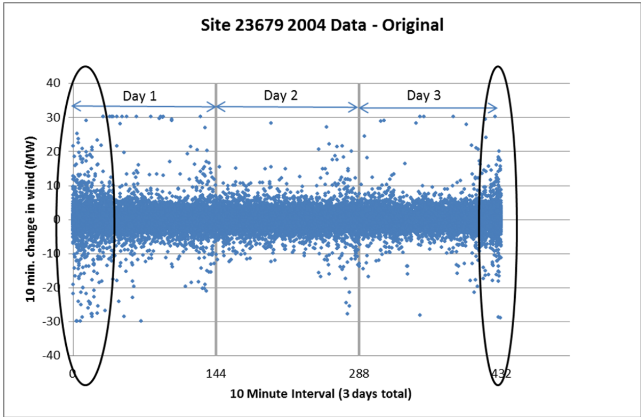
Figure 113. Distribution of wind changes by 10-minute interval number
