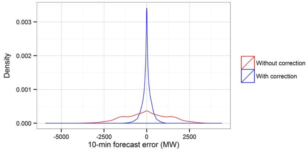
Figure 56. Ten-minute forecast error distribution with and without the clear-sky correction
