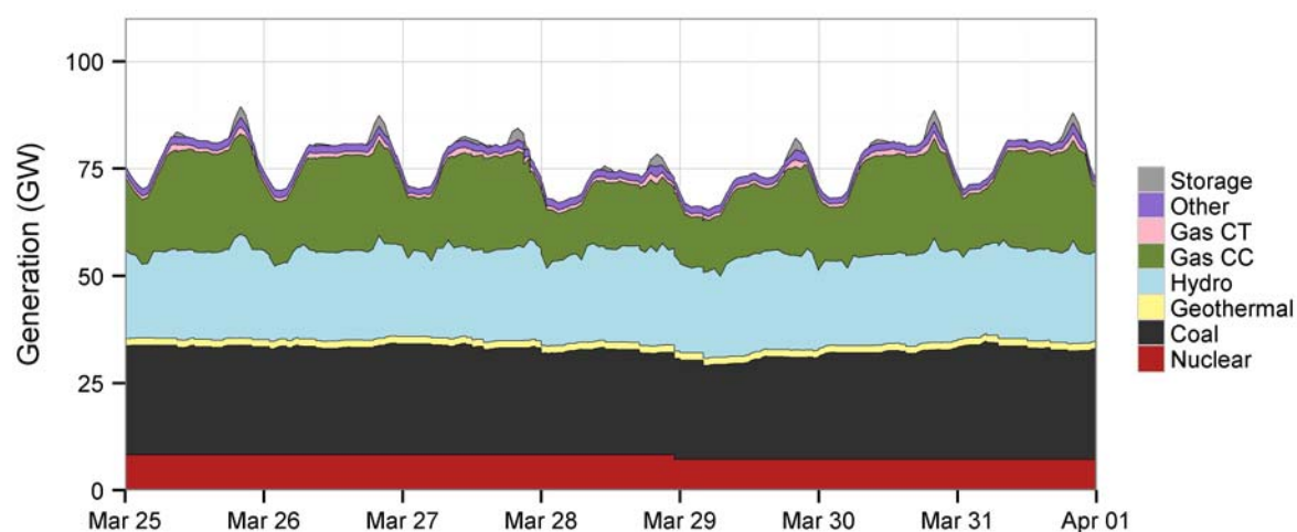
Figure 67. Spring dispatch stacks during the last week of March for the No Renewables Scenario
