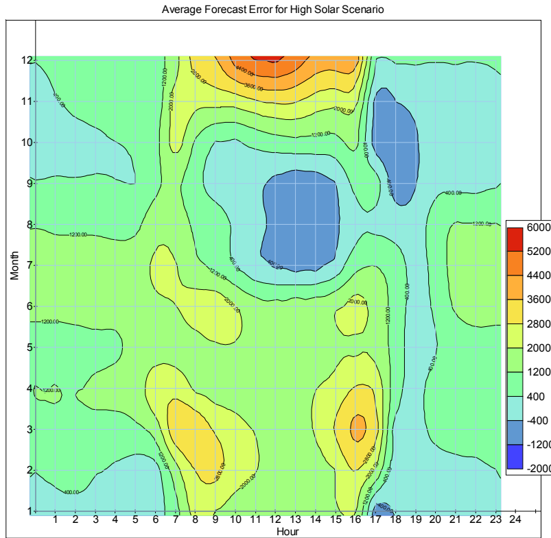
Figure 44. Contour plot of DA VG forecast errors for the High Solar Scenario
