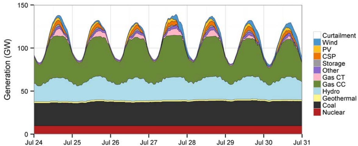
Figure 63. Summer dispatch stacks during the last week of July for the TEPPC Scenario
