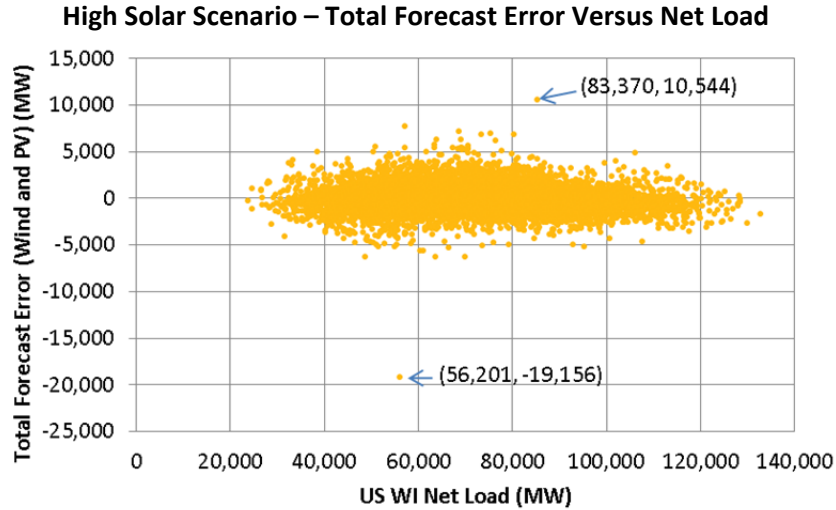
Figure 49. Four-hour-ahead wind plus PV forecast error scatter for the High Solar Scenario
