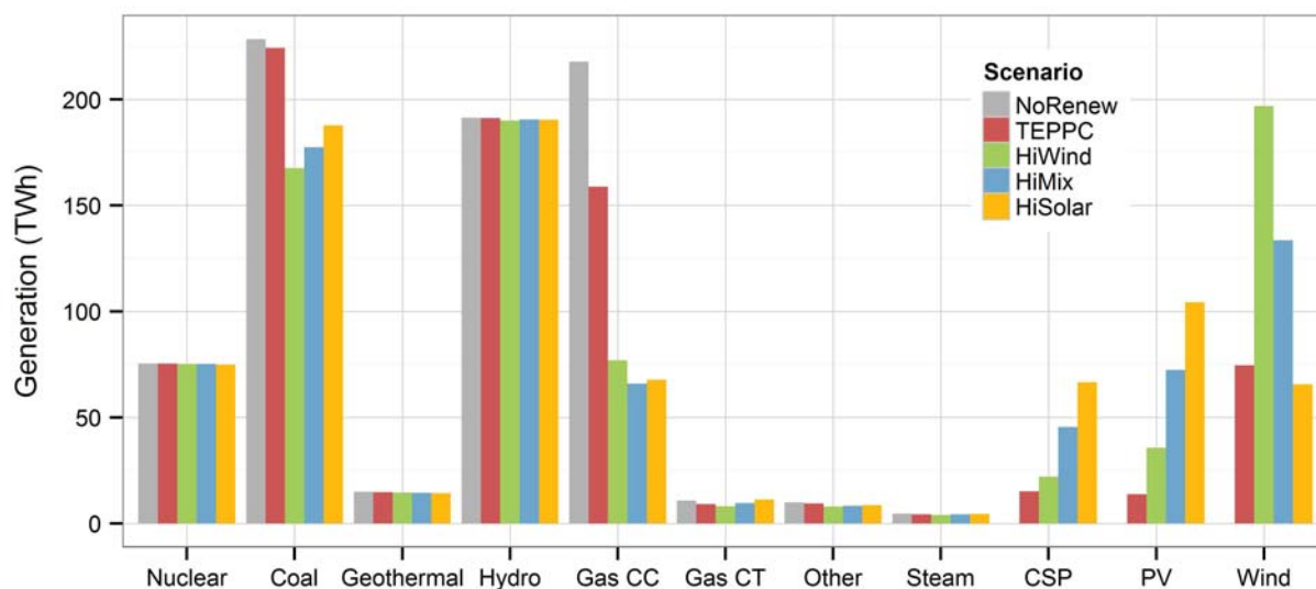
Figure 75. Generation from each type of generation unit by scenario
