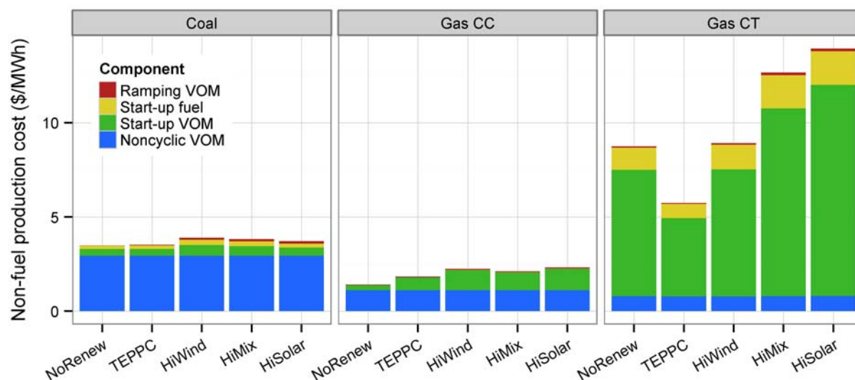
Figure 90. Lower-bound cycling costs per MWh of (left) coal, (middle) gas CC, and (right) gas CT generation
