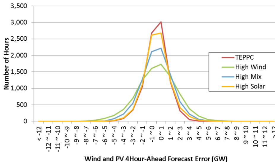
Figure 48. Four-hour-ahead wind plus PV forecast error distribution
