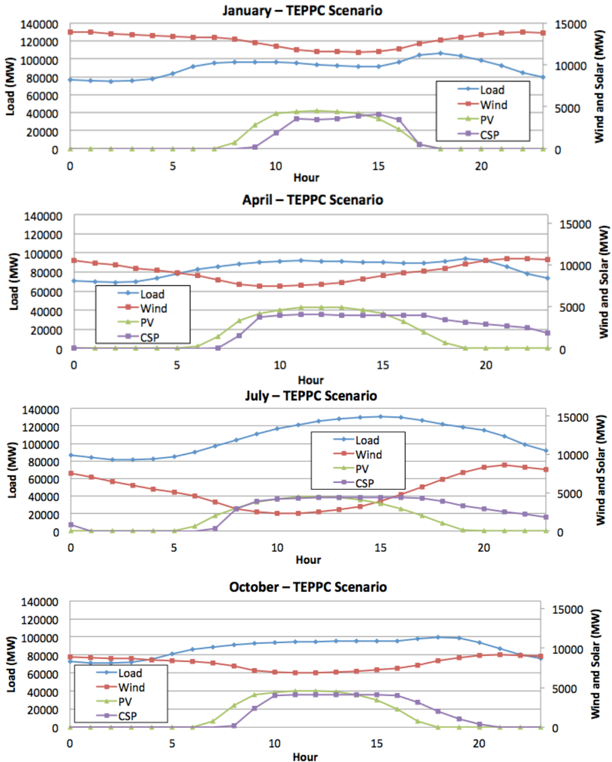
Figure 140. TEPPC Scenario—average diurnal profile
