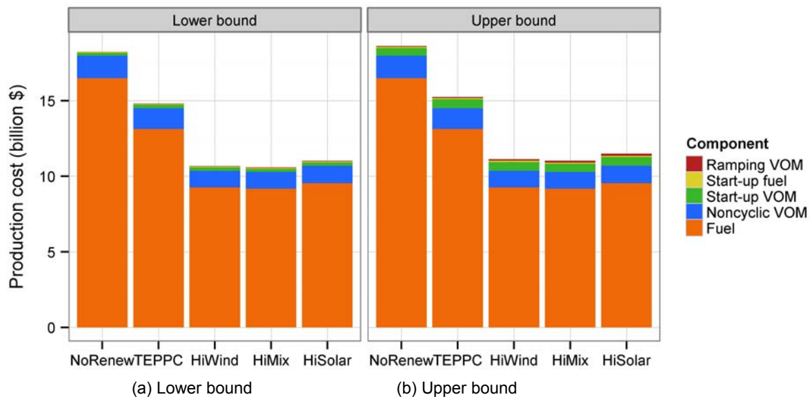
Figure 87. Total cost of each scenario broken down into fuel, noncyclic VOM, and lower- and upper-bound start wear-and-tear, start fuel, and ramping wear-and-tear costs
