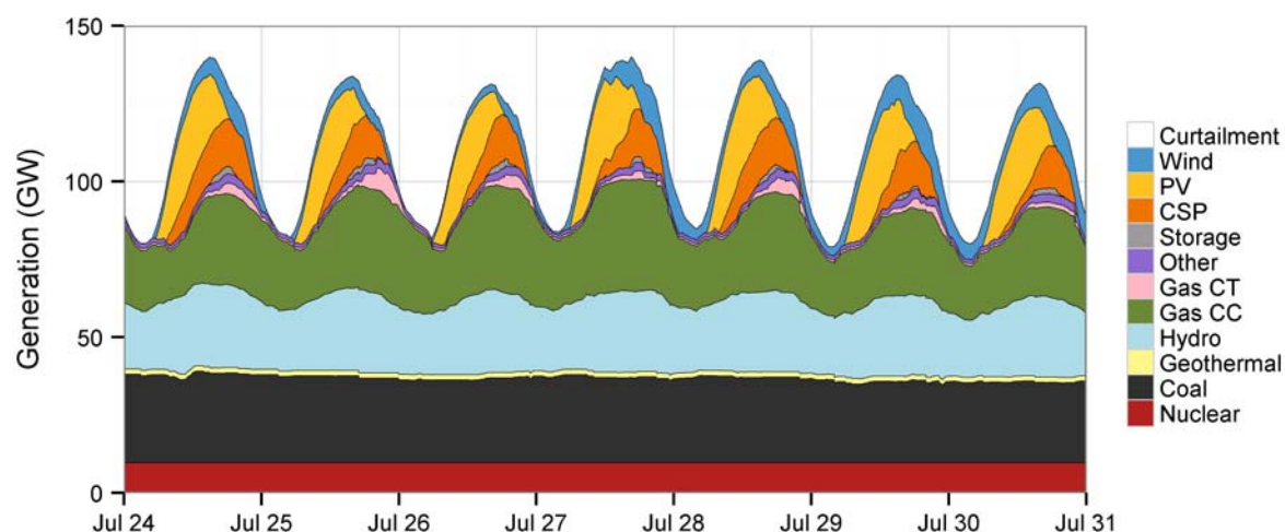
Figure 65. Summer dispatch stacks during the last week of July for the High Mix Scenario
