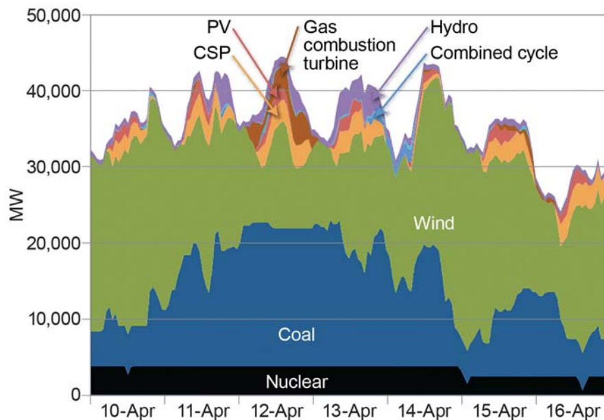
Figure 2. WWSIS-1 system dispatch for the most challenging week of 3 years of data analyzed
