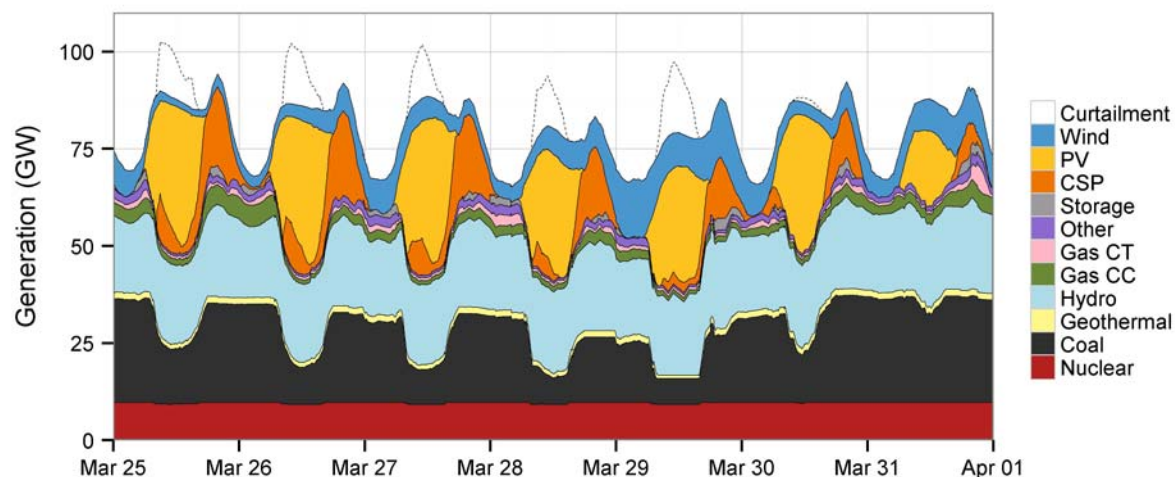
Figure 71. Spring dispatch stacks during the last week of March for the High Solar Scenario
