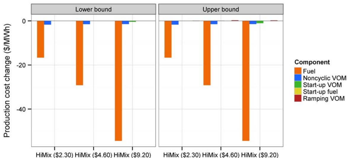
Figure 112. Production cost change per MWh of wind and solar generation in the gas price sensitivities
