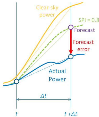
Figure 55. Graphical representation of short-term forecast for solar
