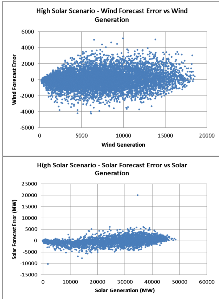
Figure 164. Wind and PV 4HA forecast error as a function of wind and PV output level for the High Solar Scenario
