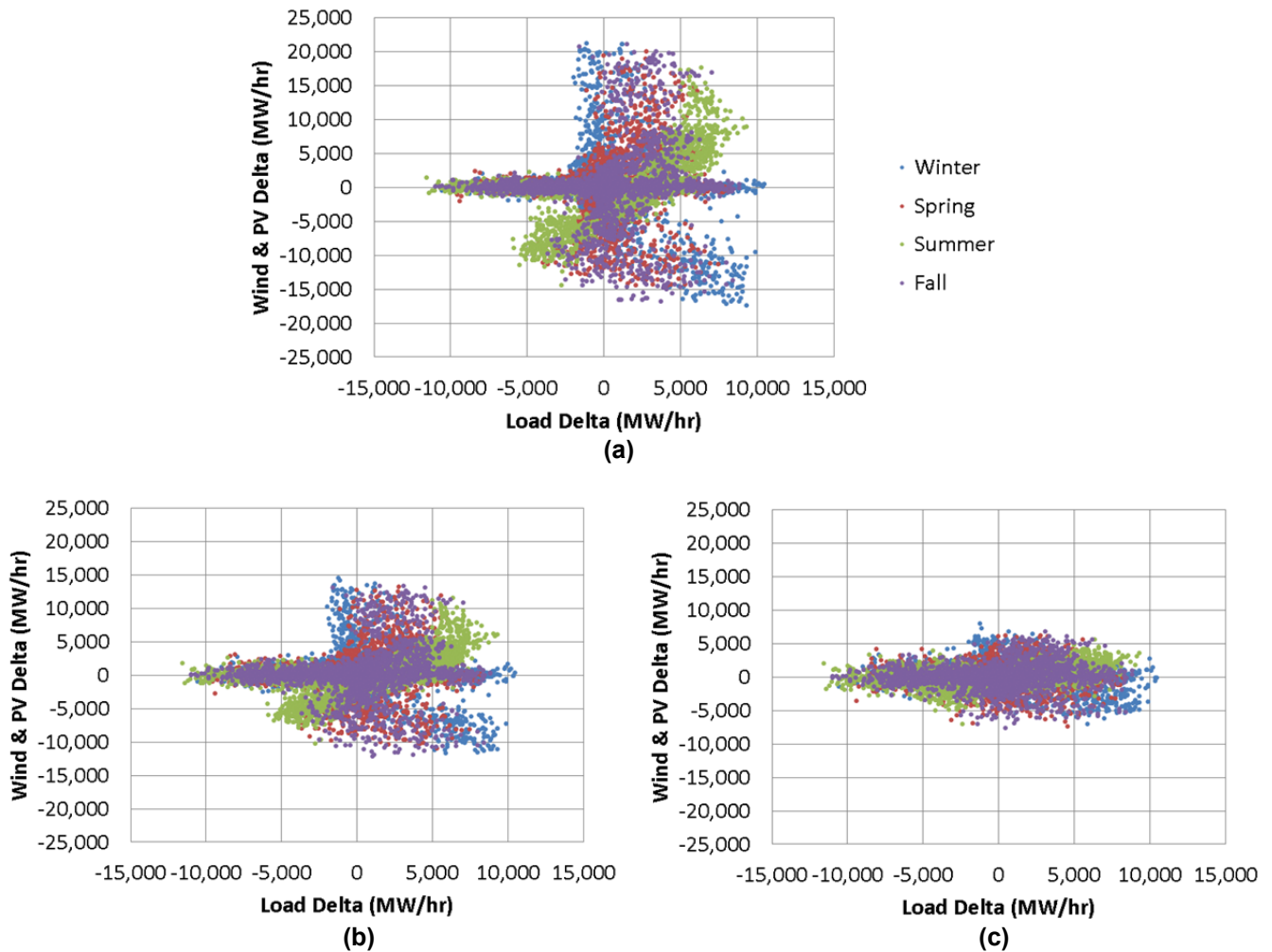
Figure 25. Hourly load change versus hourly wind and PV production change for the (a) High Solar, (b) High Mix, and (c) High Wind Scenarios for 2006
