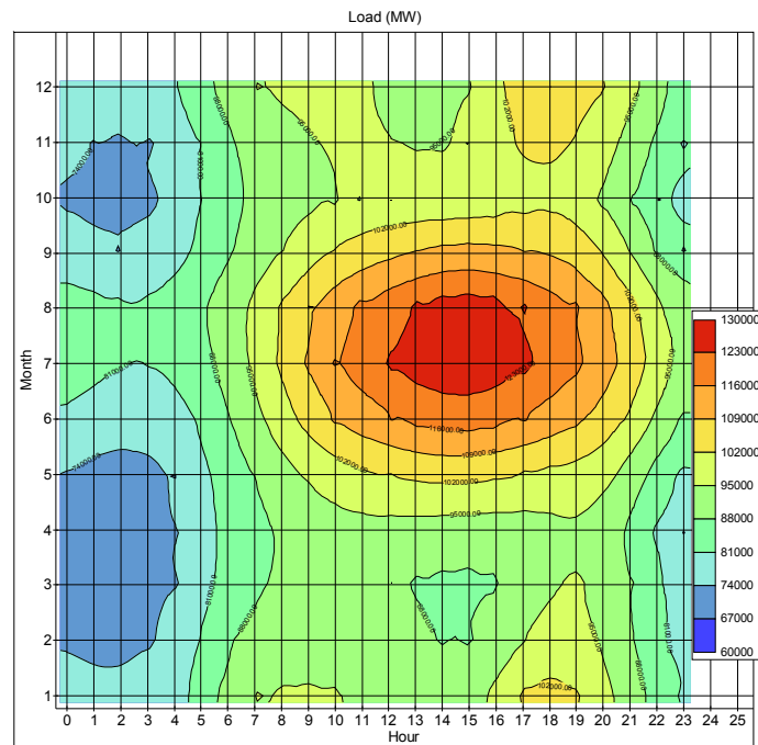
Figure 147. Load alone with monthly average values in MW
