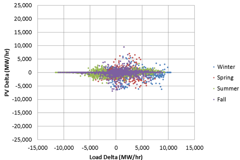
Figure 26. Weather variability component of PV variability for the High Solar Scenario
