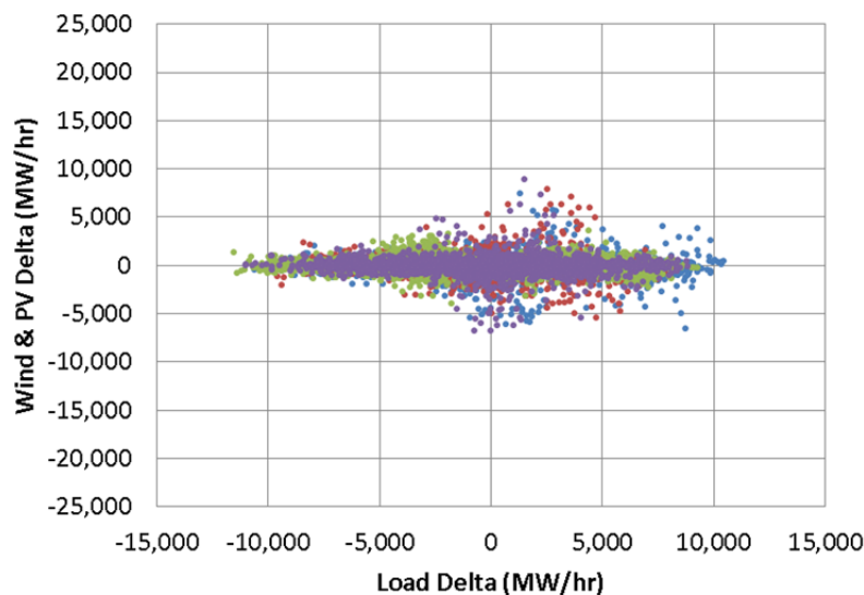
Figure 27. Total wind and PV variability excluding the diurnal solar variability for the High Solar Scenario
