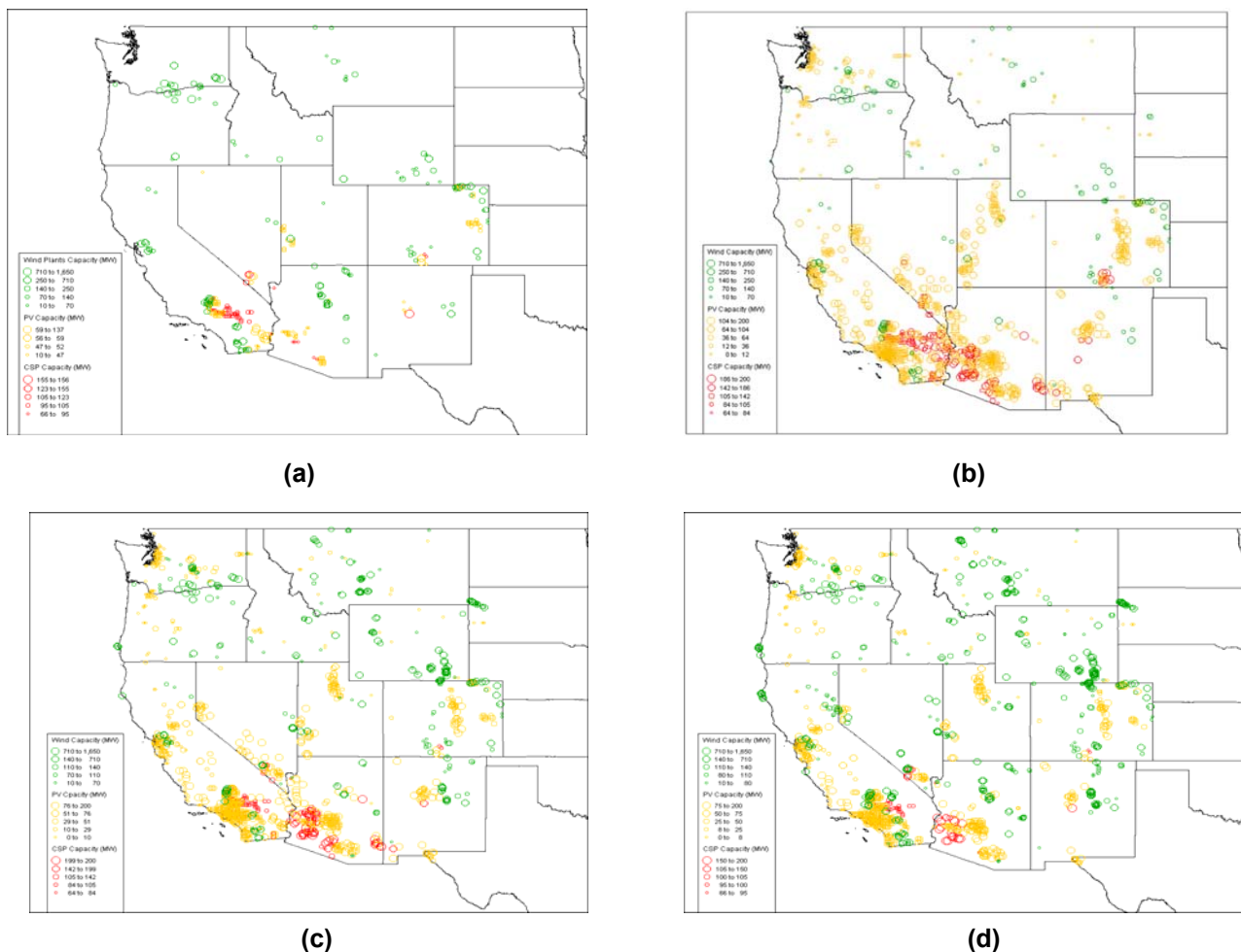
Figure 13. Siting of PV, CSP, and wind plants for the (a) TEPPC, (b) High Solar, (c) High Mix, and (d) High Wind Scenarios
