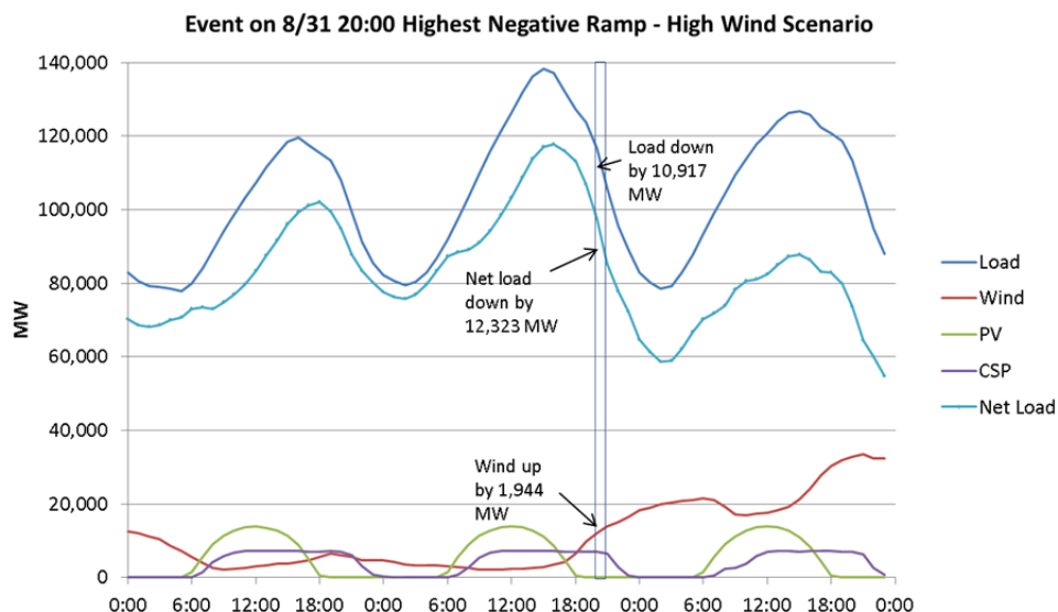
Figure 37. The largest hourly down-ramp of 12,323 MW in the High Wind Scenario occurred on August 31 at 20:00
