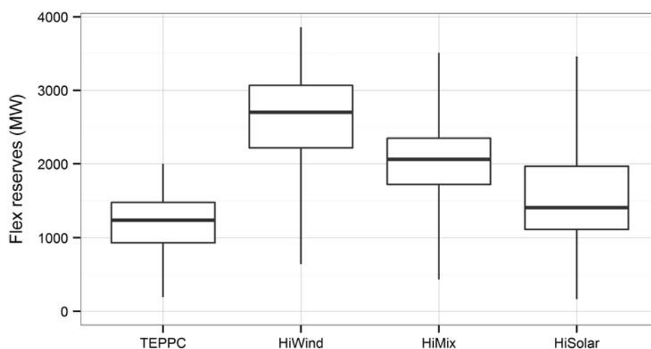
Figure 60. Distribution of flexibility reserve requirements by scenario
