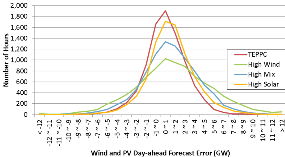
Figure 42. DA wind and PV forecast error distribution for the U.S. Western Interconnection
