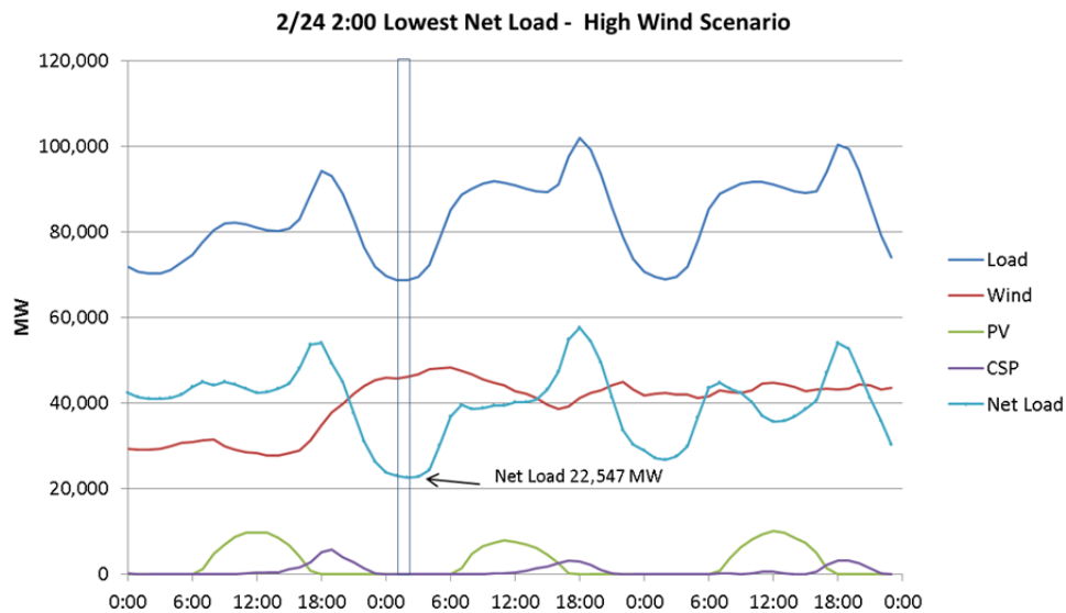
Figure 39. Minimum net load is 22,547 MW at 2:00 on February 24 in the High Wind Scenario
