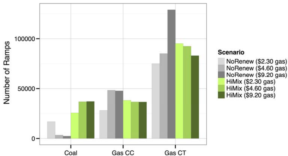
Figure 109. Number of ramps in the gas price sensitivities
