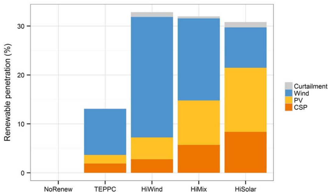
Figure 74. Renewable energy penetration of CSP, PV, and wind in the U.S. portion of the Western Interconnection for each scenario in 2006
