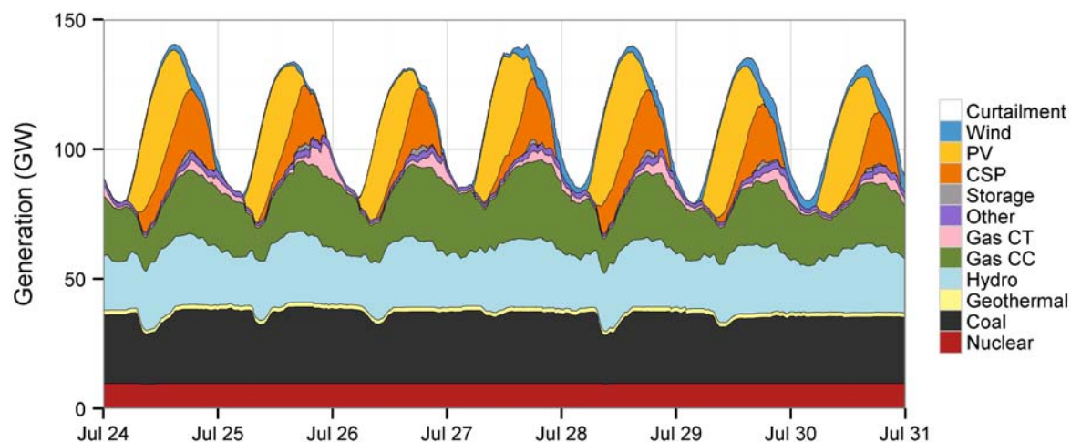
Figure 66. Summer dispatch stacks during the last week of July for the High Solar Scenario
