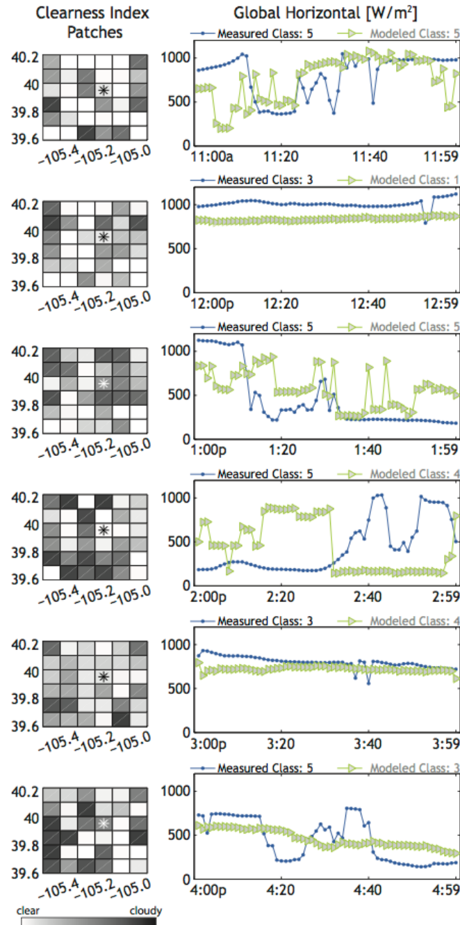
Figure 12. Snapshot satellite clearness index (left) and temporal GHI (right) from NREL on August 22, 2005
