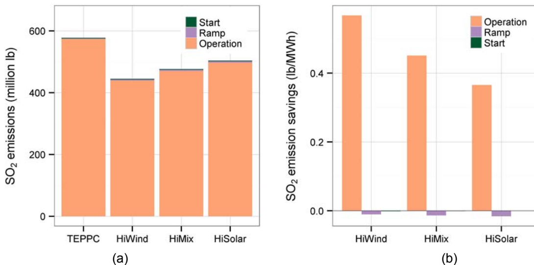
Figure 94. SO 2 emissions by scenario: (a) absolute SO 2 emissions for operation, ramping, and starts and (b) SO 2 emission reductions per MWh of wind and solar generation compared to the No Renewables Scenario, separated into the constant emissions rate assumption and adjustments for ramping and starts
