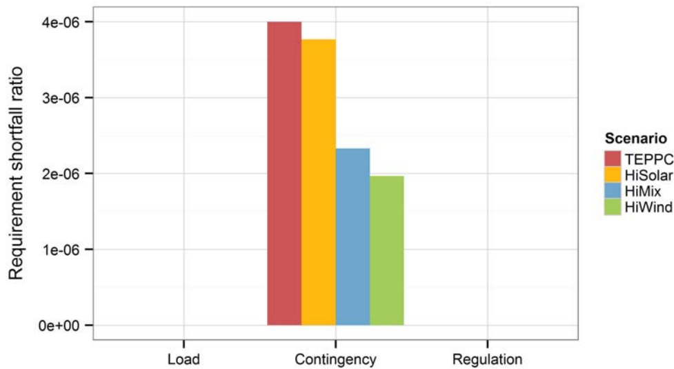
Figure 100. Unserved load and contingency and regulation reserve shortfalls, by scenario (as a fraction of total reserve requirement)
