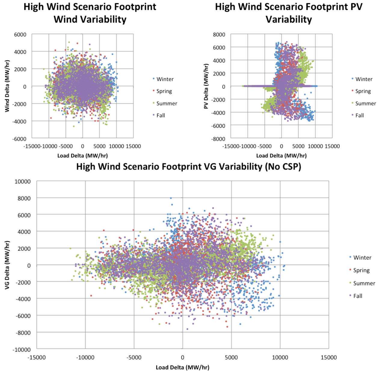
Figure 146. High Wind Scenario—hourly variability by season
