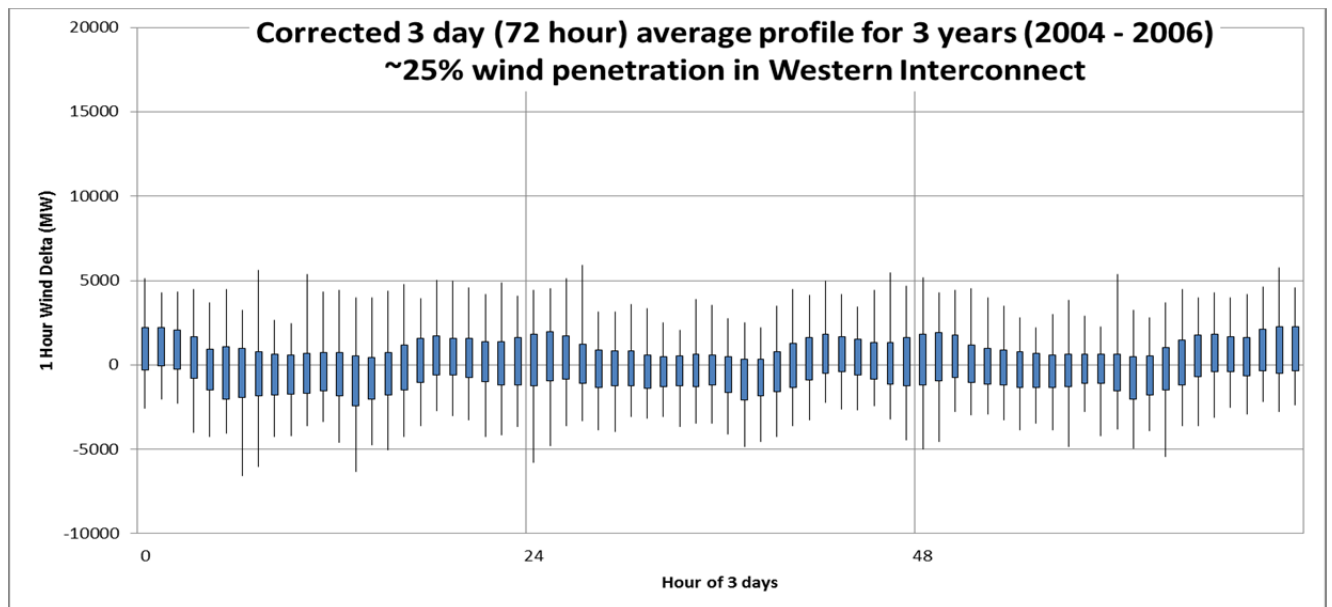
Figure 122. Bar and whisker for hourly changes for corrected data
