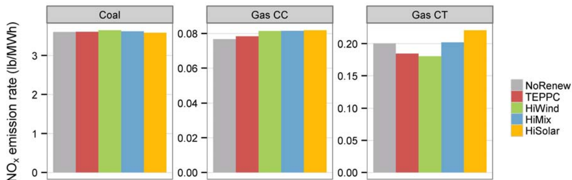
Figure 97. NO x emission rates from the average coal, gas CC, and gas CT unit
