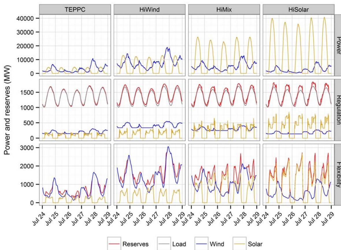
Figure 61. Power, regulation, and flexibility reserves for a few selected days in July, by scenario
