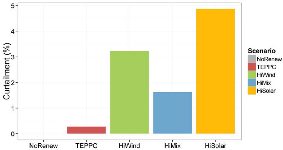
Figure 101. Curtailment as a percentage of available wind and PV generation
