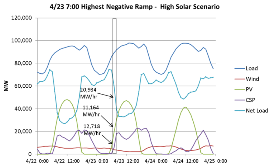
Figure 35. Highest hourly negative ramp (down-ramp) of 20,934 MW in the High Solar Scenario occurs on April 23 at 7:00
