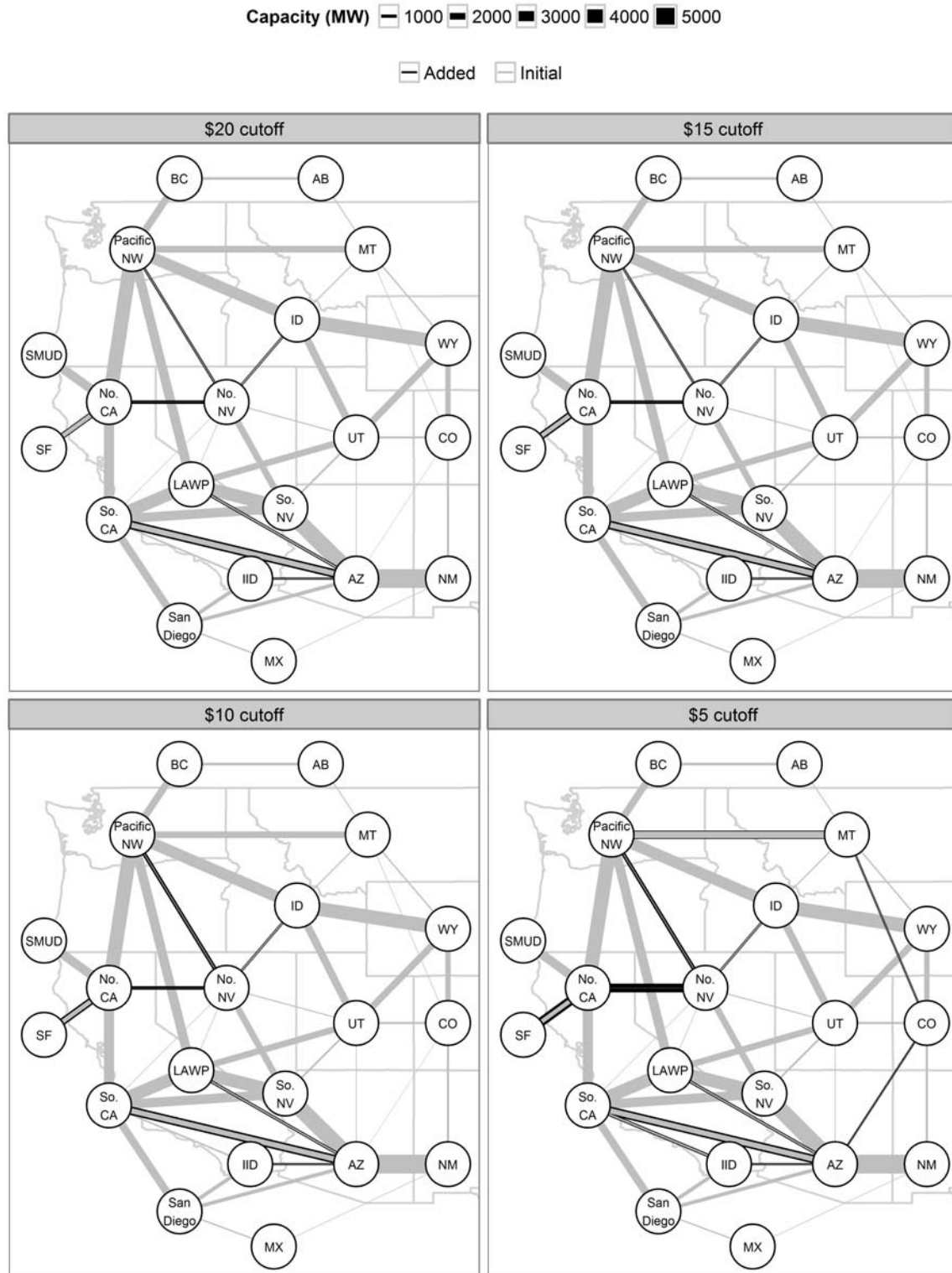
Figure 131. Transmission expansion for the High Solar Scenario showing the (gray) initial and (black) additional transmission for each shadow price cutoff value tested
