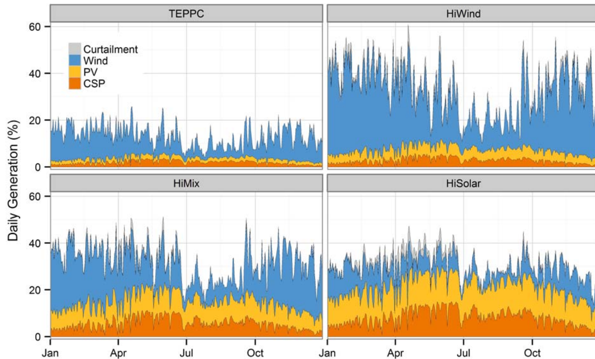
Figure 77. Daily wind and solar energy penetration for each scenario
