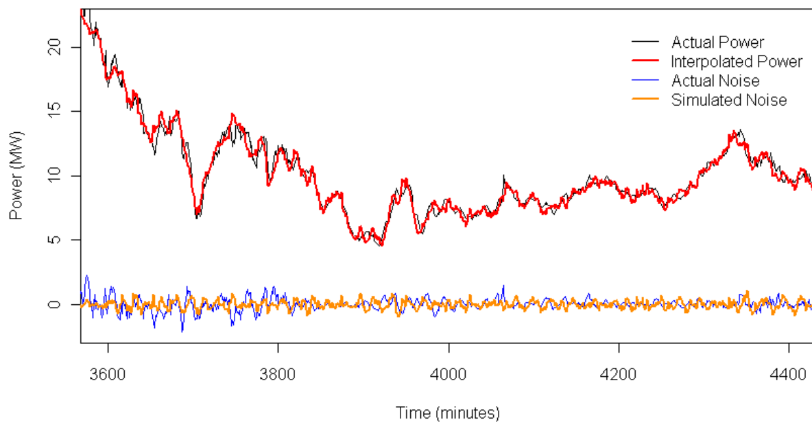
Figure 126. Comparison of interpolated 1-minute wind power data to actual data for December 2011 (time between 3,600 and 4,400 minutes)
