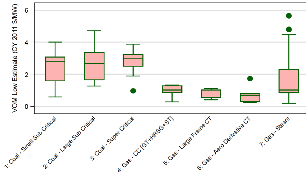
Figure 5. Lower-bound noncyclic VOM costs per MW of capacity
