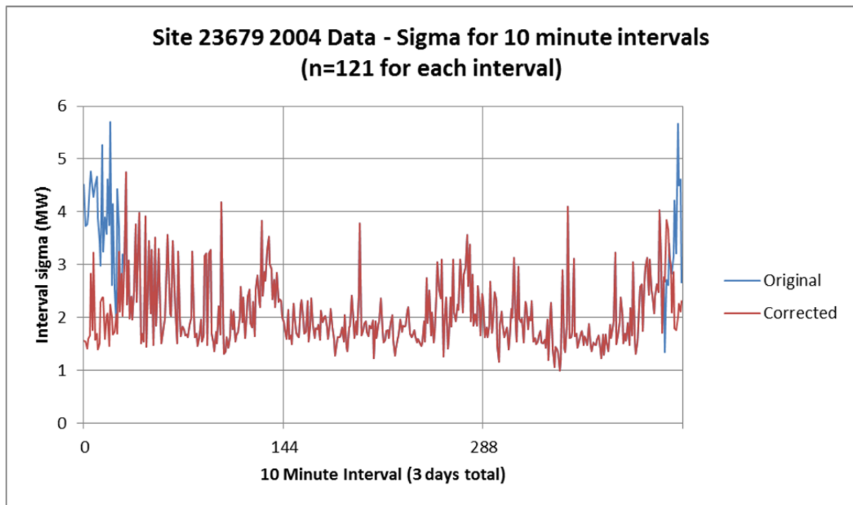
Figure 116. Standard deviation for 10-minute intervals for a single site
