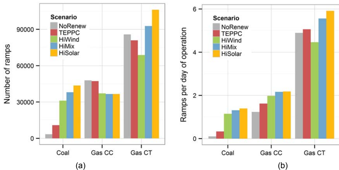
Figure 80. (a) Total number of ramps and (b) ramps per day by plant type for each scenario
