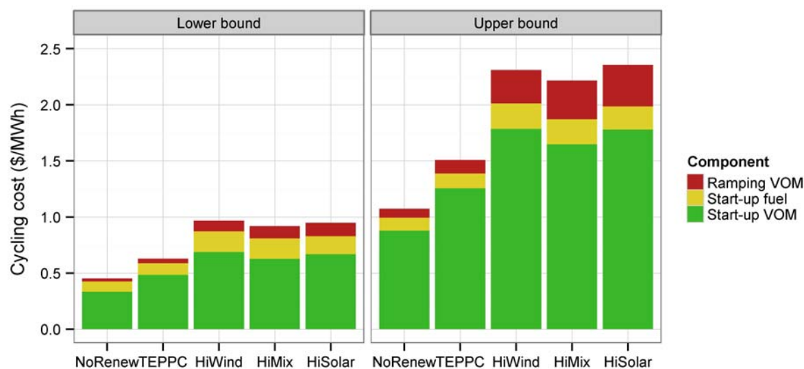
Figure 91. Lower- and upper-bound cycling costs per MWh of fossil-fueled generation for all scenarios
