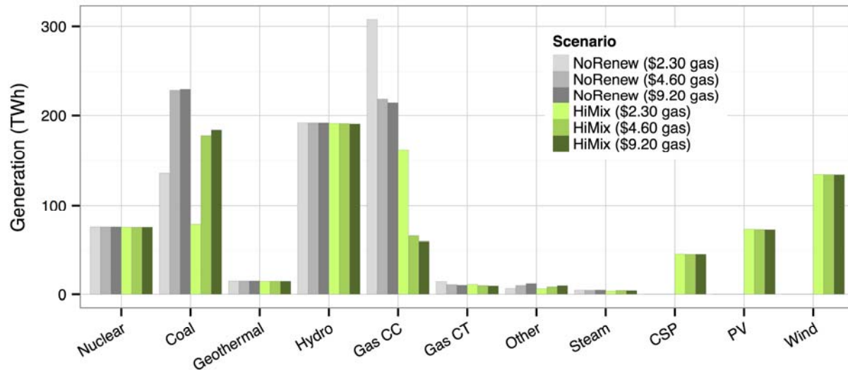
Figure 106. Annual generation by type in the gas price sensitivities
