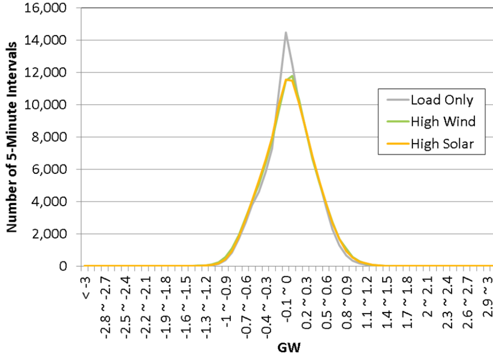
Figure 31. Distribution of 5-minute changes in load and net load for High Wind and High Solar Scenarios
