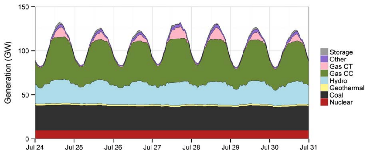
Figure 62. Summer dispatch stacks during the last week of July for the No Renewables Scenario
