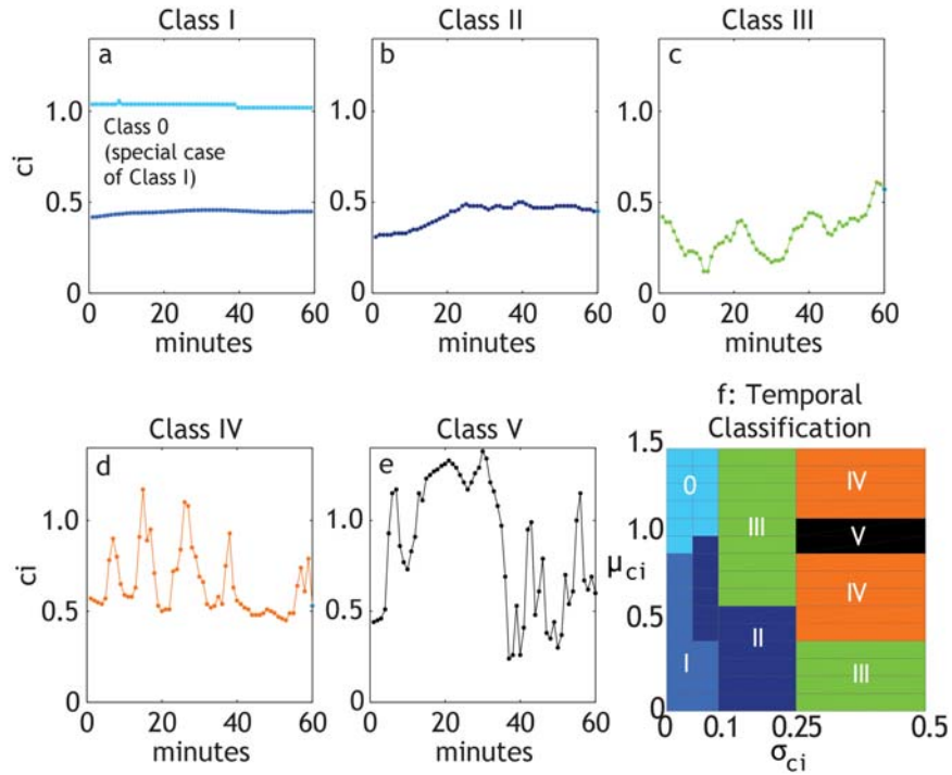
Figure 11. Examples of the five classes of temporal variability are shown in plots (a) through (e)
