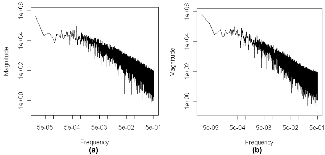
Figure 123. Power spectra of the Cedar Creek turbines for (a) August 2011 and (b) December 2011
