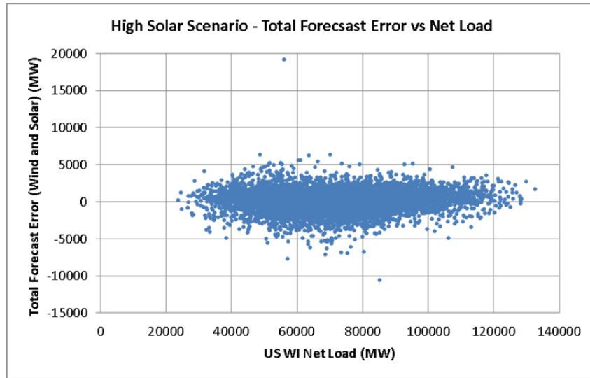
Figure 165. Wind plus PV 4HA forecast error as a function of net load level for the High Solar Scenario
