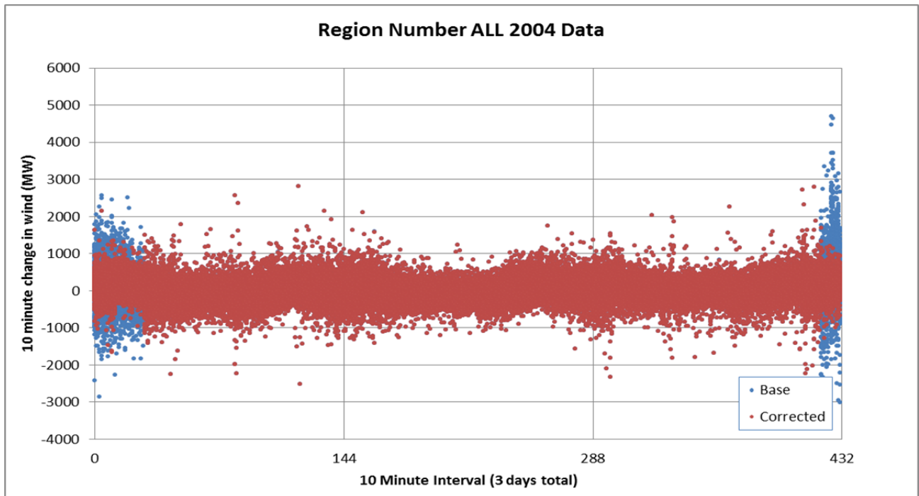
Figure 117. Ten-minute wind change distribution by interval for all regions aggregated
