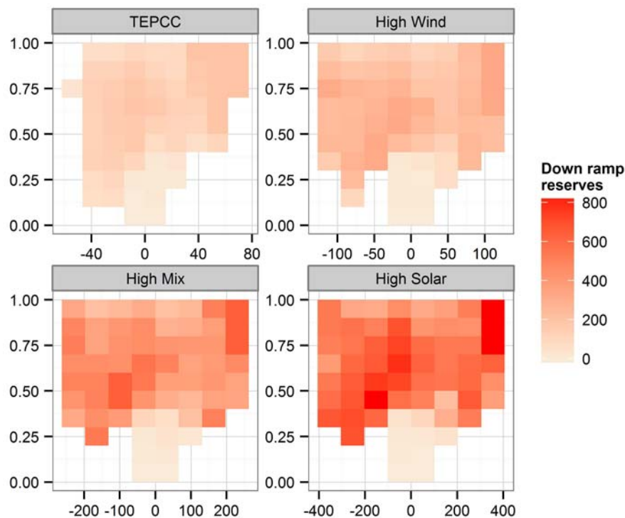
Figure 57. Regulation reserve requirements by scenario for the entire Western Interconnection
