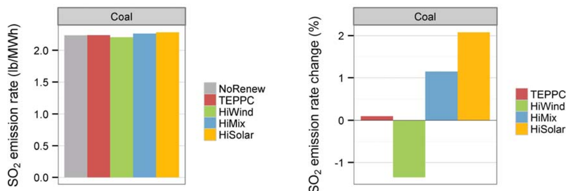
Figure 99. SO 2 emission rates from the (a) average coal unit and (b) change compared to the No Renewables Scenario
