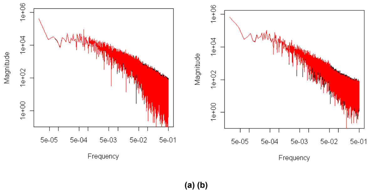
Figure 124. Power spectrums using simulated (red) high-frequency noise overlaid on (black) power spectrums from actual data for (a) August 2011 and (b) December 2011
