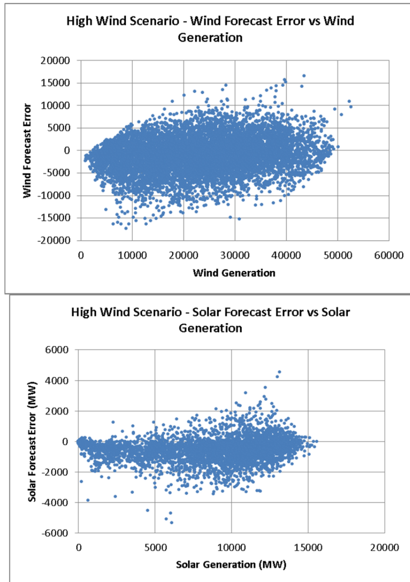
Figure 158. Wind and solar DA forecast error as a function of wind and solar output level for the High Wind Scenario
