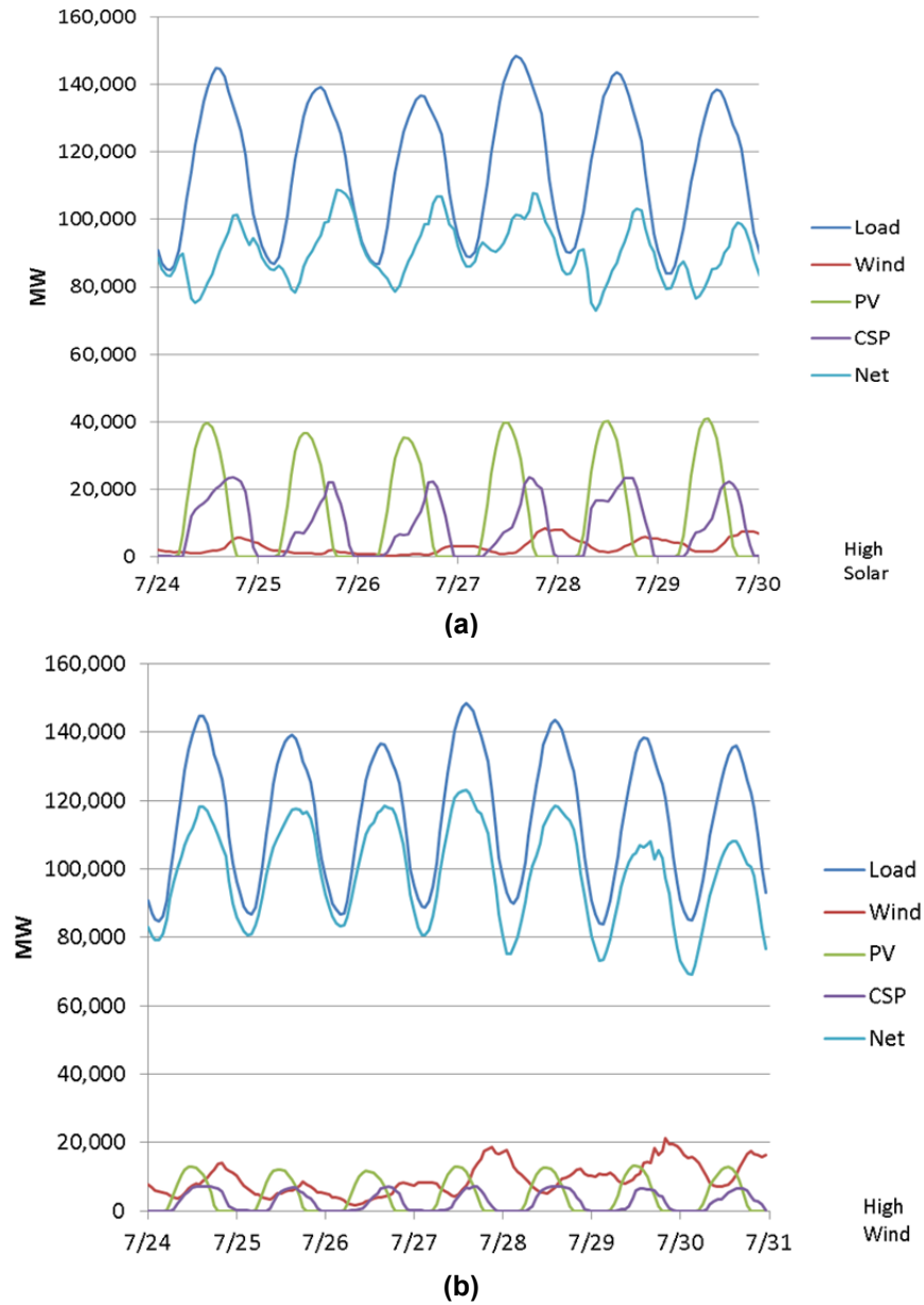
Figure 32. Profiles for the (a) High Solar and (b) High Wind Scenario for a week in July
