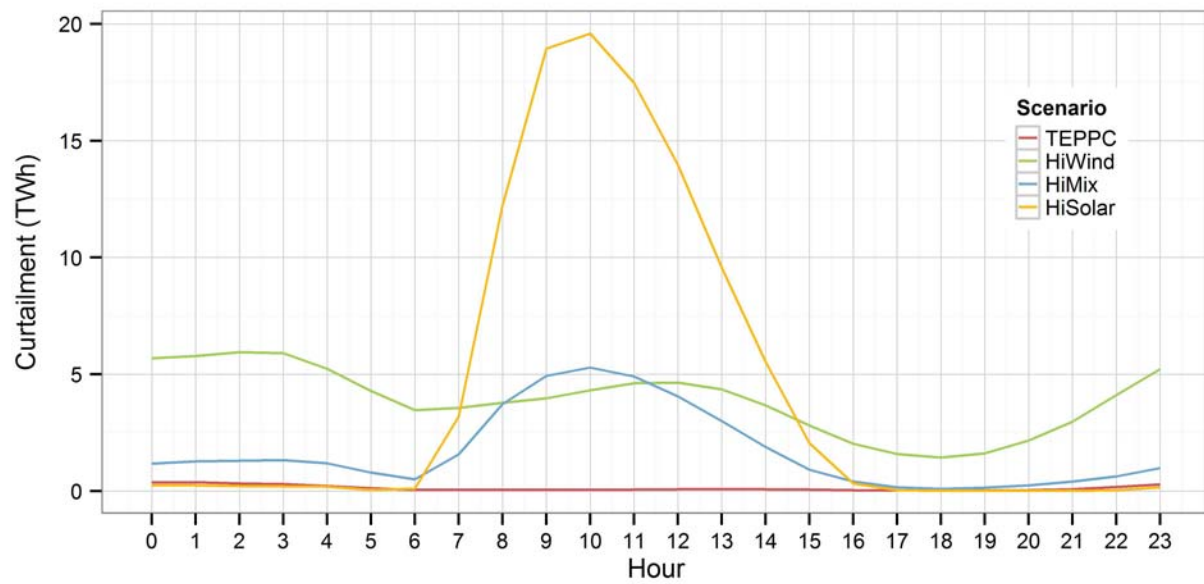
Figure 102. Curtailment diurnal profile for each scenario
