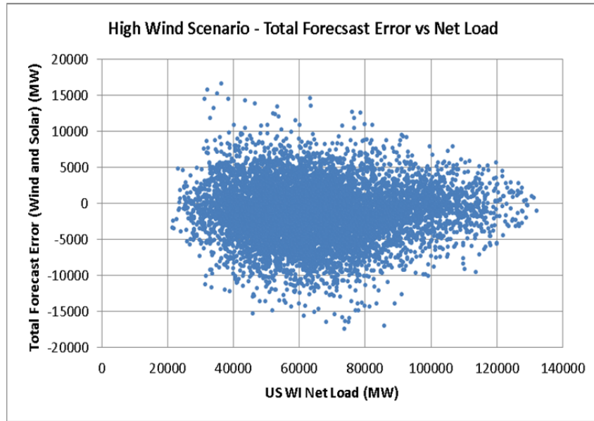
Figure 159. Wind plus PV DA forecast error as a function of net load for the High Wind Scenario
