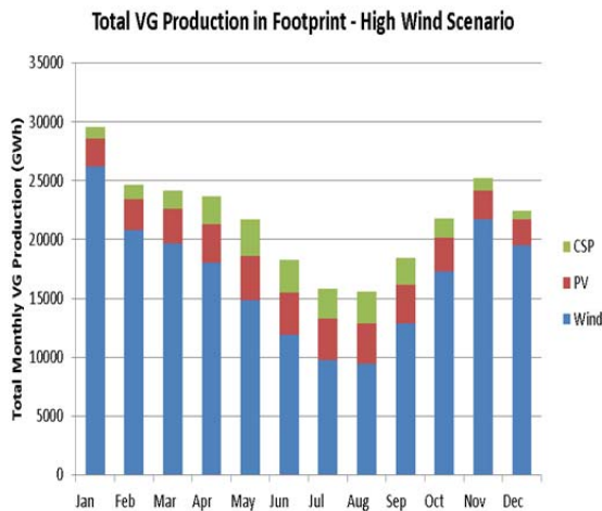
Figure 138. High Wind Scenario—monthly profiles
