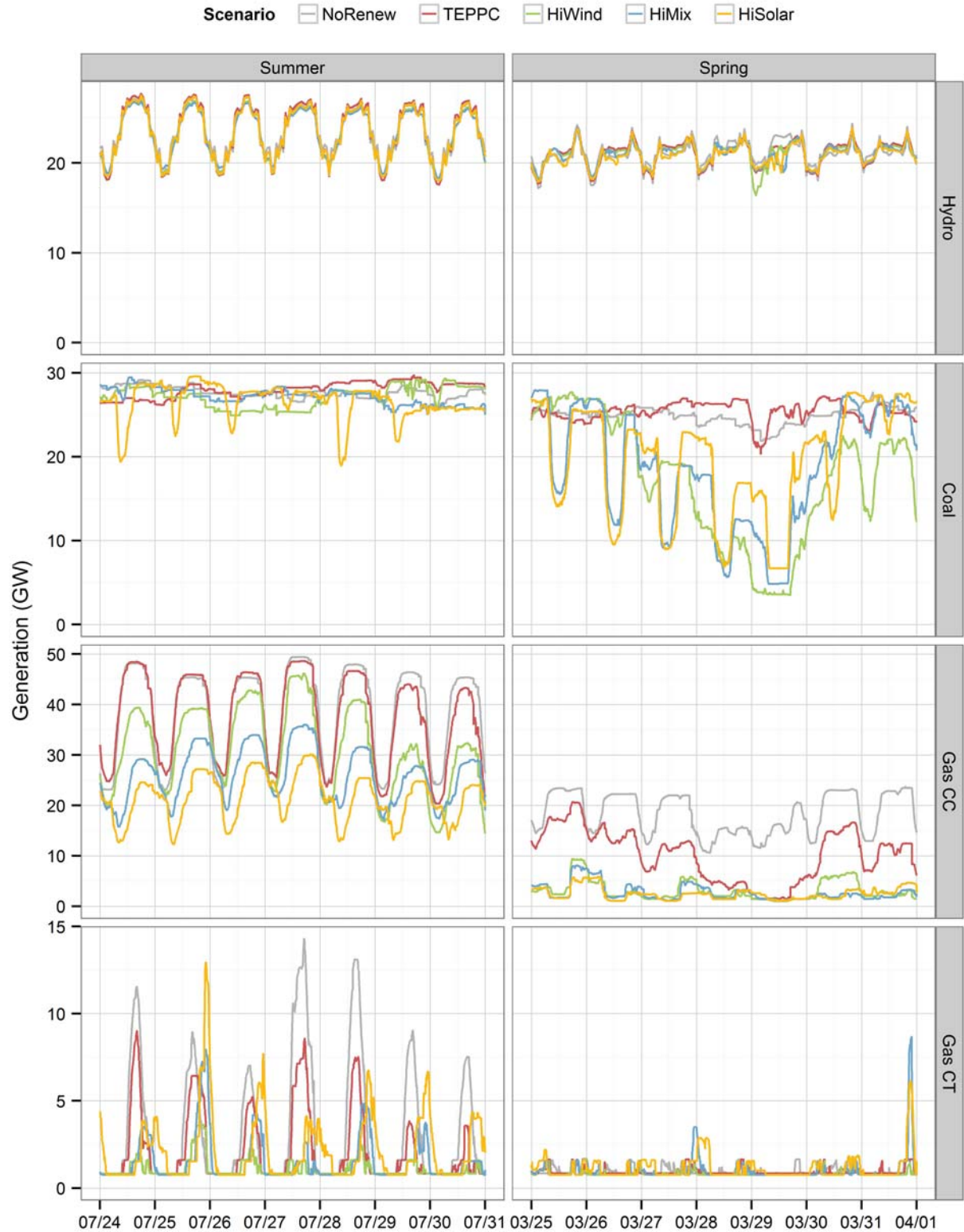
Figure 72. Hydro, coal, gas CC, and gas CT dispatch in the (left) summer and (right) spring for all scenarios
