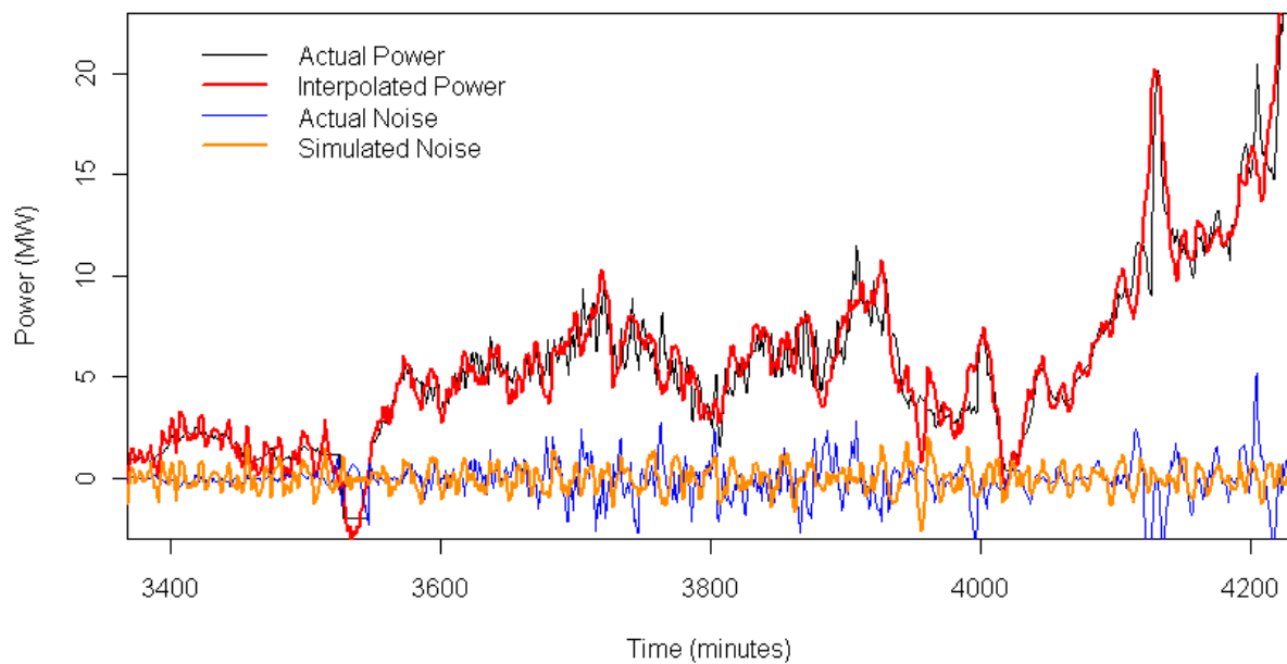
Figure 125. Comparison of interpolated 1-minute wind power data to actual data for August 2011 (time between 3,400 and 4,200 minutes)
