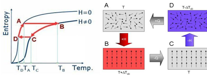
Figure 3-10: Magnetic Cooling Cycle
