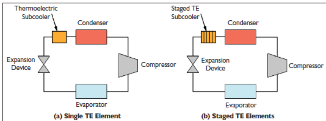
Figure 3-7: Vapor-compression Systems with TE Subcoolers
