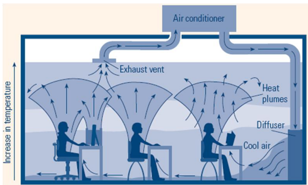
Figure 3-24: Typical Airflow Pattern of a Thermal Displacement Ventilation System Source: CEC (2008)
