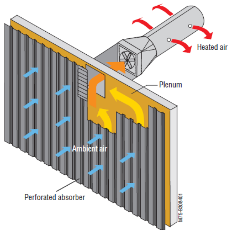
Figure 3-15: Typical Solar Ventilation System
