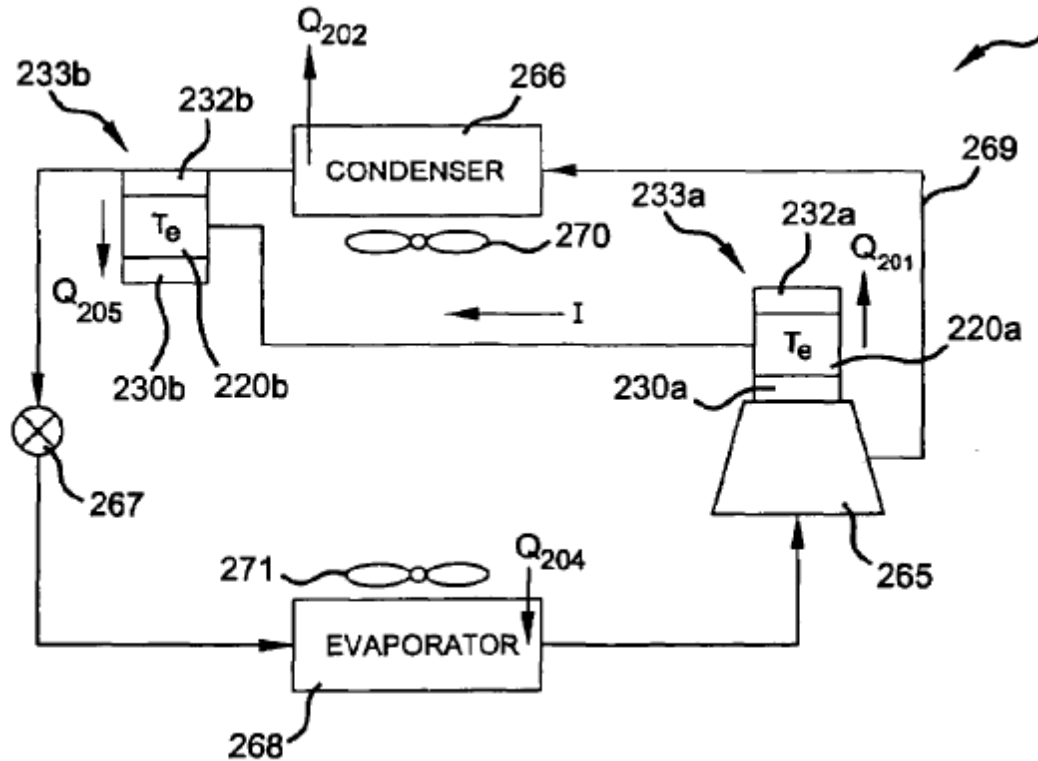
Figure 3-6: Vapor-compression System with TE Subcooler Powered by TE Generator
