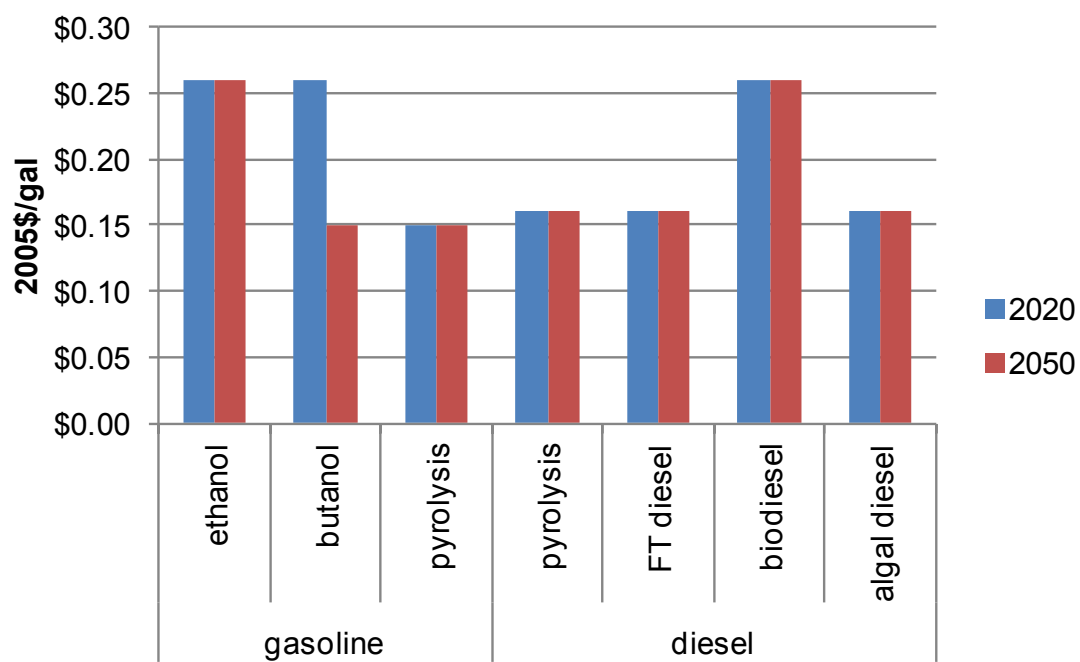
Figure G.1. Fuel distribution and marketing costs
