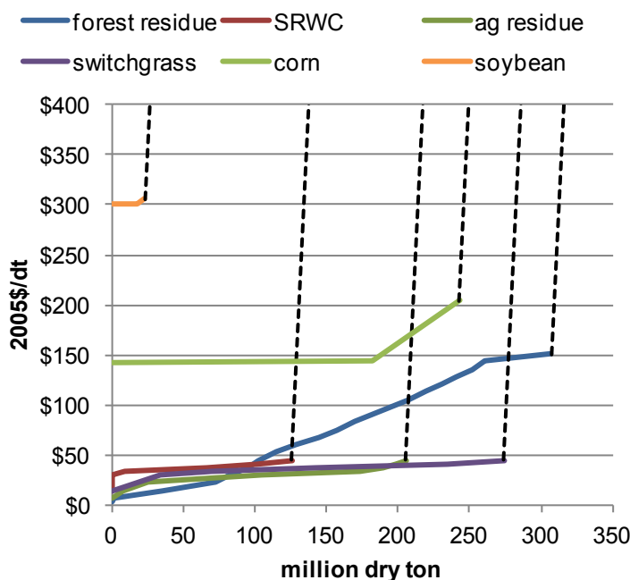
Figure C.10. Supply curves used for the 2050 BASE runs
