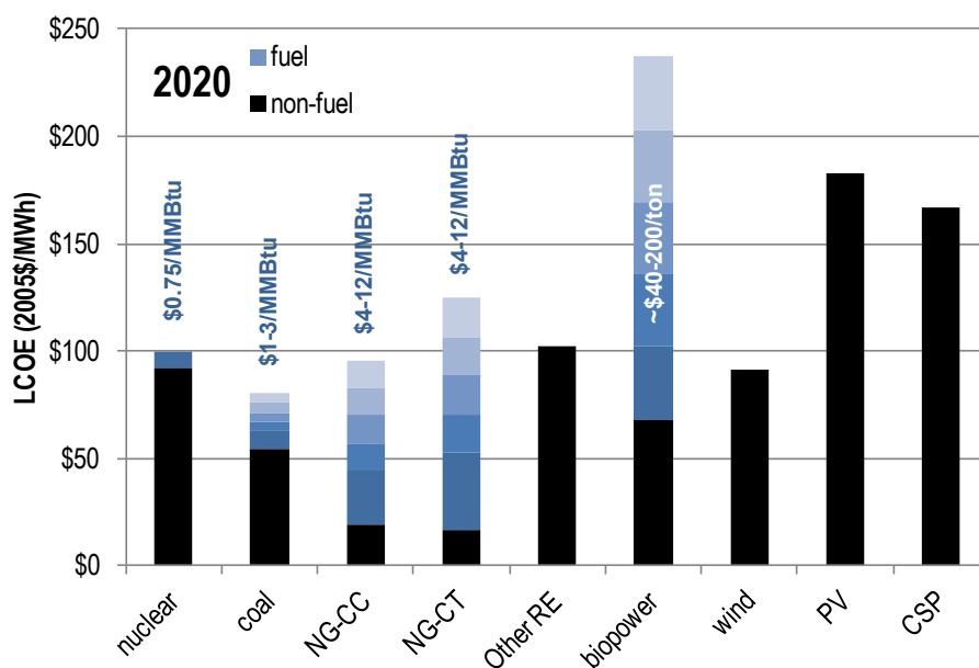
Figure 4.5. LCOE breakdown for electricity in 2020
