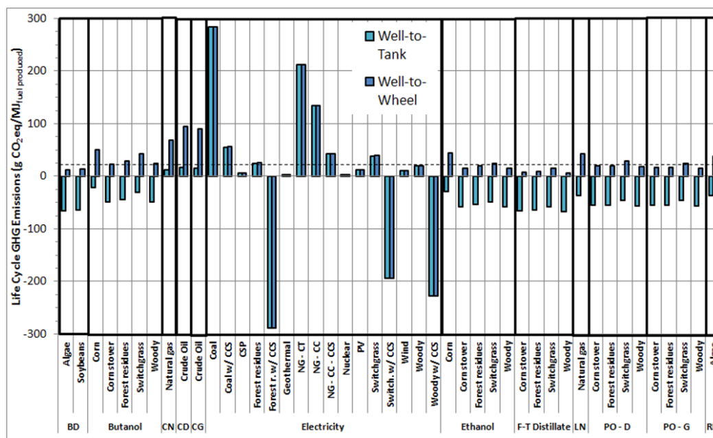
Figure 3.6. WTW and WTT life cycle GHG emission estimates used in the BASE model for 2050
