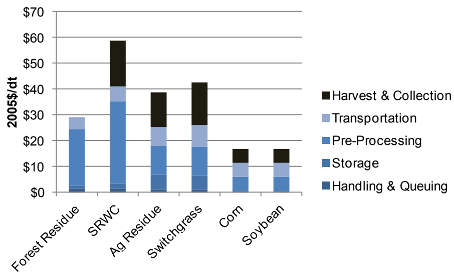
Figure E.2. Feedstock logistic and transport costs
