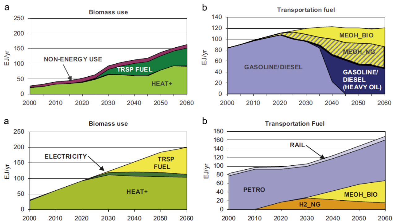
Figure A.2. Time evolution of biomass usage and break out of transportation fuels predicted by the two models
