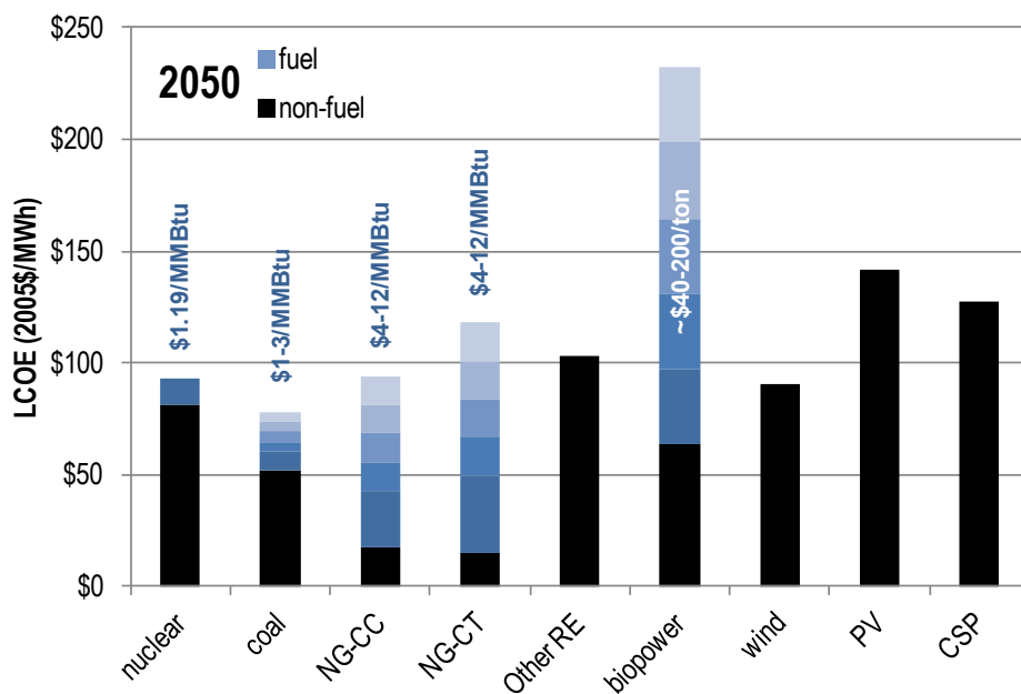
Figure 4.6. LCOE breakdown for electricity in 2050
