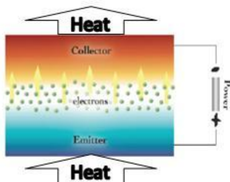
Figure G.8-1. Schematic of Thermotunneling System
