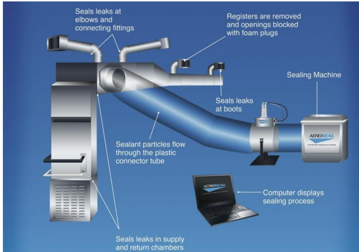
Figure G.17-1. Aerosol Duct Sealing System
