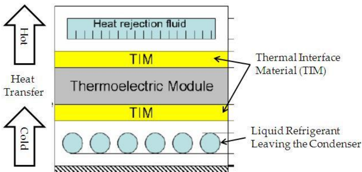
Figure G.7-2. TE Subcooler Cross-Section
