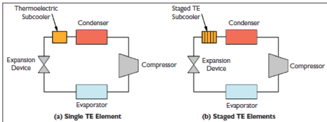
Figure G.7-4. Vapor-Compression Systems with TE Subcoolers
