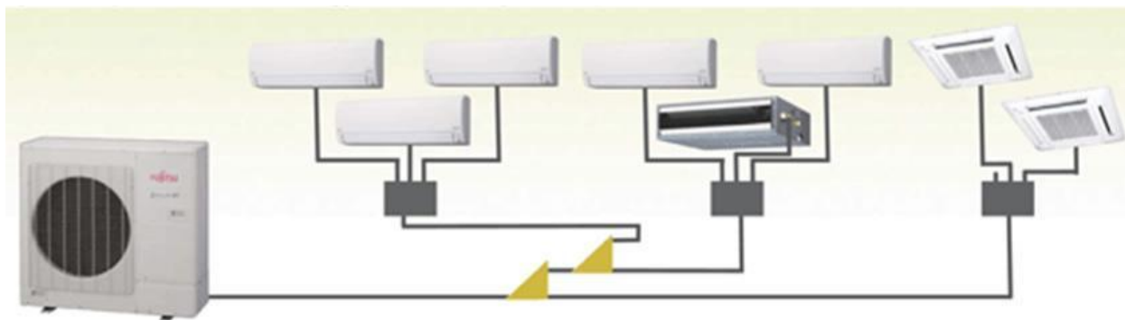
Figure G.10-1. Example Ductless Multi-Split System
