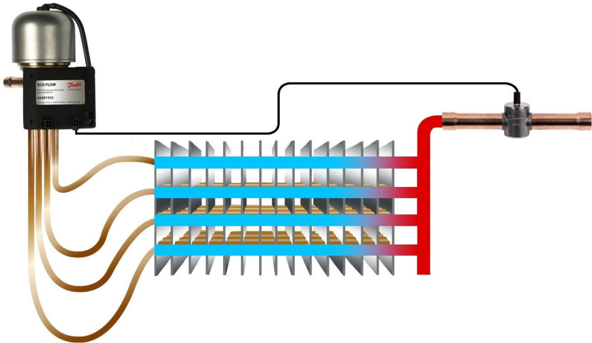
Figure G.3-1. Evaporator with Optimized Refrigerant Distribution
