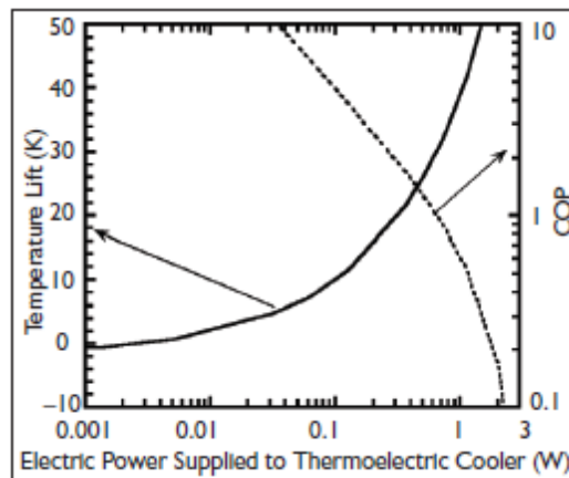
Figure G.7-1. Temperature Lift and COP of a Sample TE Device vs. Applied Power
