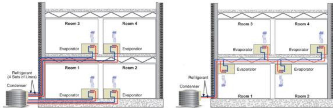
Figure G.10-2. Example Ductless Multi-Split Configurations: 2-sets of lines to each indoor unit, and 2-common lines
