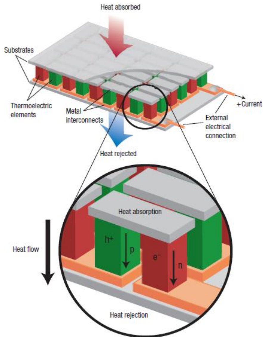
Figure G.6-1. Thermoelectric Cooling Module
