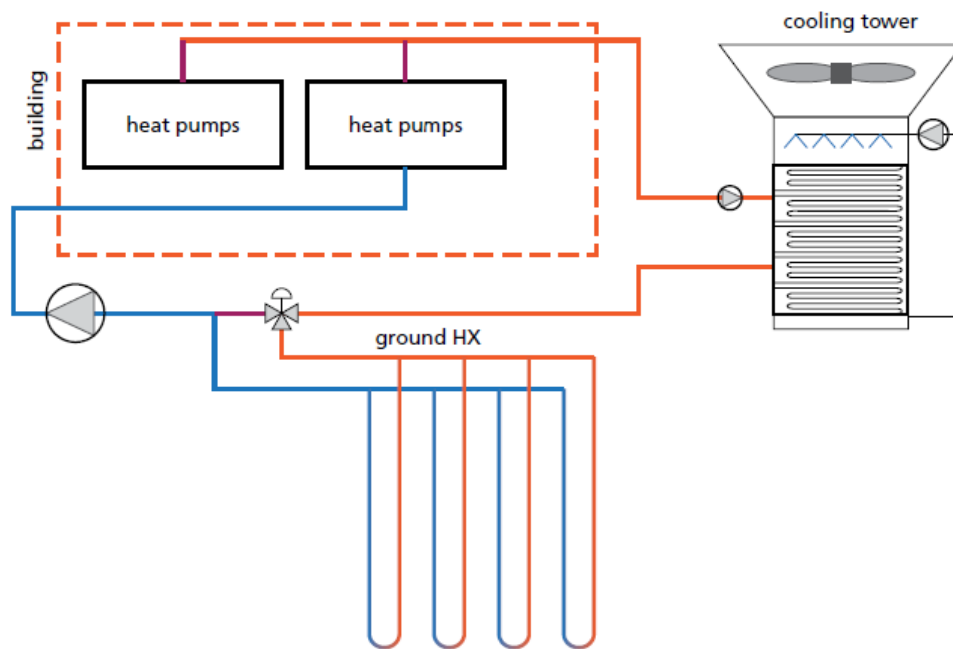
Figure G.14-1. Sample Hybrid Geothermal Heat Pump with Cooling Tower 34
