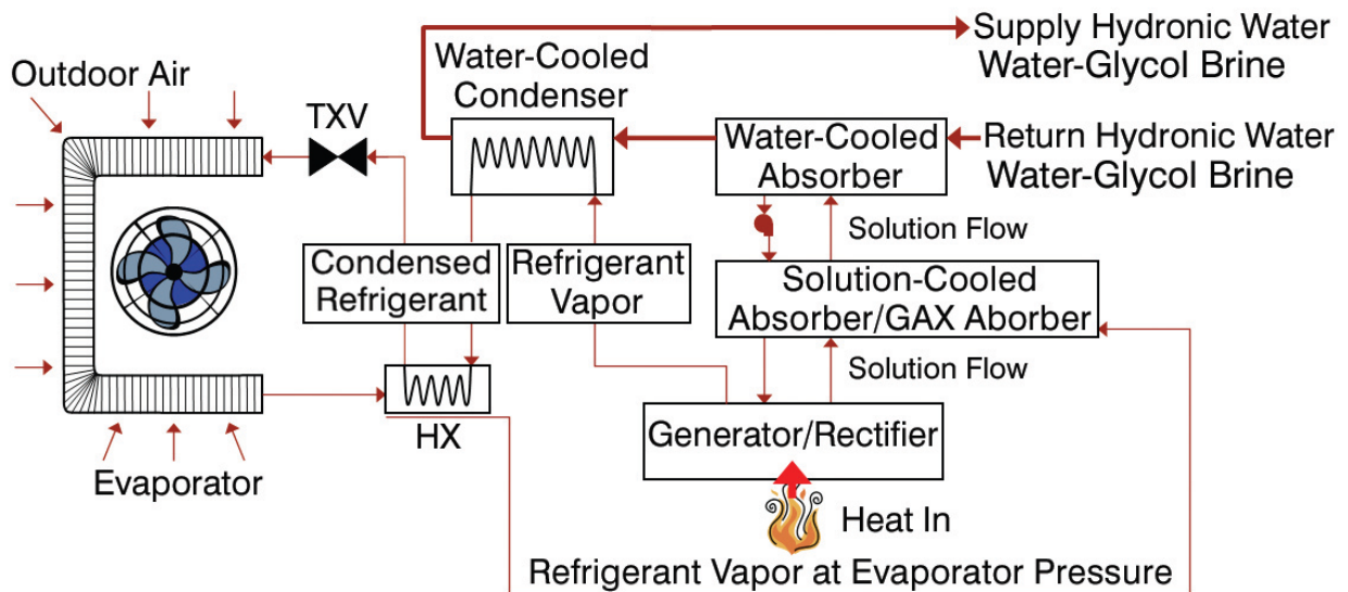
Figure G.5-1. Schematic of a Heating-Only GAHP System employing Generator-Absorber Heat Exchange (GAX)
