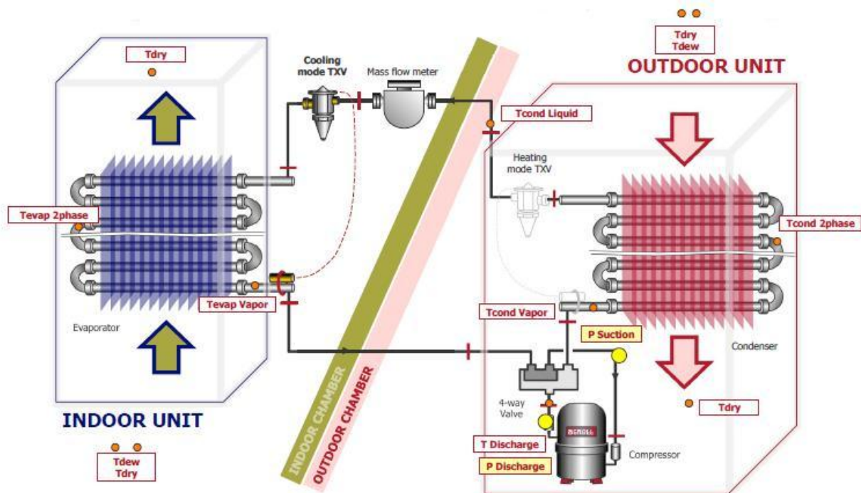
Figure G.21-1. Example Split-System with Embedded Sensors
