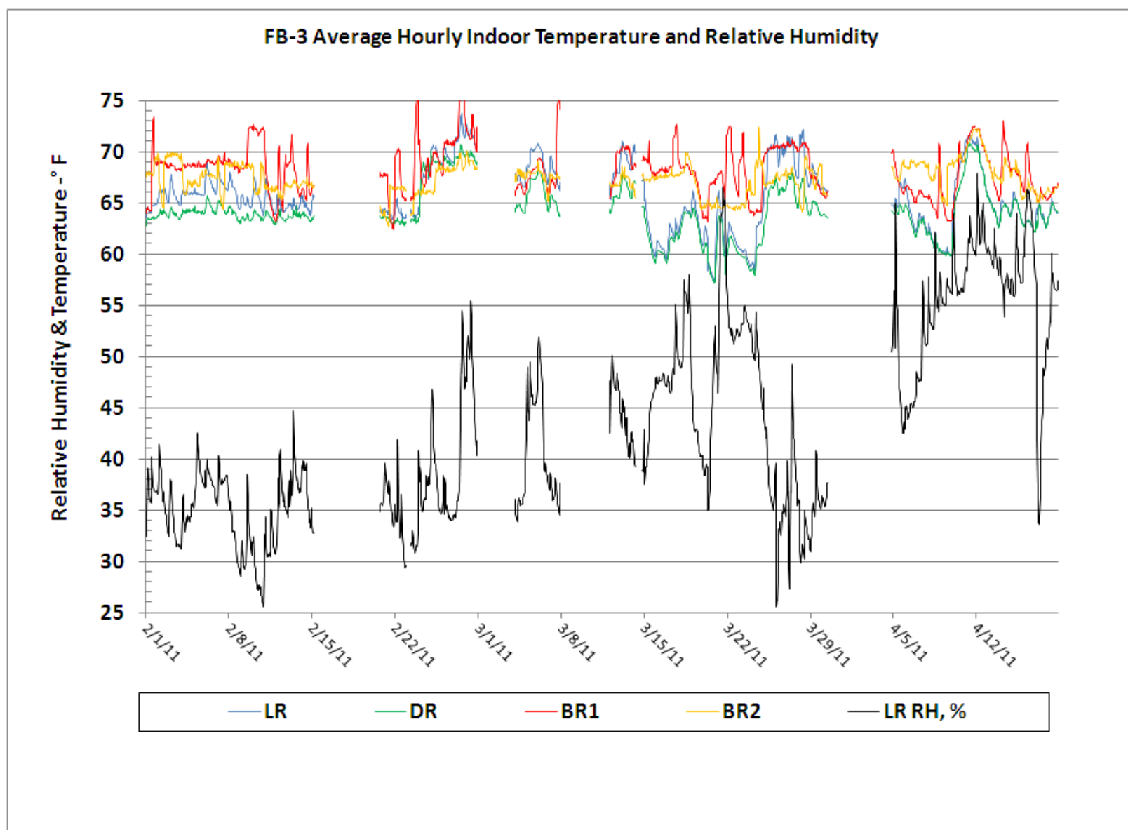
Figure 73. FB-3 Average Hourly Temperature – February 2011 to April 2011.
