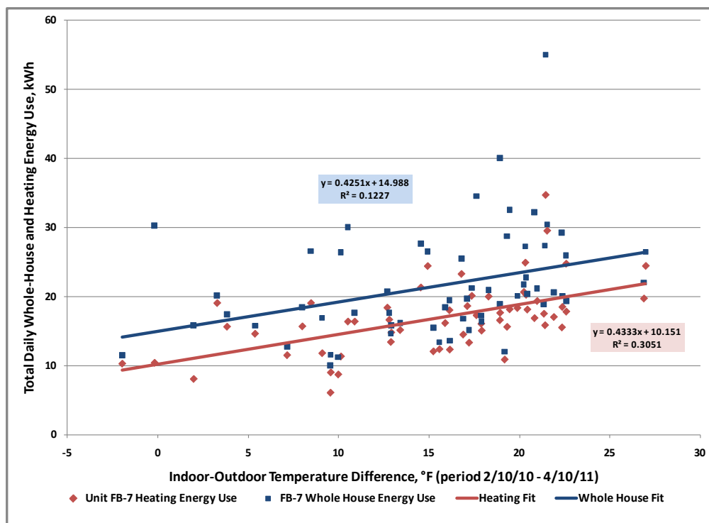
Figure 16. FB-7 Whole house and heating electric usage.
