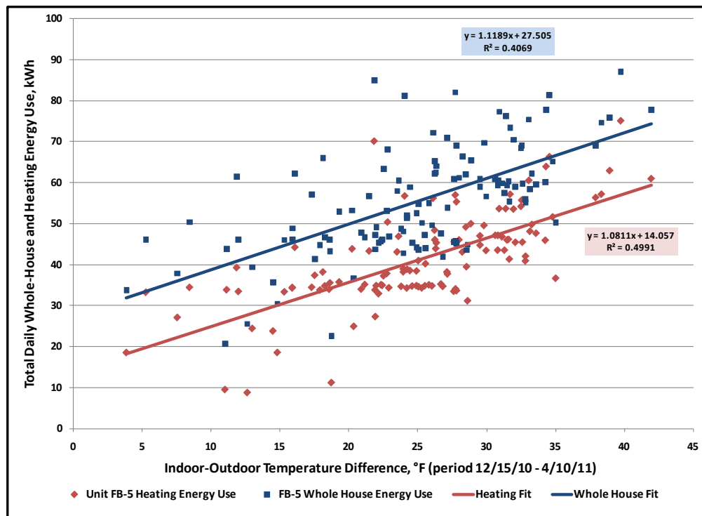
Figure 14. FB-5 Whole house and heating electric usage.
