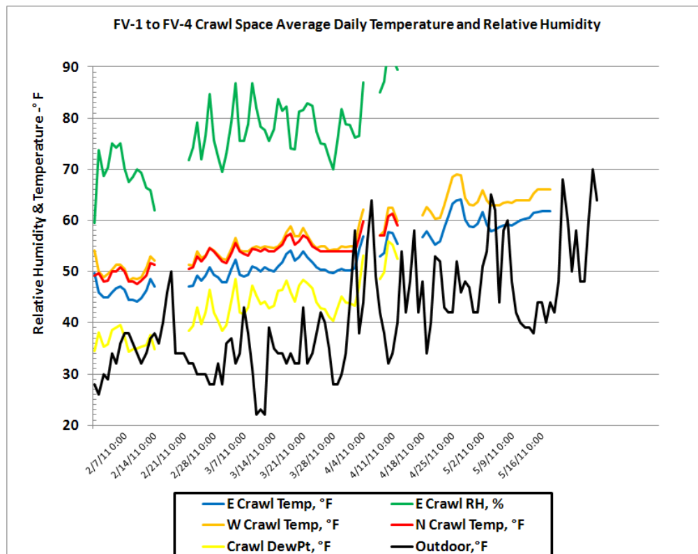
Figure 44. Crawlspace temperature and relative humidity FV-1 through FV-4.
