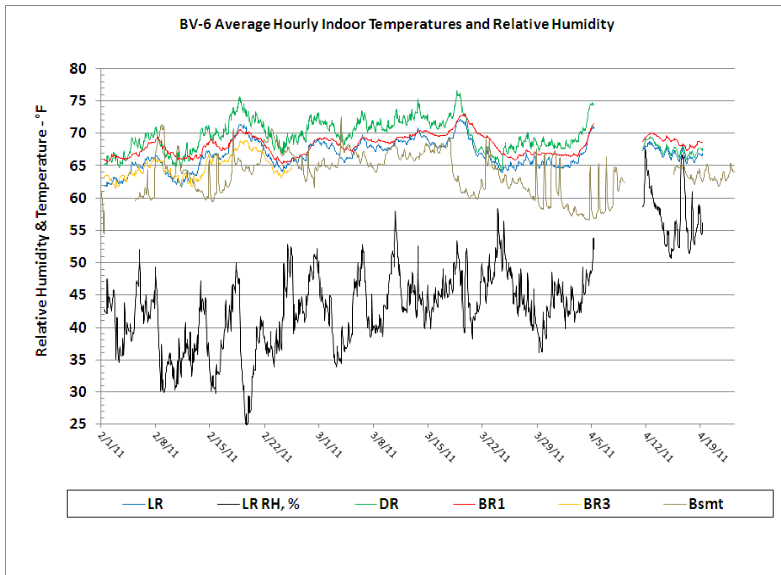
Figure 87. BV-6 Average Hourly Temperature – February 2011 to April 2011.
