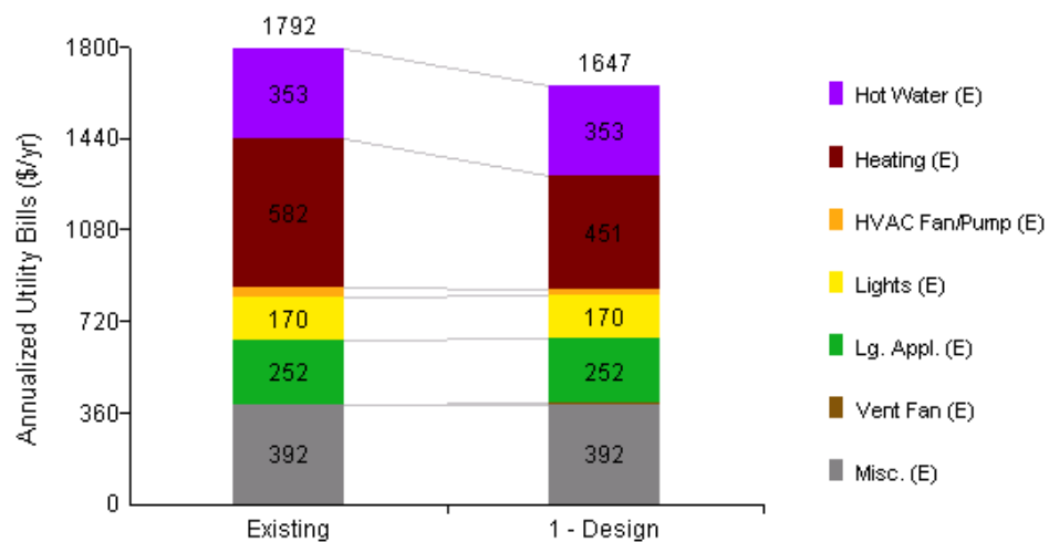
Figure 53. Modeled energy use FB-2.
