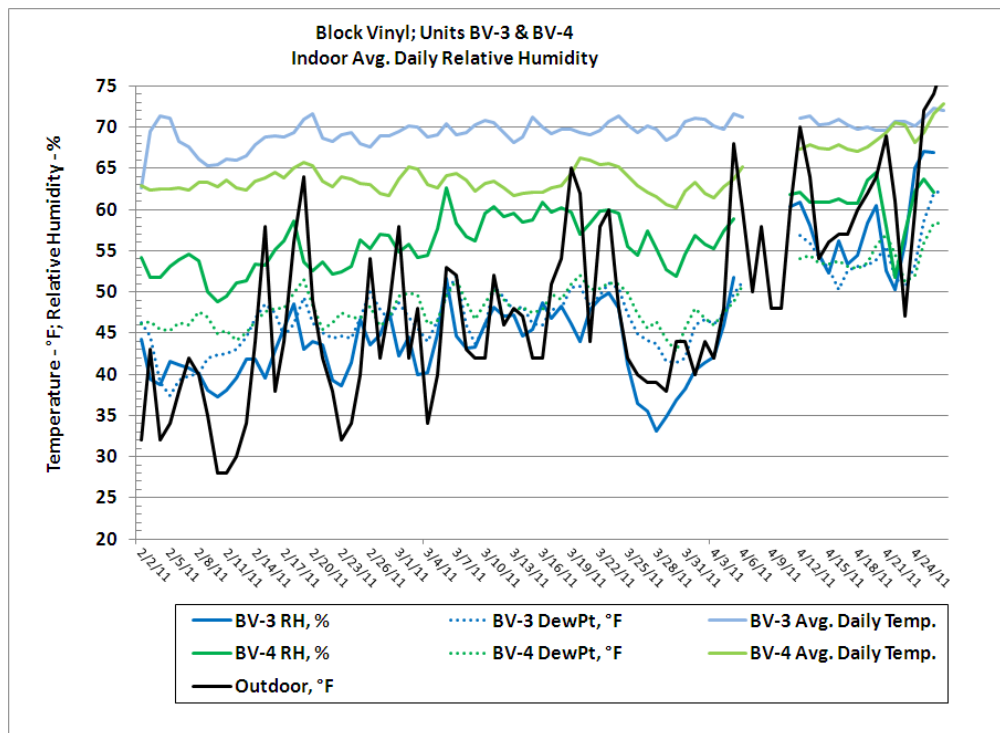
Figure 31. Indoor relative humidity BV-3 and BV-4.
