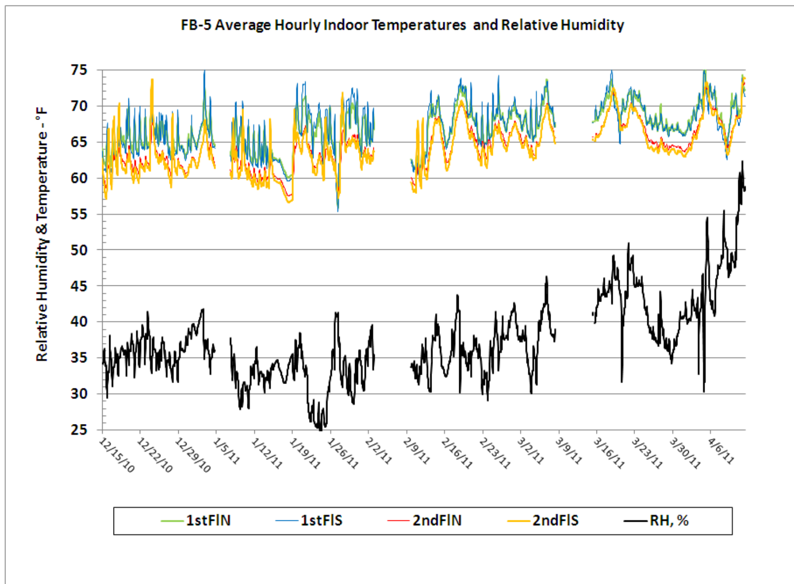
Figure 75. FB-5 Average Hourly Temperature – December 2010 to April 2011.
