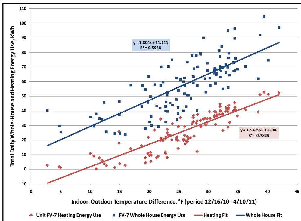
Figure 21. FV-7 Whole house and heating electric usage.
