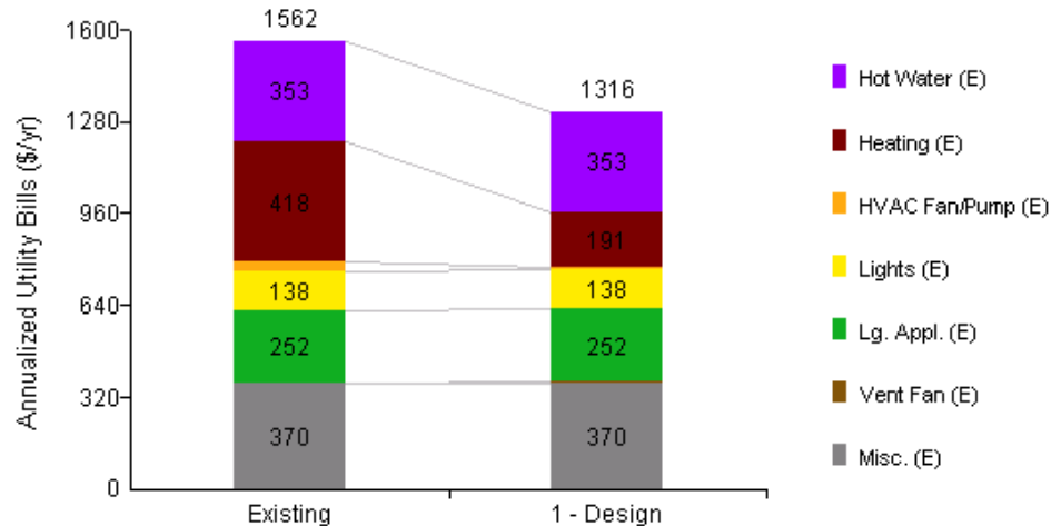
Figure 55. Modeled energy use FV-3.
