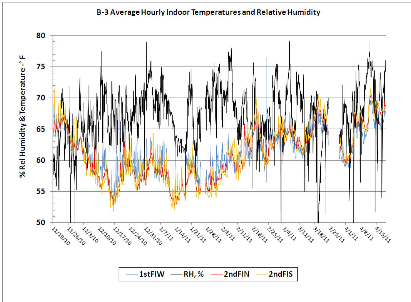
Figure 61. B-3 Average Hourly Temperature – November 2010 through April 2011.
