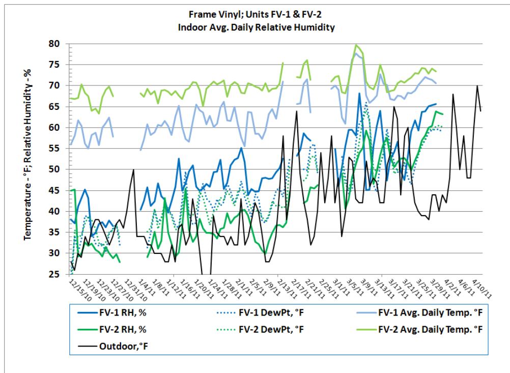
Figure 37. Indoor relative humidity FV-1 and FV-2.
