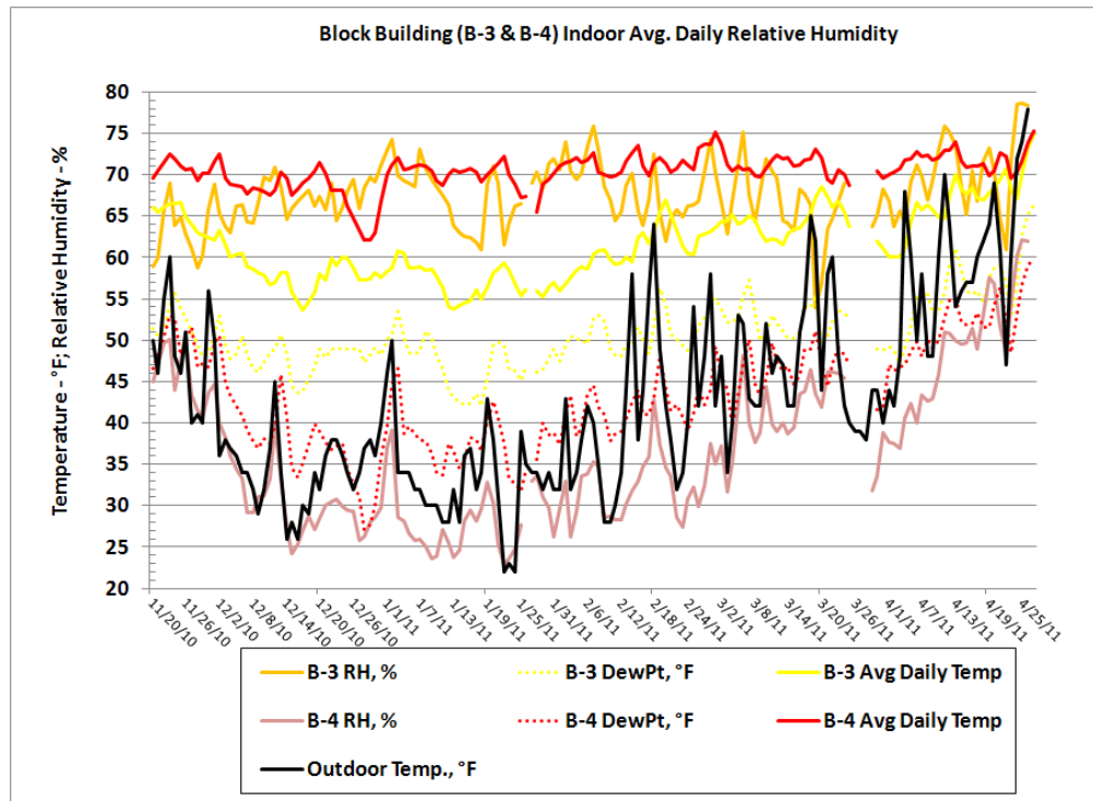
Figure 28. Indoor relative humidity B-3 and B-4.
