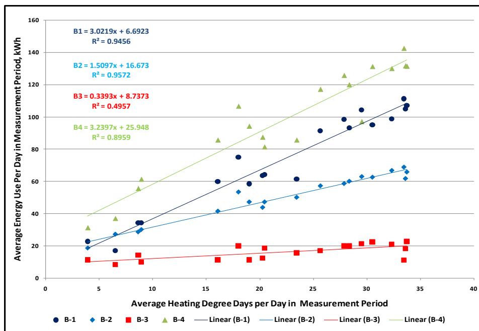
Figure 13. B-1 through B-4 average daily electricity use based on HDDs in the period.
