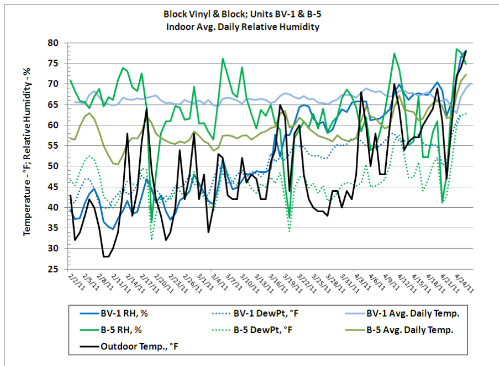
Figure 29. Indoor relative humidity BV-1 and B-5.
