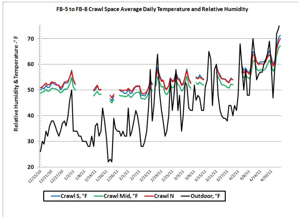
Figure 45. Crawlspace temperature and relative humidity FV-5 through FV-8.
