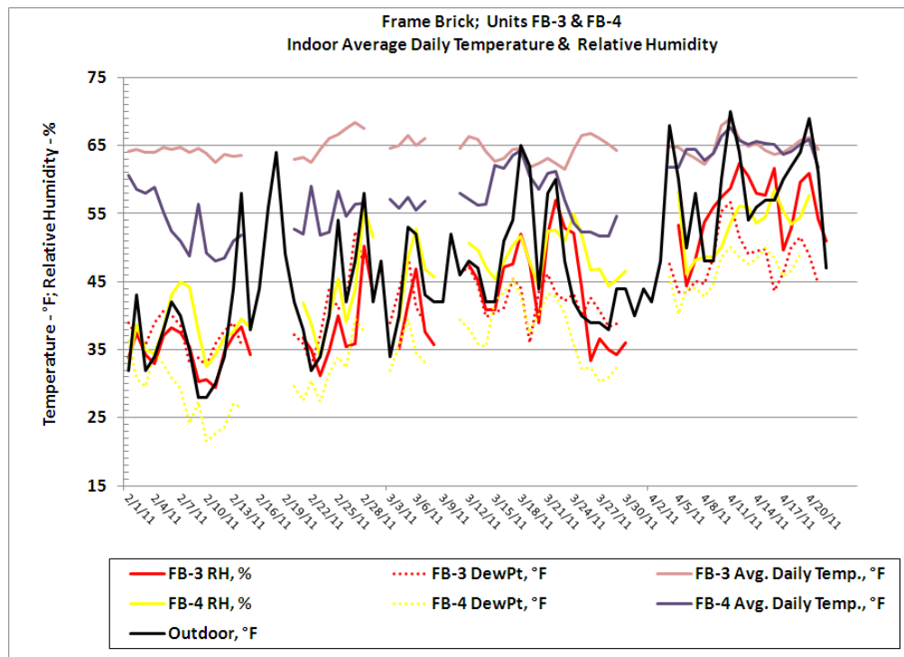
Figure 34. Indoor relative humidity FB-3 and FB-4.
