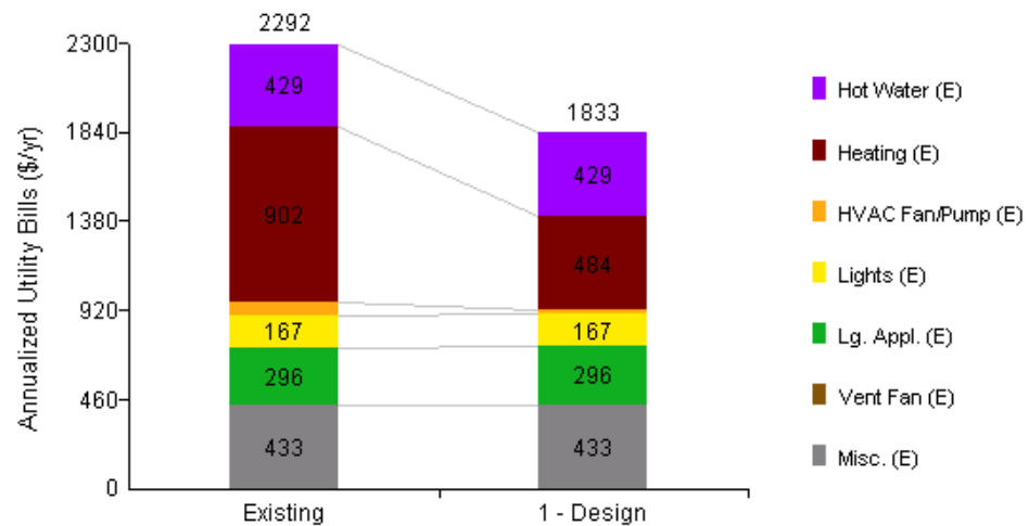
Figure 58. Modeled energy use FV-8.
