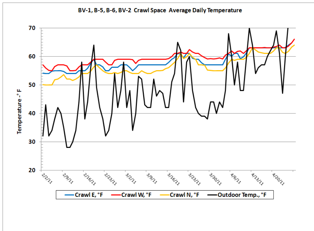
Figure 40. Crawlspace temperature; BV-1, B-5, B-6 and BV-2.
