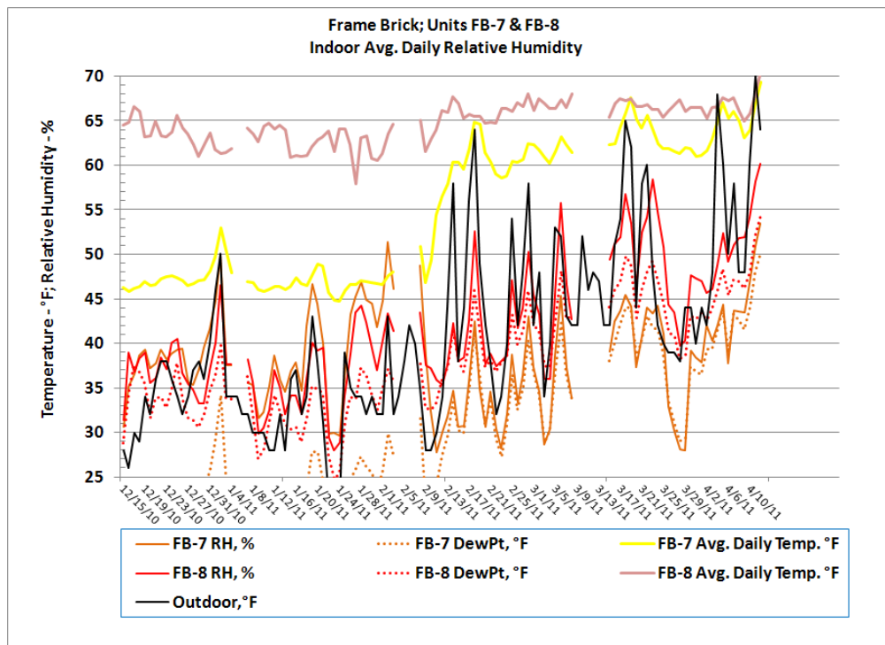
Figure 36. Indoor relative humidity FB-7 and FB-8.
