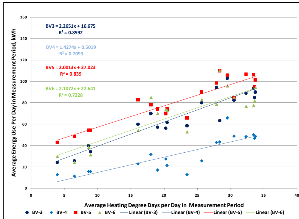
Figure 25. BV-3 through BV-6 average daily usage and HDD for the heating period.
