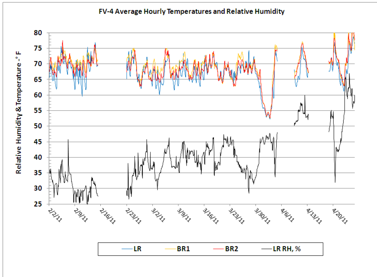
Figure 82. FV-4 Average Hourly Temperature – February 2011 to April 2011.
