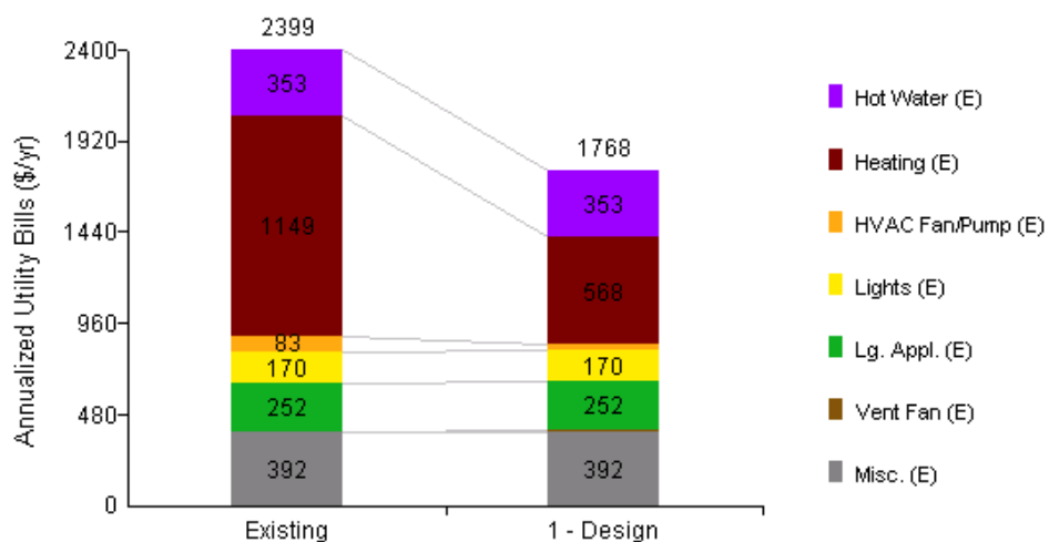
Figure 48. Modeled energy use BV-3.
