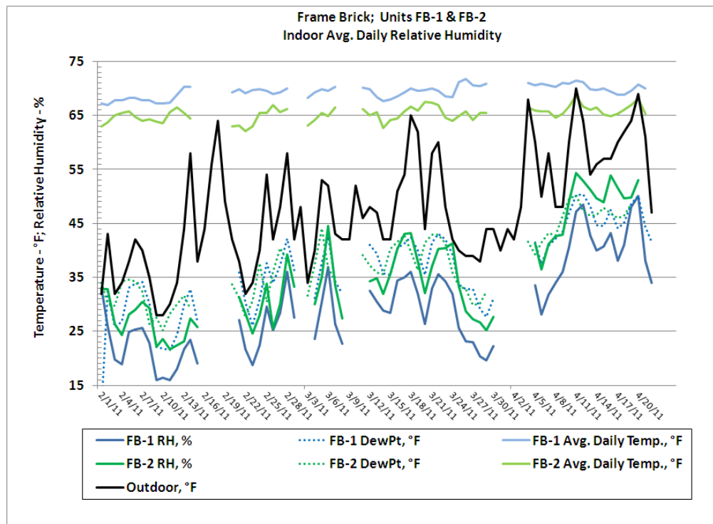
Figure 33. Indoor relative humidity FB-1 and FB-2.
