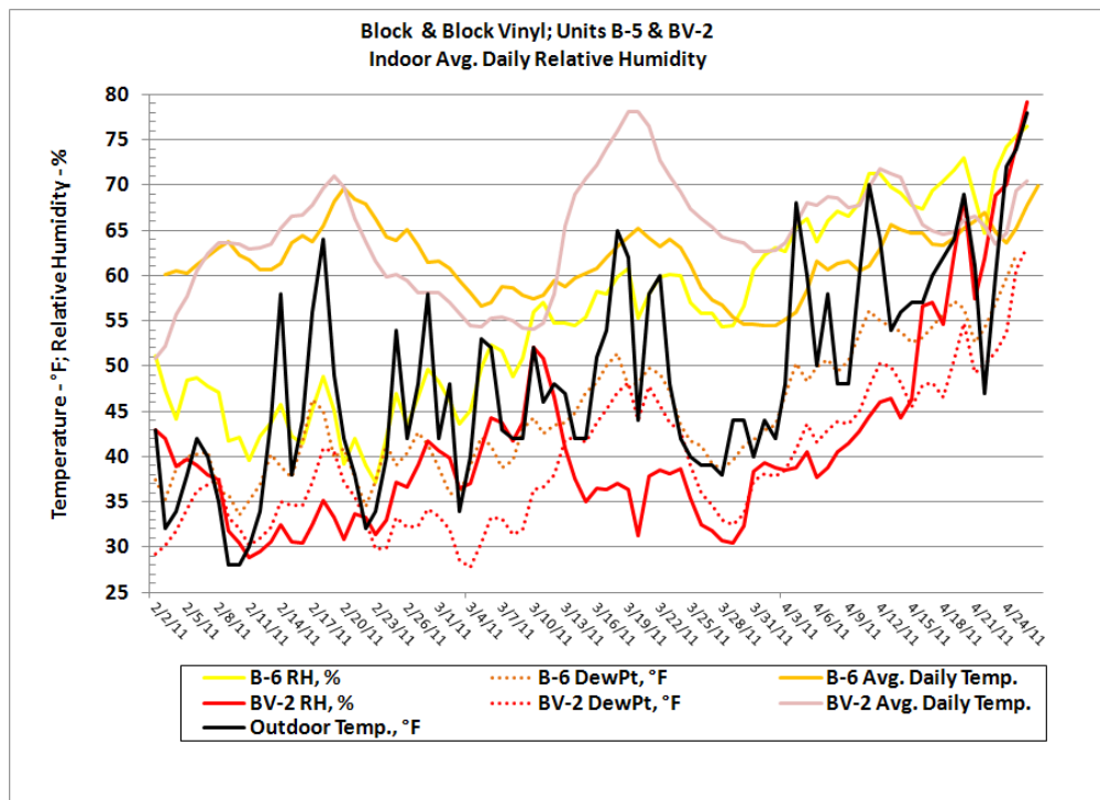
Figure 30. Indoor relative humidity B-6 and BV-2.
