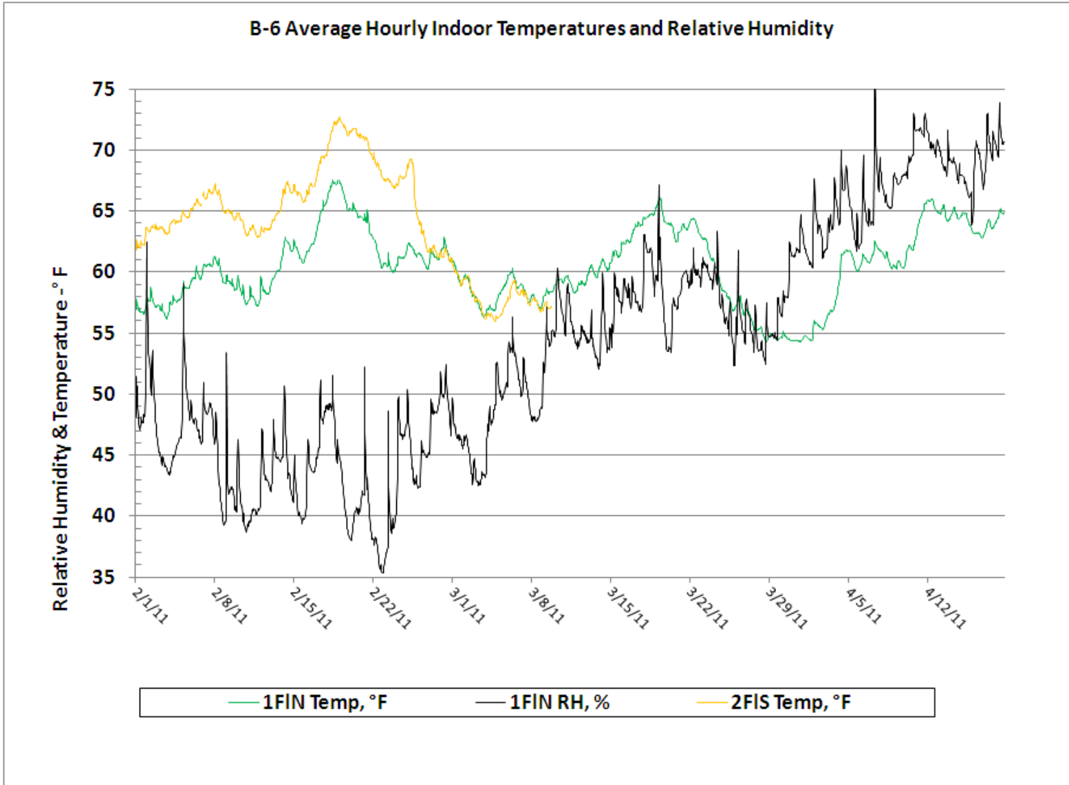
Figure 64. B-6 Average Hourly Temperature – February 2011 through April 2011.
