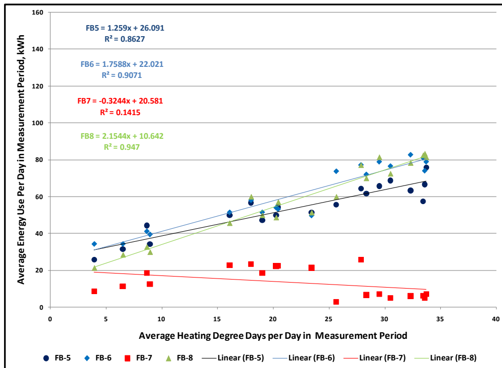
Figure 18. FB-5 through FB-8 average daily usage and HDD during the period.
