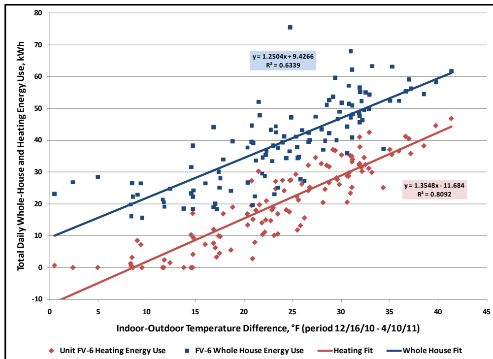
Figure 20. FV-6 Whole house and heating electric usage.
