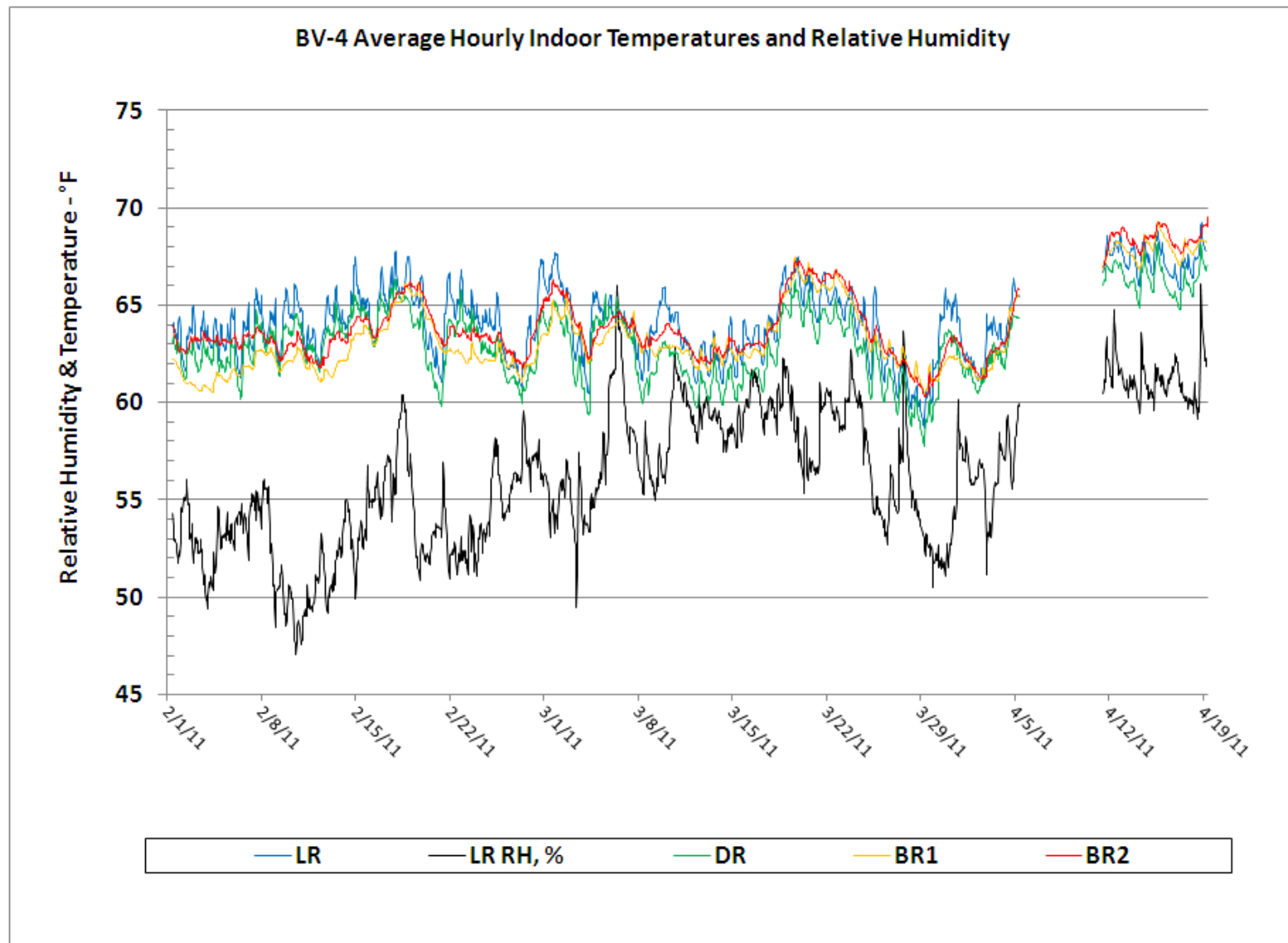
Figure 68. BV-4 Average Hourly Temperature – February 2011 through April 2011.
