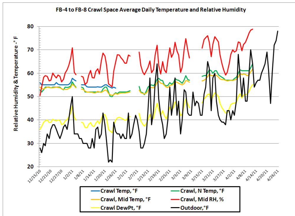
Figure 43. Crawlspace temperature and relative humidity FB-5 through FB-8.
