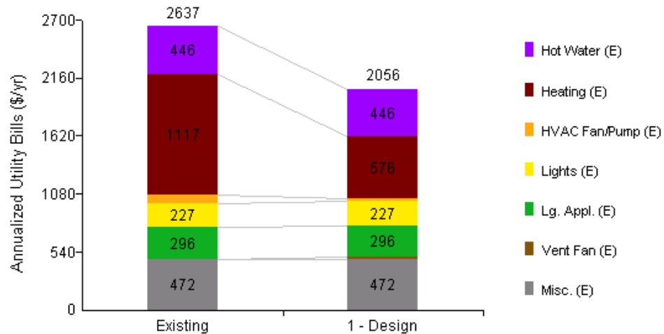
Figure 50. Modeled energy use BV-5.
