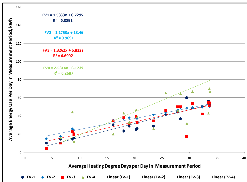
Figure 27. FV-1 through FV-4 average daily usage and HDD for the heating period.
