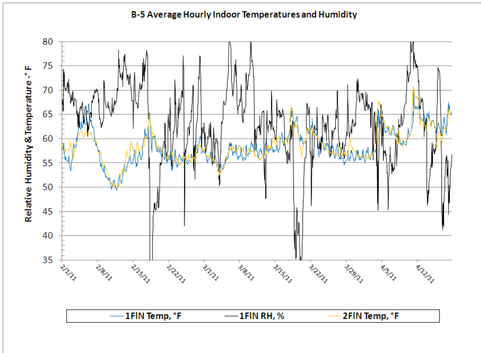
Figure 63. B-5 Average Hourly Temperature – February 2011 through April 2011.
