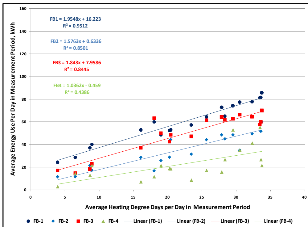
Figure 26. FB-1 through FB-4 average daily usage and HDD during the period.
