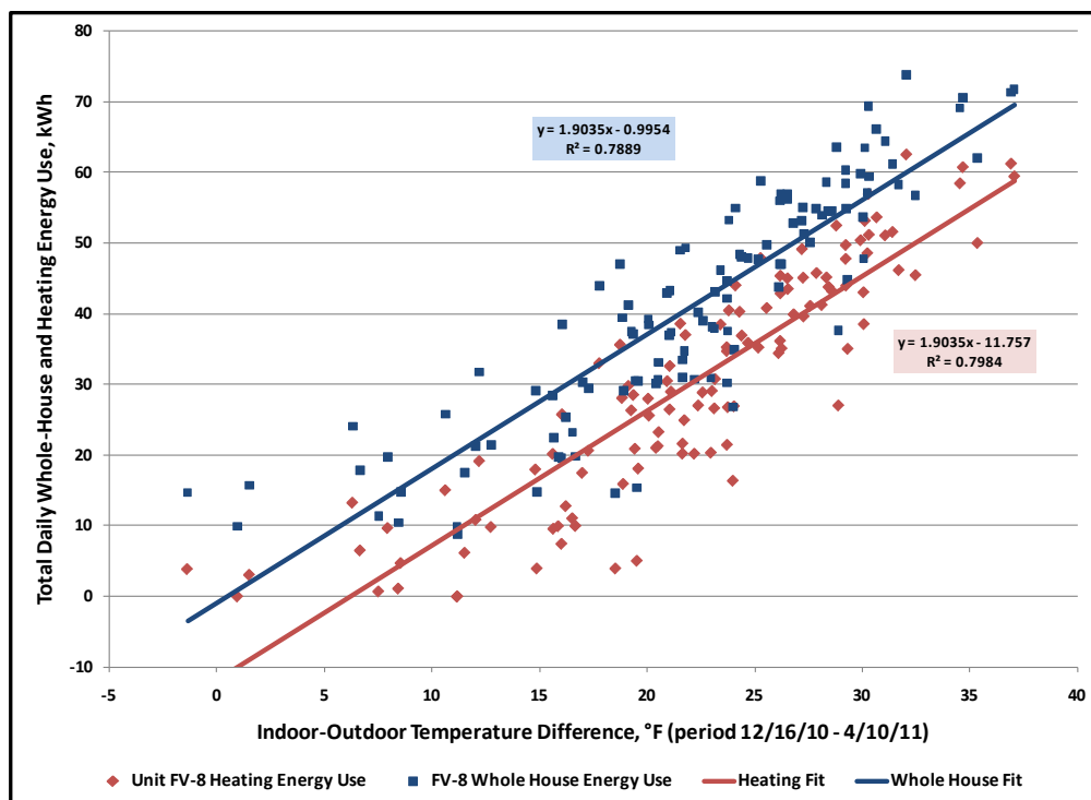
Figure 22. FV-8 Whole house and heating electric usage.
