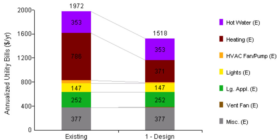
Figure 56. Modeled energy use FV-4.
