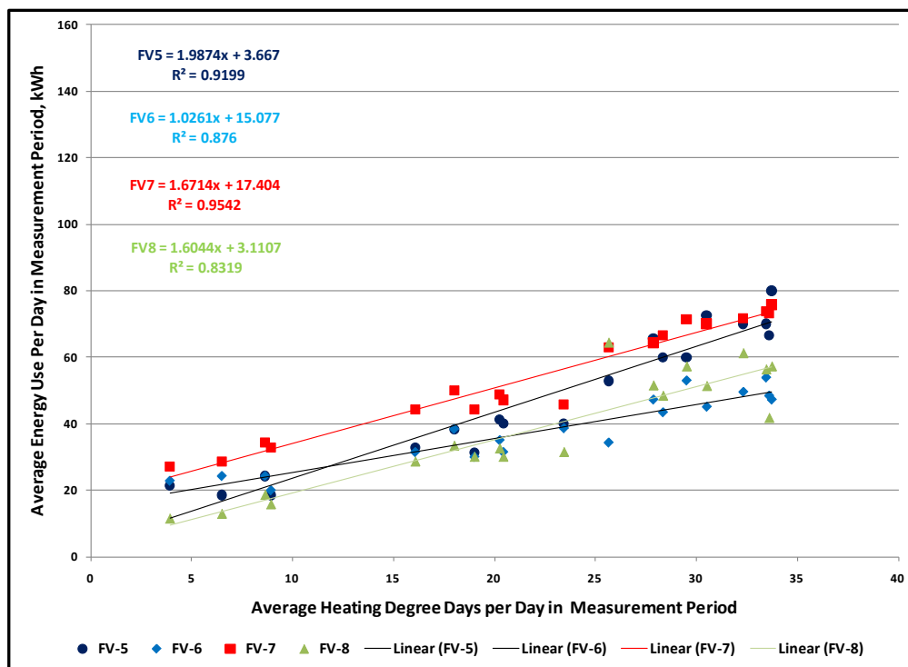
Figure 23. Average daily usage and HDD during the period; FV-5 through FV-8.
