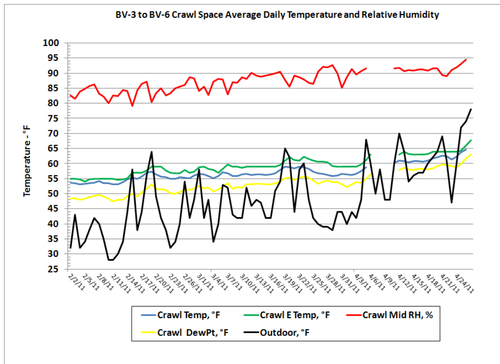
Figure 41. Crawlspace temperature and relative humidity BV-3 through BV-6s.
