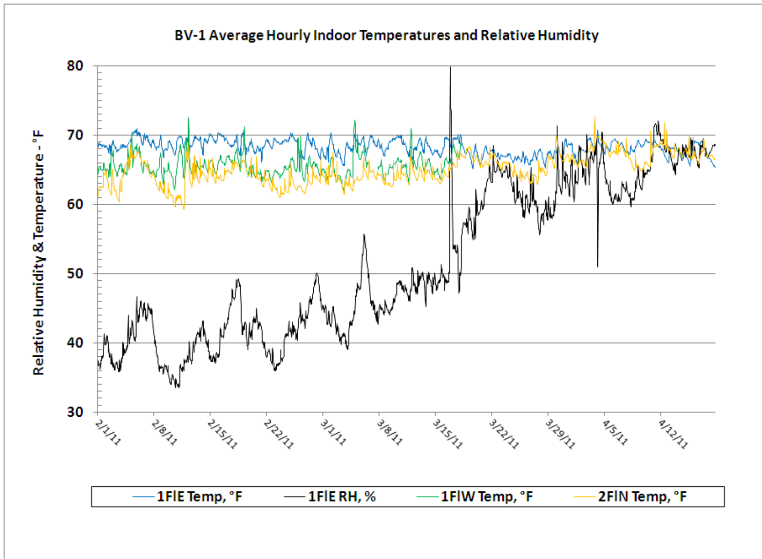
Figure 65. BV-1 Average Hourly Temperature – February 2011 through April 2011.
