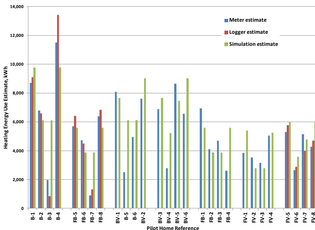
Figure 8. Summary comparison of heating energy use estimates for the heating period November 2010 – March 2011.
