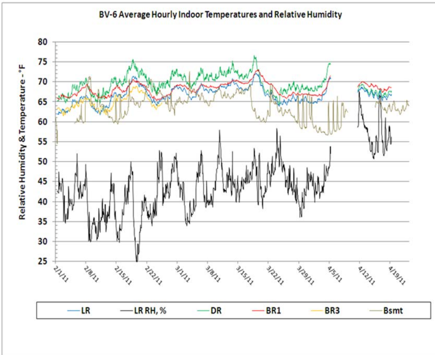
Figure 70. BV-6 Average Hourly Temperature – February 2011 to April 2011.
