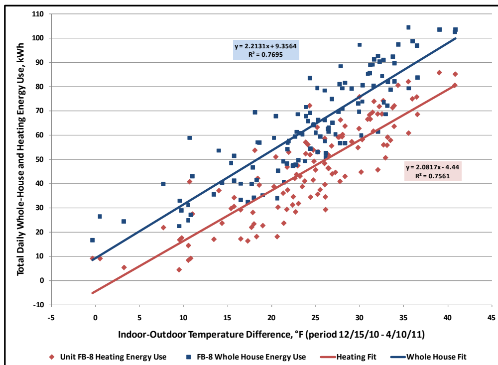
Figure 17. FB-8 Whole house and heating electric usage.
