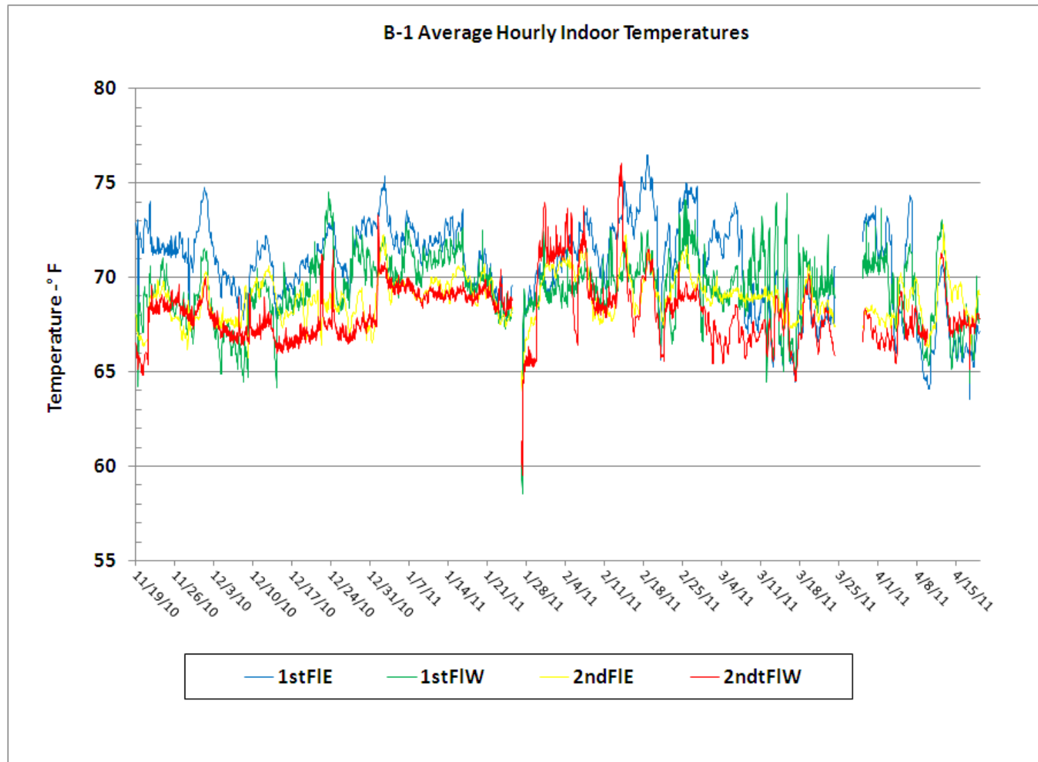
Figure 59. B-1 Average Hourly Indoor Temperature – November 2010 through April 2011.
