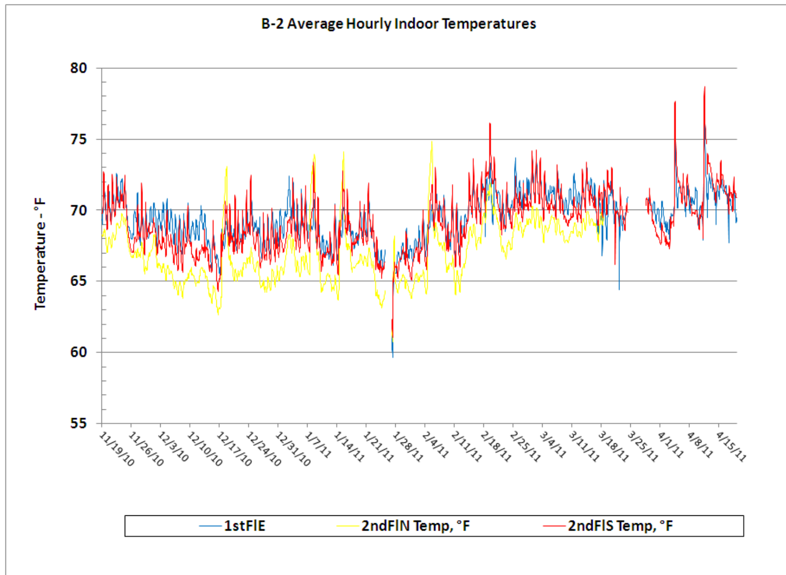
Figure 60. B-2 Average Hourly Temperature – November 2010 through April 2011.
