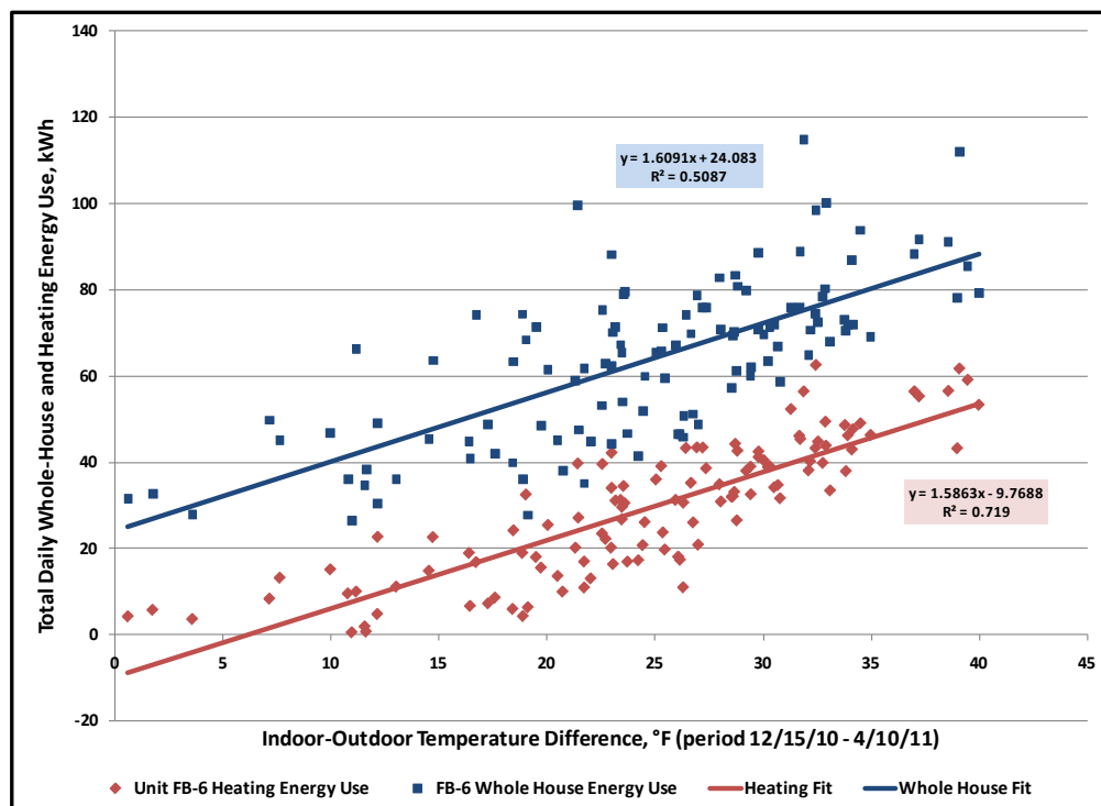
Figure 15. FB-6 Whole house and heating electric usage.
