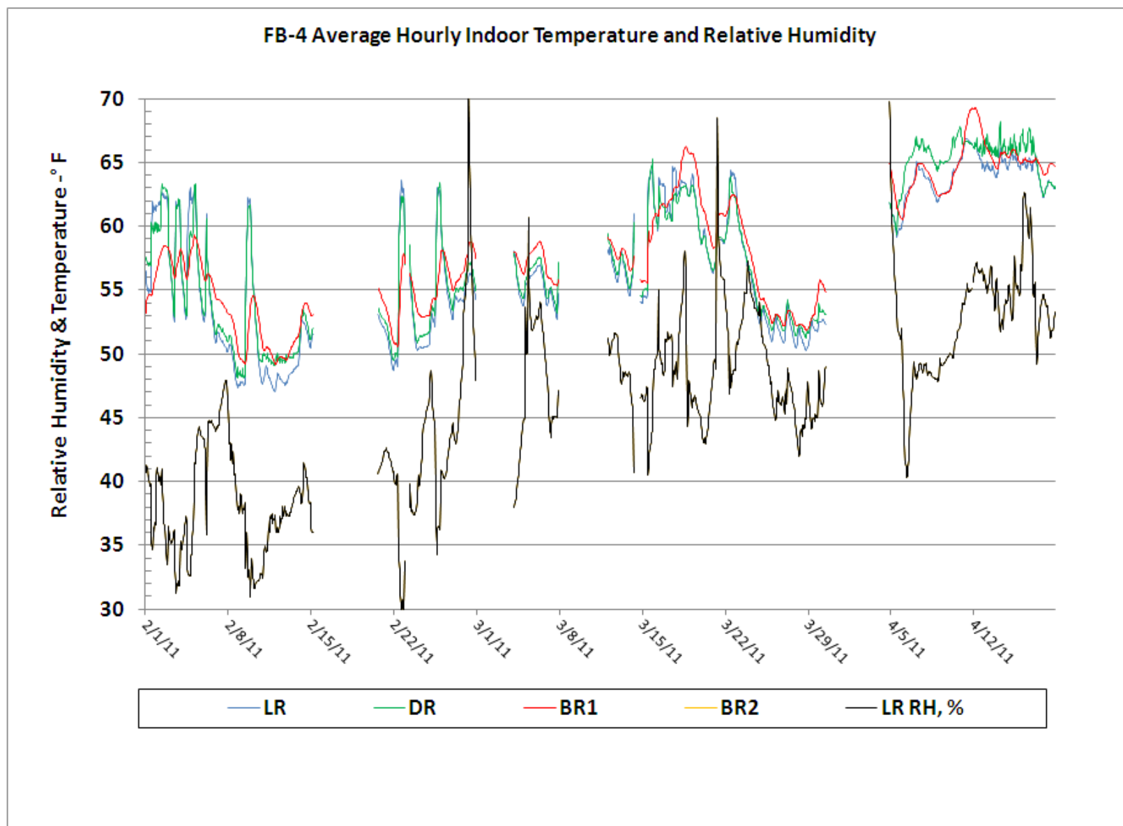
Figure 74. FB-4 Average Hourly Temperature – February 2011 to April 2011.
