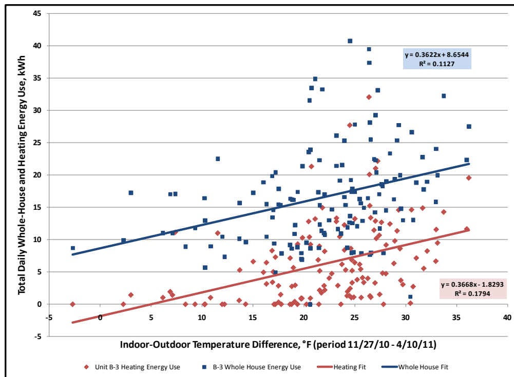
Figure 11. B-3 Whole house and heating electric use analysis.
