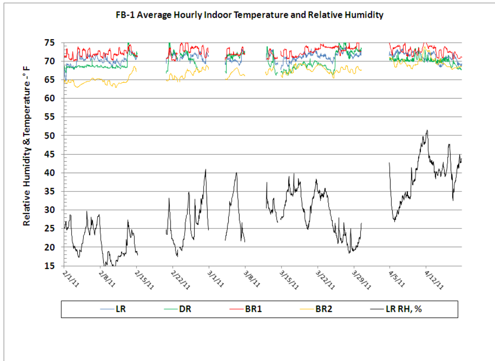
Figure 71. FB-1 Average Hourly Temperature – February 2011 to April 2011.
