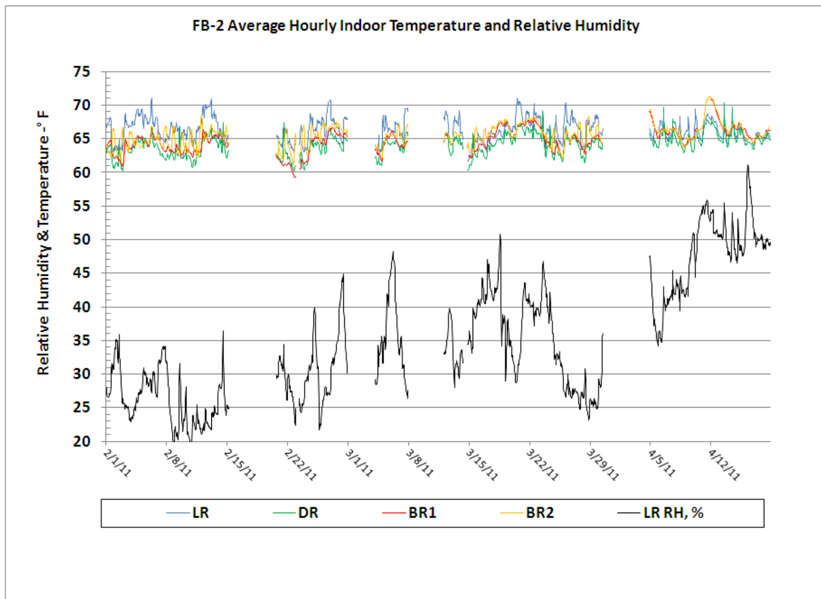
Figure 72. FB-2 Average Hourly Temperature – February 2011 to April 2011.
