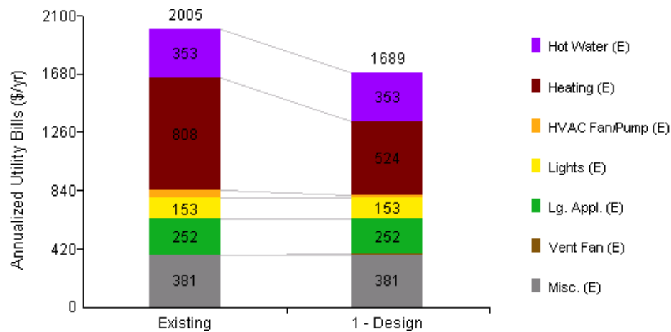
Figure 54. Modeled energy use FV-1.
