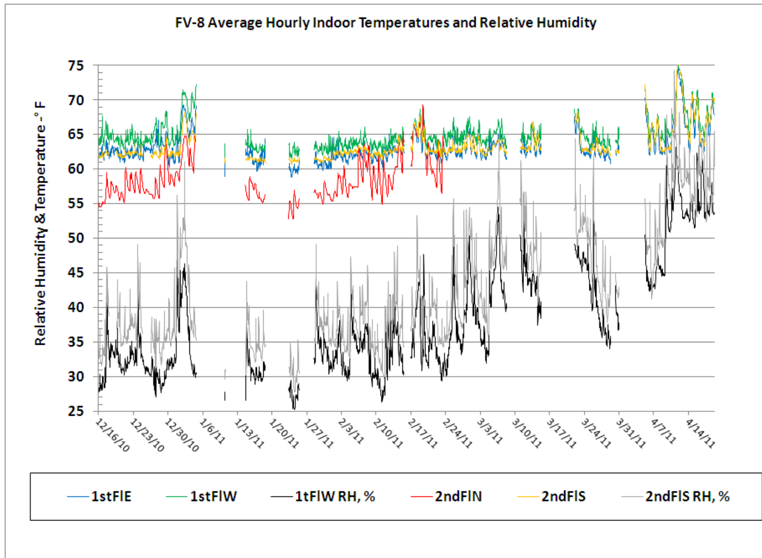
Figure 86. FV-8 Average Hourly Temperature – December 2010 to April 2011.
