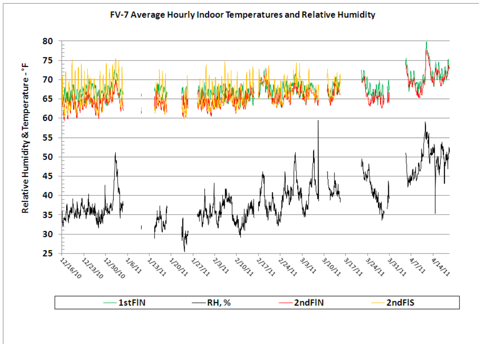
Figure 85. FV-7 Average Hourly Temperature – December 2010 to April 2011.
