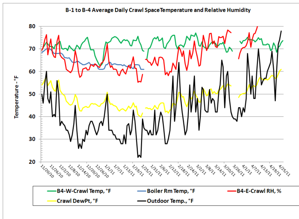
Figure 39. Crawlspace relative humidity; Units B-1 through B-4.
