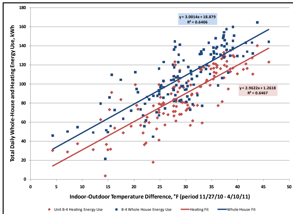
Figure 12. B-4 Whole house and heating electric use analysis.
