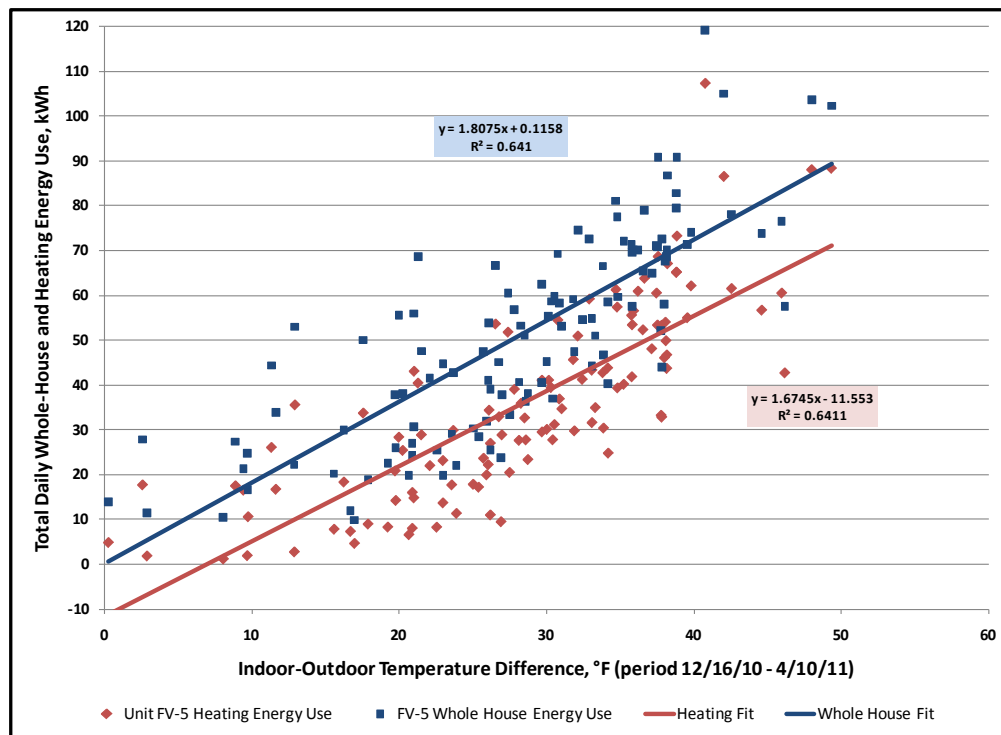
Figure 19. FV-5 Whole house and heating electric usage.
