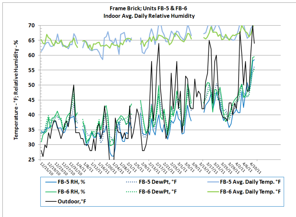
Figure 35. Indoor relative humidity FB-5 and FB-6.
