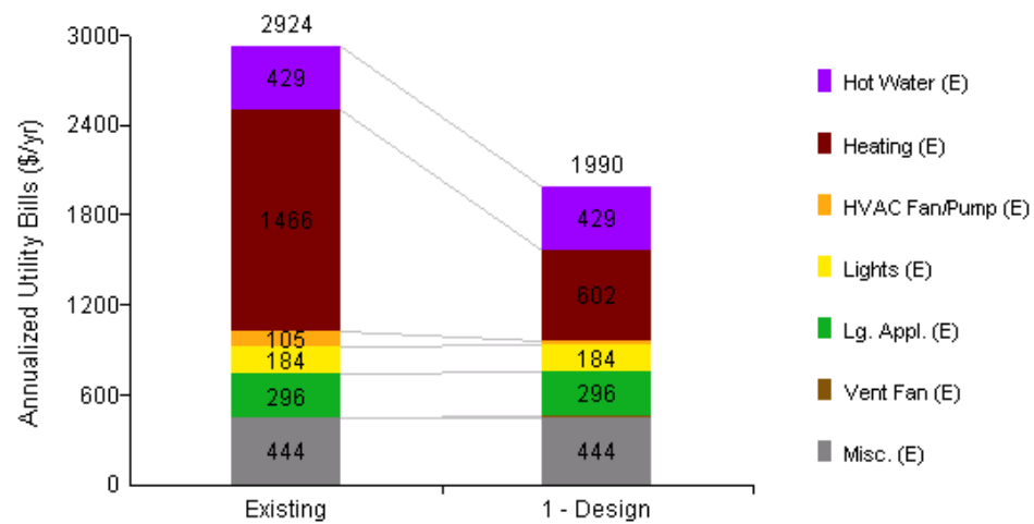
Figure 46. Modeled energy use B-1.
