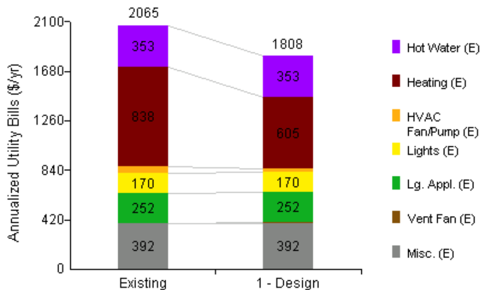
Figure 52. Modeled energy use FB-1.
