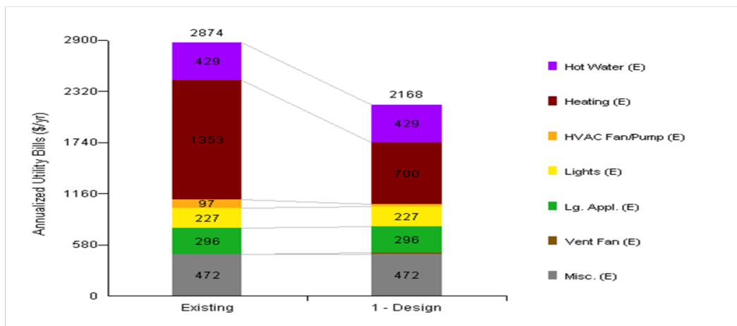
Figure 51. Modeled Energy Use BV-6.
