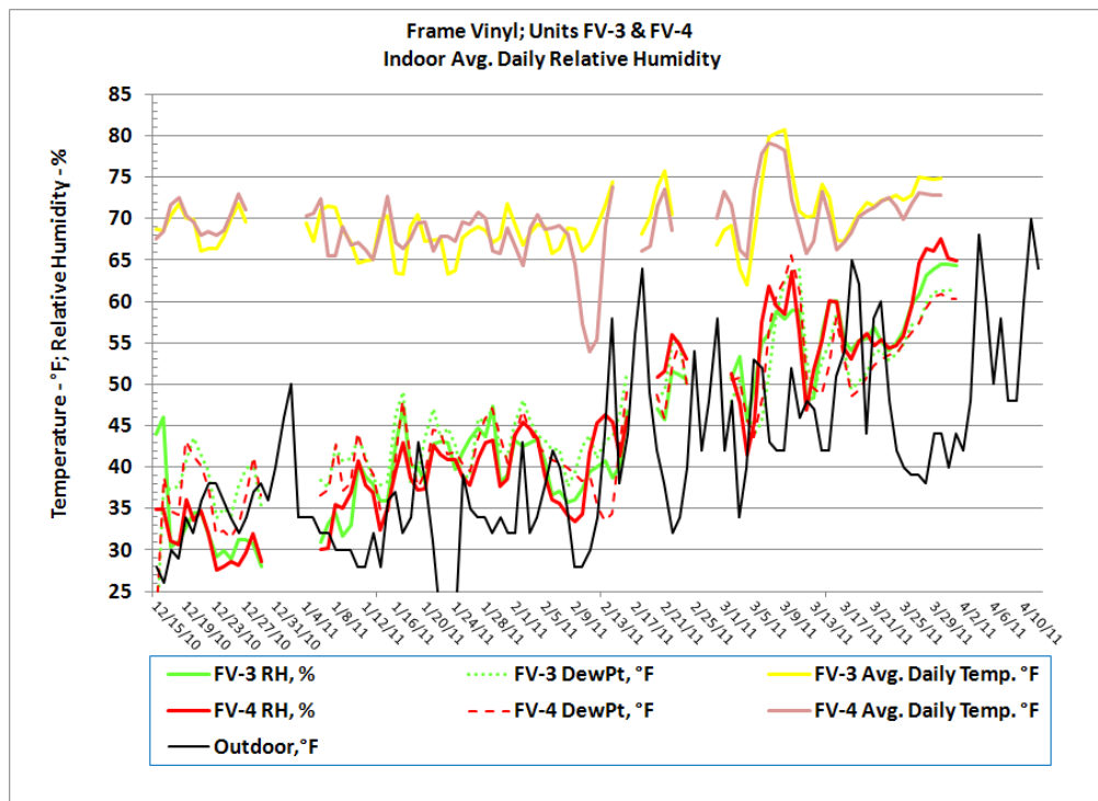
Figure 38. Indoor relative humidity FV-3 and FV-4.
