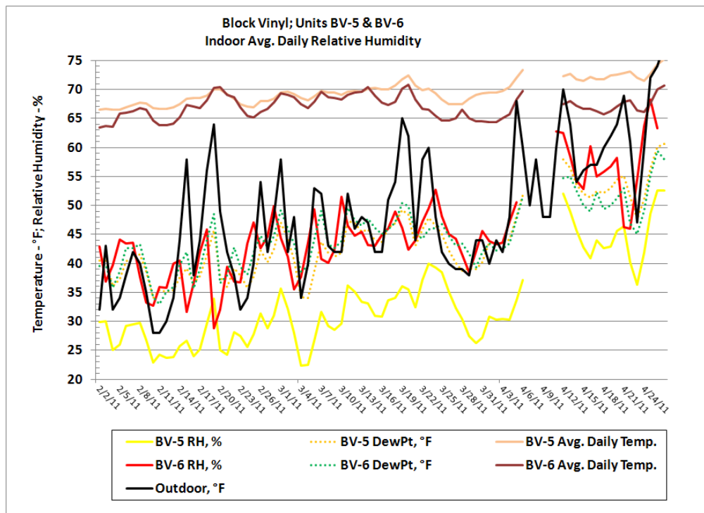
Figure 32. Indoor relative humidity BV-5 and BV-6.
