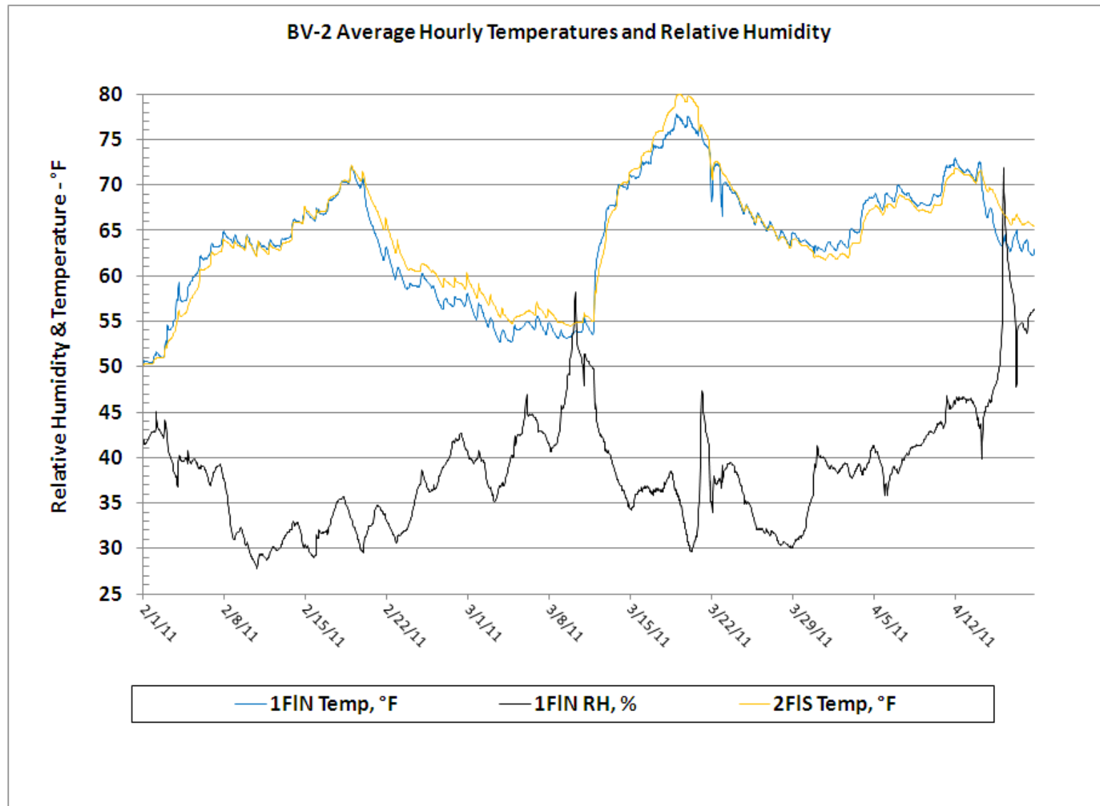
Figure 66. BV-2 Average Hourly Temperature – February 2011 through April 2011.
