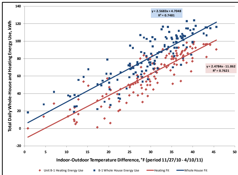
Figure 9. B-1 Whole house and heating electric use analysis.
