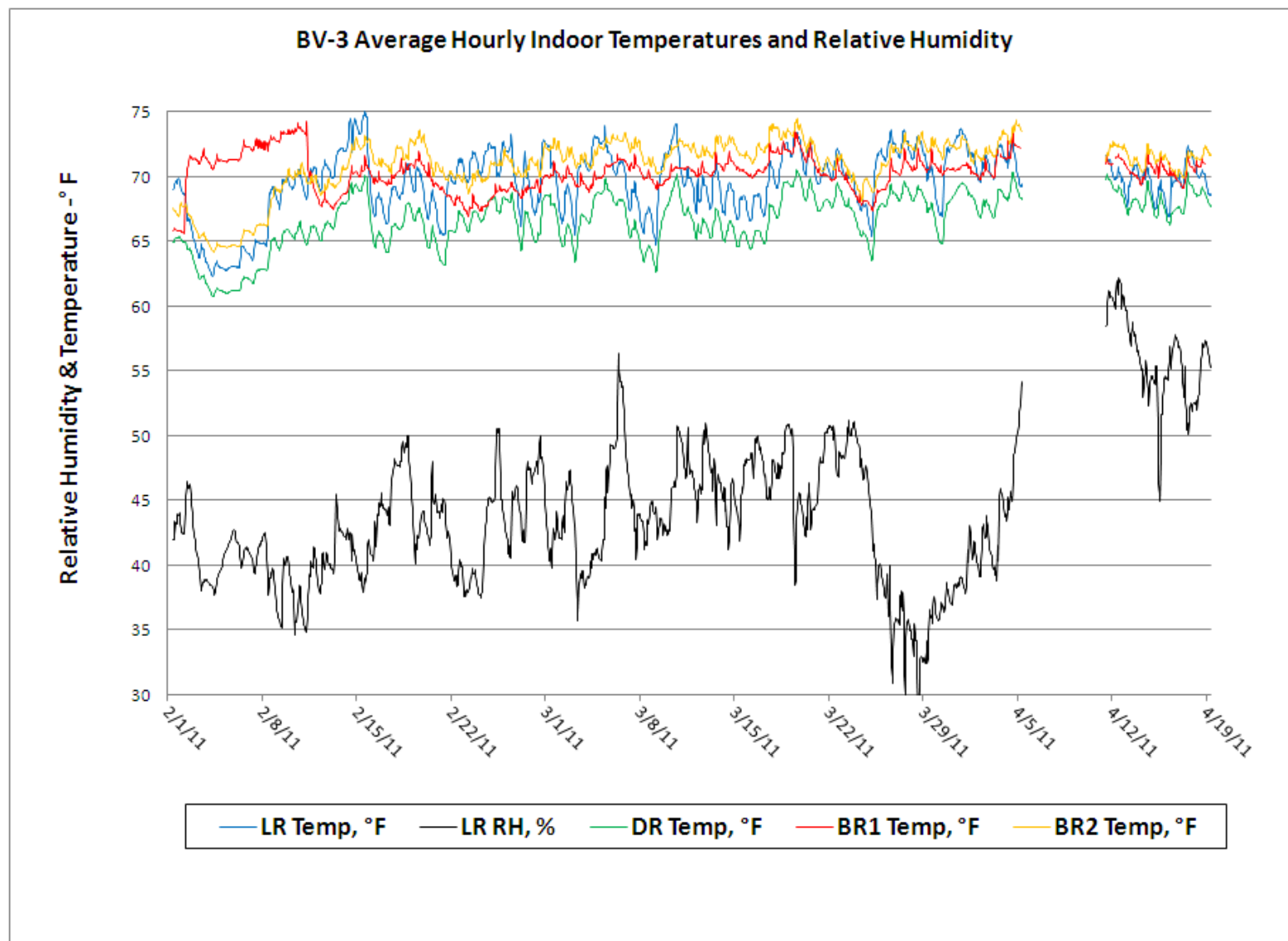
Figure 67. BV-3 Average Hourly Temperature – February 2011 through April 2011.
