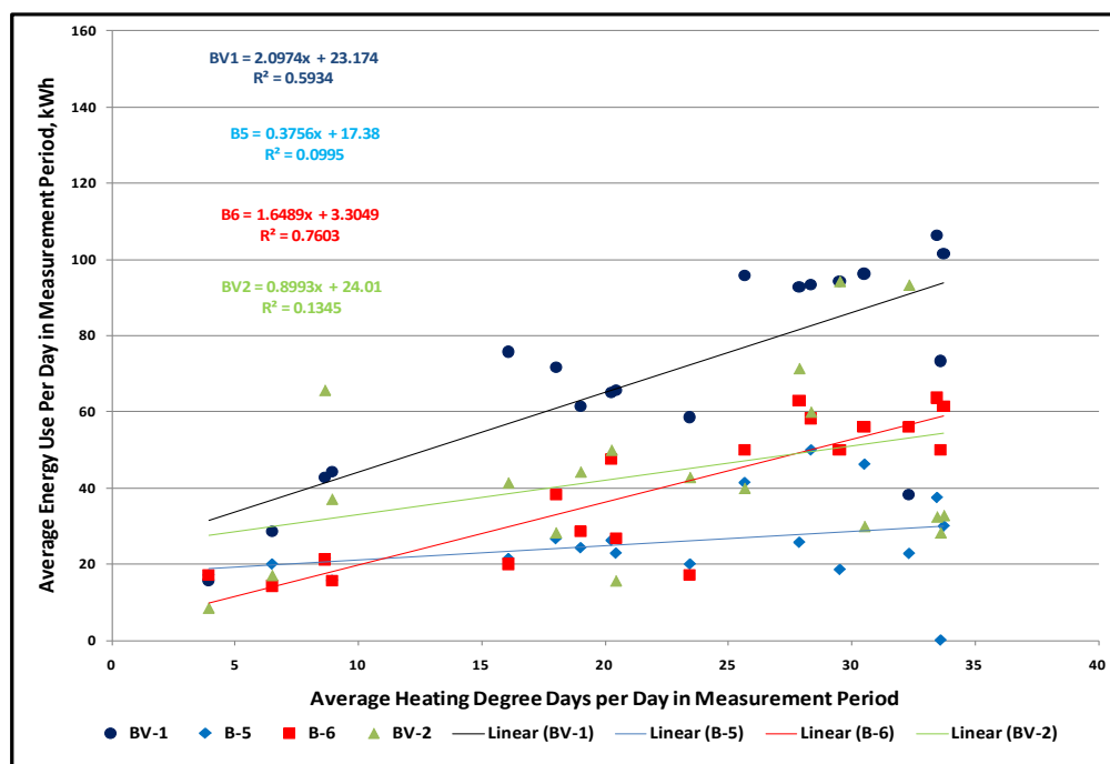
Figure 24. BV-1, B-5, B-6 and BV-2 average daily usage and HDD for the heating period.
