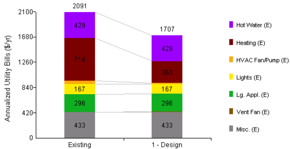
Figure 57. Modeled energy use FV-7.
