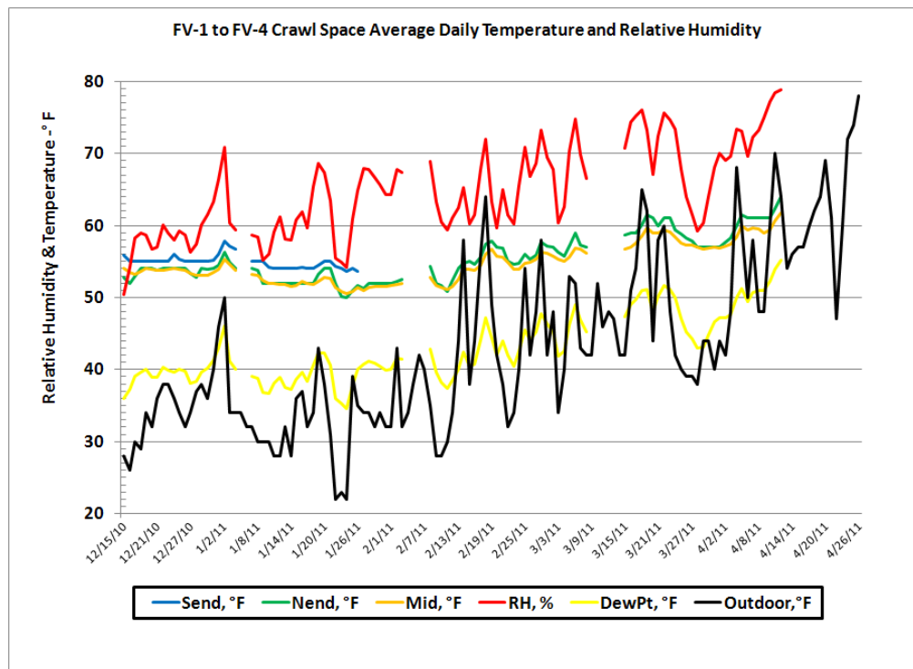
Figure 42. Crawlspace temperature and relative humidity FB-1 through FB-4.
