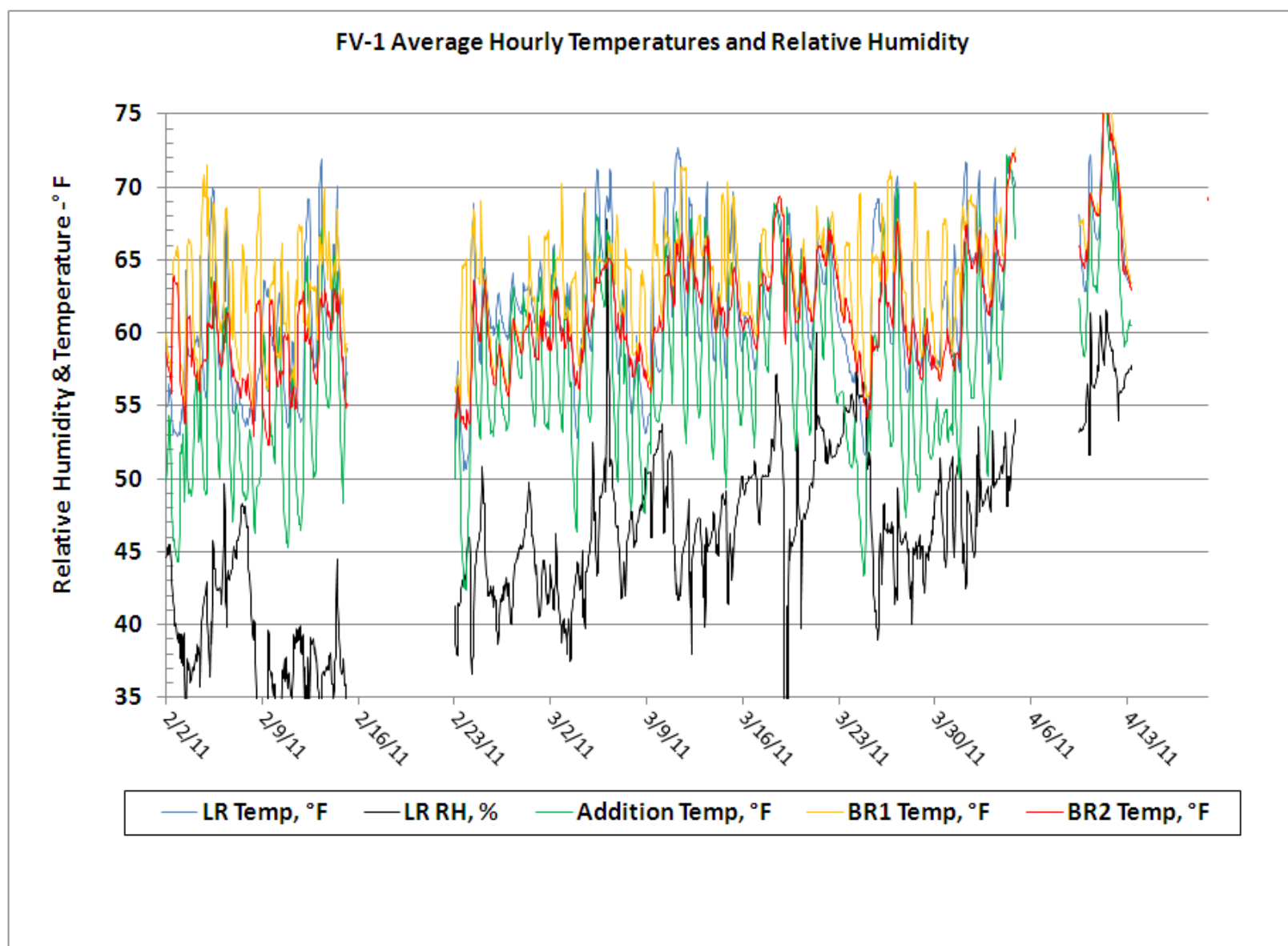
Figure 79. FV-1 Average Hourly Temperature – February 2011 to April 2011.
