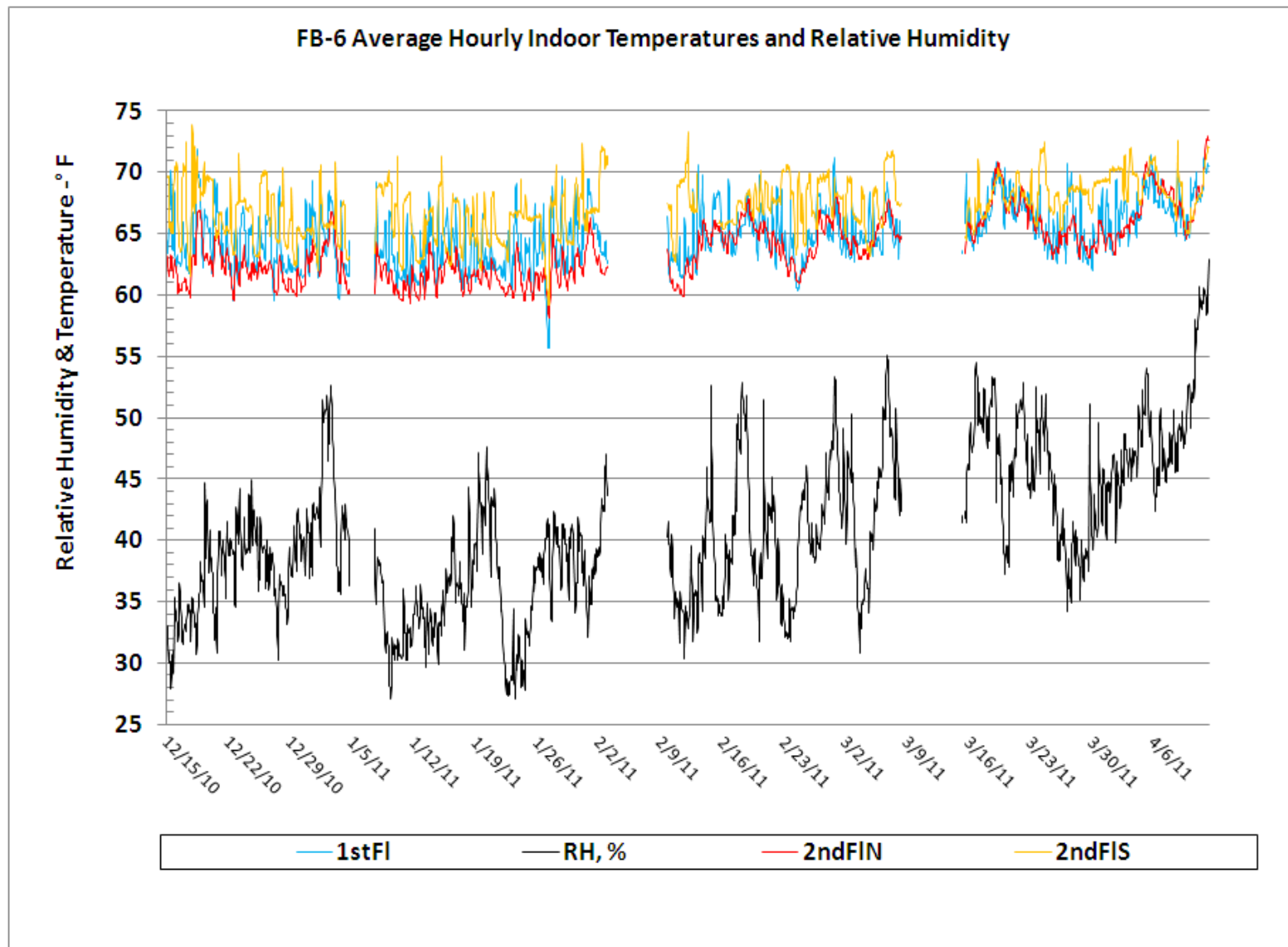
Figure 76. FB-6 Average Hourly Temperature – December 2010 to April 2011.
