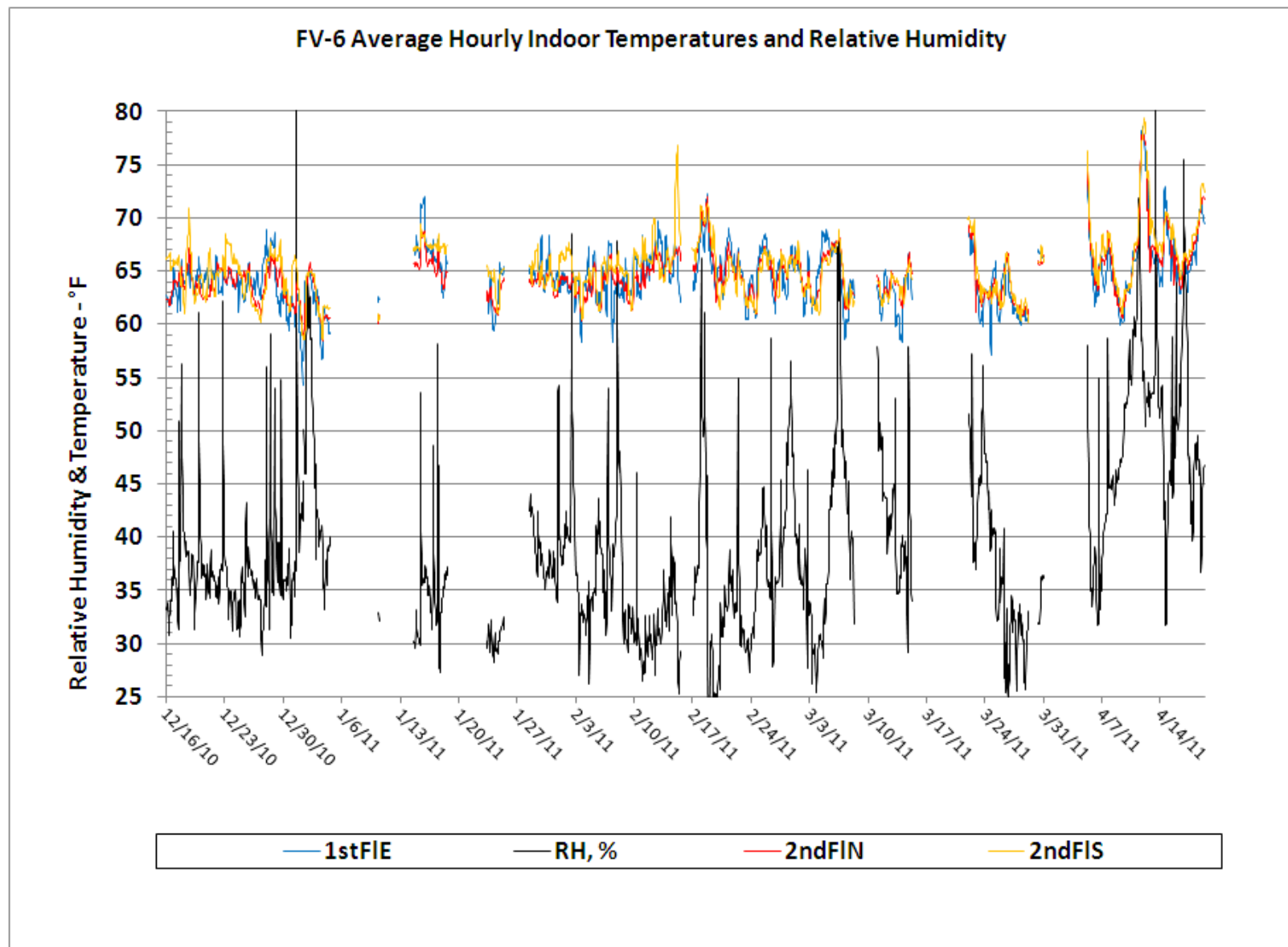
Figure 84. FV-6 Average Hourly Temperature – December 2010 to April 2011.
