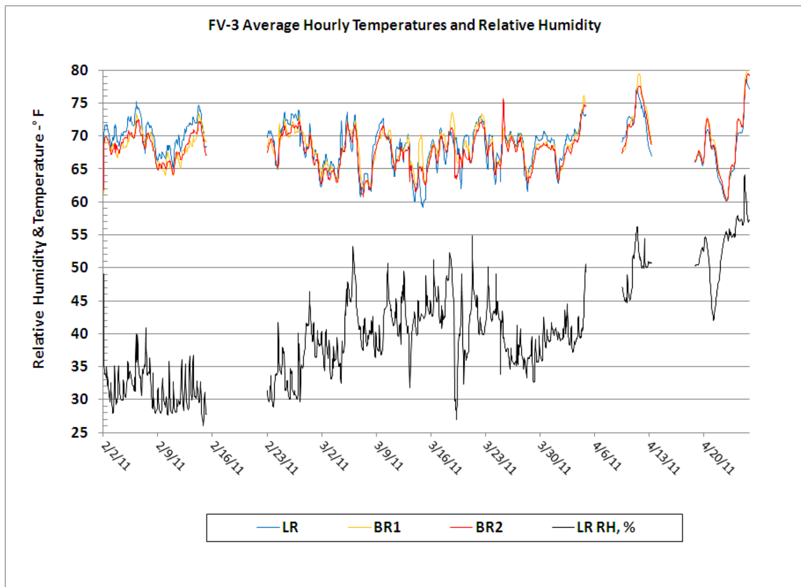
Figure 81. FV-3 Average Hourly Temperature – February 2011 to April 2011.
