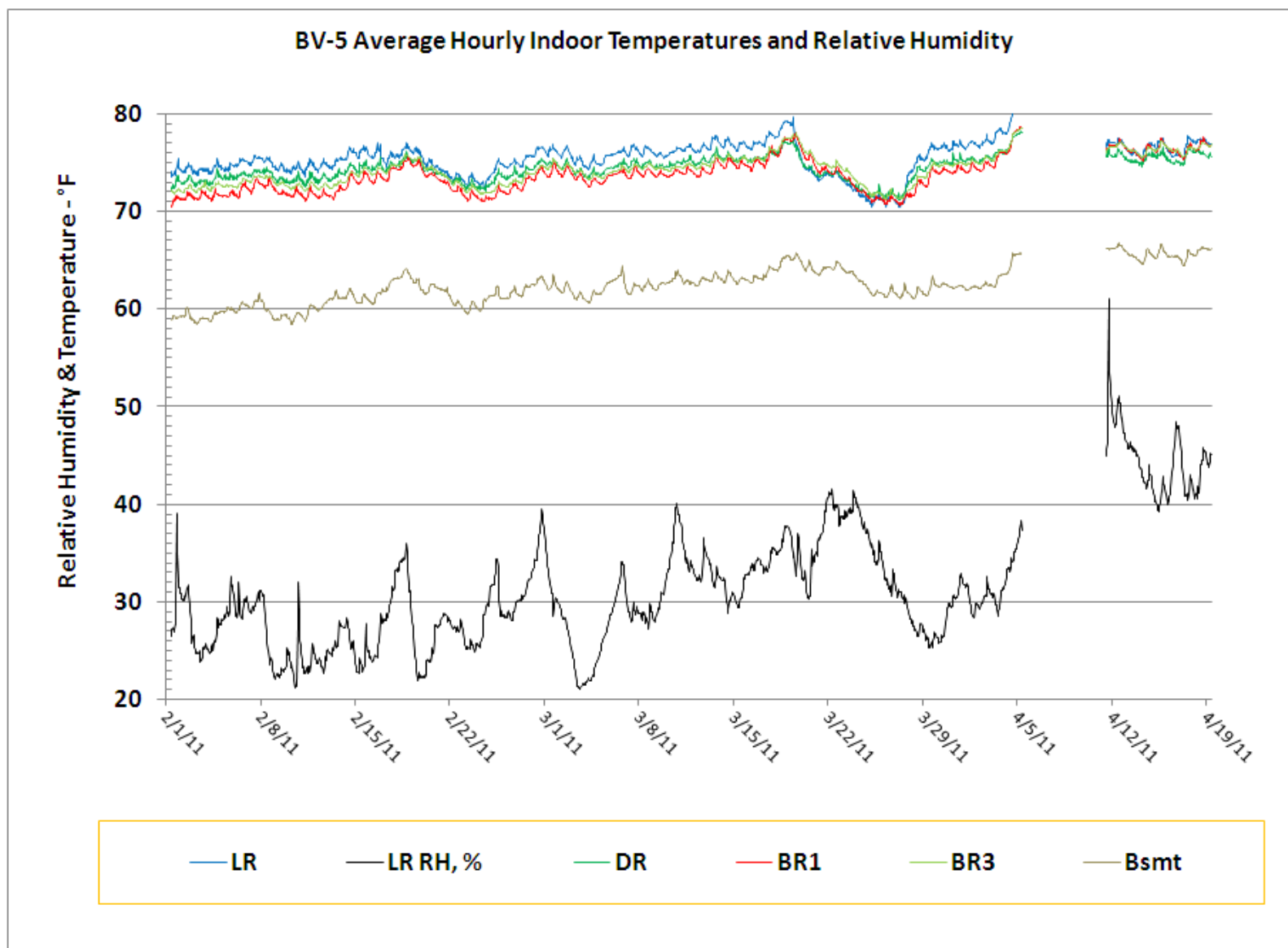
Figure 69. BV-5 Average Hourly Temperature – February 2011 to April 2011.
