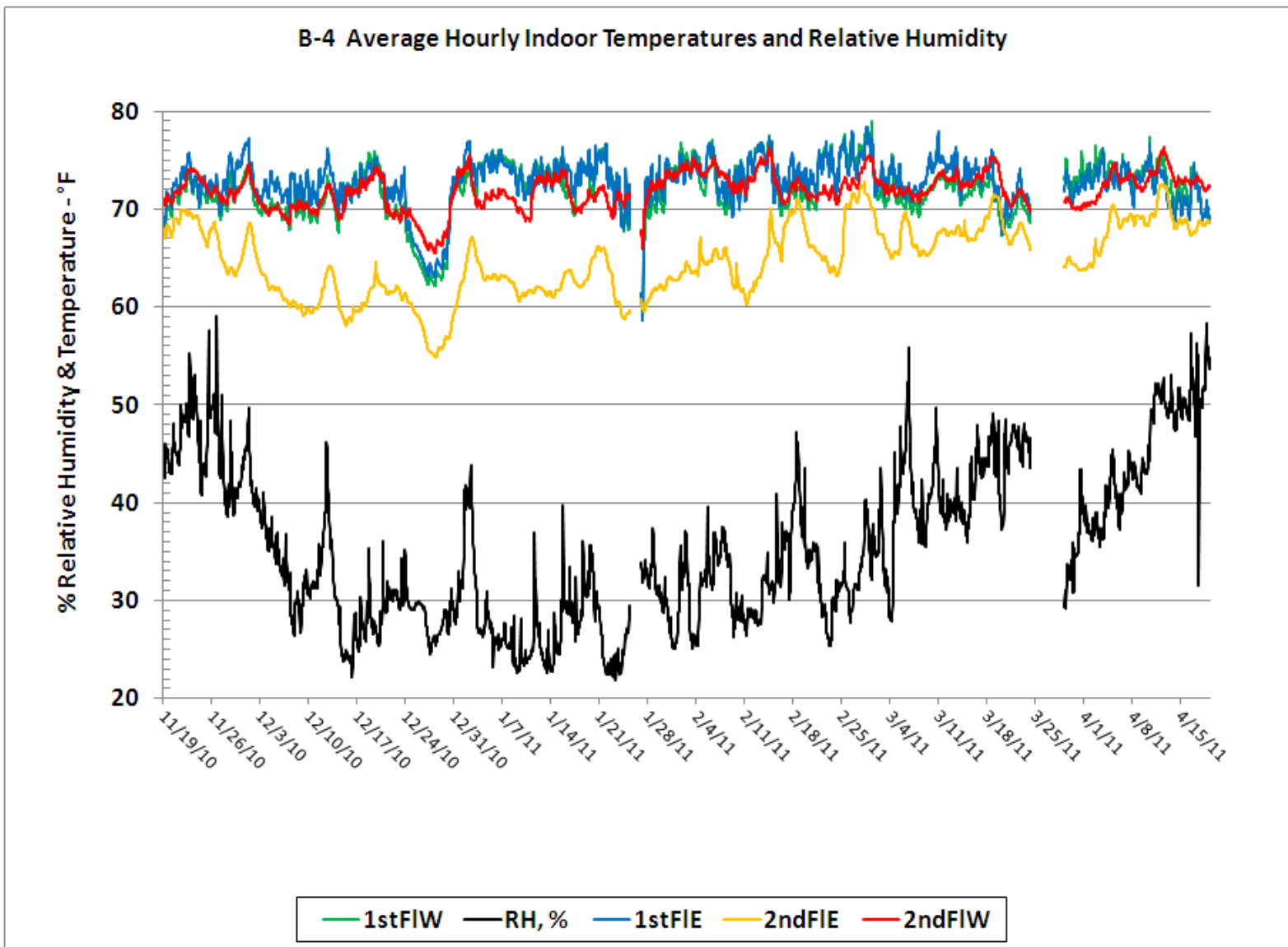
Figure 62. B-4 Average Hourly Temperature – November 2010 through April 2011.
