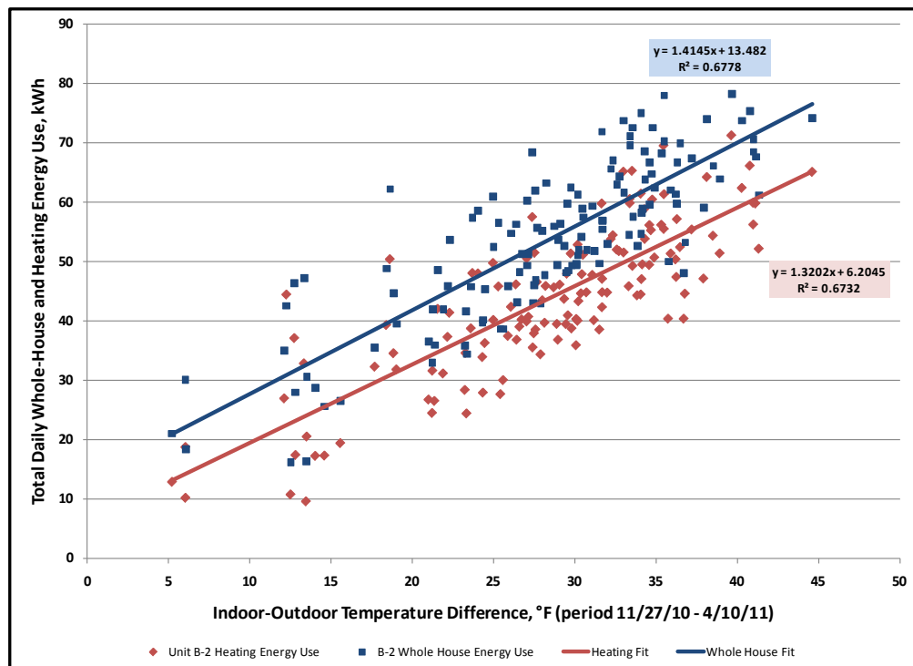
Figure 10. B-2 Whole house and heating electric use analysis.
