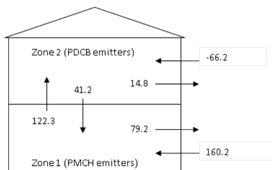
Figure 58. Air exchange profile in \text{m}^3/\text{h} between zones and across the envelope for Townsend
