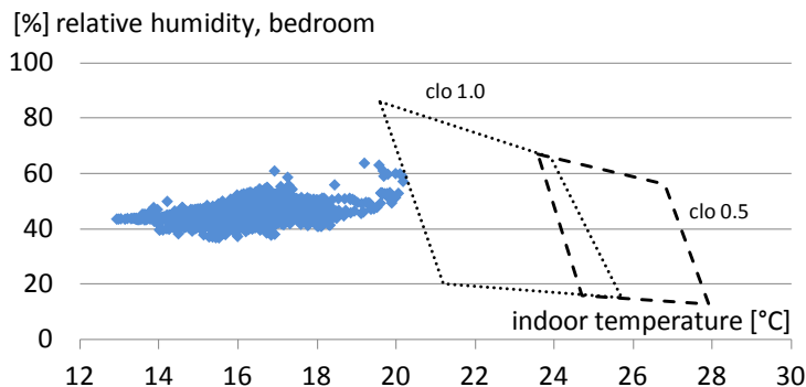
Figure 41. Comfort rating for a bedroom in Townsend
