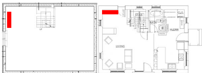
Figure 3. Floor plans and position of the mini-split indoor units (red boxes) in the Stow home Left: Basement. Right: 1st floor. The positions of the mini-split indoor units are marked by the red boxes.
