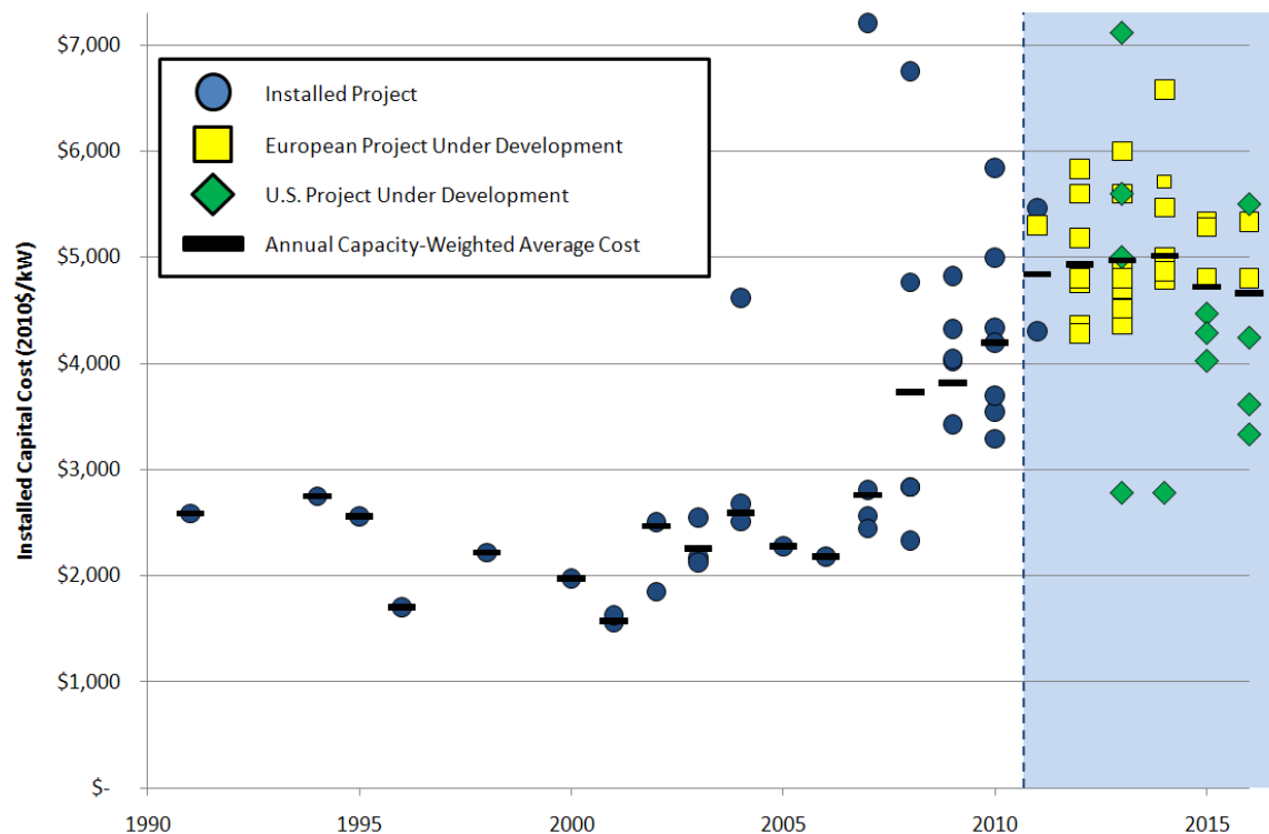
Figure 22. Offshore wind project ICC per kilowatt
