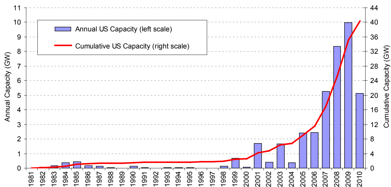
Figure 6. Growth in installed wind energy capacity
