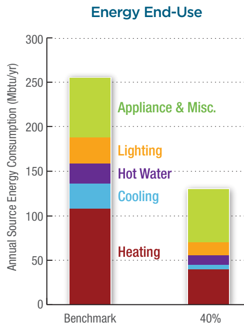
A comparison of energy usage by end use for a home built to the Building America benchmark and a home built to the 40% energy savings target in the mixed-humid climate. Example based on a 2,140 ft 2 -house in Seaford, Delaware. Analysis by IbACOS.
