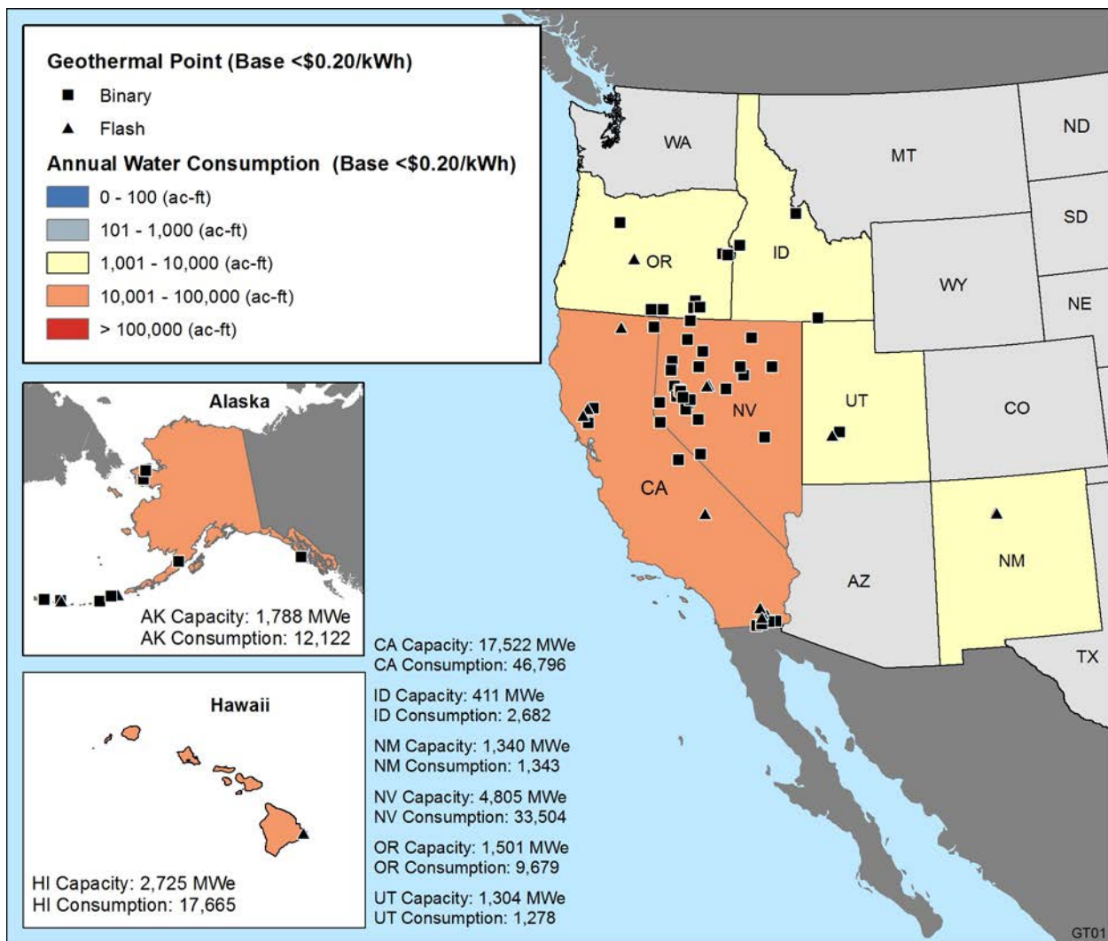
FIGURE A7 Geothermal Resources with LCOE < $0.20/kWh, Base Cost Curve.
