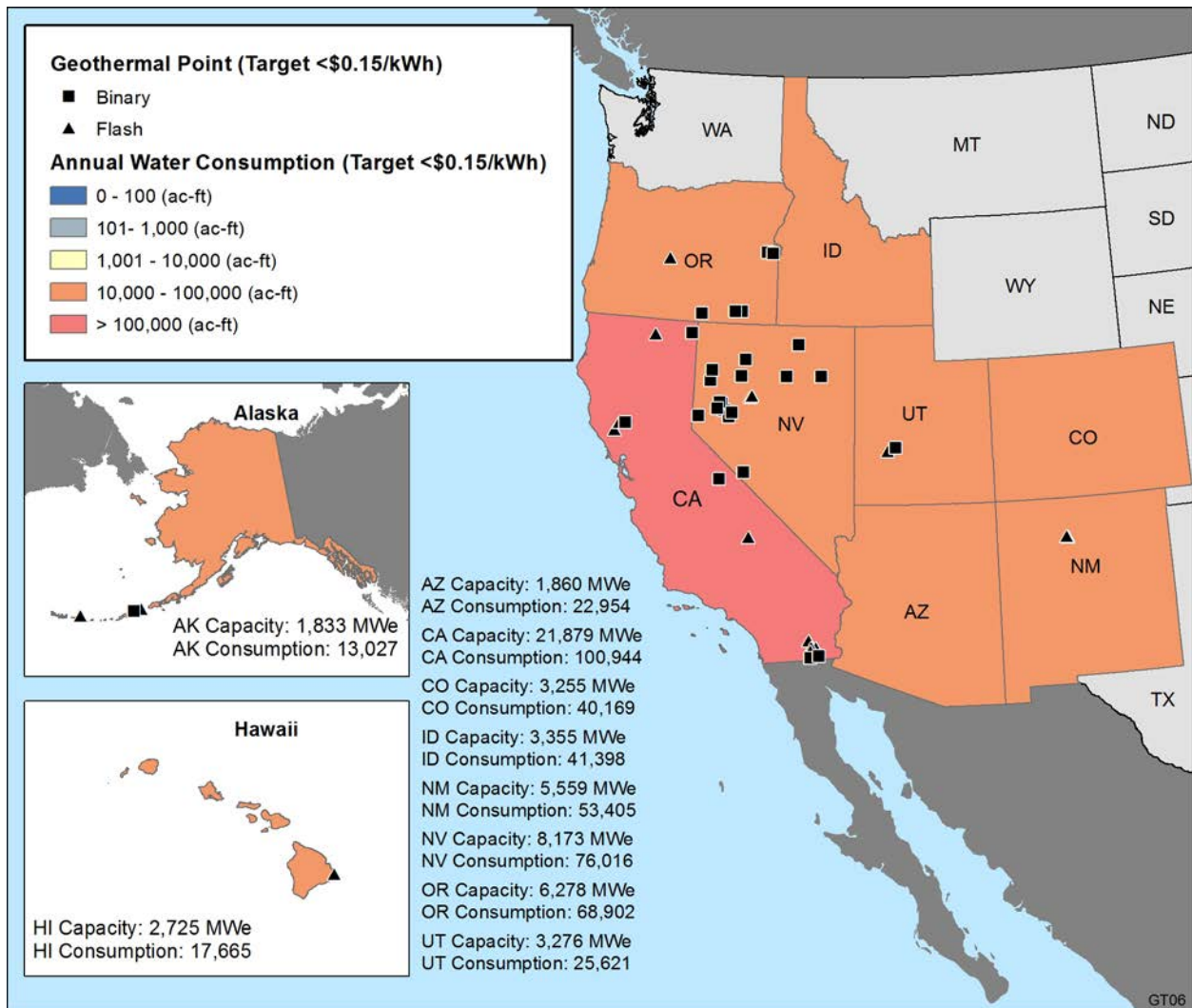
FIGURE A10 Geothermal Resources with LCOE < $0.15/kWh, Target Cost Curve.
