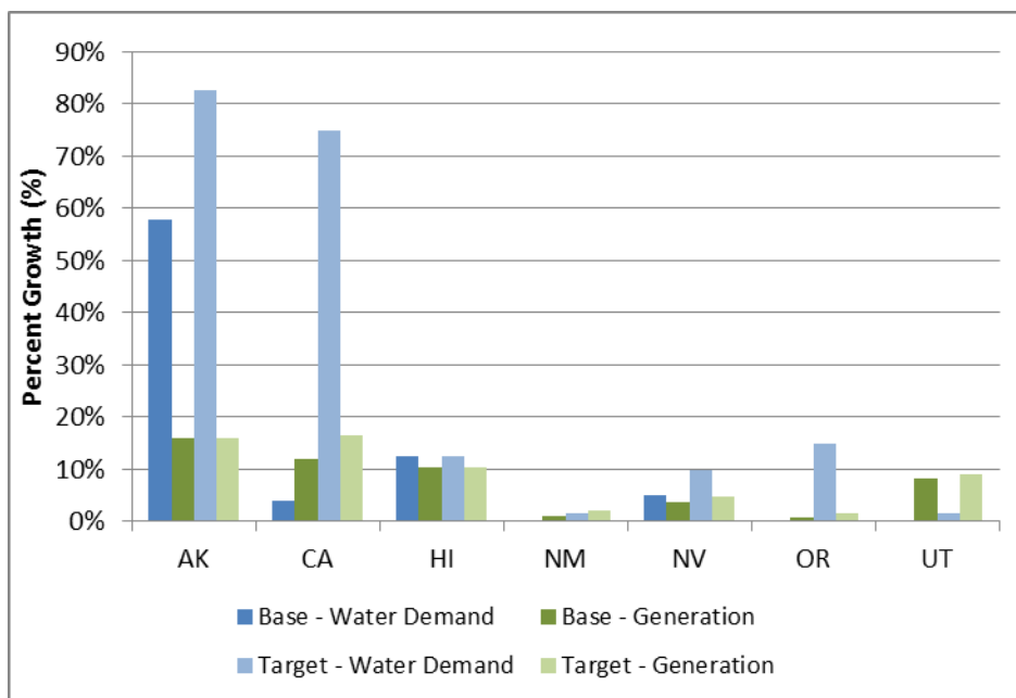
FIGURE 10 NEMS-GPRA 2030, Growth in Electricity Generation and Water Demand from Geothermal as a Percent of Existing Total Electricity Generation and Water Consumption for Thermoelectric Generation by State.
