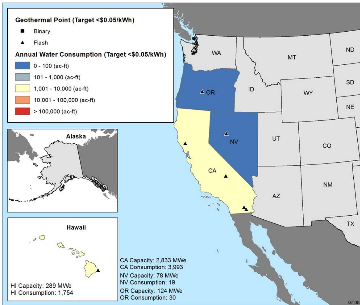
FIGURE A8 Geothermal Resources with LCOE < $0.05/kWh, Target Cost Curve.
