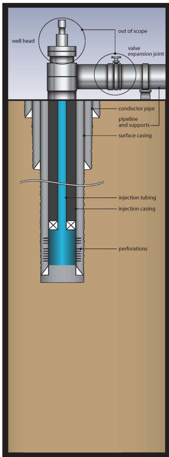
FIGURE B.2 Design for Injection Well.
