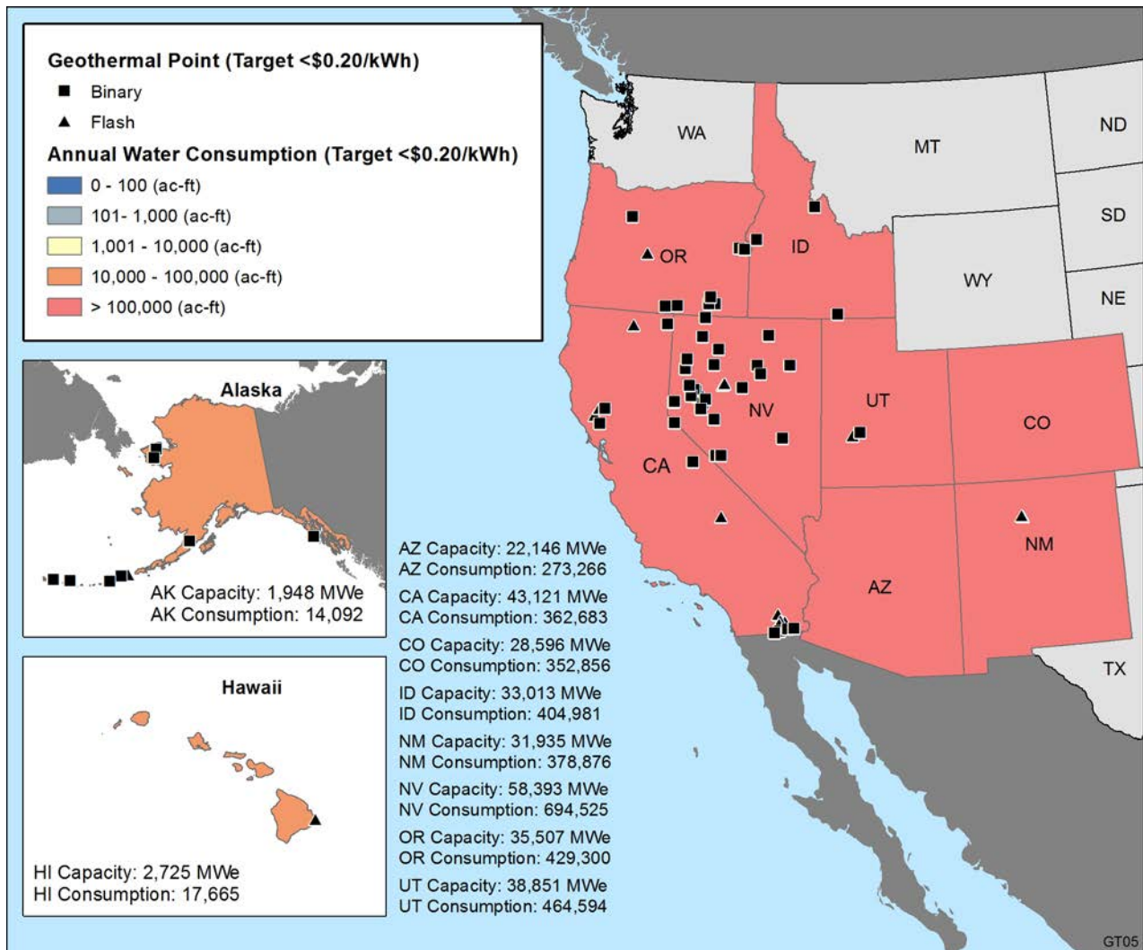
FIGURE A11 Geothermal Resources with LCOE < $0.20/kWh, Target Cost Curve.
