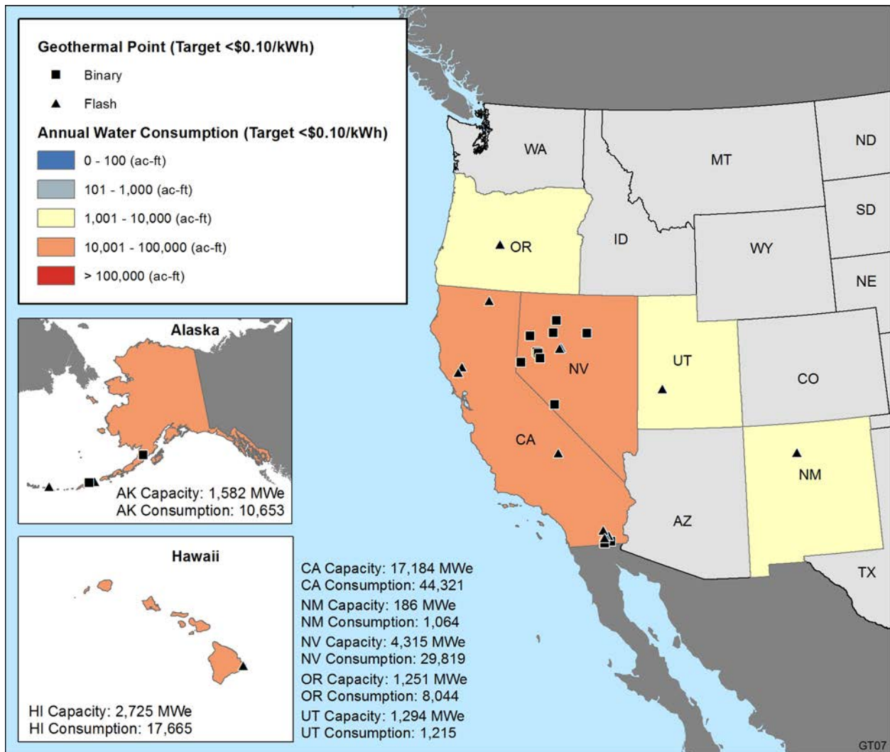
FIGURE A9 Geothermal Resources with LCOE < $0.10/kWh, Target Cost Curve.
