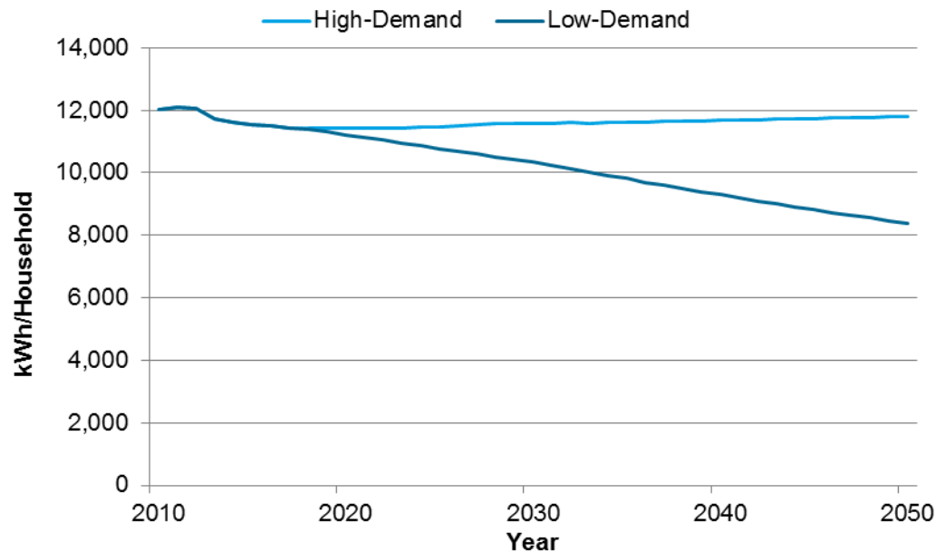
Figure H-2. Electricity intensities for residential buildings: High-Demand Baseline versus Low-Demand Baseline
