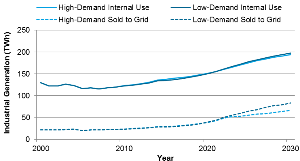
Figure J-6. Industrial generation used internally or sold to the grid (TWh)
