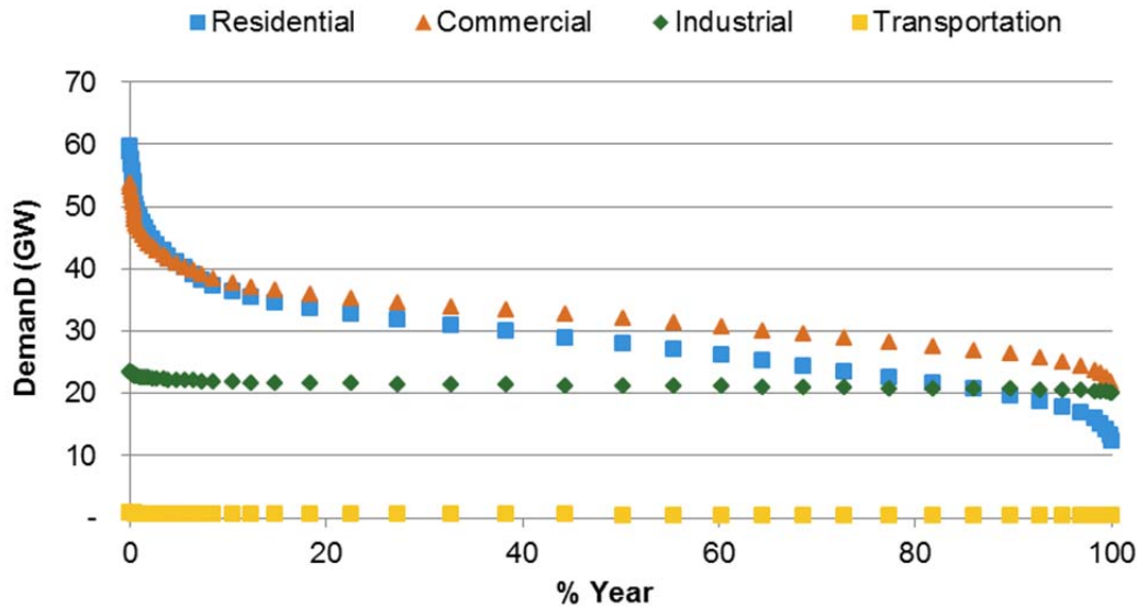
Figure I-5. Calculated load duration curves for East Central Area Reliability Coordination Agreement in 2050
