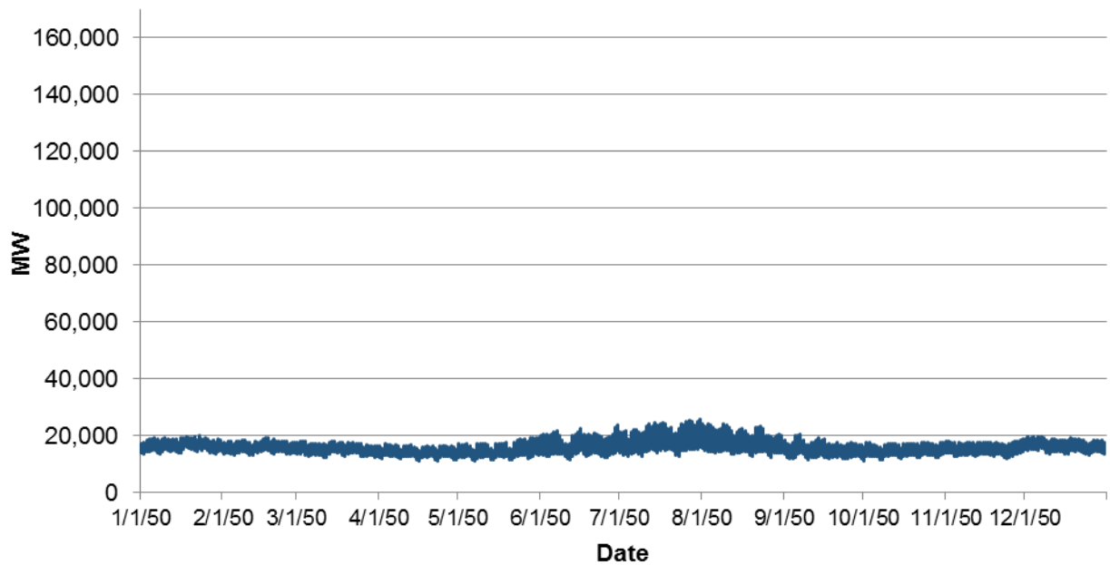
Figure N-5. Non-PEV hourly demand in 2050, Region 5 (Mid-Continent Area Power Pool)
