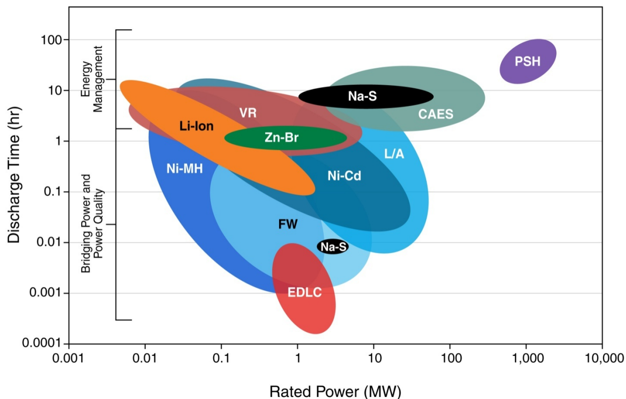
Figure 12-2. Energy storage applications and technologies
