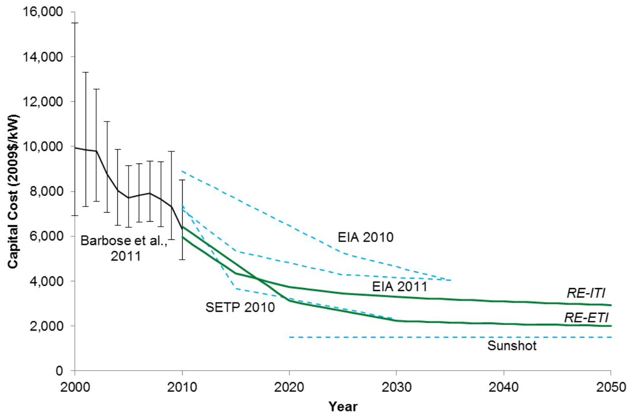
Figure 10-12. Capital cost projections for residential rooftop PV systems, 2000–2050 ($/kW of DC capacity)
