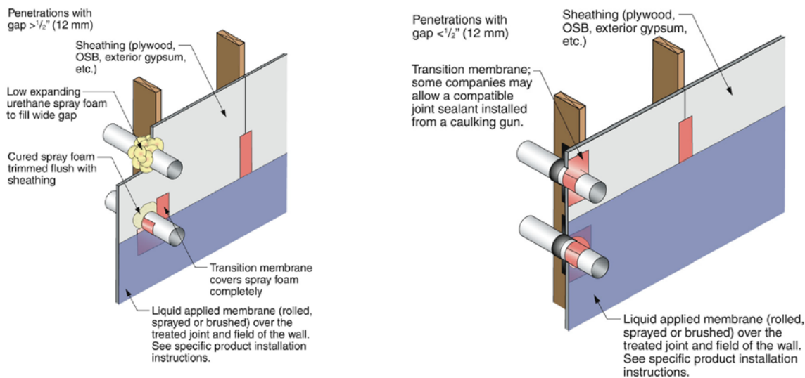
Figure 28. Mechanical penetrations
