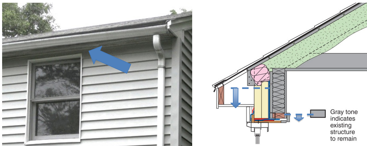
Figure 20. Left: Short eave overhang and limited separation between window head and soffit prior to retrofit at Test Home 1; Right: Roof overhang detail at Test Home 1 showing position of soffit and window head relative to pre-retrofit conditions.
