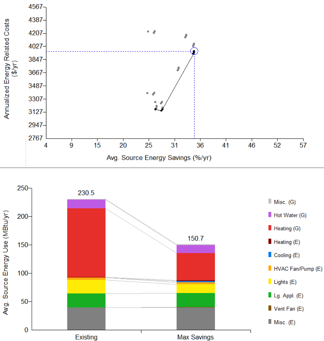
Figure 66. Test Home 2 BEopt results for as-built condition and alternatives
