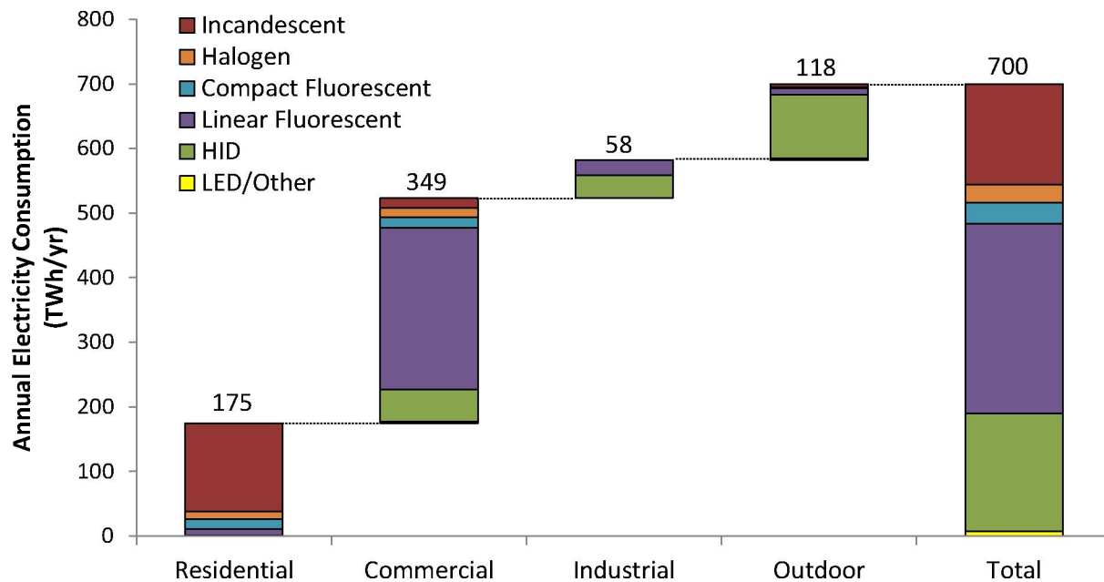
Figure 5-3 U.S. Lighting Electricity Consumption by Sector and Lamp Type in 2010
