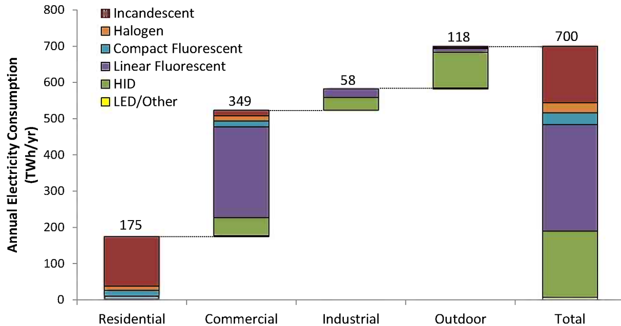
Figure ES-1 U.S. Lighting Electricity Consumption by Sector and Lamp Type in 2010
