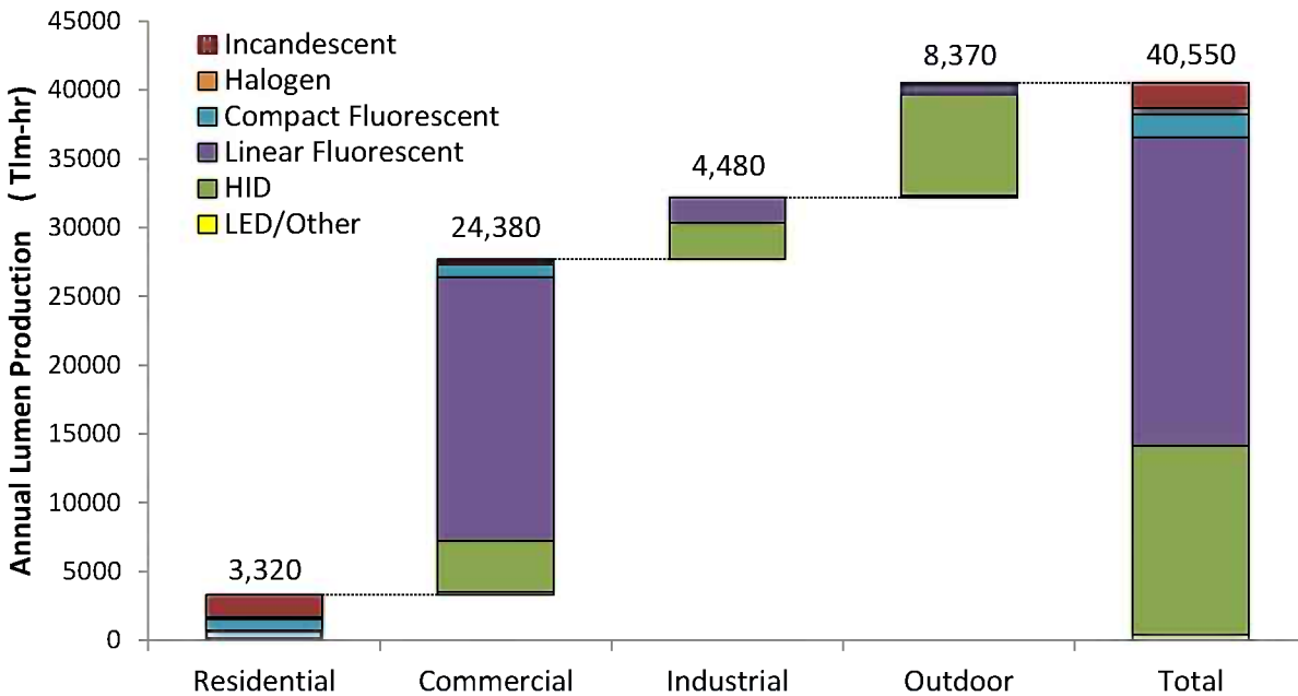
Figure 5-4 U.S. Lumens Production by Sector and Lamp Type in 2010
