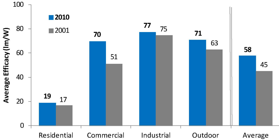
Figure 5-5 Average Efficacy by Sector
