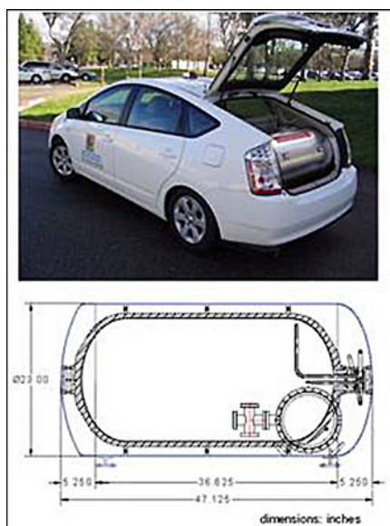
LLNL's Cryo-Compressed Hydrogen Storage Vessel
