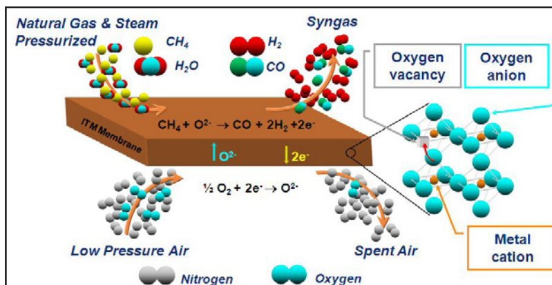
ITM Syngas Process
