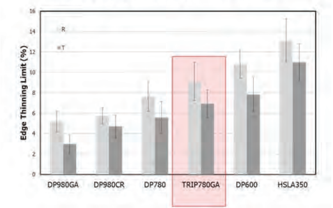
Figure 2. AHSS edge stretch limit for thinning.
