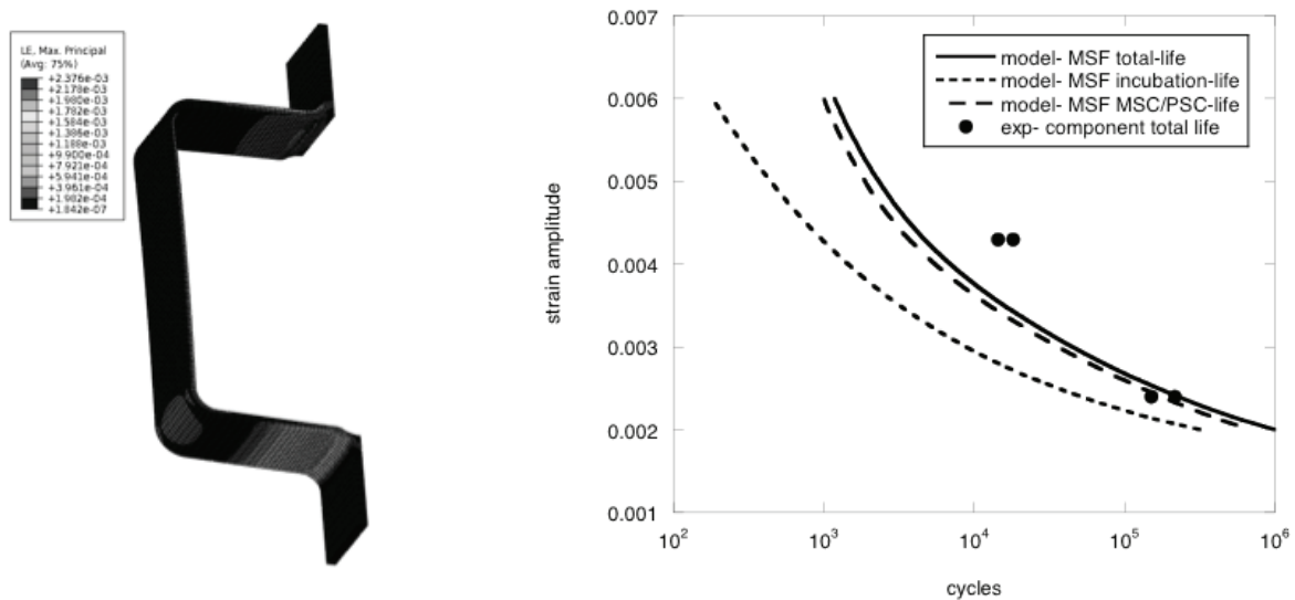
Figure 2. Results of three-dimensional FE simulations: (a) maximum principal strain contour plot of the FE analysis of the Mg AZ61 components; (b) comparison of the multistage fatigue (MSF) model to the experimental fatigue results of the AZ61 component test.
