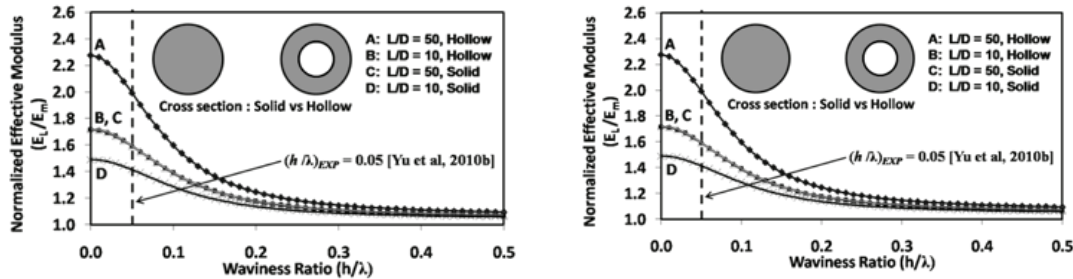
Figure 4. Effect of fiber waviness on effective longitudinal modulus for nanocomposites containing aligned (a) solid ( R_i/R_o = 0 , E_f = 240 GPa) and hollow ( R_i/R_o = 0.3 , E_f = 490 GPa) nanofibers with no interphase and (b) solid ( R_i/R_o = 0 , E_f = 240 GPa) and hollow ( R_i/R_o = 0.3 , E_f = 490 GPa, R_i/R_o = 0.3 ) nanofibers with interphase ( t/R = 0.3 , E_i/E_m = 10 ) at 0.63v% VGCNF.
