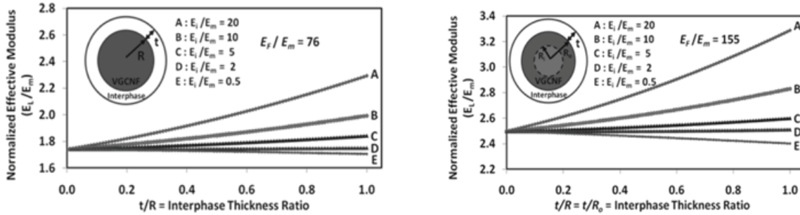
Figure 3. Effect of interphase thickness on effective longitudinal modulus for nanocomposites containing (a) solid straight nanofibers ( R_i/R_o = 0 , L/D = 100 , E_f = 240 GPa) and (b) hollow straight nanofibers ( R_i/R_o = 0.3 , L/D = 100 , E_f = 490 GPa) at 0.63v% VGCNF.
