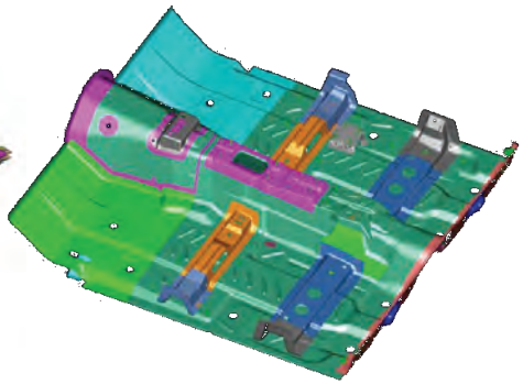
Figure 3. ACC composite underbody design
