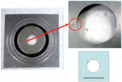
Figure 3. Medium cutout panel and large-size cutout measurement.
