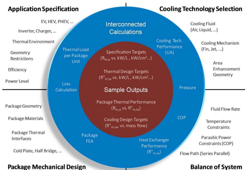
Fig. 42. Program flow
