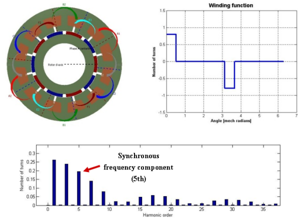
Fig. 4. Six phase (6P) machine: 2 slots/10 poles.
