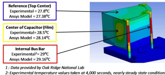
Fig. 40. Preliminary validation of DC-link capacitor thermal model
