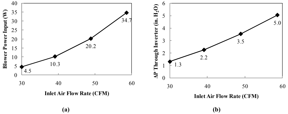
Fig. 2. Ideal blower power input (a) and \Delta P across the inverter as a function of inlet air flow rate (b).
