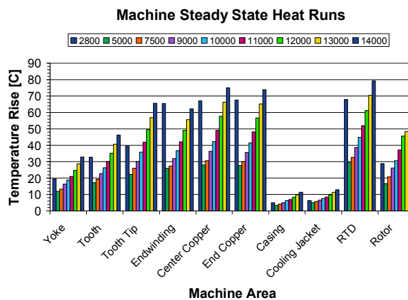
Fig. 15. Second proof-of-principle machine heat runs temperature rises in the various machine components at various speeds.
