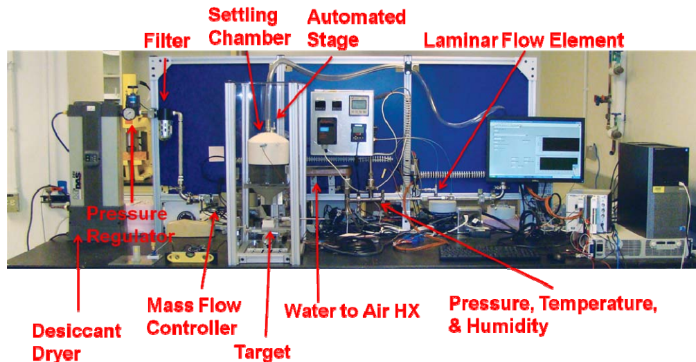
Fig. 10. Air-cooling technology characterization platform
