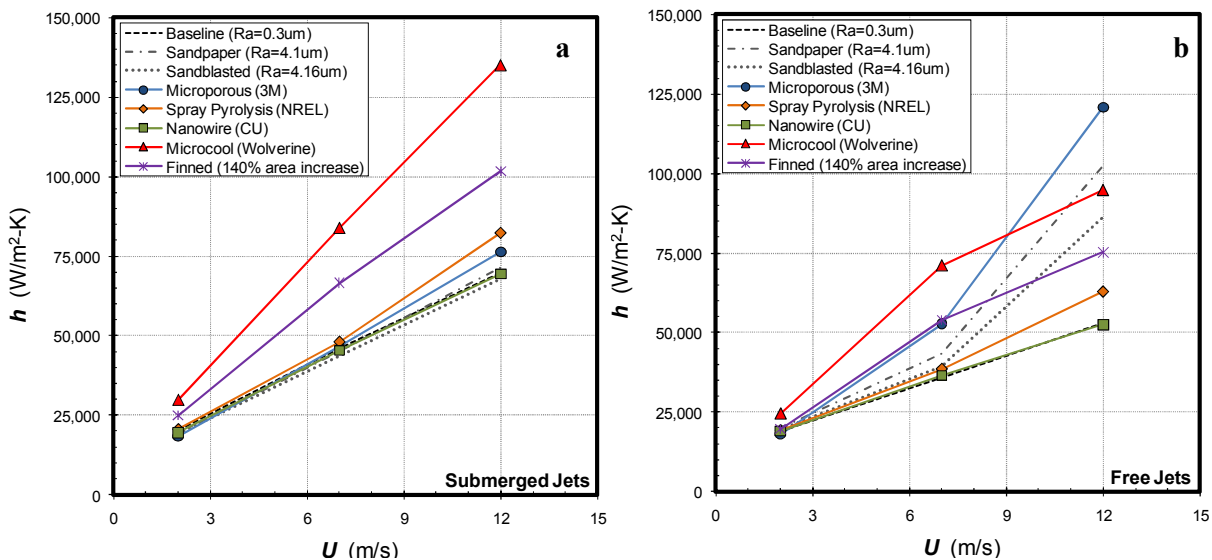
Fig. 21. Heat transfer coefficients versus fluid velocity for the various surfaces in the submerged (left) and free (right) jet configuration
