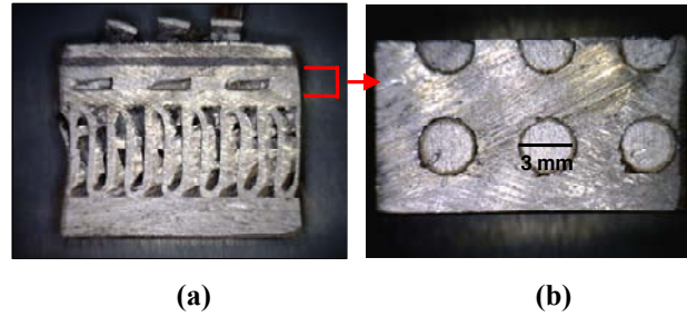
Fig. 6. Cross-sectional views of extracted 2010 Prius PEM: (a) side; (b) top.
