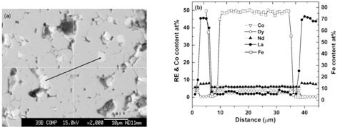
Fig. 2. Microstructure and electron microprobe composition profiles with La substituted for Y.
