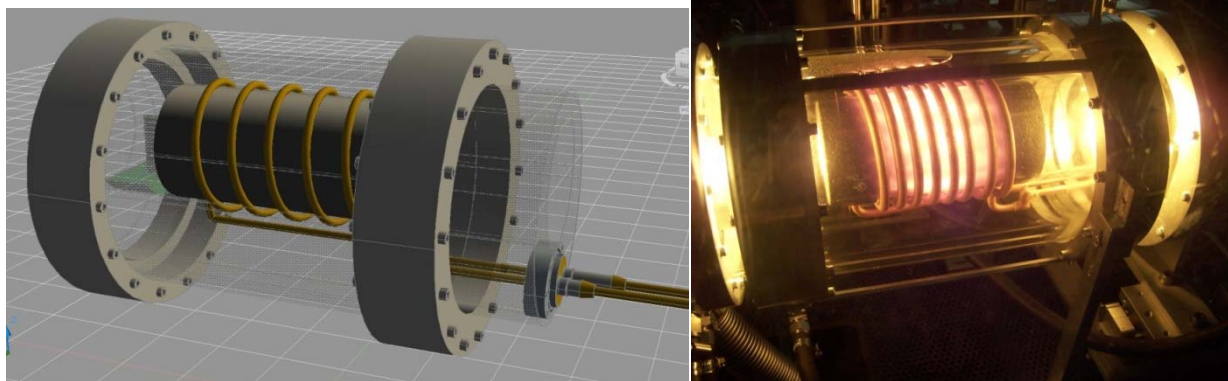
Fig. 6. (Left) Design drawing of hot-wall SiC epitaxial growth reactor custom-designed for integration into NASA Glenn SiC epitaxial growth facility. (Right) NASA Glenn hot-wall SiC reactor undergoing initial heat testing, October 2010.
