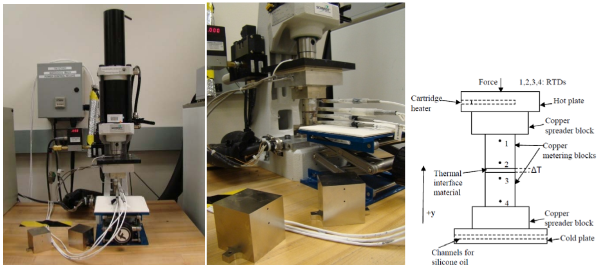
Fig. 55. Steady state thermal resistance tester (left), shown with modified 50.8 mm metering blocks (center) and as a schematic (right)
