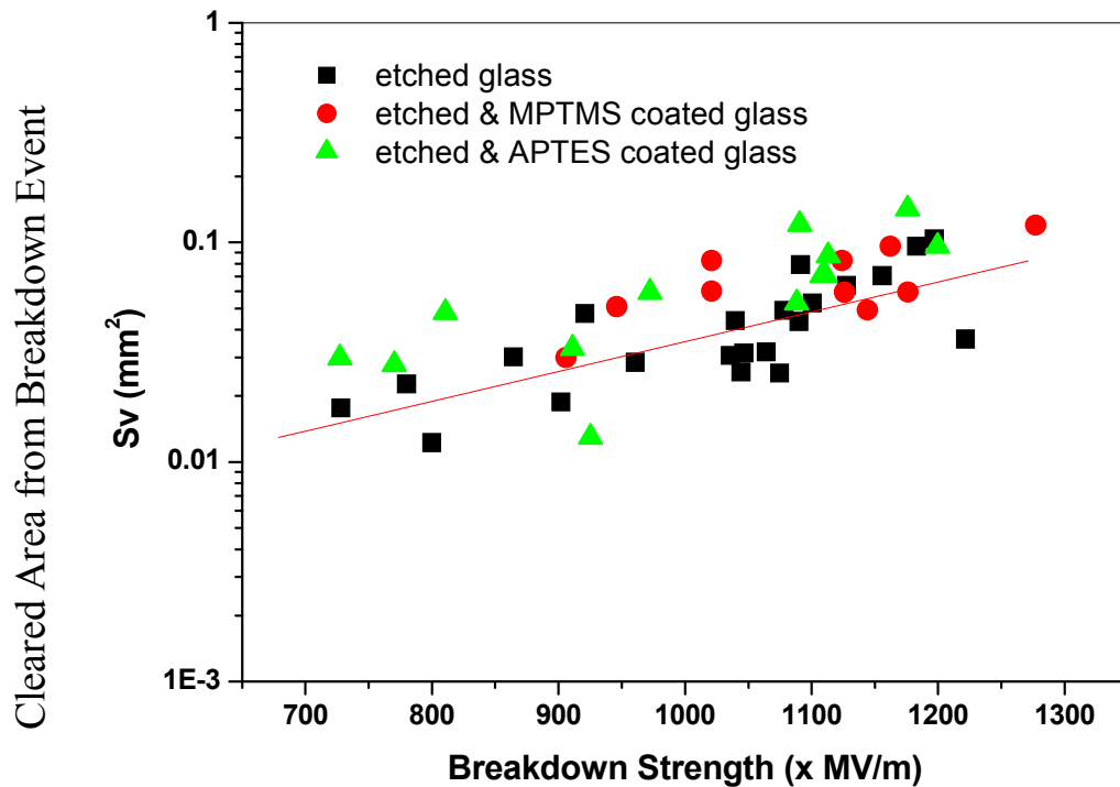
Fig. 6. Clearing area (see figure 3a for demonstration) for uncoated and polymer coated glass samples. Note that the black squares are generally lower than the green triangles or red circles. Dielectric breakdown is a statistical process that has a range of dielectric breakdown strengths.
