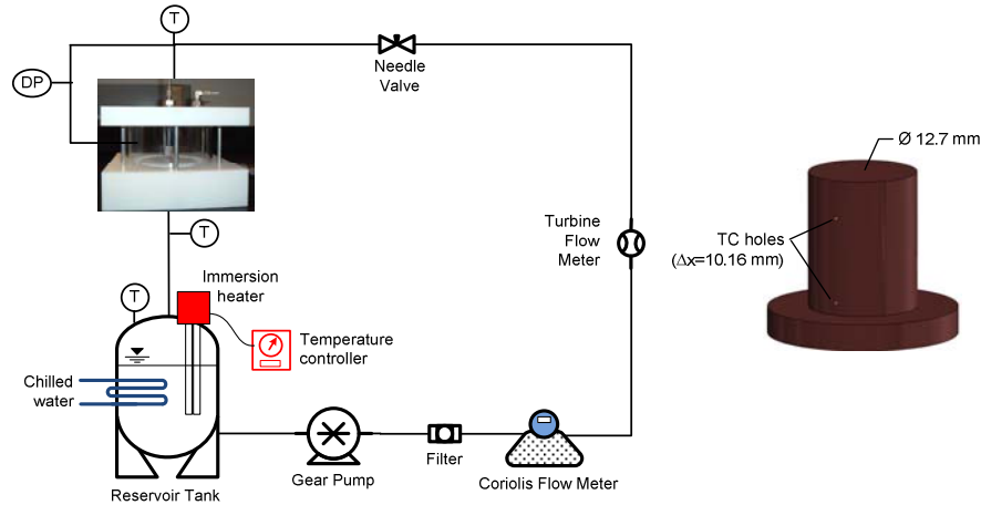
Fig. 18. Schematic of the single-phase flow loop (left) and 3-D rendering of the test heater block (right).
