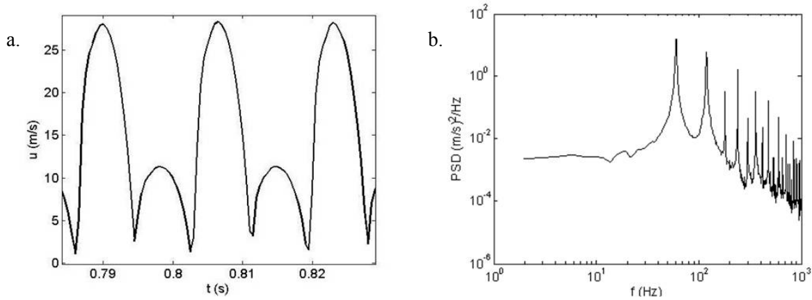
Fig. 12. Synthetic jet orifice exit velocity measurements: a. Time history b. Power spectral density
