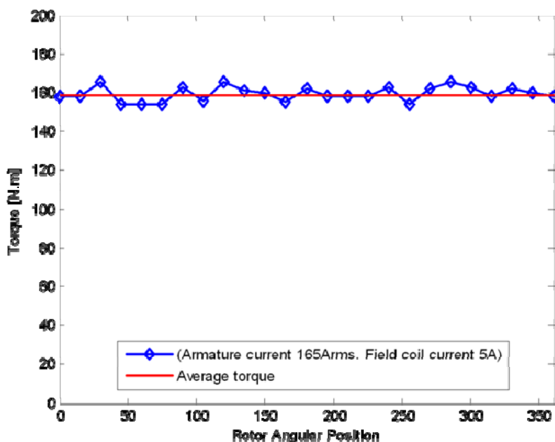
Fig. 9. Torque quality.
