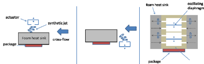
Fig. 9. Schematic (above) and CAD model (below) of possible cooling configurations
