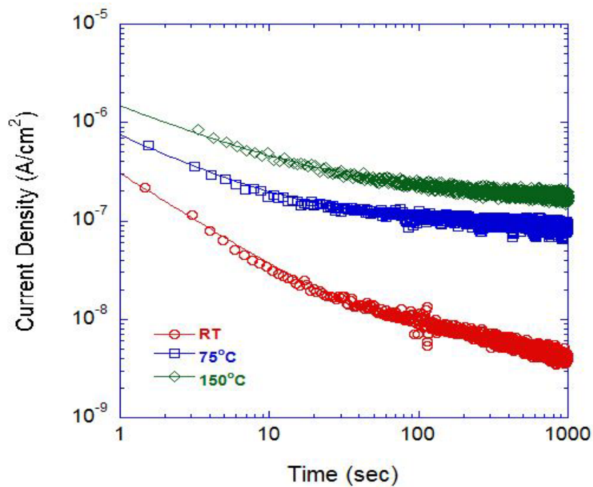
Fig. 3. Time-relaxation current density measured on a PLZT/LNO/Ni sample under 8.7 \times 10^4 V/cm electric field at room temperature, 75°C, and 150°C.
