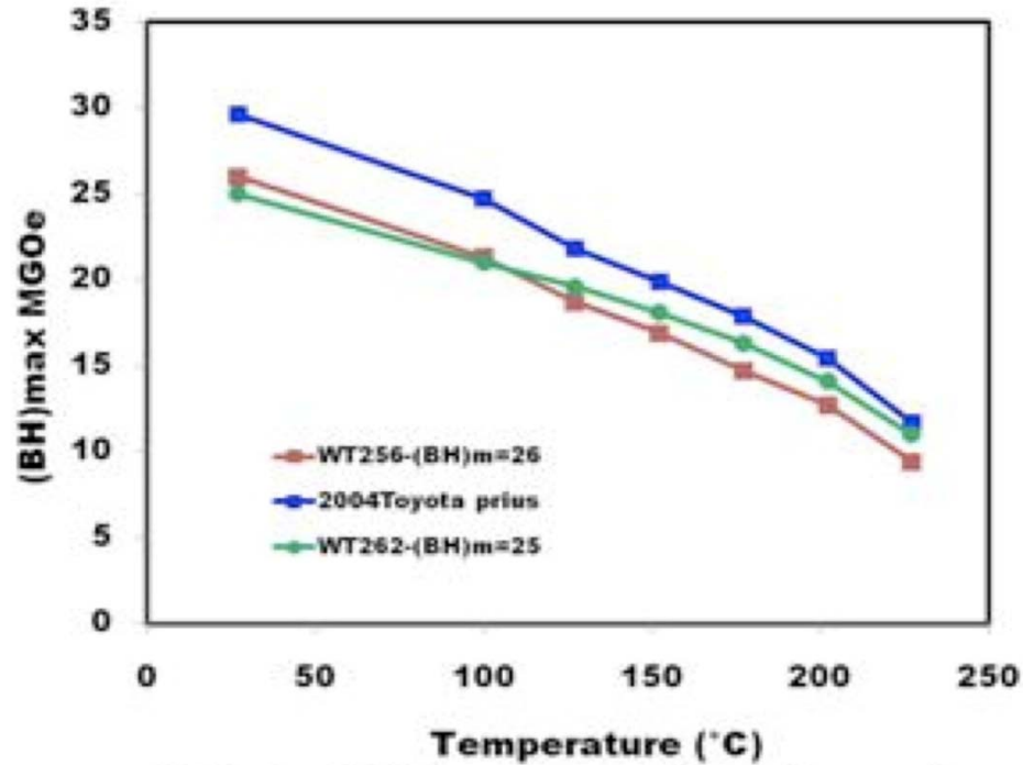
Fig. 1. (BH)_{\max} as a function of temperature for experimental and commercial magnets.
