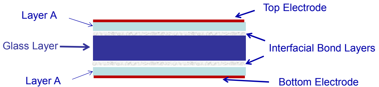
Fig. 5. Schematic of a capacitor cross section with a polymer (layer A), interfacial bond layers (surfactant) and glass.
