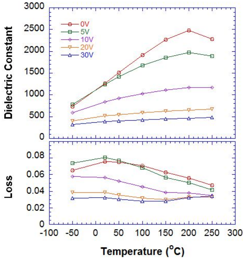
Fig. 2. Dielectric constant and loss as a function of temperature measured under applied bias voltages.
