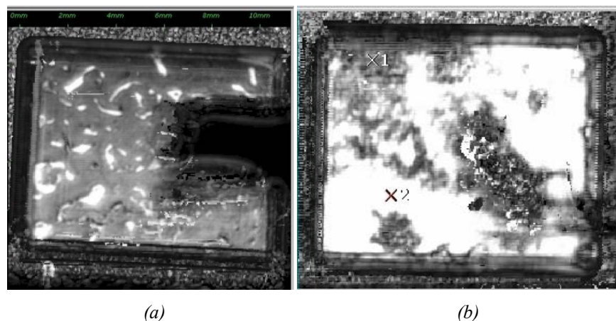
Fig. 10. Comparison of die attach delamination (shown as white areas) under the diode for a Co-Pack sample that underwent a) 0 cycles and b) 1500 cycles from 25°C to 200°C.
