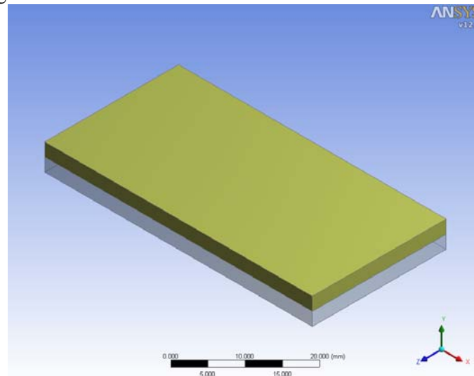
Fig. 5. FEA model of the bi-metal assembly from Suhir (1986)
