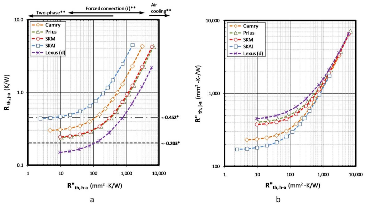
Fig. 31. Package configuration thermal performance. All packages are cooled on one side, except for the Lexus package. Cooling performance ranges are based on Mudawar [4]. (a) Junction to coolant thermal resistance; (b) Unit area junction to coolant thermal resistance.
