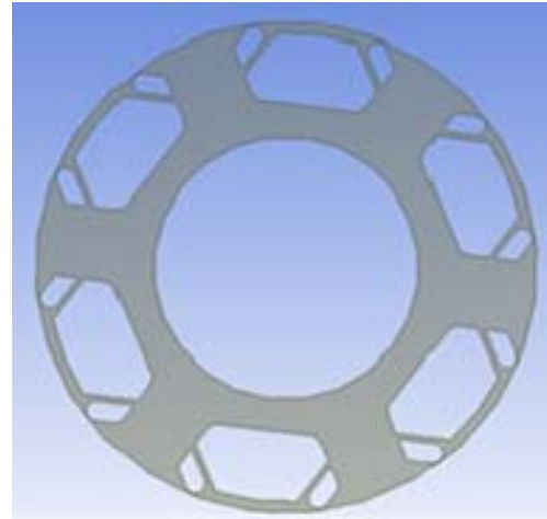
Fig. 4. Rotor punching.
