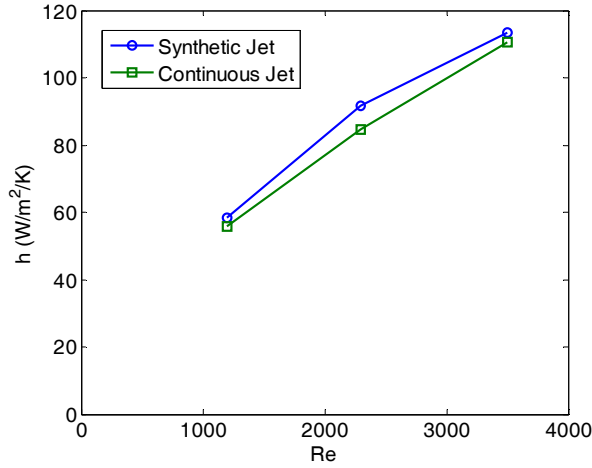
Fig. 14. Comparison of the thermal performance of synthetic and continuous jets for an orifice diameter (d) of 5 mm and an orifice-to-heater distance of 5d.
