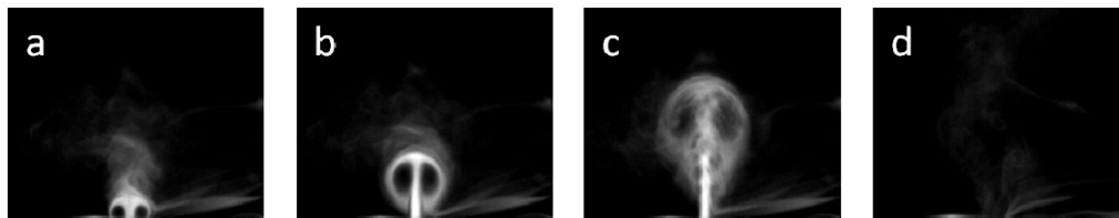
Fig. 8. Synthetic jet smoke visualization showing the progressive evolution of the leading vortical structure
