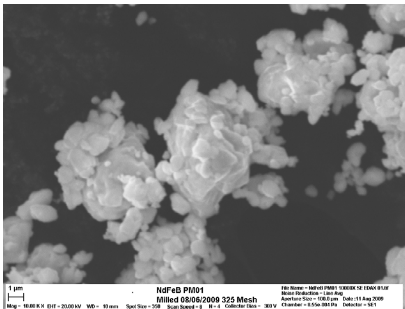
Fig. 20. Scanning Electron Microscopy image of hydrided and planetary milled Nd 15 Fe 77 B 8 powder produced at GE Global Research. Average particle size is 3 to 5 \mu\text{m} , with some finer particles agglomerated to larger particles.
