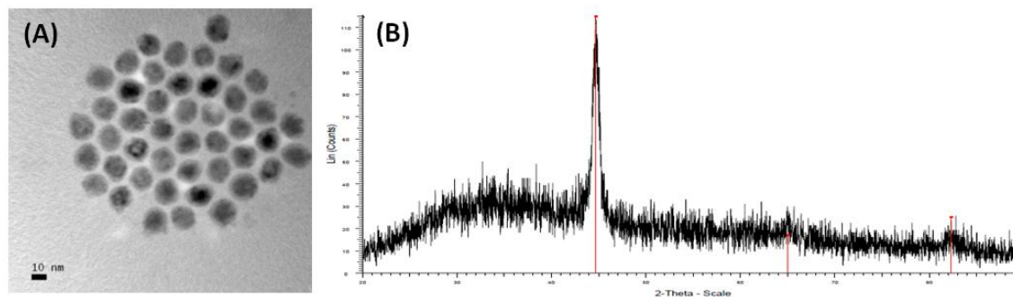
Fig. 13. TEM image of the 14 nm Fe nano-particles; (B) XRD of the 14 nm FePt nano-particles showing typical body centered cubic (bcc) structure.
