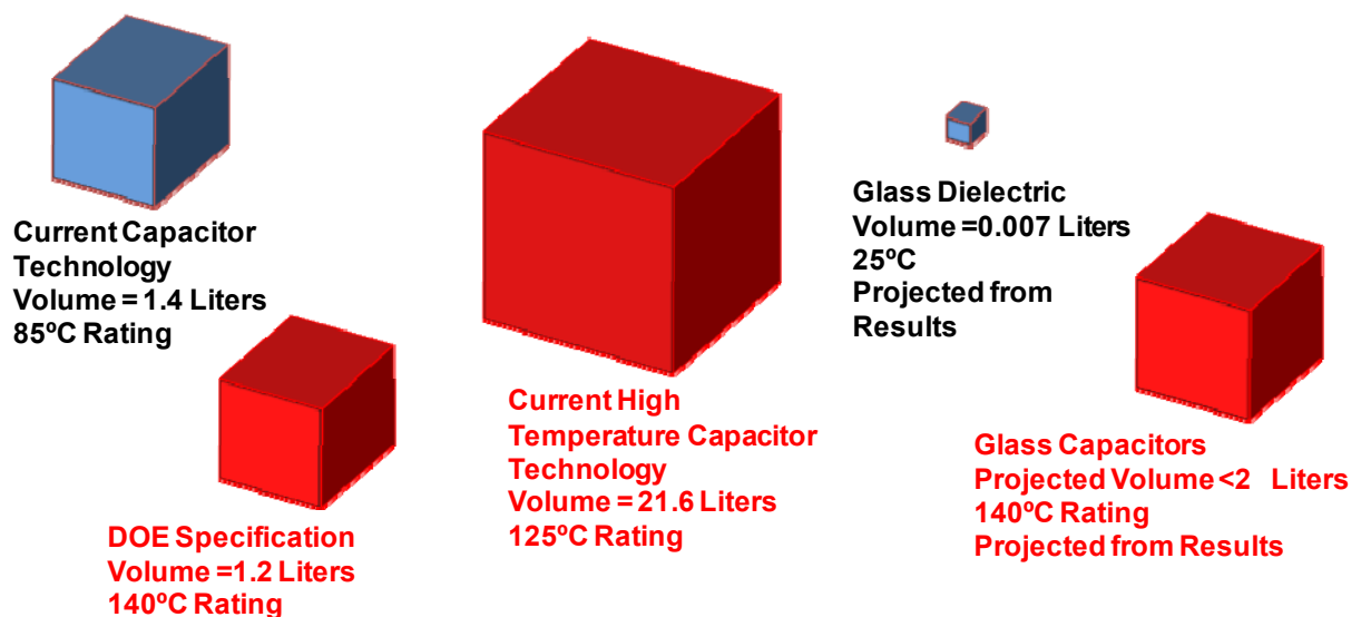
Fig. 1. Volumetric comparison between DOE capacitor specifications, commercial capacitors and the projected capacitor volumes from the research at Penn State. All volumes shown are for a 1000 \mu\text{F} 1000 V capacitor.
