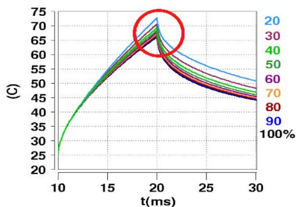
Fig. 8. Effect of die attach thermal conductivity level on junction temperature
