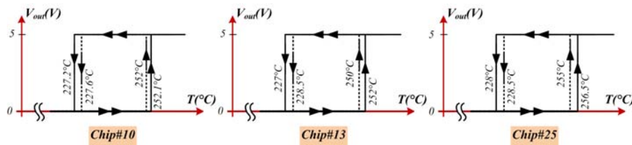
Fig. 8. Temperature sensor output in response to temperature cycling.
