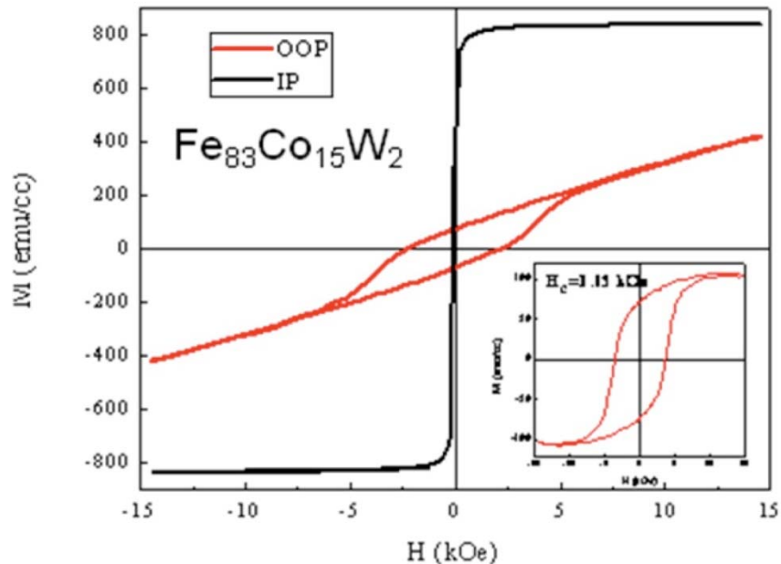
Fig. 15. MH loops of one of the compositions that displays a large coercive field in the out of plane (OOP) direction. The inset is the out-of-plane loop with the “linear” background subtracted.
