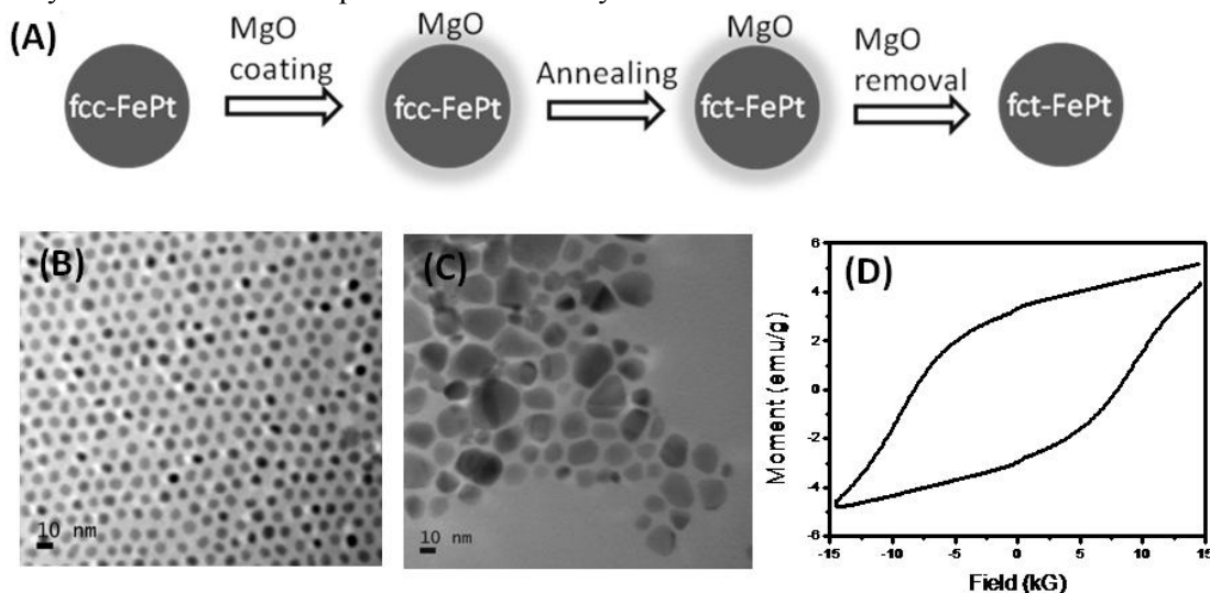
Fig. 12. (A) Schematic illustration of the synthesis of fct-FePt nano-particles; (B) TEM image of the 7 nm fcc-Fe 60 Pt 40 nano-particles; (C) TEM image of the fct-FePt nano-particles after MgO removal; (D) room temperature hysteresis loop of the fct-FePt nano-particles.
