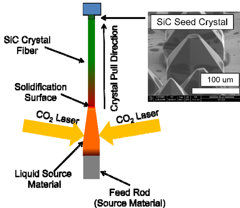
Fig. 2. Solvent Laser Heated Float Zone (Solvent-LHFZ) approach for growing single-crystal SiC fibers.
