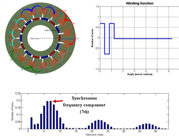
Fig. 3. Five phase (5P) machine: 15 slots/14 poles.
