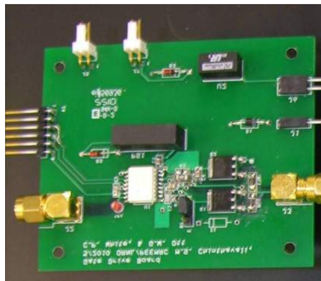
Fig. 4. Gate Drive Board used for Testing
