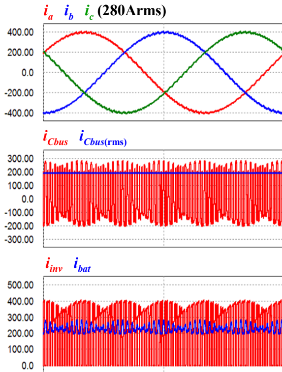
Figure 2. Simulated waveforms in the standard VSI based drive system.
