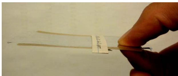
Fig. 10. Image of hot pressed stacked capacitor using discrete Al layers
