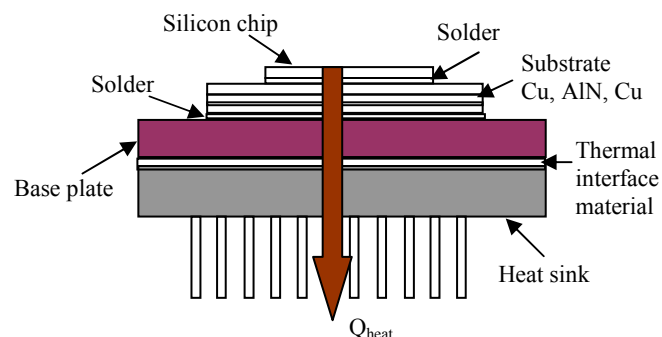
Fig. 52. A typical power electronics package
