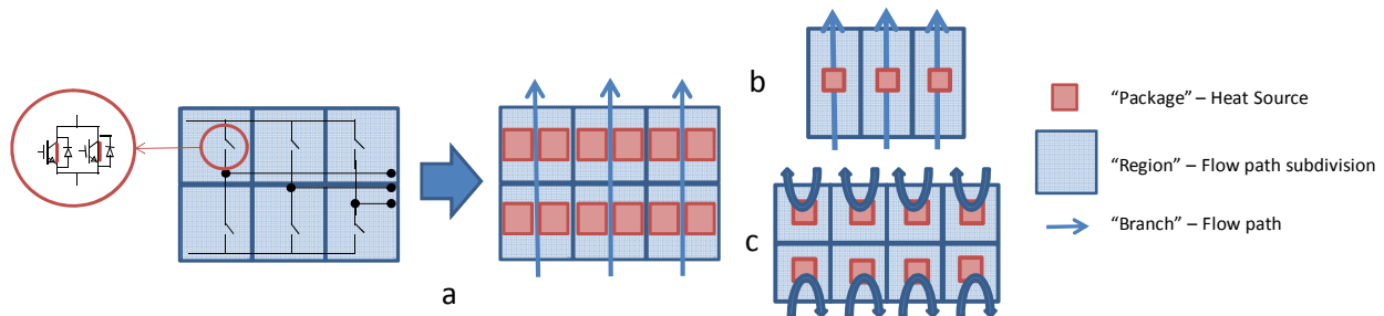
Fig. 16. a. Coolant system flow path abstraction and definition; b. Cold plate; c. DC-DC converter
