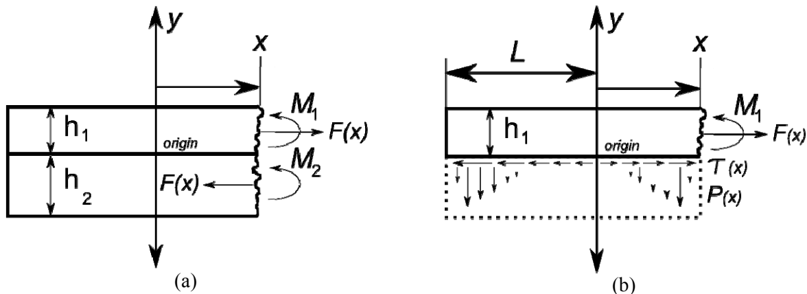
Fig. 1. Forces and moments in a bi-material assembly under thermally induced stress. (a) is the full assembly while (b) shows layer 1 with a ghosted (dashed) image of layer 2 and indicates the shearing forces that arise at the interface between layer 1 and 2
