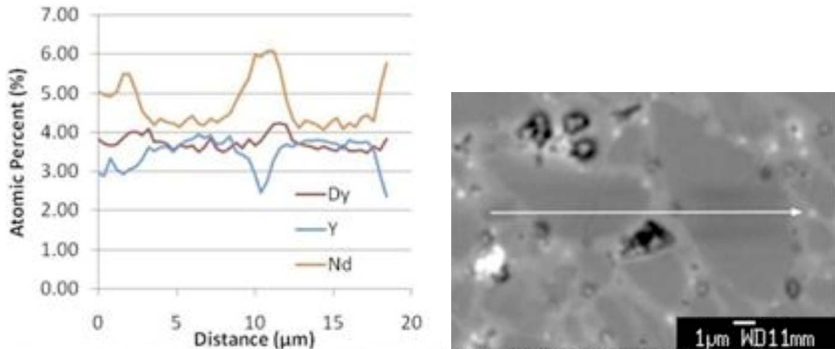
Fig. 5. Microstructure and electron microprobe composition profiles of sample sintered at 825°C/1h with 110MPa applied pressure in vacuum hot press.
