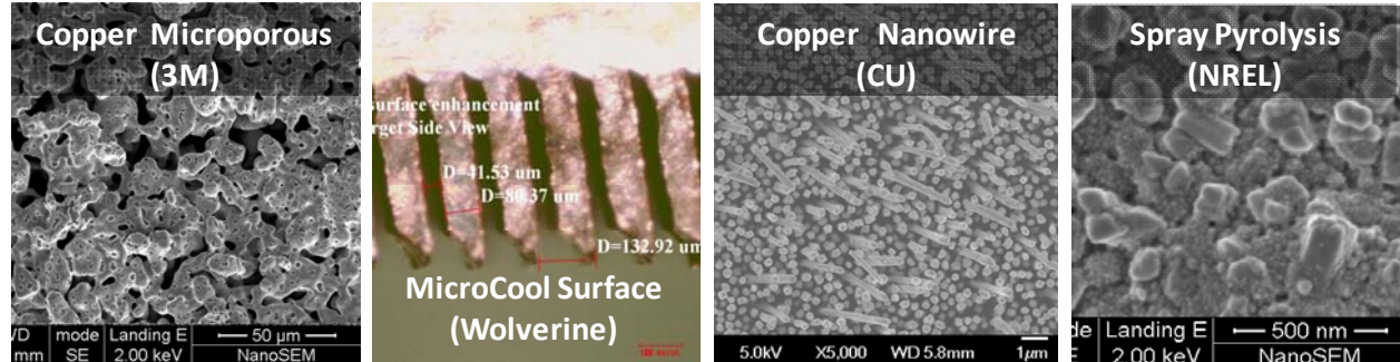
Fig. 17. SEM images of the enhanced surfaces tested
