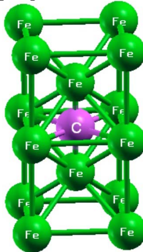
Fig. 9. Illustration of C in interstitial site of bcc-Fe lattice.
