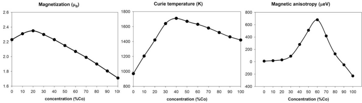
Fig. 8. Electronic structure calculation results for intrinsic magnetic properties of Fe-Co system.
