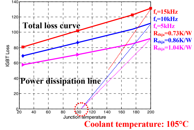
Fig. 18. IGBT power losses and thermal analysis at different frequencies.
