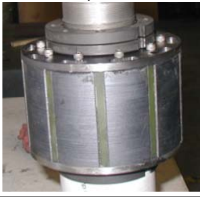
Fig. 3. Rotor of the first proof-of-principle machine
