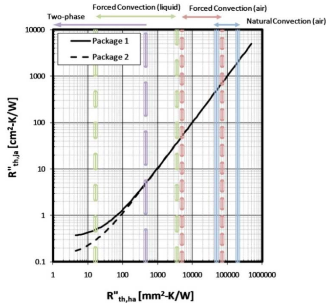
Fig. 43. Package mechanical design thermal performance. Cooling ranges based on heat transfer coefficients from Mudawar [4].
