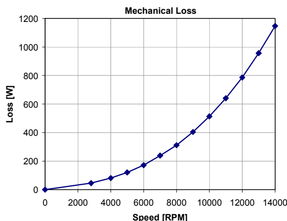
Fig.11. Mechanical loss test result of the second PoP machine with unmagnetized magnets
