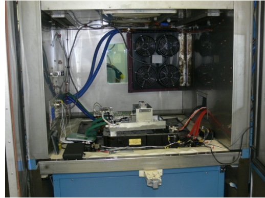
ESS Inverter Testing
