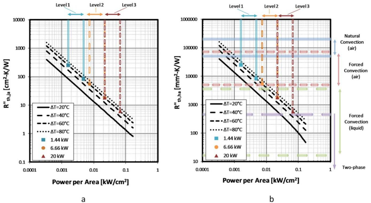
Fig. 45. (a) Impact of application technical specifications on thermal performance requirements with level 1, 2, and 3 charge levels highlighted, (b) Application technical specification linked to thermal design targets with cooling ranges highlighted. Cooling ranges based on Mudawar [4] for convection coefficients (surface enhancements would reduce the effective thermal resistance).
