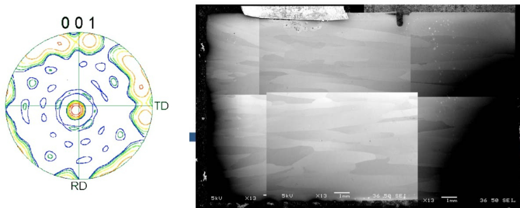
Fig. 17. OIM pole figure (left) from transverse section of Alnico 5-7 that shows excellent grain alignment along the magnetization direction, but random orthogonal alignment. Also, a composite SEM micrograph of the transverse section is shown (right), where very large aligned grains are visible.
