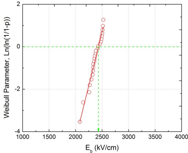
Fig. 8. Weibull distribution of capacitors formed using hydrogenated polymer with stoichiometry n = 3m
