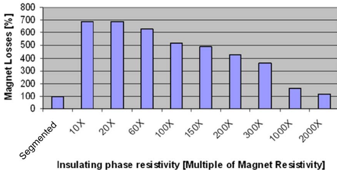
Fig. 19. Effect of insulating phase resistivity on magnet losses. An insulating phase with a resistivity with a resistivity of at least 2000X that of the resistivity of NdFeB is needed to approach the low magnet loss of mechanically segmented magnets.
