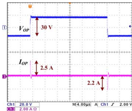
Fig. 2. R-C load test results at 200^\circ\text{C} with R_G = 3.4\ \Omega and C_{\text{Load}} = 10 nF.
