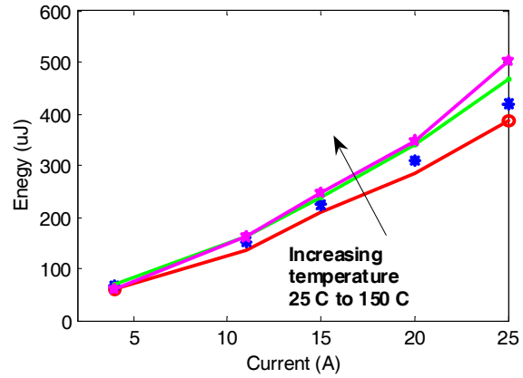
Fig. 4. Total switching energy losses of a 1,200 V, 50 A, SiC JFET at 400 V.
