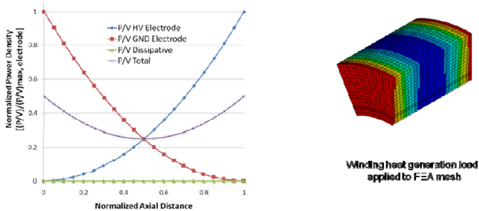
Fig. 39. Non-uniform heat generation in the capacitor windings
