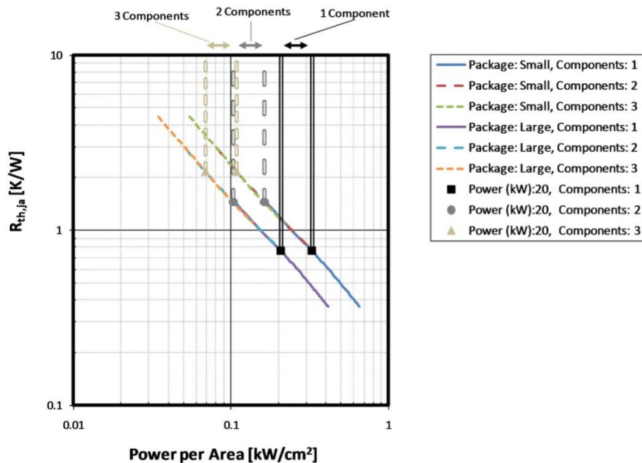
Fig. 50. Application technical specifications with variable number of components in parallel with application ranges highlighted
