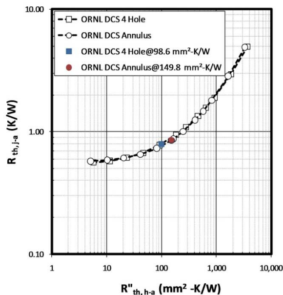
Fig. 34. Total thermal resistance thermal performance characterization of ORNL baseline 4-hole and annulus package designs
