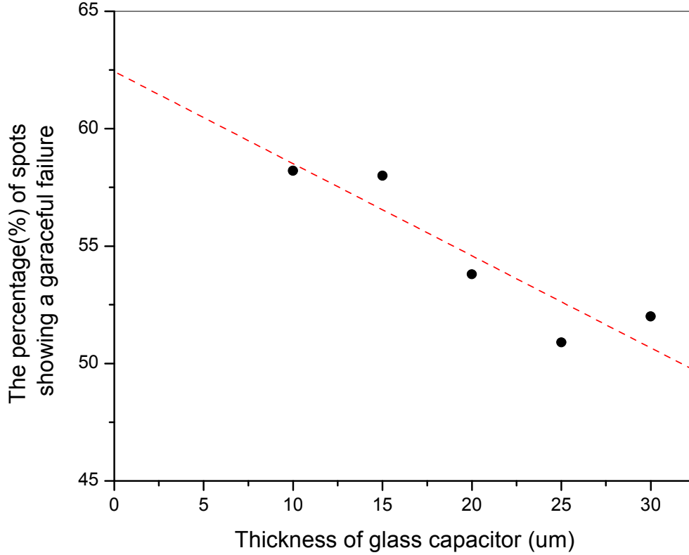
Fig. 4. Percentage (%) of spots showing graceful failure for thinned glass sheet
