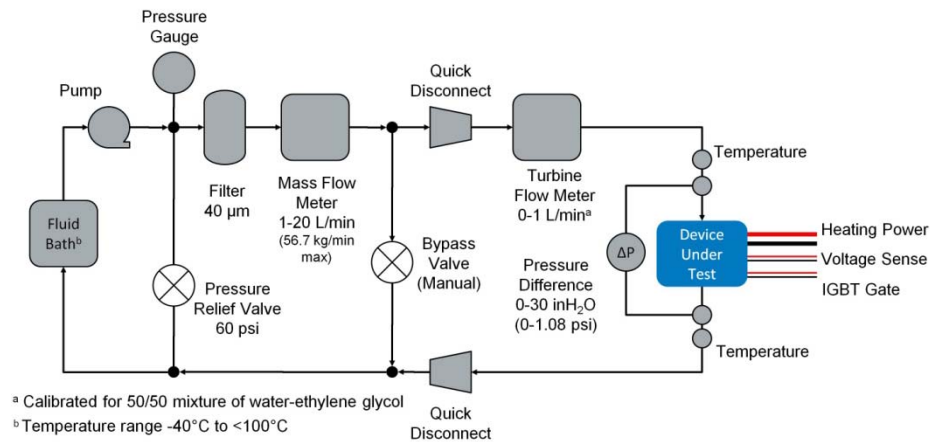
Fig. 36. Integrated power semiconductor and cooling technology thermal characterization hardware diagram
