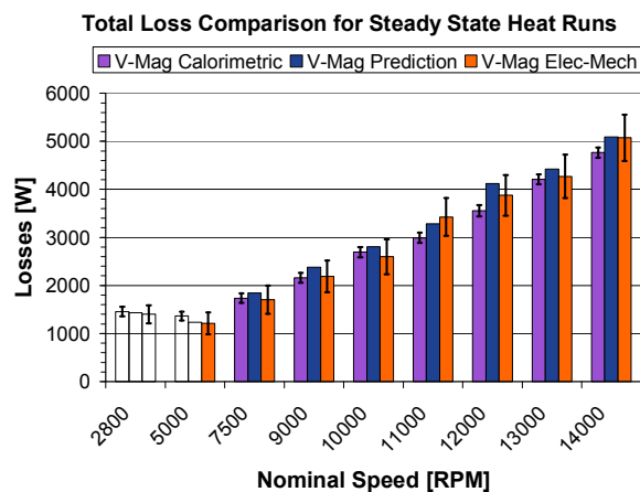
Fig. 14. Second proof-of-principle machine measured (electrical and calorimetric) vs. predicted losses at rated power
