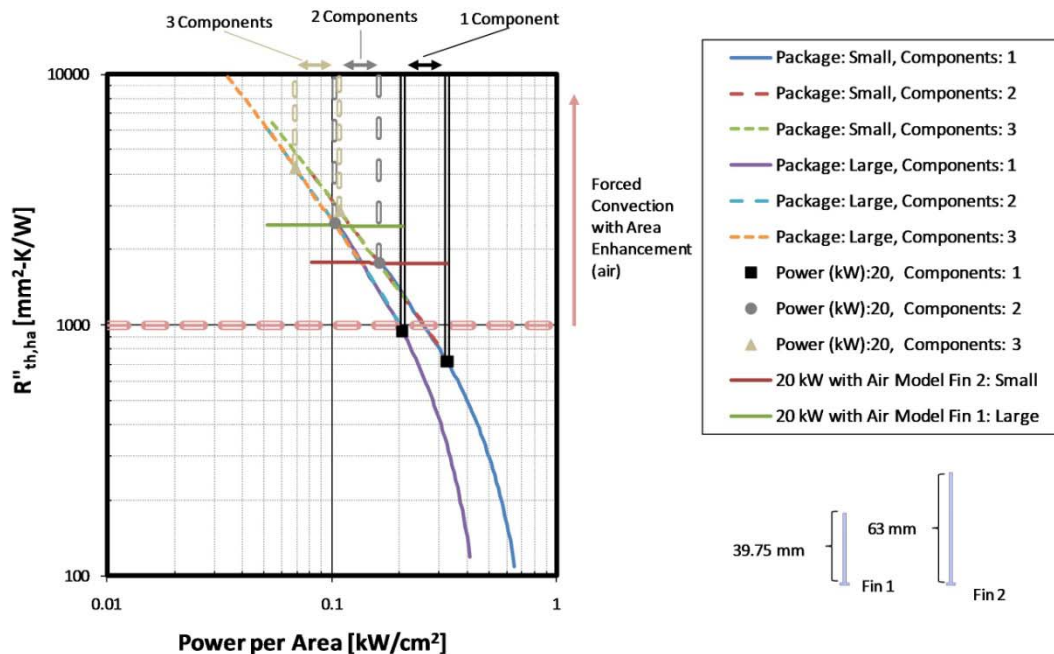
Fig. 51. Application technical specification linked to thermal design targets with air cooling
