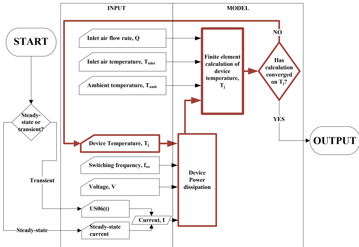
Fig. 1. Flowchart outlining junction temperature iterative procedure.
