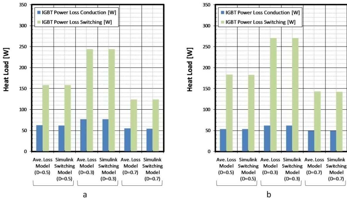
Fig. 49. Loss model comparison based on data sheet values from two IGBT modules operating at 20 kW with input voltage of 400 V, switching frequency of 10 kHz, and a range of duty cycles (D). (a) Semikron SKM 300GB128D; (b) Infineon FS450R12KE3.
