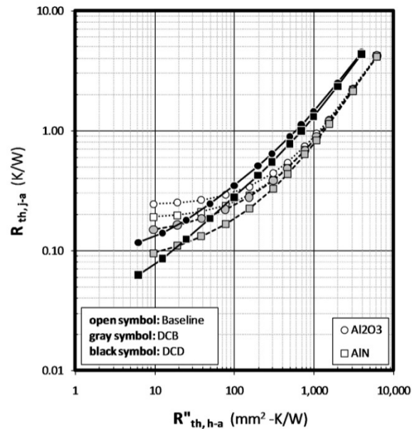
Fig. 32. Material impacts vs. package configuration based on the Semikron SKM package. DCB (direct-cooled baseplate) removes the TIM and aluminum heat exchanger. DCD (direct-cooled DBC) removes the TIM, aluminum heat sink, solder layer, and baseplate.
