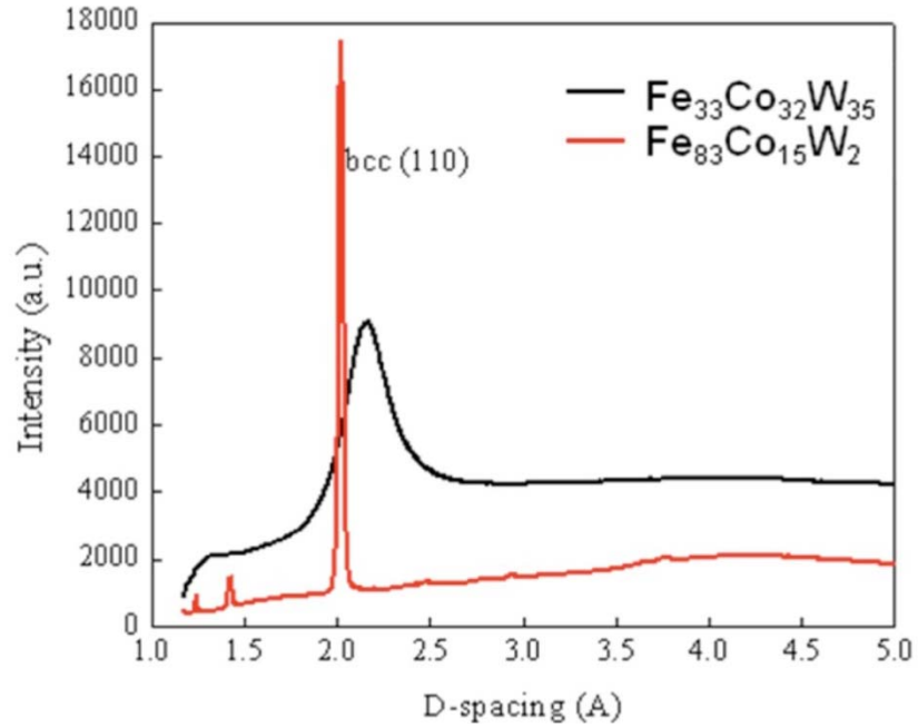
Fig. 14. Synchrotron diffraction results of selected compositions. Peak broadening at higher W concentration indicates that the material has not fully crystallized at the annealing temperature of 600 °C.
