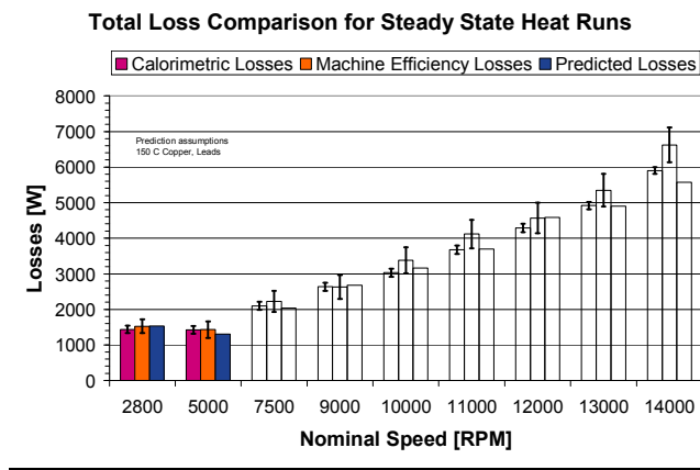
Fig.7. First proof-of-principle machine measured (electrical and calorimetric) vs. predicted losses at rated power
