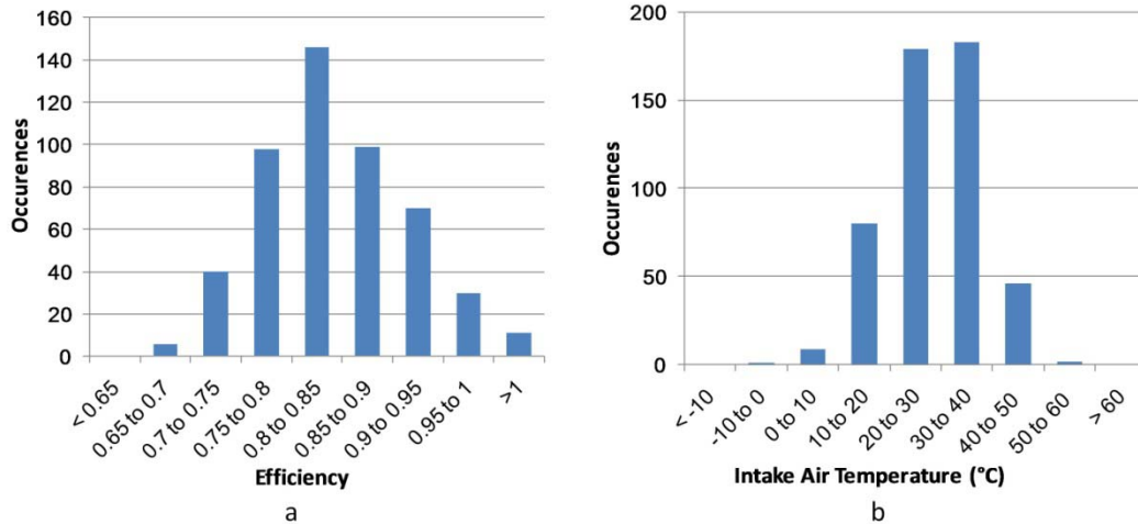
Fig. 44. INL charger analysis [5] (a) Efficiency, (b) Inlet air temperature
