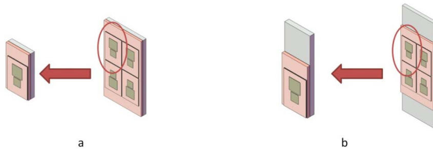
Fig. 47. Package geometry configurations. (a) Small heat sink area (15.34 cm 2 ); (b) Large or extended heat sink area (24.19 cm 2 ).
