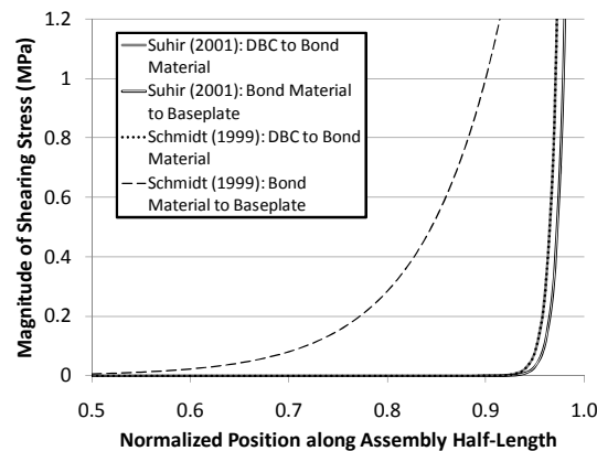
Fig. 4. Tri-material shear stress predicted using the Schmidt (1999) and Suhir (2001) models
