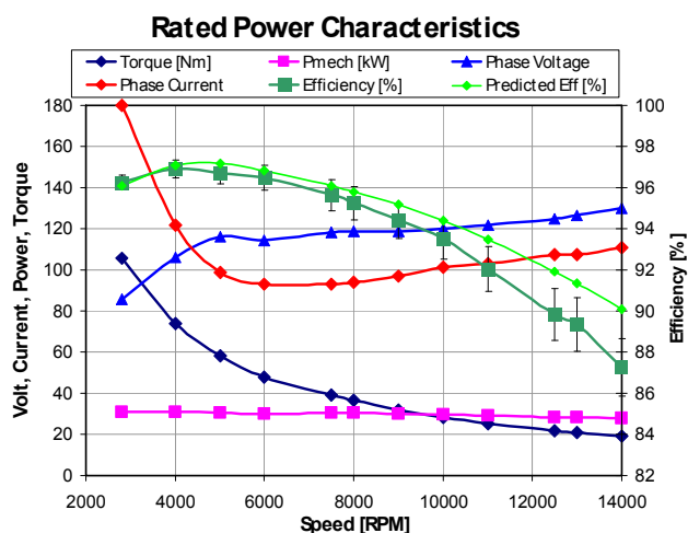
Fig. 12. Second proof-of-principle machine measured performance at rated power
