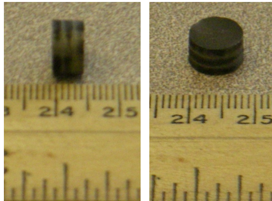
Fig.23. Optical image of a 3/8" multilayer pressed and sintered NdFeB magnet with three magnet layers (dark contrast) and two insulating layers (light contrast)
