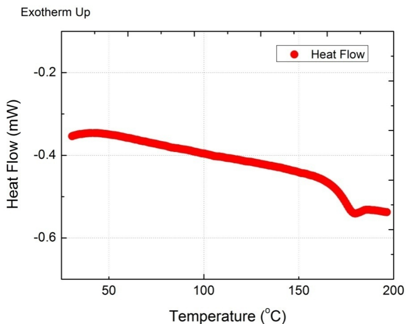
Fig. 6. DSC data on polymer 2 where n = 3m
