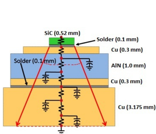
Fig. 7. Outline of electrothermal model for the SiC MOSFET in the Co-Pack Module
