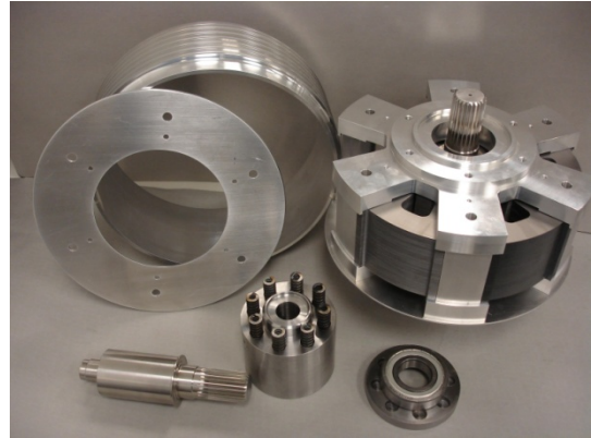
Fig. 14. First phase prototype.
