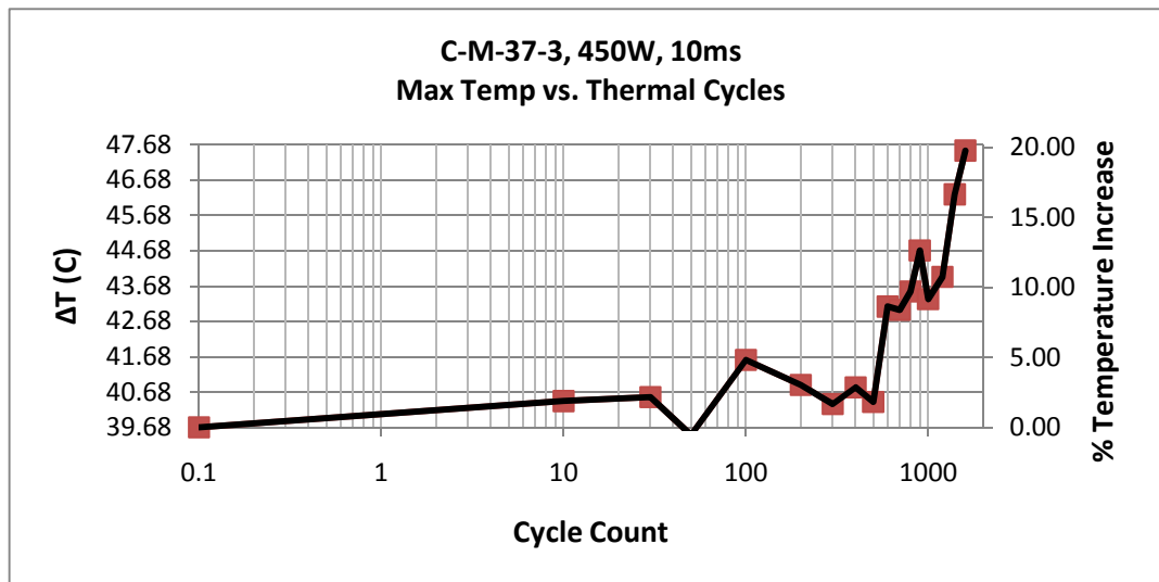
Fig. 9. Increase in \Delta T_j resulting from thermal cycle damage to the module
