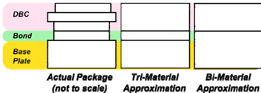
Fig. 2. Example bonded joint and depiction of a tri-material and bi-material approximation
