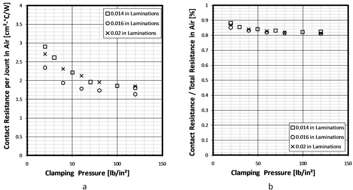
Fig. 27. Thermal contact resistance across laminations, extracted from [6]: (a) Thermal contact resistance per joint for stacked laminations; (b) Ratio of total lamination stack resistance due to contact resistance.
