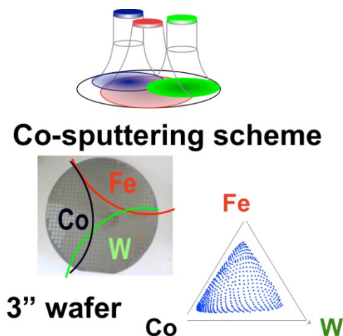
Fig. 10. Schematic of combinatorial synthesis experiment to generate composition field of Co-Fe-W.
