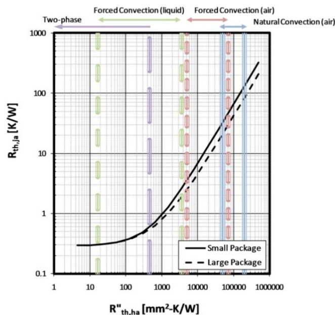
Fig. 48. Package mechanical design thermal performance. Cooling bands based on convection coefficients from Mudawar [4].
