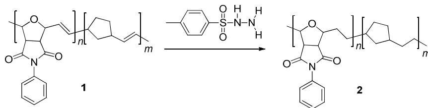
Fig. 5. Hydrogenation of a model polymer dielectric
