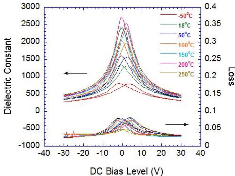
Fig. 1. Dielectric properties of a \approx 1.15\text{-}\mu\text{m} -thick PLZT/LNO/Ni film-on-foil measured as a function of applied bias voltage at various temperatures.
