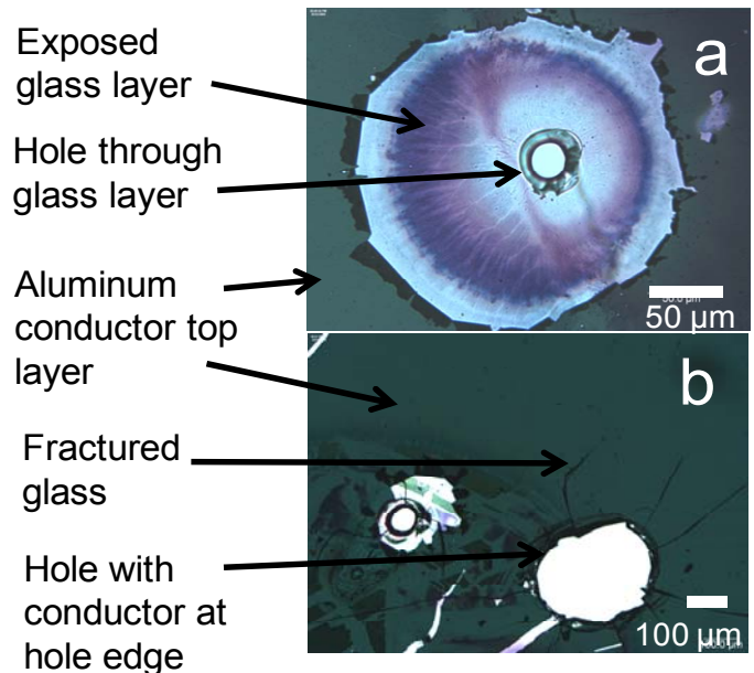
Fig. 3. (a) Self-healing and (b) catastrophic dielectric failure modes in a 15 \mu\text{m} thick glass layer with evaporated 10 nm thick aluminum electrodes. Figure 3a shows a classic self-healing mode with a significant clearing of the electrode away from the glass and very little damage to the glass. Note that the hole has a ring of glass that has melted during the breakdown event. Figure 3b illustrates extended fracture due to thermal shock and the electrodes cover the entire glass layer except for the hole created by breakdown. Note a significant cracking in the lower left hole for Figure 3b.
