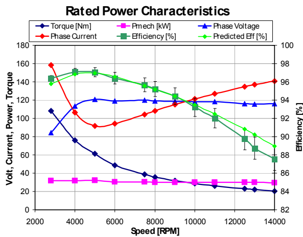
Fig. 5. First proof-of-principle machine measured performance at rated power
