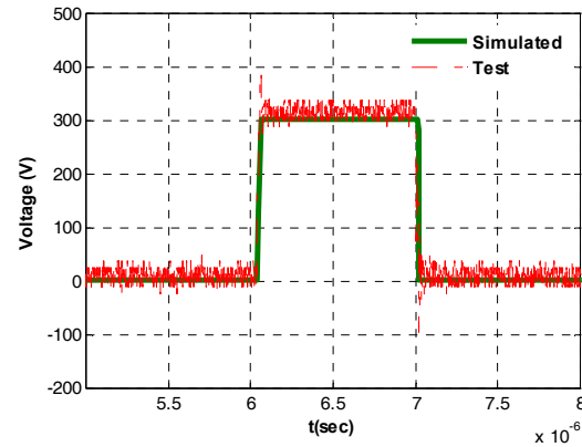
Fig. 30. Comparison of voltage waveforms of the JFET.
