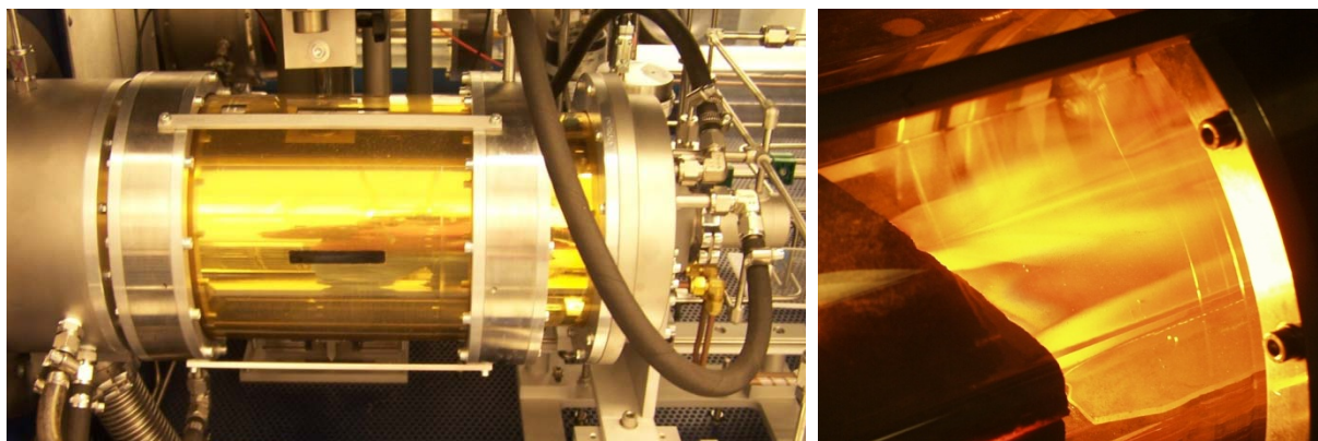
Fig. 5. (Left)NASA GRC horizontal cold-wall SiC growth reactor as installed by manufacturer. (Right) Operation of NASA GRC cold-wall SiC reactor in “pseudo-hot-wall” configuration.
