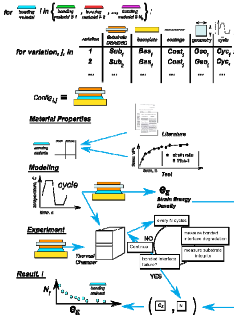
Fig. 6. Procedure to determine the relationship between strain energy density and cycles to failure
