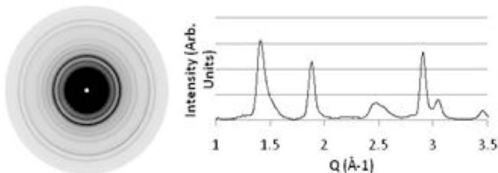
Fig. 3. XRD pattern of an amorphous ribbon that was crystallized during vacuum hot pressing.
