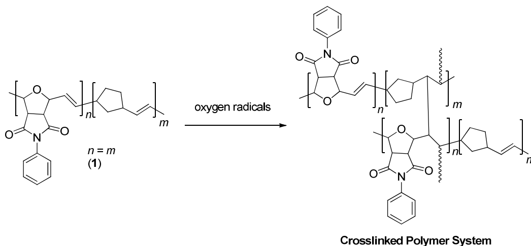
Fig. 3. Crosslinking reaction that results in polymer precipitation from casting solutions
