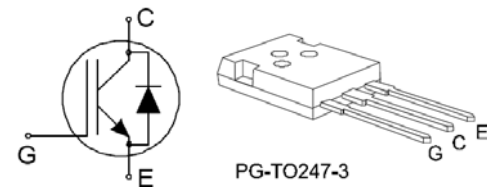
Fig. 9. IKW40N120H3-Si IGBT with antiparallel diode.
