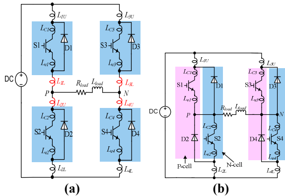
Fig. 5. (a) Conventional full bridge inverter; (b) phase leg constructed by P-cell and N-cell.
