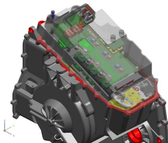
Integrated Electric Traction System
