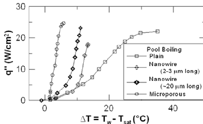
Fig. 23. Pool boiling curves
