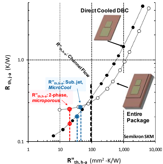
Fig. 26. Total thermal resistance as a function of the inverse of the convective coefficient.
