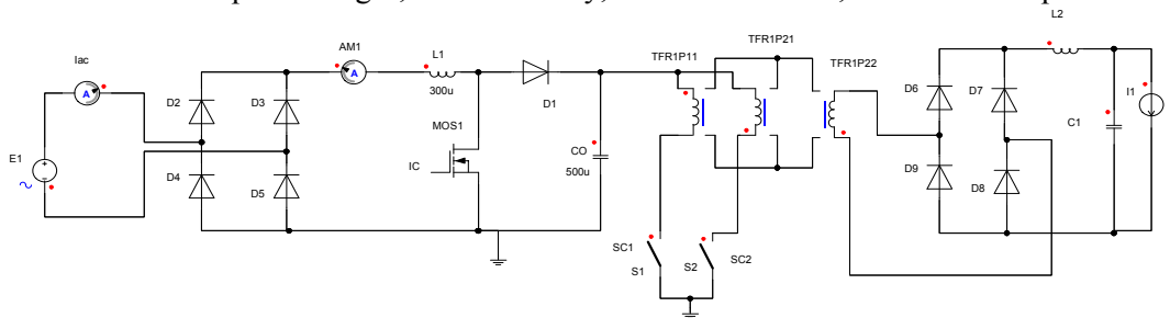
Fig. 1. Industry Current Approach Two Stages Isolated Unity Power Factor Battery Charger
