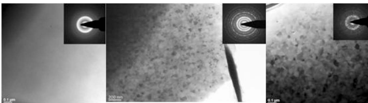
Fig. 4. TEM bright field images with corresponding electron diffraction patterns of (left) NO-121-B (as-spun), (middle) NO-121-B-2 (580°C/60min., 110MPa), and (right) NO-121-B-3 (580°C/60min., no applied pressure).
