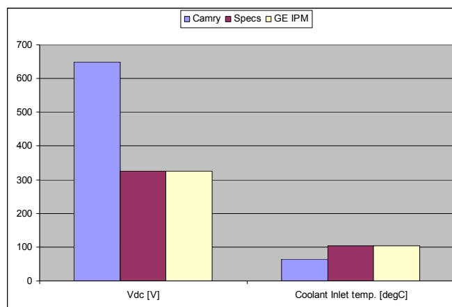
Fig.17. Comparisons of DC bus voltage and coolant inlet temperature
