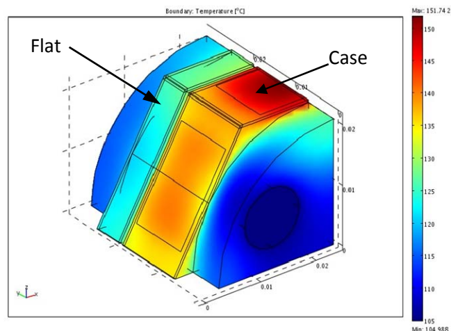
Fig. 4. FEA output for four-hole design.
