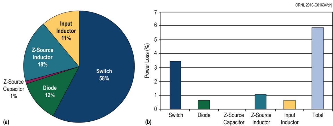
Fig. 15. Buck mode loss breakdown by component for the 55 kW CF-trans-qZSI design: (a) component loss as a percent of the whole; (b) individual component power loss.
