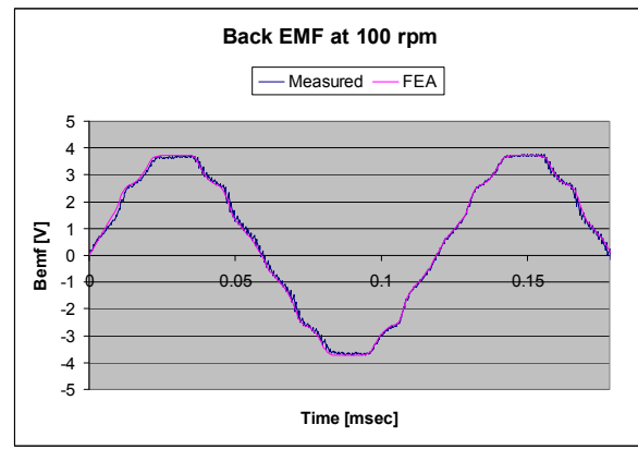
Fig. 4. Predicted vs. measured back emf of the first proof-of-principle machine at 100 rpm.
