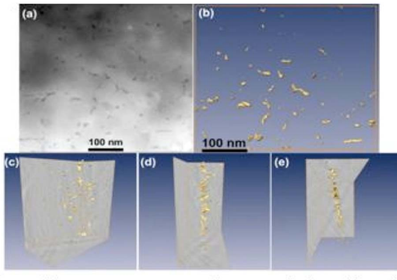
Fig. 6. (a) STEM HAADF image of the alloy (TiC particles in darker contrast) and corresponding ET 3-D reconstructed volume shown in (b) z-axis, (c) random, (d) x-axis, and (e) y-axis. The shape and morphology of the TiC particles are illustrated in yellow by using the iso-surface method.
