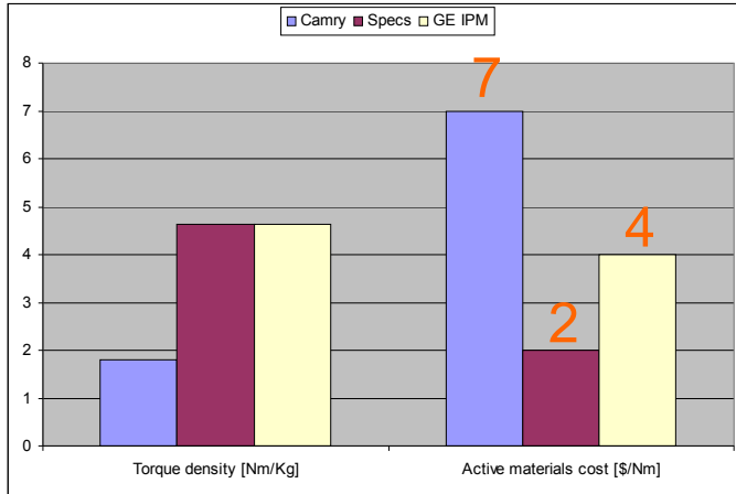
Fig.18. Comparisons of torque density and active material cost
