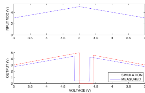
Fig. 10. UVLO detecting an undervoltage at 200°C on the 5 V rail.
