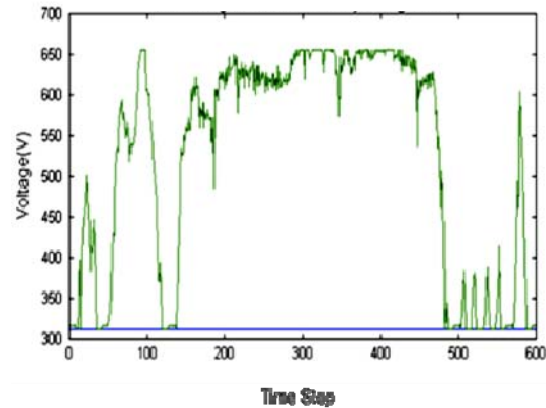
Fig. 22. Bus voltage (green) and battery voltage (blue).
