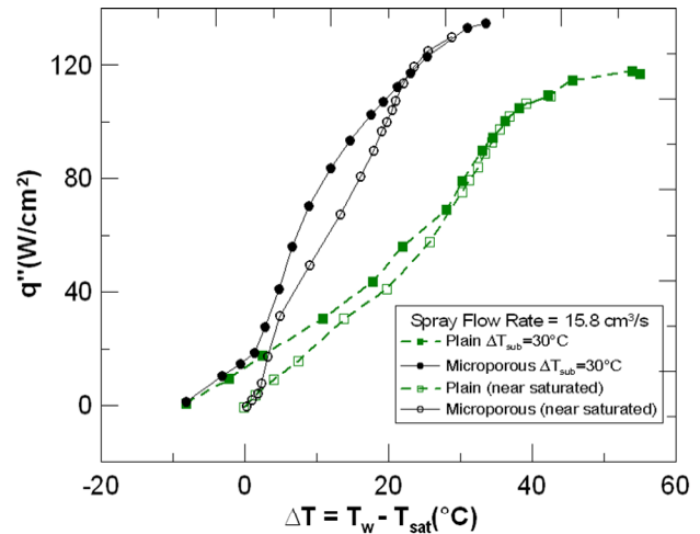
Fig. 24. Spray boiling curves for both near-saturated and subcooled conditions
