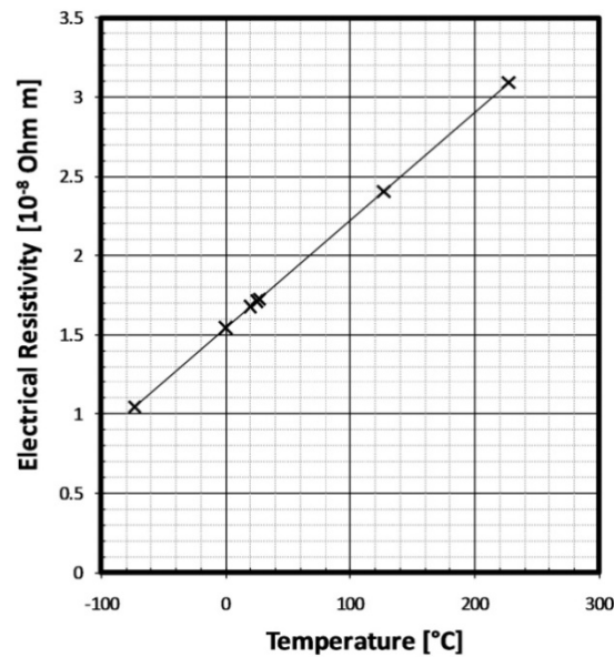
Fig. 28. Electric resistivity vs. temperature for pure copper [13]
