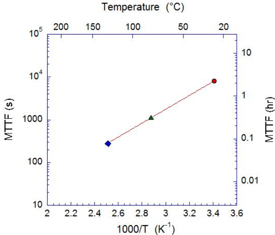
Fig. 9. Mean time to failure as a function of temperature for \approx 1.15\text{-}\mu\text{m} -thick PLZT/LNO/Ni film-on-foils measured with 120 V applied voltage.
