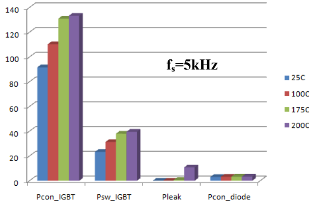
Fig. 17. Power losses in one phase leg at different temperatures ( f_s=5\text{kHz} ).
