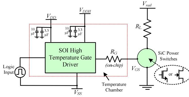
Fig. 4. Schematic of test setup for MOSFET ( V_{DDH} = 15 V, V_{SS} = -5 V) and for normally ON JFET module ( V_{DDH} = 3 V, V_{SS} = -5 V).
