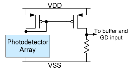
Fig. 20. Photodetector configuration.
