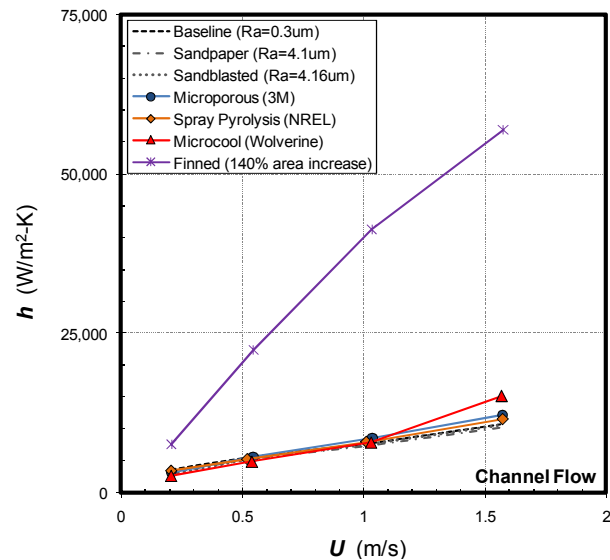
Fig. 20. Heat transfer coefficients versus fluid velocity for the various surfaces in the channel flow configuration
