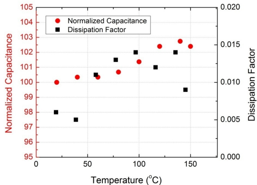
Fig. 11. Electrical Characterization of discrete Al based stacked capacitors.
