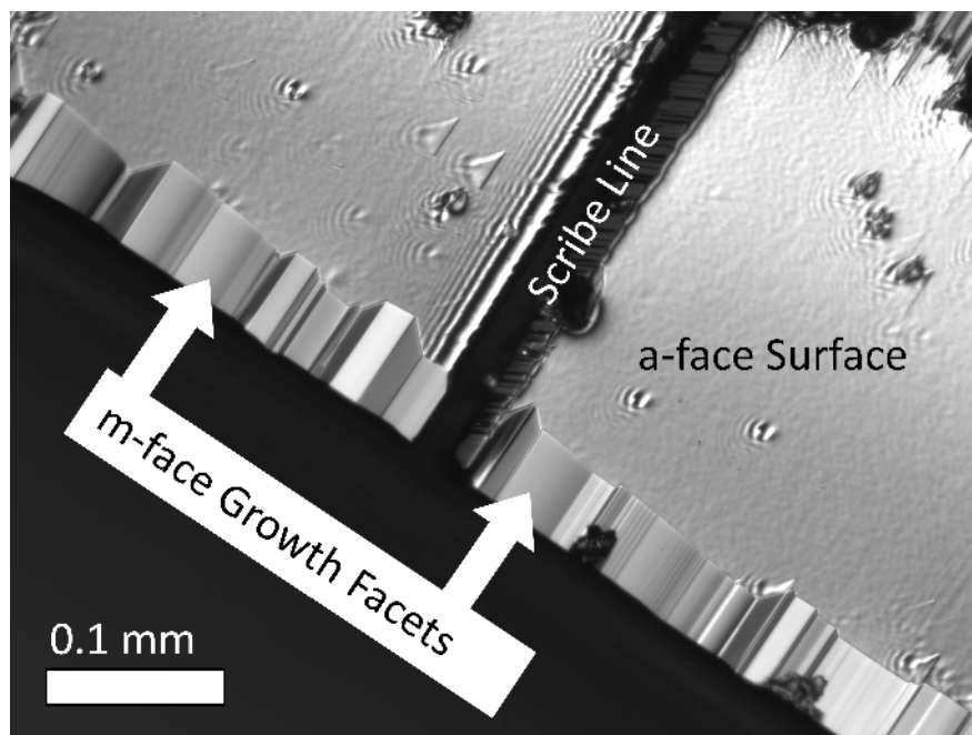
Fig. 7 Optical micrograph of portion of 6H-SiC pseudo-fiber following 1 hour of growth in NASA Glenn modified hot-wall SiC reactor.
