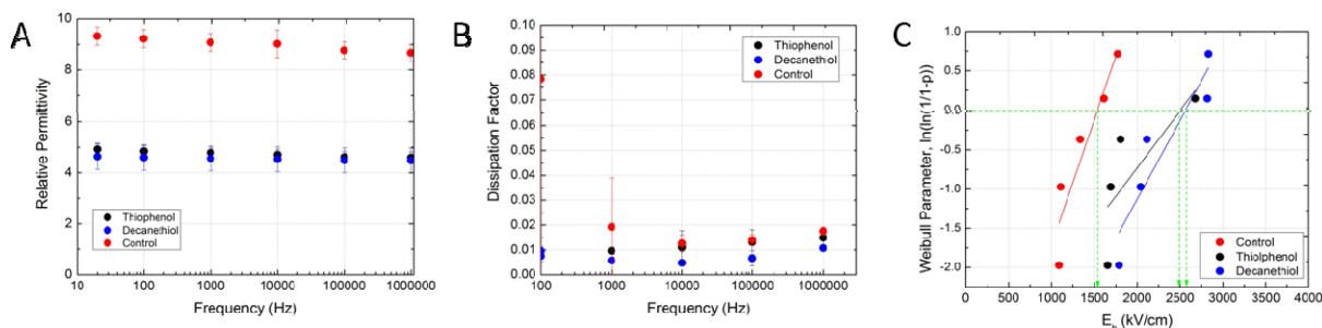
Fig. 14. Electrical characterization of polymer modified using the thiol-ene reaction A) Relative permittivity B) Dissipation factor and C) Dielectric breakdown
