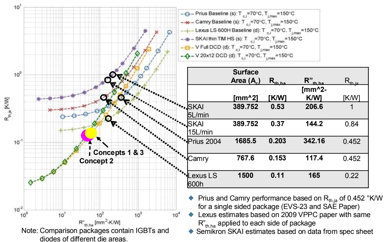
Fig. 5. Comparisons of Delphi's thermal performance concepts 1,2 and 3 vs. commercially available products
