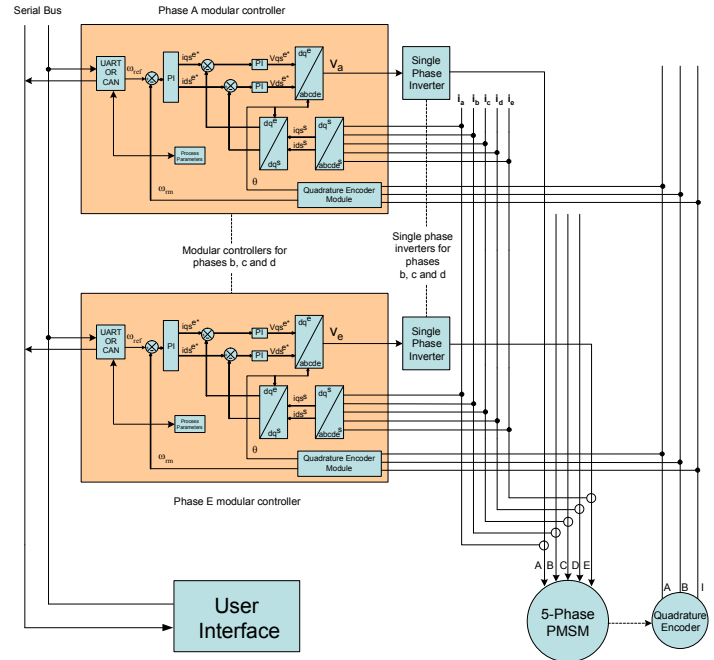
Fig. 8. Heterarchical controller implementation for field-oriented control of a 5 phase IMMD.
