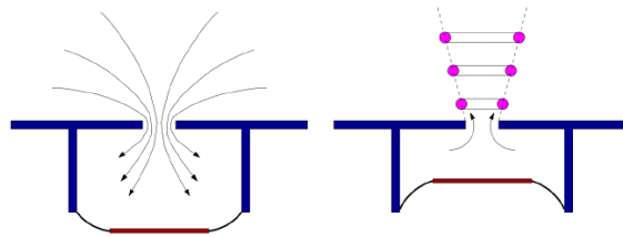
Fig. 7. Schematic of synthetic jet operation displaying the suction and ejection strokes [2]
