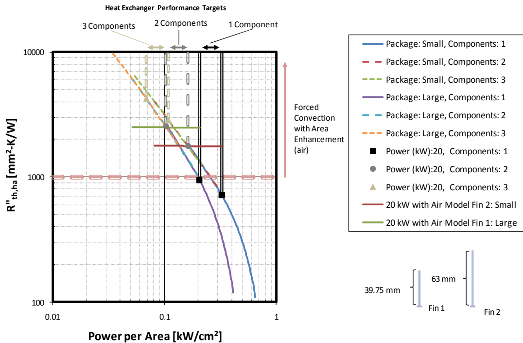
Fig. 6. Example system analysis, air-cooled 20 kW DC-DC converter for vehicle charging application
