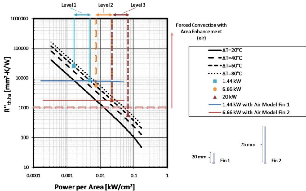
Fig. 46. Application technical specification linked to thermal design targets with air cooling range with area enhancement
