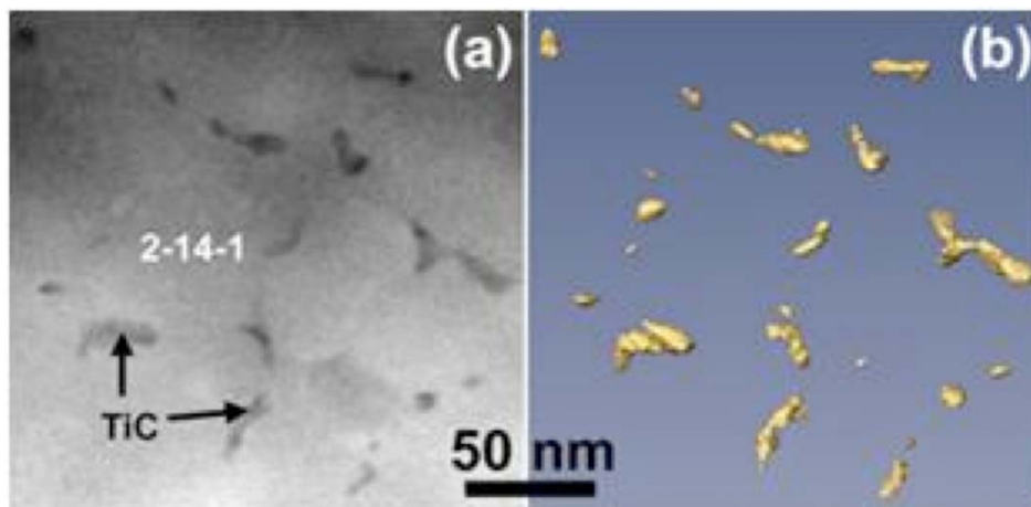
Fig. 7. (a) STEM HAADF image and (b) corresponding ET 3-D reconstructed volume, where the TiC particles are represented by the iso-surface.
