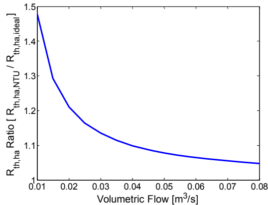
Fig. 15. Heat exchanger to air thermal resistance ratio, R_{th,ha,NTU}/R_{th,ha,ideal}
