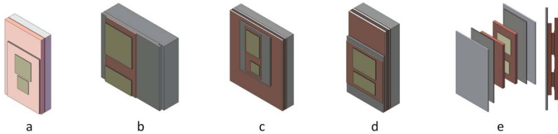
Fig. 29. Alternative package configurations for package thermal performance comparison. Configuration geometries are based on existing commercial packages: (a) Semikron SKM, (b) Semikron SKAI, (c) 2004 Prius, (d) 2007 Camry, (e) 2008 Lexus LS 600H.
