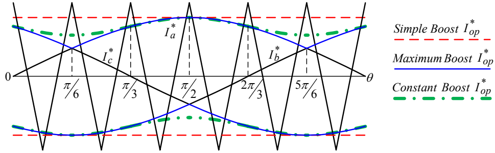
Fig. 7. Pulse width modulated control methods using three different open circuit–zero state references.
