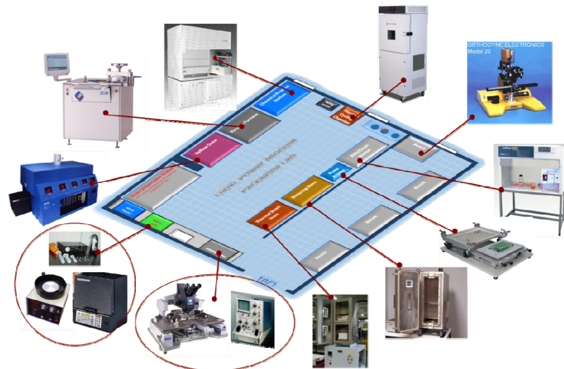
Fig. 9. Power module packaging process facilities and layout in a specially built laboratory.
