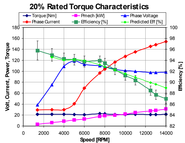
Fig. 6. First proof-of-principle machine measured performance at 20% rated torque
