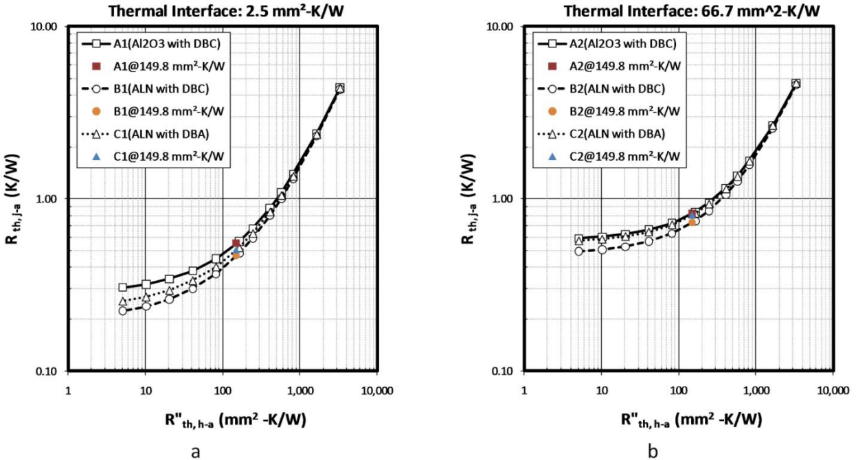
Fig. 35. Total thermal resistance thermal performance characterization of modified annulus package design: (a) Low thermal interface resistance, (b) High thermal interface resistance
