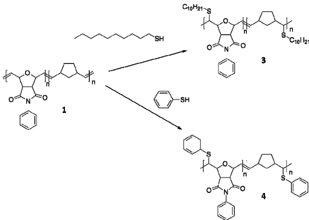
Fig. 13. Thiol-ene reactions in order to decrease reactive double bond content
