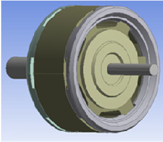
Fig. 3. Rotor of prototype motor.
