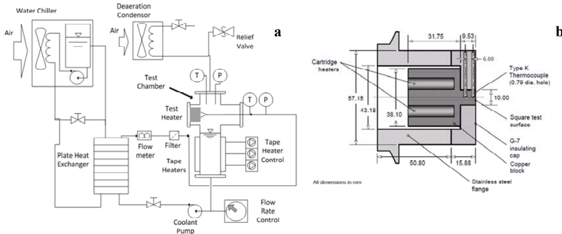
Fig. 22. Schematic of the two-phase flow loop (left) and heater (right)
