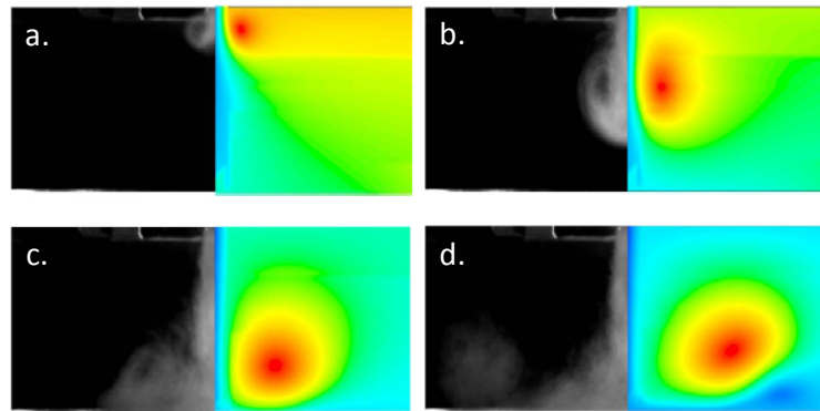
Fig. 11. Comparison between experiment and numerical modeling for an impinging jet
