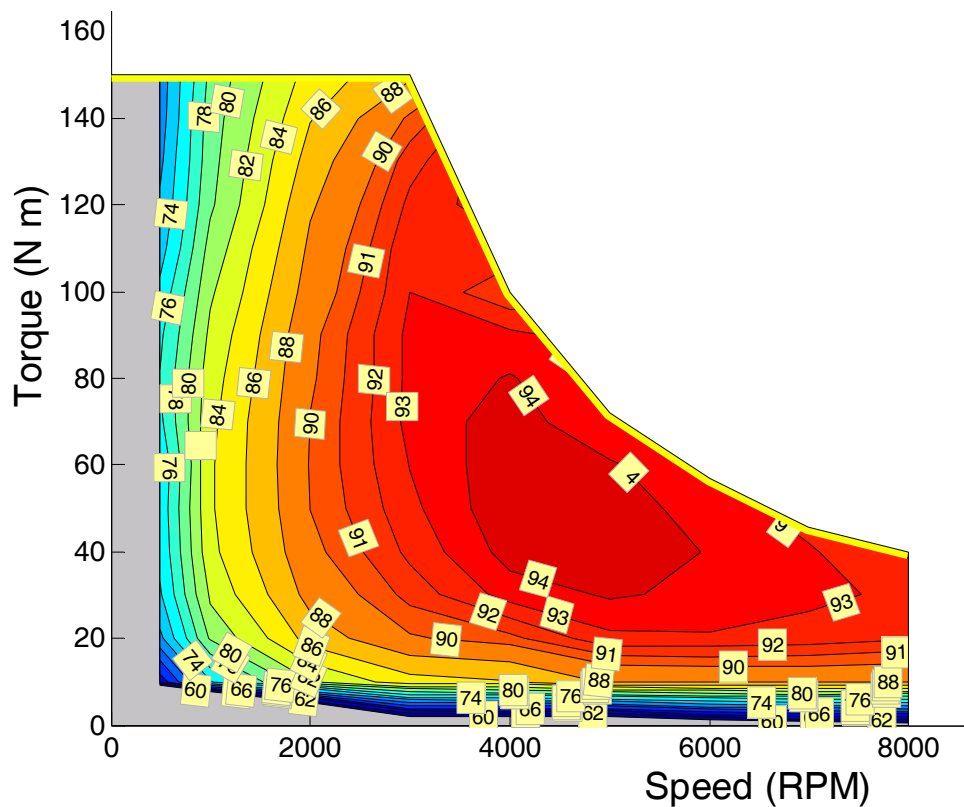
Fig. 13. 2010 Prius combined motor-inverter efficiency map for 500 Vdc.
