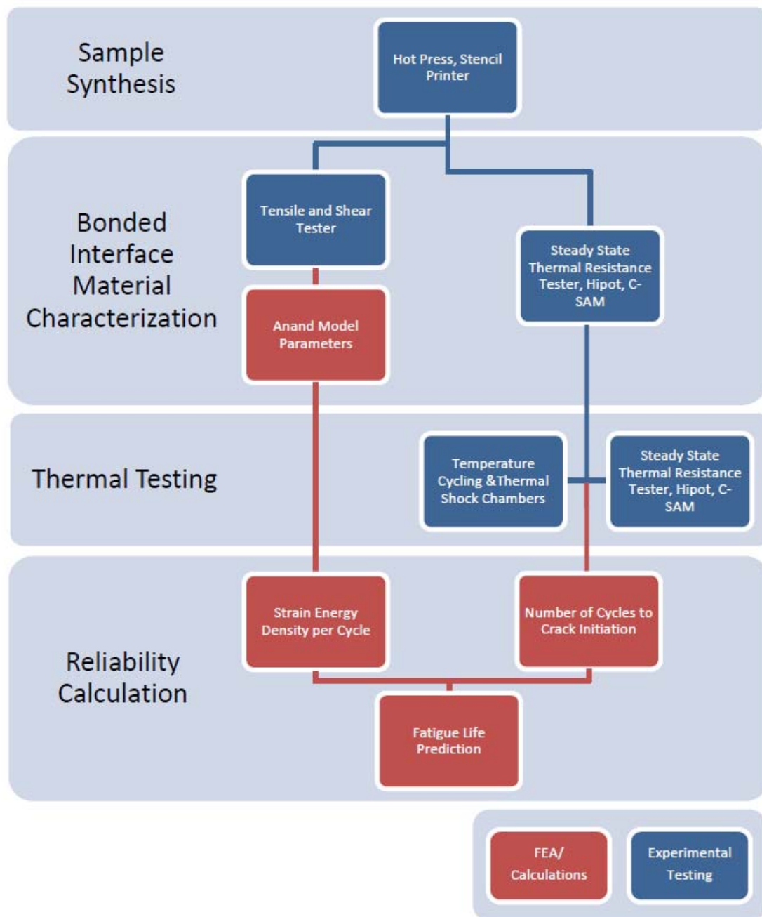
Fig. 58. Flowchart of bonded interface thermal reliability testing procedure
