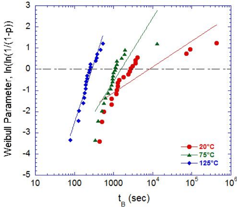
Fig. 8. Weibull plot of time to breakdown for \approx 1.15\text{-}\mu\text{m} PLZT/LNO/Ni film-on-foils measured at 20^\circ\text{C} , 75^\circ\text{C} , and 125^\circ\text{C} with 120 V applied voltage.
