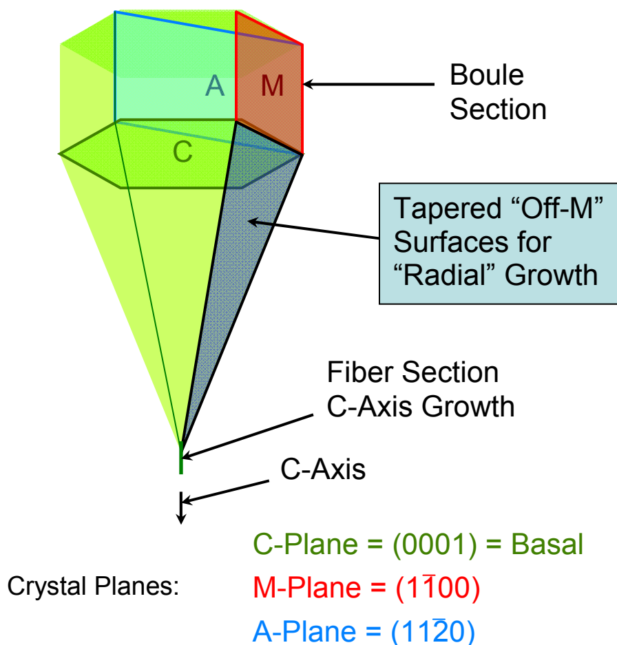
Figure 4. Boule shape and crystal planes pertinent to LTC radial growth process.
