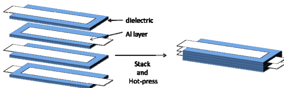
Fig. 9. Scheme for fabrication of larger value capacitors
