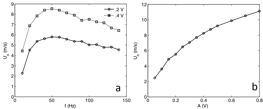
Fig. 13. Average velocity at the orifice as a function of actuator driving a. frequency b. amplitude
