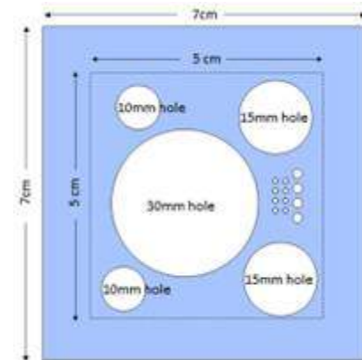
Fig. 2. Mask set to allow larger for area capacitors
