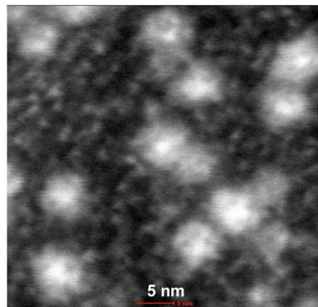
Fig. 16. High resolution STEM micrograph of as-deposited Co-W nano-particulate from cluster deposition experiments.
