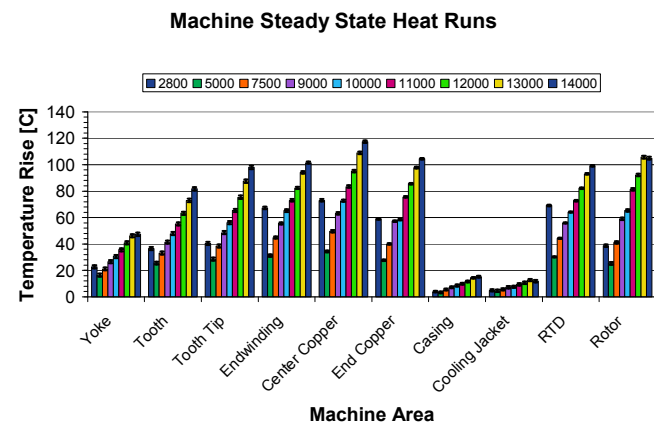
Fig.8. First proof-of-principle machine heat runs temperature rises in the various machine components at various speeds.
