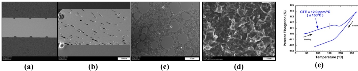
Fig. 4. Honda Insight (Mitsubishi TPM) microstructure: (a) dimple in heat spreader, (b) voids in solder layer, (c) molding component, (d) TCIL, and (e) thermal expansion of molding
