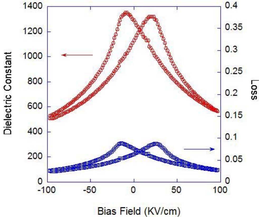
Fig. 6. Dielectric properties of a 20-mm-diameter, \approx 3\text{-}\mu\text{m} -thick PLZT/LNO/Ni film-on-foil measured at room temperature as a function of bias field.
