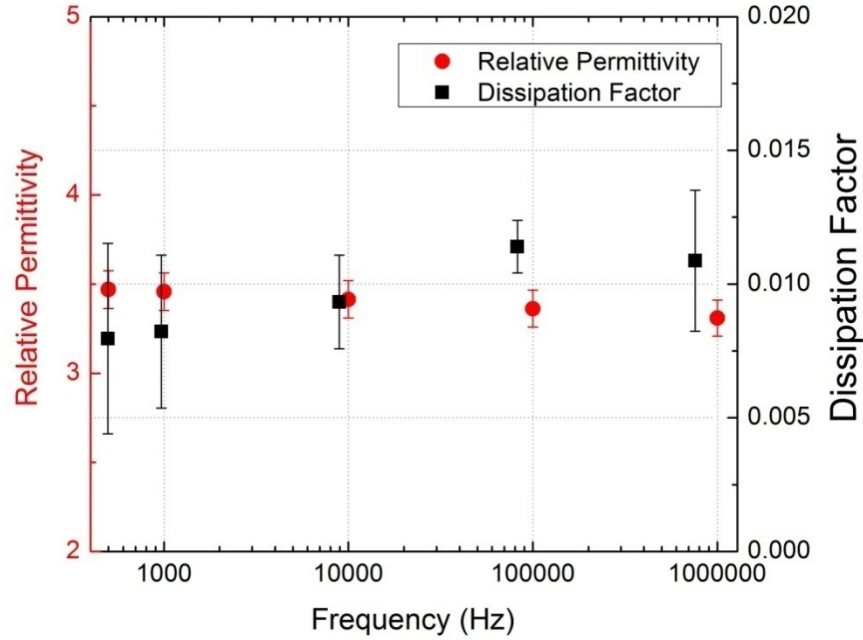
Fig. 7. Dielectric properties as a function of frequency
