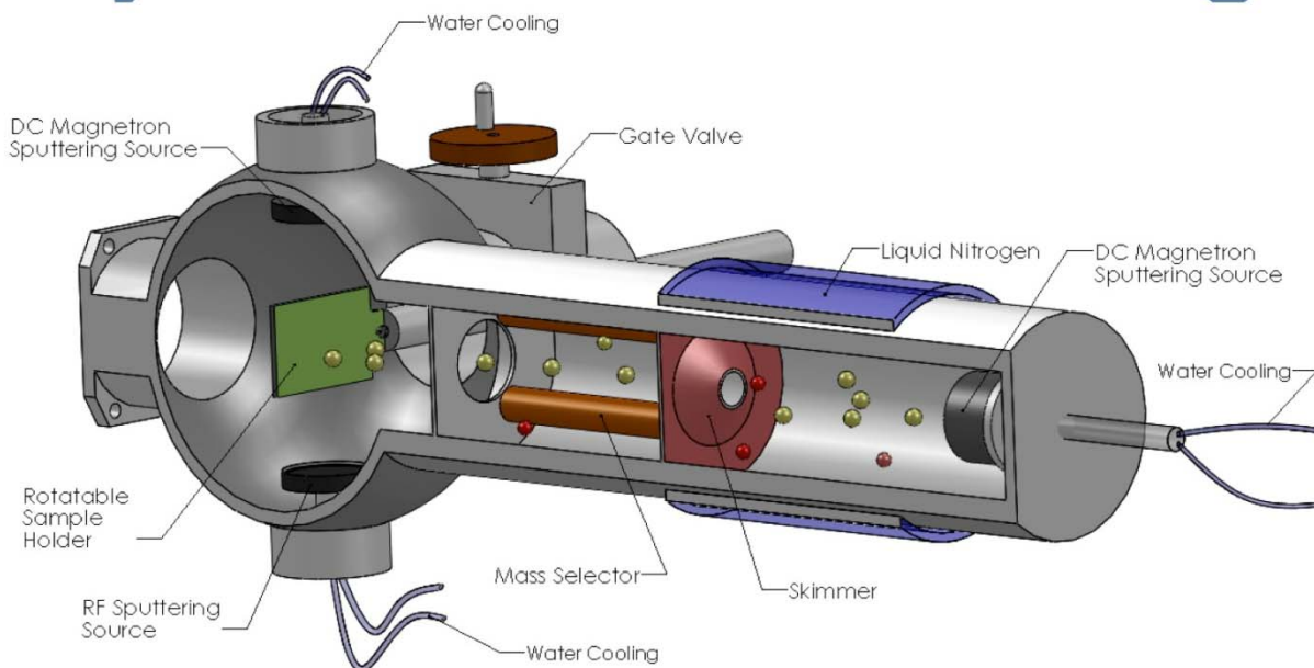
Fig. 11. Schematic of cluster deposition system for producing nano-particulate of magnet alloys.
