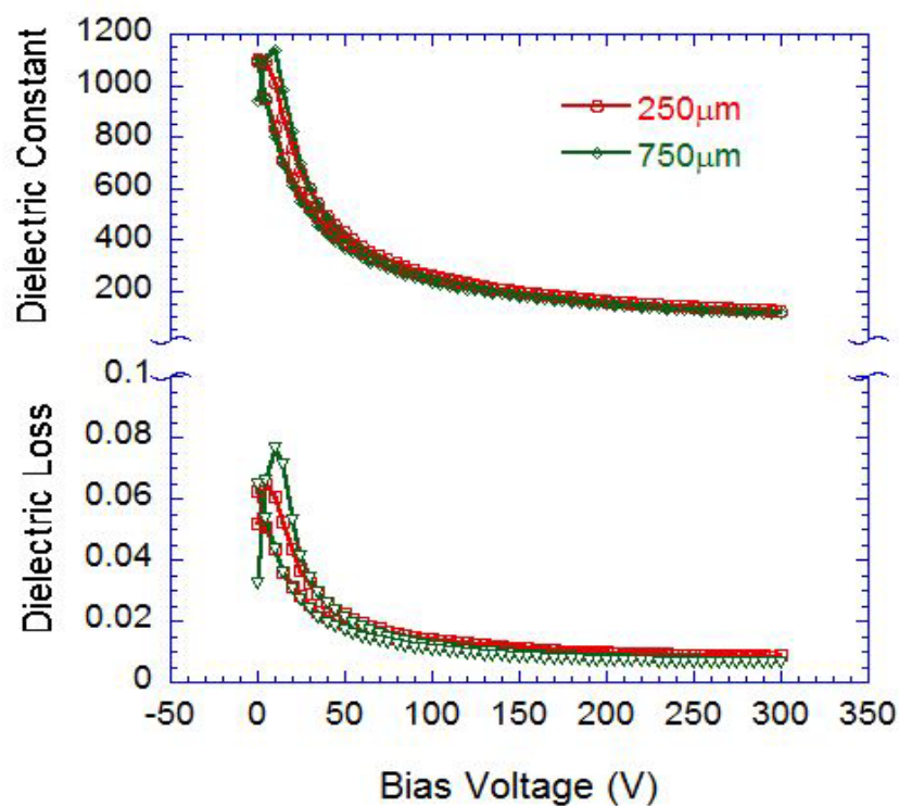
Fig. 4. Dielectric properties as a function of bias voltage measured on a \sim 3\text{-}\mu\text{m} -thick PLZT/LNO/Ni film-on-foil at room temperature.
