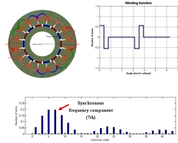
Fig. 2. Four phase (4P) machine: 16 slots/14 poles.
