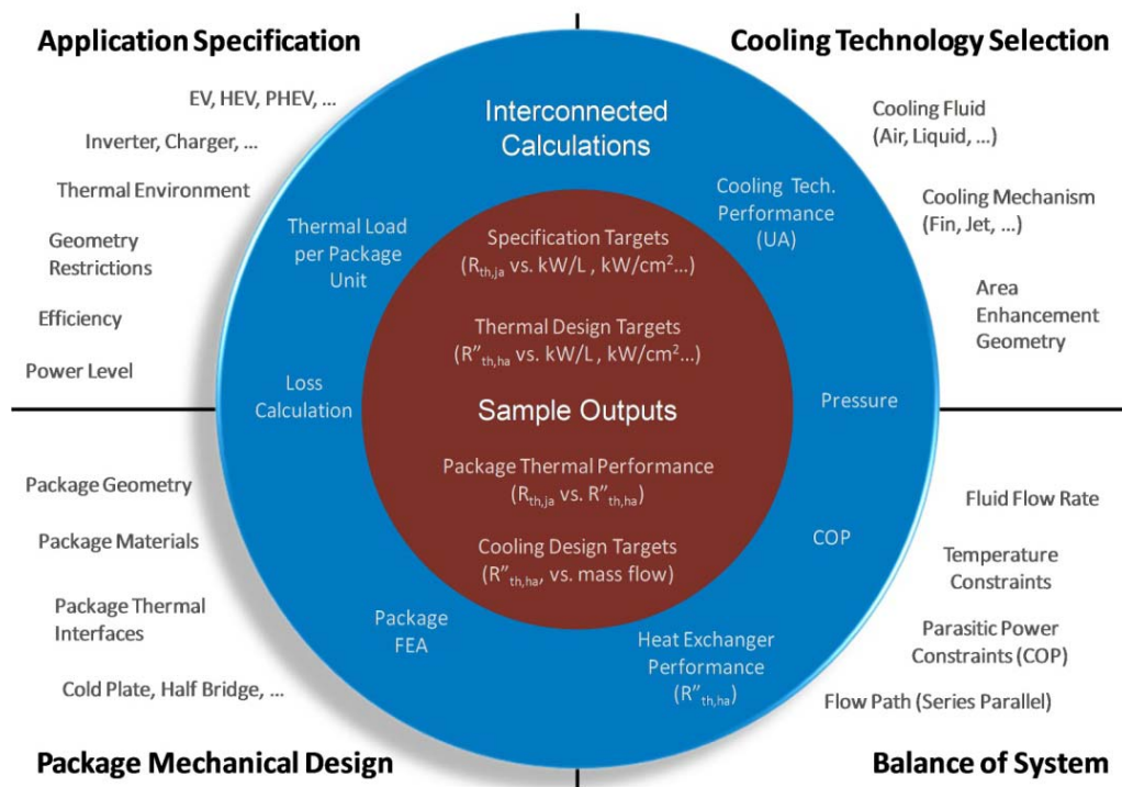
Fig. 5. Power electronics system analysis parameter overview
