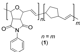
Fig. 1. Structure of the high temperature polymer dielectric polymer
