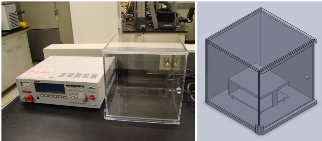
Fig. 56. Dielectric resistance tester.
