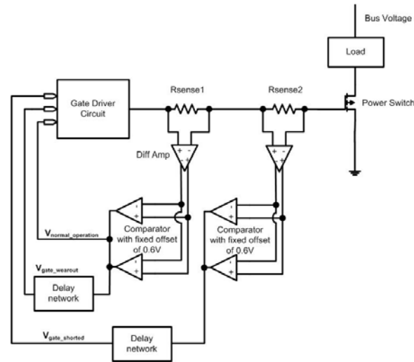
Fig. 27. Gate current monitoring.
