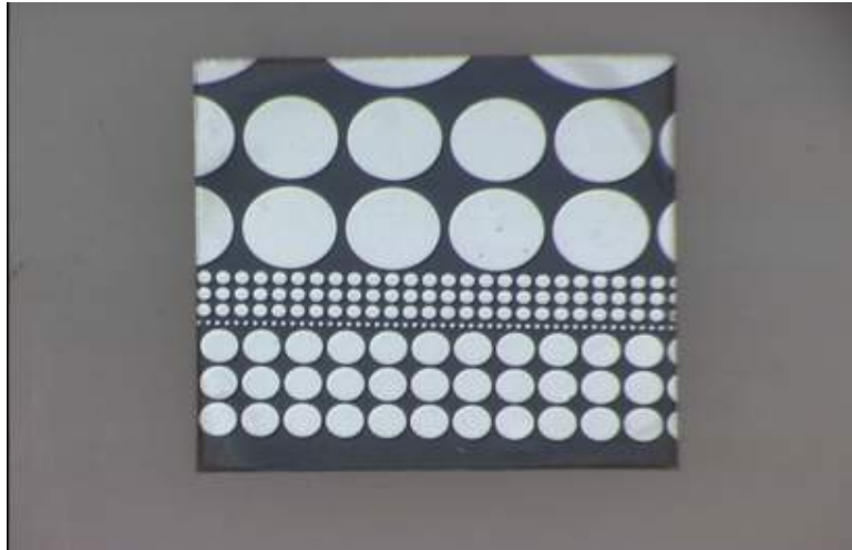
Fig. 1. Capacitors made at Purdue on metalized Si substrate
