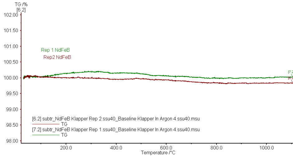
Fig. 21. Thermogravimetric analysis (TGA) on \text{Nd}_{15}\text{Fe}_{77}\text{B}_8 powder heated at 10 °C/min under gettered Argon.
