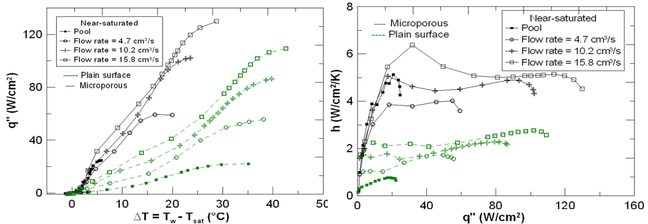
Fig. 25. Spray boiling curves (left) and heat transfer coefficients (right) for plain and microporous surfaces
