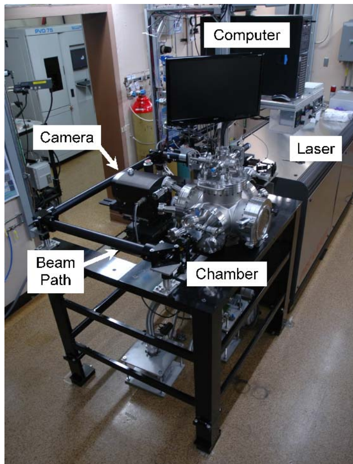
Fig. 3. Solvent-LHFZ system featuring growth chamber, high power CO 2 laser, beam path, long range optical microscope camera, and automation/data collection computer.
