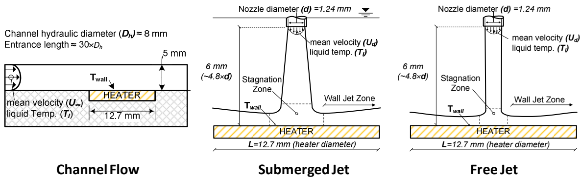
Fig. 19. Schematics, with relevant test parameter dimensions, for channel flow, submerged jet, and free jet experimental setups
