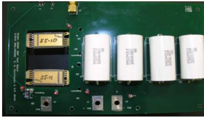
Fig. 3. Power Board used for Testing
