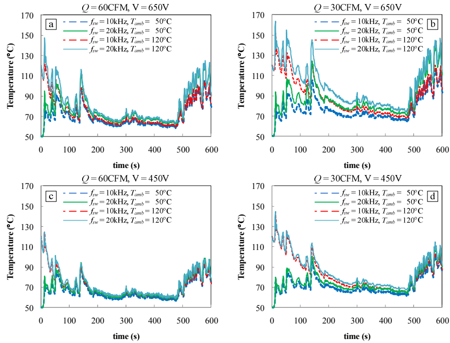
Fig. 4. Results of all 16 transient simulations of the US06 drive cycles for design A.
