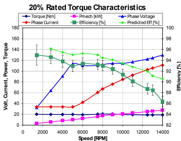
Fig. 13. Second proof-of-principle machine measured performance at 20% rated torque
