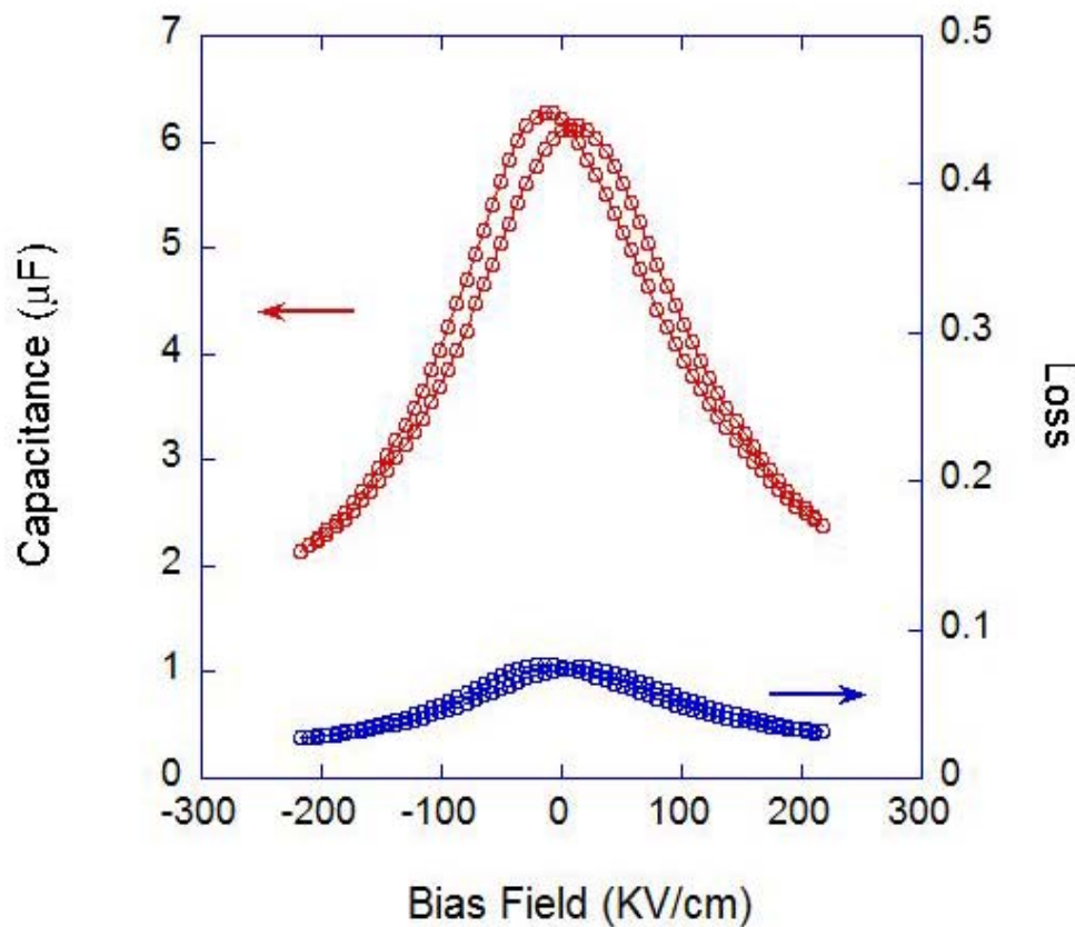
Fig. 5. Dielectric properties of a \approx 0.7\text{-}\mu\text{m} -thick PLZT on Pt/Si substrate measured at room temperature on a \approx 20\text{-mm} -diameter top electrode.
