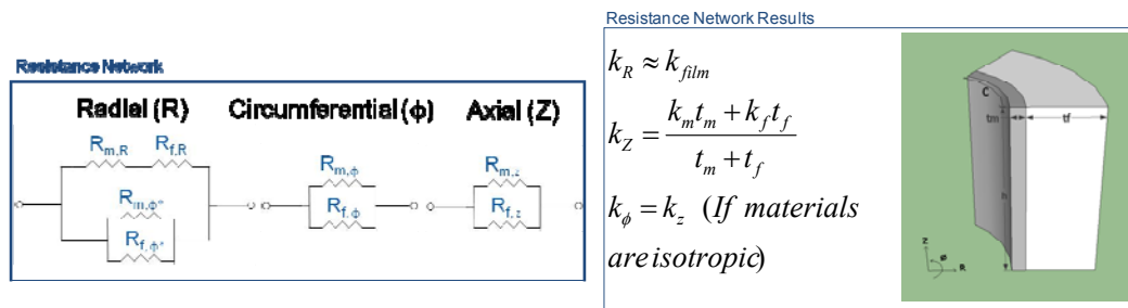
Fig. 38. Resistance network and resulting equations
